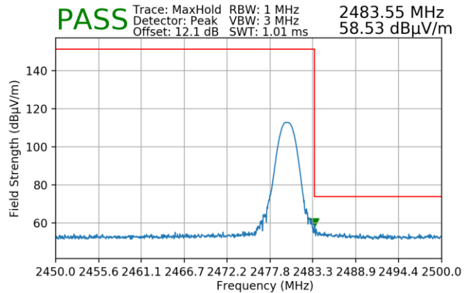
Plot 7-180. Radiated Restricted Upper Band Edge Measurement (Peak) – ANT1– WPT
