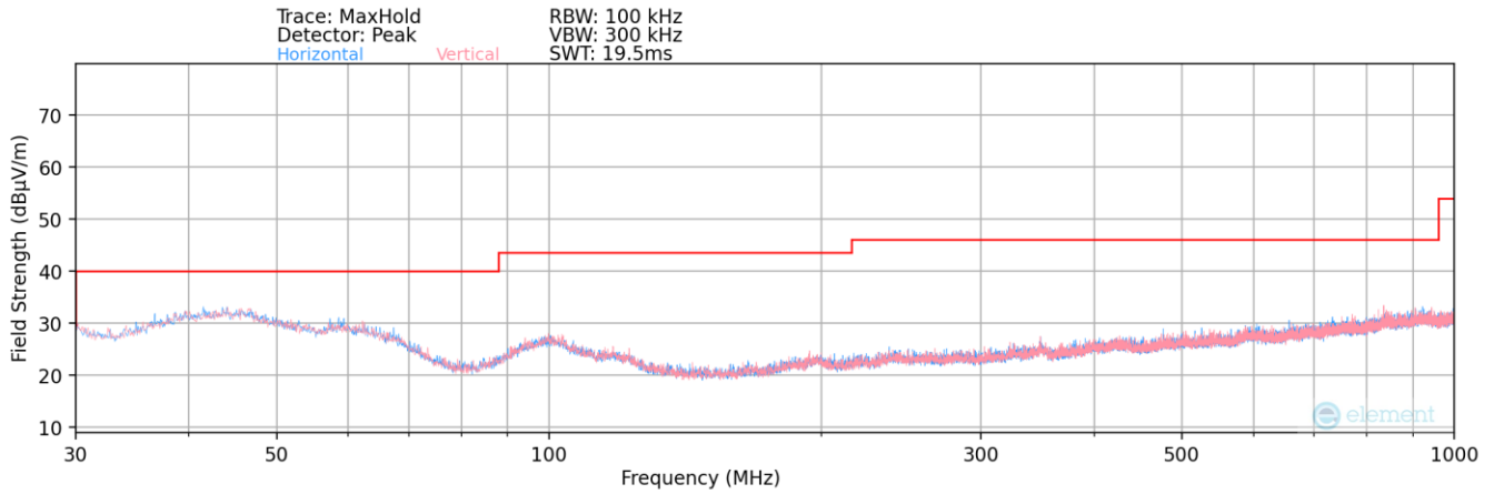
Plot 7-185. Radiated Spurious Plot below 1GHz
