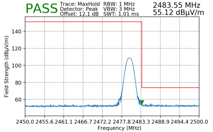
Plot 7-184. Radiated Restricted Upper Band Edge Measurement (Peak) – Dual
