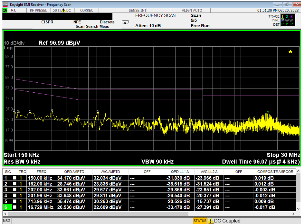
Plot 7-189. Line-Conducted Test Plot (N) – WPT
