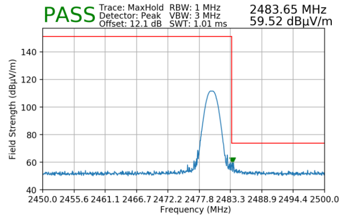
Plot 7-182. Radiated Restricted Upper Band Edge Measurement (Peak) – ANT2
