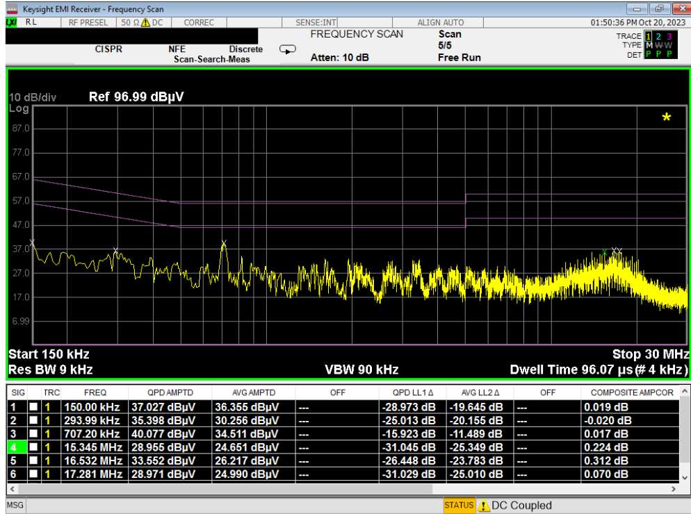
Plot 7-188. Line-Conducted Test Plot (L1) – WPT
