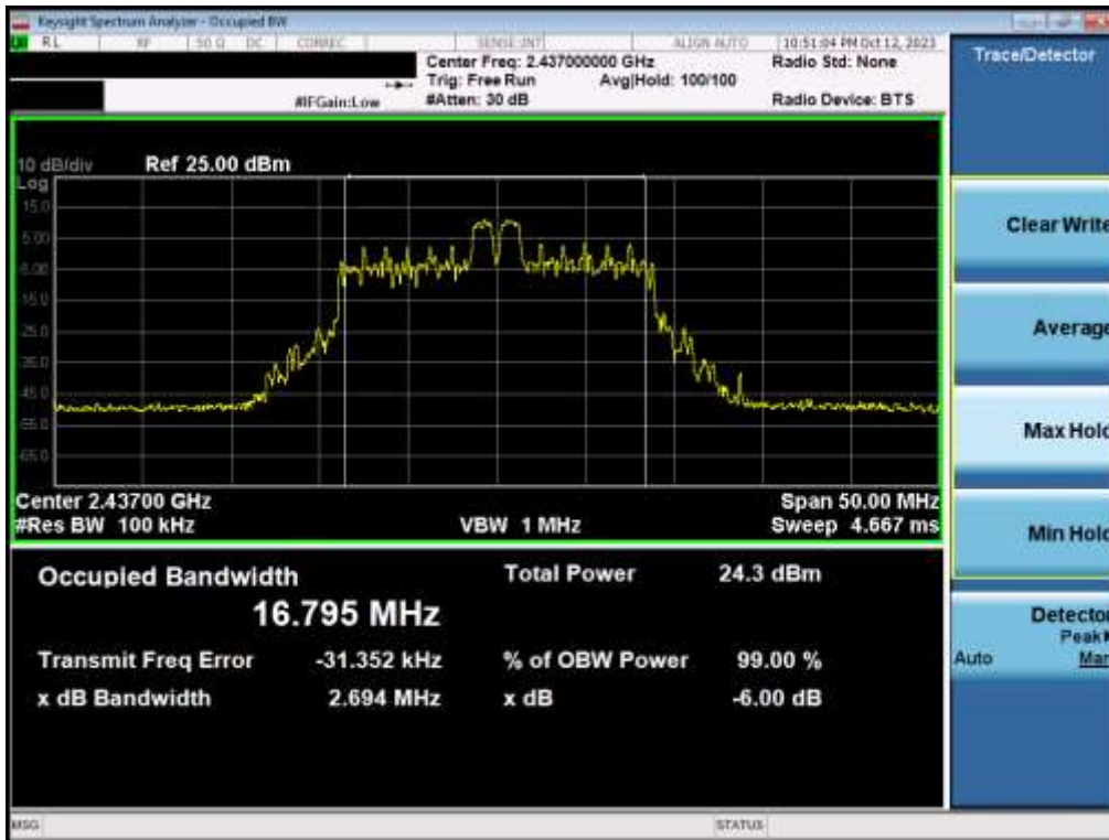
Plot 7-8. 6dB Bandwidth Plot MIMO ANT2 (802.11be OFDMA – 26 Tones – Ch. 6)
