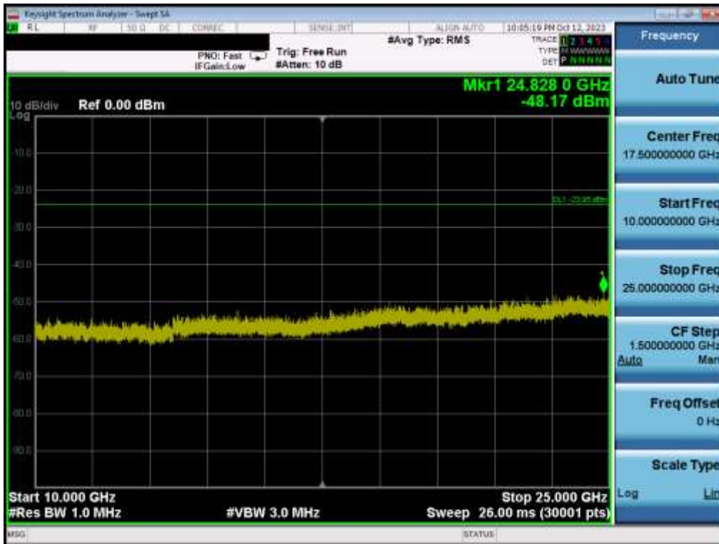
Plot 7-64. Conducted Spurious Plot MIMO ANT1 (802.11be OFDMA – 242 Tones – Ch. 11)
