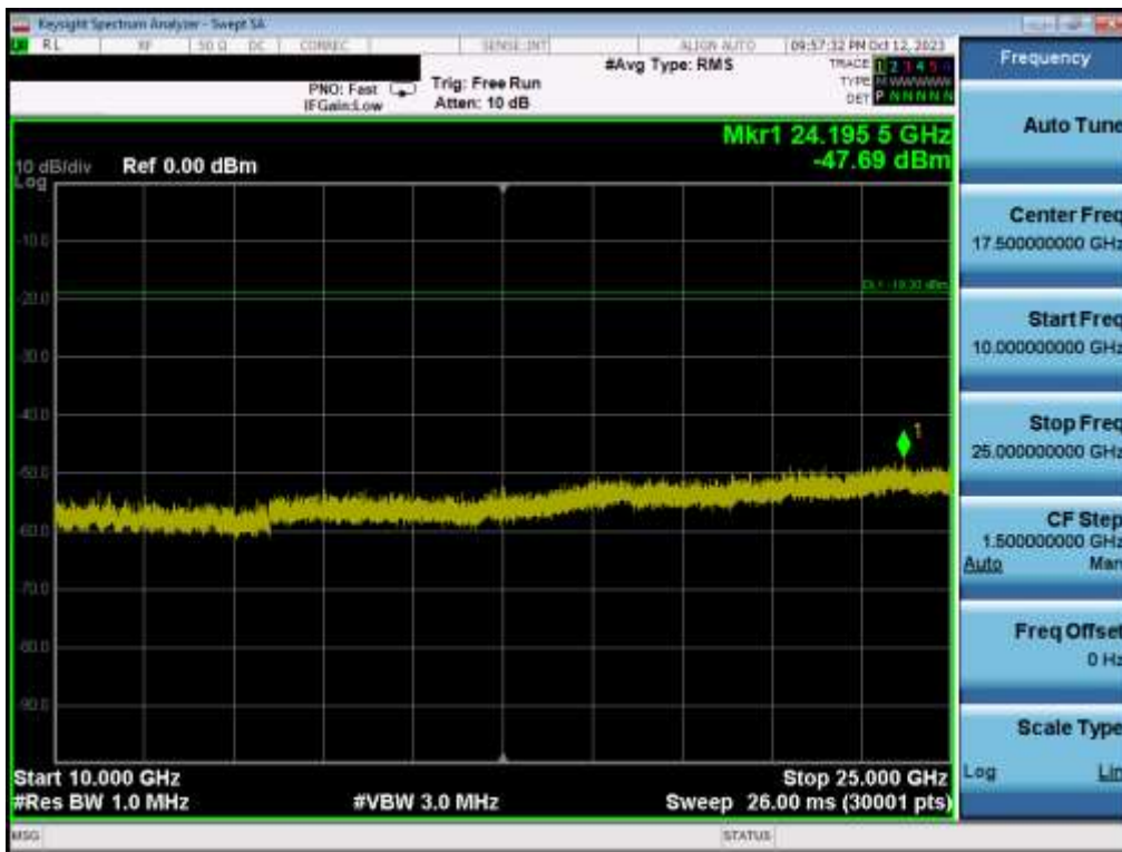
Plot 7-56. Conducted Spurious Plot MIMO ANT1 (802.11be OFDMA – 26 Tones – Ch. 6)
