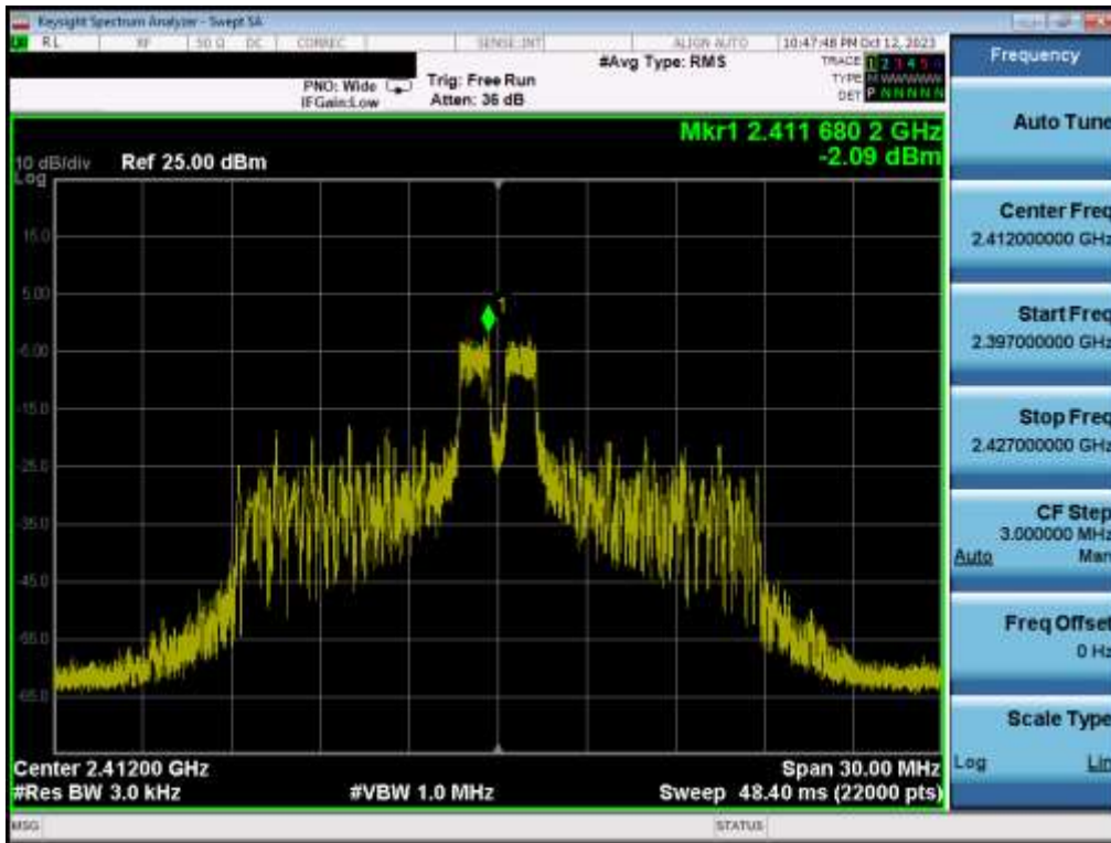
Plot 7-21. Power Spectral Density Plot MIMO ANT2 (802.11be OFDMA – 26 Tones – Ch. 1)
