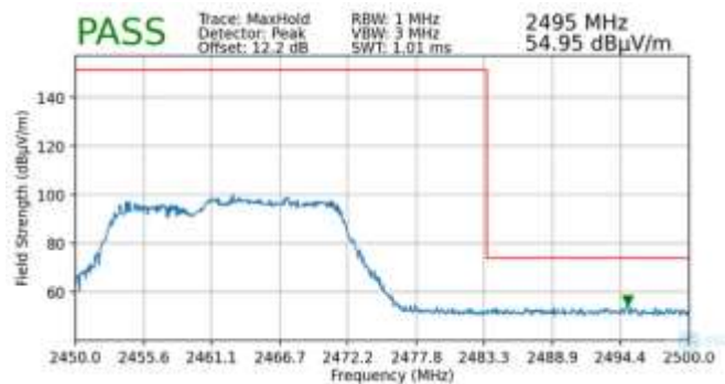
Plot 7-88. Radiated Restricted Upper Band Edge Measurement MIMO (Peak – 106 + 26 Tones)
