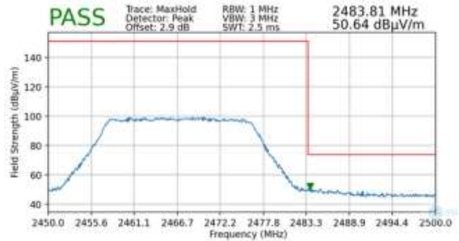
Plot 7-98. Radiated Restricted Upper Band Edge Measurement MIMO (Peak – 242 Tones)
