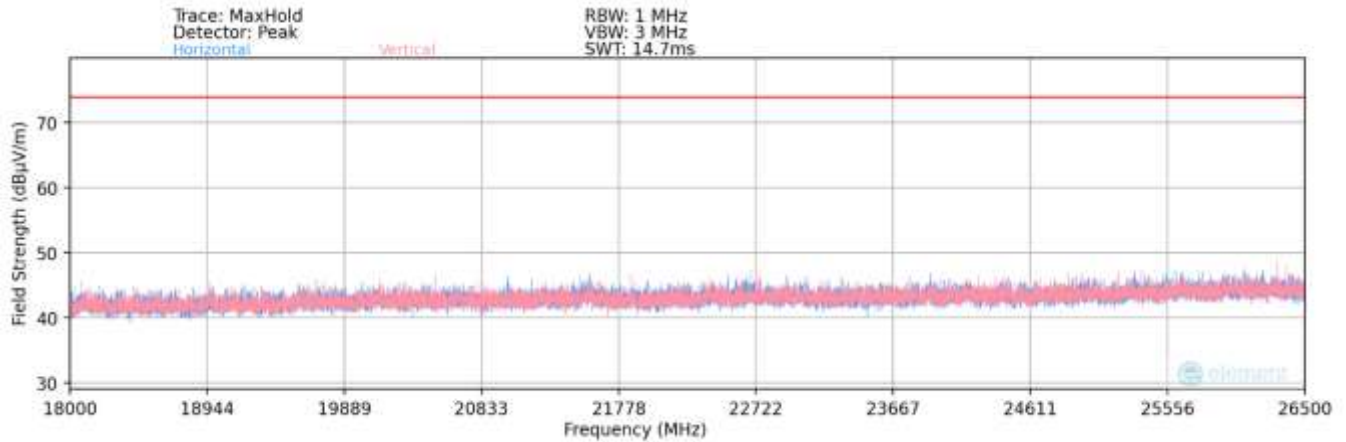
Plot 7-80. Radiated Spurious Plot above 18GHz MIMO (802.11be OFDMA – 26 Tones)
