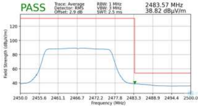
Plot 7-97. Radiated Restricted Upper Band Edge Measurement MIMO (Average – 242 Tones)
