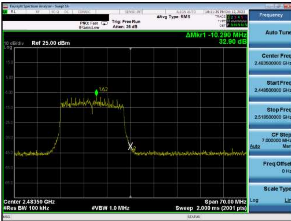
Plot 7-40. Band Edge Plot MIMO ANT1 (802.11be OFDMA – 242 Tones – Ch. 13)
