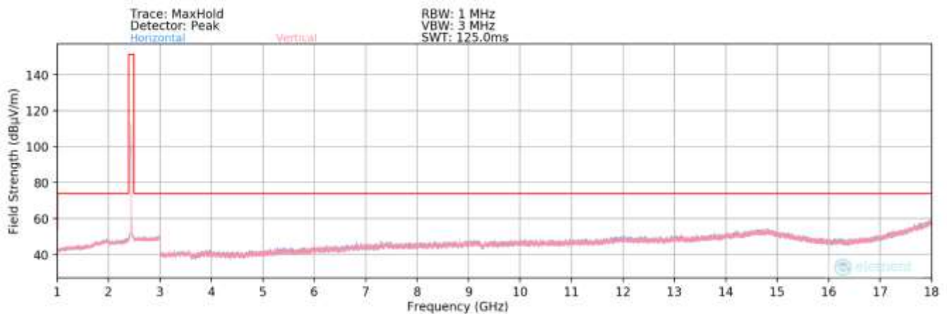
Plot 7-78. Radiated Spurious Plot above 1GHz MIMO (802.11be OFDMA – 26 Tones – Ch. 6)
