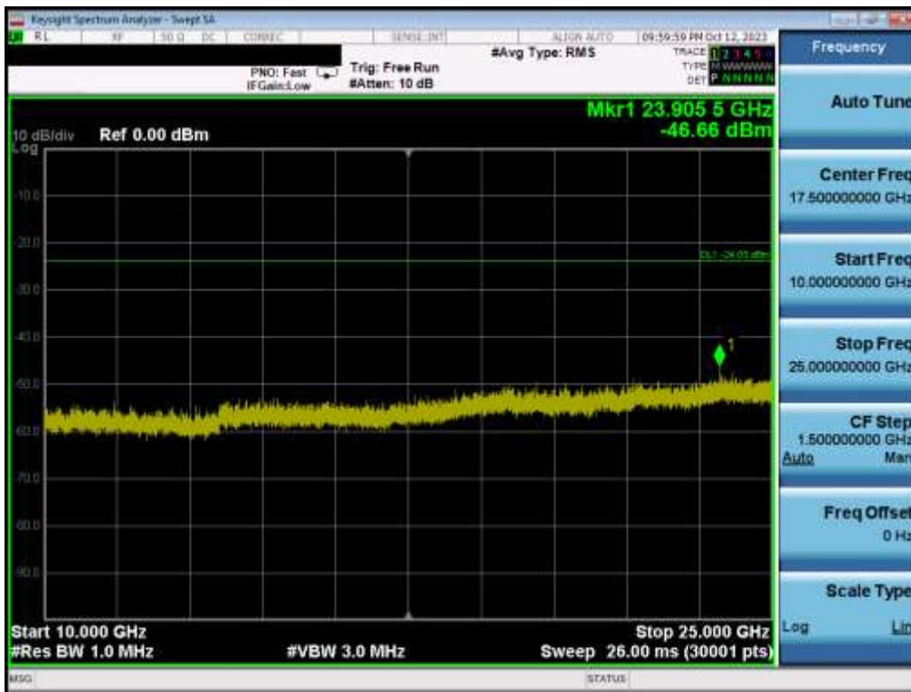
Plot 7-62. Conducted Spurious Plot MIMO ANT1 (802.11be OFDMA – 242 Tones – Ch. 6)
