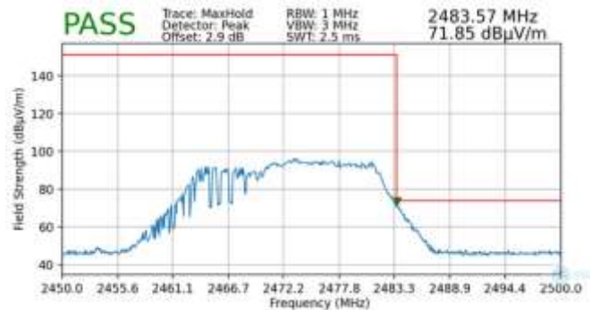
Plot 7-92. Radiated Restricted Upper Band Edge Measurement MIMO (Peak – 106 + 26 Tones)
