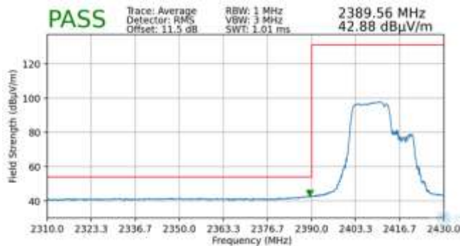
Plot 7-85. Radiated Restricted Lower Band Edge Measurement MIMO (Average – 106 + 26 Tones)
