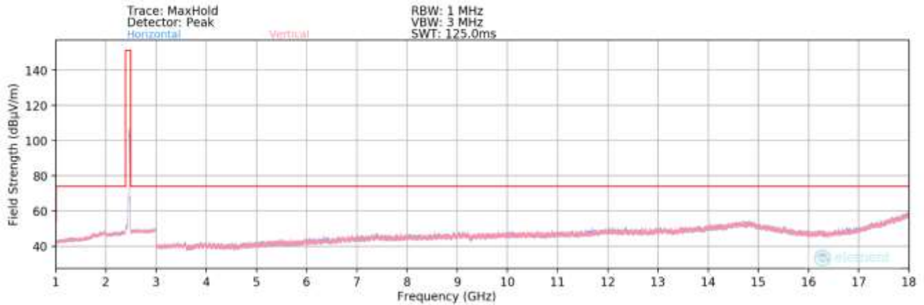
Plot 7-83. Radiated Spurious Plot above 1GHz MIMO (802.11be OFDMA – 242 Tones – Ch. 11)
