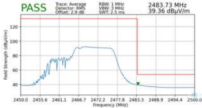
Plot 7-89. Radiated Restricted Upper Band Edge Measurement MIMO (Average – 106 + 26 Tones)
