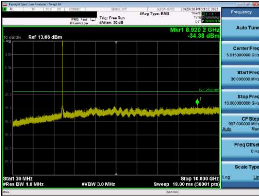
Plot 7-61. Conducted Spurious Plot MIMO ANT1 (802.11be OFDMA – 242 Tones – Ch. 6)
