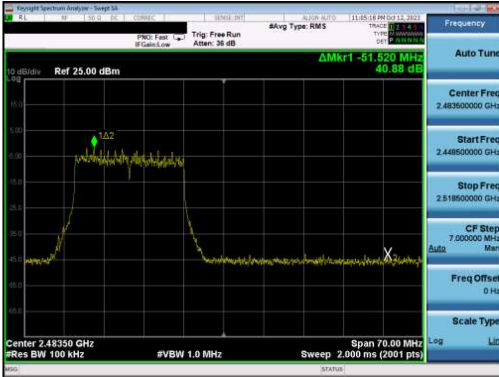
Plot 7-51. Band Edge Plot MIMO ANT2 (802.11be OFDMA – 242 Tones – Ch. 12)
