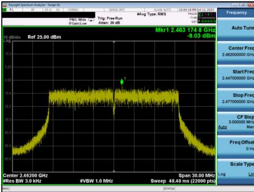
Plot 7-18. Power Spectral Density Plot MIMO ANT1 (802.11be OFDMA – 242 Tones – Ch. 11)
