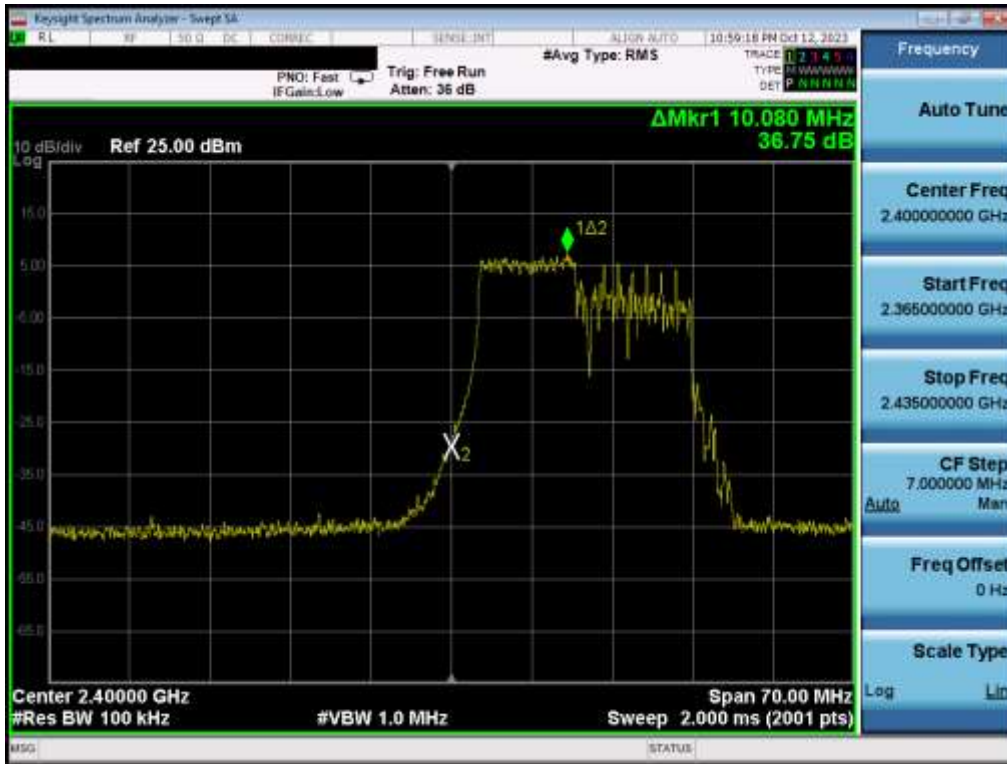
Plot 7-41. Band Edge Plot MIMO ANT2 (802.11be OFDMA – 106 Tones – Ch. 1)
