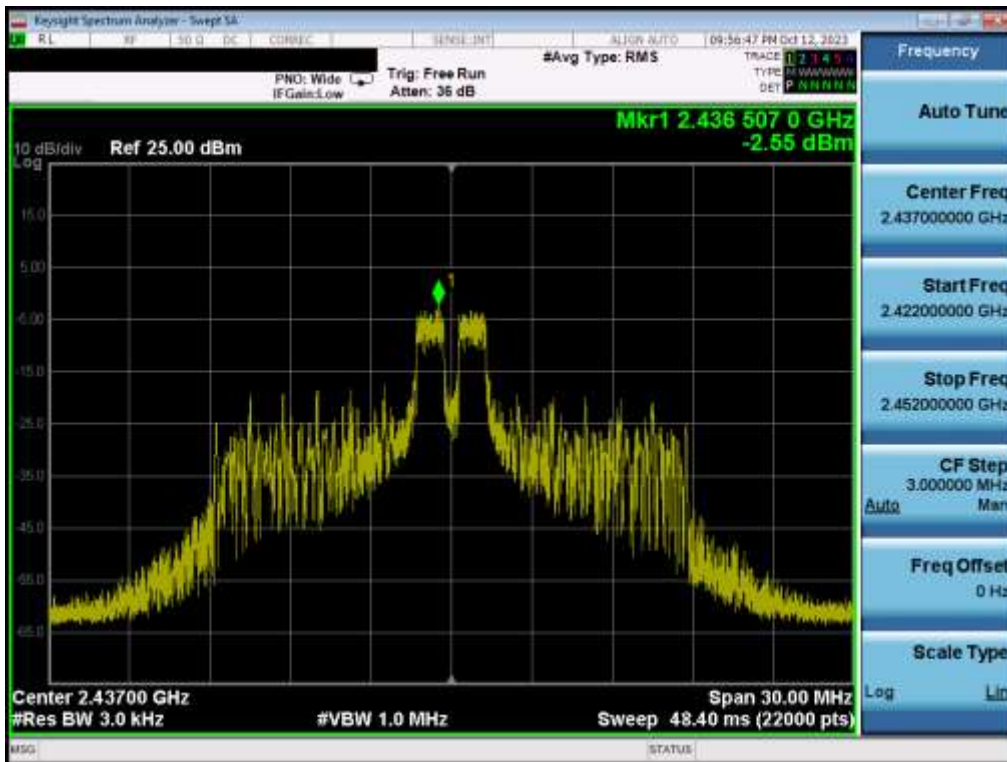
Plot 7-14. Power Spectral Density Plot MIMO ANT1 (802.11be OFDMA – 26 Tones – Ch. 6)
