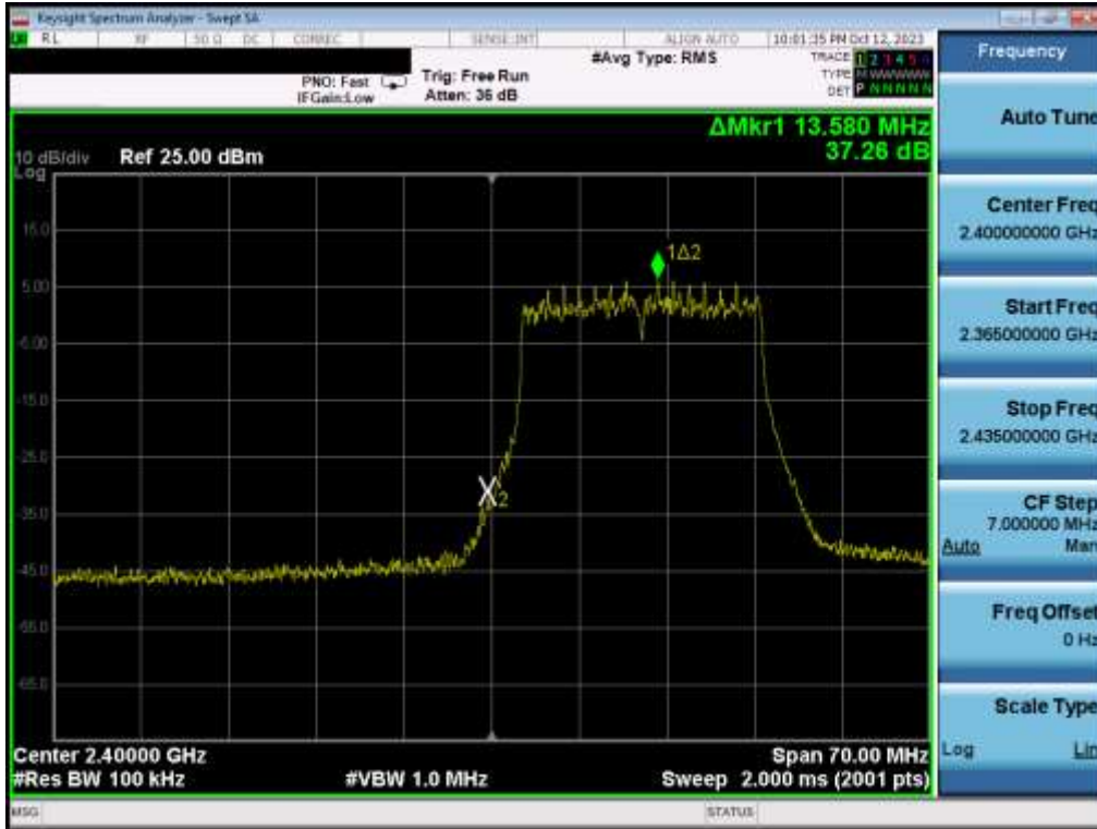
Plot 7-37. Band Edge Plot MIMO ANT1 (802.11be OFDMA – 242 Tones – Ch. 1)
