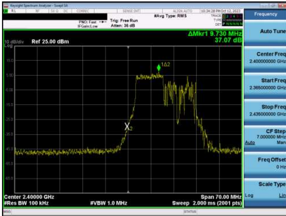
Plot 7-29. Band Edge Plot MIMO ANT1 (802.11be OFDMA – 106 Tones – Ch. 1)
