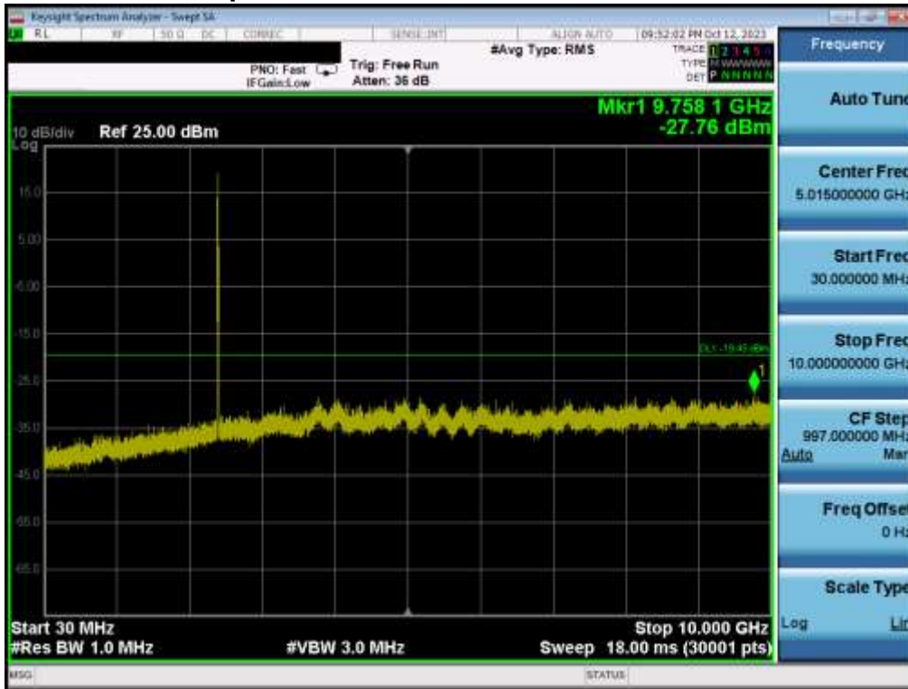
Plot 7-53. Conducted Spurious Plot MIMO ANT1 (802.11be OFDMA – 26 Tones – Ch. 1)
