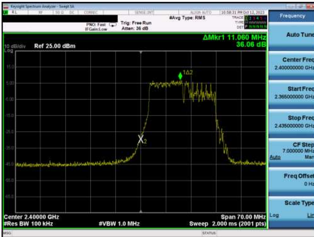
Plot 7-42. Band Edge Plot MIMO ANT2 (802.11be OFDMA – 106 + 26 Tones – Ch. 1)
