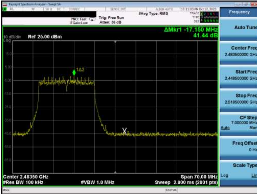
Plot 7-39. Band Edge Plot MIMO ANT1 (802.11be OFDMA – 242 Tones – Ch. 12)
