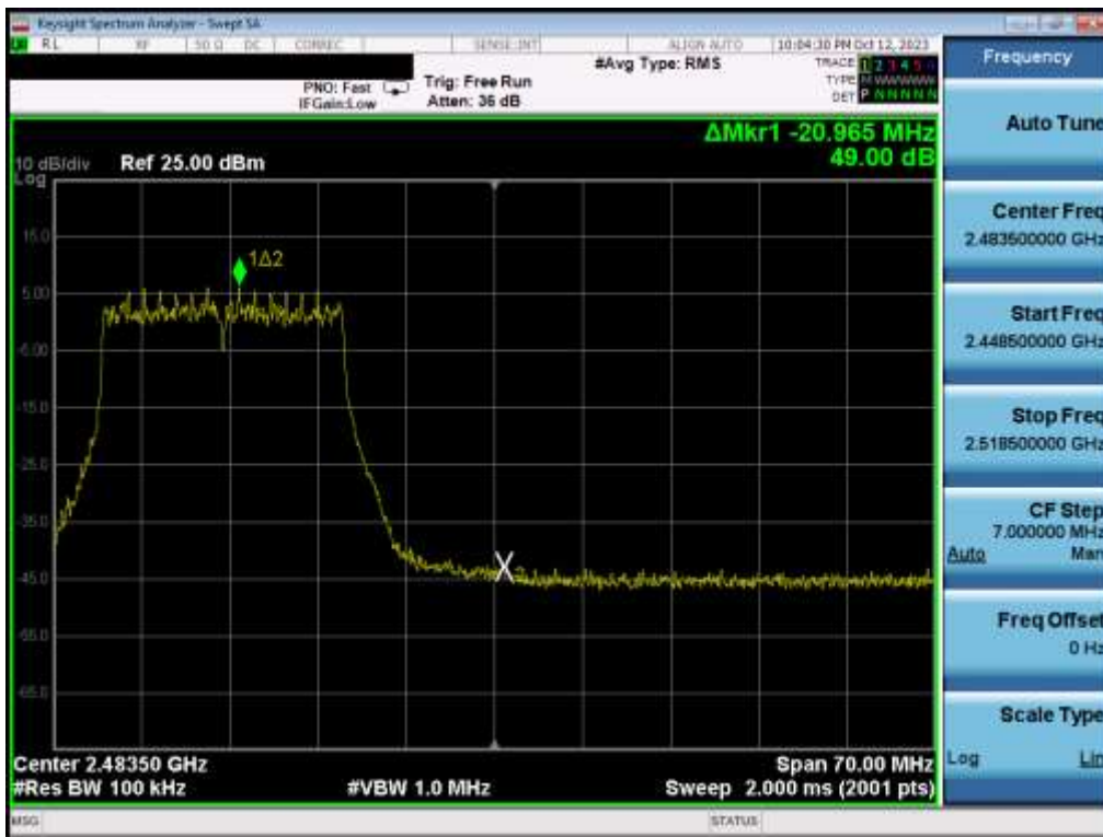
Plot 7-38. Band Edge Plot MIMO ANT1 (802.11be OFDMA – 242 Tones – Ch. 11)
