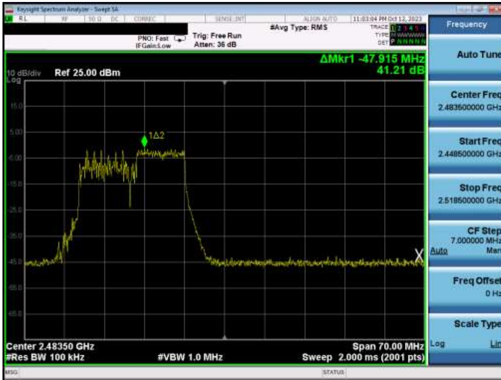
Plot 7-45. Band Edge Plot MIMO ANT2 (802.11be OFDMA – 106 Tones – Ch. 12)
