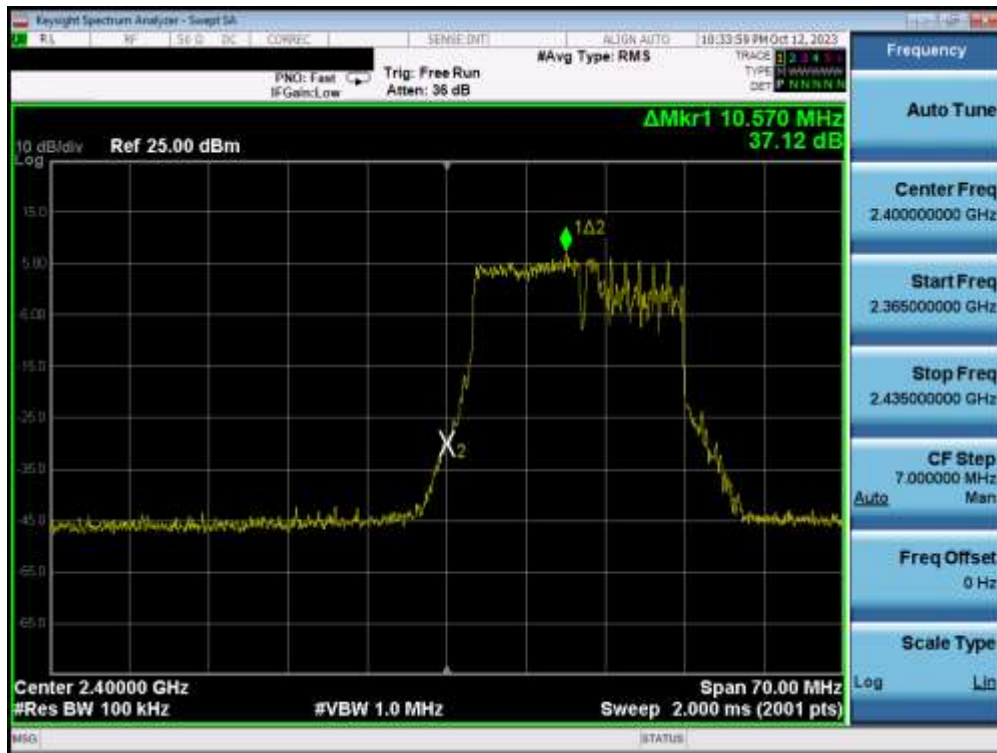
Plot 7-30. Band Edge Plot MIMO ANT1 (802.11be OFDMA – 106 + 26 Tones – Ch. 1)
