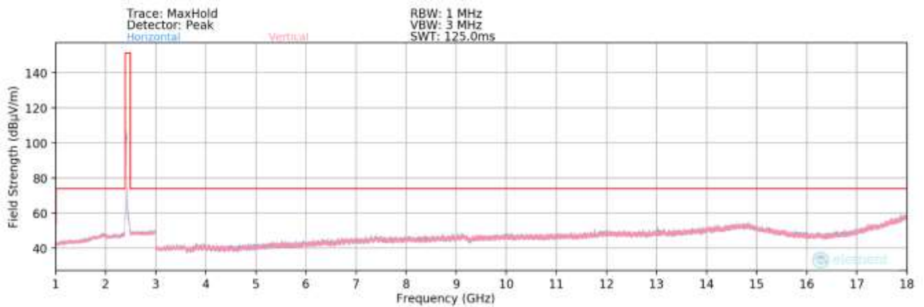
Plot 7-81. Radiated Spurious Plot above 1GHz MIMO (802.11be OFDMA – 242 Tones – Ch. 1)
