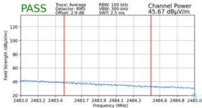
Plot 7-91. Radiated Restricted Upper Band Edge Measurement MIMO (Average – 106 + 26 Tones)
