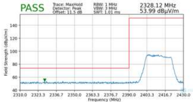
Plot 7-94. Radiated Restricted Lower Band Edge Measurement MIMO (Peak – 242 Tones)
