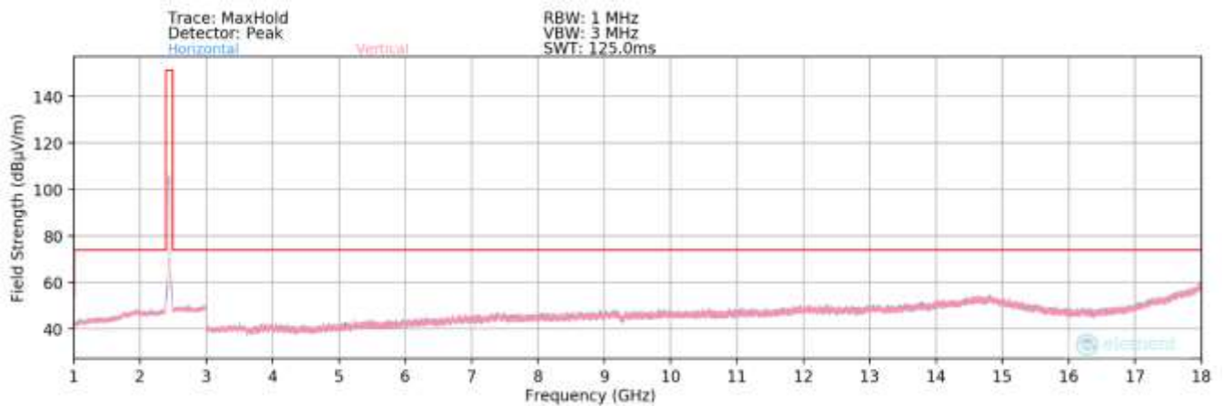
Plot 7-82. Radiated Spurious Plot above 1GHz MIMO (802.11be OFDMA – 242 Tones – Ch. 6)
