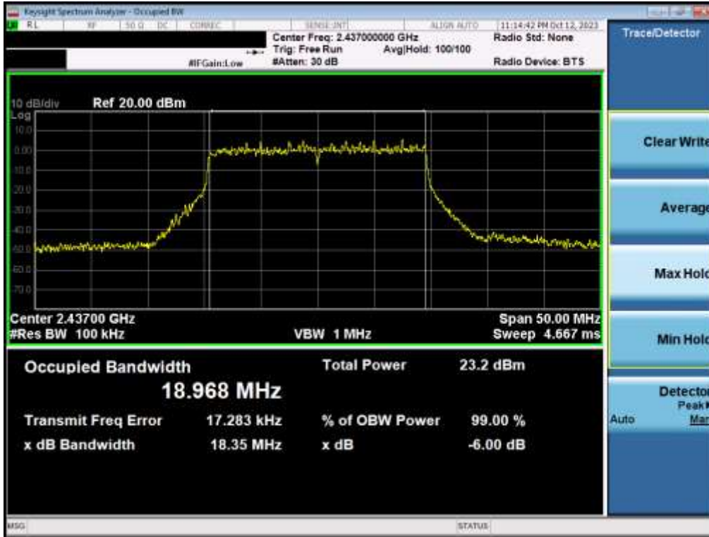
Plot 7-11. 6dB Bandwidth Plot MIMO ANT2 (802.11be OFDMA – 242 Tones – Ch. 6)
