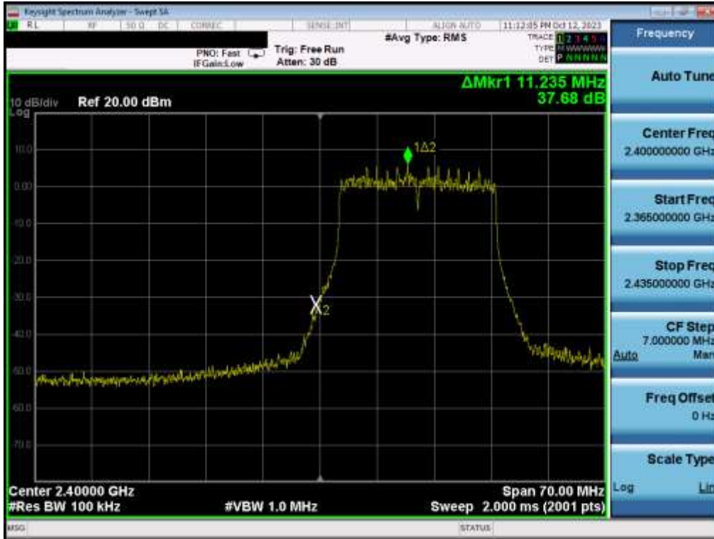
Plot 7-49. Band Edge Plot MIMO ANT2 (802.11be OFDMA – 242 Tones – Ch. 1)
