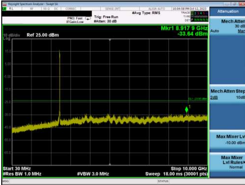
Plot 7-63. Conducted Spurious Plot MIMO ANT1 (802.11be OFDMA – 242 Tones – Ch. 11)
