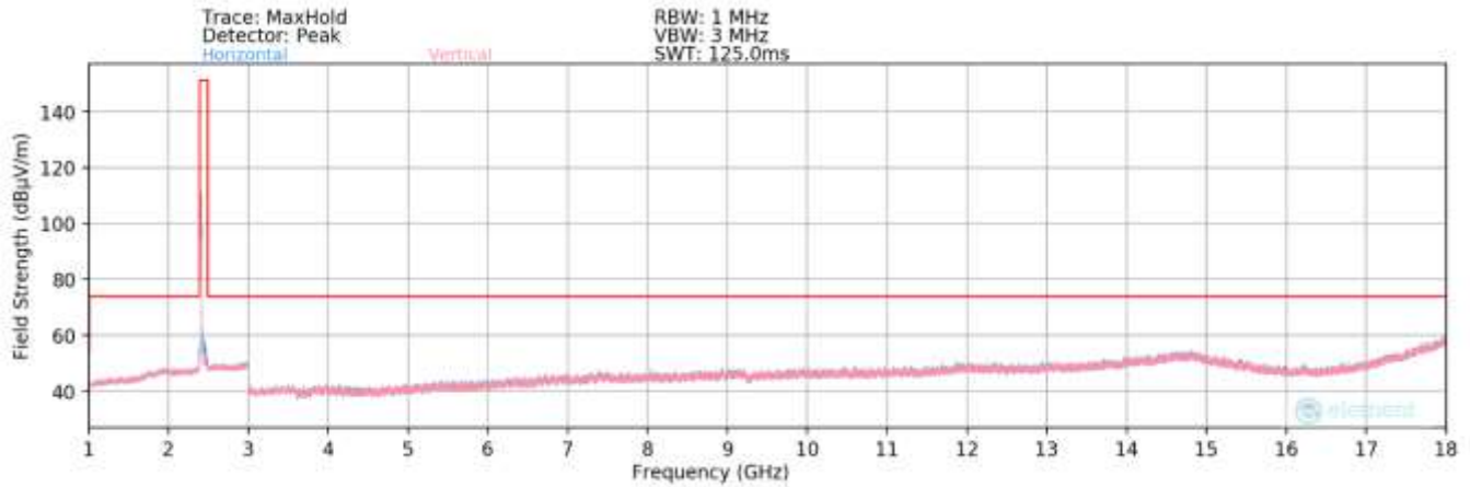
Plot 7-77. Radiated Spurious Plot above 1GHz MIMO (802.11be OFDMA – 26 Tones – Ch. 1)
