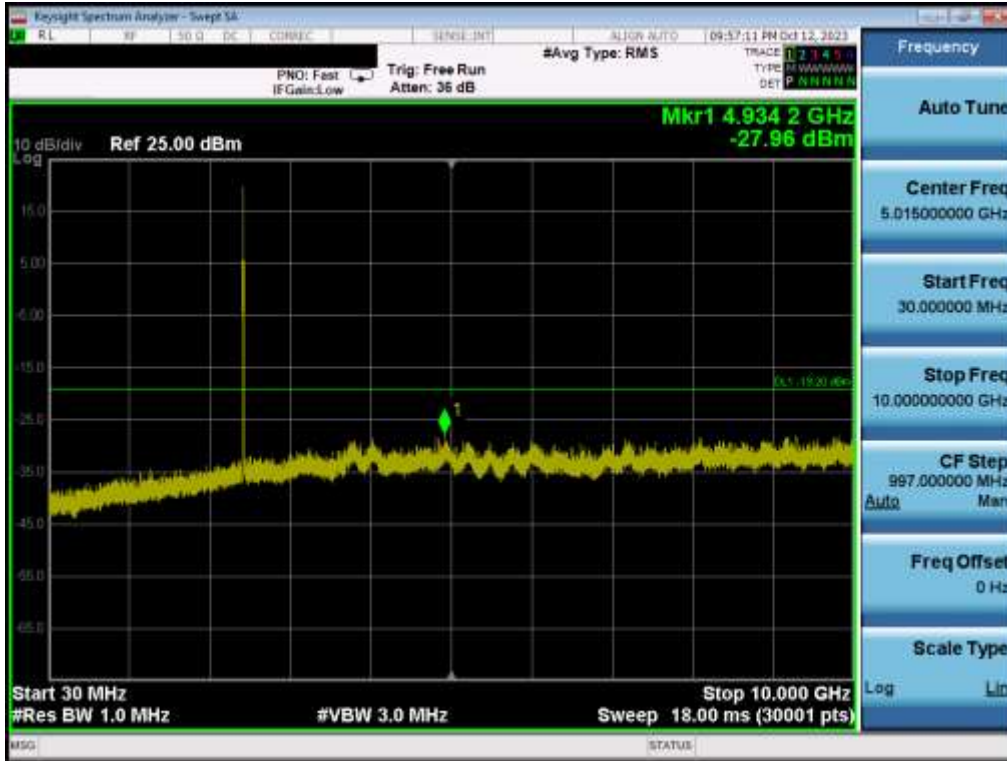
Plot 7-55. Conducted Spurious Plot MIMO ANT1 (802.11be OFDMA – 26 Tones – Ch. 6)
