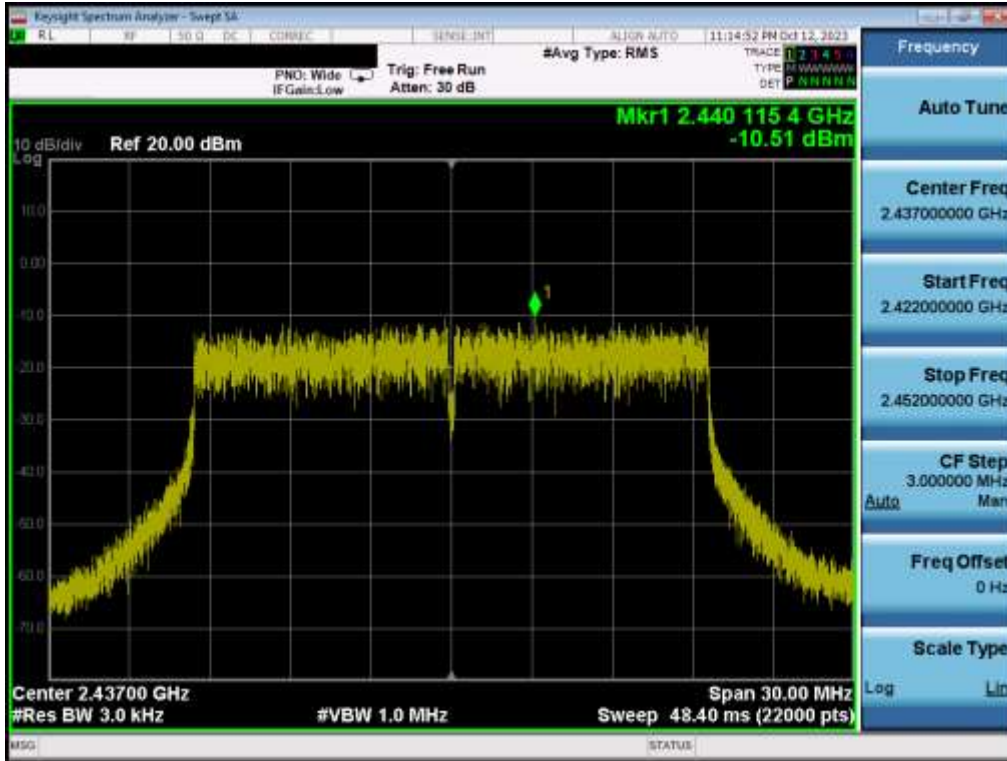
Plot 7-25. Power Spectral Density Plot MIMO ANT2 (802.11be OFDMA – 242 Tones – Ch. 6)
