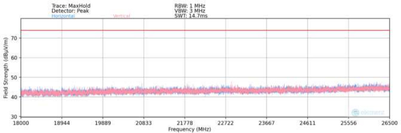
Plot 7-84. Radiated Spurious Plot above 18GHz MIMO (802.11be OFDMA – 242 Tones)
