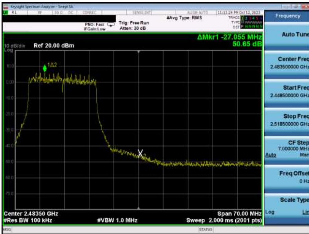
Plot 7-50. Band Edge Plot MIMO ANT2 (802.11be OFDMA – 242 Tones – Ch. 11)
