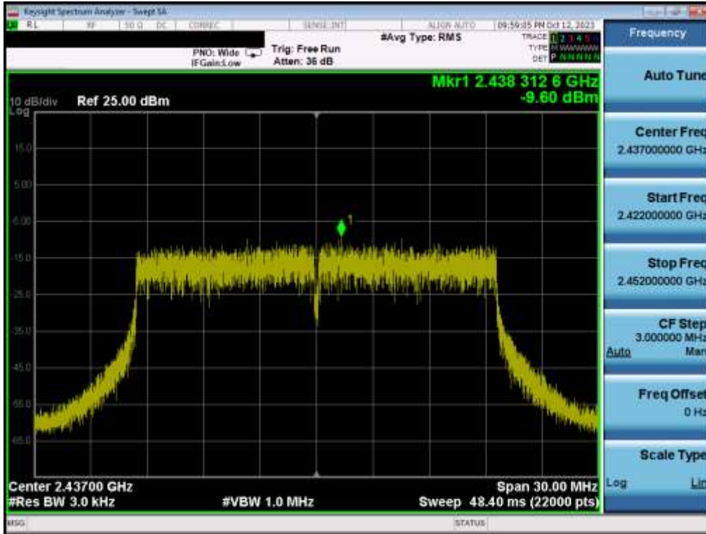
Plot 7-17. Power Spectral Density Plot MIMO ANT1 (802.11be OFDMA – 242 Tones – Ch. 6)
