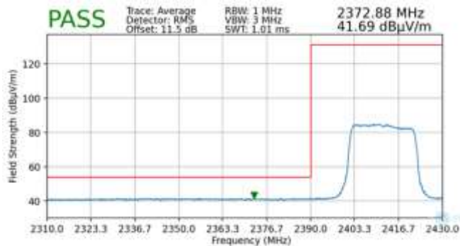
Plot 7-93. Radiated Restricted Lower Band Edge Measurement MIMO (Average – 242 Tones)
