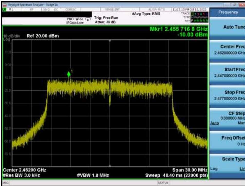
Plot 7-26. Power Spectral Density Plot MIMO ANT2 (802.11be OFDMA – 242 Tones – Ch. 11)
