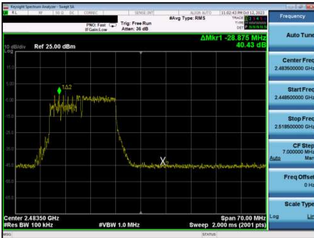
Plot 7-46. Band Edge Plot MIMO ANT2 (802.11be OFDMA – 106 + 26 Tones – Ch. 12)
