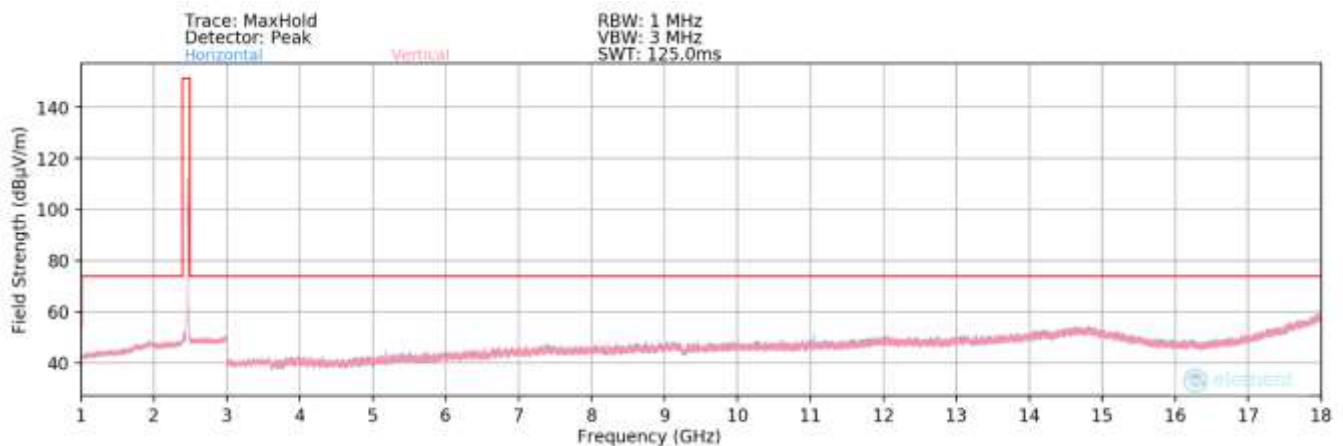
Plot 7-79. Radiated Spurious Plot above 1GHz MIMO (802.11be OFDMA – 26 Tones – Ch. 11)
