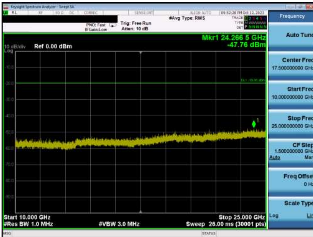
Plot 7-54. Conducted Spurious Plot MIMO ANT1 (802.11be OFDMA – 26 Tones – Ch. 1)
