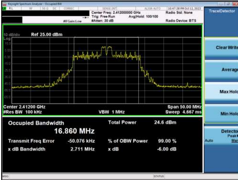
Plot 7-7. 6dB Bandwidth Plot MIMO ANT2 (802.11be OFDMA – 26 Tones – Ch. 1)
