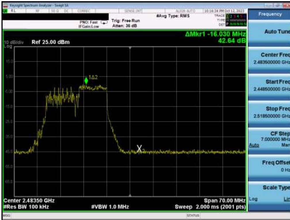
Plot 7-33. Band Edge Plot MIMO ANT1 (802.11be OFDMA – 106 Tones – Ch. 12)
