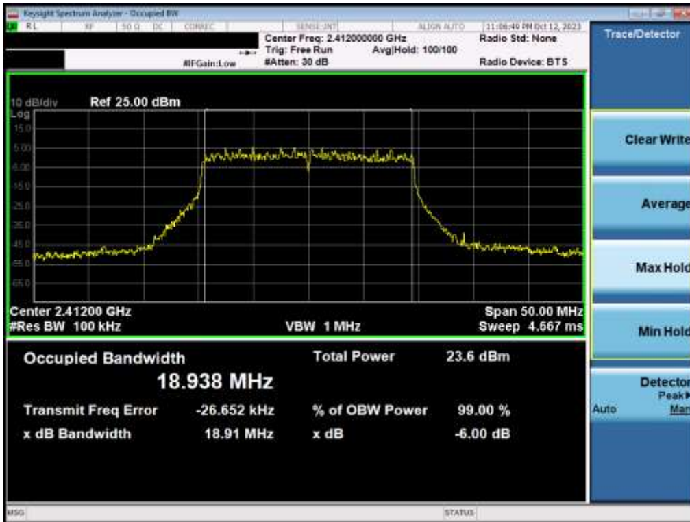
Plot 7-10. 6dB Bandwidth Plot MIMO ANT2 (802.11be OFDMA – 242 Tones – Ch. 1)
