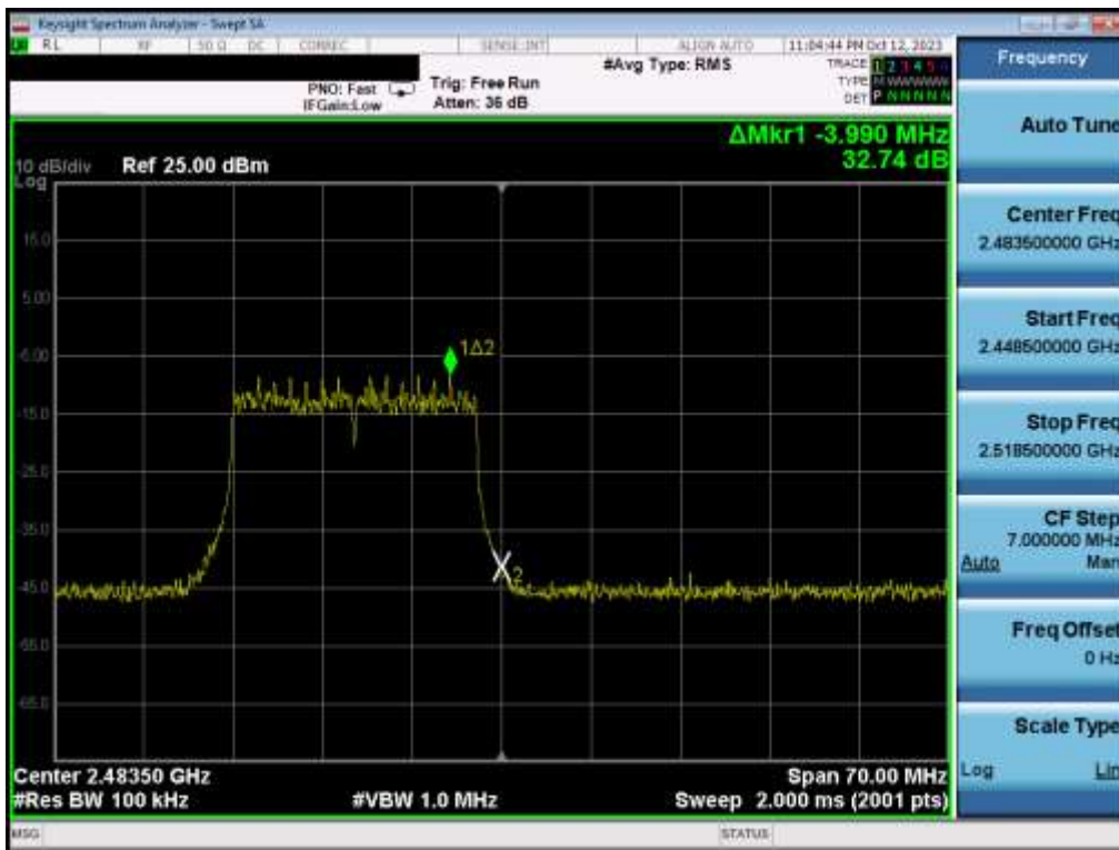
Plot 7-52. Band Edge Plot MIMO ANT2 (802.11be OFDMA – 242 Tones – Ch. 13)
