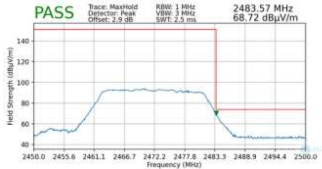
Plot 7-100. Radiated Restricted Upper Band Edge Measurement MIMO (Peak – 242 Tones)
