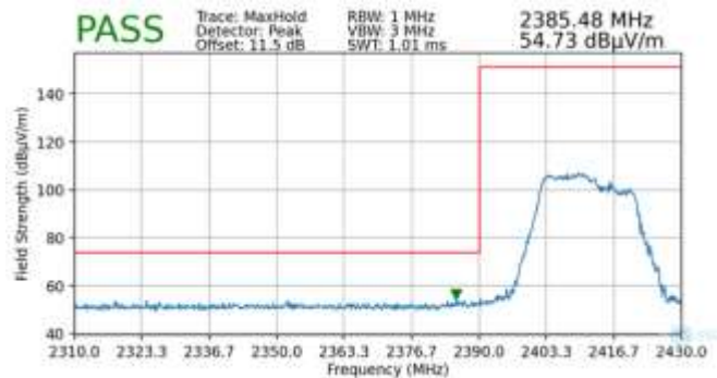
Plot 7-86. Radiated Restricted Lower Band Edge Measurement MIMO (Peak – 106 + 26 Tones)
