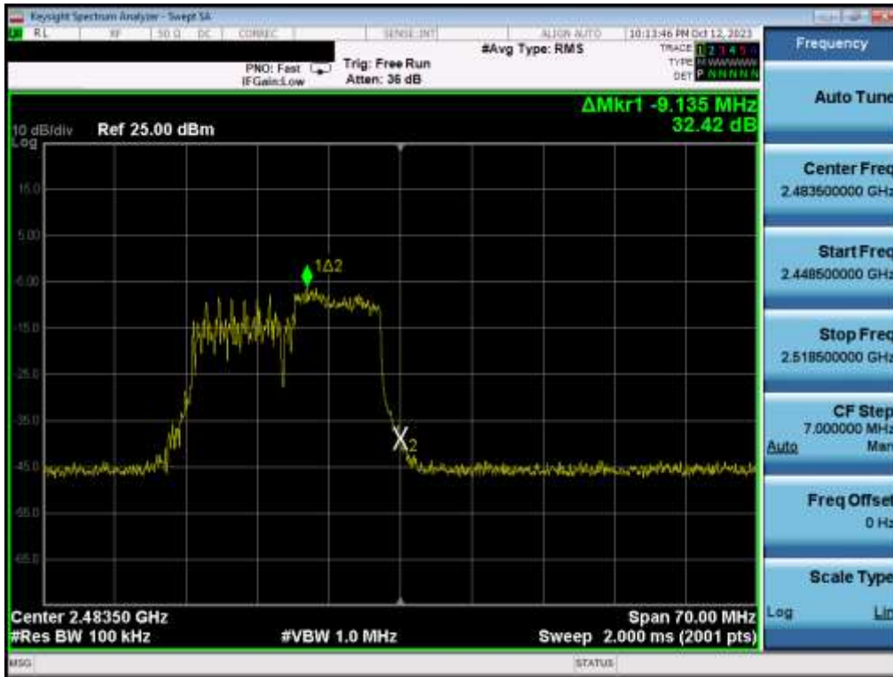
Plot 7-35. Band Edge Plot MIMO ANT1 (802.11be OFDMA – 106 Tones – Ch. 13)
