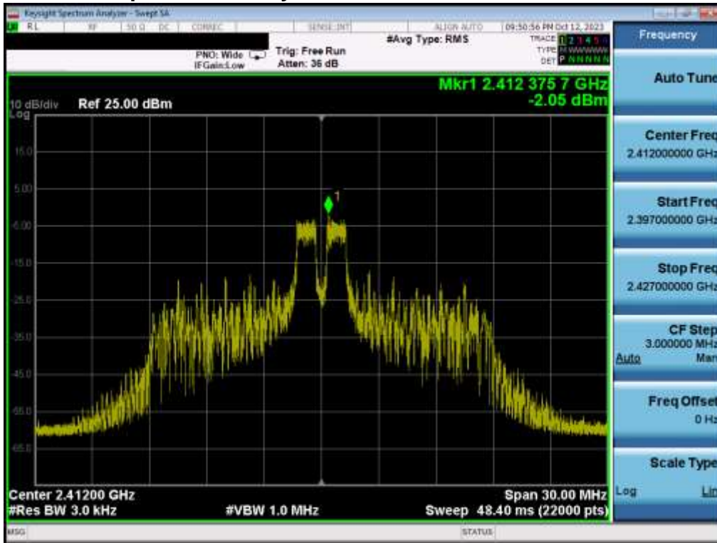
Plot 7-13. Power Spectral Density Plot MIMO ANT1 (802.11be OFDMA – 26 Tones – Ch. 1)
