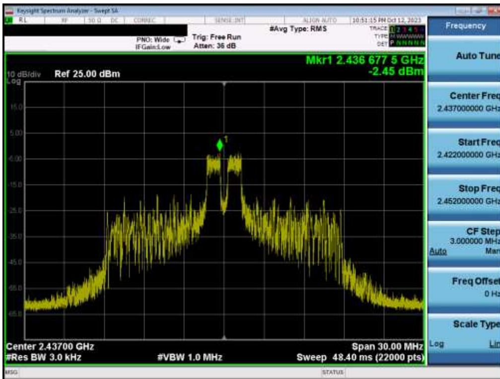
Plot 7-22. Power Spectral Density Plot MIMO ANT2 (802.11be OFDMA – 26 Tones – Ch. 6)
