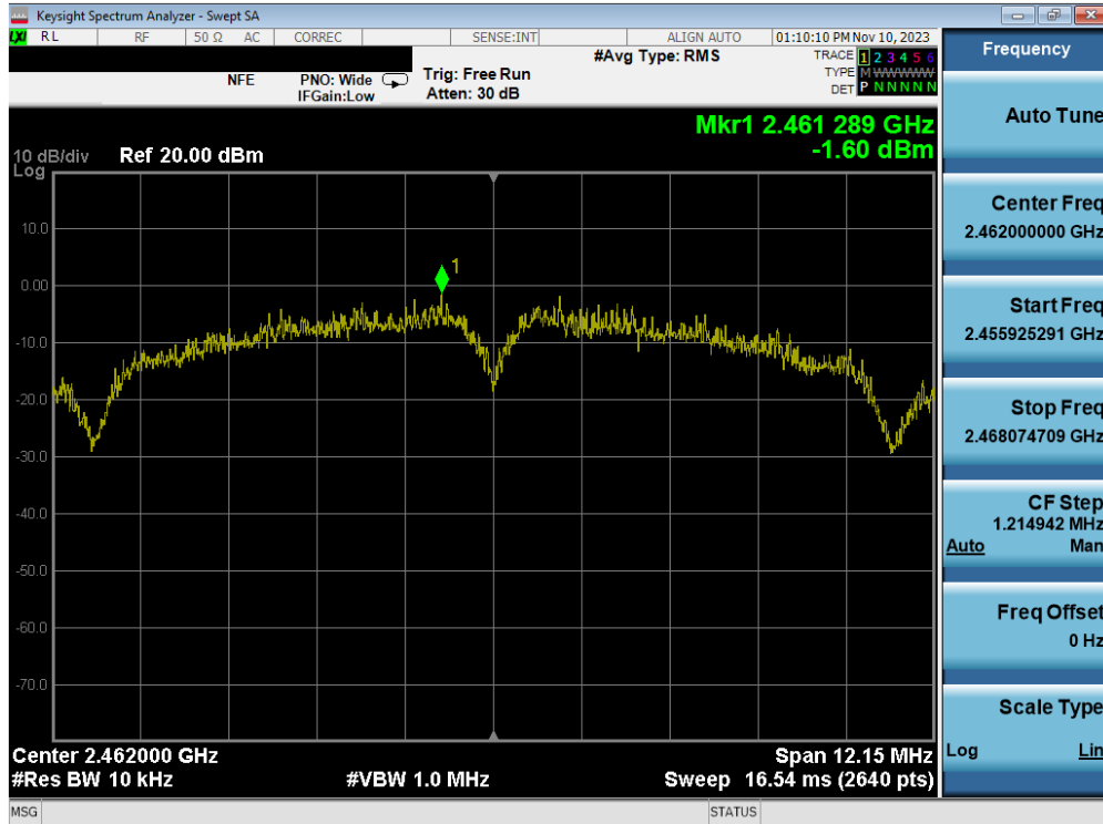
Plot 7-57. Power Spectral Density Plot MIMO ANT2 (802.11b – Ch. 11)
