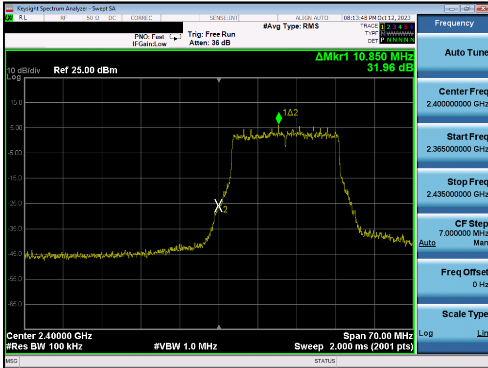
Plot 7-93. Band Edge Plot MIMO ANT1 (802.11be (2.4GHz) – Ch. 1)
