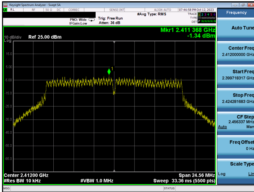
Plot 7-58. Power Spectral Density Plot MIMO ANT2 (802.11g – Ch. 1)
