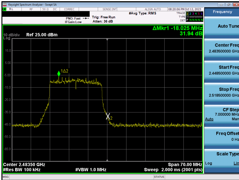
Plot 7-96. Band Edge Plot MIMO ANT1 (802.11be (2.4GHz) – Ch. 13)
