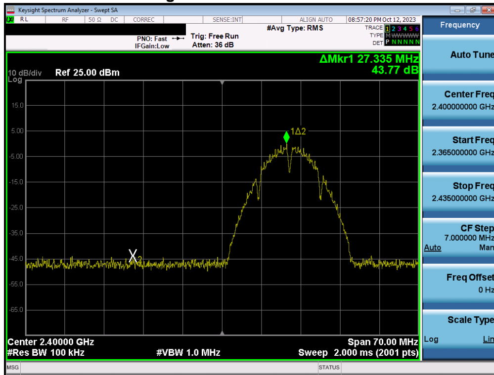
Plot 7-73. Band Edge Plot MIMO ANT1 (802.11b – Ch. 1)
