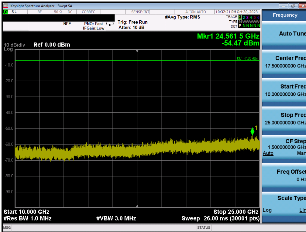
Plot 7-138. Conducted Spurious Plot (Bluetooth (LE), 1Mbps – Ch. 19) – MIMO ANT2
