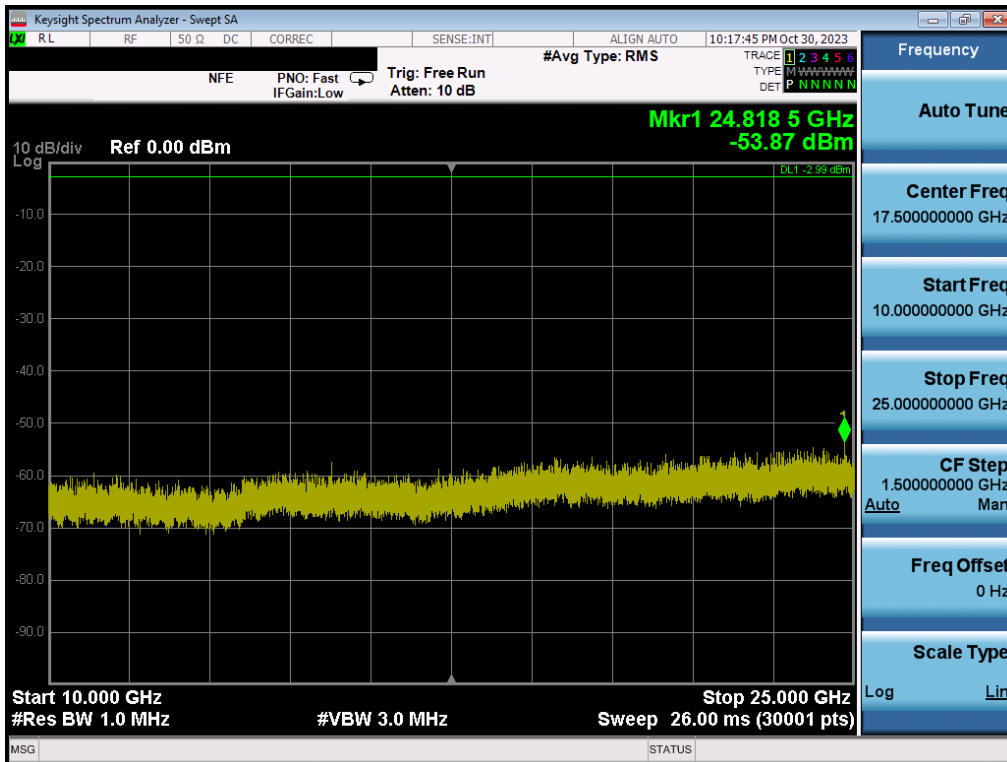
Plot 7-128. Conducted Spurious Plot (Bluetooth (LE), 1Mbps – Ch. 39) – SISO ANT2
