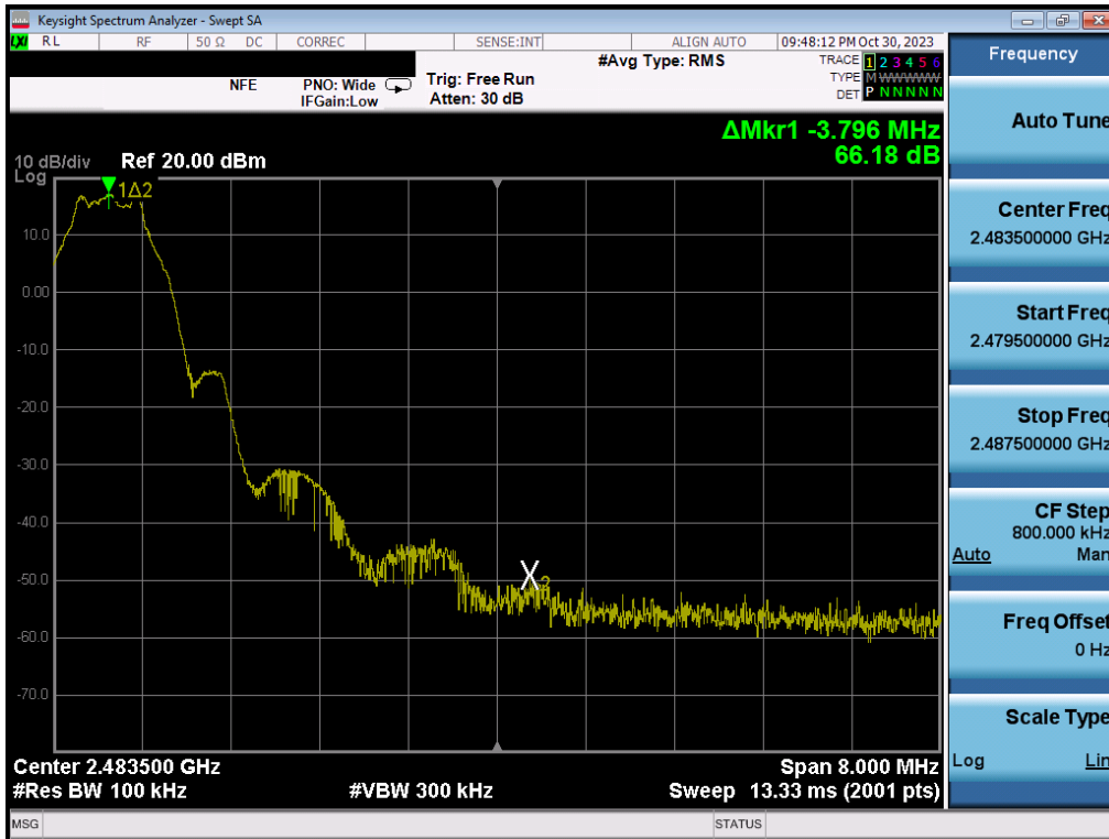
Plot 7-110. Band Edge Plot (Bluetooth (LE), 1Mbps – Ch. 39) – SISO ANT1
