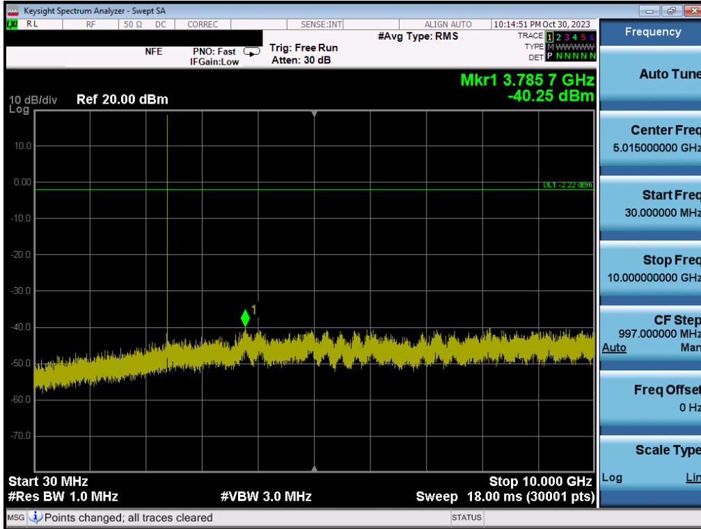
Plot 7-123. Conducted Spurious Plot (Bluetooth (LE), 1Mbps – Ch. 0) – SISO ANT2
