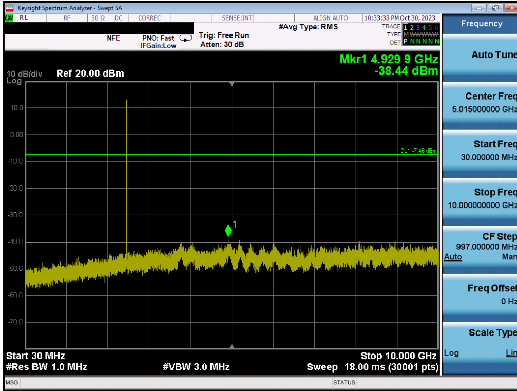
Plot 7-139. Conducted Spurious Plot (Bluetooth (LE), 1Mbps – Ch. 39) – MIMO ANT2
