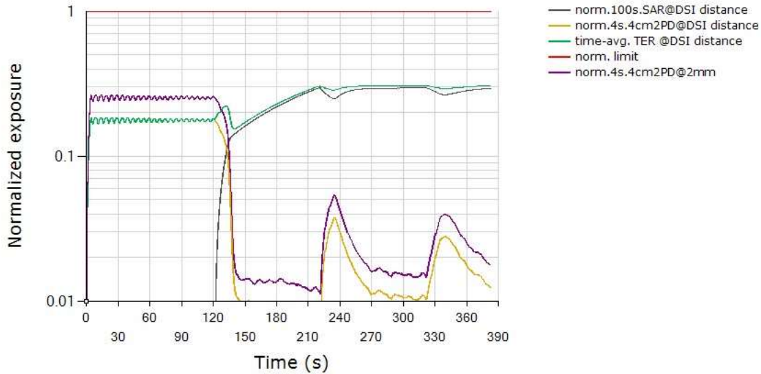
Total Normalized Time-averaged RF Exposure Tech: LTE, Band 2 / Tech: NR5G MMW, Band 261
