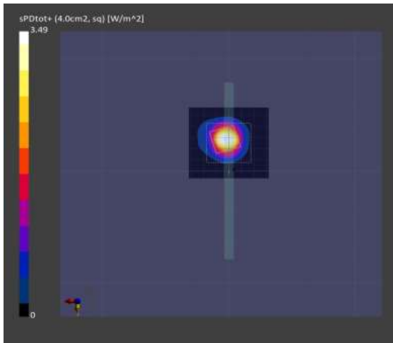
Figure 9-2: 4cm 2 psPD distribution measured at input.power.limit of 2.4 dBm on the front for n261 Beam 40
