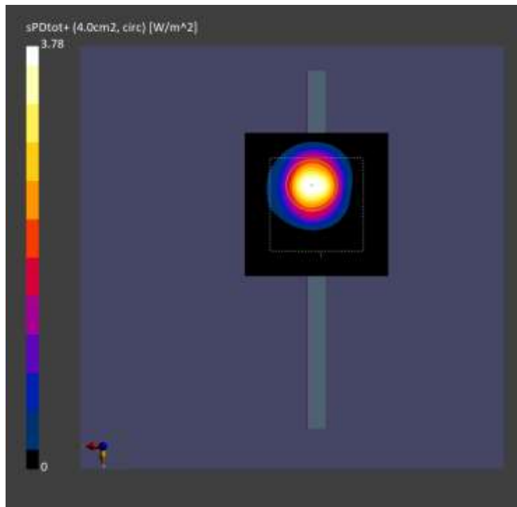
Figure 9-2: 4cm 2 psPD distribution measured at input.power.limit of 2.4 dBm on the front for n261 Beam 40
