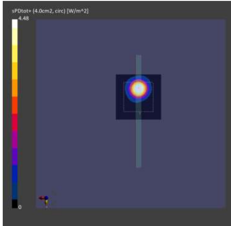
Figure 9-3: 4cm 2 psPD distribution measured at input.power.limit of 10.1 dBm on the front for n261 Beam 5
