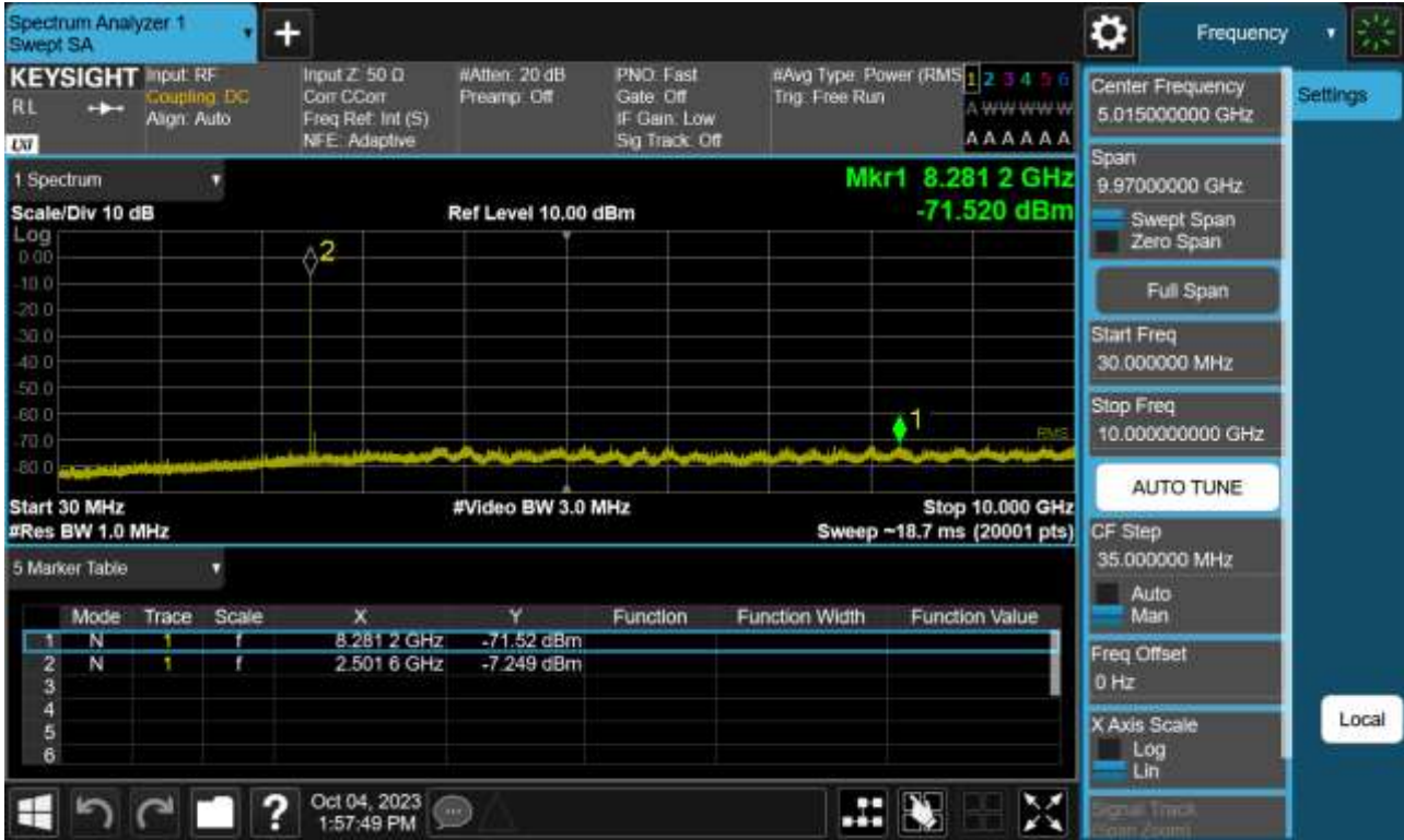
Sub6 n41. Conducted Spurious Plot 1 (80 MHz Ch.508002 BPSK RB 1)
