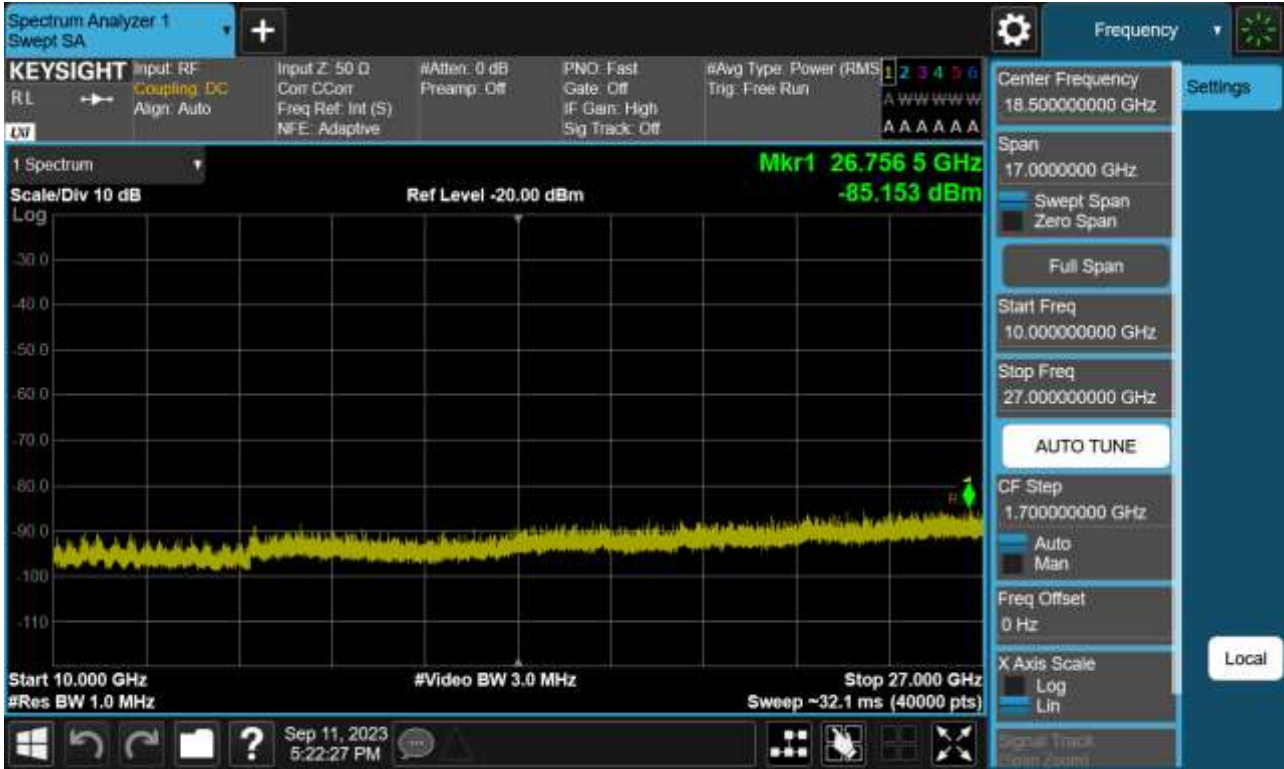
Sub6 n41. Conducted Spurious Plot 2 (80 MHz Ch.52998 BPSK RB 1)
