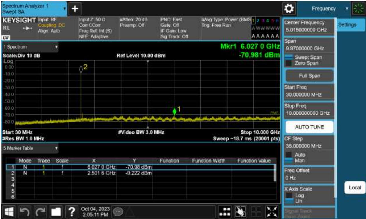
Sub6 n41. Conducted Spurious Plot 1 (100 MHz Ch.5 10000 BPSK RB 1)
