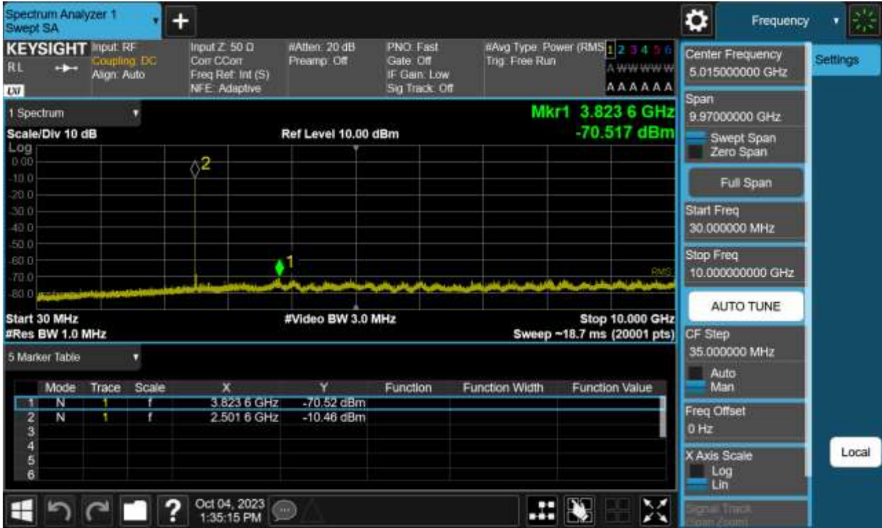
Sub6 n41. Conducted Spurious Plot 1 (25 MHz Ch.502500 BPSK RB 1)
