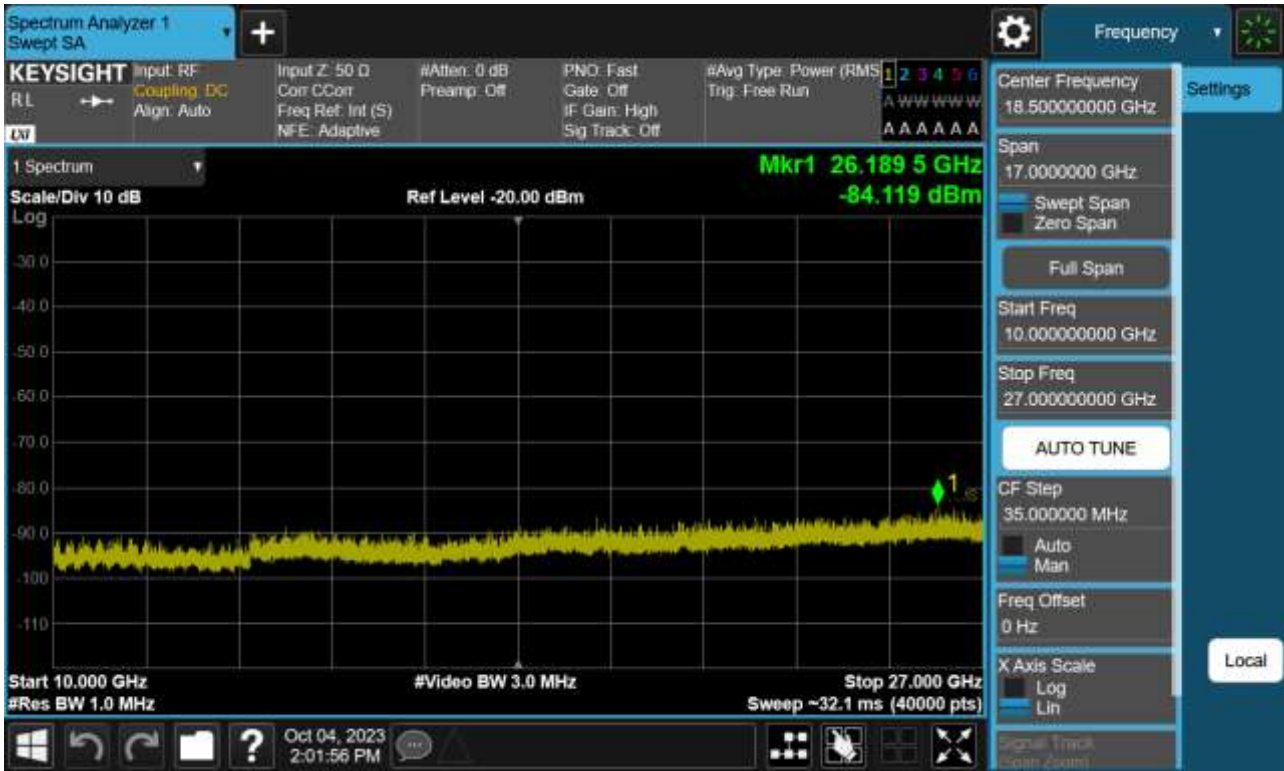
Sub6 n41. Conducted Spurious Plot 2 (90 MHz Ch.509004 BPSK RB 1)
