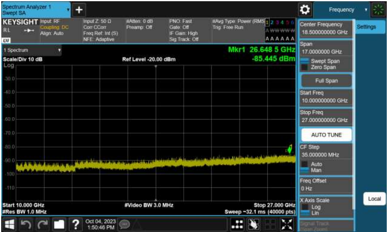
Sub6 n41. Conducted Spurious Plot 2 (60 MHz Ch.506004 BPSK RB 1)
