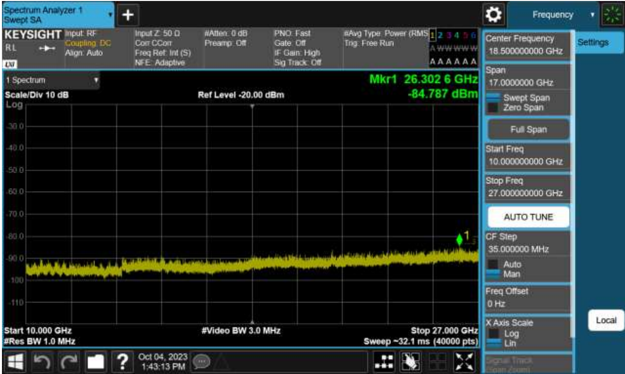
Sub6 n41. Conducted Spurious Plot 2 (40 MHz Ch.504000 BPSK RB 1)
