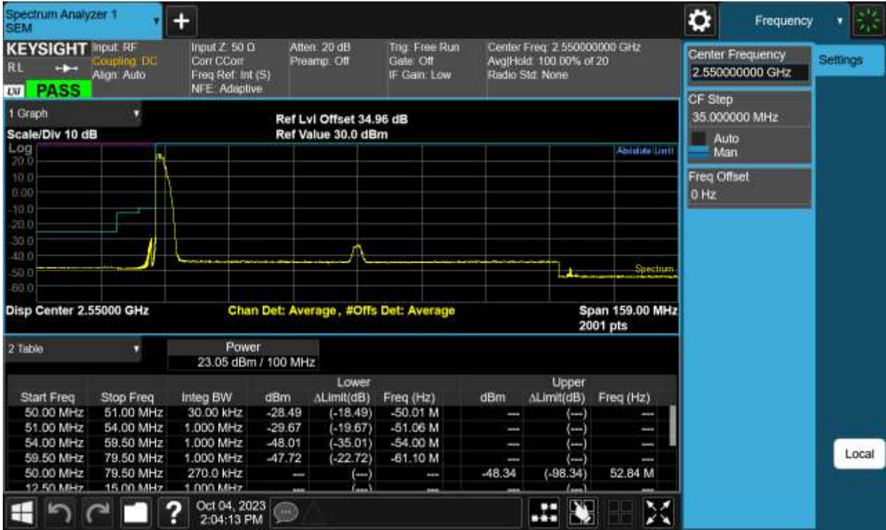
Sub6 n41. Low Channel Edge Plot (100 MHz Ch.510000 BPSK_RB1)-3
