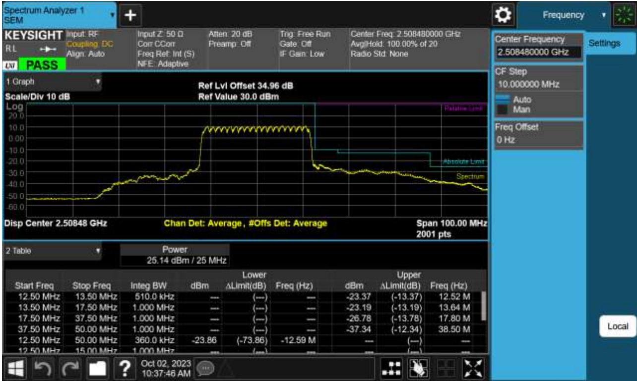
Sub6 n41. Low Channel Edge Plot (25 MHz Ch.501702 BPSK)-2
