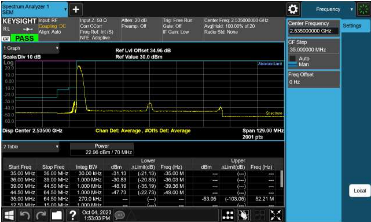
Sub6 n41. Low Channel Edge Plot (70 MHz Ch.507000 BPSK_RB1)-3
