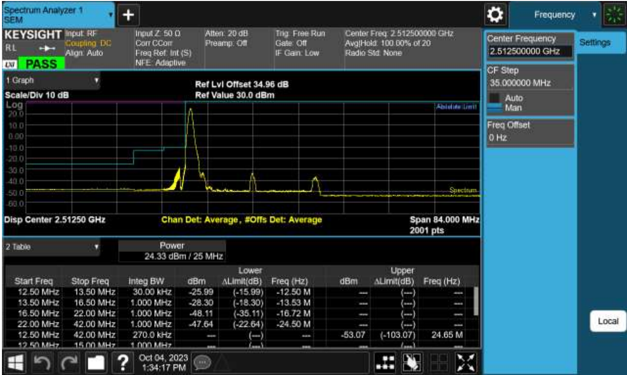
Sub6 n41. Low Channel Edge Plot (25 MHz Ch.502500 BPSK_RB 1)-3
