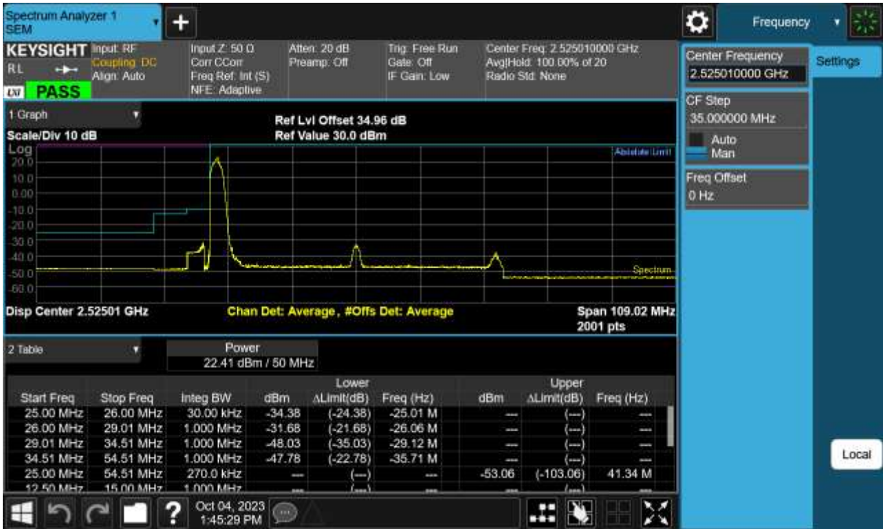
Sub6 n41. Low Channel Edge Plot (50 MHz Ch.505002 BPSK_RB1)-3
