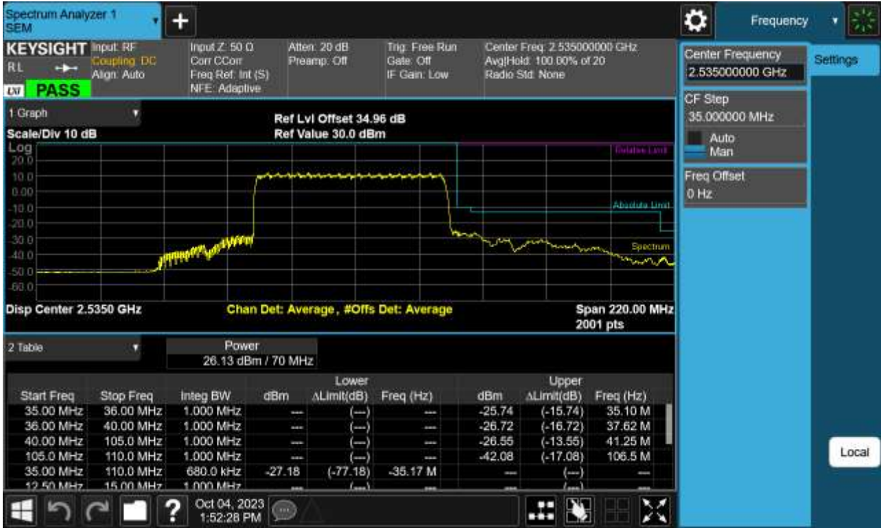
Sub6 n41. Low Channel Edge Plot (70 MHz Ch.507000 BPSK)-4
