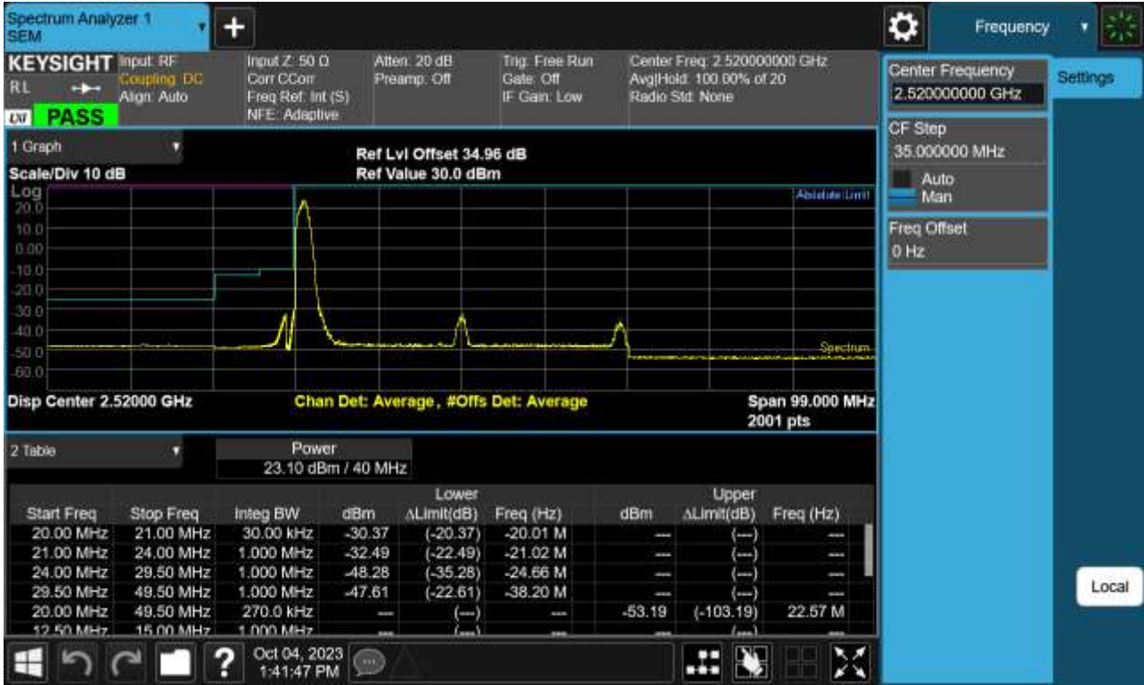
Sub6 n41. Low Channel Edge Plot (40 MHz Ch.504000 BPSK_RB1)-3
