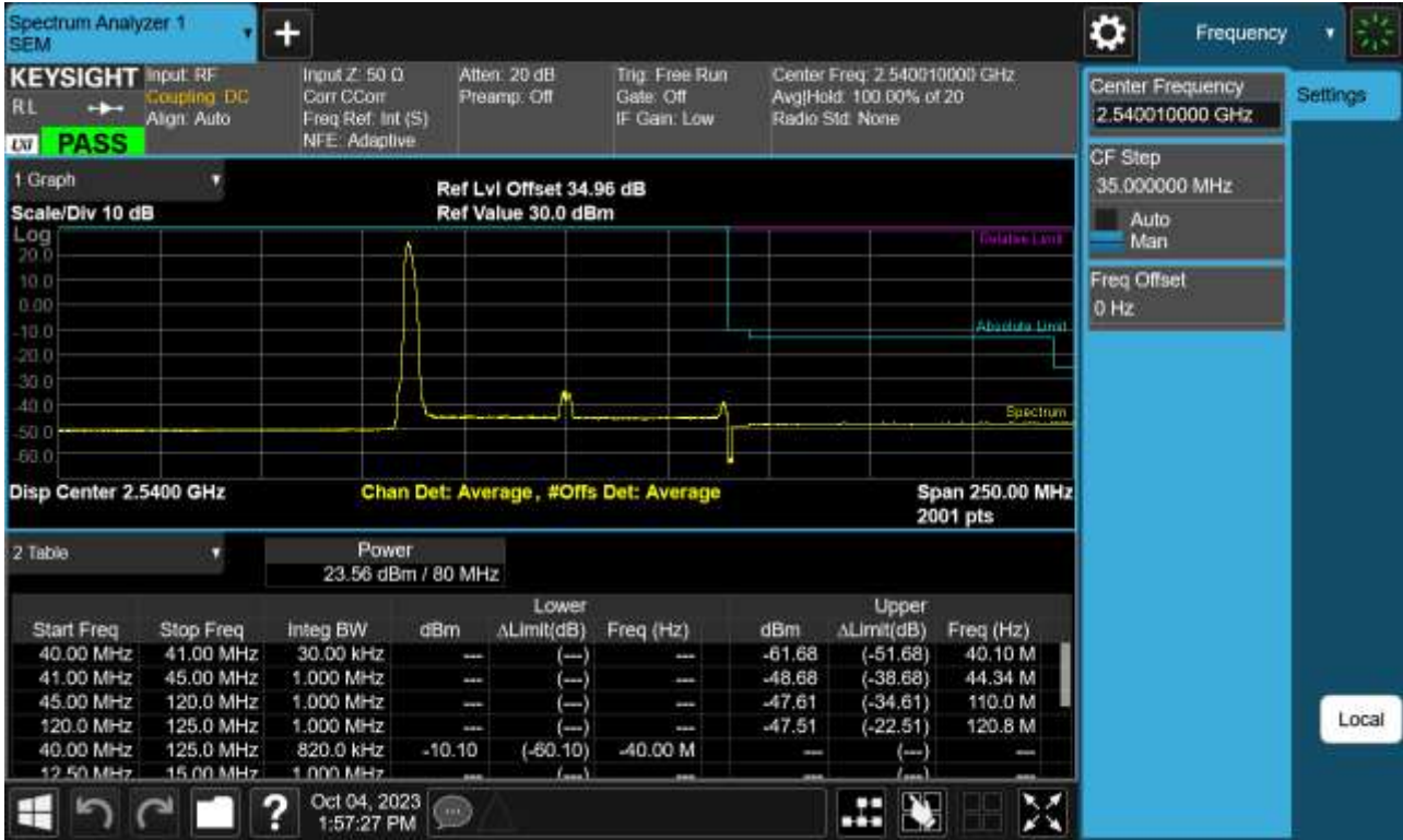
Sub6 n41. Low Channel Edge Plot (80 MHz Ch.508002 BPSK_RB1)-4
