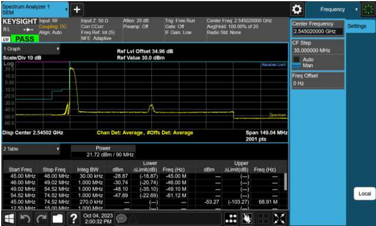
Sub6 n41. Low Channel Edge Plot (90 MHz Ch.509004 BPSK_RB1)-3
