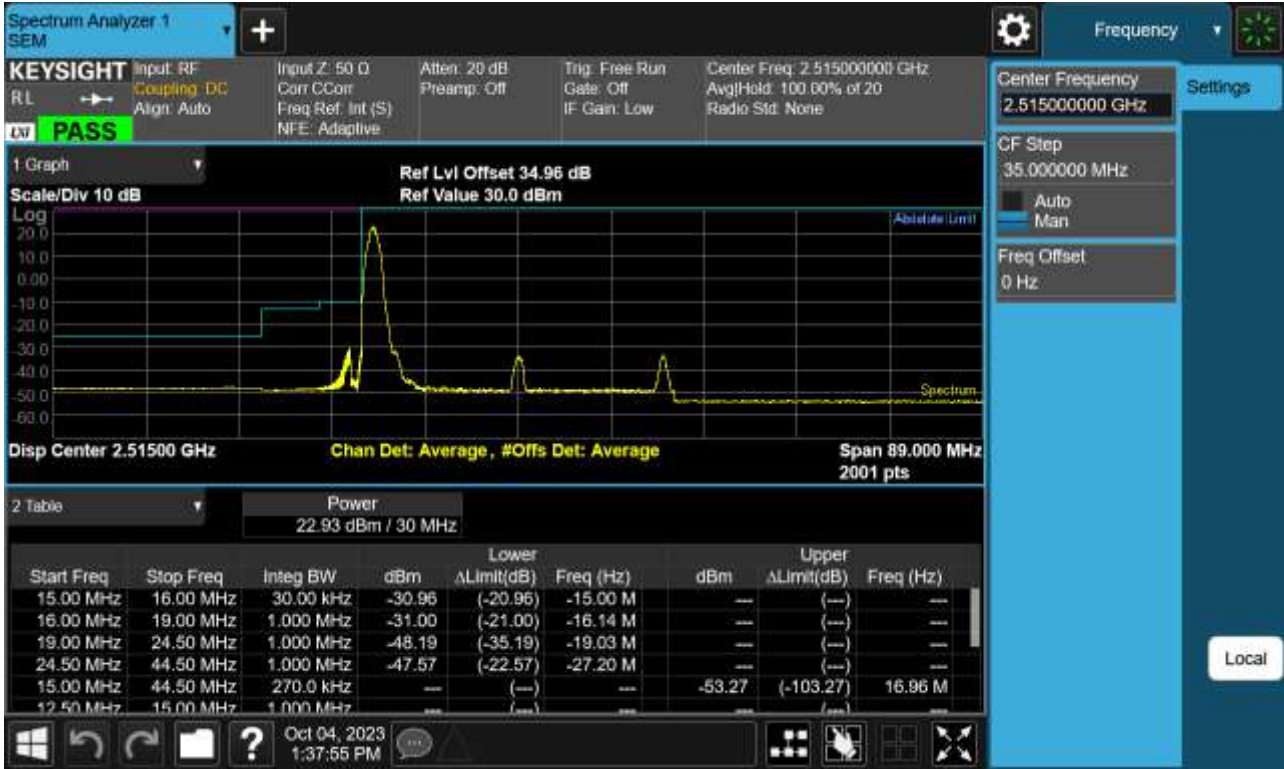
Sub6 n41. Low Channel Edge Plot (30 MHz Ch.503004 BPSK_RB1)-3
