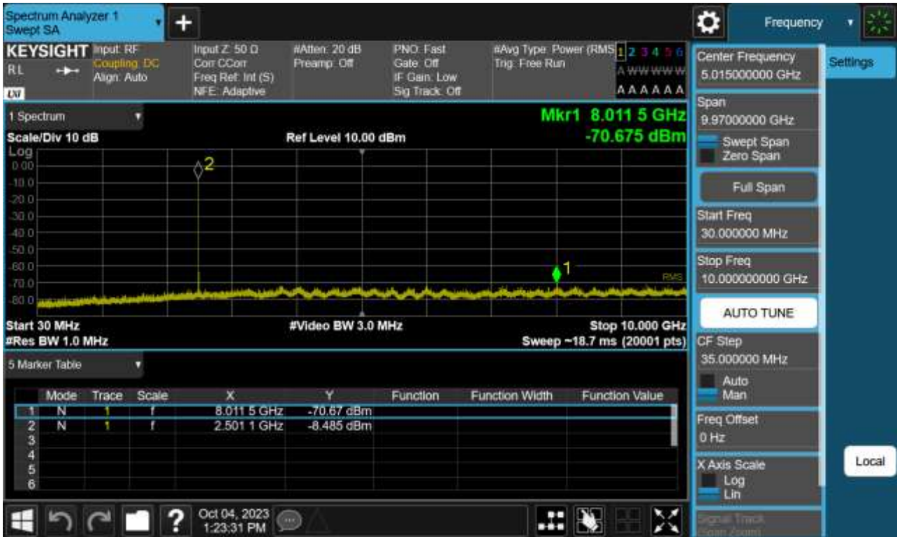
Sub6 n41. Conducted Spurious Plot 1 (15 MHz Ch.501504 BPSK RB 1)
