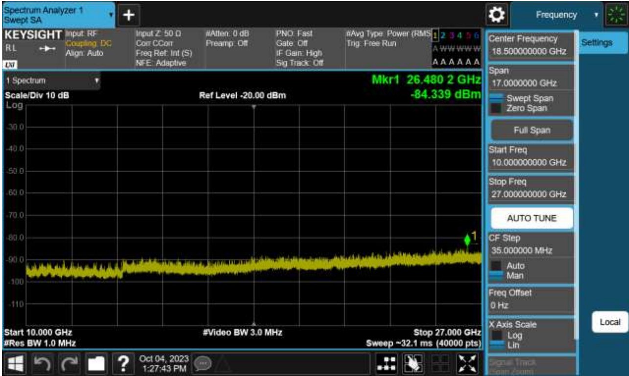
Sub6 n41. Conducted Spurious Plot 2 (20 MHz Ch.502002 BPSK RB 1)
