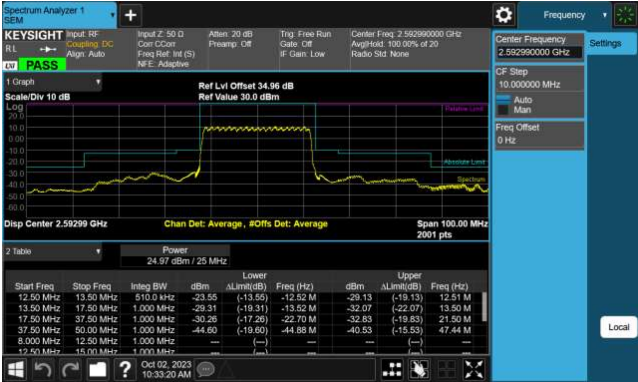
Sub6 n41. Mid Channel Edge Plot (25 MHz Ch.518598 BPSK )
