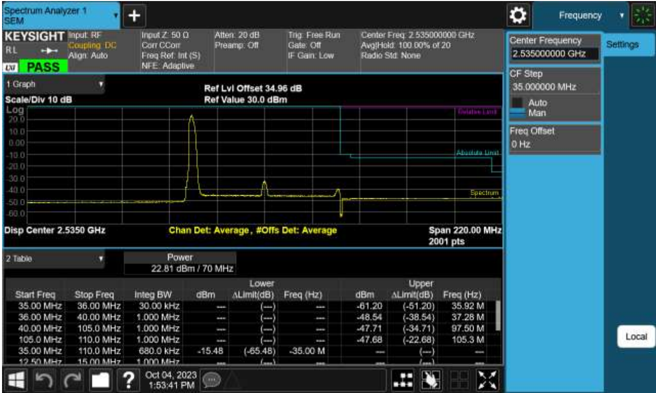
Sub6 n41. Low Channel Edge Plot (70 MHz Ch.507000 BPSK_RB1)-4
