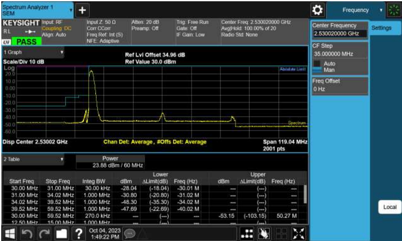
Sub6 n41. Low Channel Edge Plot (60 MHz Ch.506004 BPSK_RB1)-3
