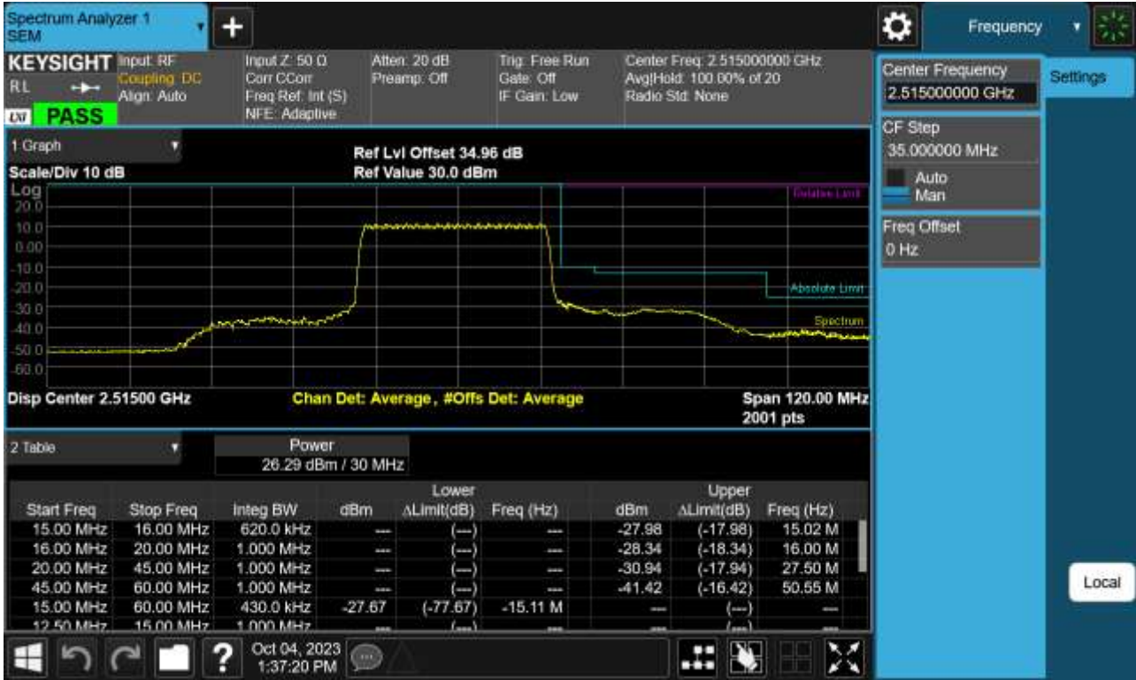
Sub6 n41. Low Channel Edge Plot (30 MHz Ch.503004 BPSK)-4
