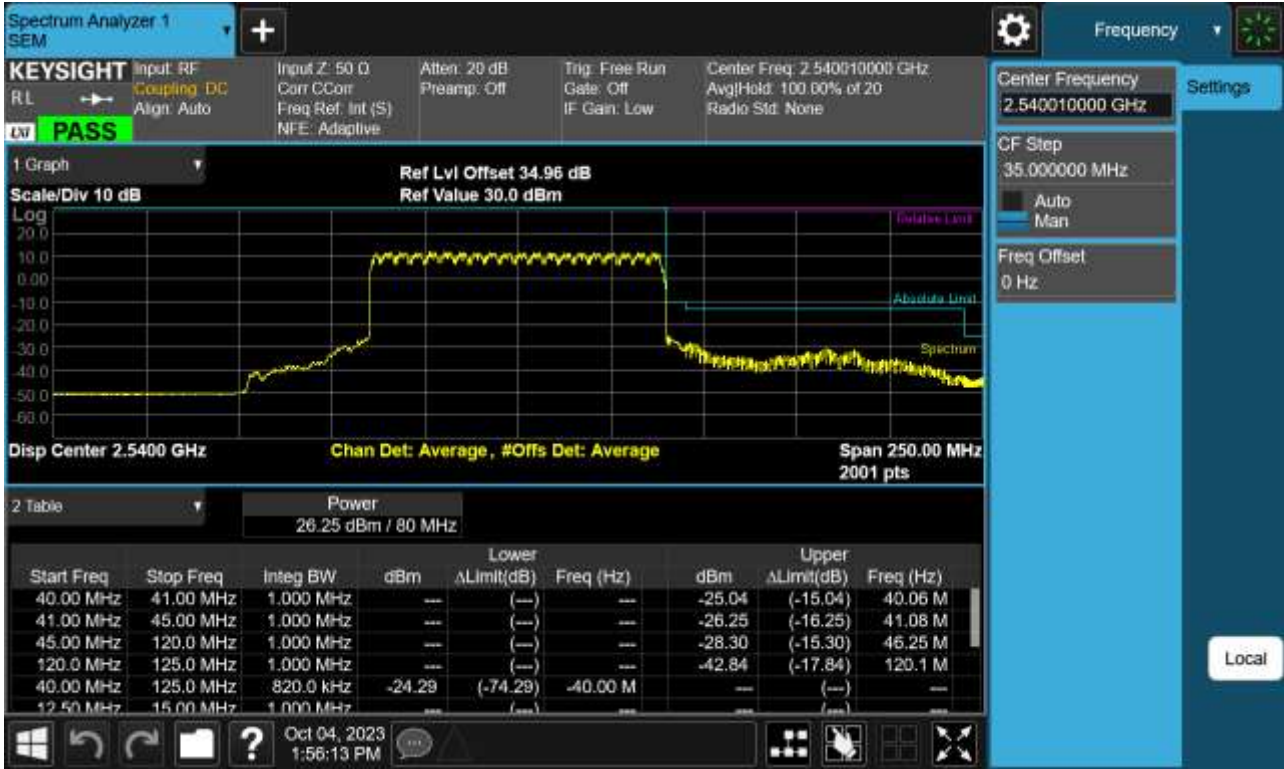
Sub6 n41. Low Channel Edge Plot (80 MHz Ch.508002 BPSK)-4
