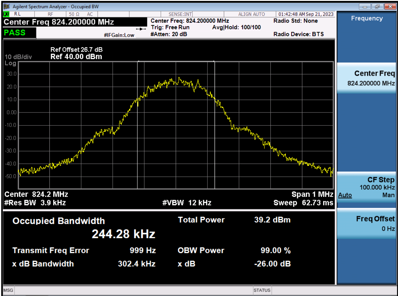
■ GSM850 MODE (128 CH.) Occupied Bandwidth
