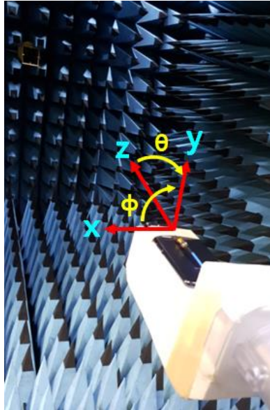
Figure 1: Geometry for SM-S926U for Radiation patterns.
