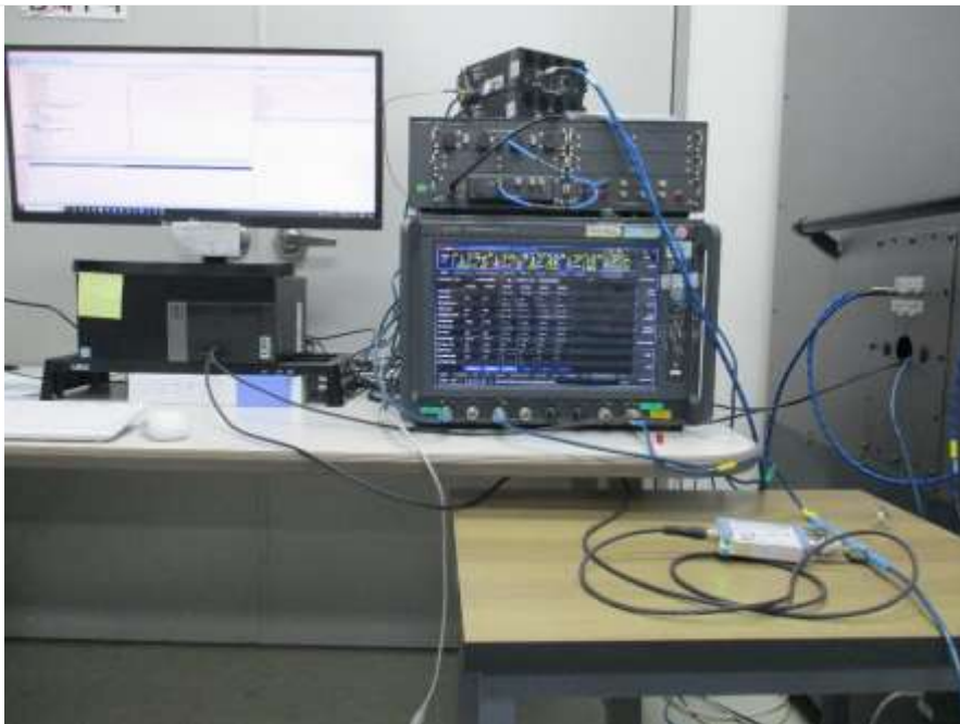
Test setup photo-10 (9-1(b)) mmW NR radiated power measurement
