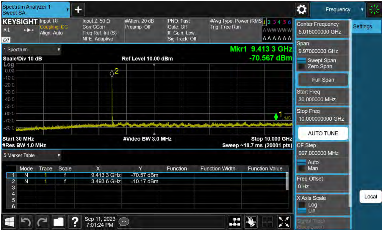
Sub6 n77(78). Conducted Spurious Plot_1 (633334ch_15 MHz_BPSK)
