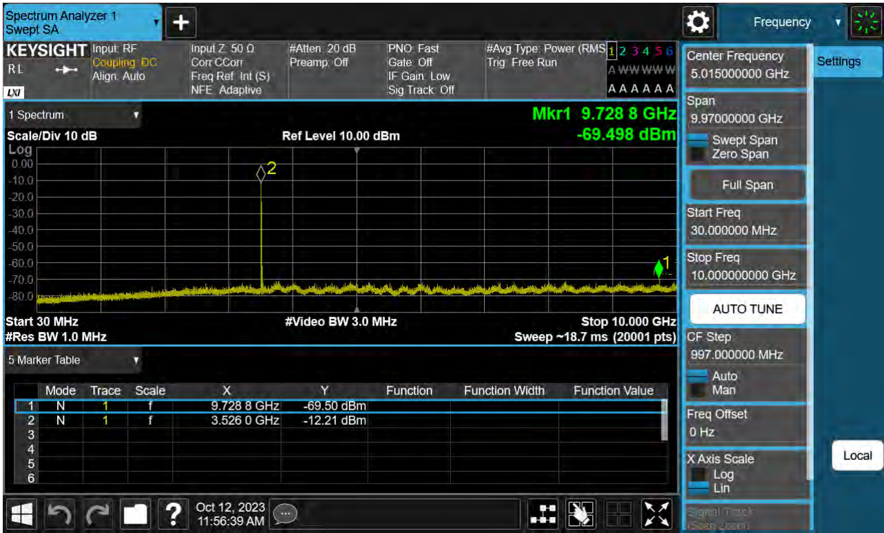
Sub6 n77(78). Conducted Spurious Plot_1 (635834ch_25 MHz_BPSK)
