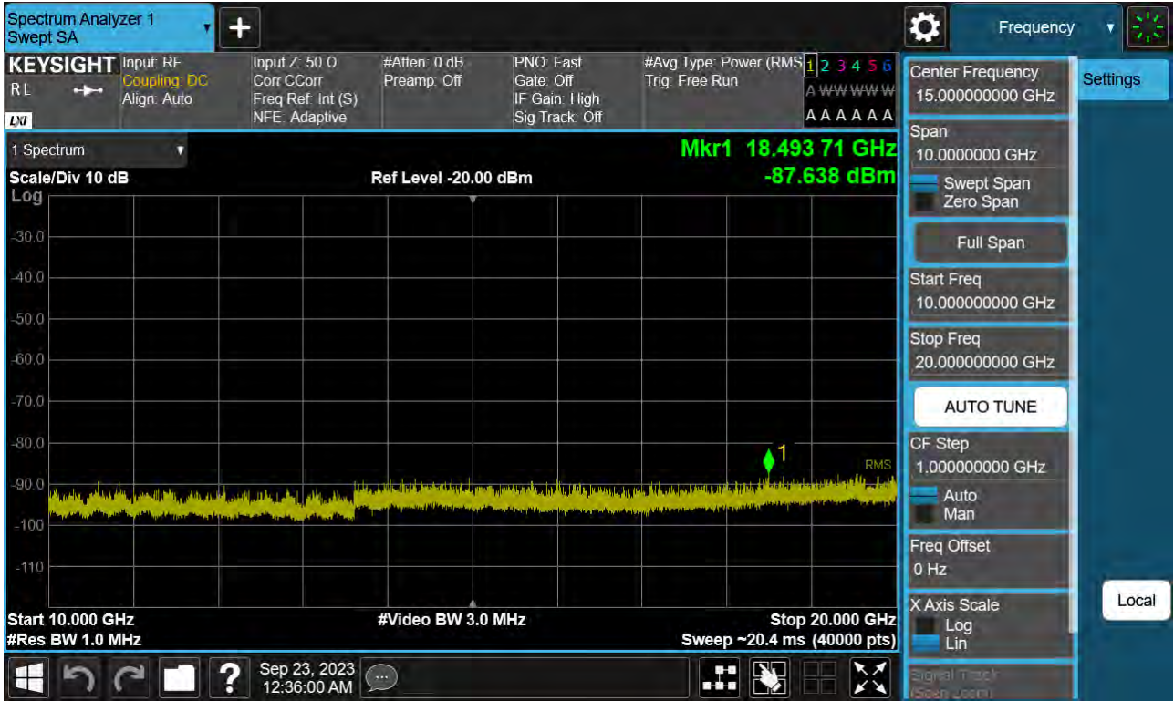
Sub6 n66. Conducted Spurious Plot_2 (352000ch_40 MHz_BPSK_RB 1_1)
