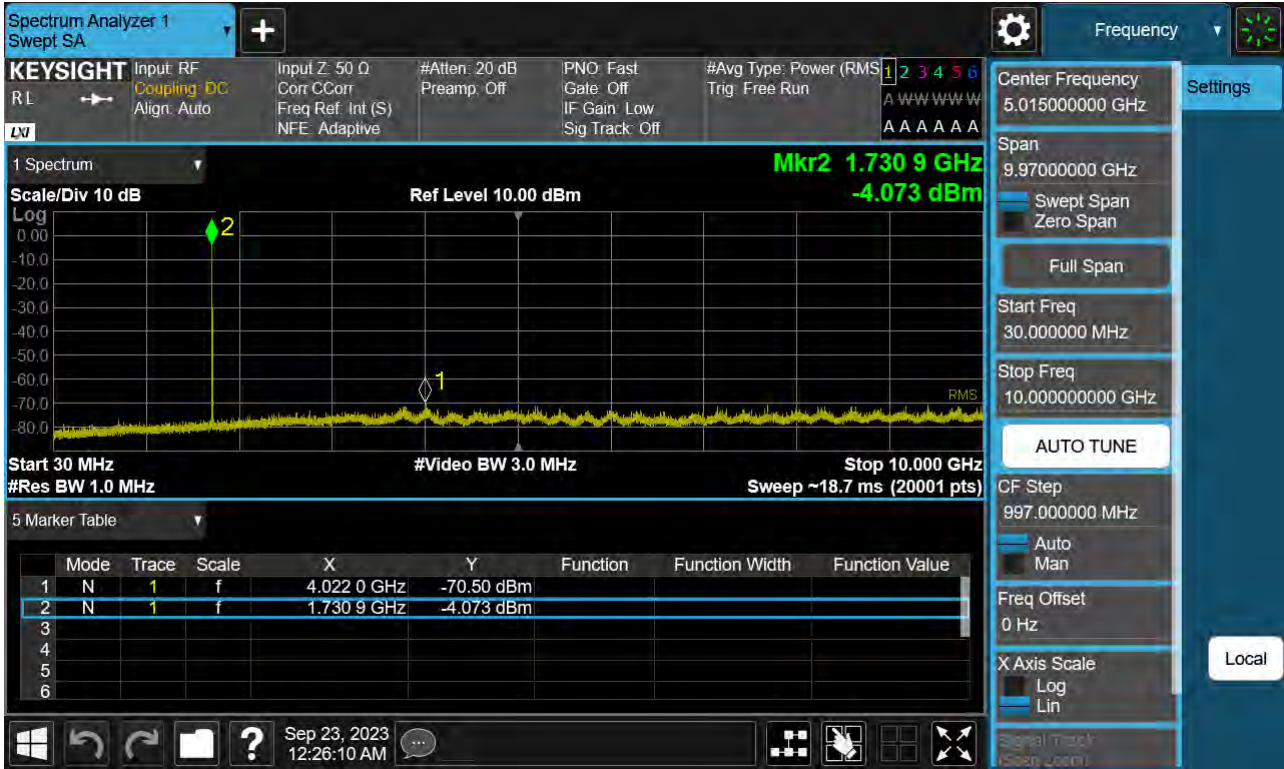
Sub6 n66. Conducted Spurious Plot_1 (349000ch_30 MHz_BPSK_RB 1_1)
