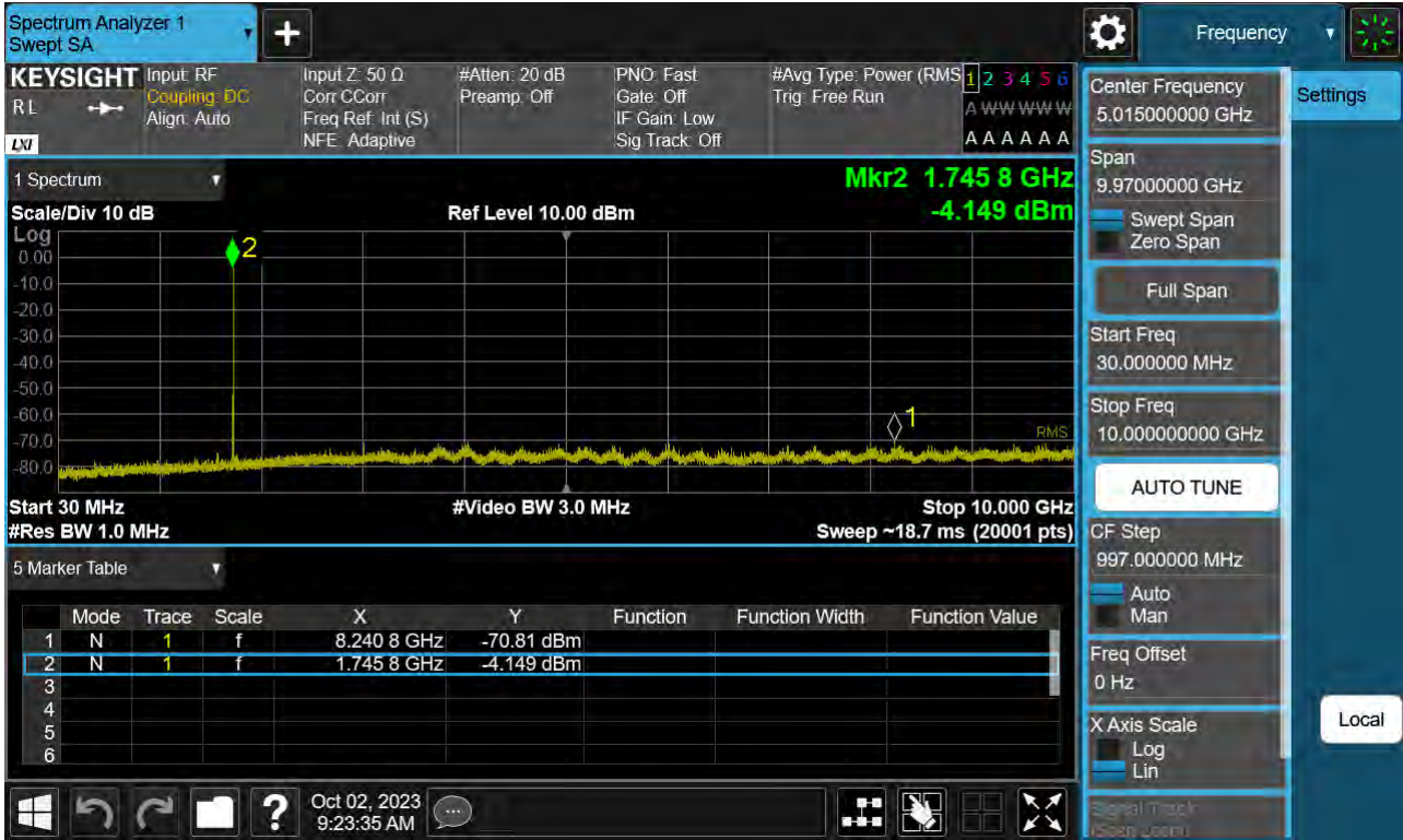
Sub6 n66. Conducted Spurious Plot_1 (352500ch_35 MHz_BPSK_RB 1_1)
