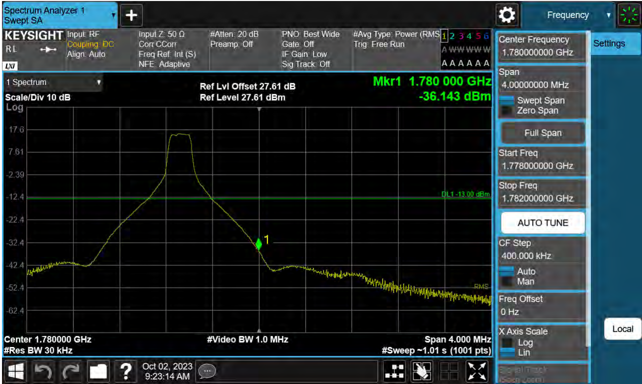
Sub6 n66. Upper Band Edge Plot (35 M BW Ch.352500 BPSK_RB1_Offset 105) -1
