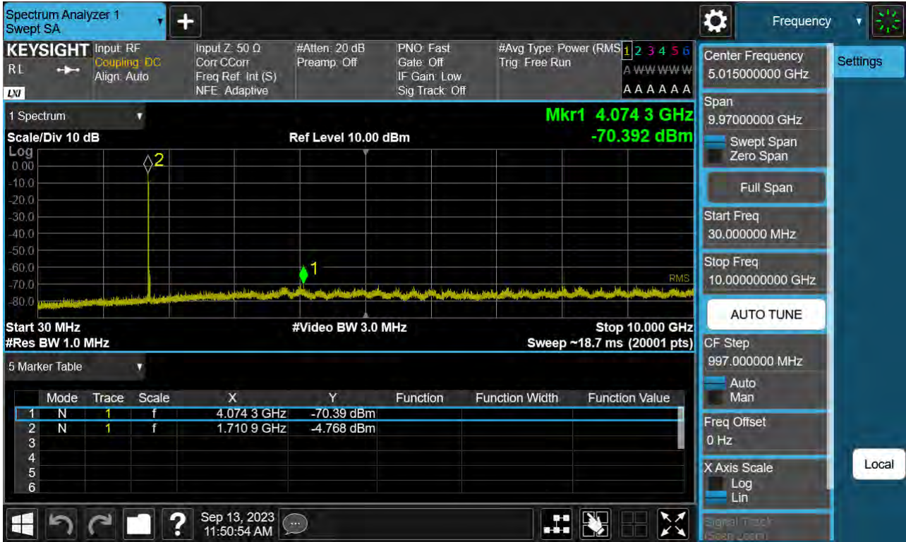
Sub6 n66. Conducted Spurious Plot_1 (344500ch_25 MHz_BPSK_RB 1_1)
