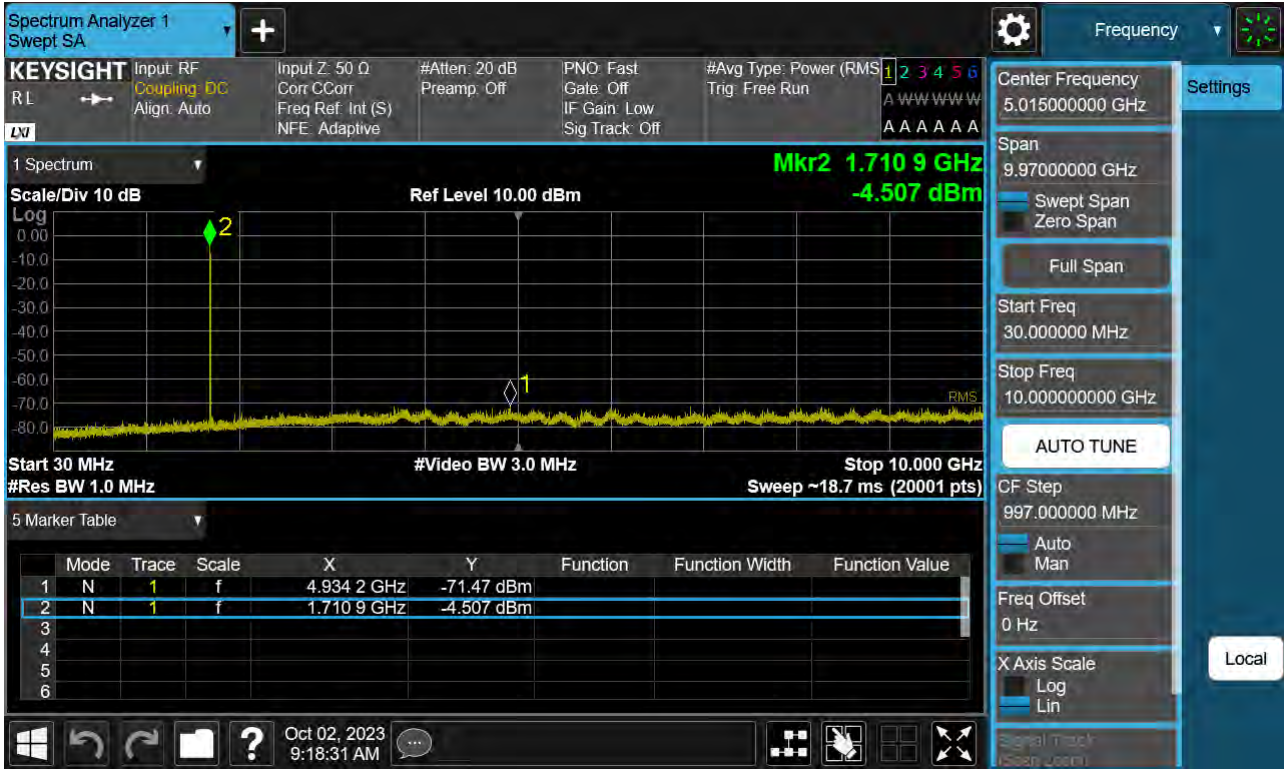
Sub6 n66. Conducted Spurious Plot_1 (345500ch_35 MHz_BPSK_RB 1_1)
