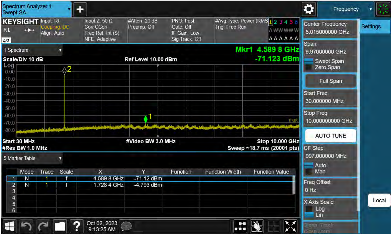
Sub6 n66. Conducted Spurious Plot_1 (349000ch_35 MHz_BPSK_RB 1_1)
