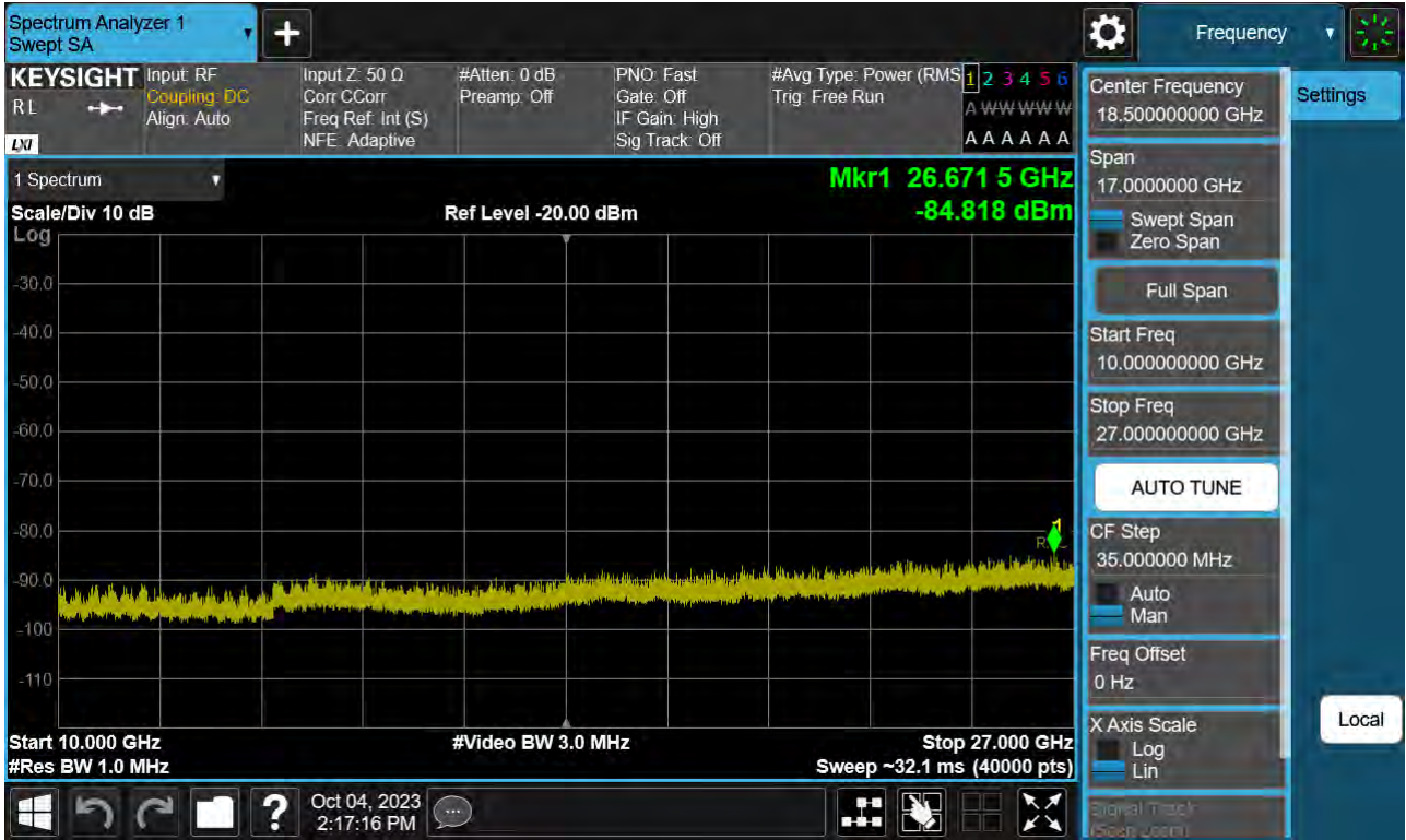
Sub6 n41. Conducted Spurious Plot 2 (15 MHz Ch.501504 BPSK RB 1)
