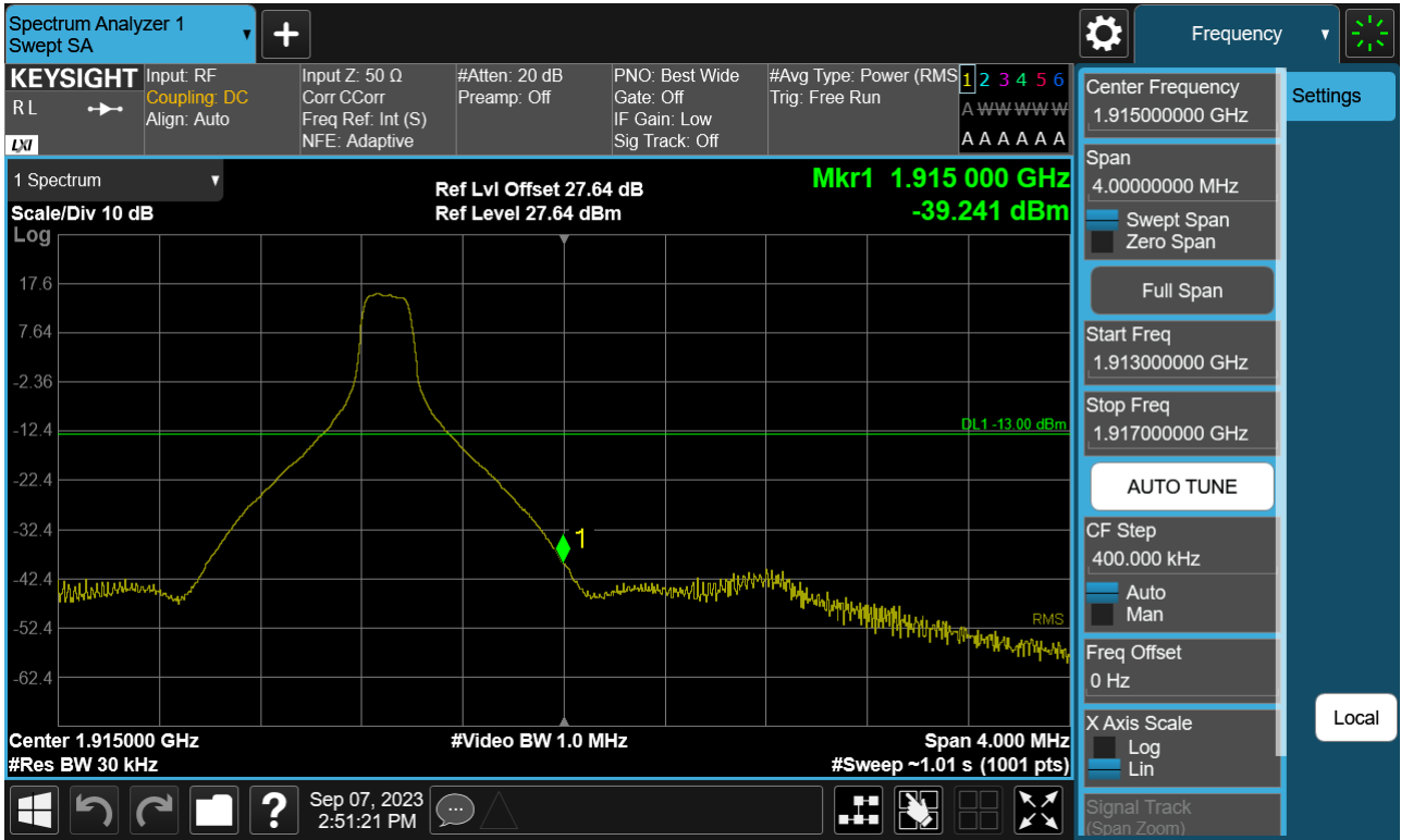
Sub6 n25. Upper Band Edge Plot (30 M BW Ch.380000 BPSK_RB1_Offset 159)
