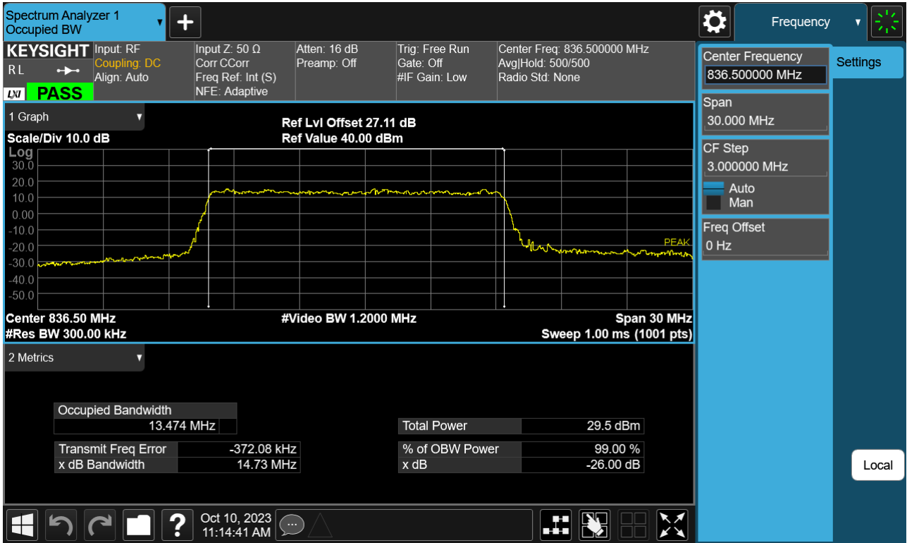
Sub6 n5. Occupied Bandwidth Plot (15 M BW Ch.167300 64QAM RB 75_0)
