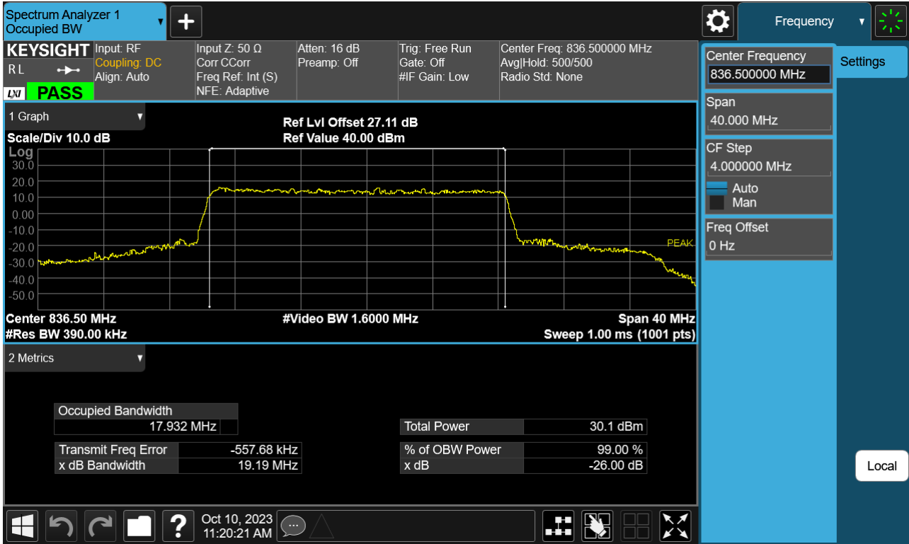
Sub6 n5. Occupied Bandwidth Plot (20 M BW Ch.167300 16QAM RB 100_0)
