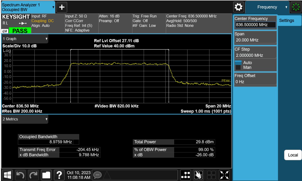
Sub6 n5. Occupied Bandwidth Plot (10 M BW Ch.167300 16QAM_RB 50_0)
