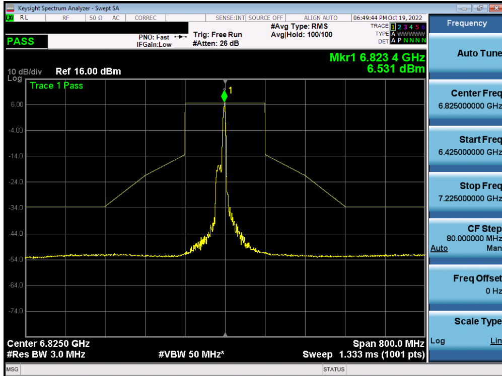
Plot 7-487. In-Band Emission Plot MIMO ANT1 (160MHz BW 802.11ax (26 Tones) (UNII Band 7) – Ch. 175) – SP
