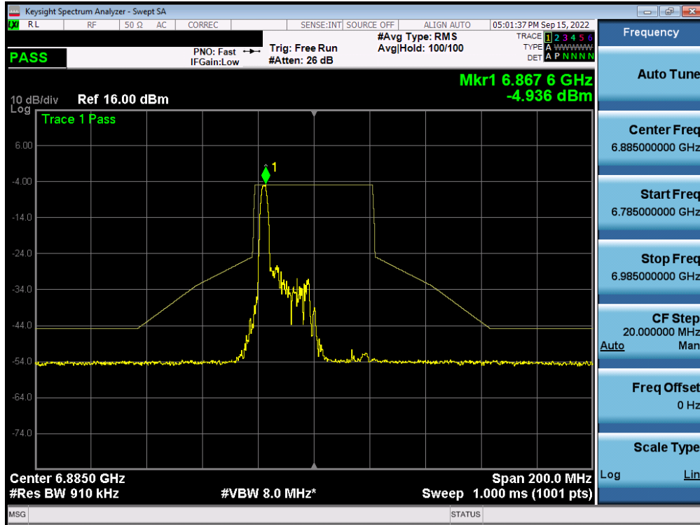
Plot 7-459. In-Band Emission Plot MIMO ANT1 (40MHz BW 802.11ax (26 Tones) (UNII Band 8) – Ch. 187) – LPI
