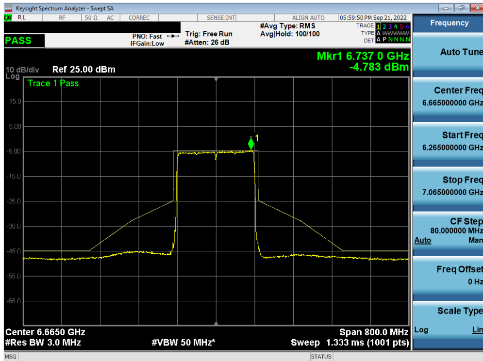
Plot 7-517. In-Band Emission Plot MIMO ANT1 (160MHz BW 802.11ax (Full Tone) (UNII Band 7) – Ch. 143) – LPI/SP
