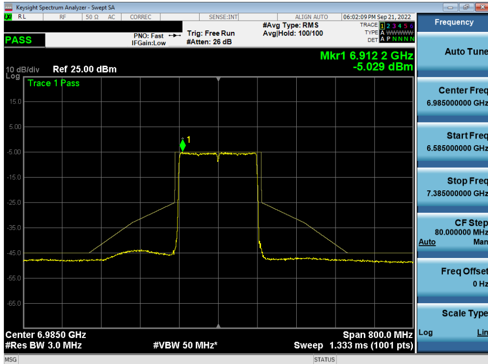
Plot 7-527. In-Band Emission Plot MIMO ANT1 (160MHz BW 802.11ax (Full Tone) (UNII Band 8) – Ch. 207) – LPI
