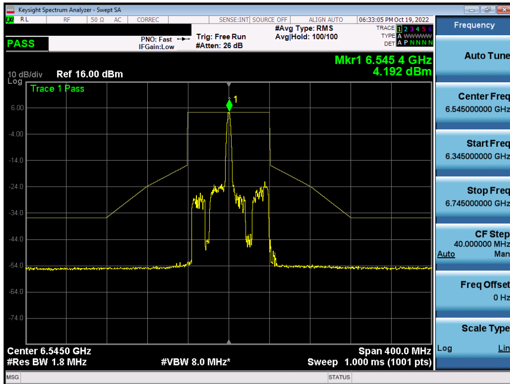
Plot 7-483. In-Band Emission Plot MIMO ANT1 (80MHz BW 802.11ax (26 Tones) (UNII Band 7) – Ch. 119) – SP
