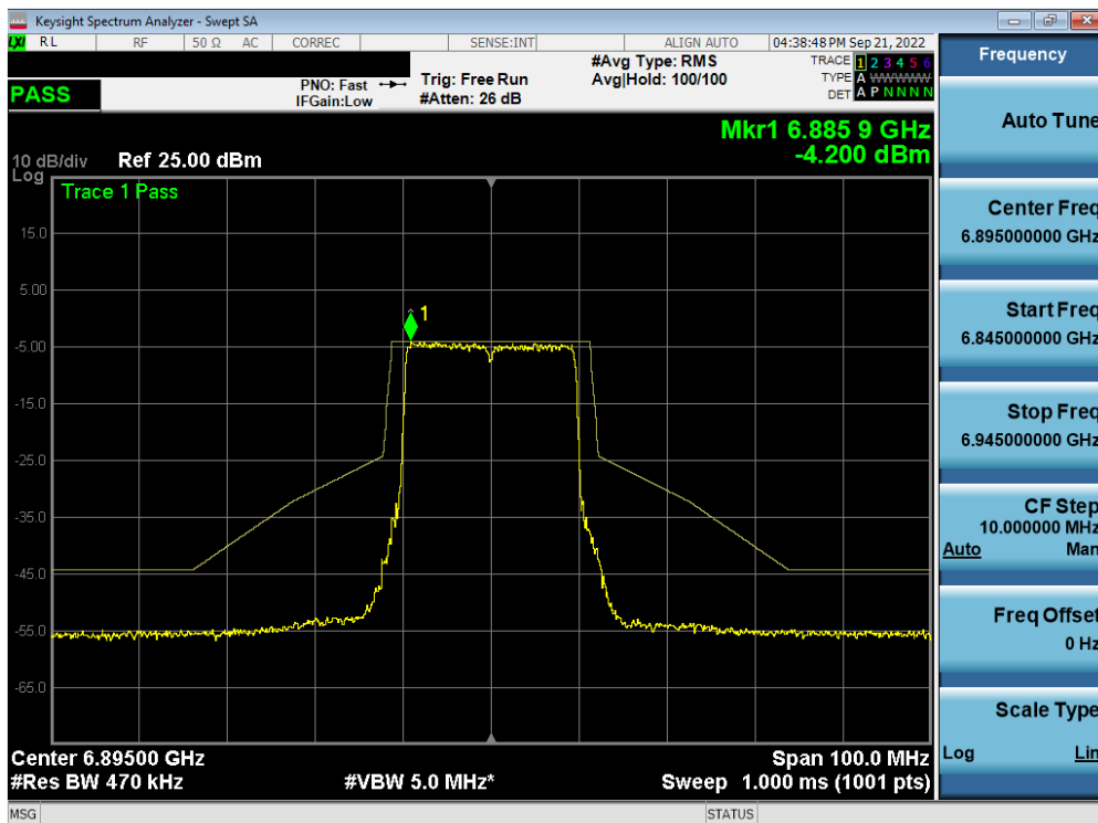
Plot 7-519. In-Band Emission Plot MIMO ANT1 (20MHz BW 802.11ax (Full Tone) (UNII Band 8) – Ch. 189) – LPI
