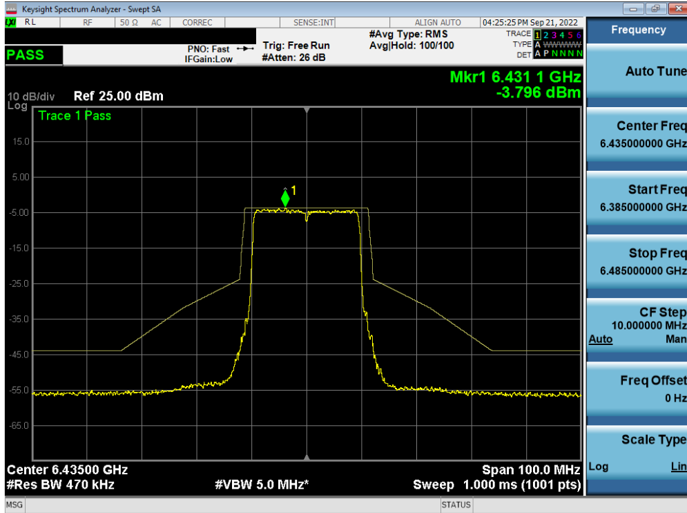
Plot 7-500. In-Band Emission Plot MIMO ANT1 (20MHz BW 802.11ax (Full Tone) (UNII Band 6) – Ch. 97) – LPI
