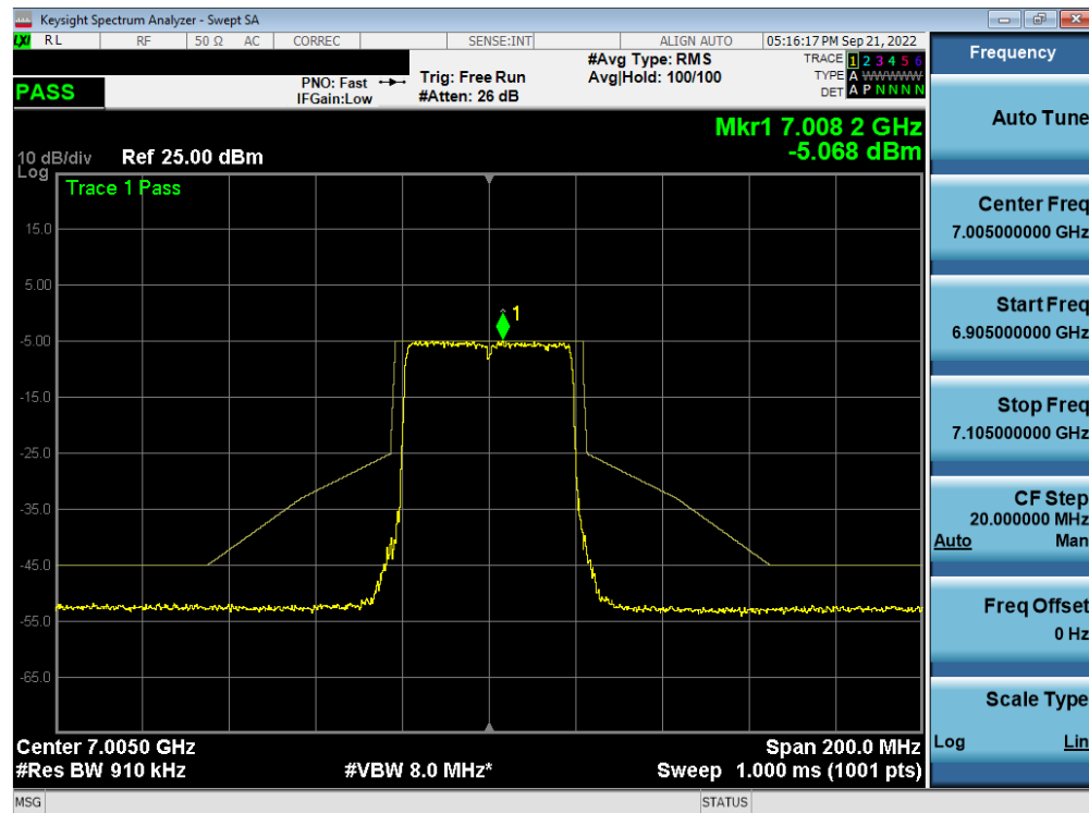
Plot 7-523. In-Band Emission Plot MIMO ANT1 (40MHz BW 802.11ax (Full Tone) (UNII Band 8) – Ch. 211) – LPI
