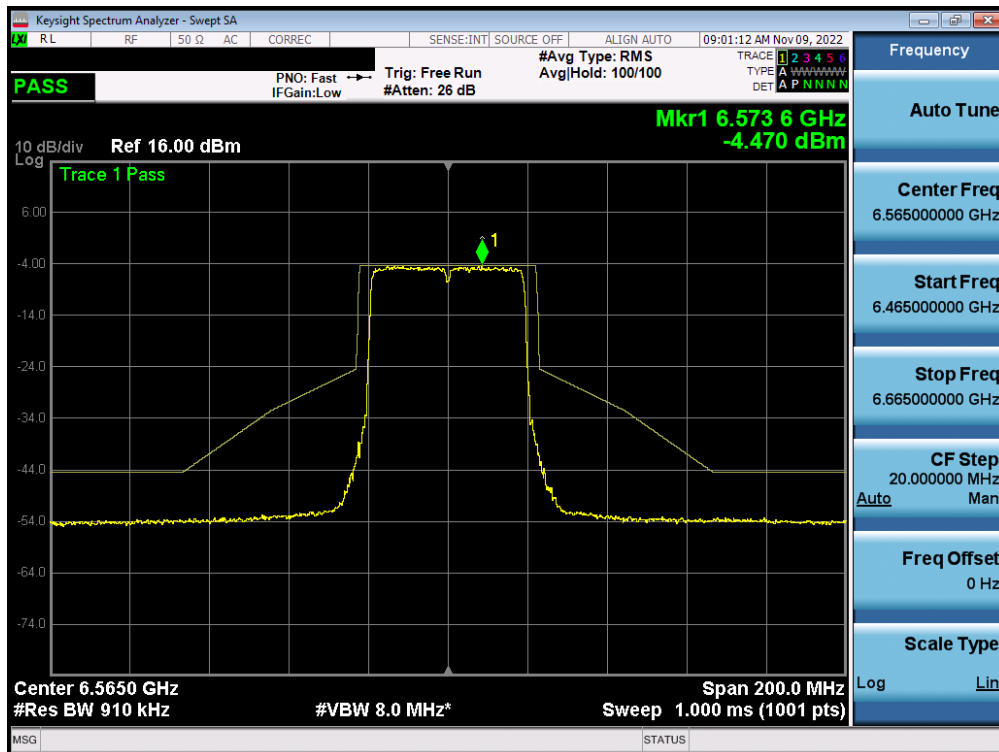
Plot 7-511. In-Band Emission Plot MIMO ANT1 (40MHz BW 802.11ax (Full Tone) (UNII Band 7) – Ch. 123) – LPI/SP
