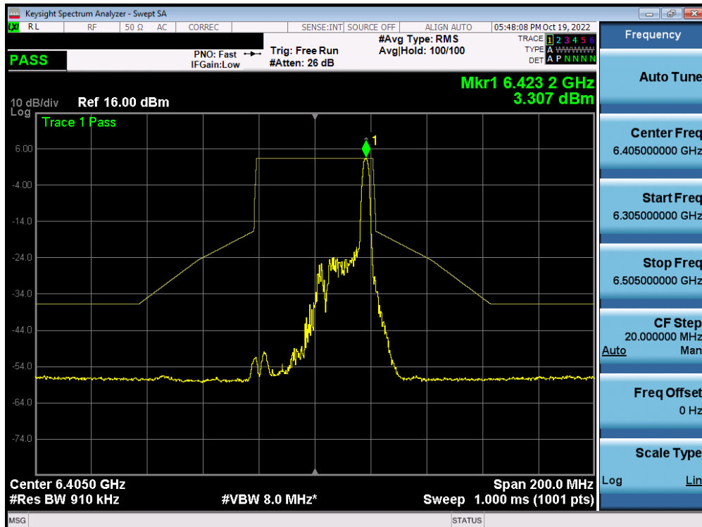
Plot 7-470. In-Band Emission Plot MIMO ANT1 (40MHz BW 802.11ax (26 Tones) (UNII Band 5) – Ch. 91) - SP
