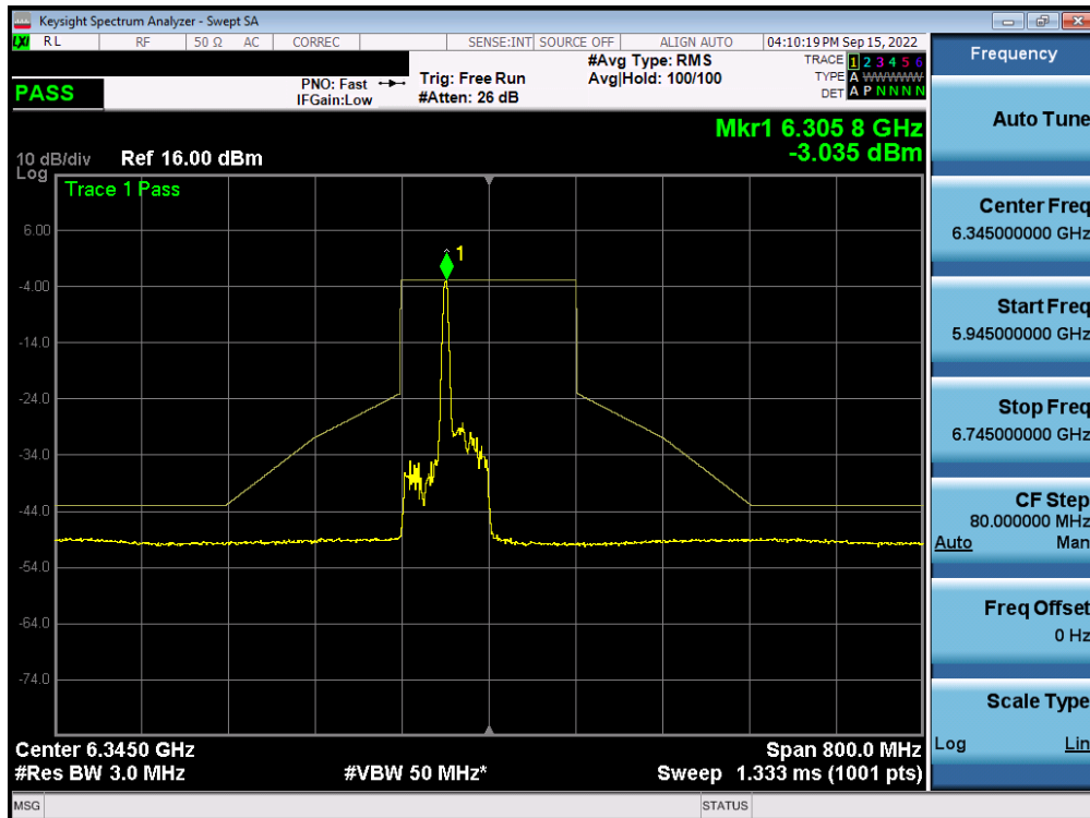
Plot 7-539. In-Band Emission Plot MIMO ANT2 (160MHz BW 802.11ax (26 Tones) (UNII Band 5) – Ch. 79) – LPI
