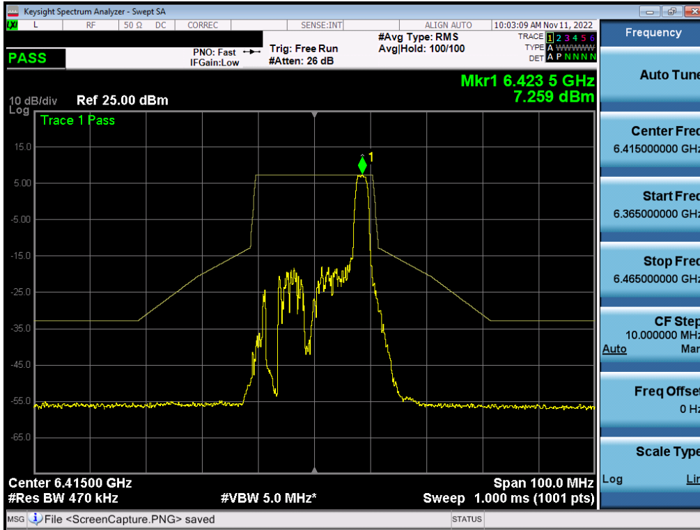
Plot 7-467. In-Band Emission Plot MIMO ANT1 (20MHz BW 802.11ax (26 Tones) UNII Band 5) – Ch. 93) - SP
