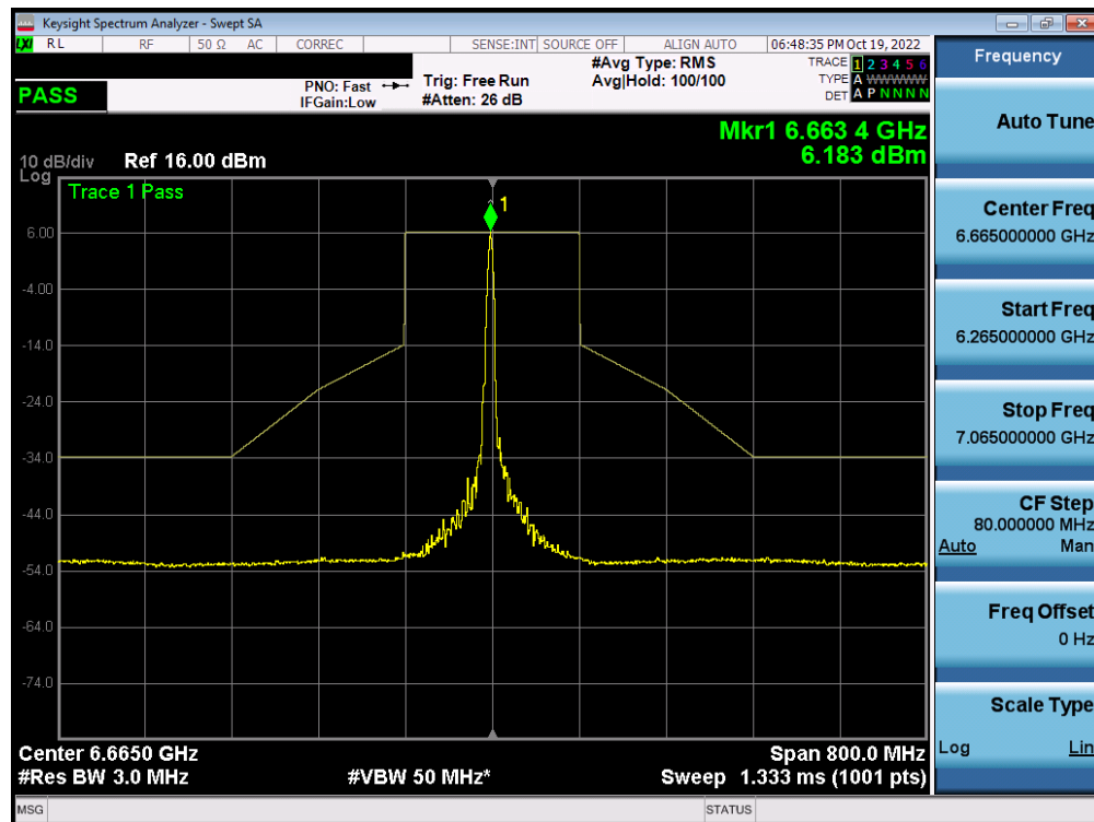
Plot 7-486. In-Band Emission Plot MIMO ANT1 (160MHz BW 802.11ax (26 Tones) (UNII Band 7) – Ch. 143) – SP
