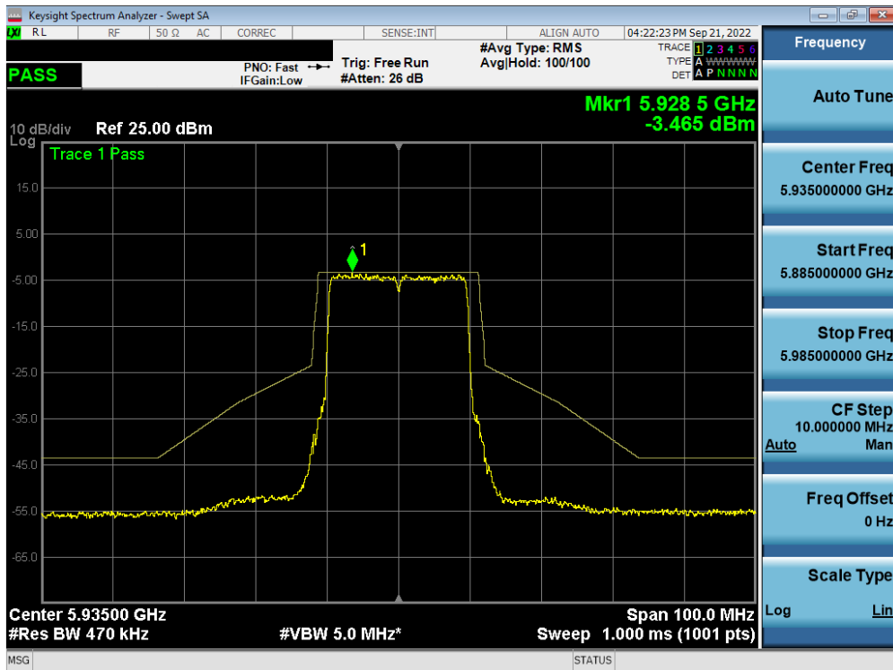
Plot 7-488. In-Band Emission Plot MIMO ANT1 (20MHz BW 802.11ax (Full Tone) UNII Band 5) – Ch. 2 – LPI
