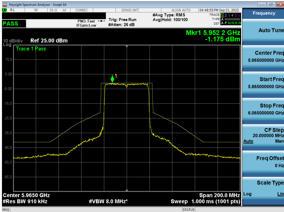
Plot 7-491. In-Band Emission Plot MIMO ANT1 (40MHz BW 802.11ax (Full Tone) (UNII Band 5) – Ch. 3) – LPI/SP
