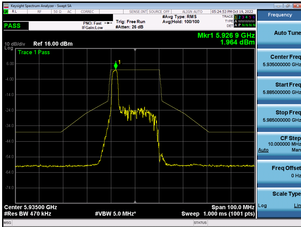
Plot 7-465. In-Band Emission Plot MIMO ANT1 (20MHz BW 802.11ax (26 Tones) UNII Band 5) – Ch. 2 - SP
