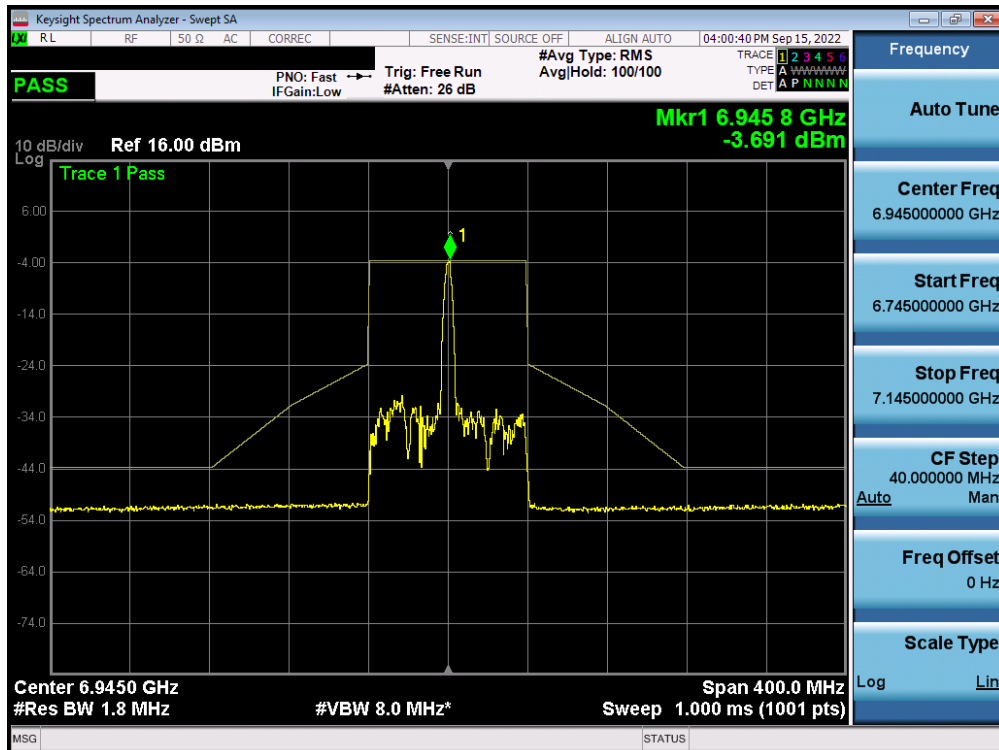
Plot 7-565. In-Band Emission Plot MIMO ANT2 (80MHz BW 802.11ax (26 Tones) (UNII Band 8) – Ch. 199) – LPI
