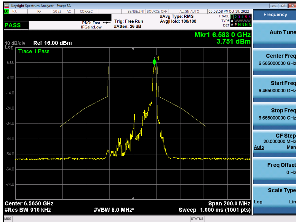
Plot 7-480. In-Band Emission Plot MIMO ANT1 (40MHz BW 802.11ax (26 Tones) (UNII Band 7) – Ch. 123) – SP
