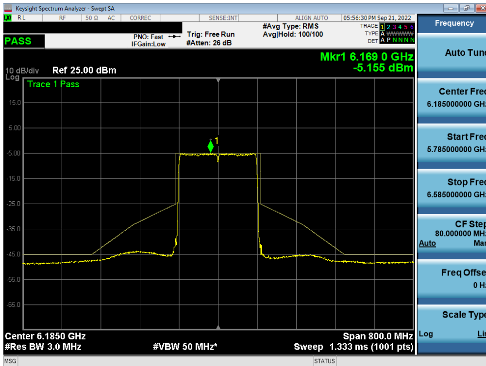
Plot 7-498. In-Band Emission Plot MIMO ANT1 160MHz BW 802.11ax (Full Tone) (UNII Band 5) – Ch. 47) – LPI/SP
