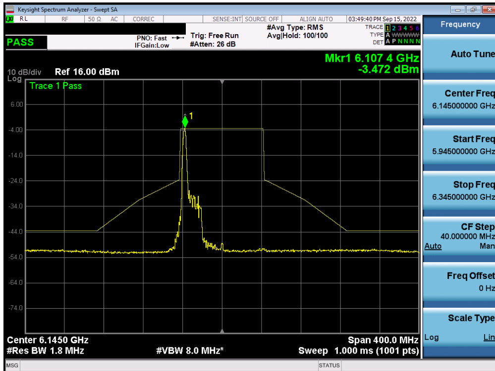
Plot 7-535. In-Band Emission Plot MIMO ANT2 (80MHz BW 802.11ax (26 Tones) (UNII Band 5) – Ch. 39) – LPI
