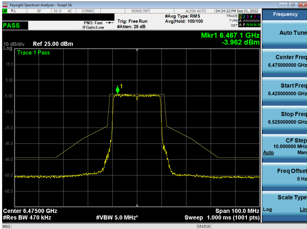
Plot 7-501. In-Band Emission Plot MIMO ANT1 (20MHz BW 802.11ax (Full Tone) (UNII Band 6) – Ch. 105) – LPI
