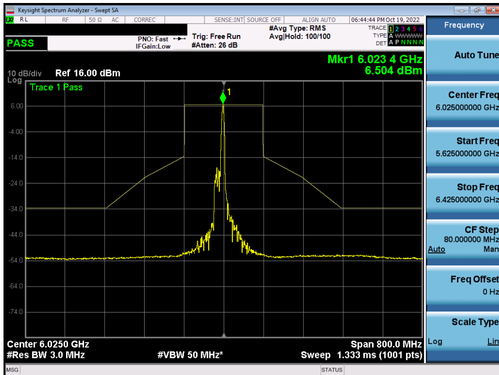
Plot 7-474. In-Band Emission Plot MIMO ANT1 (160MHz BW 802.11ax (26 Tones) (UNII Band 5) – Ch. 15) - SP
