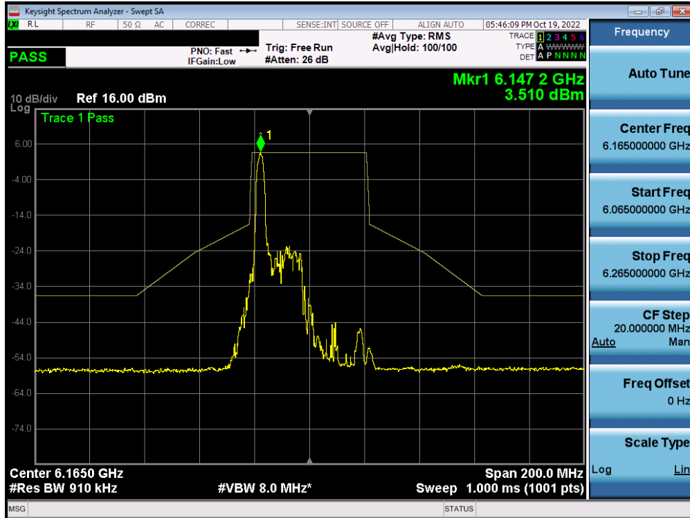
Plot 7-469. In-Band Emission Plot MIMO ANT1 (40MHz BW 802.11ax (26 Tones) (UNII Band 5) – Ch. 43) - SP
