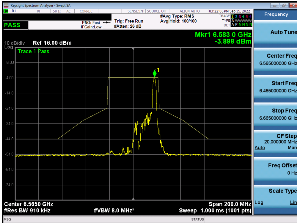
Plot 7-551. In-Band Emission Plot MIMO ANT2 (40MHz BW 802.11ax (26 Tones) (UNII Band 7) – Ch. 123) – LPI
