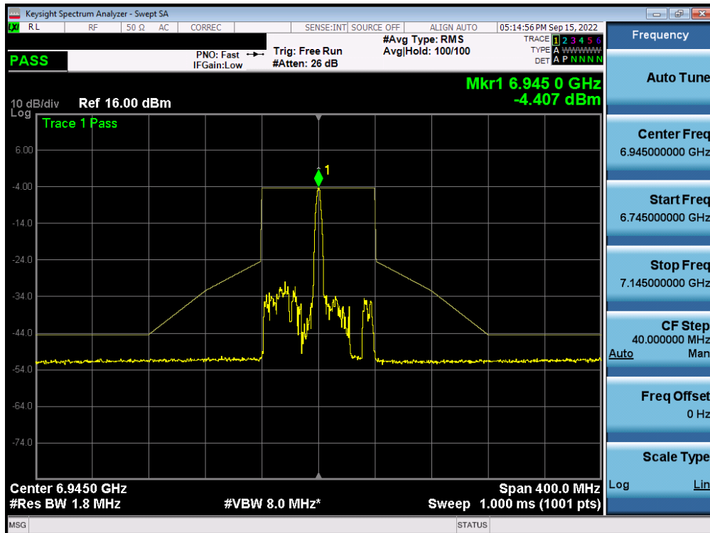
Plot 7-462. In-Band Emission Plot MIMO ANT1 (80MHz BW 802.11ax (26 Tones) (UNII Band 8) – Ch. 199) – LPI
