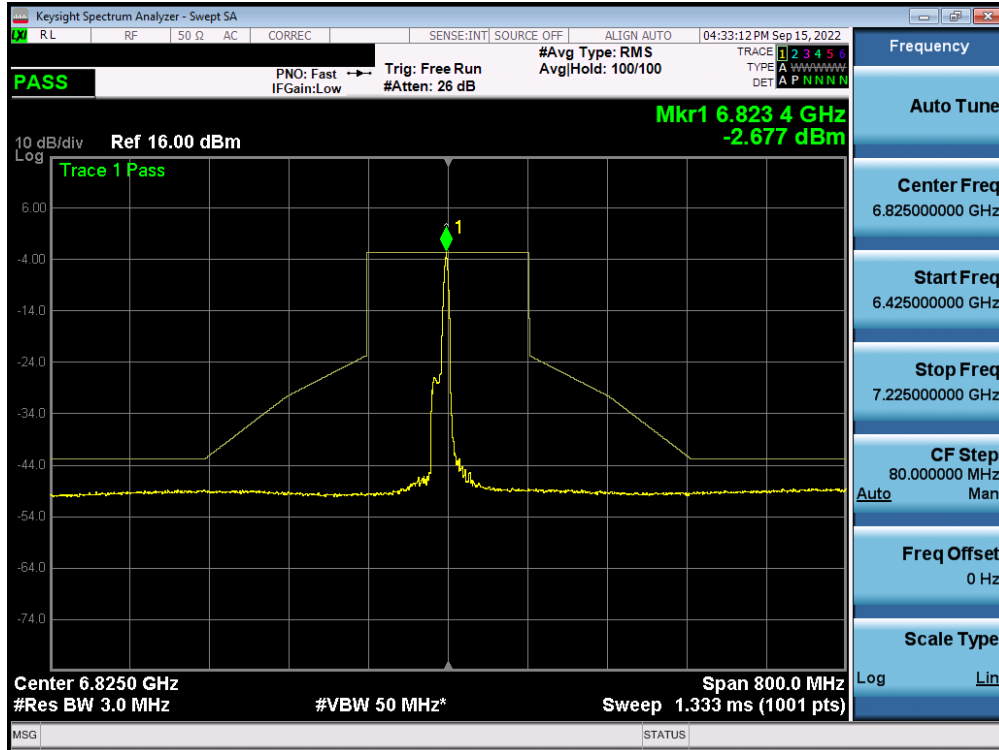
Plot 7-455. In-Band Emission Plot MIMO ANT1 (160MHz BW 802.11ax (26 Tones) (UNII Band 7) – Ch. 175) – LPI
