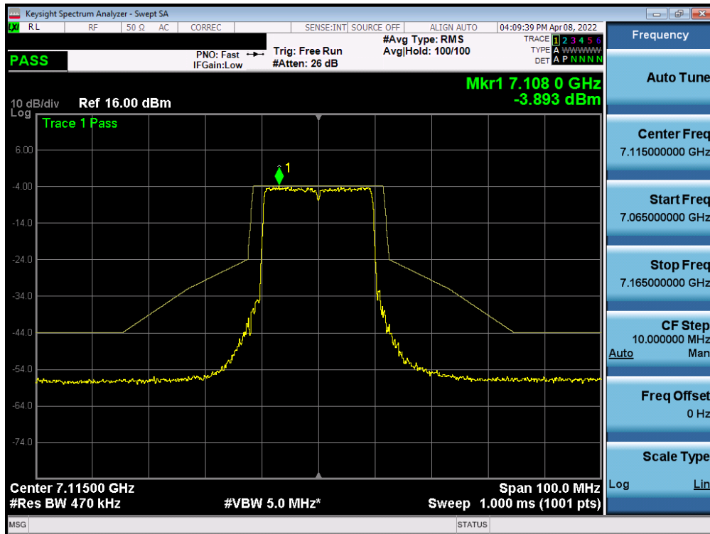
Plot 7-521. In-Band Emission Plot MIMO ANT1 (20MHz BW 802.11ax (Full Tone) (UNII Band 8) – Ch. 233) – LPI
