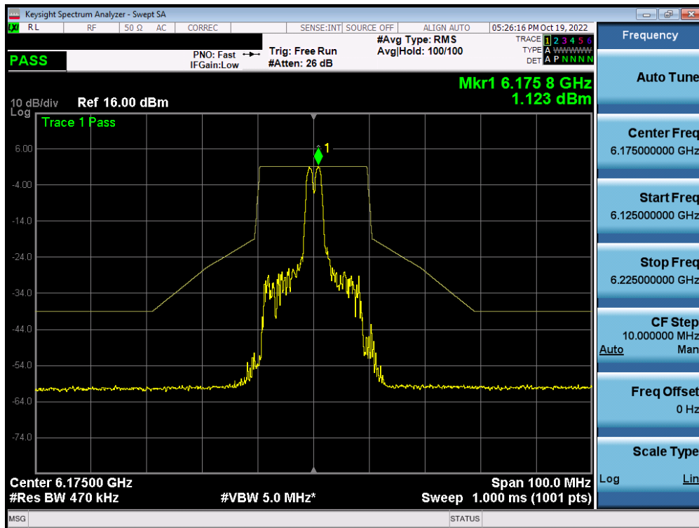
Plot 7-466. In-Band Emission Plot MIMO ANT1 (20MHz BW 802.11ax (26 Tones) (UNII Band 5) – Ch. 45) - SP
