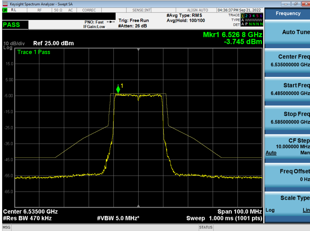
Plot 7-508. In-Band Emission Plot MIMO ANT1 (20MHz BW 802.11ax (Full Tone) (UNII Band 7) – Ch. 117) – LPI/SP
