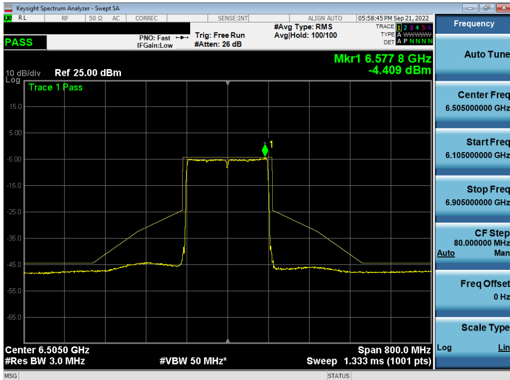
Plot 7-507. In-Band Emission Plot MIMO ANT1 (160MHz BW 802.11ax (Full Tone) (UNII Band 6) – Ch. 111) – LPI
