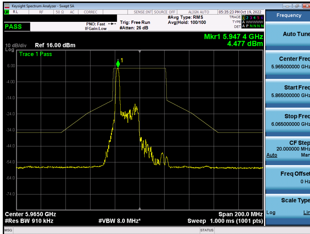
Plot 7-468. In-Band Emission Plot MIMO ANT1 (40MHz BW 802.11ax (26 Tones) (UNII Band 5) – Ch. 3) - SP
