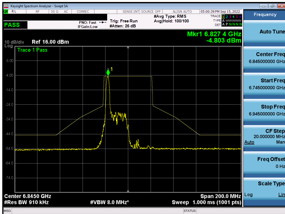
Plot 7-553. In-Band Emission Plot MIMO ANT2 (40MHz BW 802.11ax (26 Tones) (UNII Band 7) – Ch. 179) – LPI
