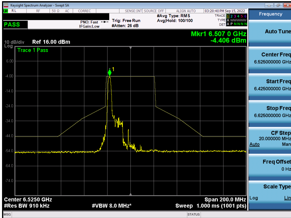
Plot 7-545. In-Band Emission Plot MIMO ANT2 (40MHz BW 802.11ax (26 Tones) (UNII Band 6) – Ch. 115) – LPI
