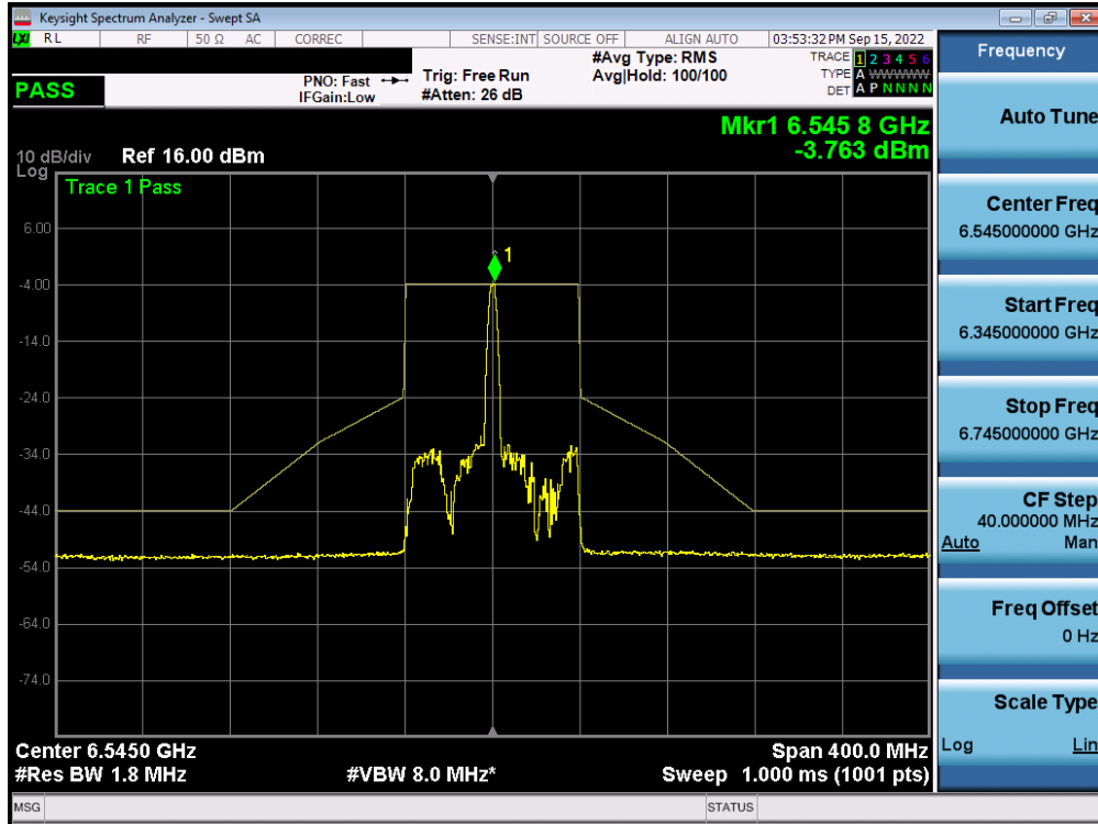
Plot 7-554. In-Band Emission Plot MIMO ANT2 (80MHz BW 802.11ax (26 Tones) (UNII Band 7) – Ch. 119) – LPI
