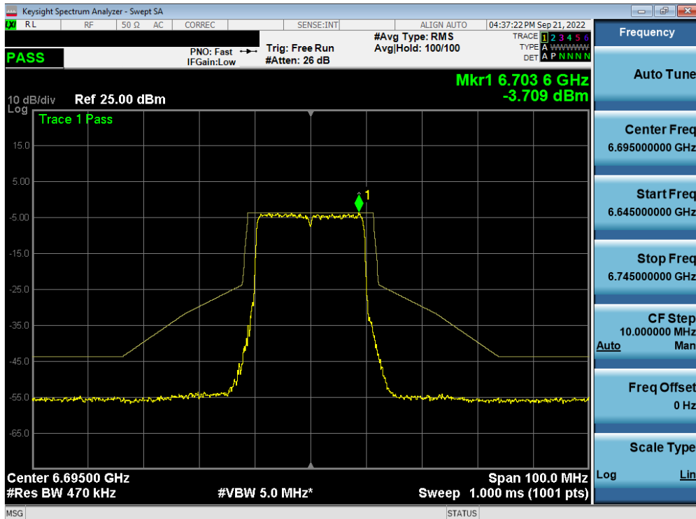
Plot 7-509. In-Band Emission Plot MIMO ANT1 (20MHz BW 802.11ax (Full Tone) (UNII Band 7) – Ch. 149) – LPI/SP
