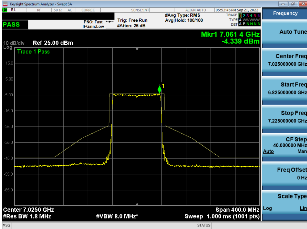
Plot 7-526. In-Band Emission Plot MIMO ANT1 (80MHz BW 802.11ax (Full Tone) (UNII Band 8) – Ch. 215) – LPI
