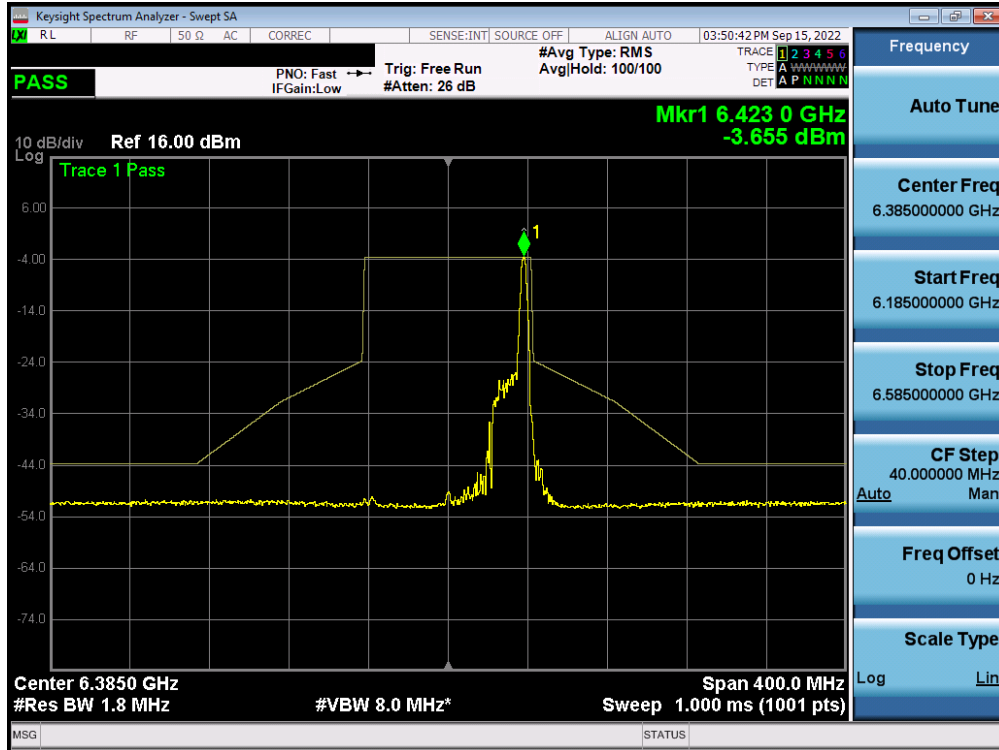
Plot 7-536. In-Band Emission Plot MIMO ANT2 (80MHz BW 802.11ax (26 Tones) (UNII Band 5) – Ch. 87) – LPI
