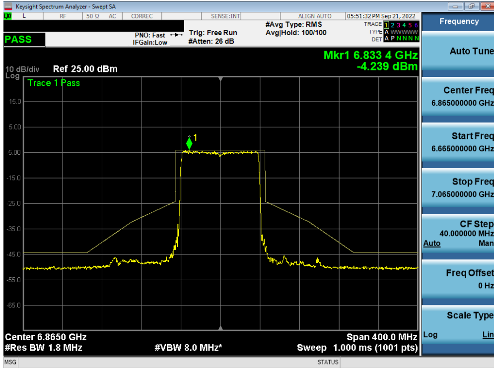
Plot 7-516. In-Band Emission Plot MIMO ANT1 (80MHz BW 802.11ax (Full Tone) (UNII Band 7) – Ch. 183) – LPI/SP
