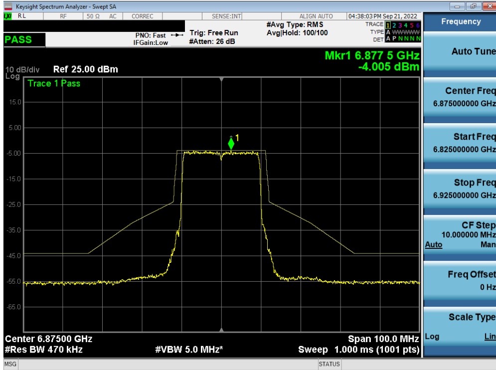
Plot 7-510. In-Band Emission Plot MIMO ANT1 (20MHz BW 802.11ax (Full Tone) (UNII Band 7) – Ch. 185) – LPI/SP
