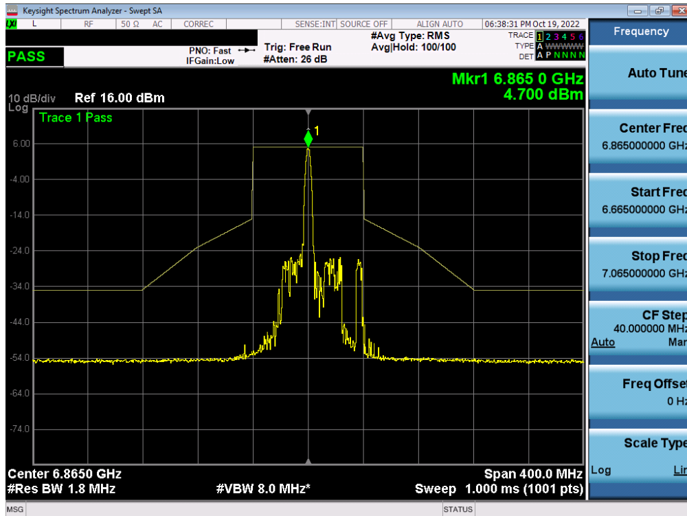
Plot 7-485. In-Band Emission Plot MIMO ANT1 (80MHz BW 802.11ax (26 Tones) (UNII Band 7) – Ch. 183) – SP
