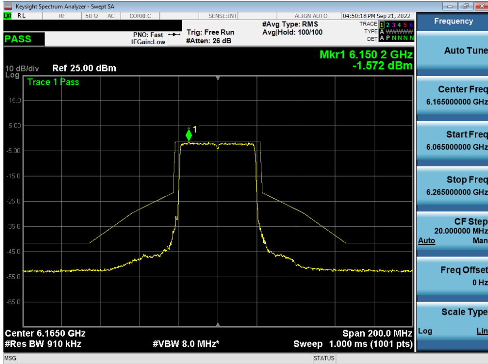
Plot 7-492. In-Band Emission Plot MIMO ANT1 (40MHz BW 802.11ax (Full Tone) (UNII Band 5) – Ch. 43) – LPI/SP
