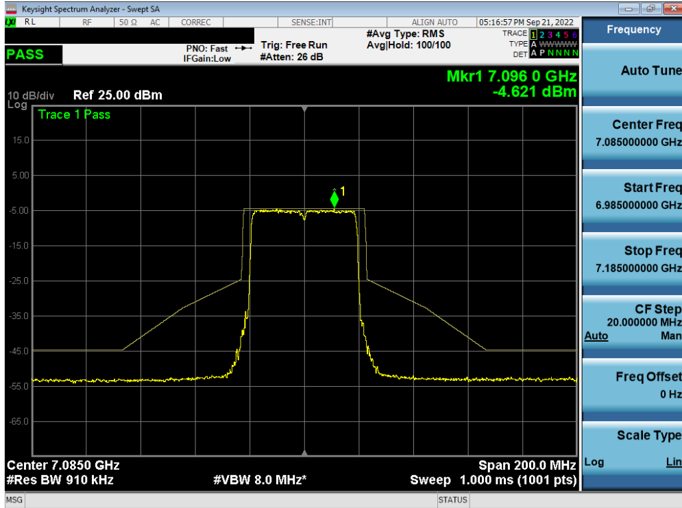
Plot 7-524. In-Band Emission Plot MIMO ANT1 (40MHz BW 802.11ax (Full Tone) (UNII Band 8) – Ch. 227) – LPI
