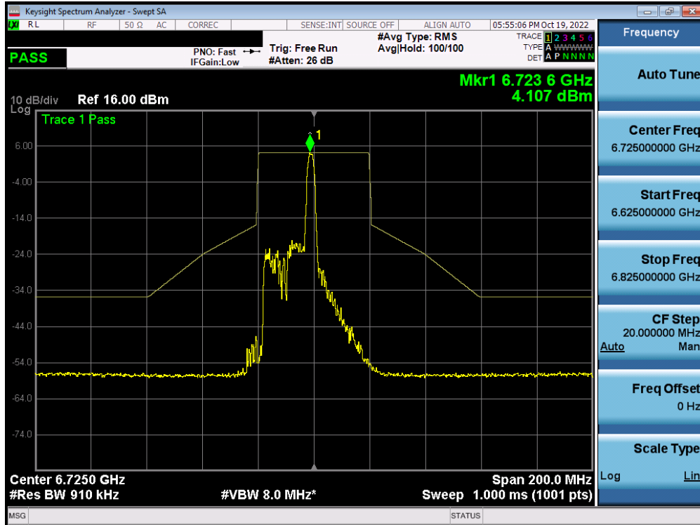
Plot 7-481. In-Band Emission Plot MIMO ANT1 (40MHz BW 802.11ax (26 Tones) (UNII Band 7) – Ch. 155) – SP
