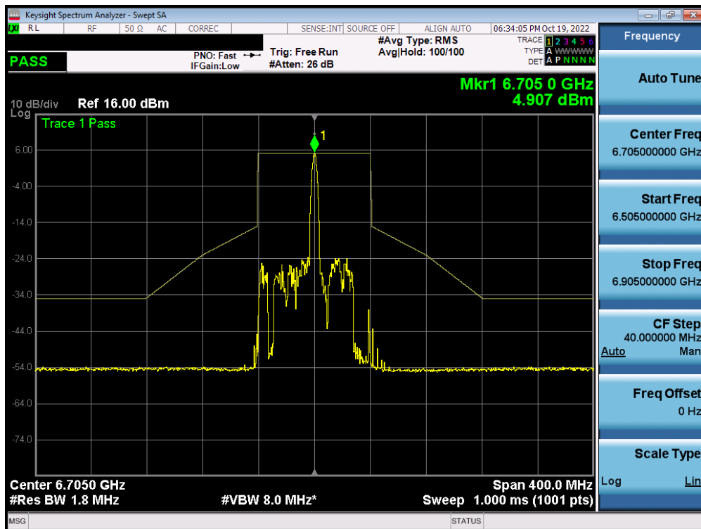
Plot 7-484. In-Band Emission Plot MIMO ANT1 (80MHz BW 802.11ax (26 Tones) (UNII Band 7) – Ch. 151) – SP
