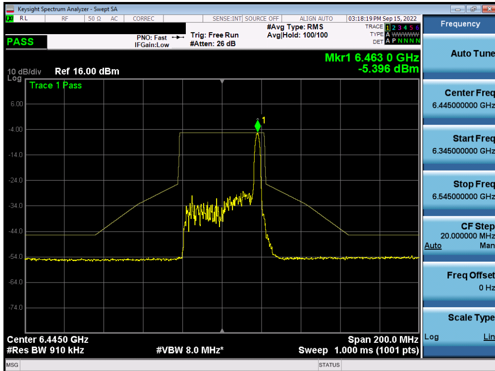
Plot 7-543. In-Band Emission Plot MIMO ANT2 (40MHz BW 802.11ax (26 Tones) (UNII Band 6) – Ch. 99) – LPI
