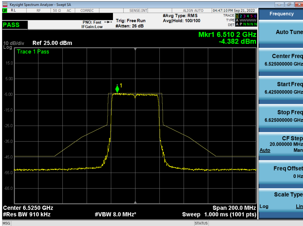
Plot 7-505. In-Band Emission Plot MIMO ANT1 (40MHz BW 802.11ax (Full Tone) (UNII Band 6) – Ch. 115) – LPI
