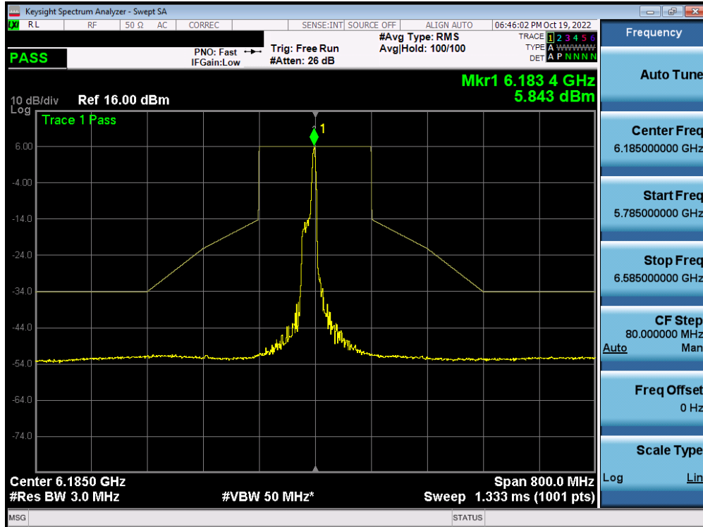
Plot 7-475. In-Band Emission Plot MIMO ANT1 (160MHz BW 802.11ax (26 Tones) (UNII Band 5) – Ch. 47) - SP
