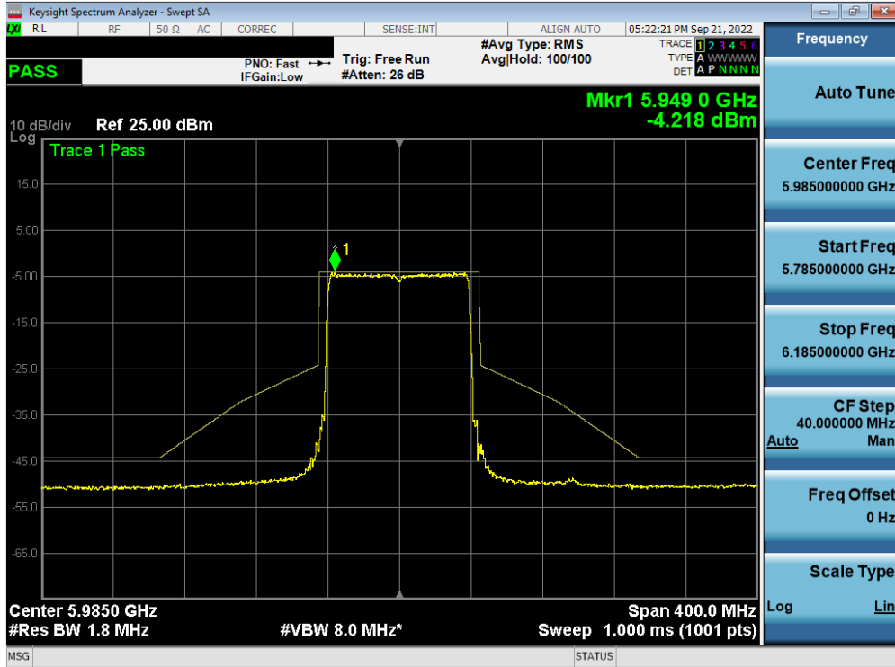
Plot 7-494. In-Band Emission Plot MIMO ANT1 (80MHz BW 802.11ax (Full Tone) (UNII Band 5) – Ch. 7) – LPI/SP
