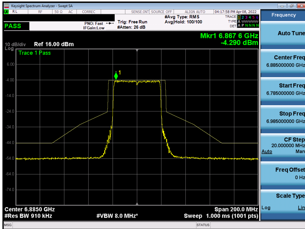
Plot 7-522. In-Band Emission Plot MIMO ANT1 (40MHz BW 802.11ax (Full Tone) (UNII Band 8) – Ch. 187) – LPI
