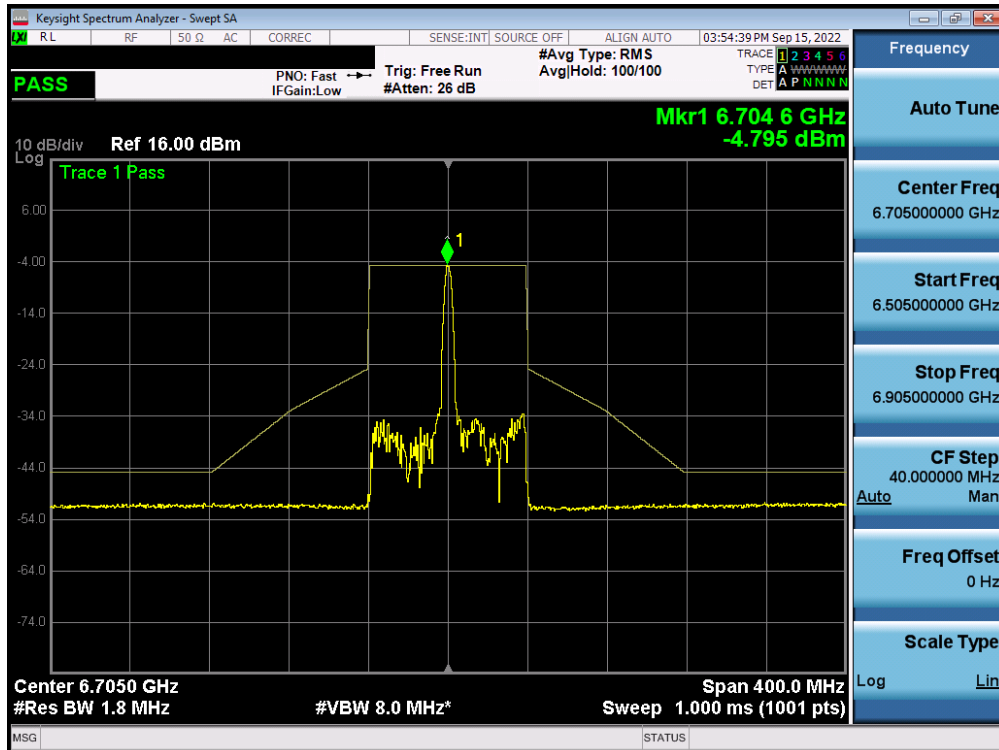
Plot 7-555. In-Band Emission Plot MIMO ANT2 (80MHz BW 802.11ax (26 Tones) (UNII Band 7) – Ch. 151) – LPI
