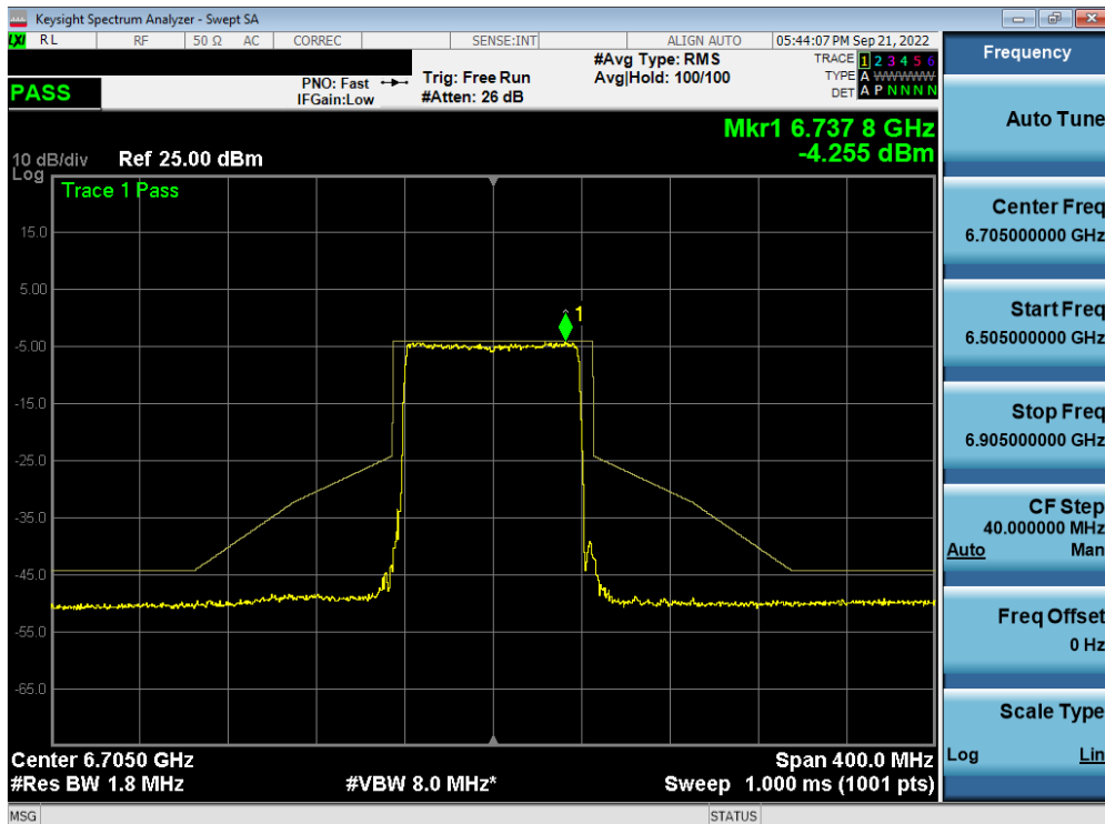
Plot 7-515. In-Band Emission Plot MIMO ANT1 (80MHz BW 802.11ax (Full Tone) (UNII Band 7) – Ch. 151) – LPI/SP
