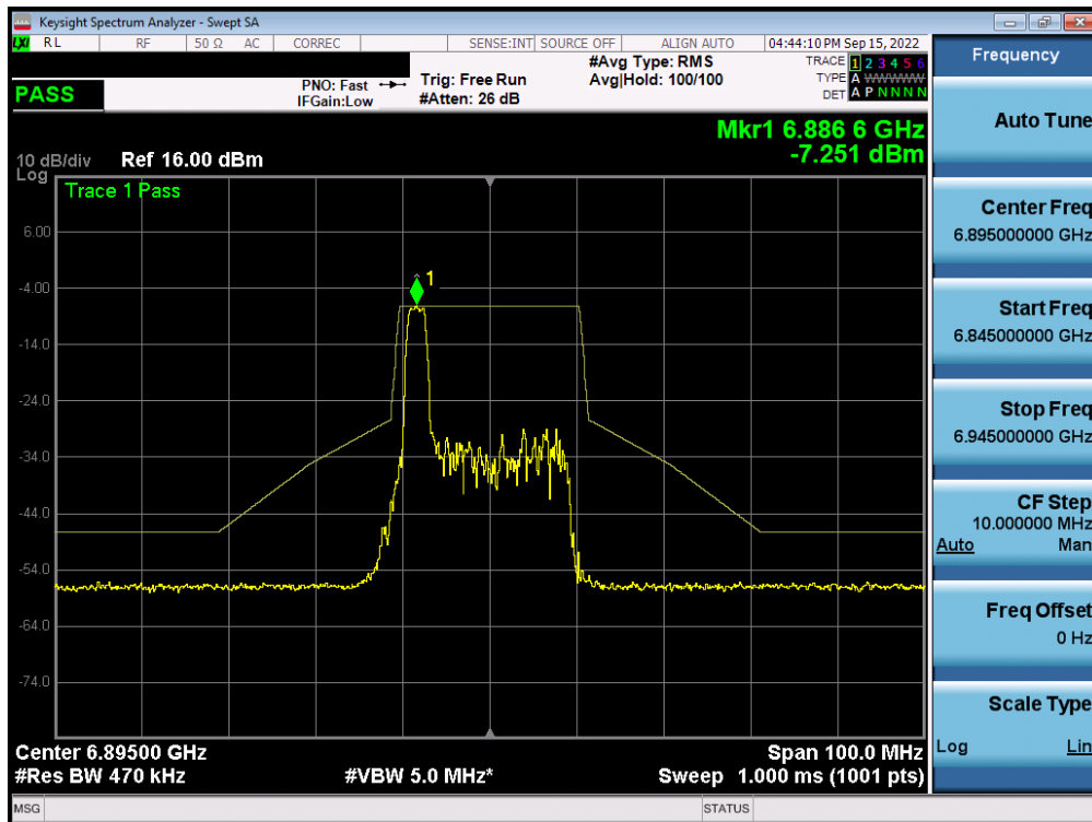
Plot 7-456. In-Band Emission Plot MIMO ANT1 (20MHz BW 802.11ax (26 Tones) (UNII Band 8) – Ch. 189) – LPI
