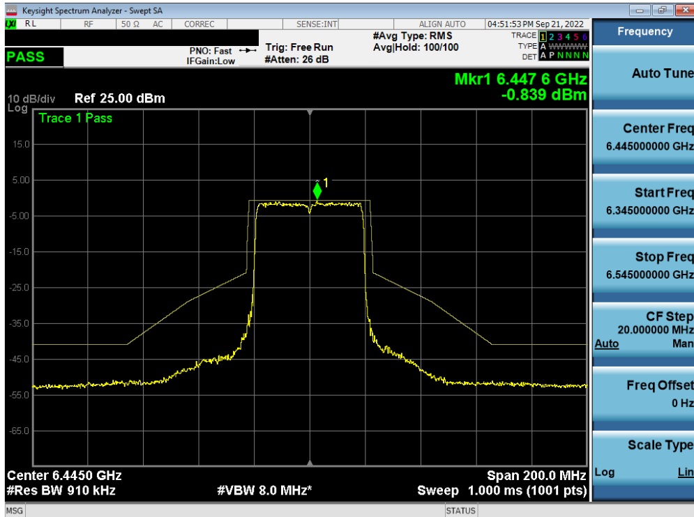
Plot 7-503. In-Band Emission Plot MIMO ANT1 (40MHz BW 802.11ax (Full Tone) (UNII Band 6) – Ch. 99) – LPI
