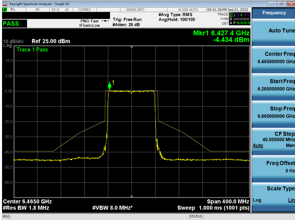
Plot 7-506. In-Band Emission Plot MIMO ANT1 (80MHz BW 802.11ax (Full Tone) (UNII Band 6) – Ch. 103) – LPI
