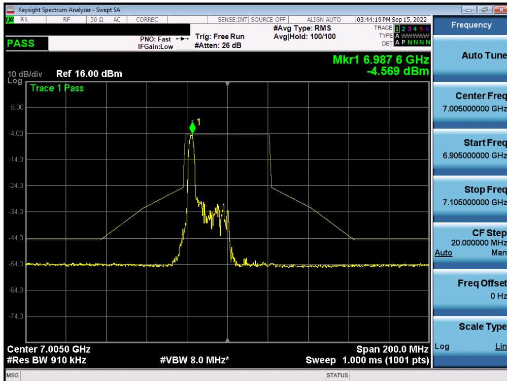
Plot 7-563. In-Band Emission Plot MIMO ANT2 (40MHz BW 802.11ax (26 Tones) (UNII Band 8) – Ch. 211) – LPI
