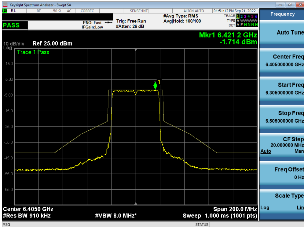
Plot 7-493. In-Band Emission Plot MIMO ANT1 (40MHz BW 802.11ax (Full Tone) (UNII Band 5) – Ch. 91) – LPI/SP
