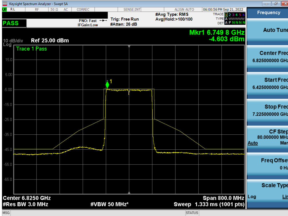
Plot 7-518. In-Band Emission Plot MIMO ANT1 (160MHz BW 802.11ax (Full Tone) (UNII Band 7) – Ch. 175) – LPI/SP
