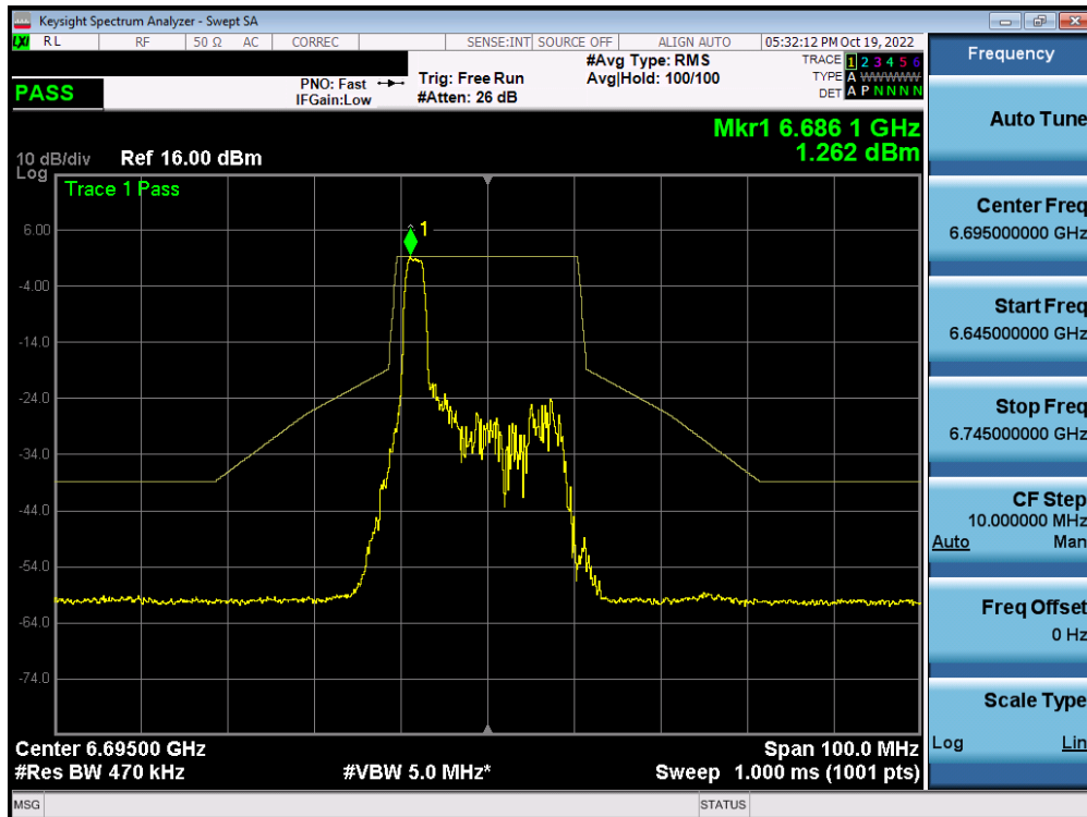
Plot 7-478. In-Band Emission Plot MIMO ANT1 (20MHz BW 802.11ax (26 Tones) (UNII Band 7) – Ch. 149) – SP
