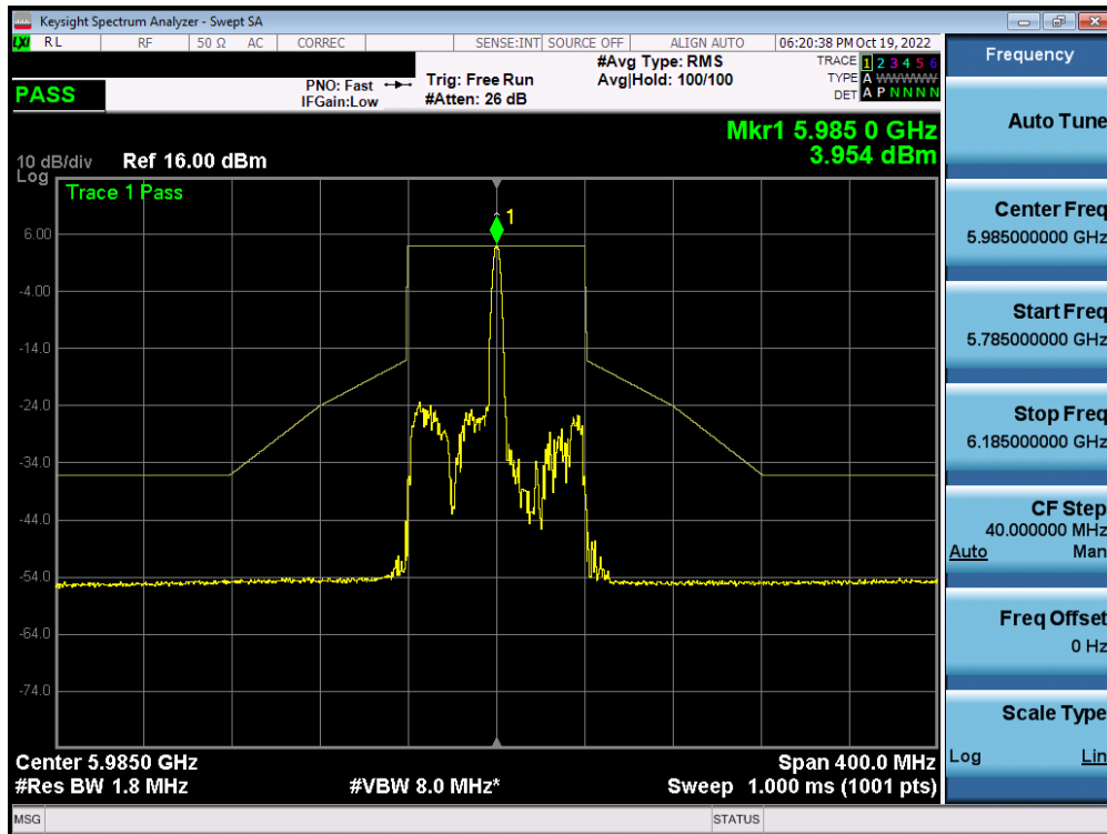
Plot 7-471. In-Band Emission Plot MIMO ANT1 (80MHz BW 802.11ax (26 Tones) (UNII Band 5) – Ch. 7) - SP
