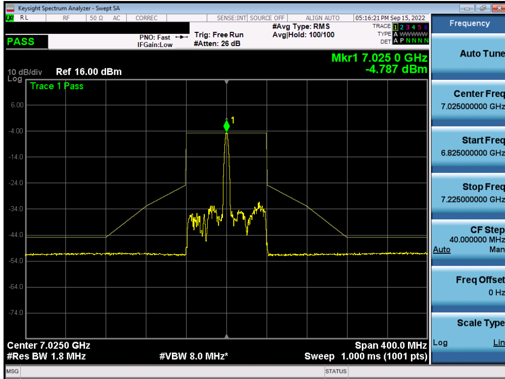
Plot 7-463. In-Band Emission Plot MIMO ANT1 (80MHz BW 802.11ax (26 Tones) (UNII Band 8) – Ch. 215) – LPI
