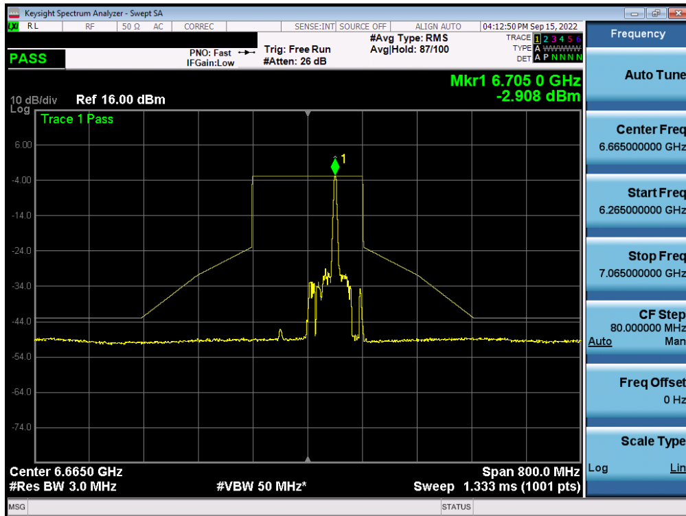
Plot 7-557. In-Band Emission Plot MIMO ANT2 (160MHz BW 802.11ax (26 Tones) (UNII Band 7) – Ch. 143) – LPI
