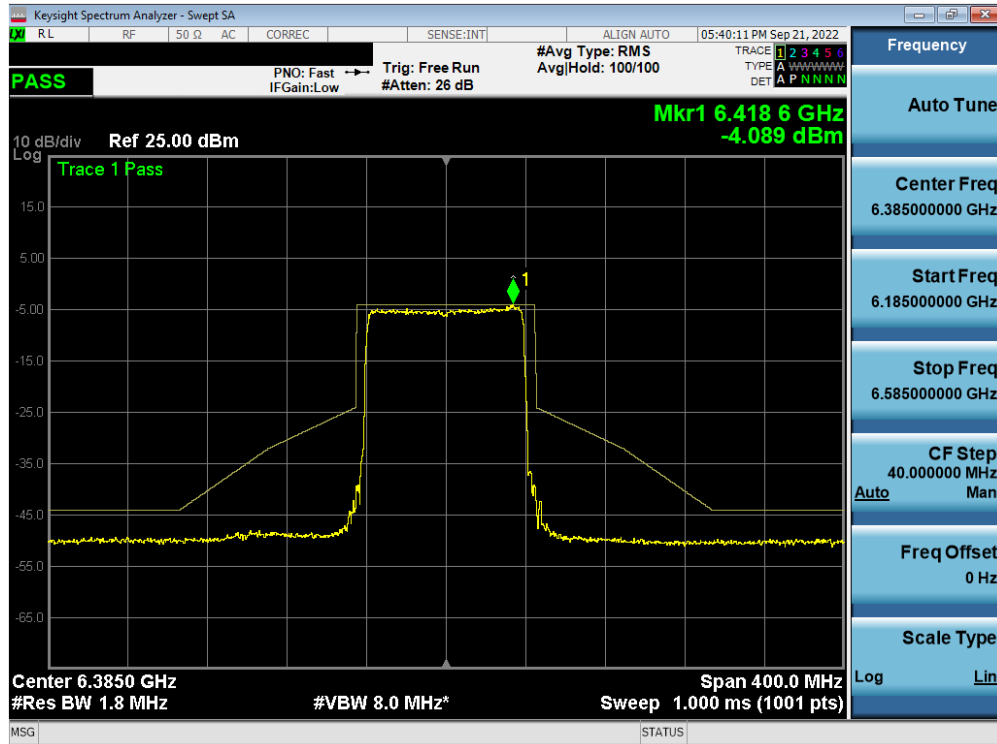
Plot 7-496. In-Band Emission Plot MIMO ANT1 (80MHz BW 802.11ax (Full Tone) (UNII Band 5) – Ch. 87) – LPI/SP
