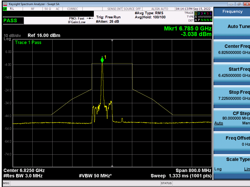
Plot 7-558. In-Band Emission Plot MIMO ANT2 (160MHz BW 802.11ax (26 Tones) (UNII Band 7) – Ch. 175) – LPI
