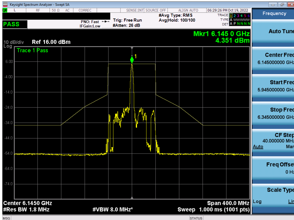
Plot 7-472. In-Band Emission Plot MIMO ANT1 (80MHz BW 802.11ax (26 Tones) (UNII Band 5) – Ch. 39) - SP
