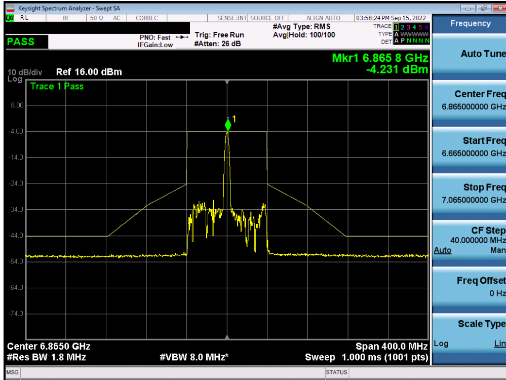
Plot 7-556. In-Band Emission Plot MIMO ANT2 (80MHz BW 802.11ax (26 Tones) (UNII Band 7) – Ch. 183) – LPI
