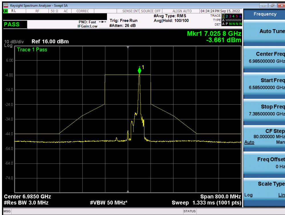
Plot 7-464. In-Band Emission Plot MIMO ANT1 (160MHz BW 802.11ax (26 Tones) (UNII Band 8) – Ch. 207) – LPI
