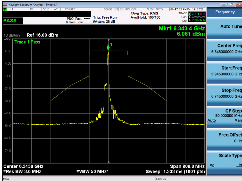
Plot 7-476. In-Band Emission Plot MIMO ANT1 (160MHz BW 802.11ax (26 Tones) (UNII Band 5) – Ch. 79) – SP
