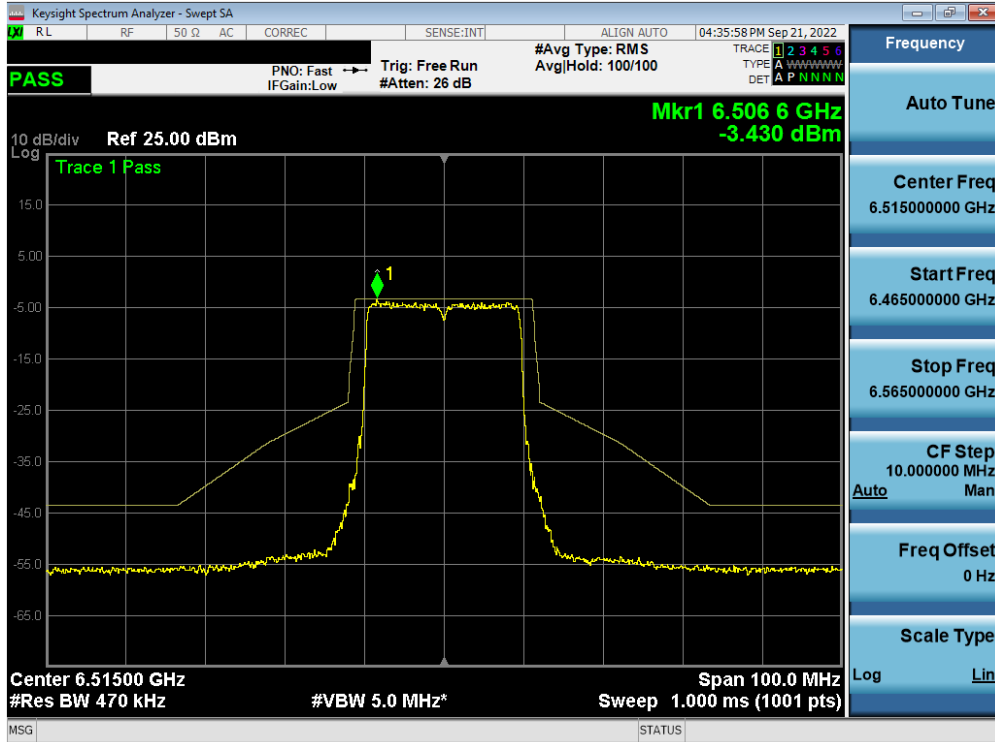
Plot 7-502. In-Band Emission Plot MIMO ANT1 (20MHz BW 802.11ax (Full Tone) (UNII Band 6) – Ch. 113) – LPI
