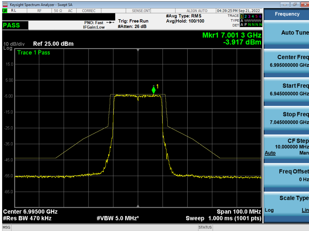
Plot 7-520. In-Band Emission Plot MIMO ANT1 (20MHz BW 802.11ax (Full Tone) (UNII Band 8) – Ch. 209) – LPI
