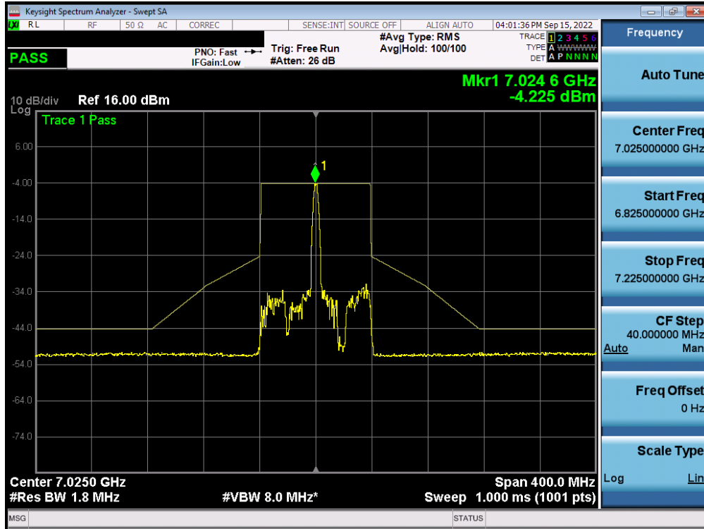
Plot 7-566. In-Band Emission Plot MIMO ANT2 (80MHz BW 802.11ax (26 Tones) (UNII Band 8) – Ch. 215) – LPI
