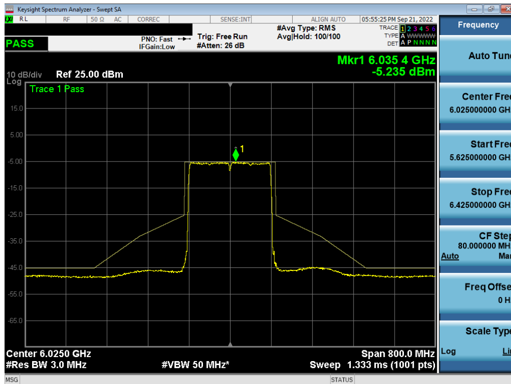
Plot 7-497. In-Band Emission Plot MIMO ANT1 (160MHz BW 802.11ax (Full Tone) (UNII Band 5) – Ch. 15) – LPI/SP
