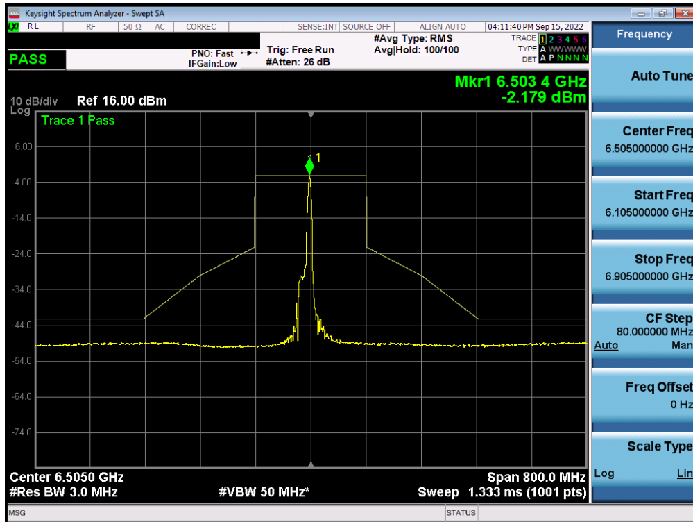
Plot 7-547. In-Band Emission Plot MIMO ANT2 (160MHz BW 802.11ax (26 Tones) (UNII Band 6) – Ch. 111) – LPI
