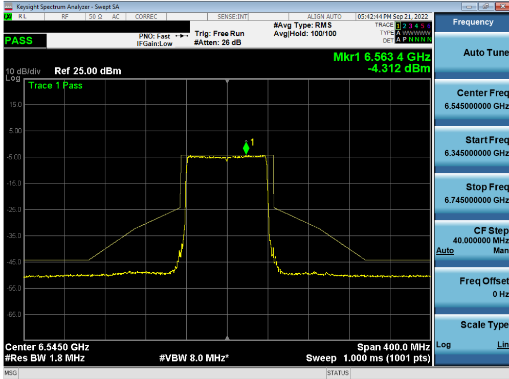
Plot 7-514. In-Band Emission Plot MIMO ANT1 (80MHz BW 802.11ax (Full Tone) (UNII Band 7) – Ch. 119) – LPI/SP
