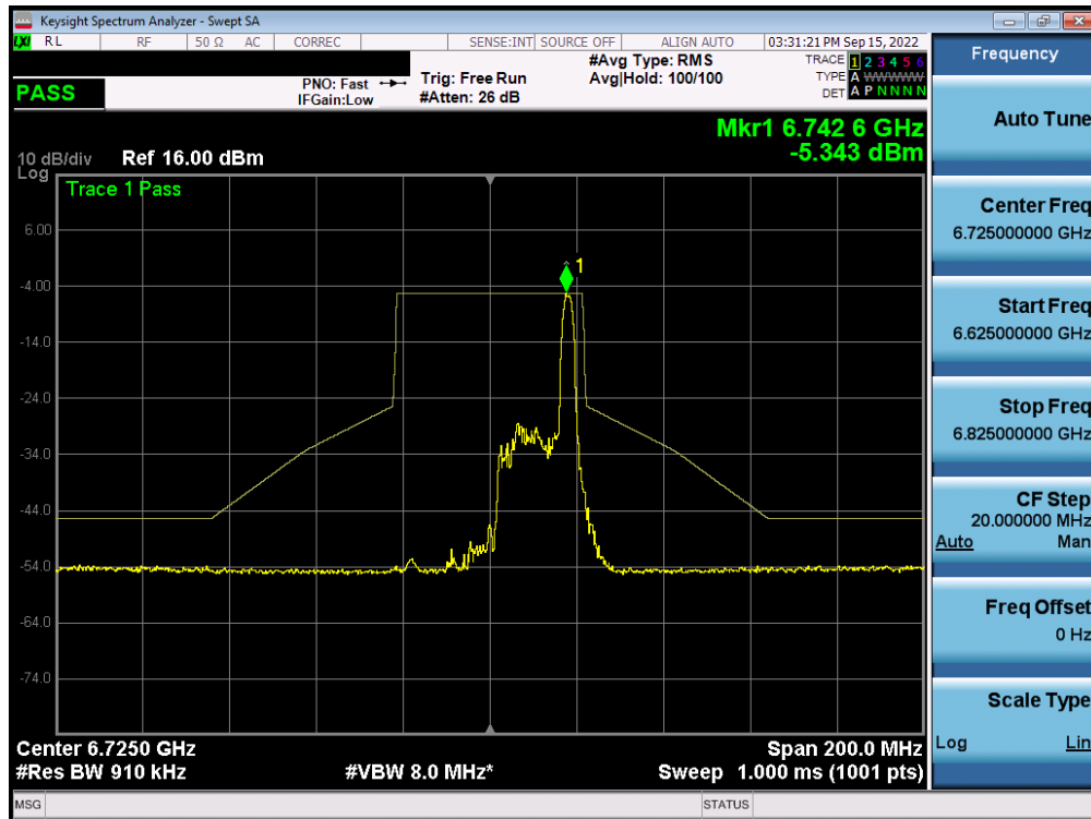
Plot 7-552. In-Band Emission Plot MIMO ANT2 (40MHz BW 802.11ax (26 Tones) (UNII Band 7) – Ch. 155) – LPI
