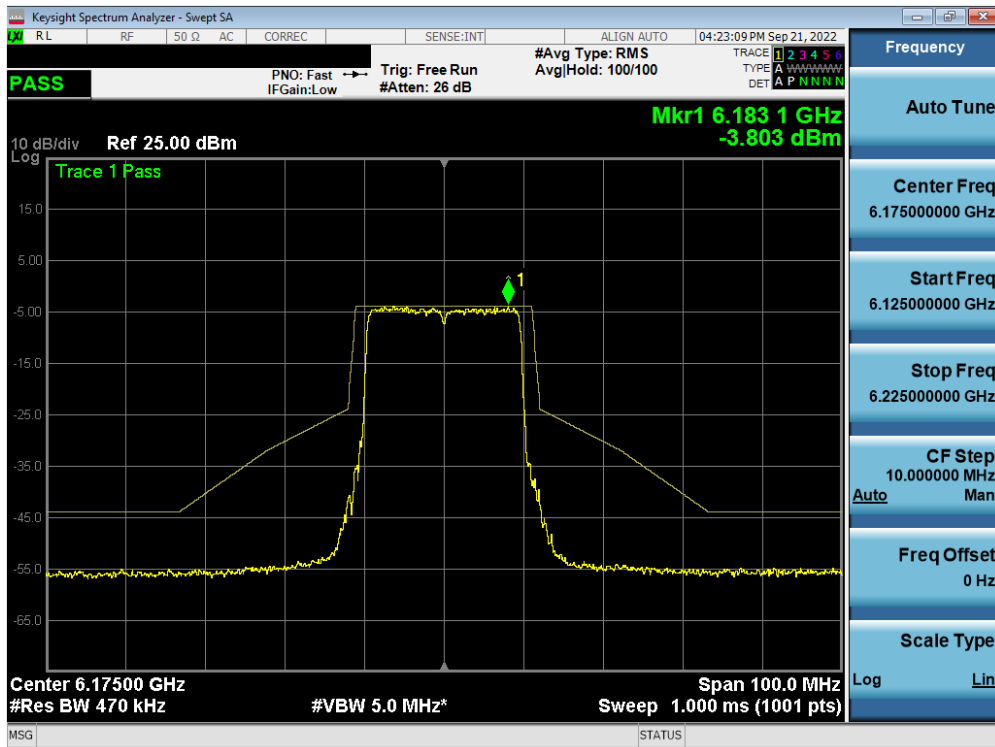
Plot 7-489. In-Band Emission Plot MIMO ANT1 (20MHz BW 802.11ax (Full Tone) (UNII Band 5) – Ch. 45) – LPI
