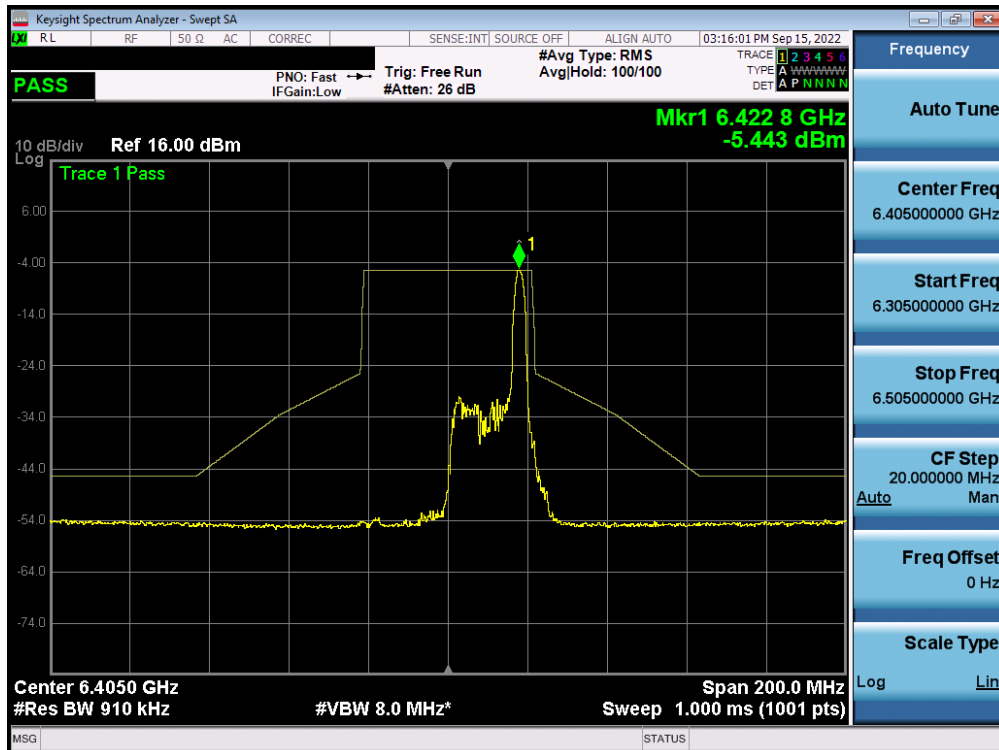
Plot 7-533. In-Band Emission Plot MIMO ANT2 (40MHz BW 802.11ax (26 Tones) (UNII Band 5) – Ch. 91) – LPI
