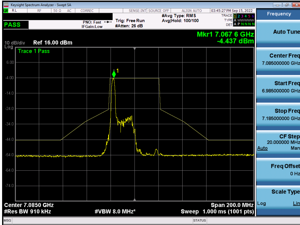
Plot 7-564. In-Band Emission Plot MIMO ANT2 (40MHz BW 802.11ax (26 Tones) (UNII Band 8) – Ch. 227) – LPI
