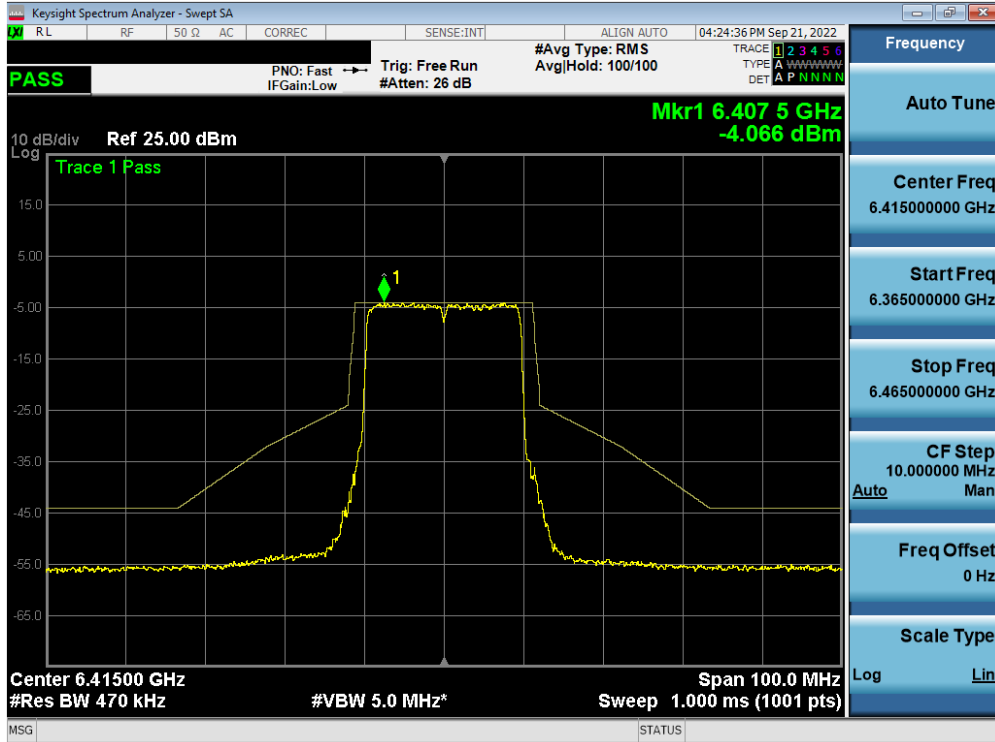
Plot 7-490. In-Band Emission Plot MIMO ANT1 (20MHz BW 802.11ax (Full Tone) UNII Band 5) – Ch. 93) – LPI
