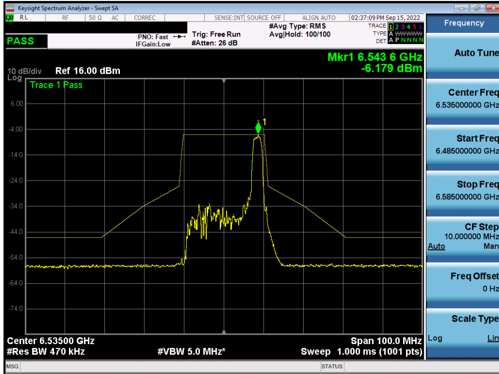
Plot 7-548. In-Band Emission Plot MIMO ANT2 (20MHz BW 802.11ax (26 Tones) (UNII Band 7) – Ch. 117) – LPI
