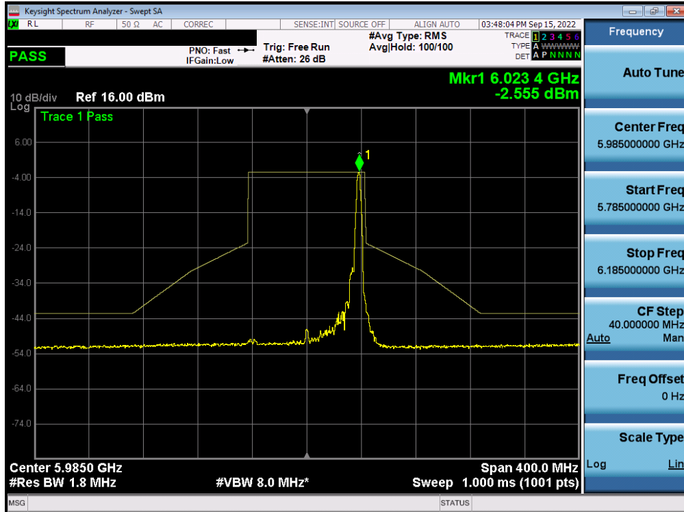
Plot 7-534. In-Band Emission Plot MIMO ANT2 (80MHz BW 802.11ax (26 Tones) (UNII Band 5) – Ch. 7) – LPI
