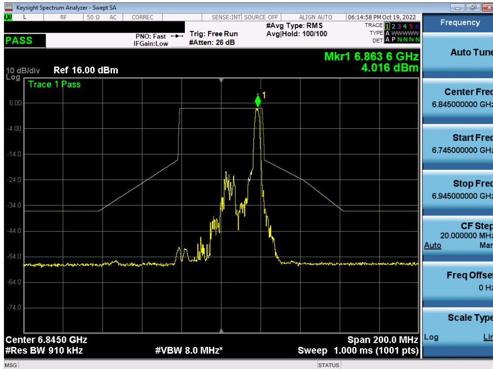
Plot 7-482. In-Band Emission Plot MIMO ANT1 (40MHz BW 802.11ax (26 Tones) (UNII Band 7) – Ch. 179) – SP
