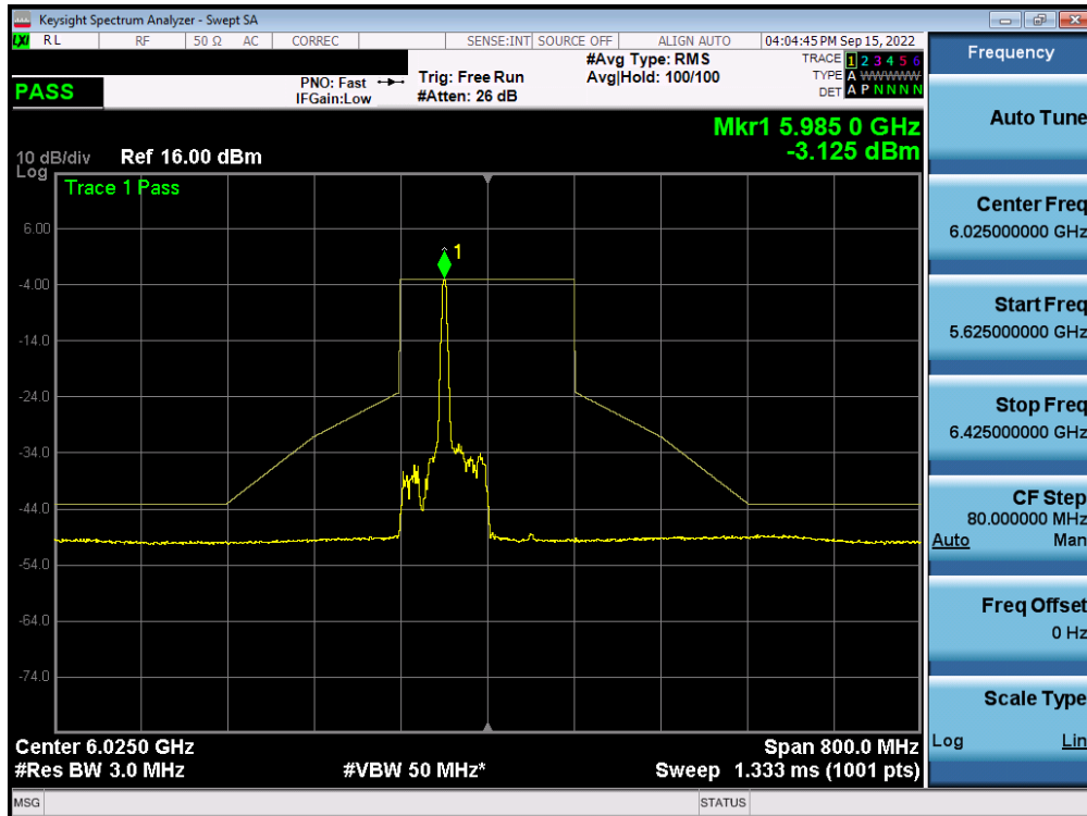
Plot 7-537. In-Band Emission Plot MIMO ANT2 (160MHz BW 802.11ax (26 Tones) (UNII Band 5) – Ch. 15) – LPI
