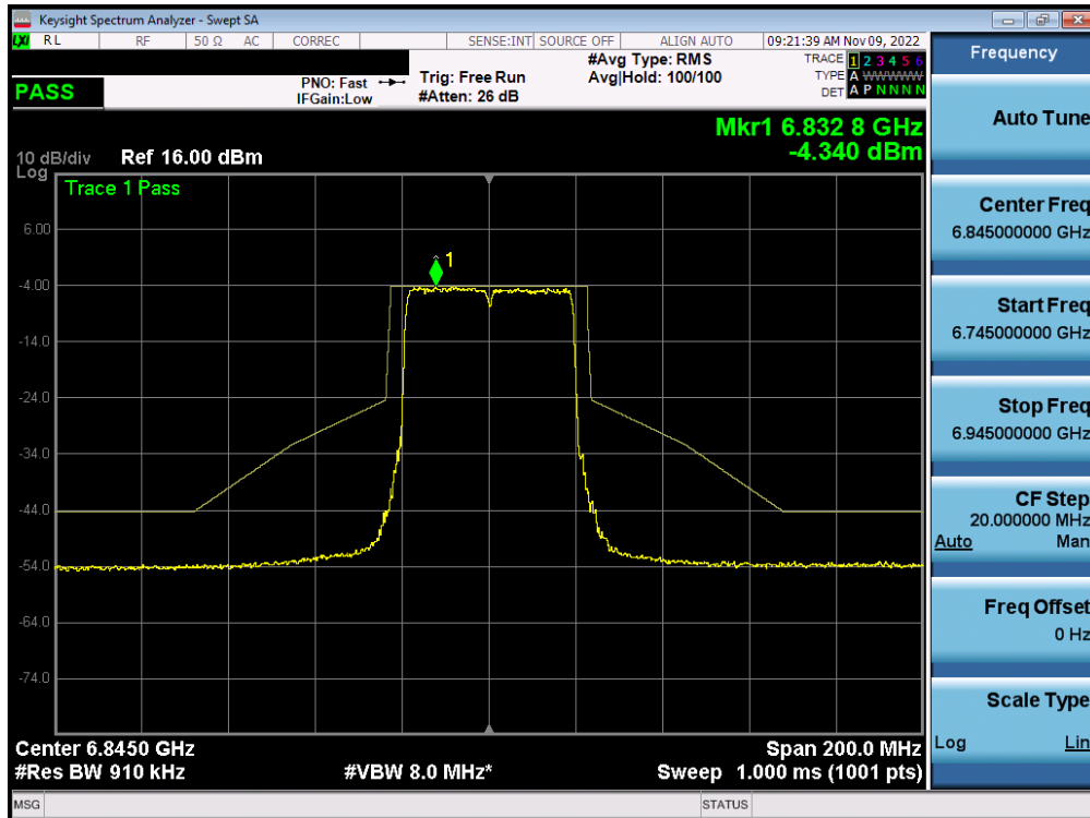
Plot 7-513. In-Band Emission Plot MIMO ANT1 (40MHz BW 802.11ax (Full Tone) (UNII Band 7) – Ch. 179) – LPI/SP
