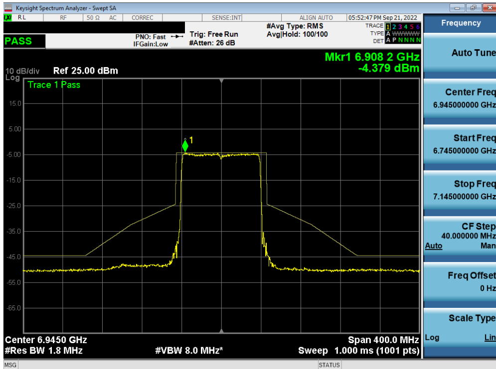
Plot 7-525. In-Band Emission Plot MIMO ANT1 (80MHz BW 802.11ax (Full Tone) (UNII Band 8) – Ch. 199) – LPI
