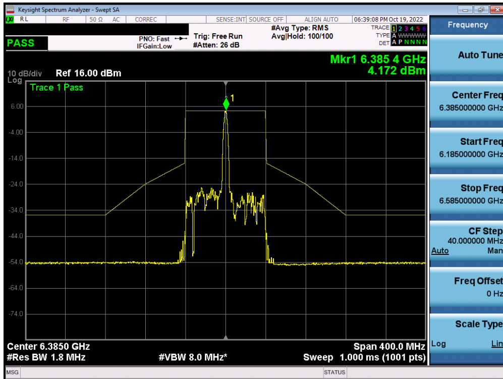
Plot 7-473. In-Band Emission Plot MIMO ANT1 (80MHz BW 802.11ax (26 Tones) (UNII Band 5) – Ch. 87) - SP
