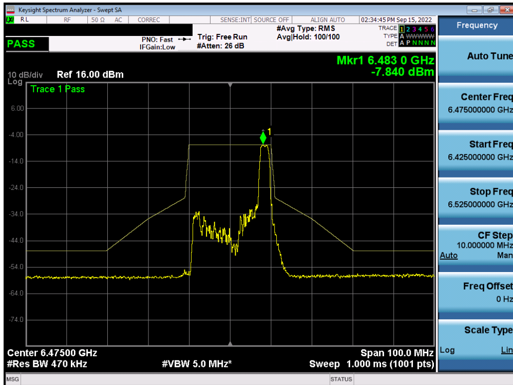
Plot 7-541. In-Band Emission Plot MIMO ANT2 (20MHz BW 802.11ax (26 Tones) (UNII Band 6) – Ch. 105) – LPI
