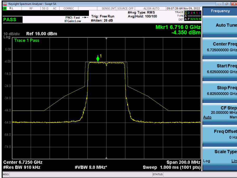
Plot 7-512. In-Band Emission Plot MIMO ANT1 (40MHz BW 802.11ax (Full Tone) (UNII Band 7) – Ch. 155) – LPI/SP
