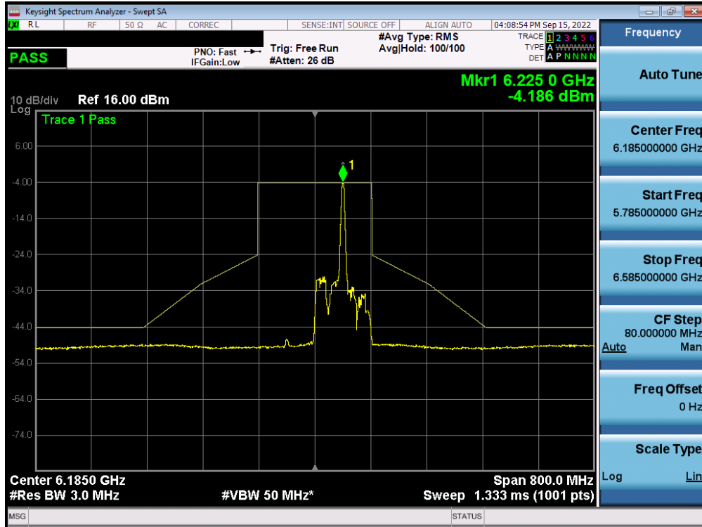
Plot 7-538. In-Band Emission Plot MIMO ANT2 (160MHz BW 802.11ax (26 Tones) (UNII Band 5) – Ch. 47) – LPI
