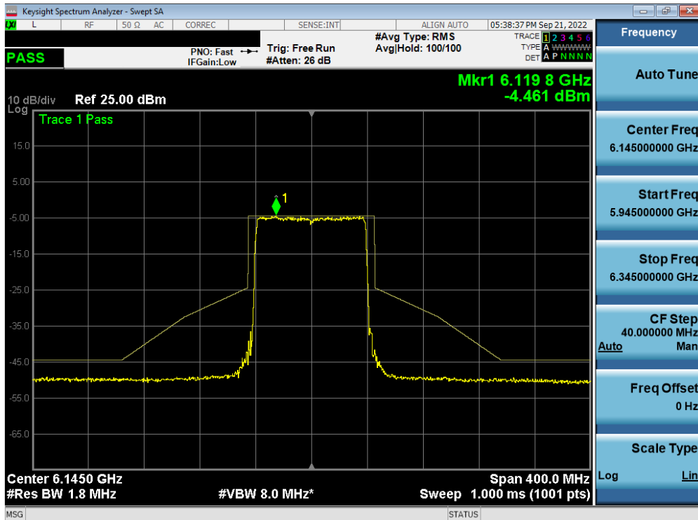
Plot 7-495. In-Band Emission Plot MIMO ANT1 (80MHz BW 802.11ax (Full Tone) (UNII Band 5) – Ch. 39) – LPI/SP
