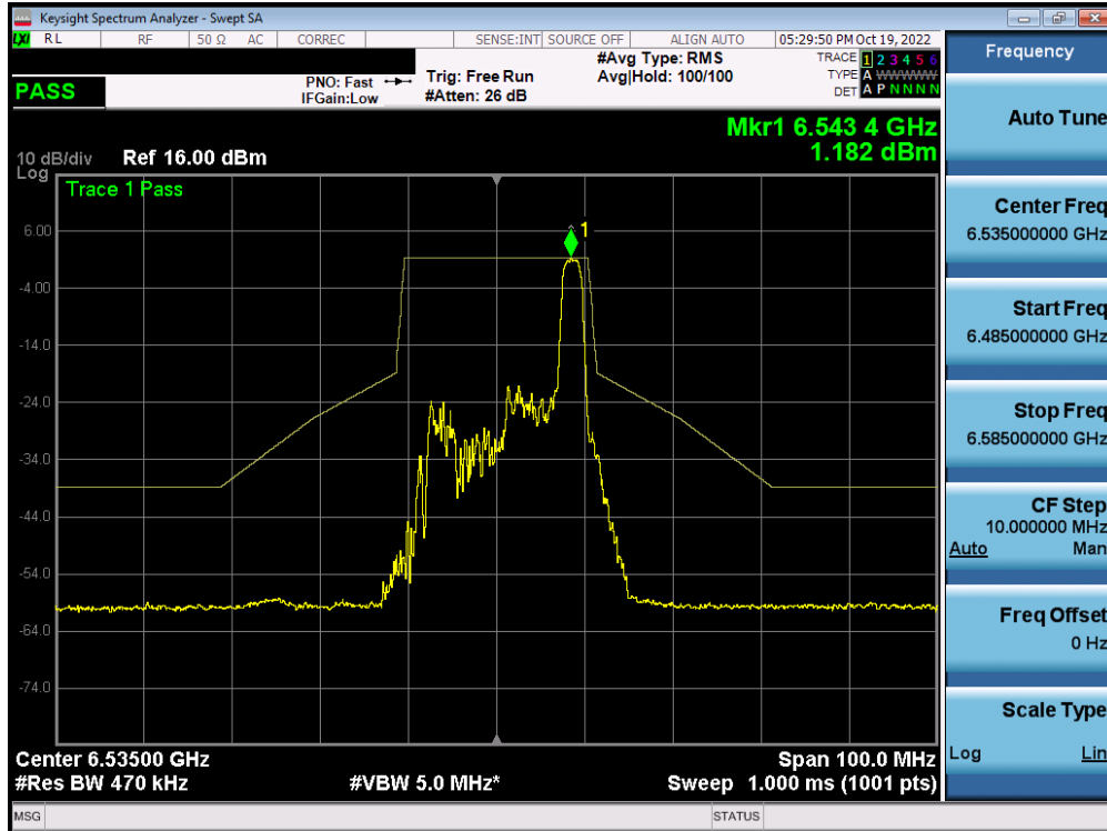
Plot 7-477. In-Band Emission Plot MIMO ANT1 (20MHz BW 802.11ax (26 Tones) (UNII Band 7) – Ch. 117) – SP
