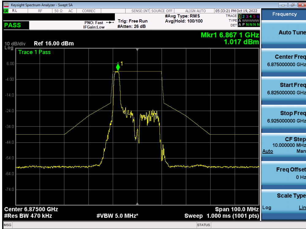
Plot 7-479. In-Band Emission Plot MIMO ANT1 (20MHz BW 802.11ax (26 Tones) (UNII Band 7) – Ch. 185) – SP
