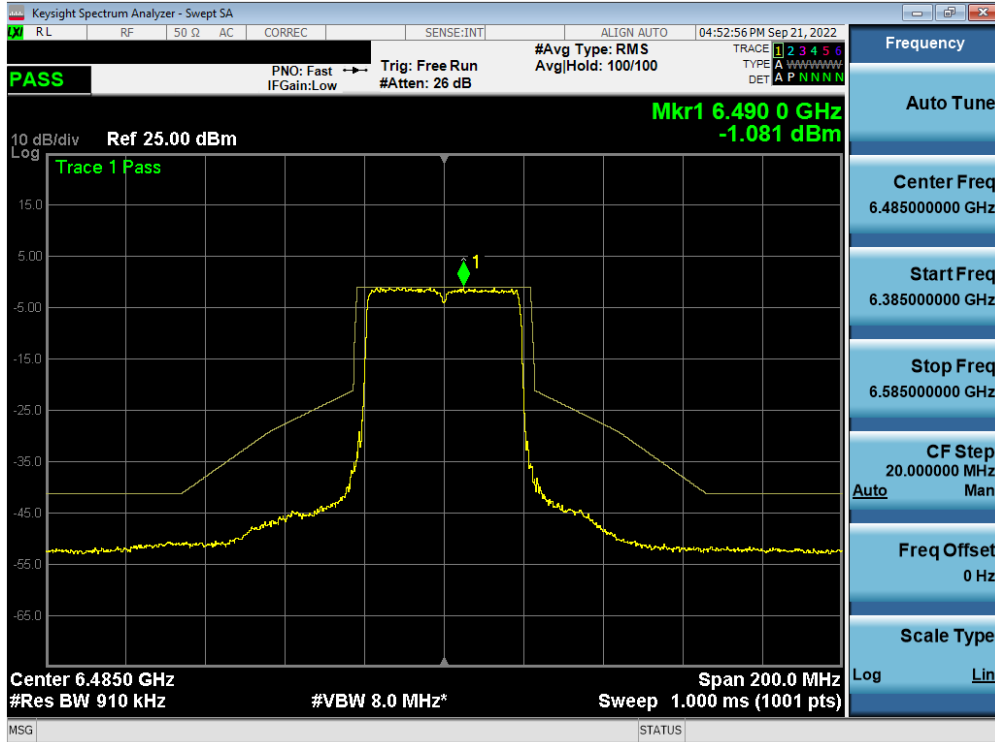
Plot 7-504. In-Band Emission Plot MIMO ANT1 (40MHz BW 802.11ax (Full Tone) (UNII Band 6) – Ch. 107) – LPI
