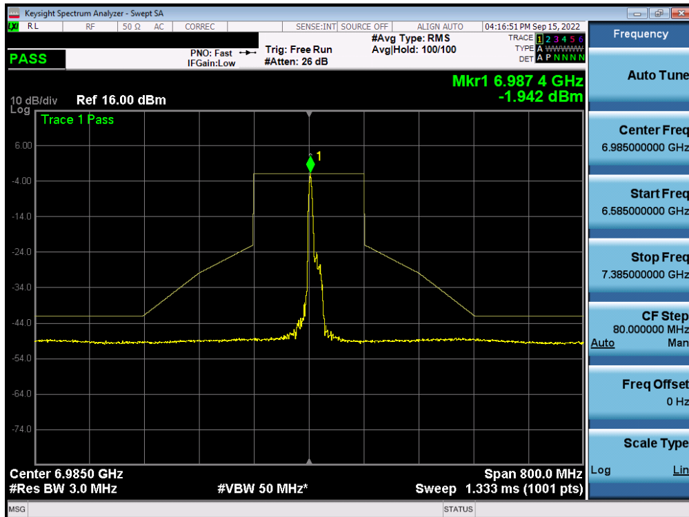
Plot 7-567. In-Band Emission Plot MIMO ANT2 (160MHz BW 802.11ax (26 Tones) (UNII Band 8) – Ch. 207) – LPI
