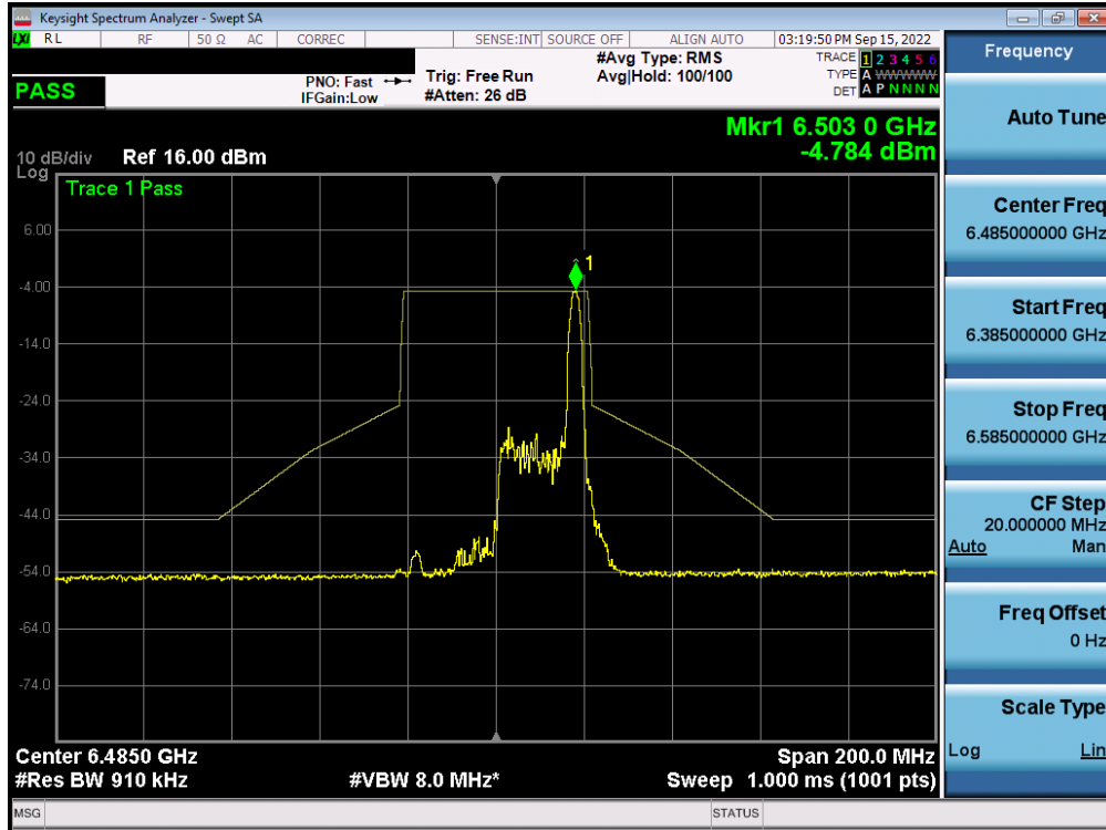
Plot 7-544. In-Band Emission Plot MIMO ANT2 (40MHz BW 802.11ax (26 Tones) (UNII Band 6) – Ch. 107) – LPI
