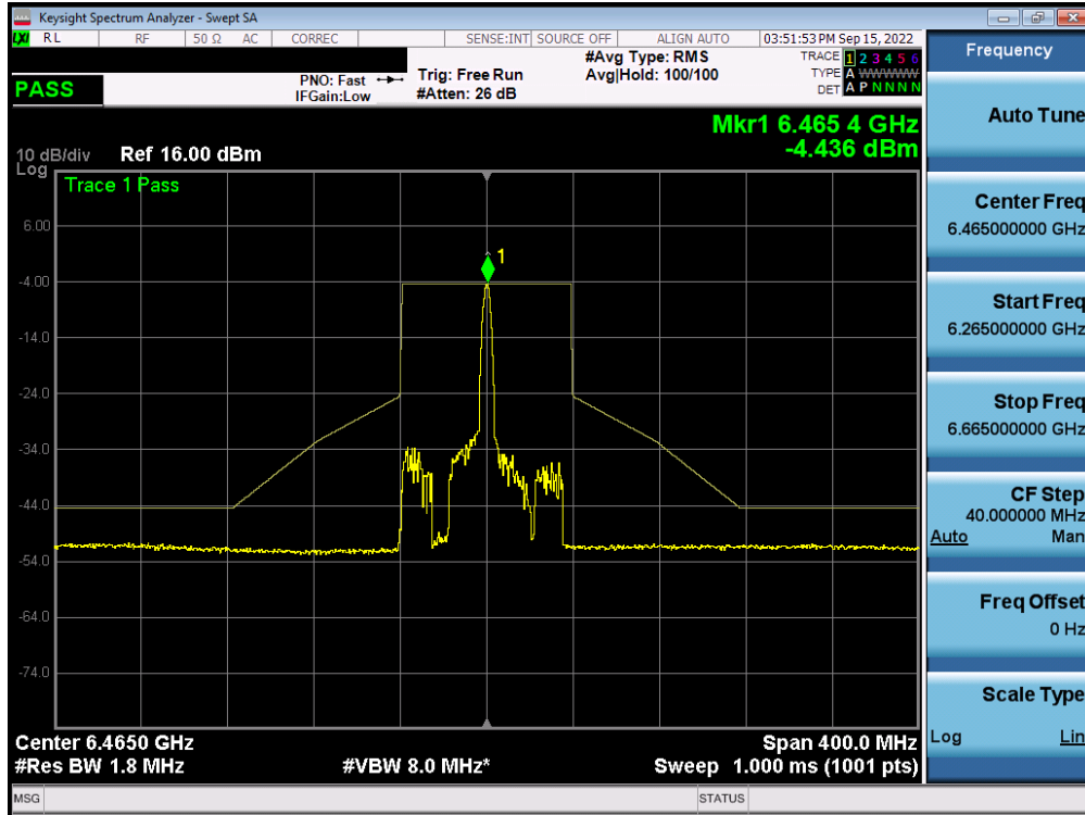
Plot 7-546. In-Band Emission Plot MIMO ANT2 (80MHz BW 802.11ax (26 Tones) (UNII Band 6) – Ch. 103) – LPI
