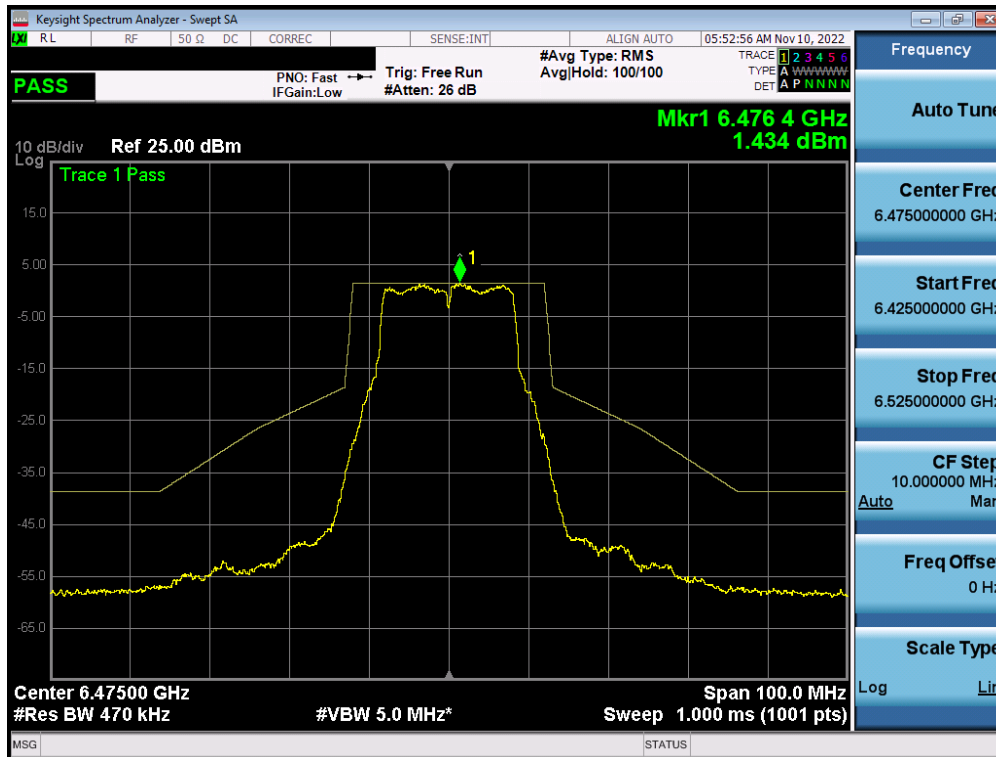
Plot 7-225. In-Band Emission Plot Measurement MIMO ANT1 (20MHz 802.11a (UNII Band 6) – Ch. 105)
