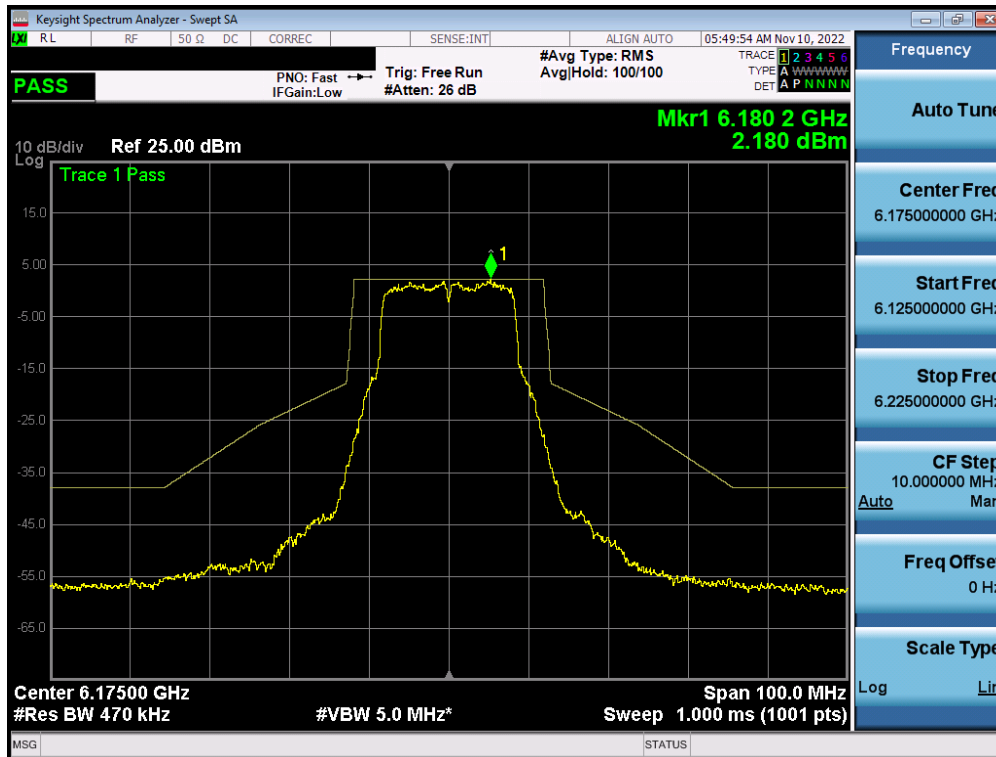
Plot 7-210. In-Band Emission Plot Measurement MIMO ANT1 (20MHz 802.11a (UNII Band 5) – Ch. 45)
