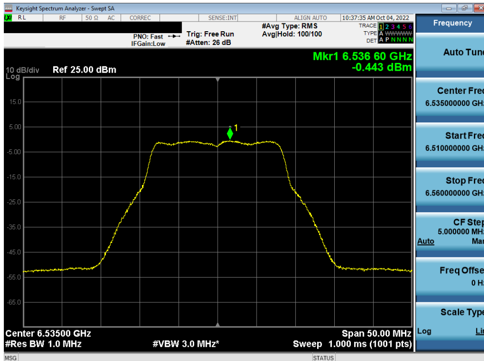
Plot 7-134. Power Spectral Density Measurement MIMO ANT1 (20MHz 802.11a (UNII Band 7) – Ch. 117)
