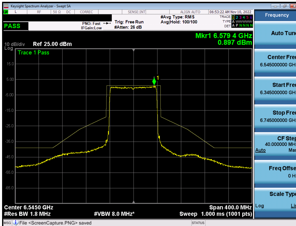
Plot 7-244. In-Band Emission Plot Measurement MIMO ANT1 (80MHz 802.11ax (UNII Band 7) – Ch. 119)
