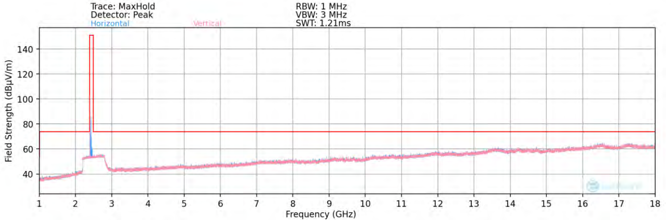
Plot 7-119. Radiated Spurious Plot above 1GHz (BT- Ch. 0) – Ant1
