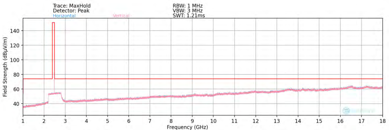
Plot 7-121. Radiated Spurious Plot above 1GHz (BT- Ch. 78) – Ant1
