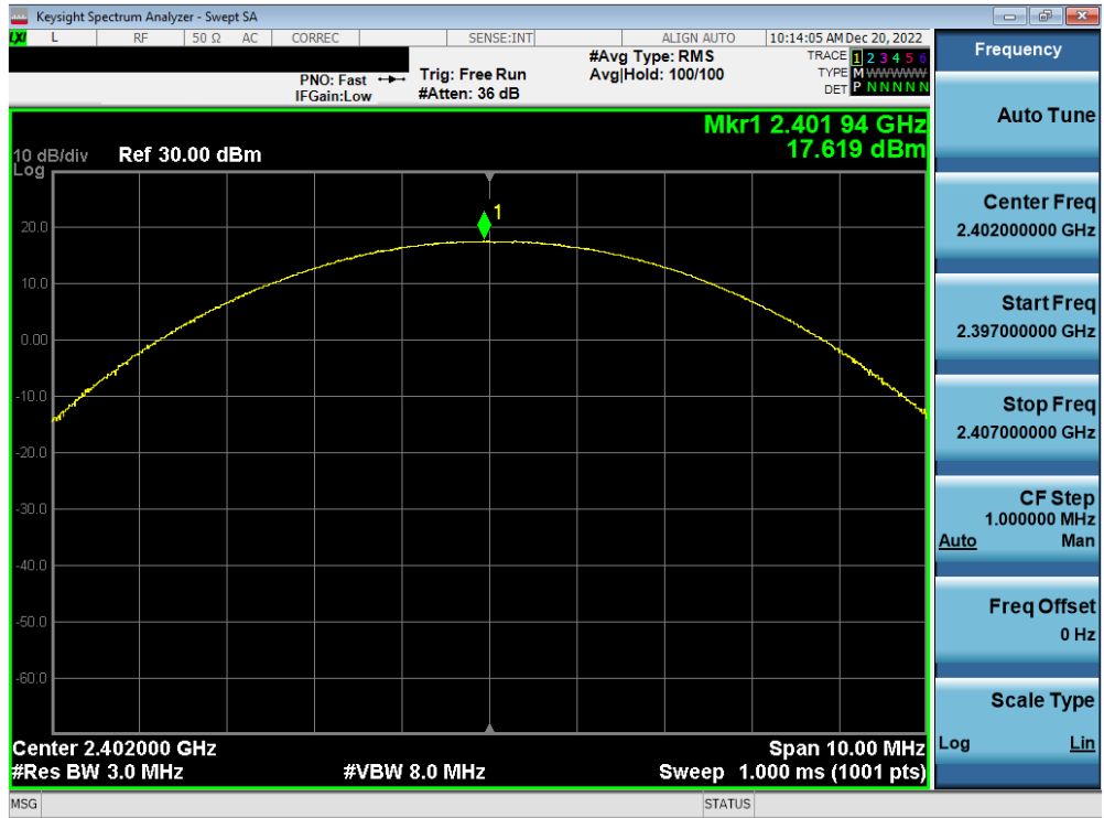
Plot 7-40. Peak Conducted Power (2Mbps – Ch. 0) – Ant 2
