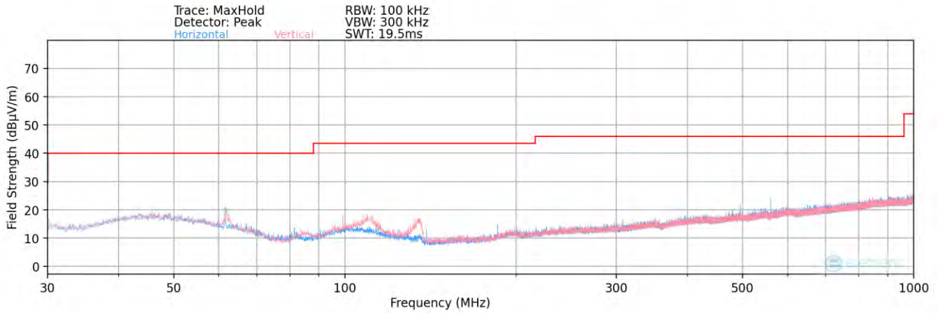
Plot 7-135. Radiated Spurious Plot below 1GHz – Ant1
