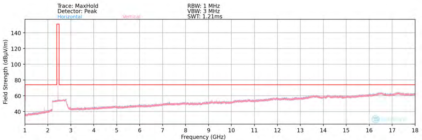
Plot 7-120. Radiated Spurious Plot above 1GHz (BT- Ch. 39) – Ant1
