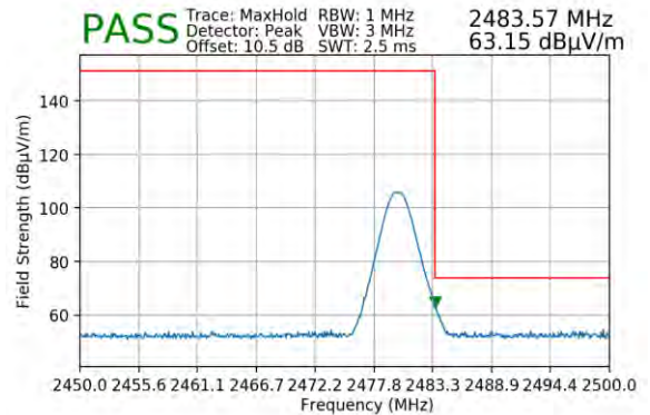
Plot 7-134. Radiated Restricted Upper Band Edge Measurement (Peak) – Dual with WCP
