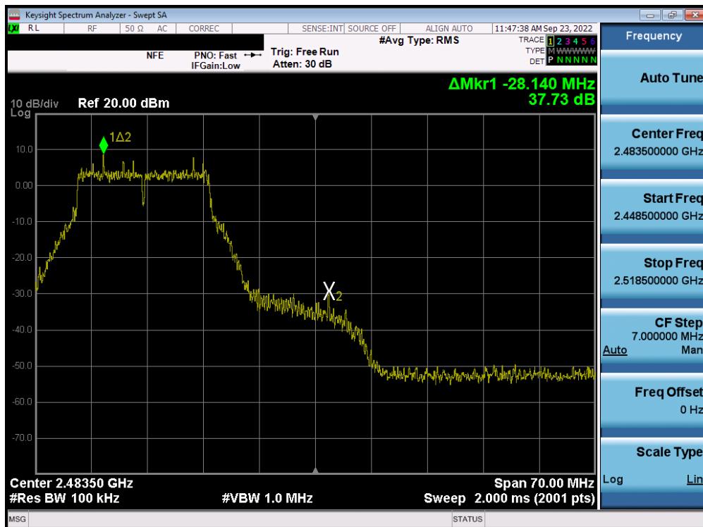
Plot 7-94. Band Edge Plot MIMO ANT1 (802.11g – Ch. 11)
