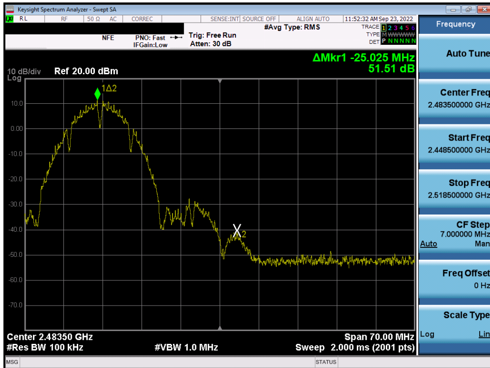
Plot 7-90. Band Edge Plot MIMO ANT1 (802.11b – Ch. 11)
