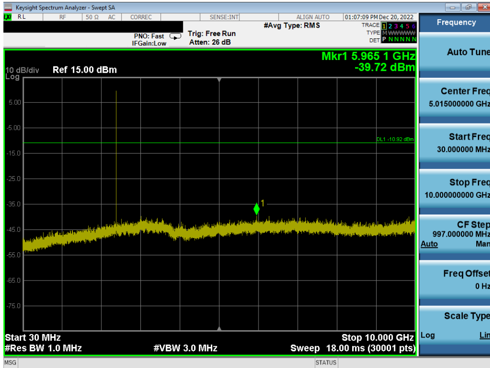
Plot 7-95. Conducted Spurious Plot (Bluetooth (LE), 2Mbps – Ch. 0) – ANT 2
