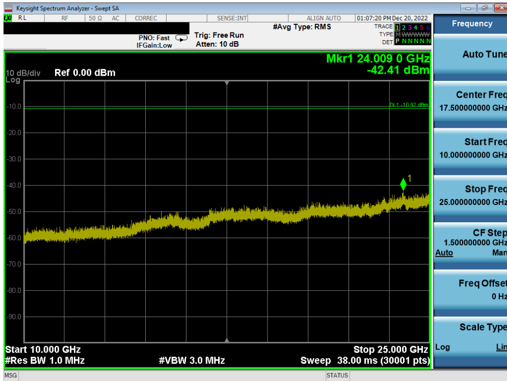
Plot 7-96. Conducted Spurious Plot (Bluetooth (LE), 2Mbps – Ch. 0) – ANT 2
