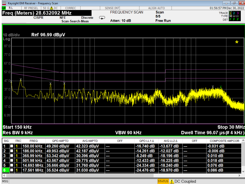
Plot 7-107. Line Conducted Plot with Bluetooth LE (L1) – ANT 2
