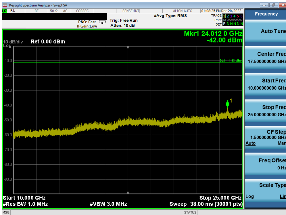
Plot 7-98. Conducted Spurious Plot (Bluetooth (LE), 2Mbps – Ch. 19) – ANT 2
