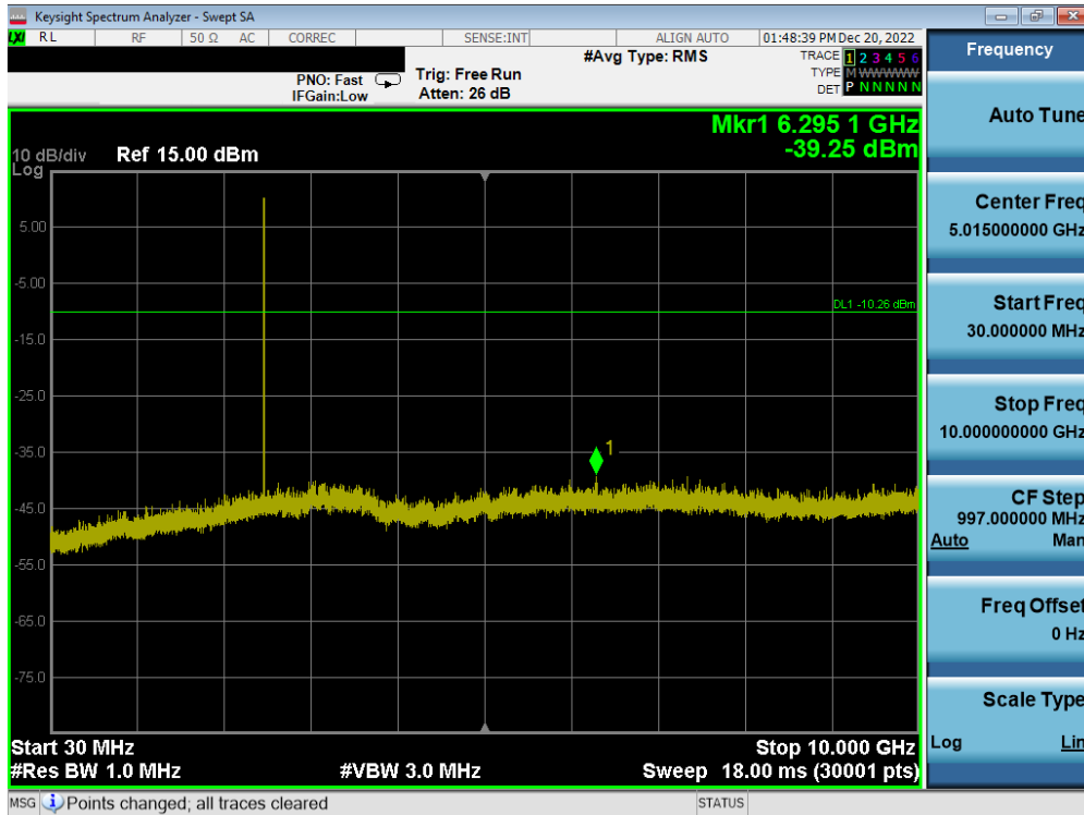
Plot 7-93. Conducted Spurious Plot (Bluetooth (LE), 2Mbps – Ch. 39) – ANT 1
