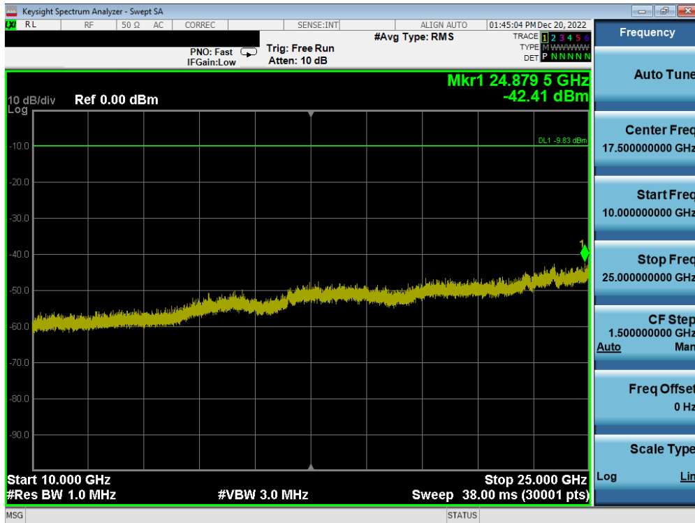
Plot 7-90. Conducted Spurious Plot (Bluetooth (LE), 2Mbps – Ch. 0) – ANT 1
