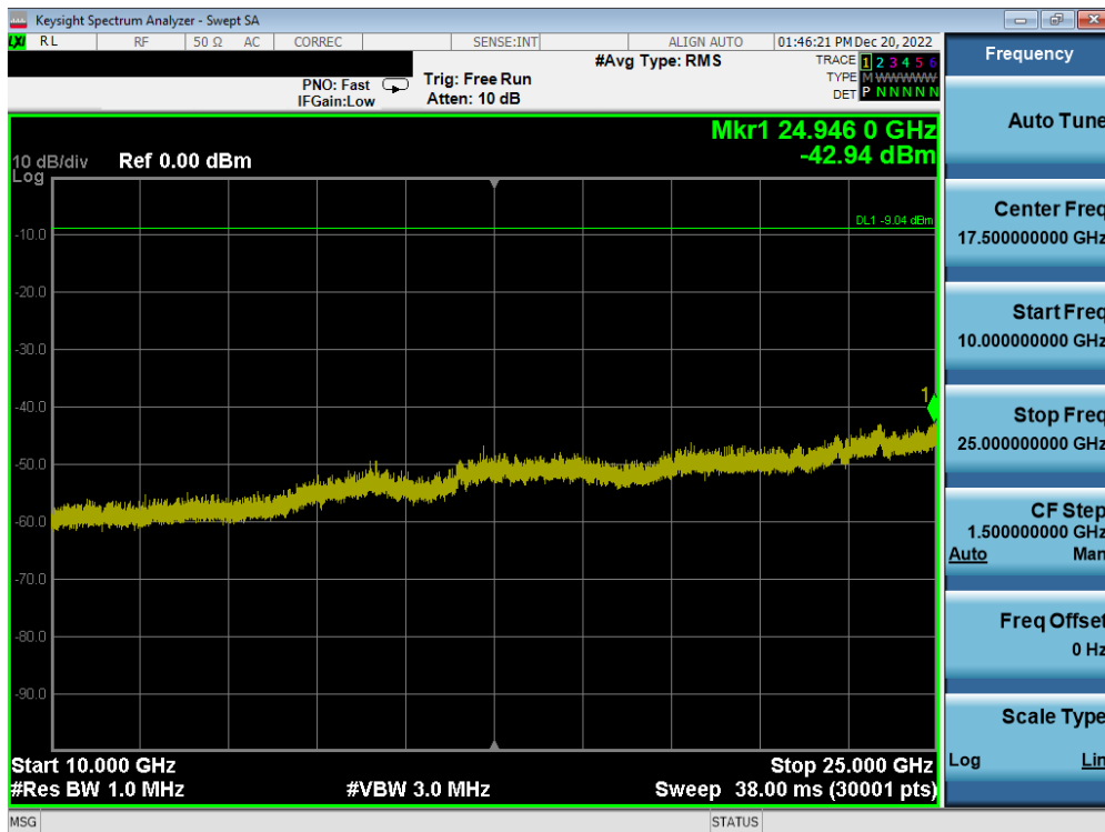
Plot 7-92. Conducted Spurious Plot (Bluetooth (LE), 2Mbps – Ch. 19) – ANT 1
