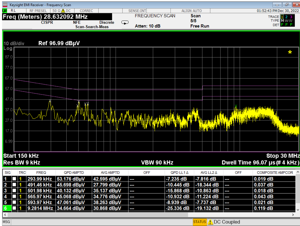
Plot 7-105. Line Conducted Plot with Bluetooth LE (L1) – ANT 1
