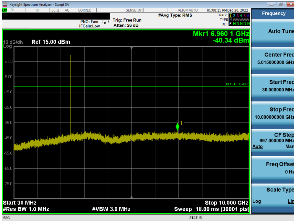
Plot 7-97. Conducted Spurious Plot (Bluetooth (LE), 2Mbps – Ch. 19) – ANT 2
