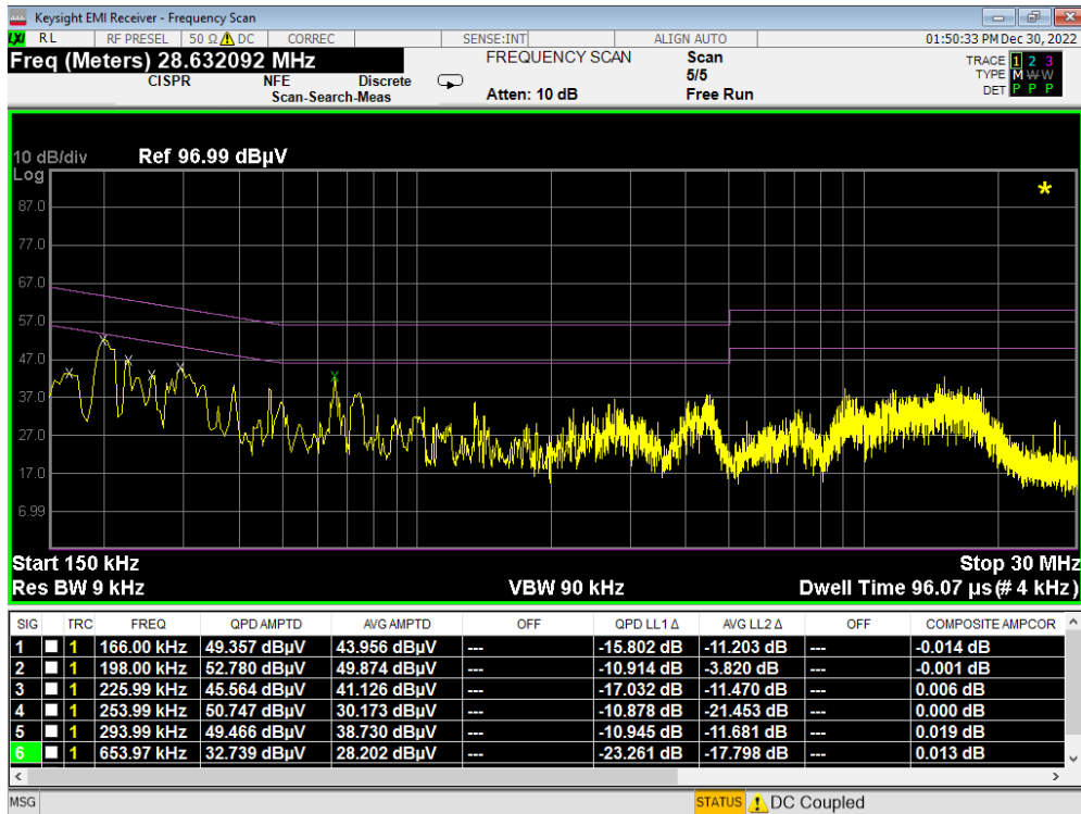
Plot 7-106. Line Conducted Plot with Bluetooth LE (N) -ANT 1
