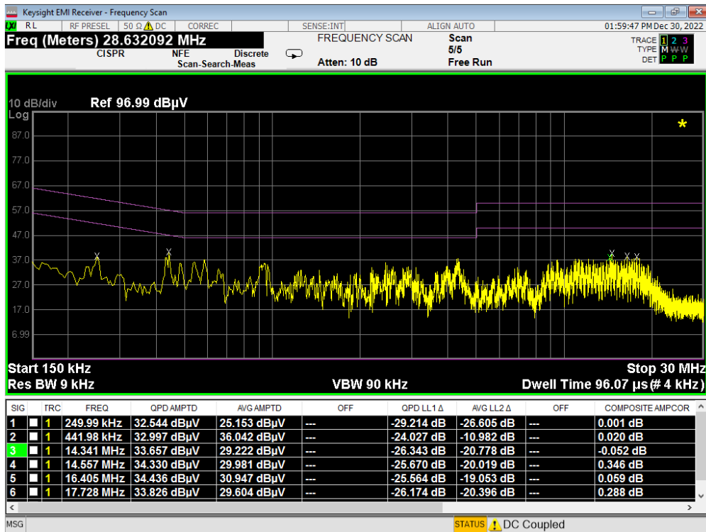
Plot 7-108. Line Conducted Plot with Bluetooth LE (N) -ANT 2
