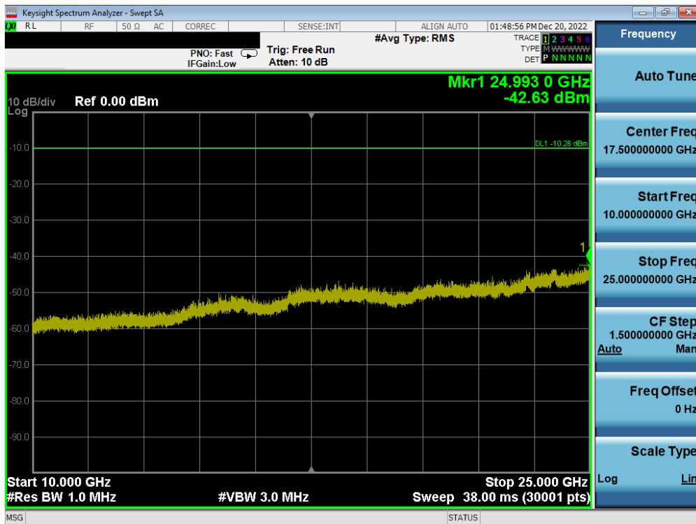
Plot 7-94. Conducted Spurious Plot (Bluetooth (LE), 2Mbps – Ch. 39) – ANT 1
