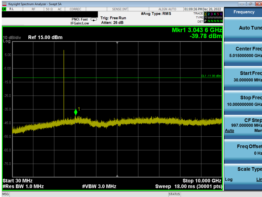
Plot 7-99. Conducted Spurious Plot (Bluetooth (LE), 2Mbps – Ch. 39) – ANT 2
