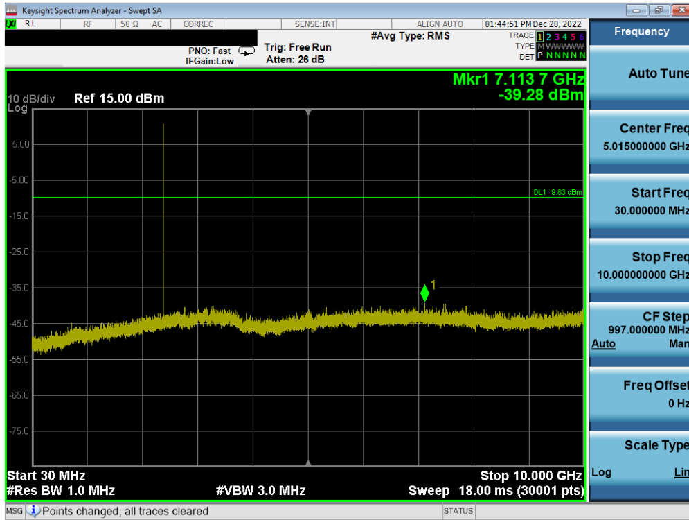
Plot 7-89. Conducted Spurious Plot (Bluetooth (LE), 2Mbps – Ch. 0) – ANT 1
