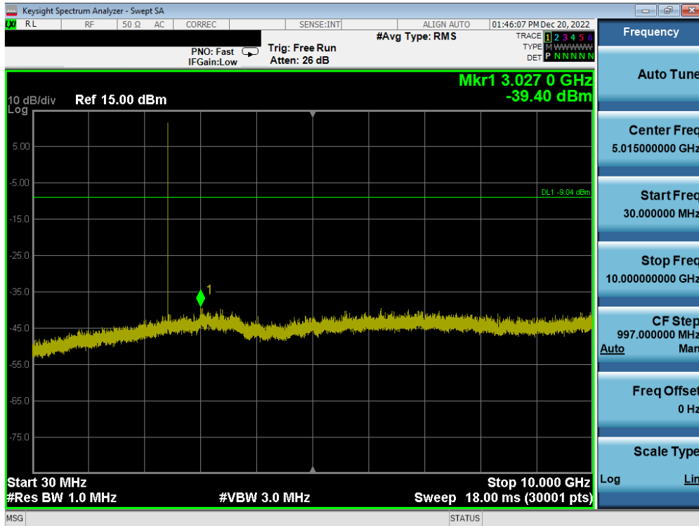
Plot 7-91. Conducted Spurious Plot (Bluetooth (LE), 2Mbps – Ch. 19) – ANT 1
