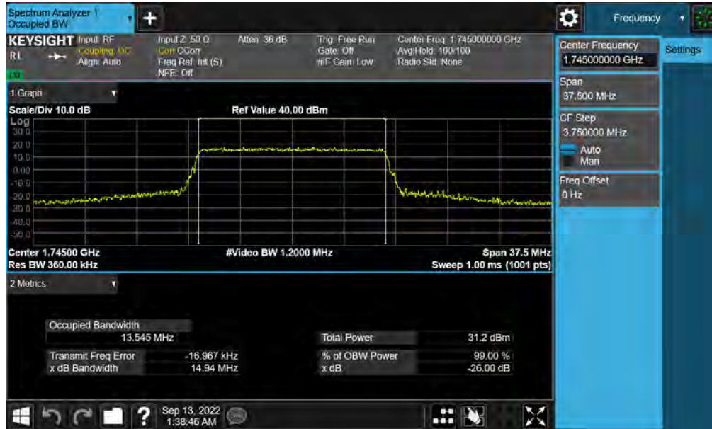
Plot 7-15. Occupied Bandwidth Plot (LTE Band 66/4 - 15MHz QPSK - Full RB)
