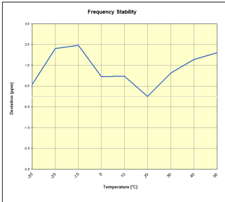
Plot 7-117. LTE Band 13 Frequency Stability Chart
