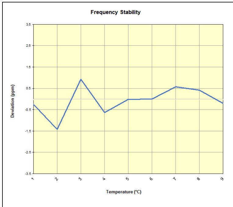
Plot 7-118. LTE Band 66/4 Frequency Stability Chart
