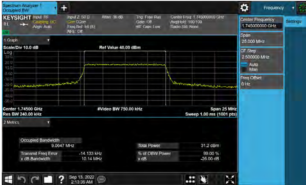
Plot 7-17. Occupied Bandwidth Plot (LTE Band 66/4 - 10MHz QPSK - Full RB)
