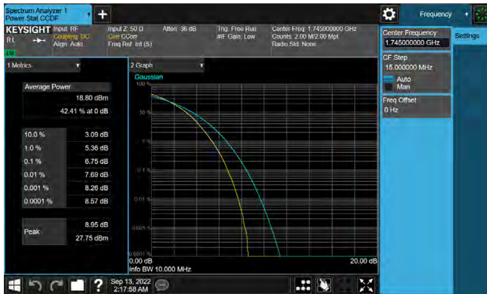
Plot 7-103. PAR Plot (LTE Band 66/4 - 10MHz 256-QAM - Full RB)
