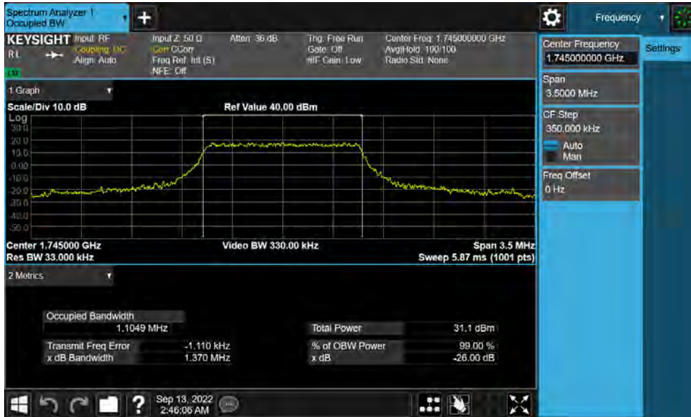
Plot 7-23. Occupied Bandwidth Plot (LTE Band 66/4 - 1.4MHz QPSK - Full RB)
