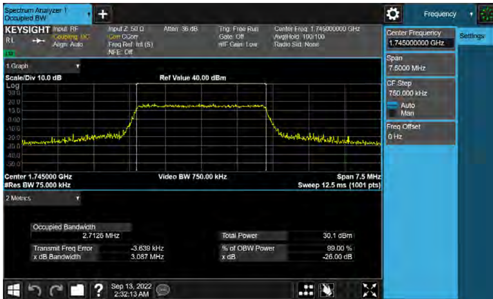
Plot 7-22. Occupied Bandwidth Plot (LTE Band 66/4 - 3MHz 16-QAM - Full RB)
