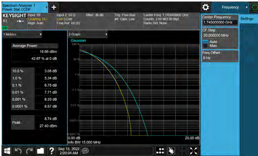
Plot 7-101. PAR Plot (LTE Band 66/4 - 15MHz 256-QAM - Full RB)
