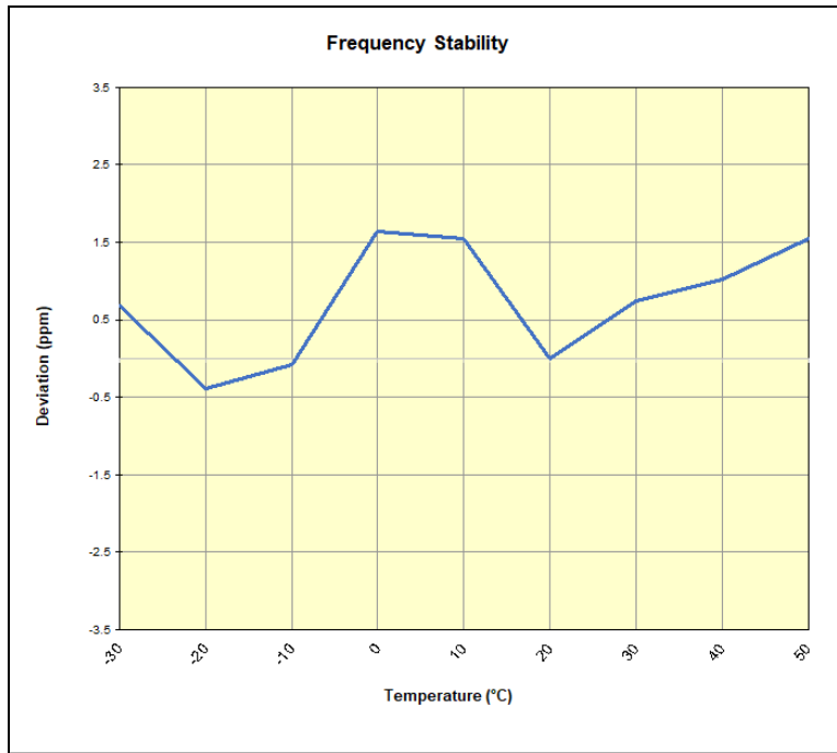
Plot 7-116. LTE Band 12 Frequency Stability Chart
