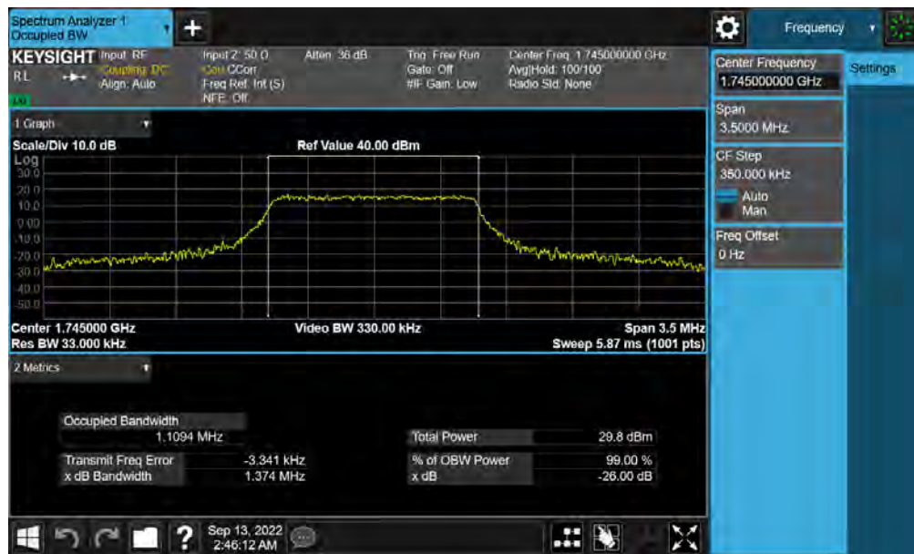
Plot 7-24. Occupied Bandwidth Plot (LTE Band 66/4 - 1.4MHz 16-QAM - Full RB)
