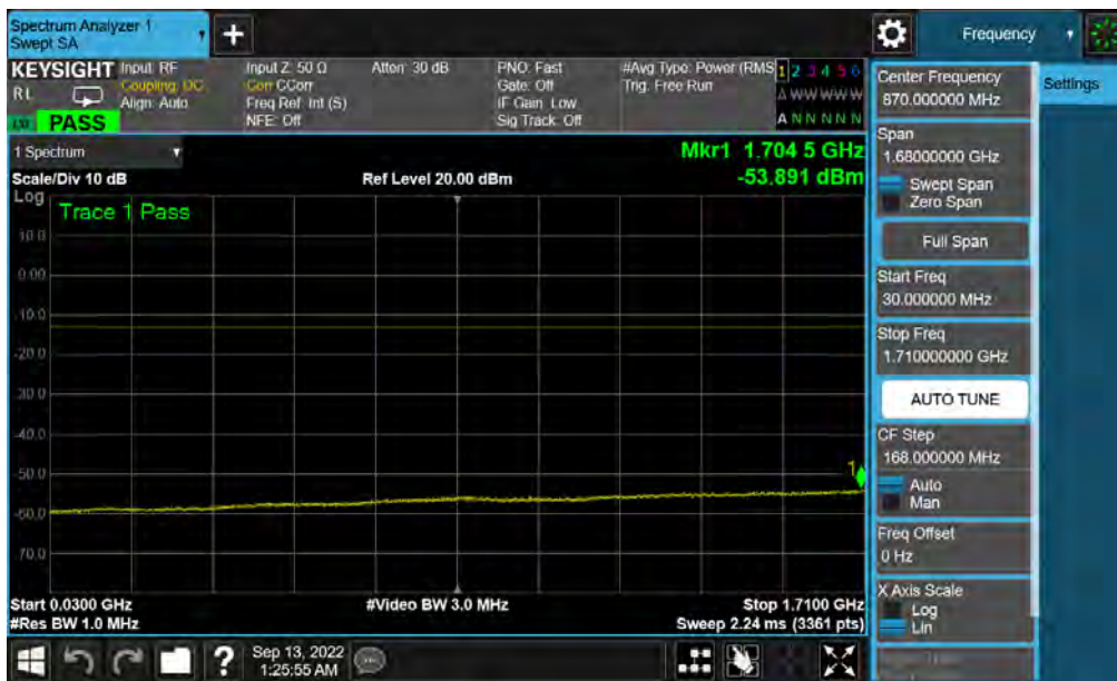
Plot 7-40. Conducted Spurious Plot (LTE Band 66/4 - 20MHz QPSK - 1 RB - Mid Channel)
