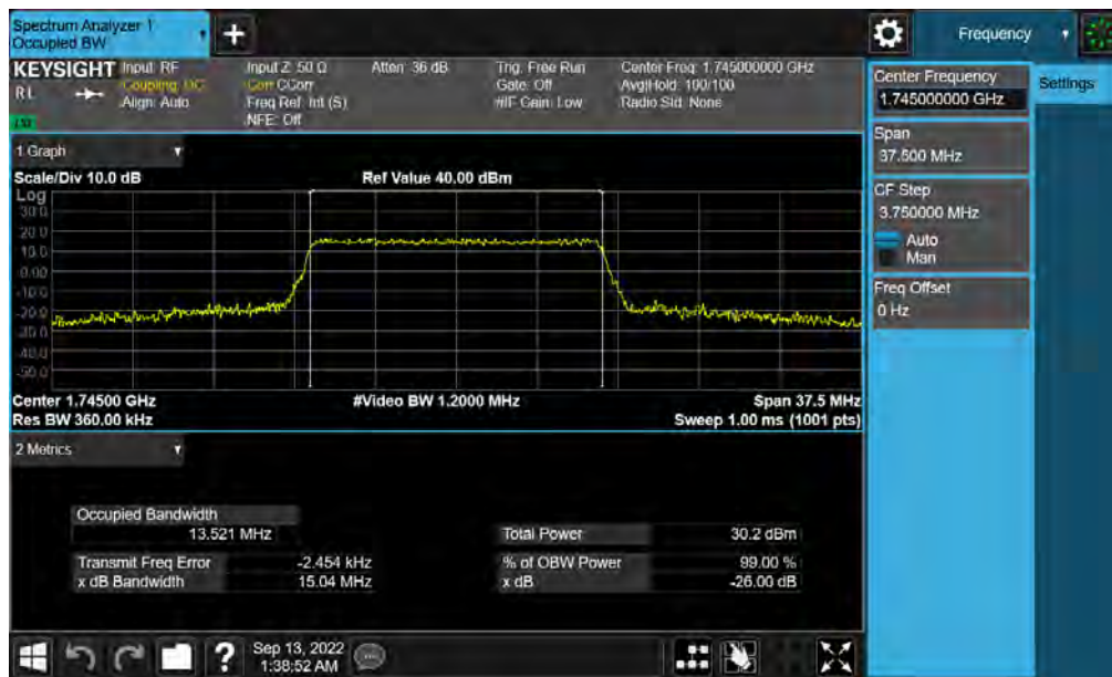
Plot 7-16. Occupied Bandwidth Plot (LTE Band 66/4 - 15MHz 16-QAM - Full RB)
