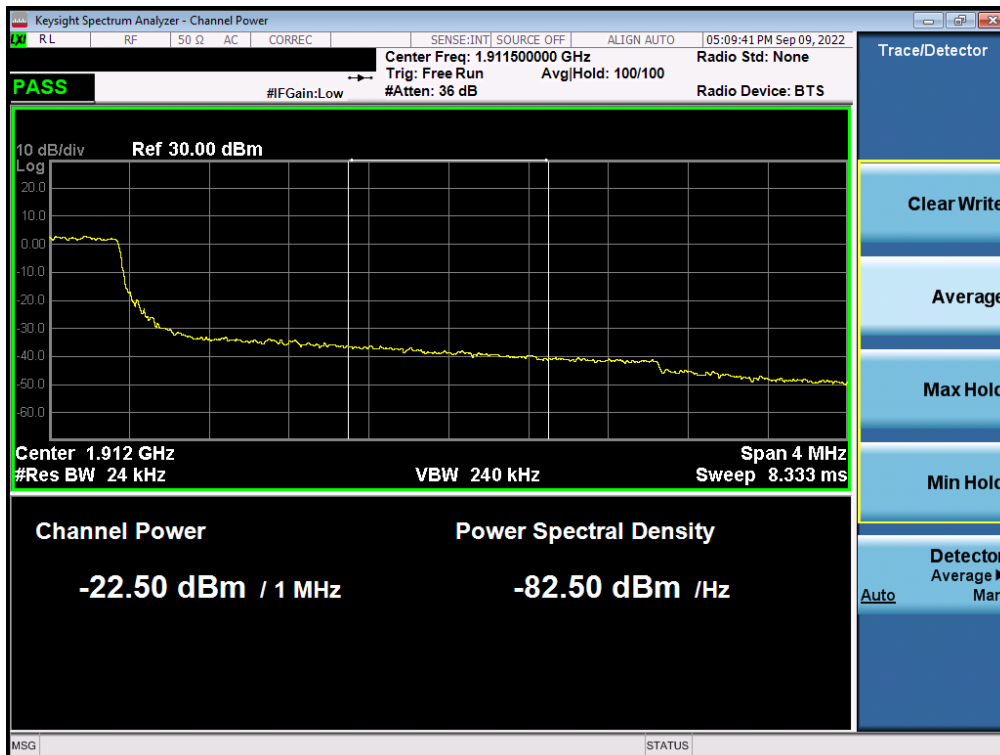
Plot 7-52. Extended Upper Band Edge Plot (LTE Band 2 - 3MHz QPSK – Full RB)
