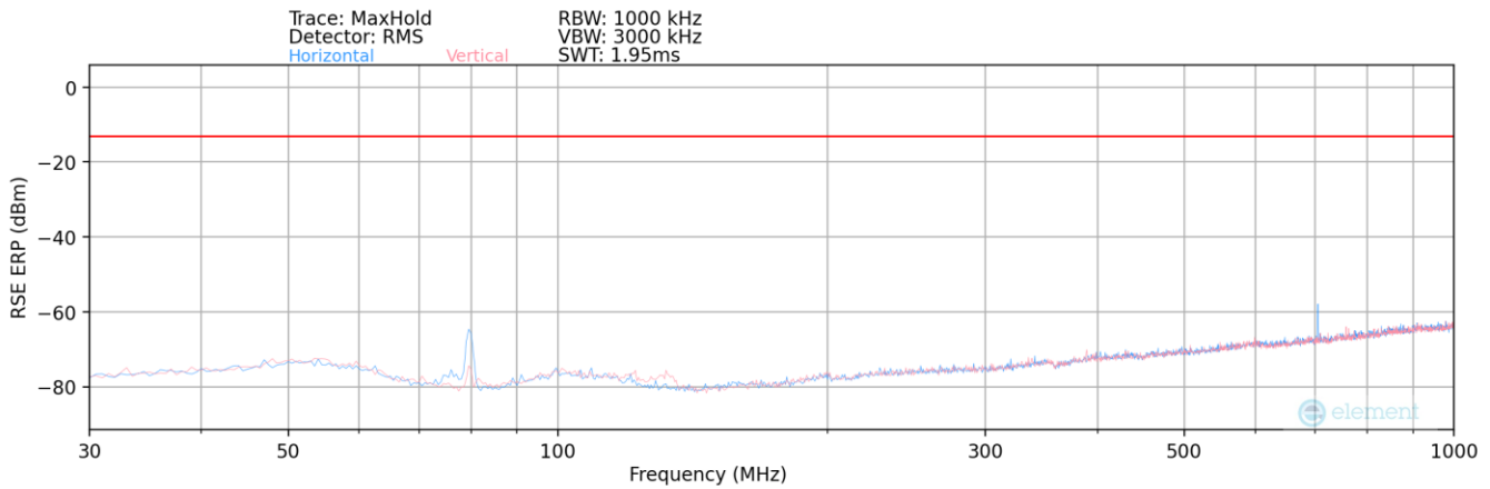
Plot 7-76. Radiated Spurious Plot <1GHz (GPRS PCS)
