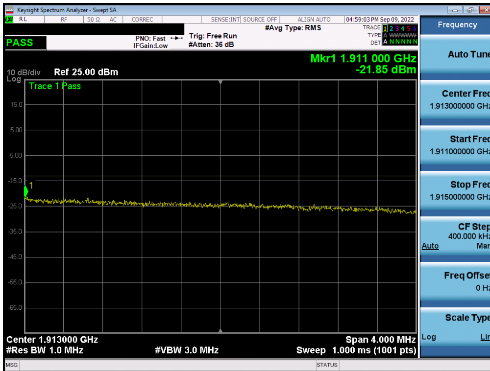
Plot 7-44. Extended Upper Band Edge Plot (LTE Band 2 - 10MHz QPSK – Full RB)
