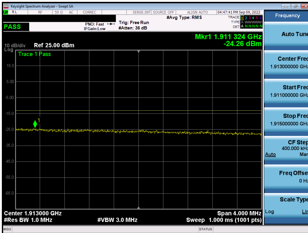
Plot 7-40. Extended Upper Band Edge Plot (LTE Band 2 - 15MHz QPSK – Full RB)
