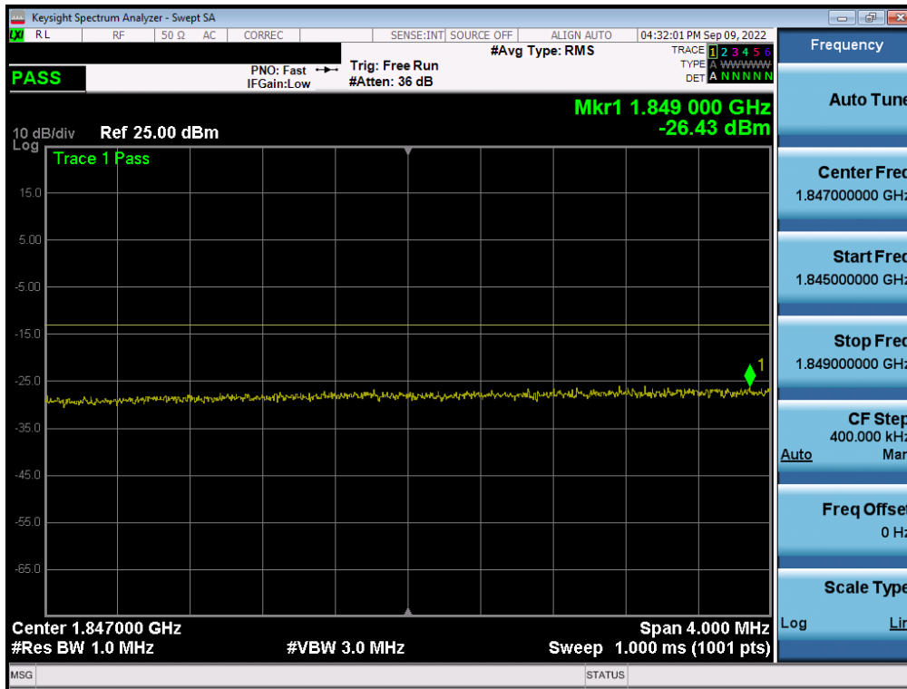
Plot 7-34. Extended Lower Band Edge Plot (LTE Band 2 - 20MHz QPSK – Full RB)
