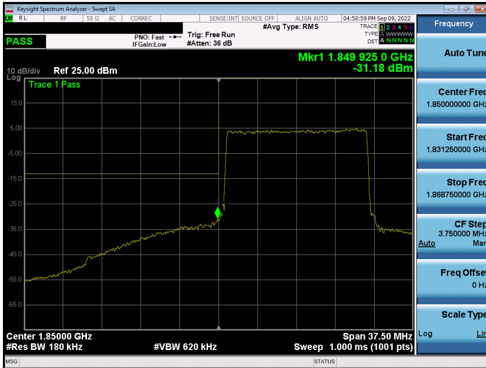
Plot 7-37. Lower Band Edge Plot (LTE Band 2 - 15MHz QPSK – Full RB)
