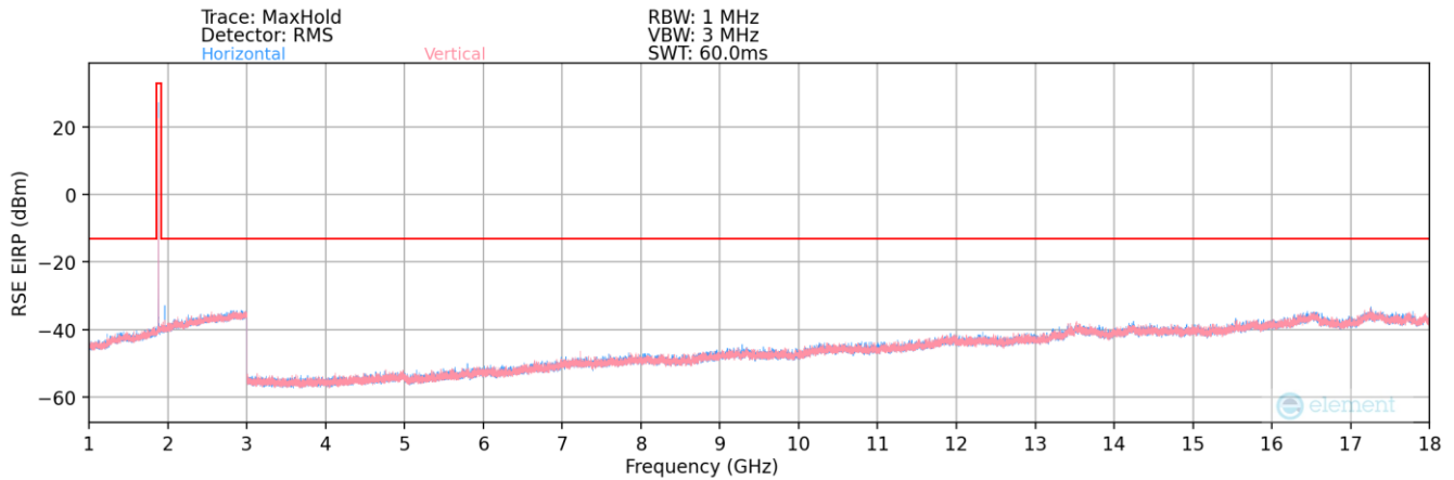
Plot 7-75. Radiated Spurious Plot >1GHz(GPRS PCS)
