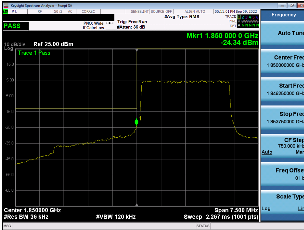
Plot 7-49. Lower Band Edge Plot (LTE Band 2 - 3MHz QPSK – Full RB)
