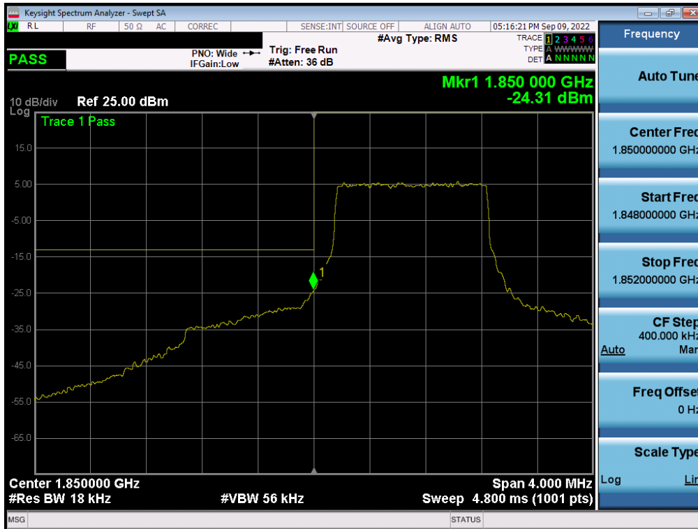
Plot 7-53. Lower Band Edge Plot (LTE Band 2 – 1.4MHz QPSK – Full RB)
