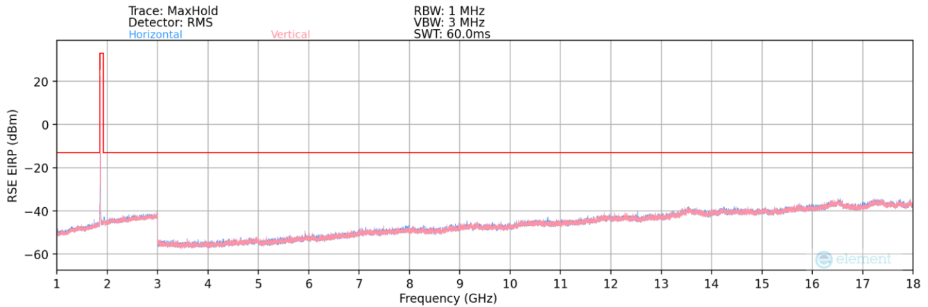
Plot 7-73. Radiated Spurious Plot >1GHz (LTE Band 2)
