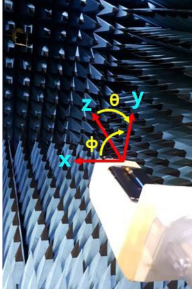
Figure 1: Geometry for SC-52D , SCG20 for Radiation patterns.
