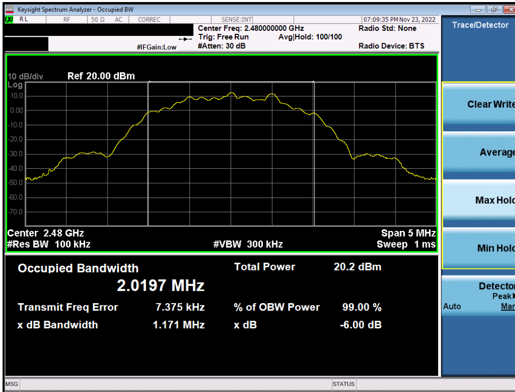
Plot 7-18. 6dB Bandwidth Plot (Bluetooth (LE), 2Mbps – Ch. 39) ANT2
