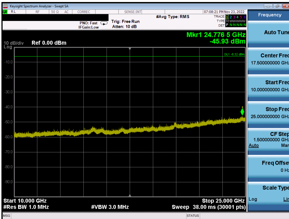
Plot 7-76. Conducted Spurious Plot (Bluetooth (LE), 2Mbps – Ch. 19) Ant2
