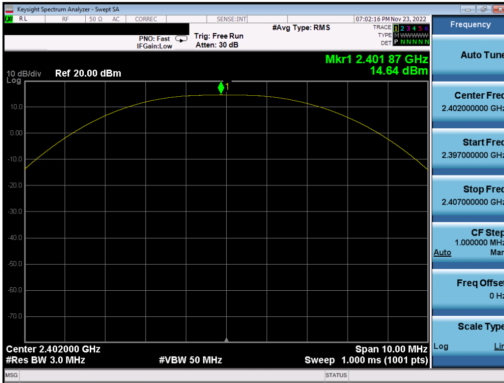
Plot 7-34. Peak Power Plot (Bluetooth (LE), 2Mbps – Ch. 0) Ant2
