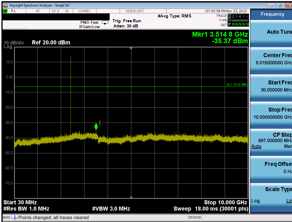
Plot 7-75. Conducted Spurious Plot (Bluetooth (LE), 2Mbps – Ch. 19) Ant2
