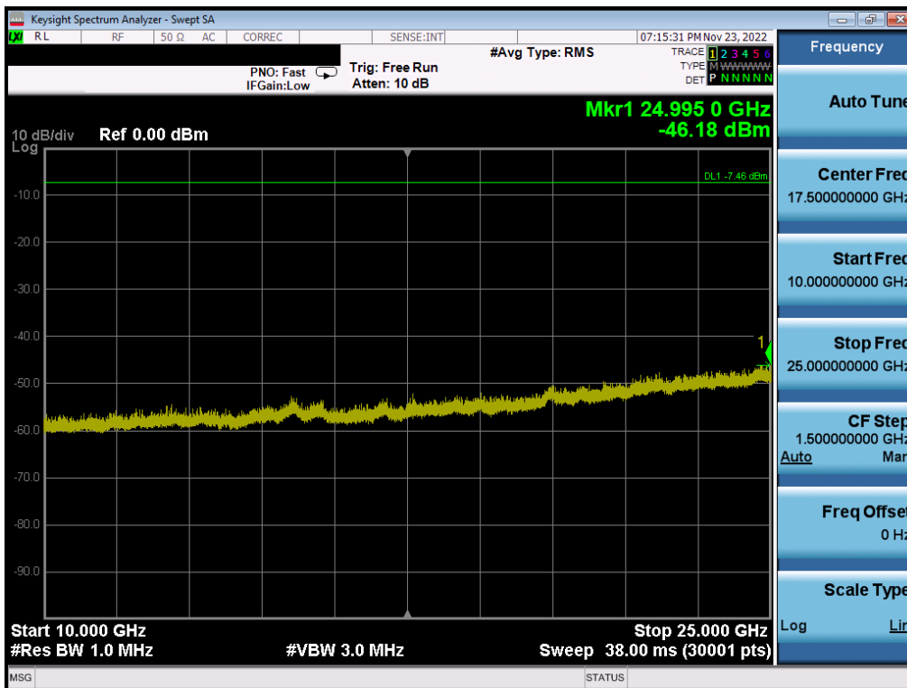
Plot 7-78. Conducted Spurious Plot (Bluetooth (LE), 2Mbps – Ch. 39) Ant2
