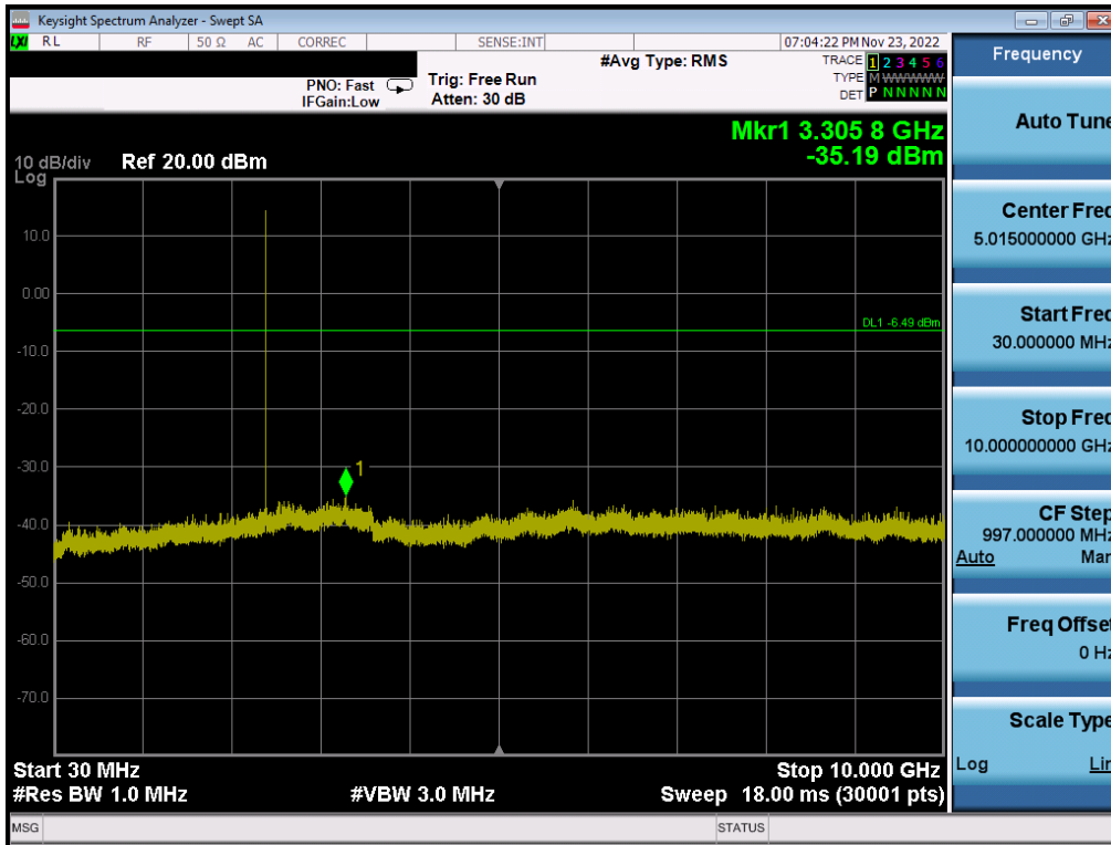
Plot 7-73. Conducted Spurious Plot (Bluetooth (LE), 2Mbps – Ch. 0) Ant2
