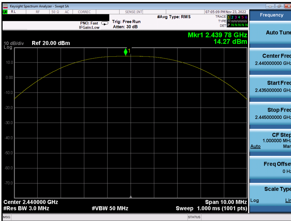
Plot 7-35. Peak Power Plot (Bluetooth (LE), 2Mbps – Ch. 19) Ant2
