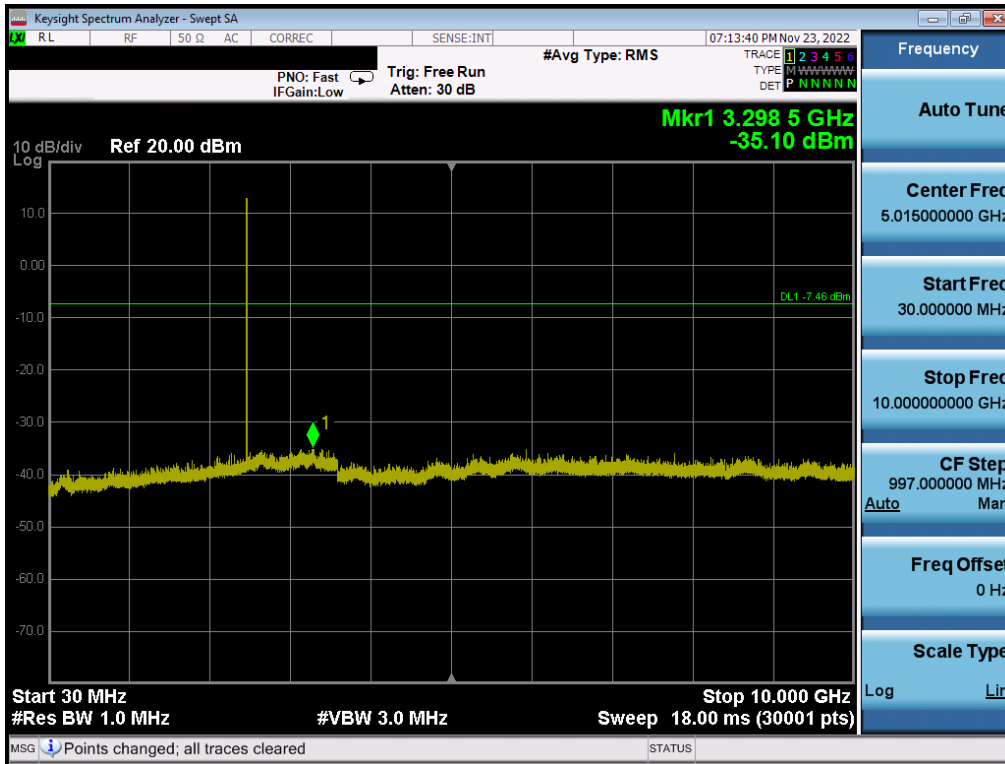
Plot 7-77. Conducted Spurious Plot (Bluetooth (LE), 2Mbps – Ch. 39) Ant2
