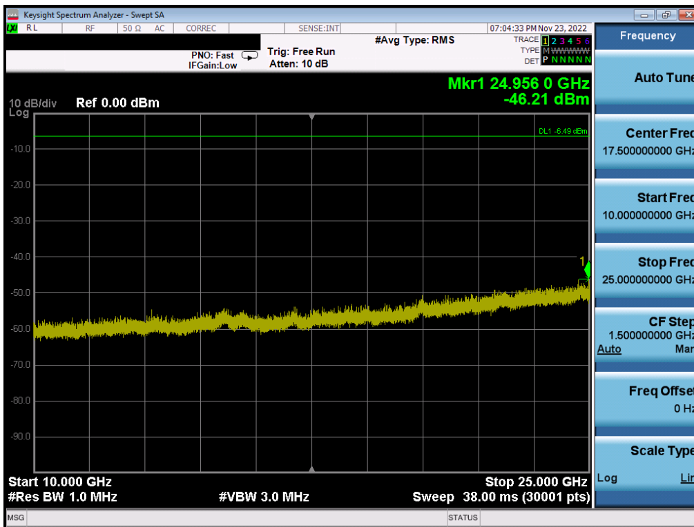
Plot 7-74. Conducted Spurious Plot (Bluetooth (LE), 2Mbps – Ch. 0) Ant2
