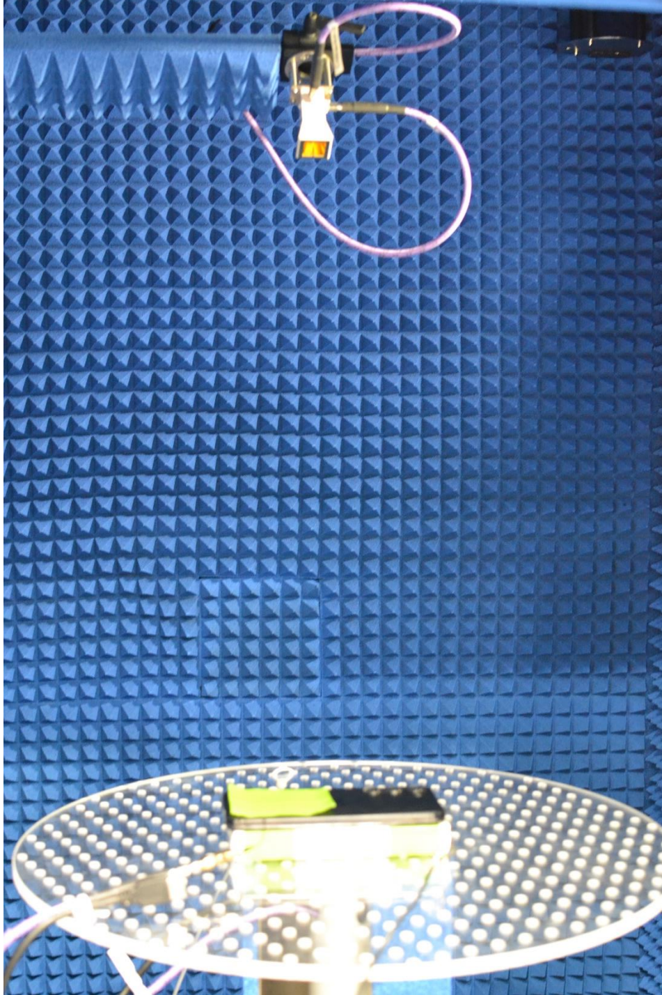
Test Setup Photo 7 – Conducted Test Setup (Figure 7-2)
