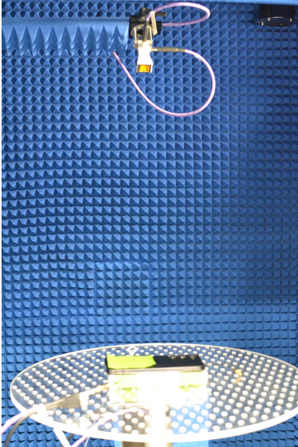
Test Setup Photo 6 – Conducted Test Setup (Figure 7-1)
