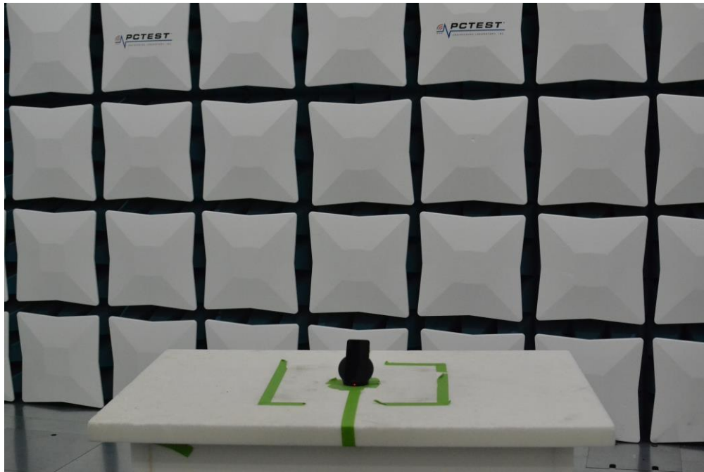
Figure 12. Test Setup – WCP Position – 30MHz-1GHz
