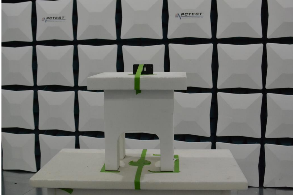
Figure 3. Test Setup – Y Position – 1GHz-18GHz
