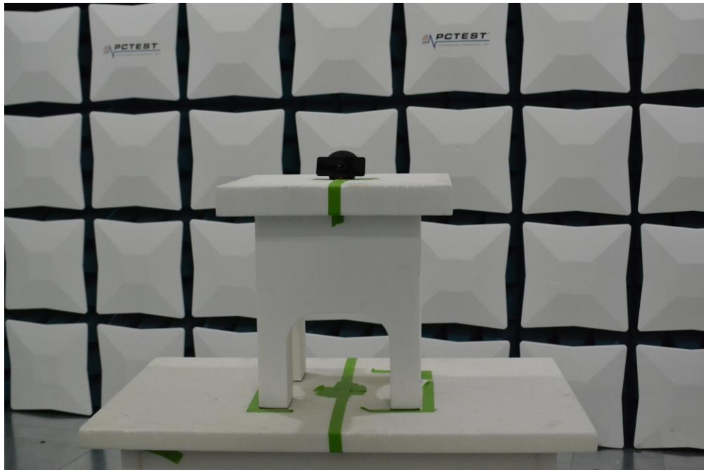
Figure 8. Test Setup – WCP Position – 1GHz-18GHz
