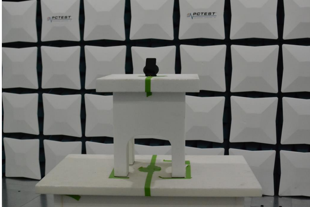
Figure 7. Test Setup – WCP Position – 1GHz-18GHz
