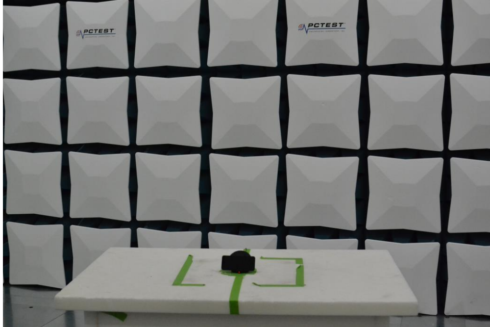
Figure 13. Test Setup – WCP Position – 30MHz-1GHz
