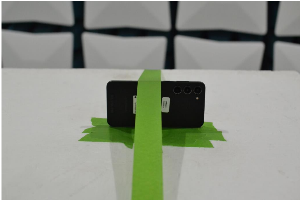
Figure 4. Test Setup – Y Position – 1GHz-18GHz
