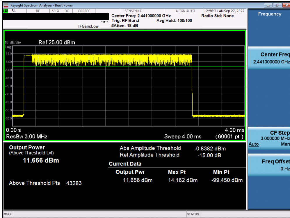
Plot 7-50. Average Conducted Power (2Mbps – Ch. 39) – Antenna 2
