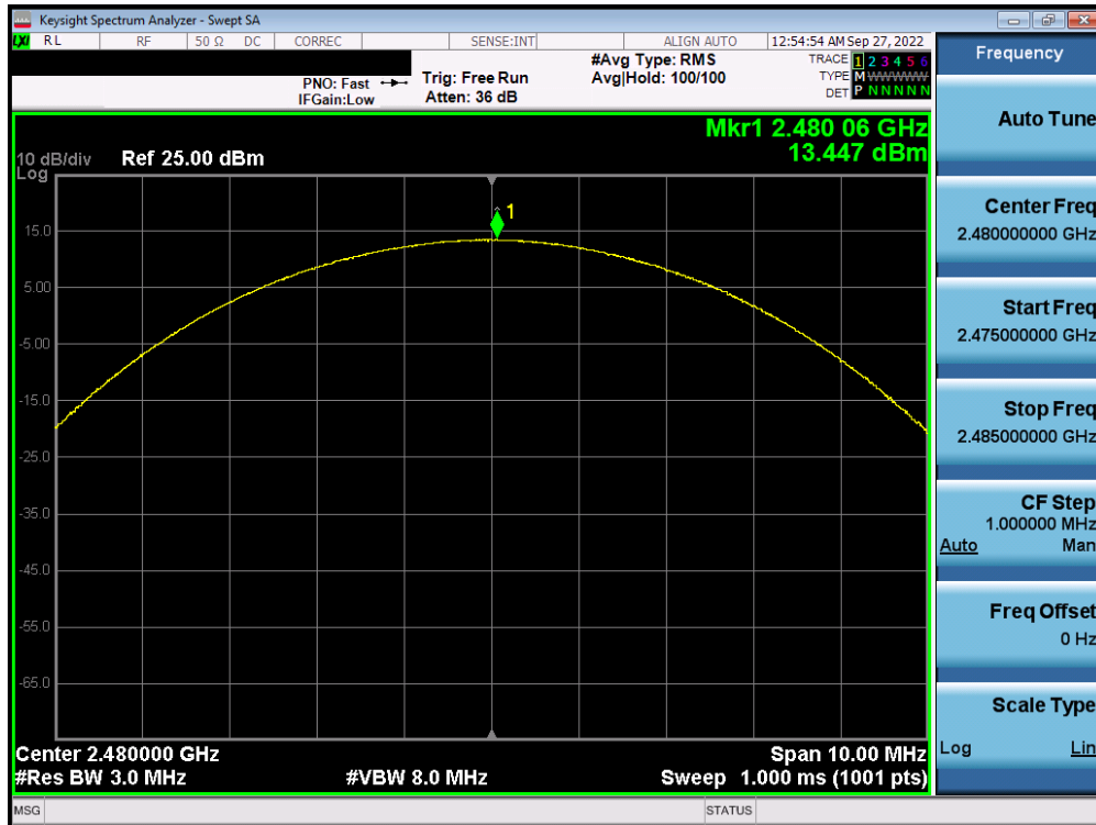
Plot 7-27. Peak Conducted Power (3Mbps – Ch. 78) – Antenna 1
