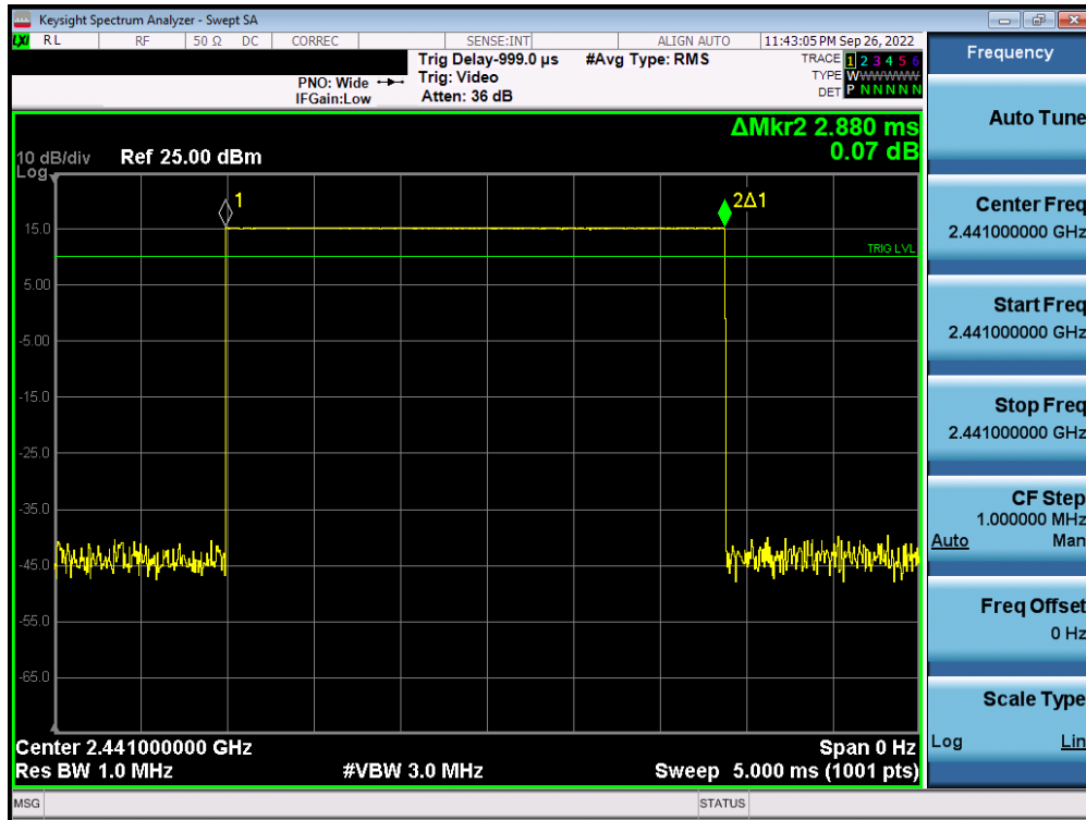
Plot 7-66. Time of Occupancy Plot (Bluetooth) – Antenna 2
