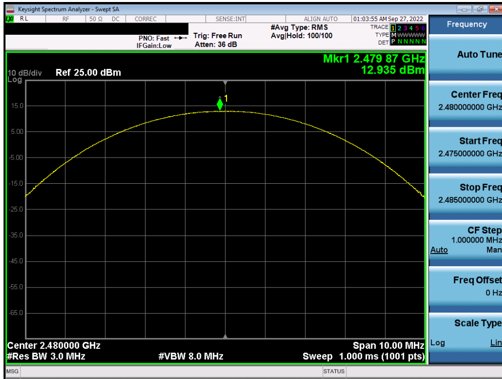
Plot 7-42. Peak Conducted Power (2Mbps – Ch. 78) – Antenna 2
