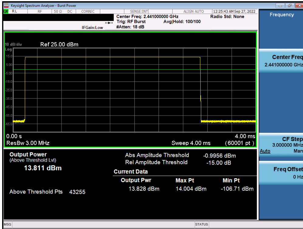
Plot 7-29. Average Conducted Power (1Mbps – Ch. 39) – Antenna 1
