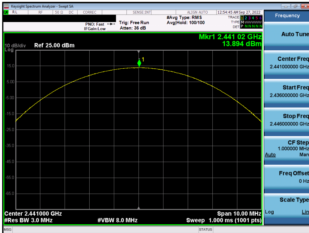
Plot 7-26. Peak Conducted Power (3Mbps - Ch. 39) - Antenna 1
