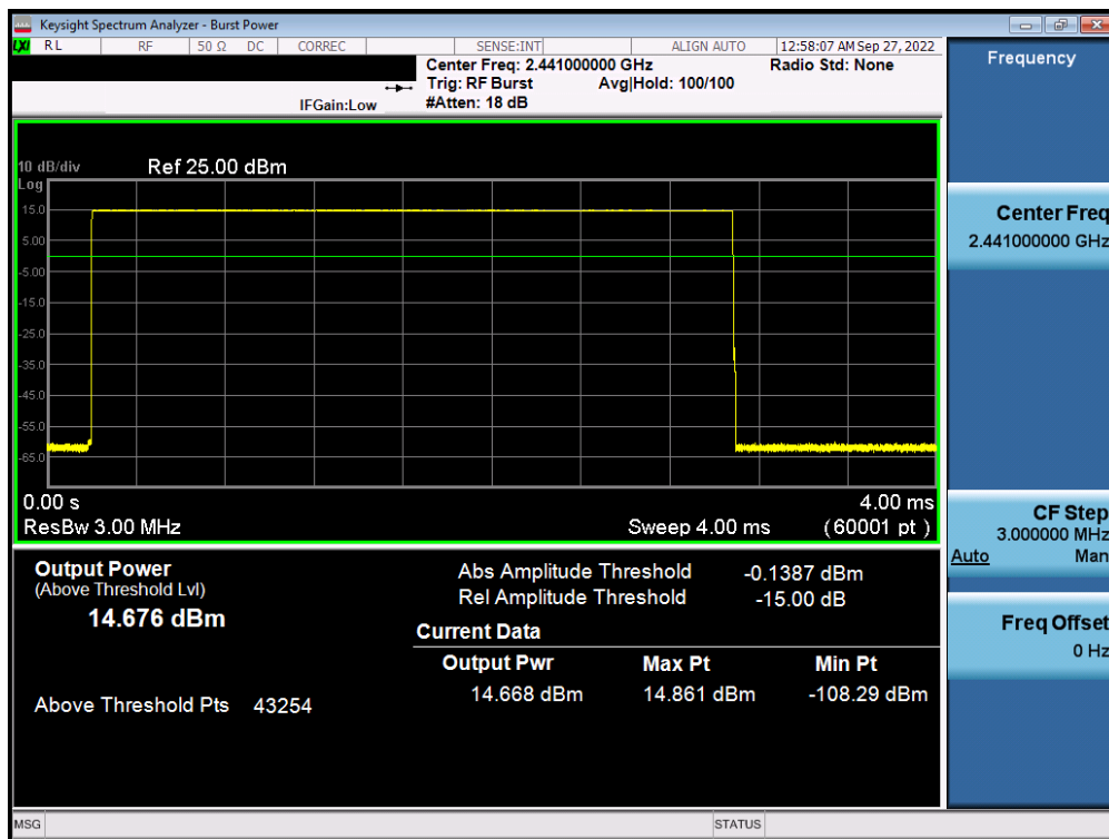
Plot 7-47. Average Conducted Power (1Mbps – Ch. 39) – Antenna 2
