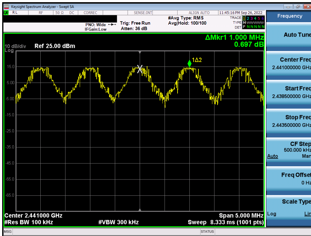
Plot 7-64. Channel Spacing Plot (Bluetooth) – Antenna 2
