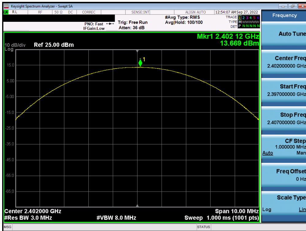
Plot 7-22. Peak Conducted Power (2Mbps – Ch. 0) – Antenna 1
