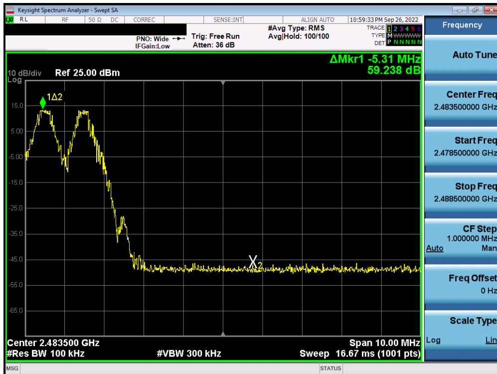
Plot 7-58. Band Edge Plot (Bluetooth with Hopping Enabled, 1 Mbps) – Antenna 1
