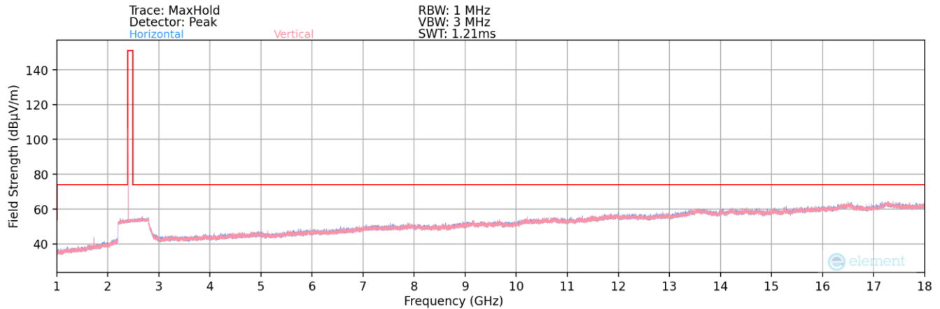
Plot 7-88. Radiated Spurious Plot above 1GHz (BT- Ch. 0) – Antenna 2
