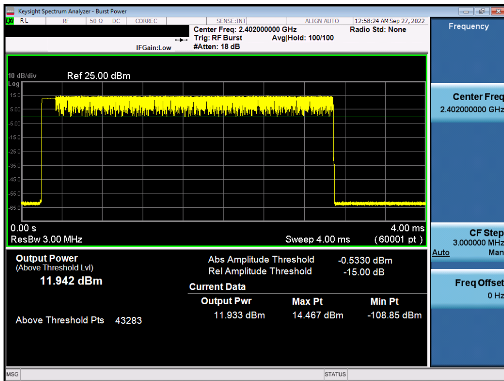
Plot 7-49. Average Conducted Power (2Mbps – Ch. 0) – Antenna 2
