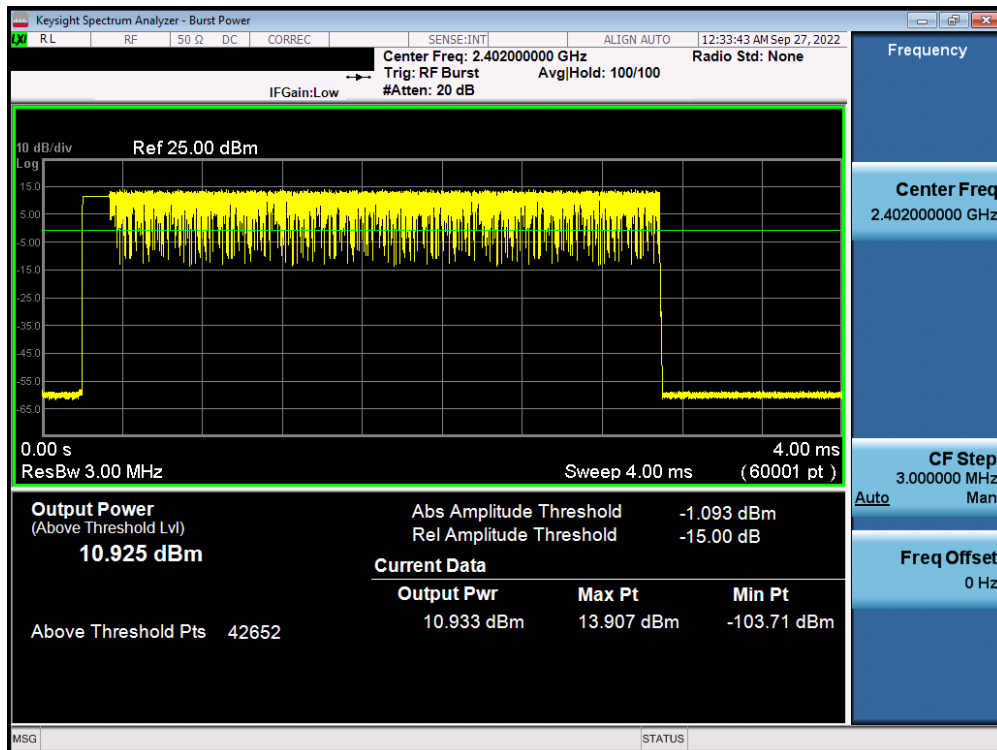
Plot 7-34. Average Conducted Power (3Mbps – Ch. 0) – Antenna 1
