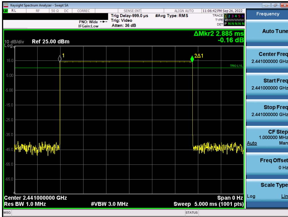
Plot 7-65. Time of Occupancy Plot (Bluetooth) – Antenna 1
