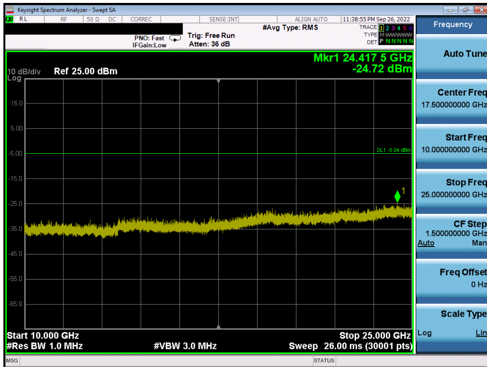
Plot 7-79. Conducted Spurious Plot (Bluetooth, 1Mbps – Ch. 0) – Antenna 2
