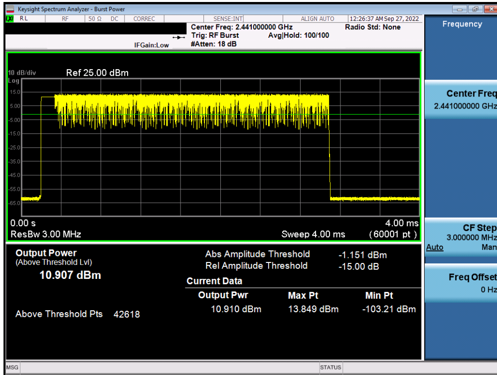
Plot 7-35. Average Conducted Power (3Mbps - Ch. 39) - Antenna 1
