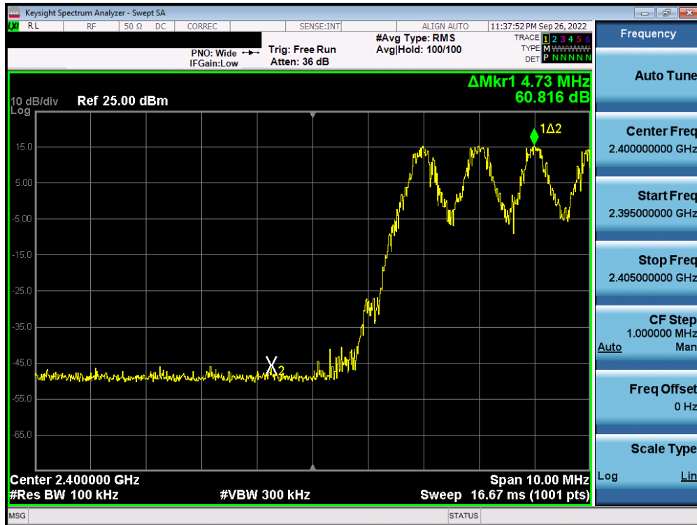
Plot 7-61. Band Edge Plot (Bluetooth with Hopping Enabled, 1 Mbps) – Antenna 2
