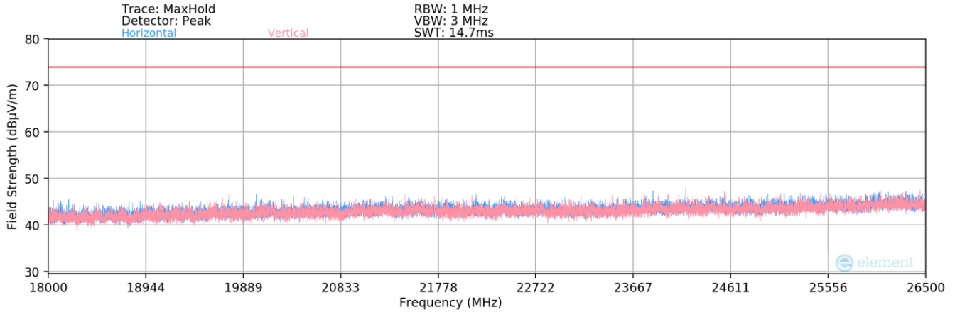
Plot 7-91. Radiated Spurious Plot above 18GHz– Antenna 2
