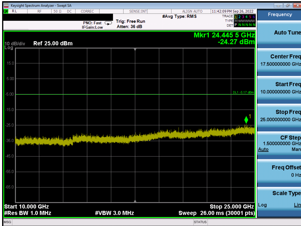
Plot 7-81. Conducted Spurious Plot (Bluetooth, 1Mbps – Ch. 39) – Antenna 2
