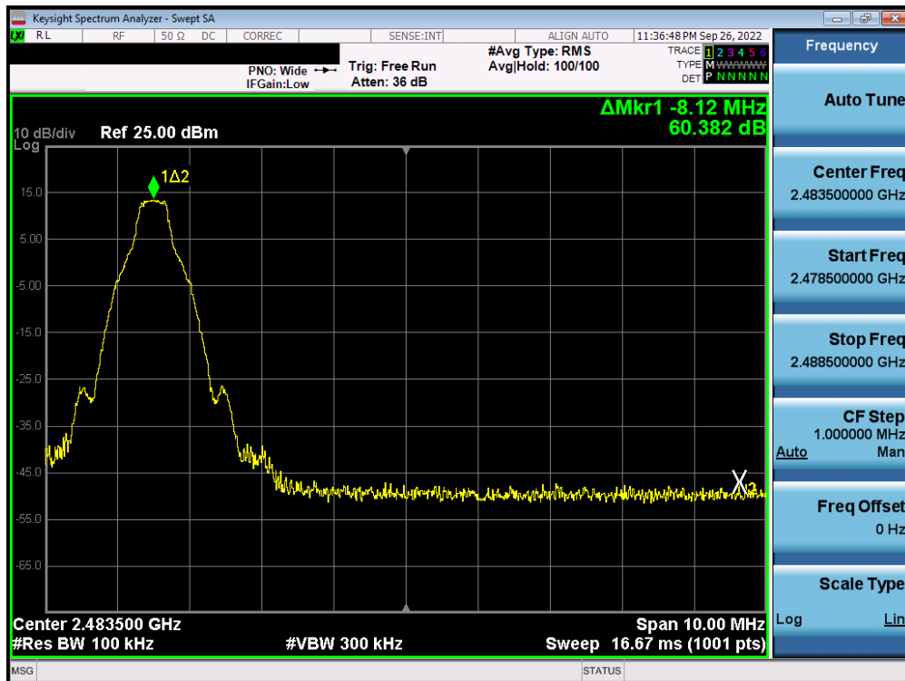
Plot 7-60. Band Edge Plot (Bluetooth with Hopping Disabled, 1 Mbps – Ch. 78) – Antenna 2
