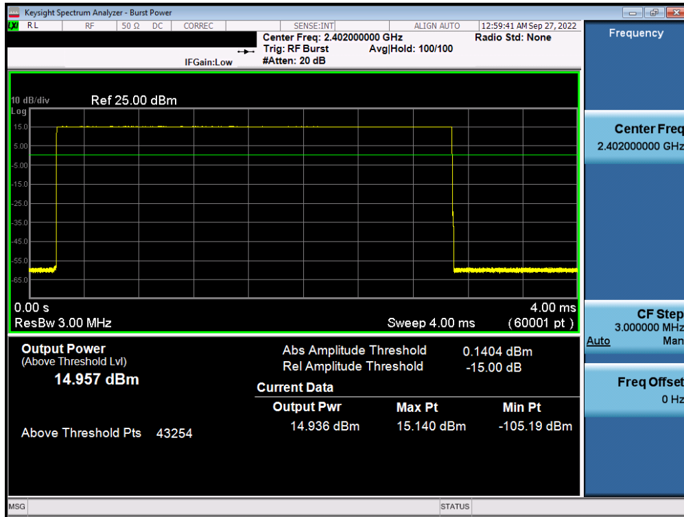
Plot 7-46. Average Conducted Power (1Mbps – Ch. 0) – Antenna 2
