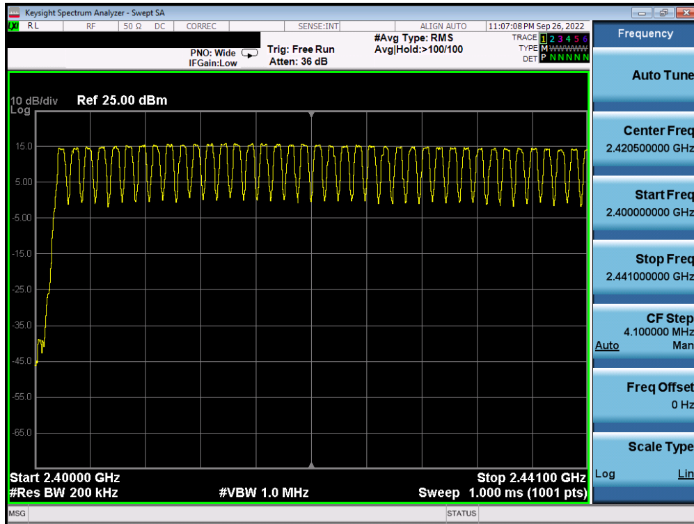
Plot 7-67. Low End Spectrum Channel Hopping Plot (Bluetooth) – Antenna 1
