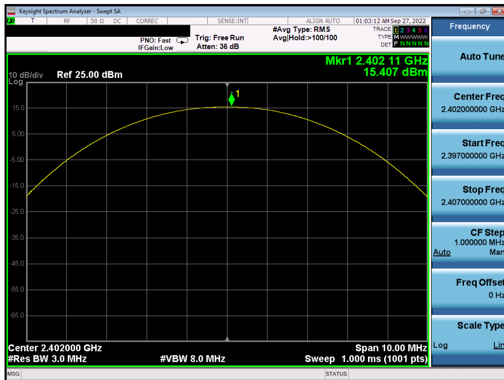
Plot 7-37. Peak Conducted Power (1Mbps – Ch. 0) – Antenna 2
