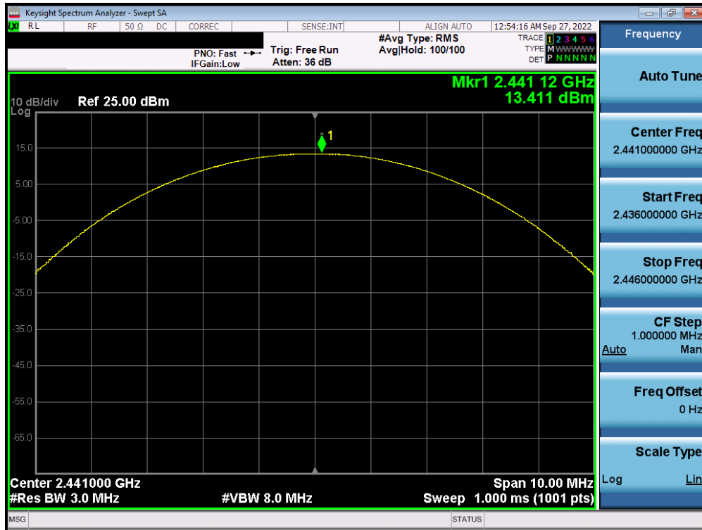
Plot 7-23. Peak Conducted Power (2Mbps – Ch. 39) – Antenna 1
