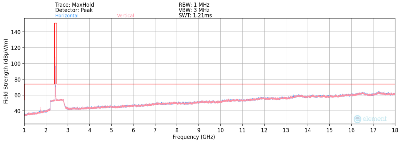
Plot 7-84. Radiated Spurious Plot above 1GHz (BT- Ch. 0) – Antenna 1
