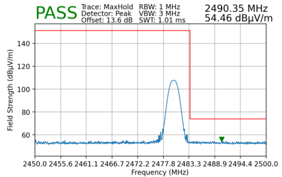
Plot 7-93. Radiated Restricted Upper Band Edge Measurement (Peak) – Antenna 1
