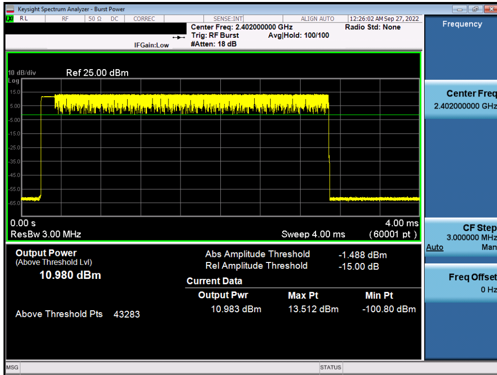
Plot 7-31. Average Conducted Power (2Mbps – Ch. 0) – Antenna 1
