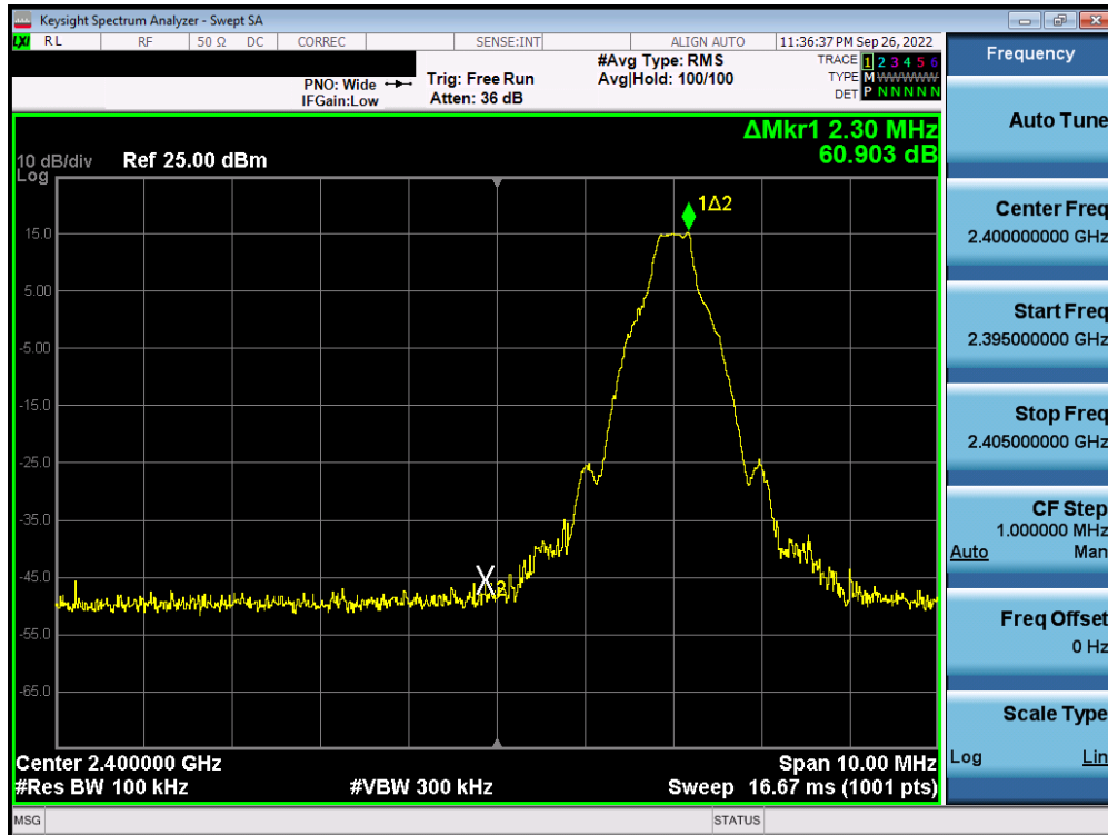
Plot 7-59. Band Edge Plot (Bluetooth with Hopping Disabled, 1 Mbps – Ch. 0) – Antenna 2
