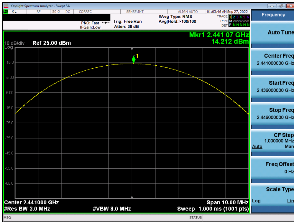
Plot 7-41. Peak Conducted Power (2Mbps – Ch. 39) – Antenna 2
