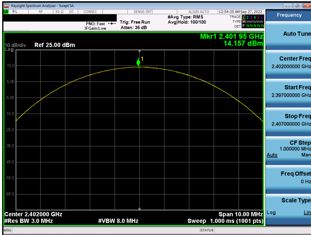
Plot 7-25. Peak Conducted Power (3Mbps - Ch. 0) - Antenna 1
