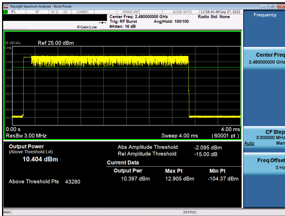
Plot 7-51. Average Conducted Power (2Mbps – Ch. 78) – Antenna 2
