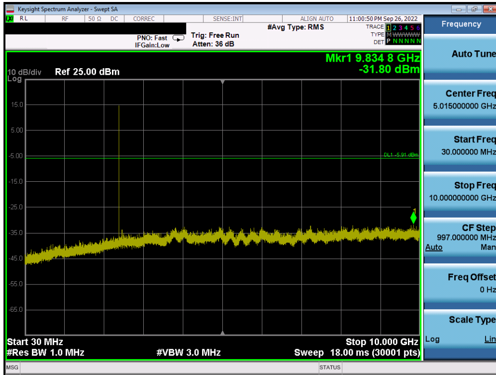
Plot 7-72. Conducted Spurious Plot (Bluetooth, 1Mbps – Ch. 0) – Antenna 1
