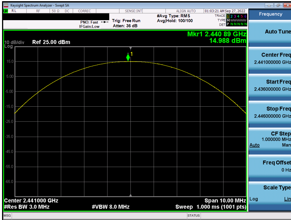
Plot 7-38. Peak Conducted Power (1Mbps – Ch. 39) – Antenna 2
