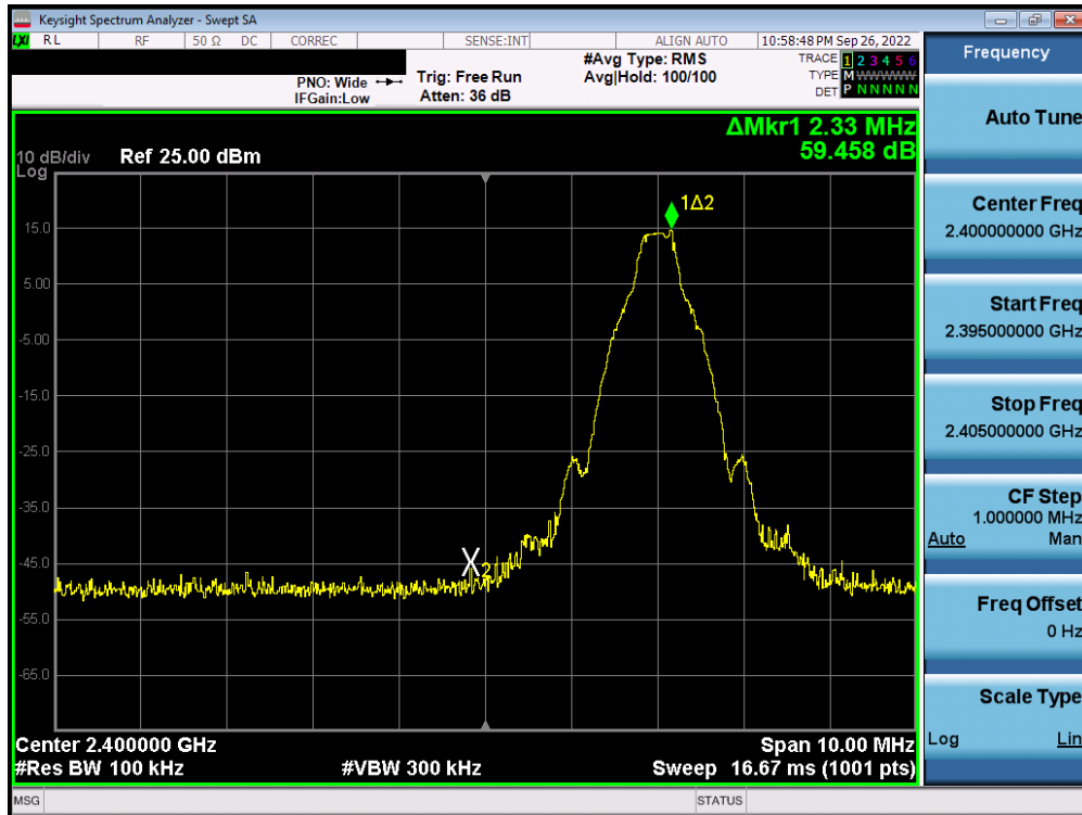
Plot 7-55. Band Edge Plot (Bluetooth with Hopping Disabled, 1 Mbps – Ch. 0) – Antenna 1
