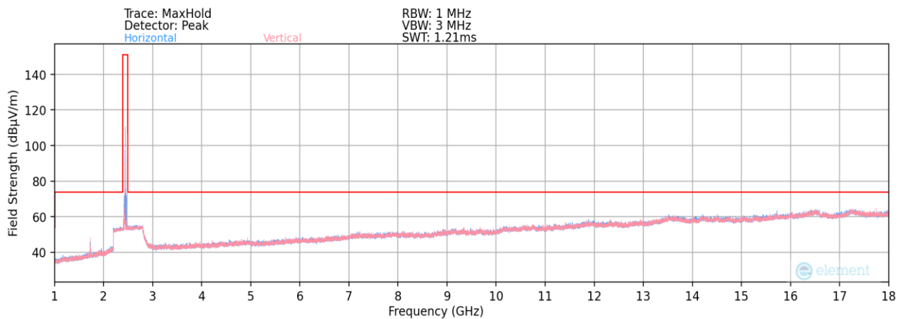
Plot 7-86. Radiated Spurious Plot above 1GHz (BT- Ch. 78) – Antenna 1
