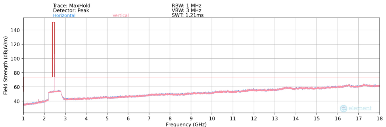
Plot 7-90. Radiated Spurious Plot above 1GHz (BT- Ch. 78) – Antenna 2
