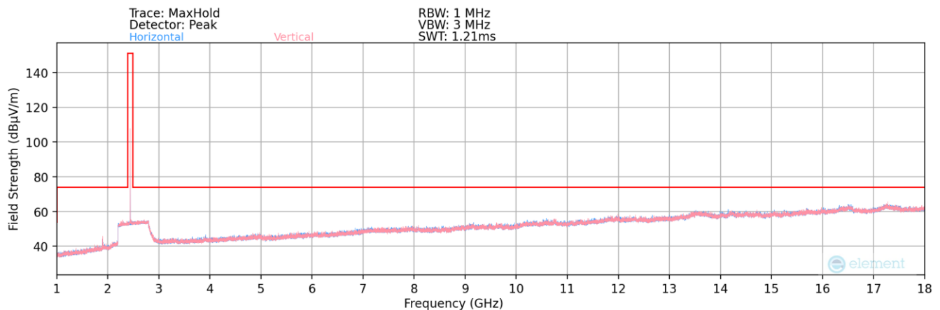
Plot 7-89. Radiated Spurious Plot above 1GHz (BT- Ch. 39) – Antenna 2
