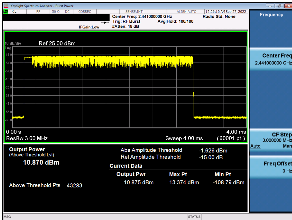
Plot 7-32. Average Conducted Power (2Mbps – Ch. 39) – Antenna 1
