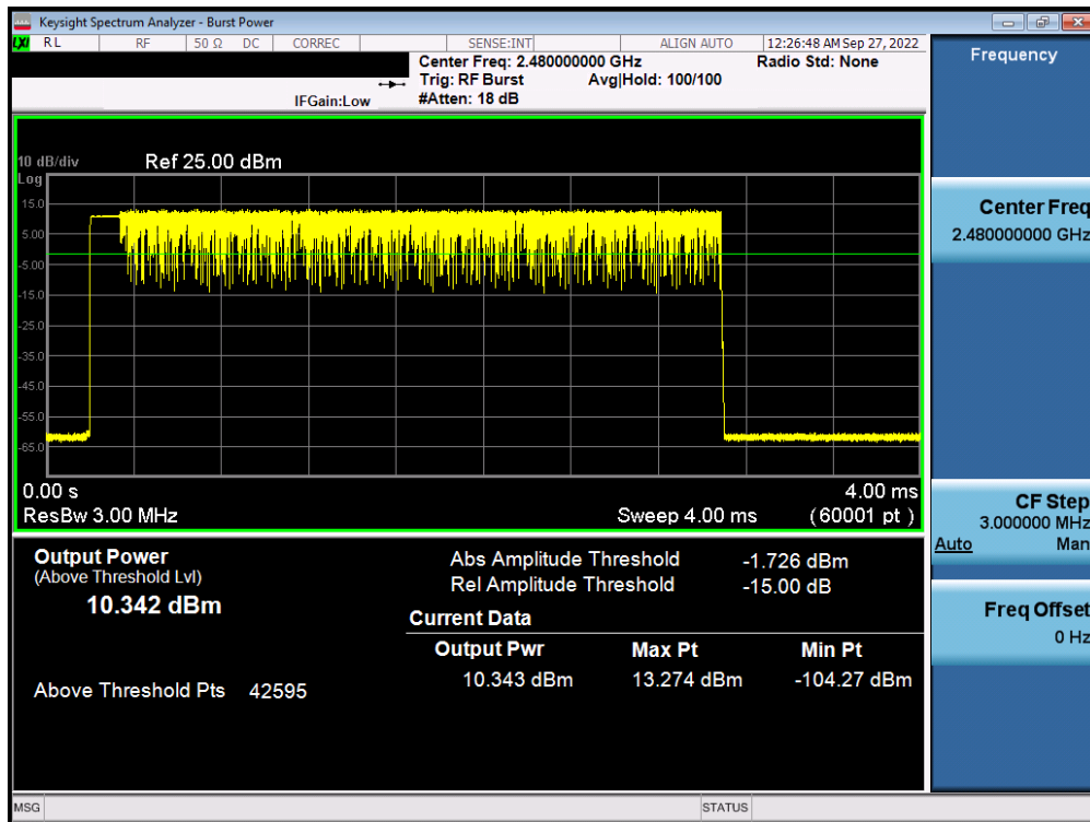
Plot 7-36. Average Conducted Power (3Mbps - Ch. 78) - Antenna 1
