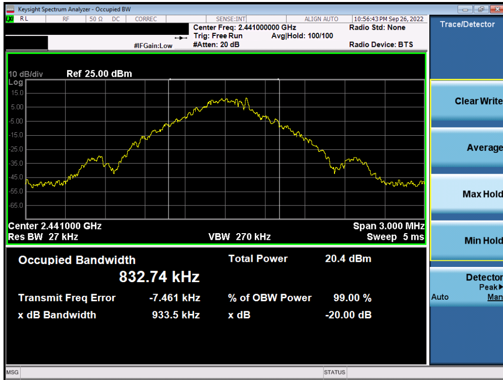
Plot 7-2. 20dB Bandwidth Plot (Bluetooth, 1Mbps – Ch. 39) – Antenna 1
