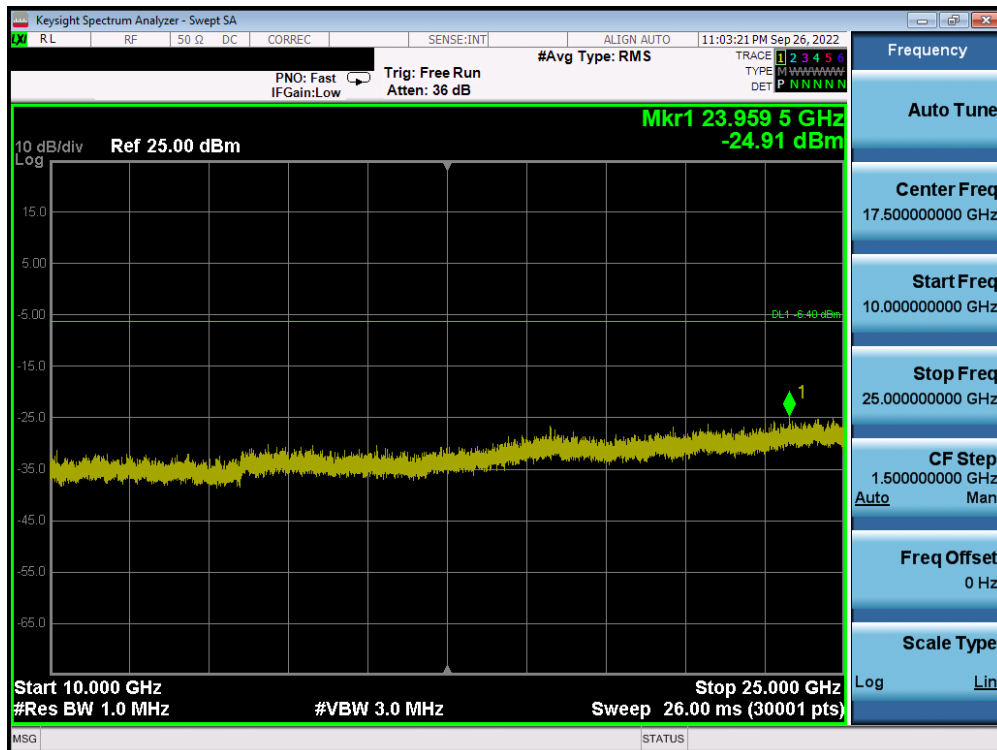
Plot 7-77. Conducted Spurious Plot (Bluetooth, 1Mbps – Ch. 78) – Antenna 1
