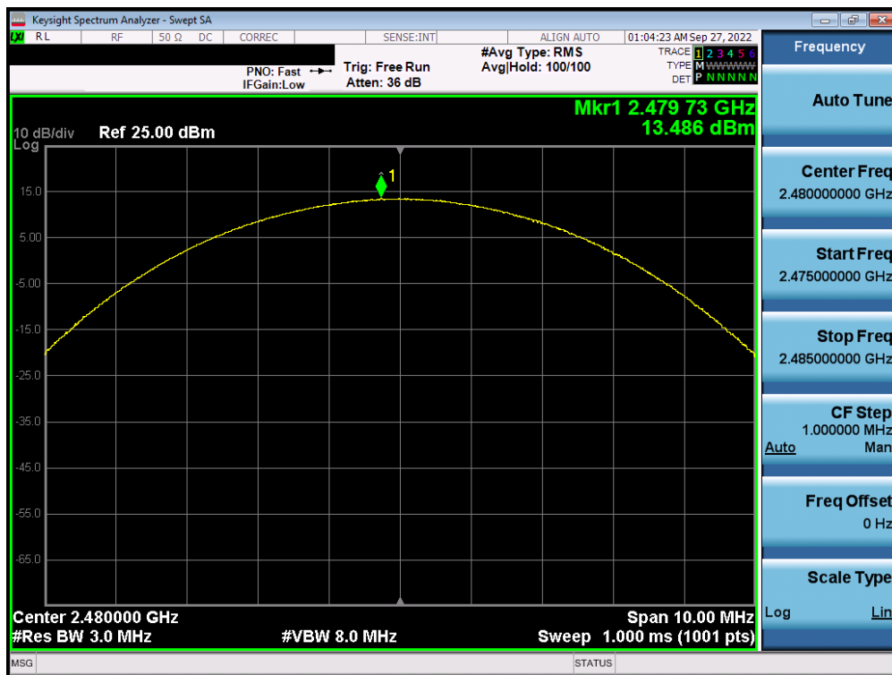
Plot 7-45. Peak Conducted Power (3Mbps – Ch. 78) – Antenna 2
