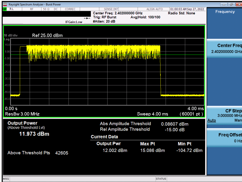
Plot 7-52. Average Conducted Power (3Mbps – Ch. 0) – Antenna 2
