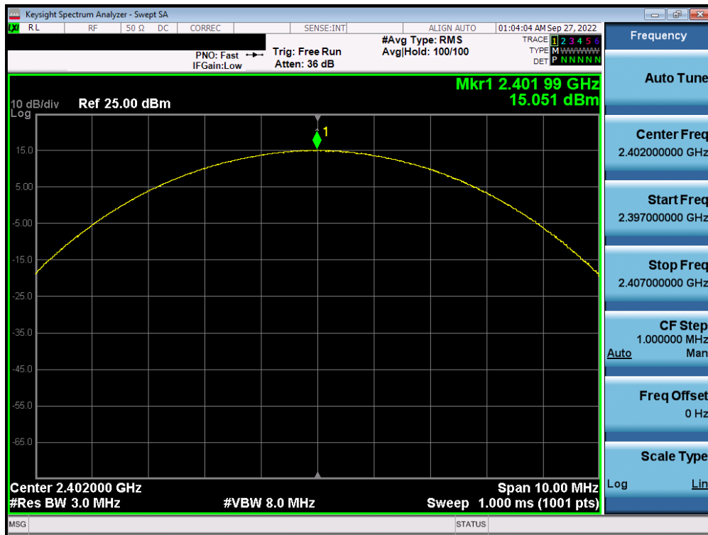
Plot 7-43. Peak Conducted Power (3Mbps – Ch. 0) – Antenna 2
