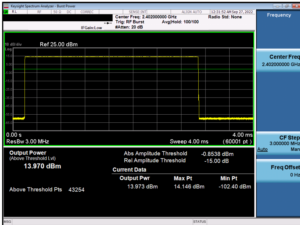
Plot 7-28. Average Conducted Power (1Mbps – Ch. 0) – Antenna 1
