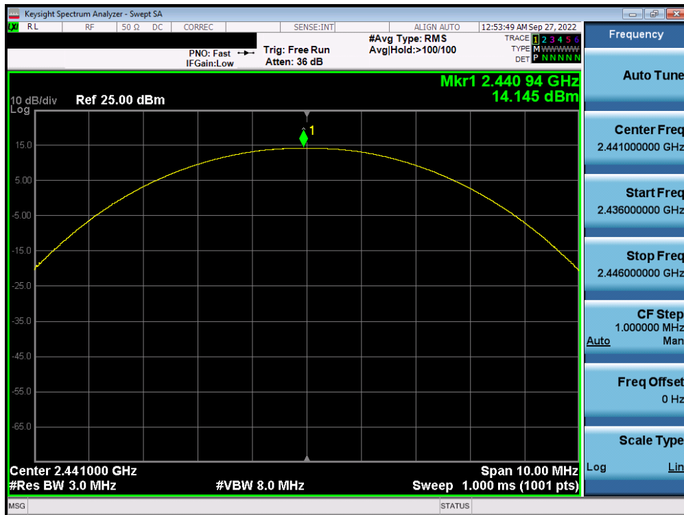
Plot 7-20. Peak Conducted Power (1Mbps - Ch. 39) - Antenna 1
