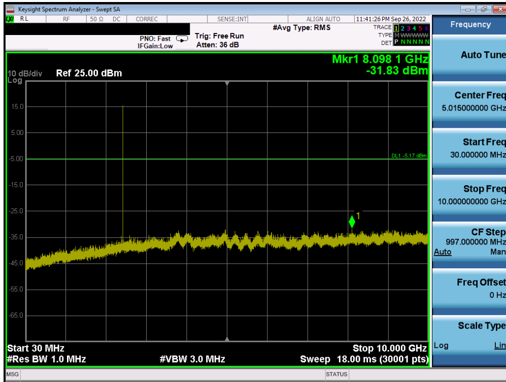
Plot 7-80. Conducted Spurious Plot (Bluetooth, 1Mbps – Ch. 39) – Antenna 2
