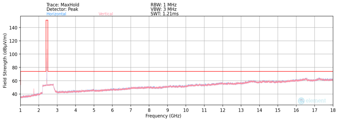
Plot 7-85. Radiated Spurious Plot above 1GHz (BT- Ch. 39) – Antenna 1
