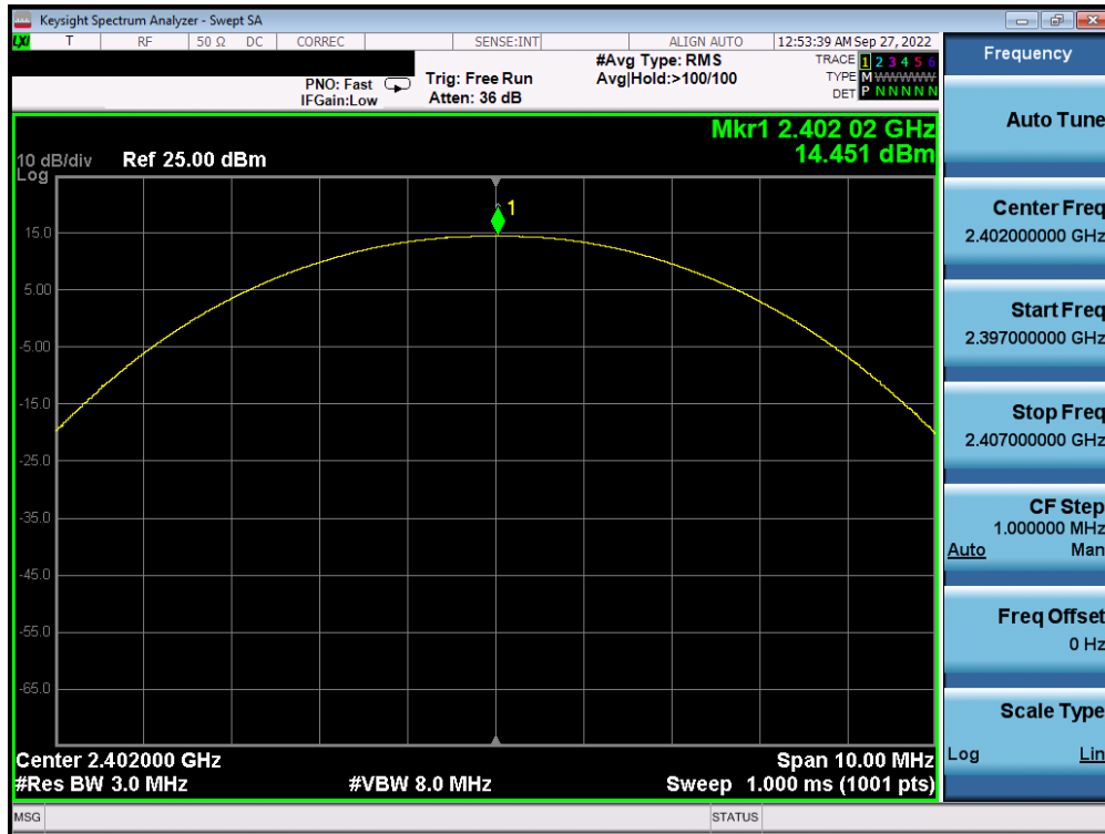
Plot 7-19. Peak Conducted Power (1Mbps - Ch. 0) - Antenna 1
