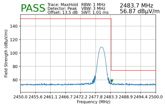
Plot 7-95. Radiated Restricted Upper Band Edge Measurement (Peak) – Antenna 1 with WCP
