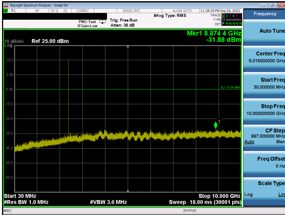
Plot 7-78. Conducted Spurious Plot (Bluetooth, 1Mbps – Ch. 0) – Antenna 2
