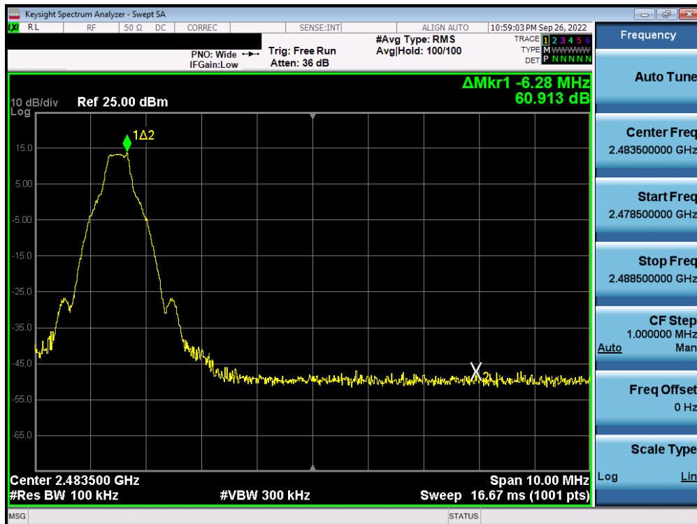
Plot 7-56. Band Edge Plot (Bluetooth with Hopping Disabled, 1 Mbps – Ch. 78) – Antenna 1
