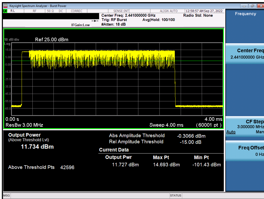
Plot 7-53. Average Conducted Power (3Mbps – Ch. 39) – Antenna 2
