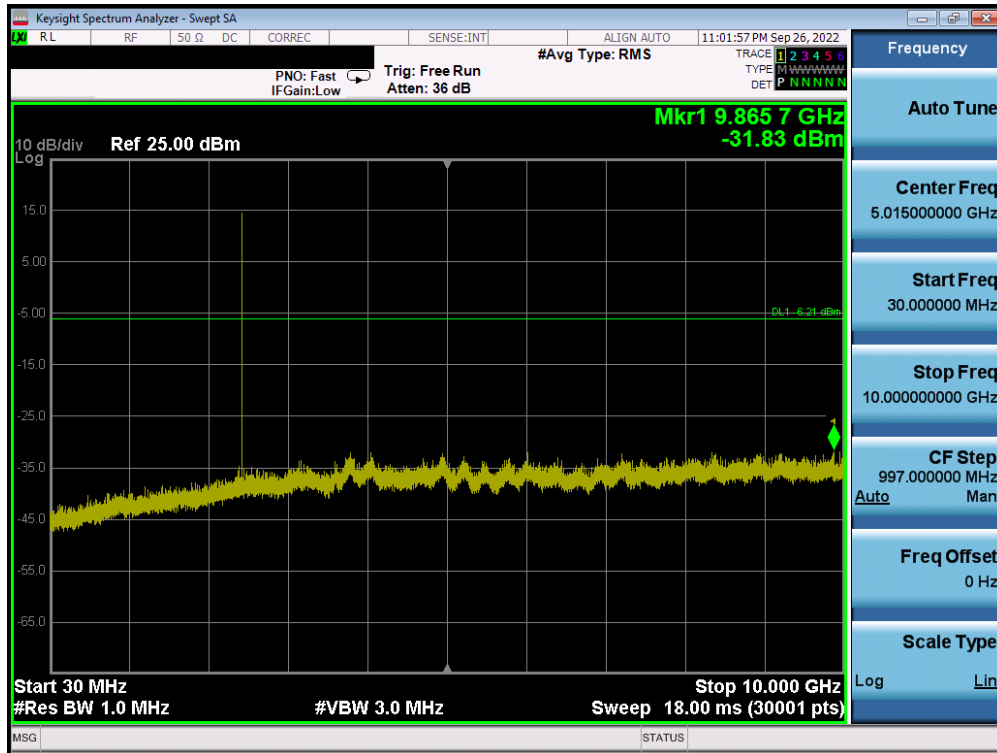
Plot 7-74. Conducted Spurious Plot (Bluetooth, 1Mbps – Ch. 39) – Antenna 1
