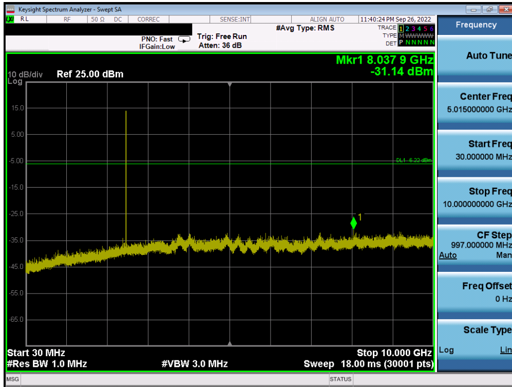
Plot 7-82. Conducted Spurious Plot (Bluetooth, 1Mbps – Ch. 78) – Antenna 2
