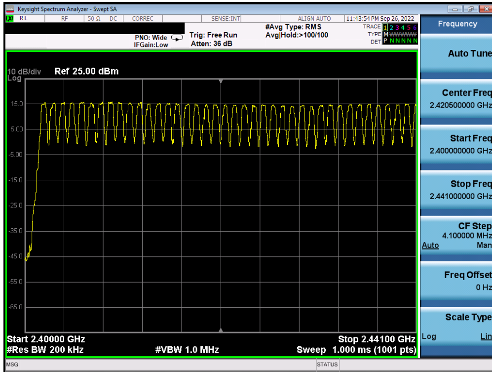
Plot 7-69. Low End Spectrum Channel Hopping Plot (Bluetooth) – Antenna 2
