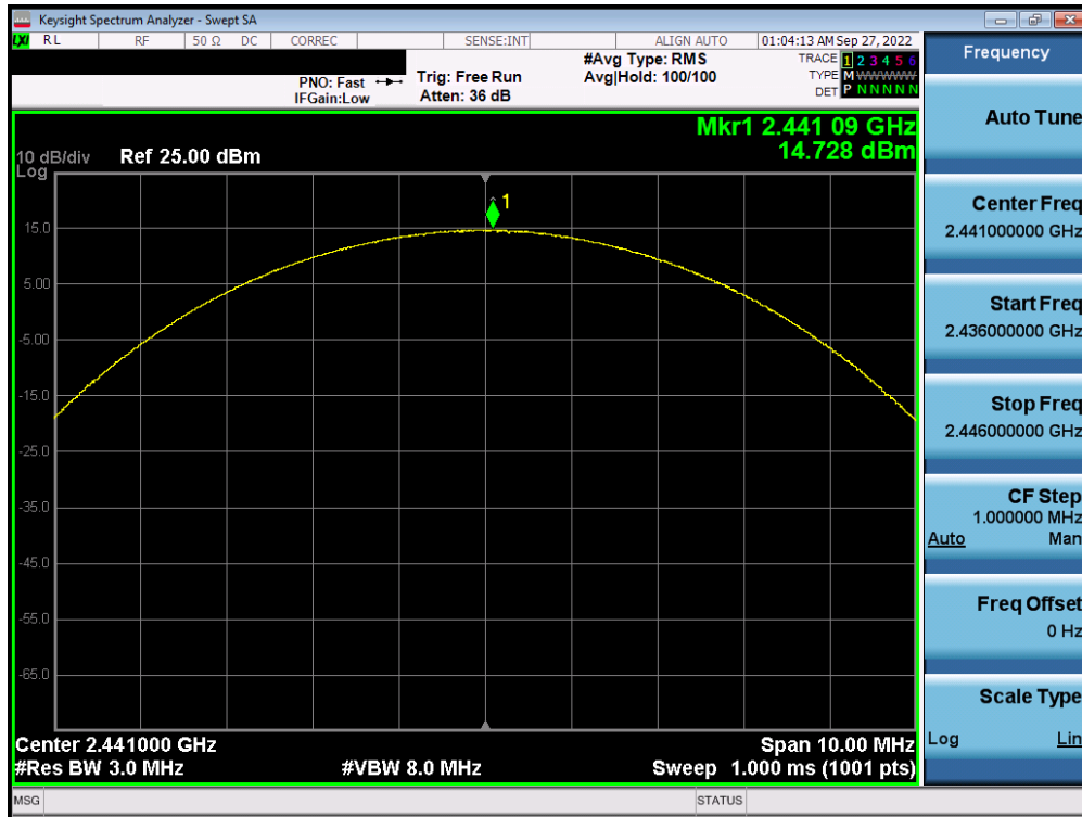
Plot 7-44. Peak Conducted Power (3Mbps – Ch. 39) – Antenna 2
