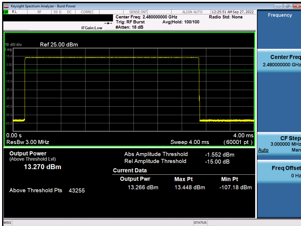
Plot 7-30. Average Conducted Power (1Mbps – Ch. 78) – Antenna 1
