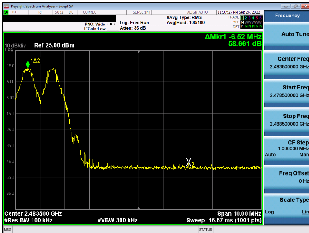
Plot 7-62. Band Edge Plot (Bluetooth with Hopping Enabled, 1 Mbps) – Antenna 2
