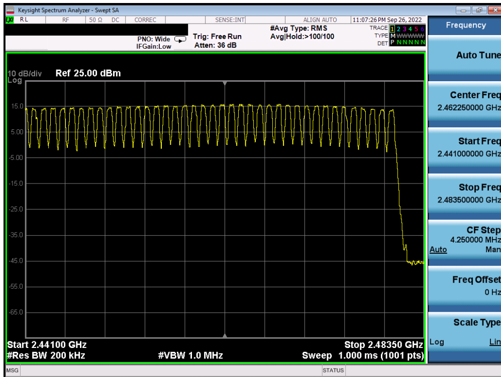
Plot 7-68. High End Spectrum Channel Hopping Plot (Bluetooth) – Antenna 1
