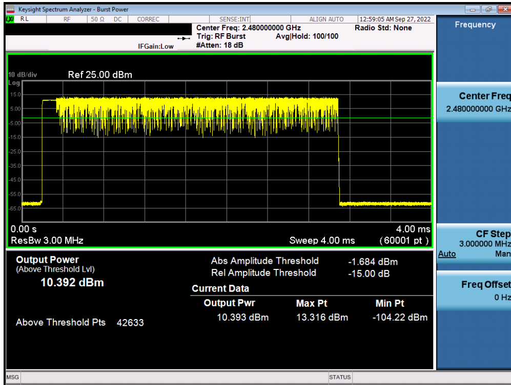
Plot 7-54. Average Conducted Power (3Mbps – Ch. 78) – Antenna 2
