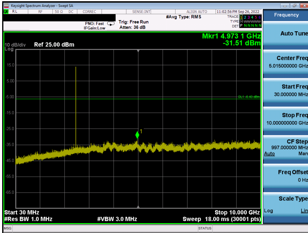
Plot 7-76. Conducted Spurious Plot (Bluetooth, 1Mbps – Ch. 78) – Antenna 1
