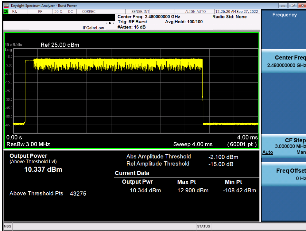
Plot 7-33. Average Conducted Power (2Mbps – Ch. 78) – Antenna 1
