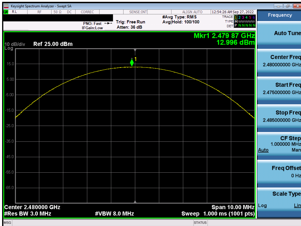
Plot 7-24. Peak Conducted Power (2Mbps – Ch. 78) – Antenna 1
