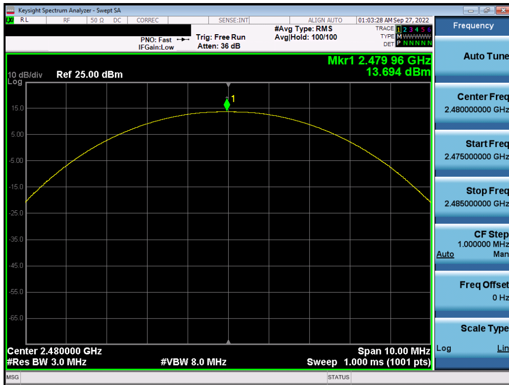
Plot 7-39. Peak Conducted Power (1Mbps – Ch. 78) – Antenna 2
