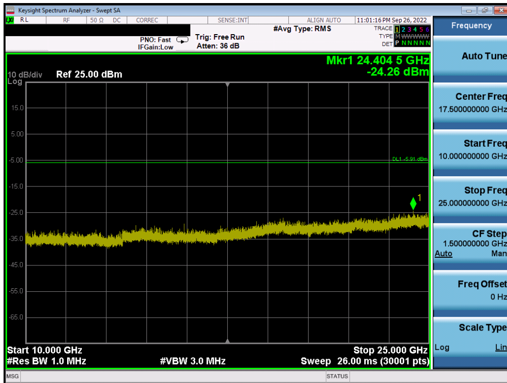
Plot 7-73. Conducted Spurious Plot (Bluetooth, 1Mbps – Ch. 0) – Antenna 1
