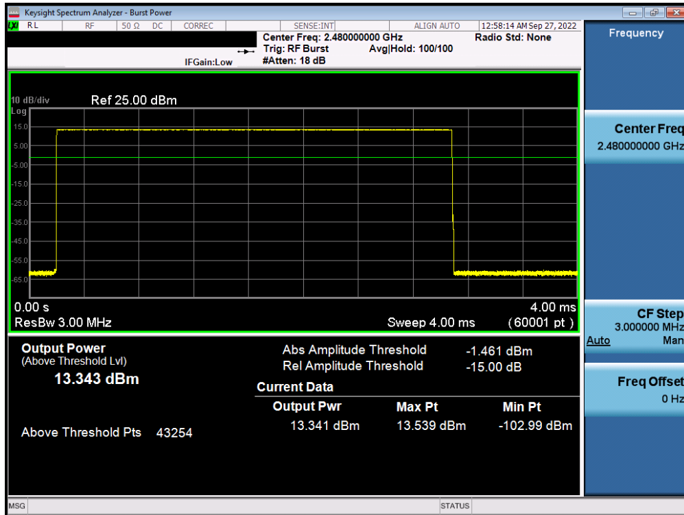
Plot 7-48. Average Conducted Power (1Mbps – Ch. 78) – Antenna 2
