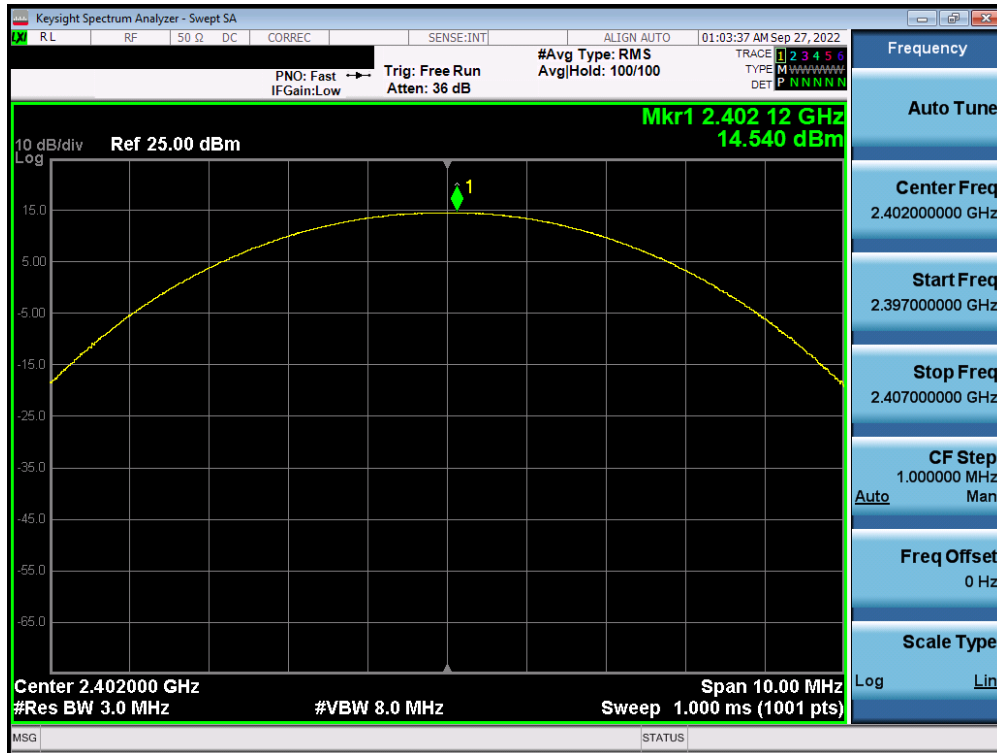
Plot 7-40. Peak Conducted Power (2Mbps – Ch. 0) – Antenna 2
