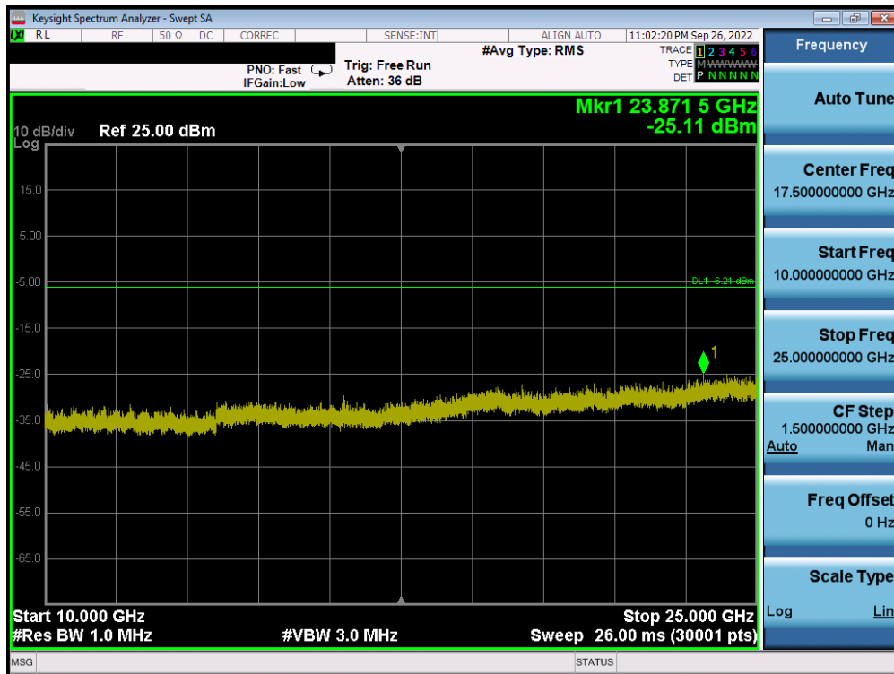
Plot 7-75. Conducted Spurious Plot (Bluetooth, 1Mbps – Ch. 39) – Antenna 1
