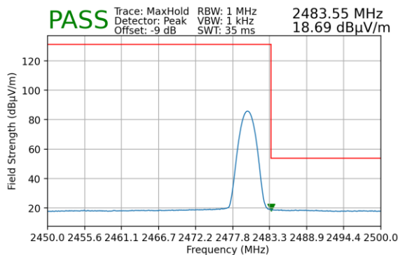
Plot 7-94. Radiated Restricted Upper Band Edge Measurement (Average) – Antenna 1 with WCP
