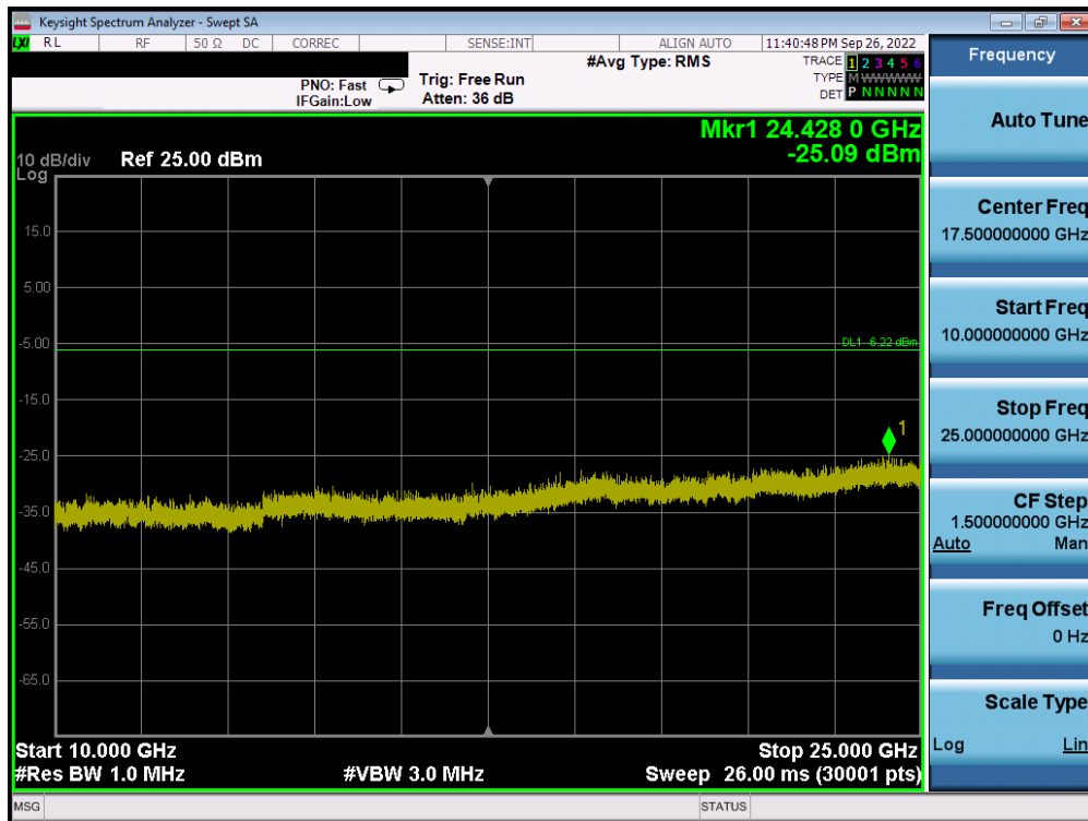
Plot 7-83. Conducted Spurious Plot (Bluetooth, 1Mbps – Ch. 78) – Antenna 2
