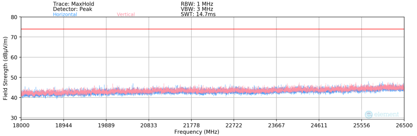
Plot 7-87. Radiated Spurious Plot above 18GHz– Antenna 1
