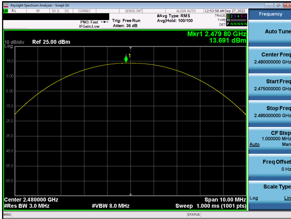
Plot 7-21. Peak Conducted Power (1Mbps – Ch. 78) – Antenna 1
