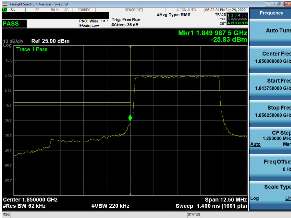
Plot 7-220. Lower Band Edge Plot (LTE Band 25/2 - 5MHz QPSK – Full RB - Ant F)
