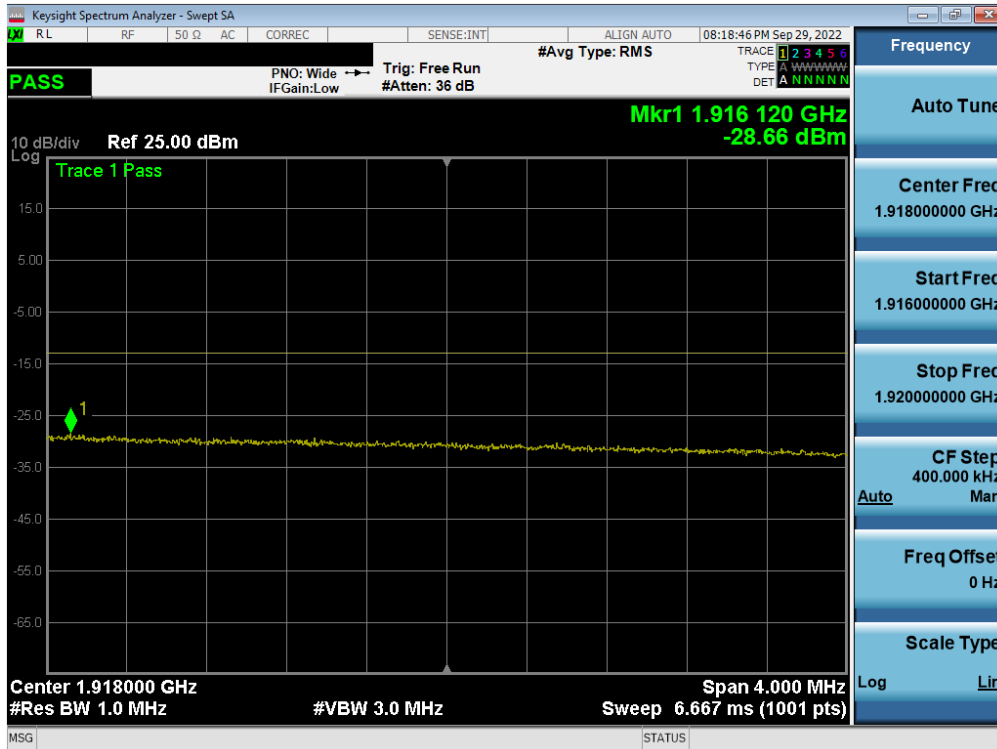
Plot 7-207. Extended Upper Band Edge Plot (LTE Band 25 - 20MHz QPSK – Full RB - Ant F)
