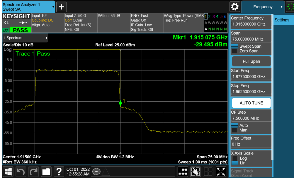
Plot 7-244. Upper Band Edge Plot (NR Band n25 - 30MHz QPSK – Full RB - Ant F)
