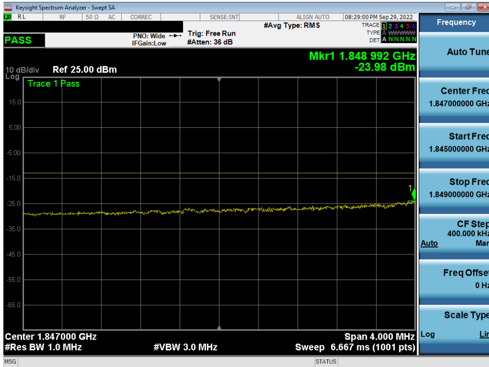
Plot 7-215. Extended Lower Band Edge Plot (LTE Band 25/2 - 10MHz QPSK – Full RB - Ant F)
