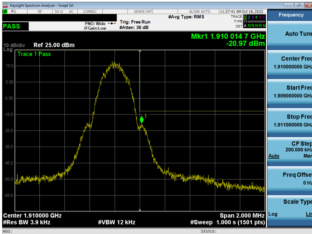
Plot 7-197. Upper Band Edge Plot (GPRS PCS – Ch. 810)
