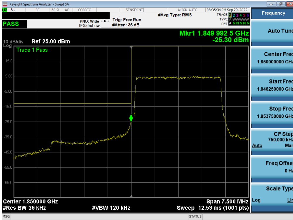
Plot 7-226. Lower Band Edge Plot (LTE Band 25/2 - 3MHz QPSK – Full RB - Ant F)
