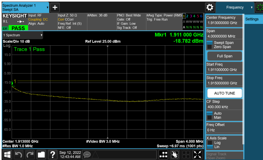
Plot 7-187. Extended Upper Band Edge Plot (NR Band n2 - 10MHz QPSK – Full RB - Ant A)
