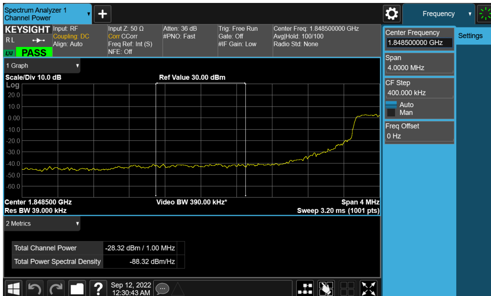
Plot 7-191. Extended Lower Band Edge Plot (NR Band n25/2 – 5MHz QPSK – Full RB - Ant A)
