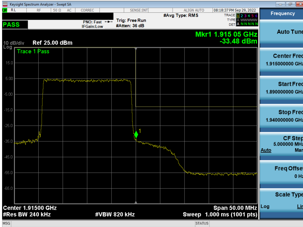
Plot 7-206. Upper Band Edge Plot (LTE Band 25 - 20MHz QPSK – Full RB - Ant F)
