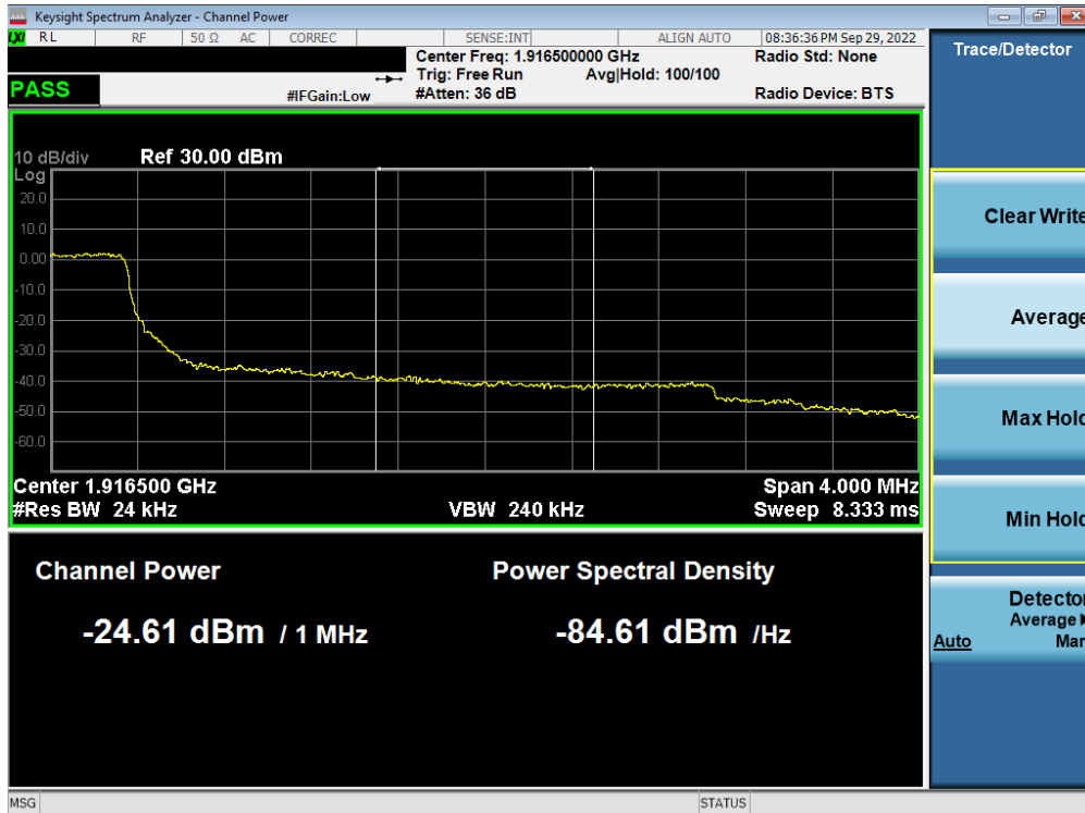
Plot 7-231. Extended Upper Band Edge Plot (LTE Band 25 - 3MHz QPSK – Full RB - Ant F)
