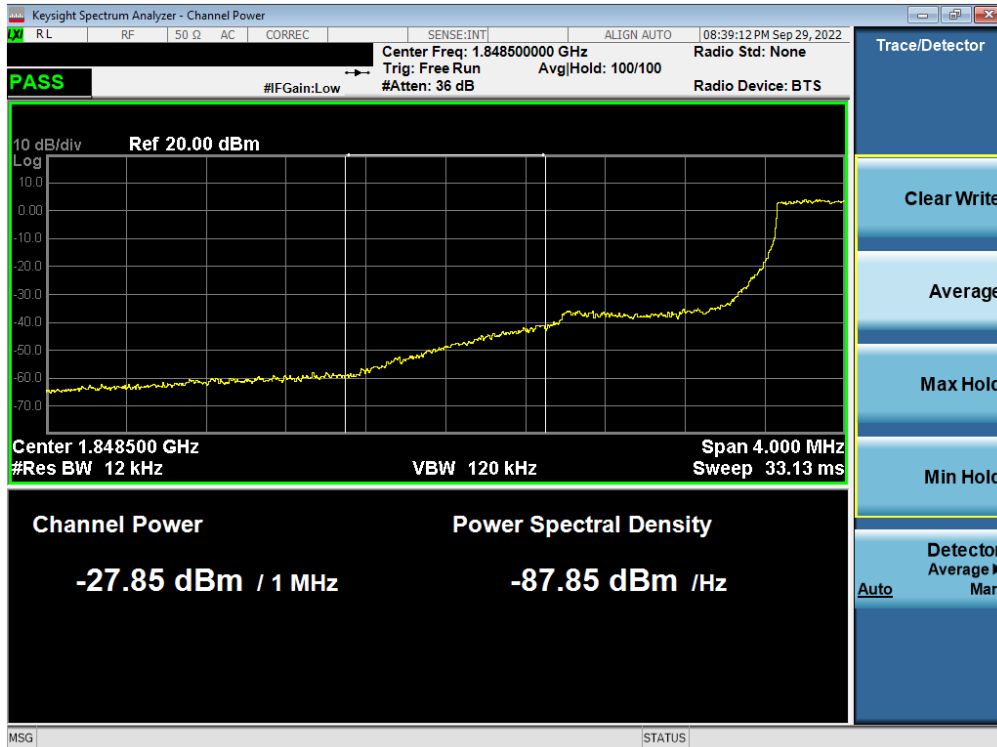
Plot 7-233. Extended Lower Band Edge Plot (LTE Band 25/2 – 1.4MHz QPSK – Full RB - Ant F)
