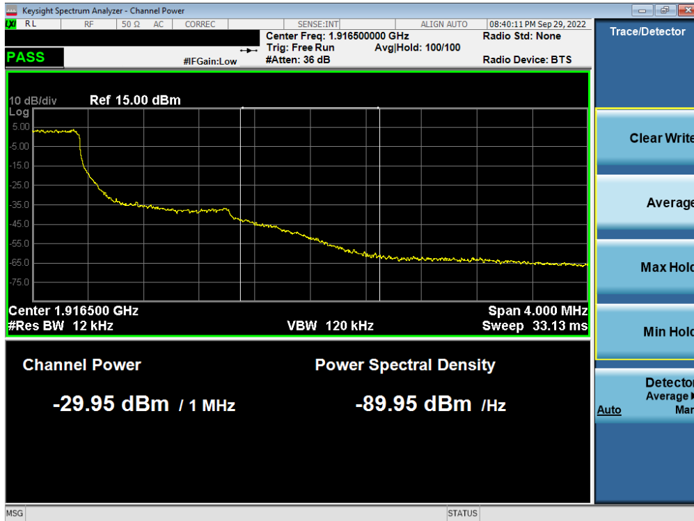
Plot 7-237. Extended Upper Band Edge Plot (LTE Band 25 – 1.4MHz QPSK – Full RB - Ant F)
