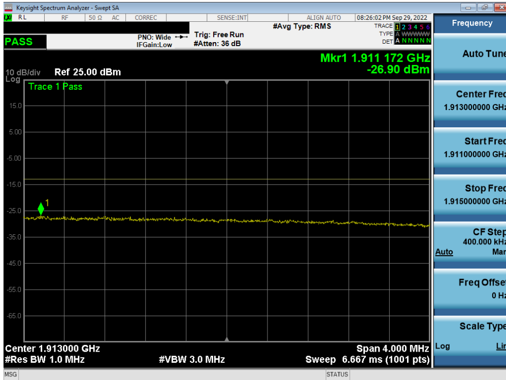
Plot 7-211. Extended Upper Band Edge Plot (LTE Band 2 - 15MHz QPSK – Full RB - Ant F)
