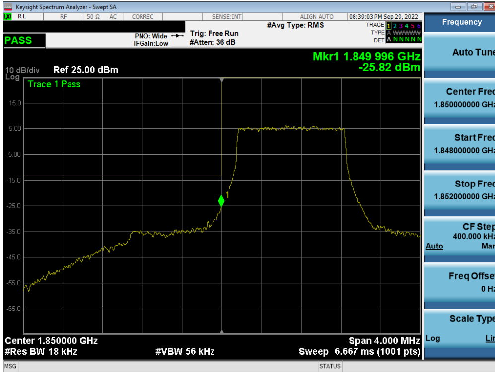
Plot 7-232. Lower Band Edge Plot (LTE Band 25/2 – 1.4MHz QPSK – Full RB - Ant F)
