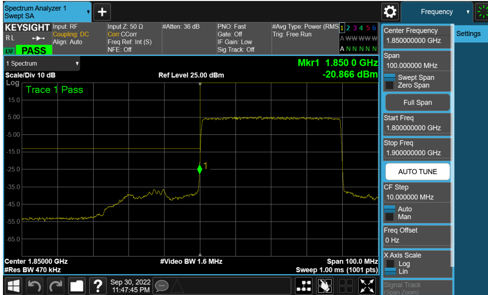
Plot 7-238. Lower Band Edge Plot (NR Band n25 - 40MHz QPSK – Full RB - Ant F)
