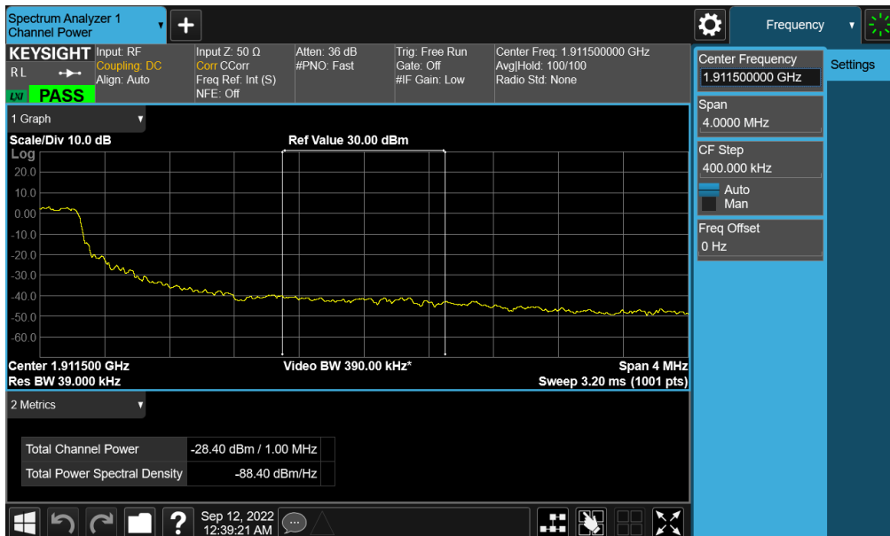
Plot 7-193. Extended Upper Band Edge Plot (NR Band n2 – 5MHz QPSK – Full RB - Ant A)
