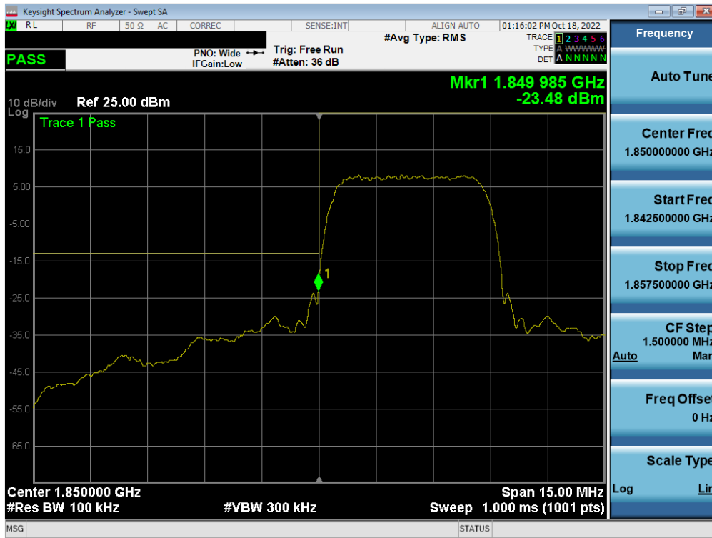
Plot 7-198. Lower Band Edge Plot (WCDMA PCS – Ch. 9262)
