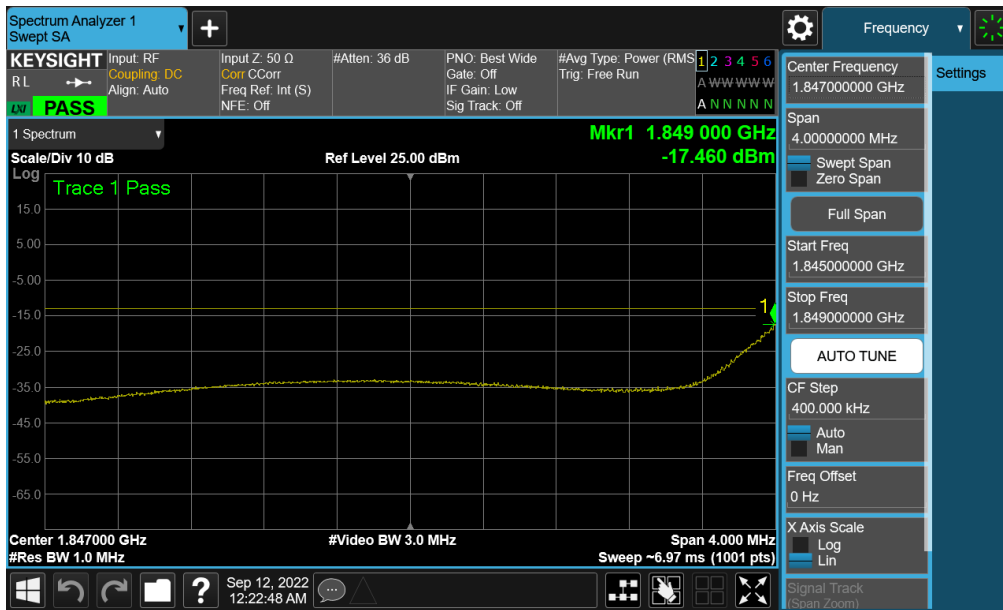
Plot 7-185. Extended Lower Band Edge Plot (NR Band n25/2 - 10MHz QPSK – Full RB - Ant A)
