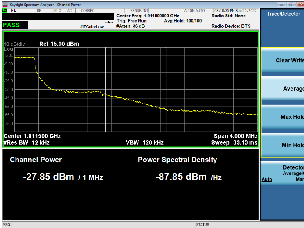
Plot 7-235. Extended Upper Band Edge Plot (LTE Band 2 – 1.4MHz QPSK – Full RB - Ant F)
