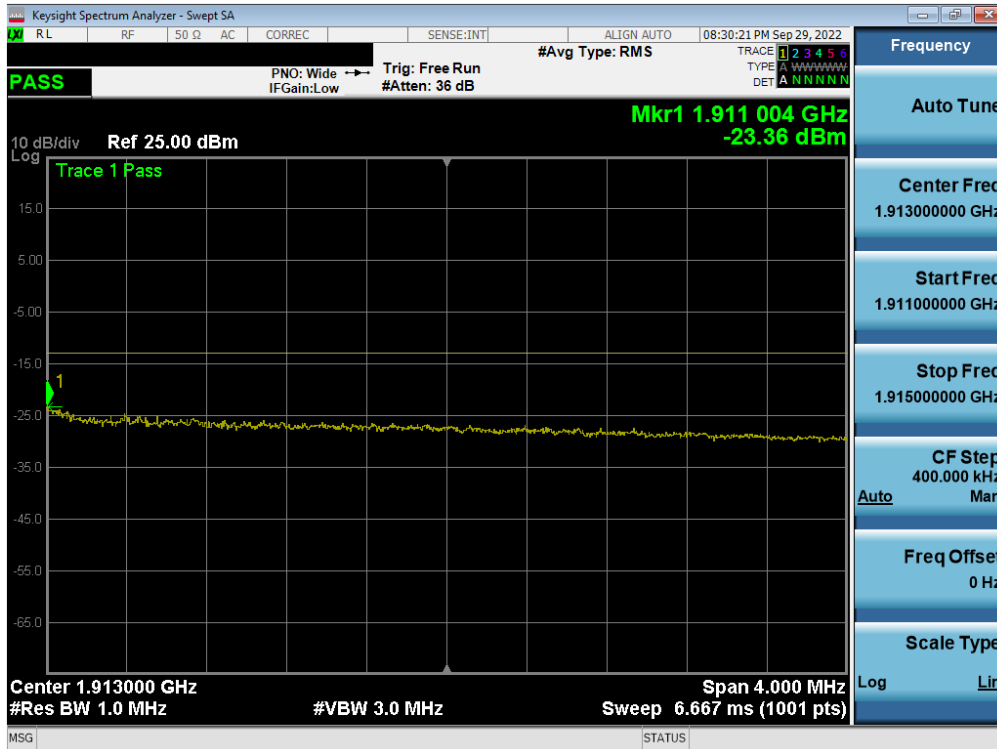
Plot 7-217. Extended Upper Band Edge Plot (LTE Band 2 - 10MHz QPSK – Full RB - Ant F)
