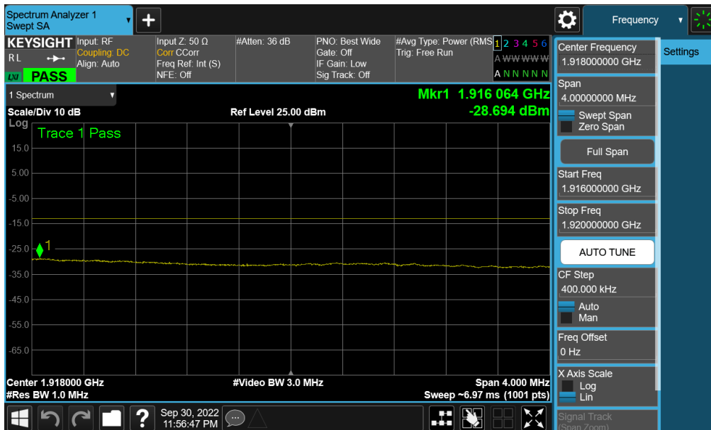
Plot 7-241. Extended Upper Band Edge Plot (NR Band n25 - 40MHz QPSK – Full RB - Ant F)
