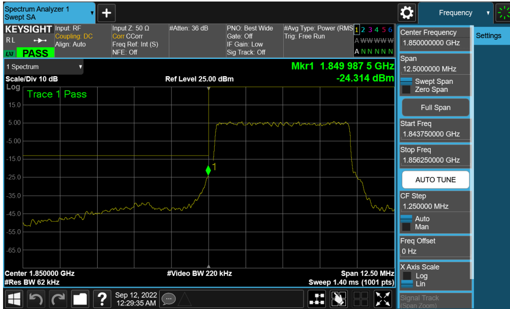
Plot 7-190. Lower Band Edge Plot (NR Band n25/2 – 5MHz QPSK – Full RB - Ant A)
