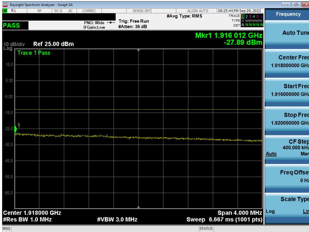
Plot 7-213. Extended Upper Band Edge Plot (LTE Band 25 - 15MHz QPSK – Full RB - Ant F)
