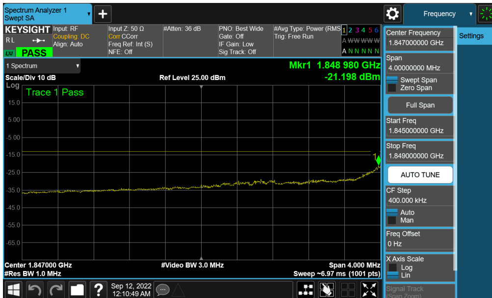
Plot 7-179. Extended Lower Band Edge Plot (NR Band n25/2 - 15MHz QPSK – Full RB - Ant A)
