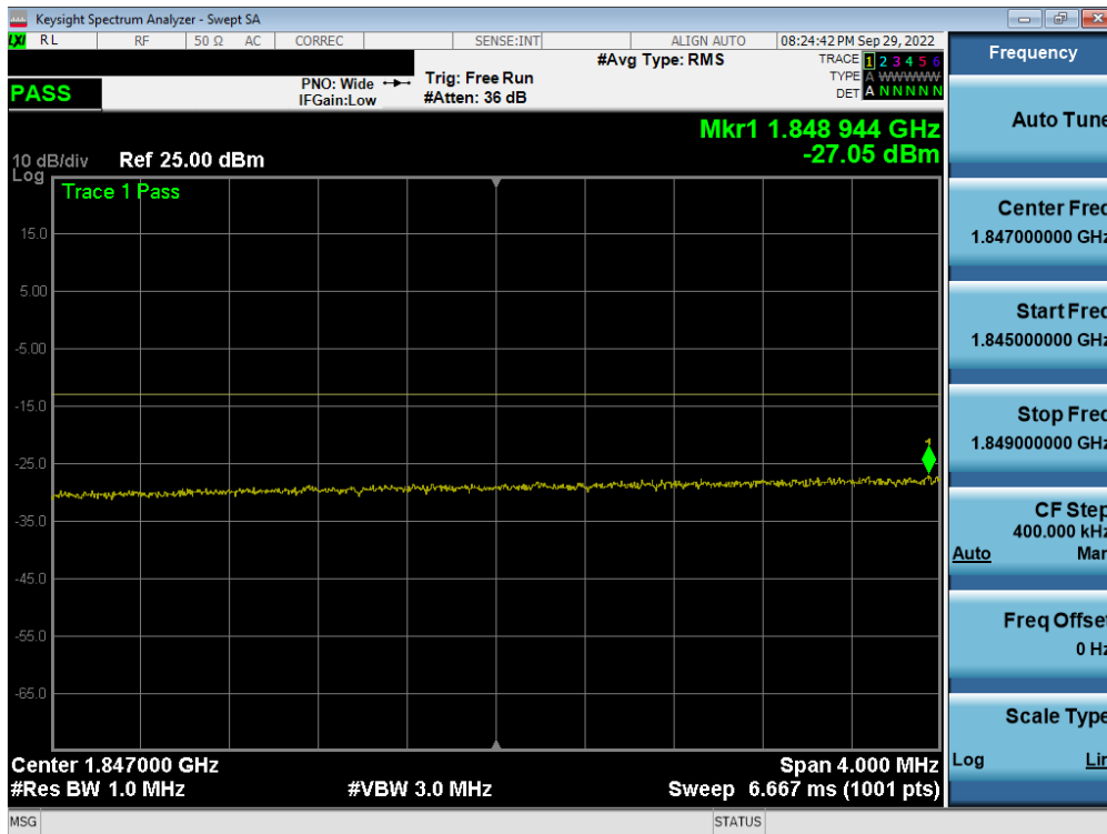
Plot 7-209. Extended Lower Band Edge Plot (LTE Band 25/2 - 15MHz QPSK – Full RB - Ant F)
