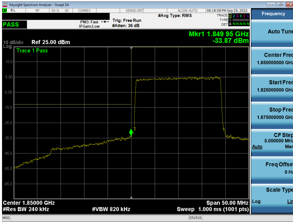
Plot 7-202. Lower Band Edge Plot (LTE Band 25/2 - 20MHz QPSK – Full RB - Ant F)
