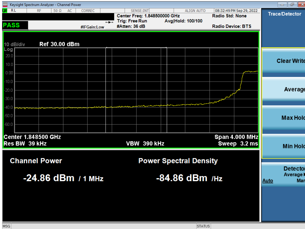
Plot 7-221. Extended Lower Band Edge Plot (LTE Band 25/2 - 5MHz QPSK – Full RB - Ant F)
