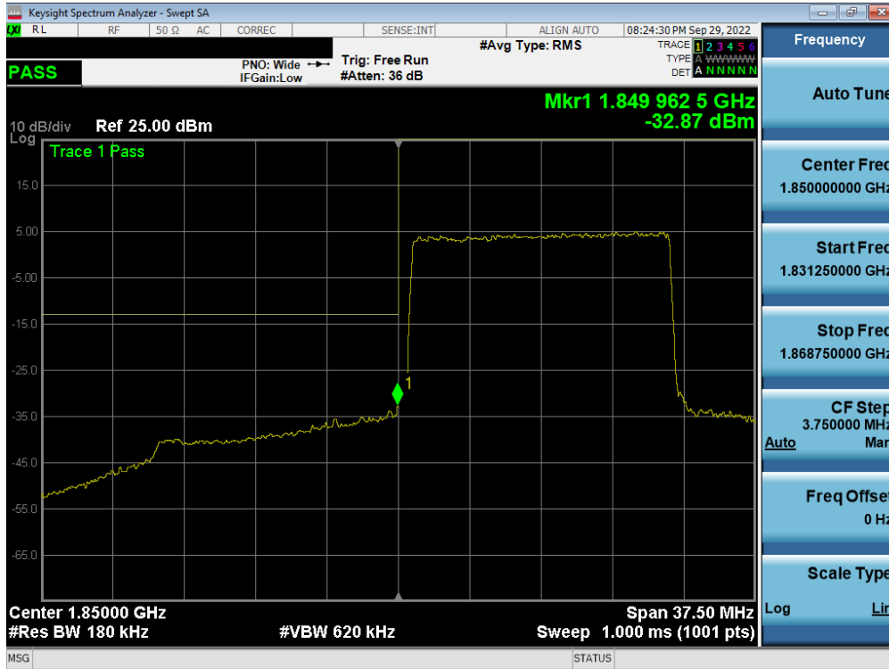
Plot 7-208. Lower Band Edge Plot (LTE Band 25/2 - 15MHz QPSK – Full RB - Ant F)
