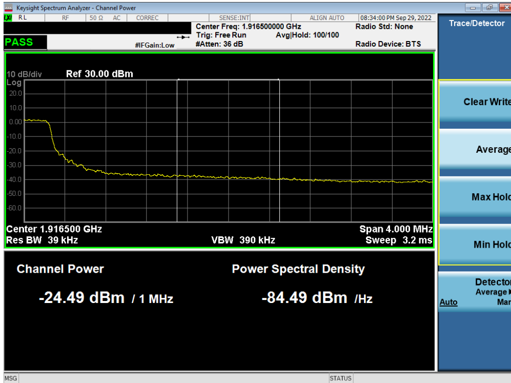
Plot 7-225. Extended Upper Band Edge Plot (LTE Band 25 - 5MHz QPSK – Full RB - Ant F)
