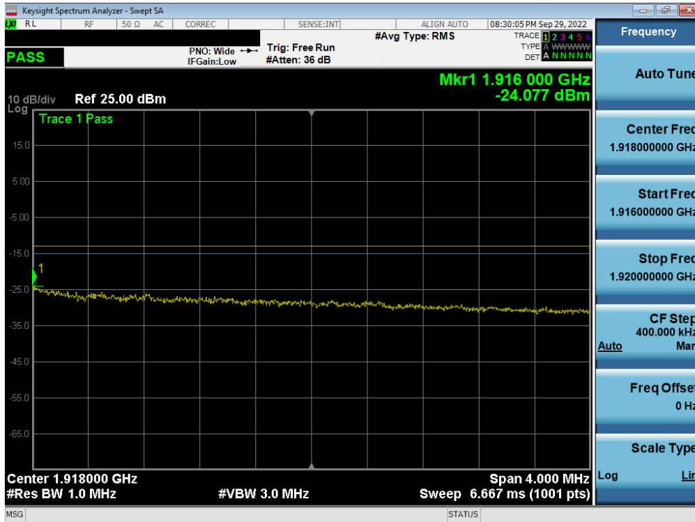
Plot 7-219. Extended Upper Band Edge Plot (LTE Band 25 - 10MHz QPSK – Full RB - Ant F)
