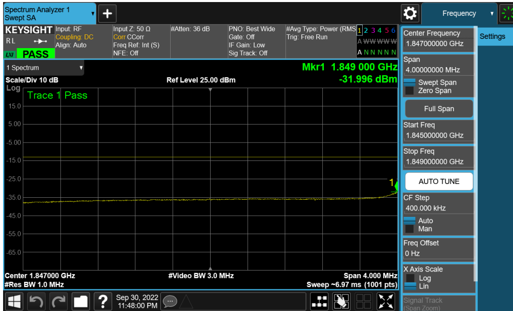
Plot 7-239. Extended Lower Band Edge Plot (NR Band n25 - 40MHz QPSK – Full RB - Ant F)
