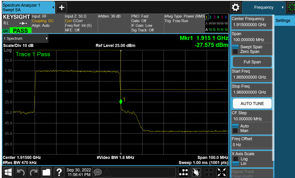
Plot 7-240. Upper Band Edge Plot (NR Band n25 - 40MHz QPSK – Full RB - Ant F)
