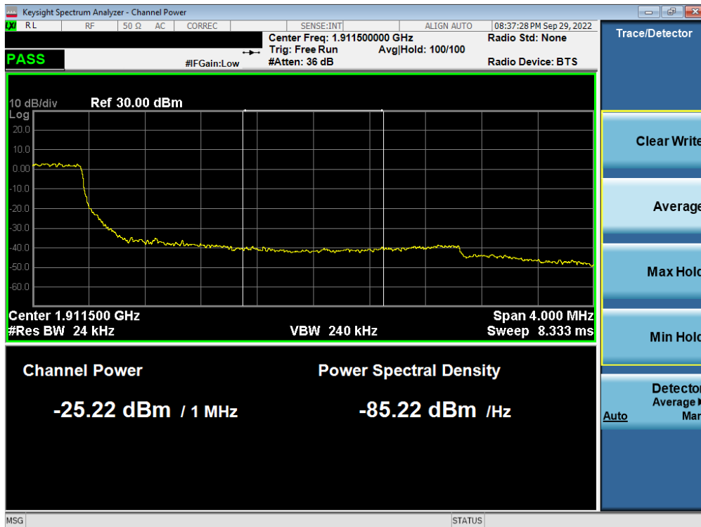
Plot 7-229. Extended Upper Band Edge Plot (LTE Band 2 - 3MHz QPSK – Full RB - Ant F)
