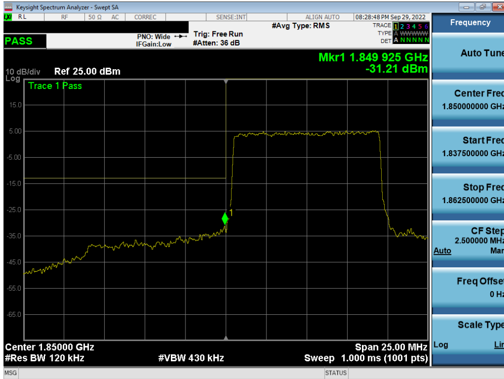
Plot 7-214. Lower Band Edge Plot (LTE Band 25/2 - 10MHz QPSK – Full RB - Ant F)
