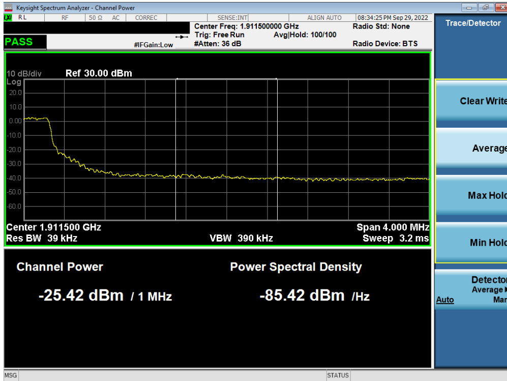
Plot 7-223. Extended Upper Band Edge Plot (LTE Band 2 - 5MHz QPSK – Full RB - Ant F)
