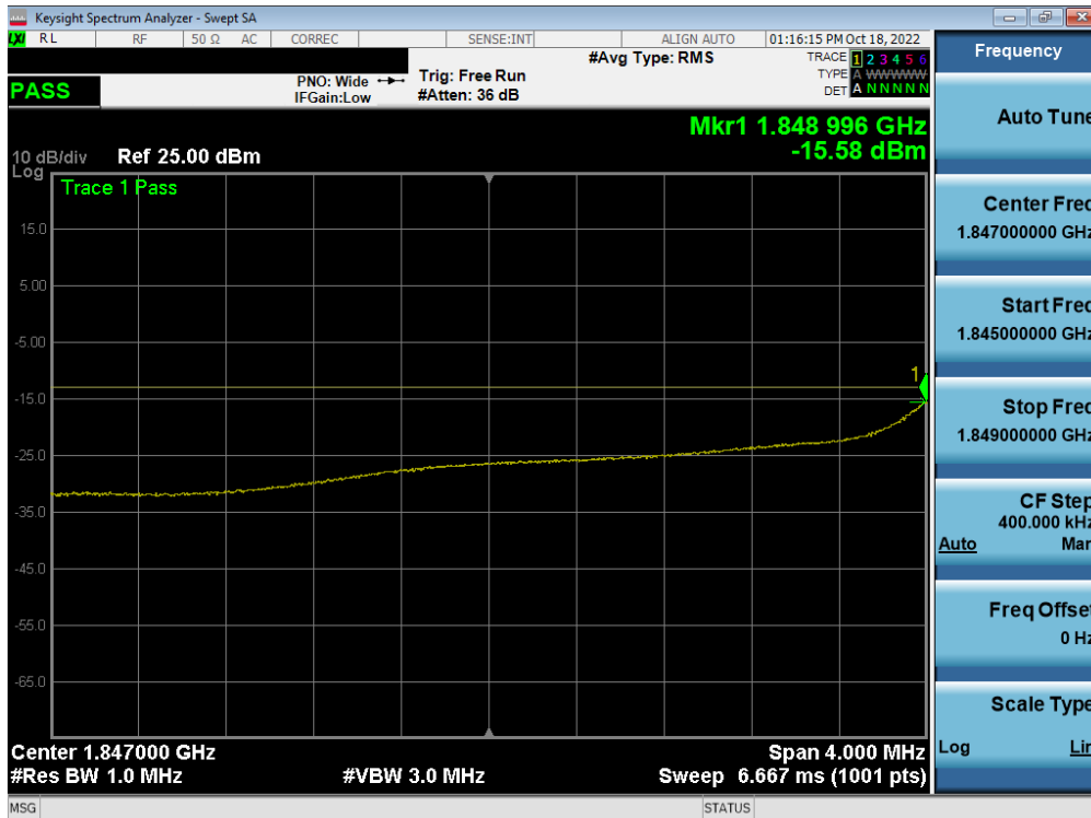
Plot 7-199. Extended Lower Band Edge Plot (WCDMA PCS – Ch. 9262)
