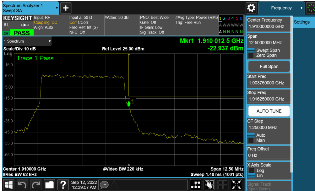
Plot 7-192. Upper Band Edge Plot (NR Band n2 – 5MHz QPSK – Full RB - Ant A)
