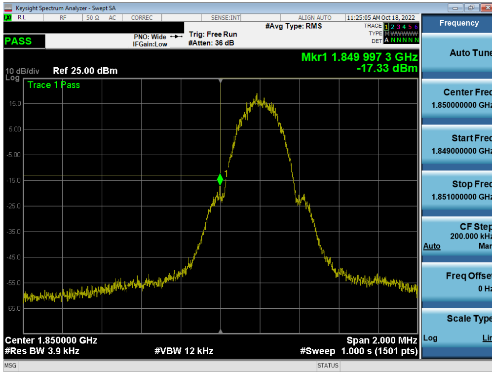
Plot 7-196. Lower Band Edge Plot (GPRS PCS – Ch. 512)
