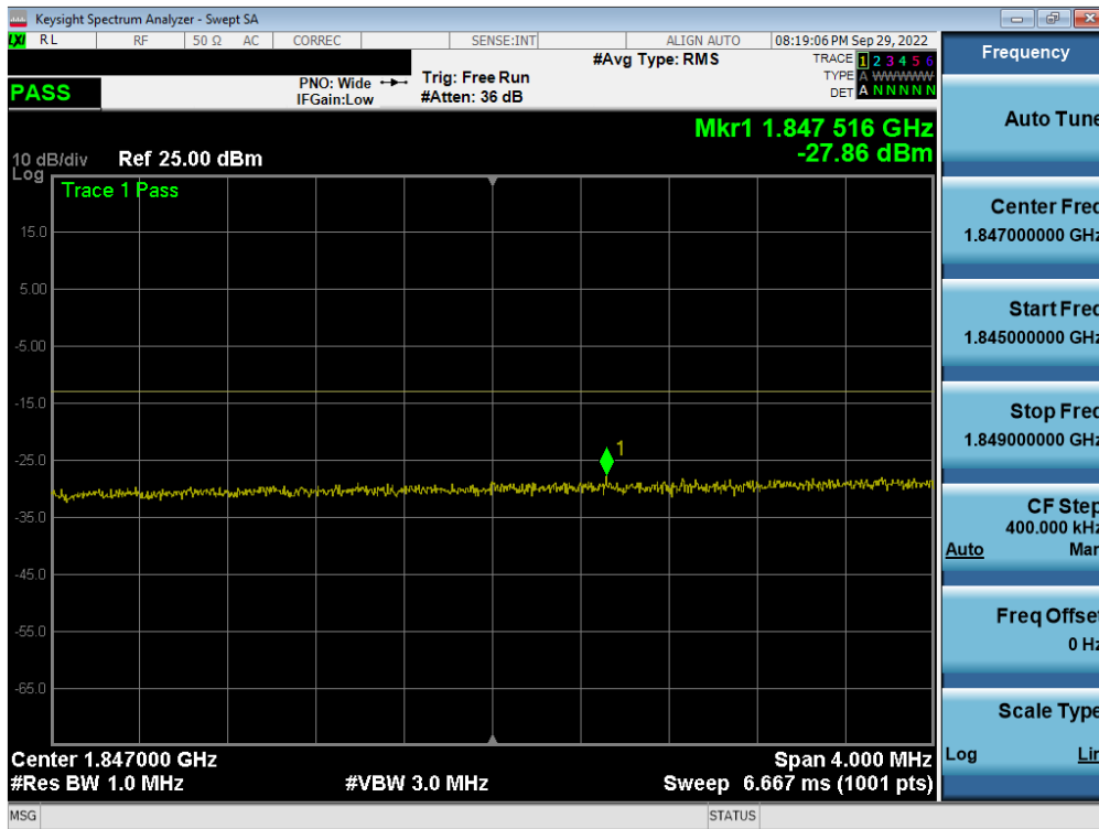
Plot 7-203. Extended Lower Band Edge Plot (LTE Band 25/2 - 20MHz QPSK – Full RB - Ant F)
