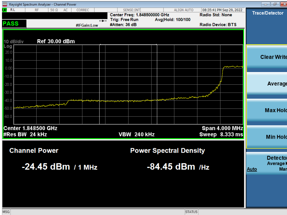
Plot 7-227. Extended Lower Band Edge Plot (LTE Band 25/2 - 3MHz QPSK – Full RB - Ant F)
