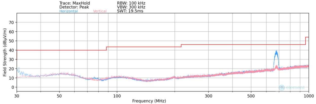
Plot 7-406. Radiated Spurious Plot below 1GHz (2.4GHz – 5GHz)
