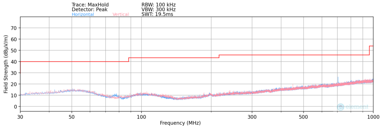
Plot 7-407. Radiated Spurious Plot below 1GHz (6GHz – 2.4GHz)
