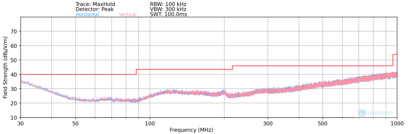
Plot 7-405. Radiated Spurious Plot below 1GHz MIMO (802.11a – U1 Ch. 48)
