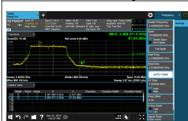
12 Channel Band-edge
