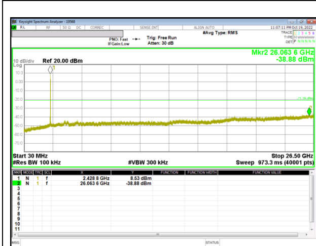
Out-Of-Band 6 Channel(4RU)
