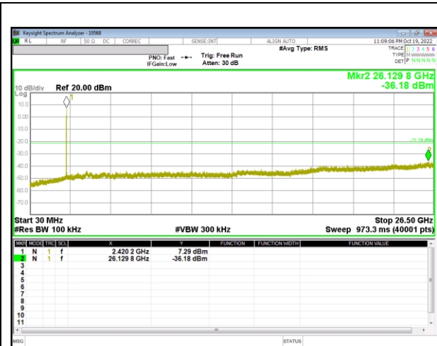
Out-Of-Band 1 Channel(8RU)
