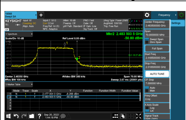
13 Channel Band-edge
