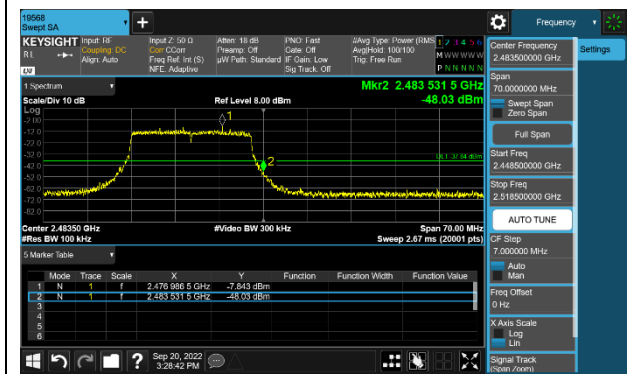
13 Channel Band-edge
