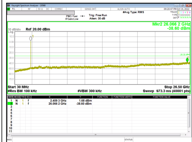
Out-Of-Band 1 Channel
