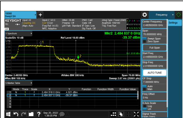
11 Channel Band-edge
