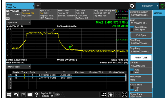
12 Channel Band-edge
