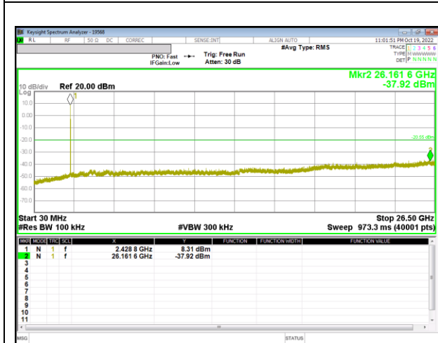
Out-Of-Band 6 Channel(0RU)
