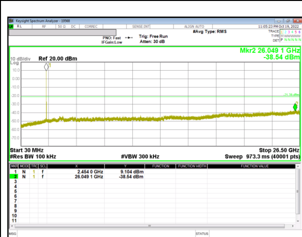
Out-Of-Band 11 Channel(0RU)
