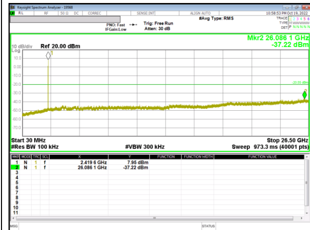
Out-Of-Band 1 Channel(8RU)
