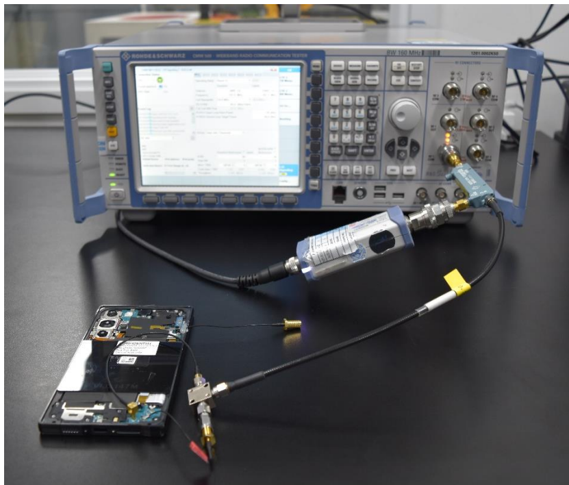
A.2 : Conducted test in CMW500 callbox
