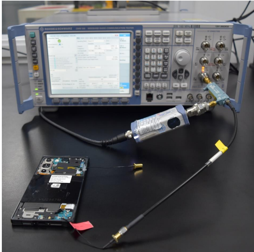
A.2 : Conducted test in CMW500 callbox
