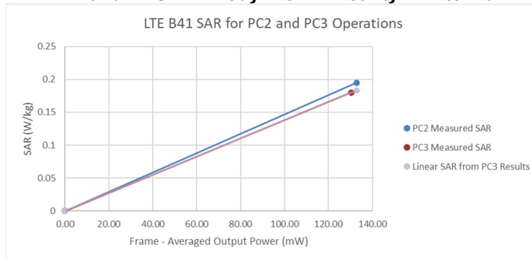
Figure 13-2 LTE Band 41 ULCA Body-Worn Linearity – Antenna B
