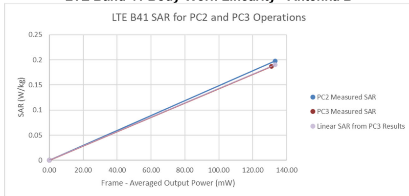
Figure 13-1 LTE Band 41 Body-Worn Linearity - Antenna B
