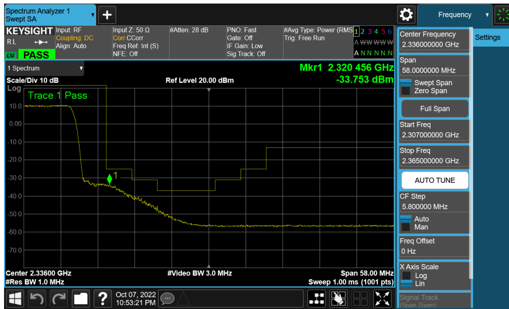
Plot 7-456. Extended Upper Band Edge Plot (NR Band n30 - 10MHz CP-OFDM-QPSK – Full RB - Ant F)
