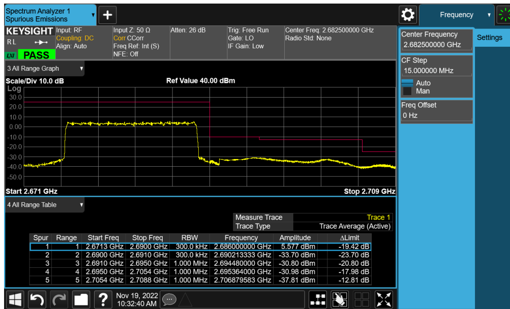
Plot 7-509. Upper ACP Plot (NR Band n41 - 15MHz CP-OFDM-QPSK – Full RB - Ant F)
