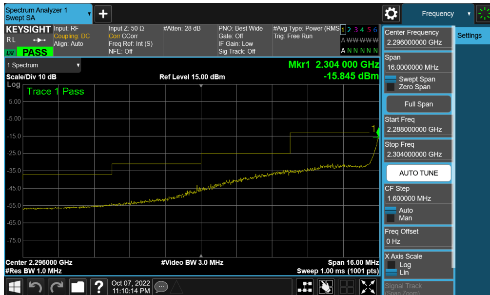
Plot 7-458. Extended Lower Band Edge Plot (NR Band n30 - 5MHz CP-OFDM-QPSK – Full RB - Ant F)
