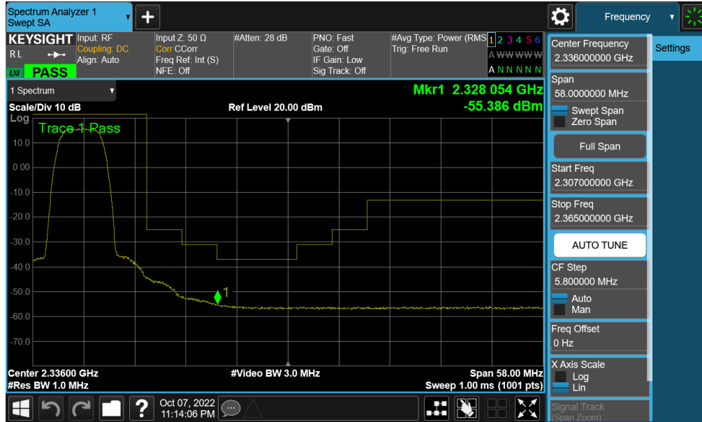
Plot 7-461. Extended Upper Band Edge Plot (NR Band n30 - 5MHz CP-OFDM-QPSK – Full RB - Ant F)
