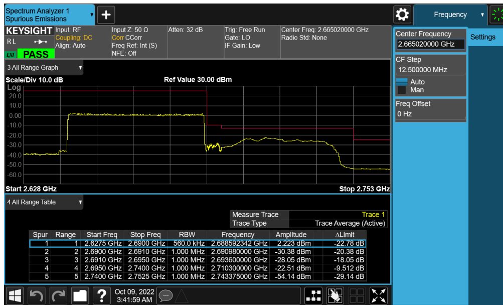
Plot 7-501. Upper ACP Plot (NR Band n41 - 50MHz CP-OFDM-QPSK – Full RB - Ant F)
