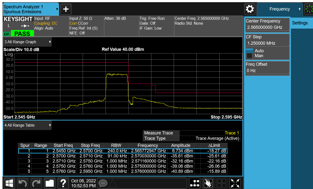
Plot 7-489. Upper Band Edge Plot (NR Band n7 - 5MHz CP-OFDM-QPSK – Full RB - Ant F)
