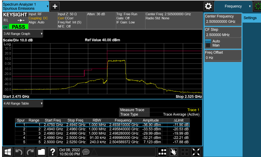
Plot 7-488. Lower Band Edge Plot (NR Band n7 - 5MHz CP-OFDM-QPSK – Full RB - Ant F)
