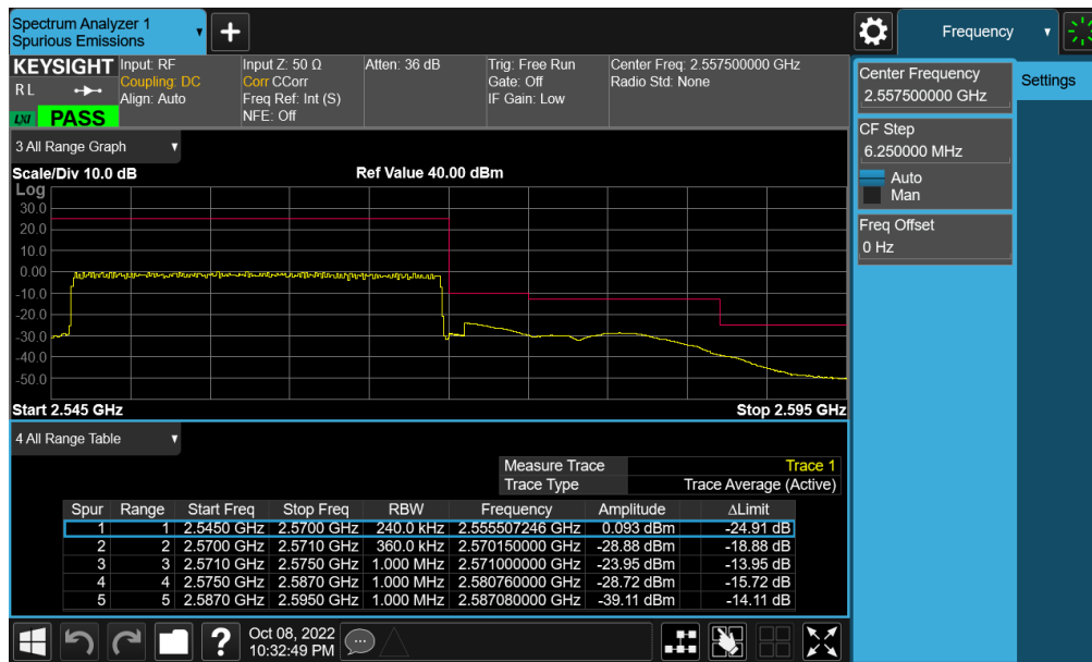
Plot 7-481. Upper Band Edge Plot (NR Band n7 - 25MHz CP-OFDM-QPSK – Full RB - ANT F)
