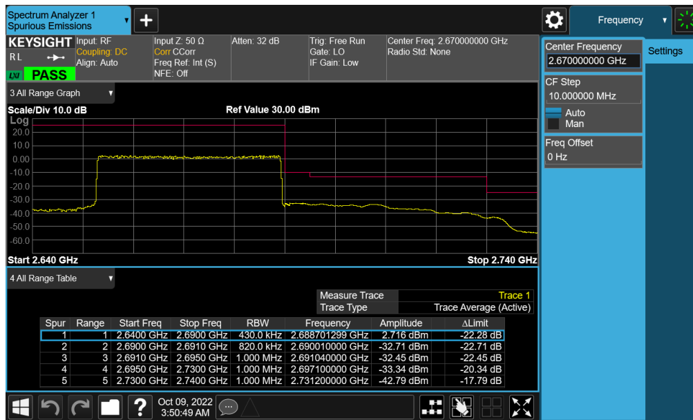
Plot 7-503. Upper ACP Plot (NR Band n41 - 40MHz CP-OFDM-QPSK – Full RB - Ant F)
