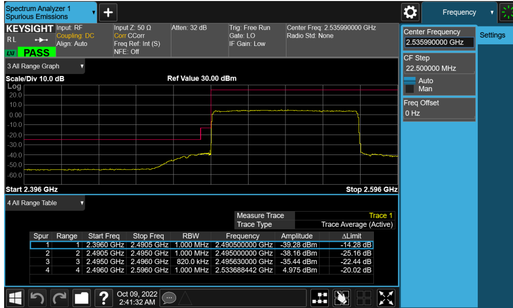
Plot 7-494. Lower ACP Plot (NR Band n41 - 80MHz CP-OFDM-QPSK – Full RB - Ant F)
