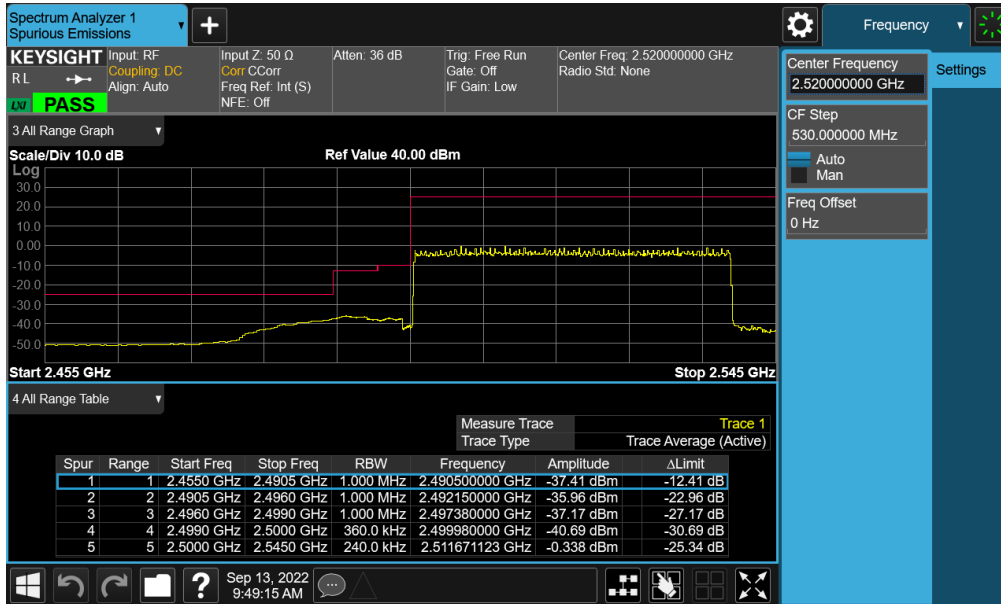
Plot 7-462. Lower Band Edge Plot (NR Band n7 - 40MHz CP-OFDM-QPSK – Full RB - ANT B)
