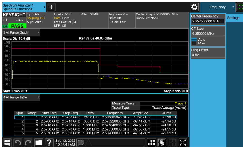
Plot 7-467. Upper Band Edge Plot (NR Band n7 - 25MHz CP-OFDM-QPSK – Full RB - ANT B)
