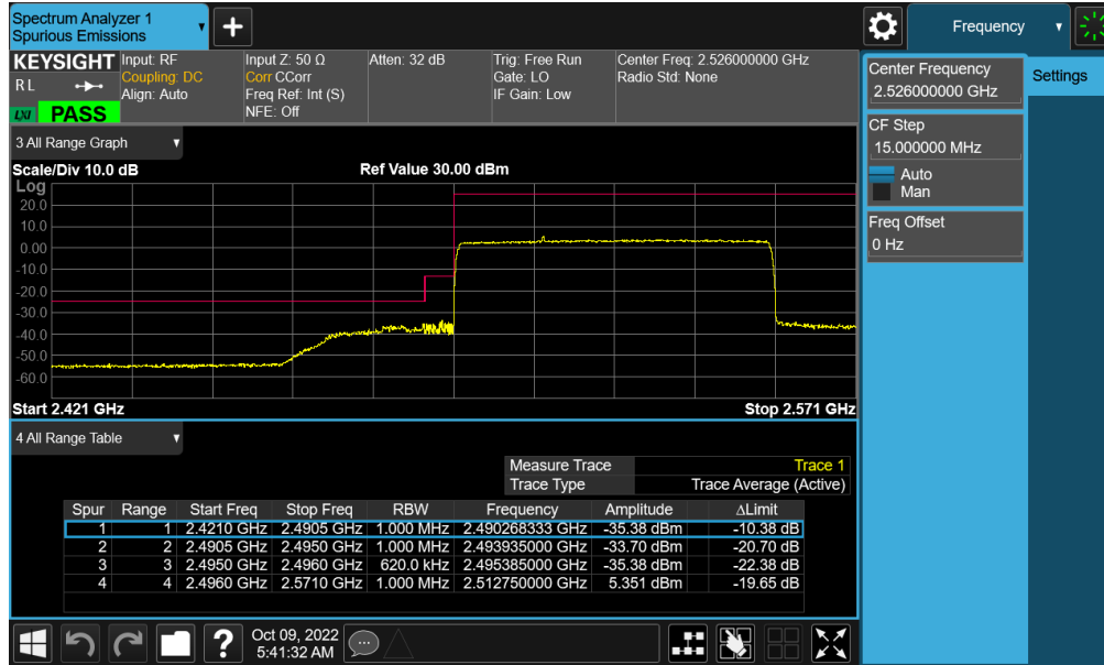
Plot 7-498. Lower ACP Plot (NR Band n41 - 60MHz CP-OFDM-QPSK – Full RB - Ant F)
