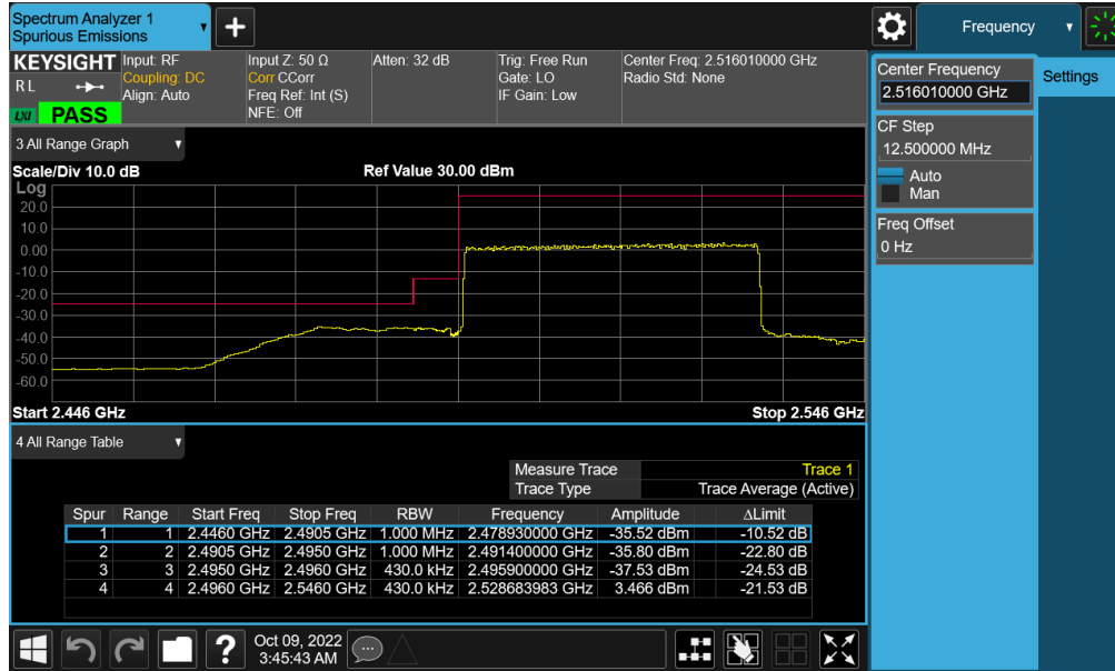
Plot 7-502. Lower ACP Plot (NR Band n41 - 40MHz CP-OFDM-QPSK – Full RB - Ant F)
