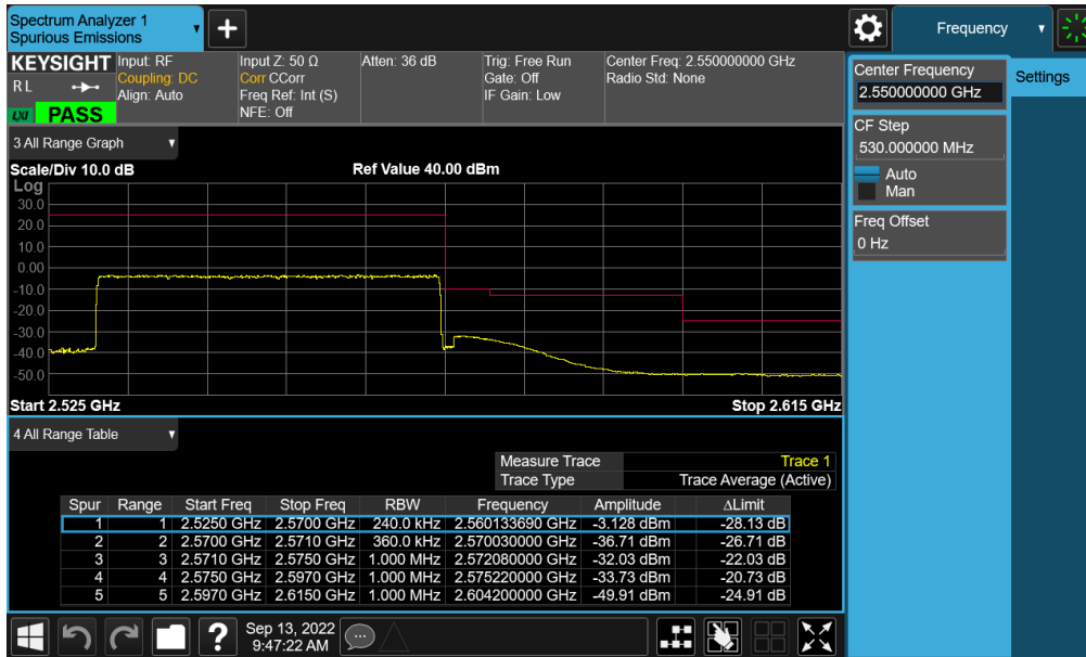
Plot 7-463. Upper Band Edge Plot (NR Band n7 - 40MHz CP-OFDM-QPSK – Full RB - ANT B)
