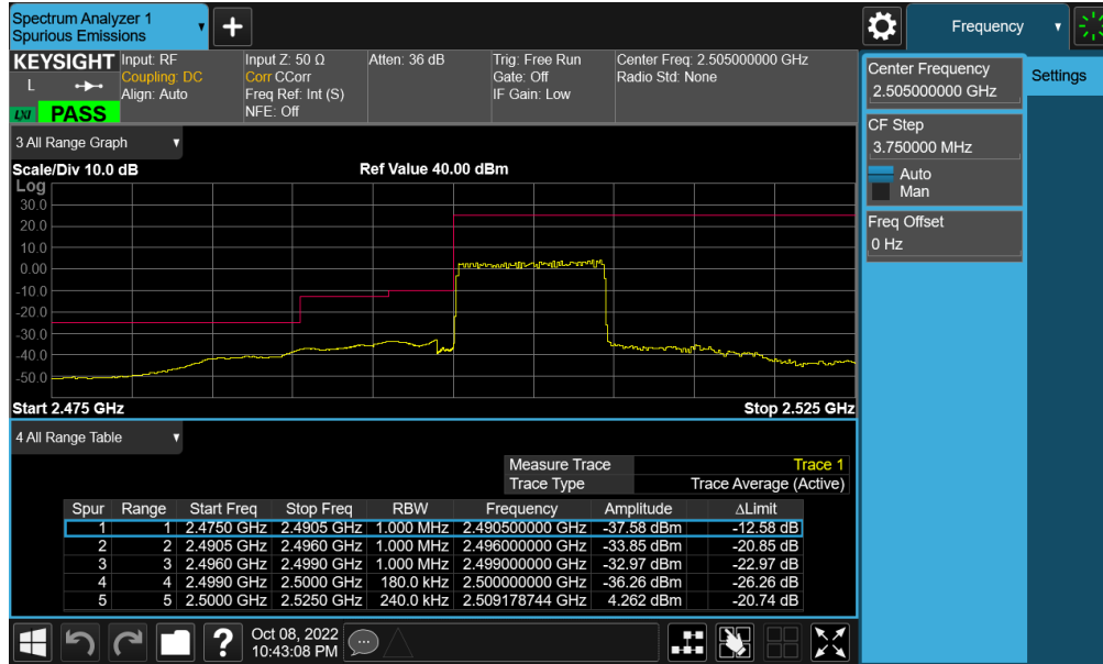
Plot 7-486. Lower Band Edge Plot (NR Band n7 - 10MHz CP-OFDM-QPSK – Full RB - Ant F)
