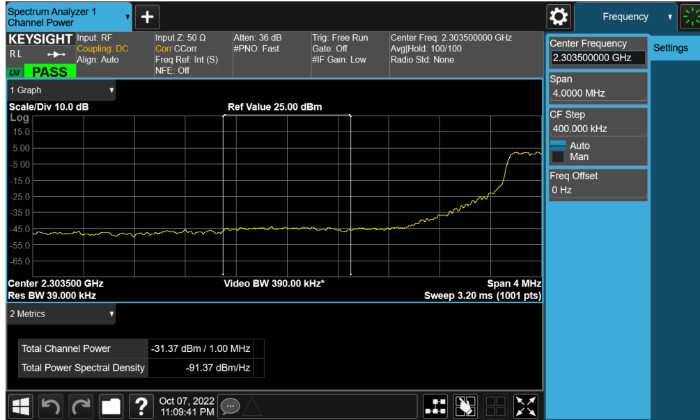
Plot 7-459. Extended Lower Band Edge Plot (NR Band n30 - 5MHz CP-OFDM-QPSK – Full RB - Ant F)
