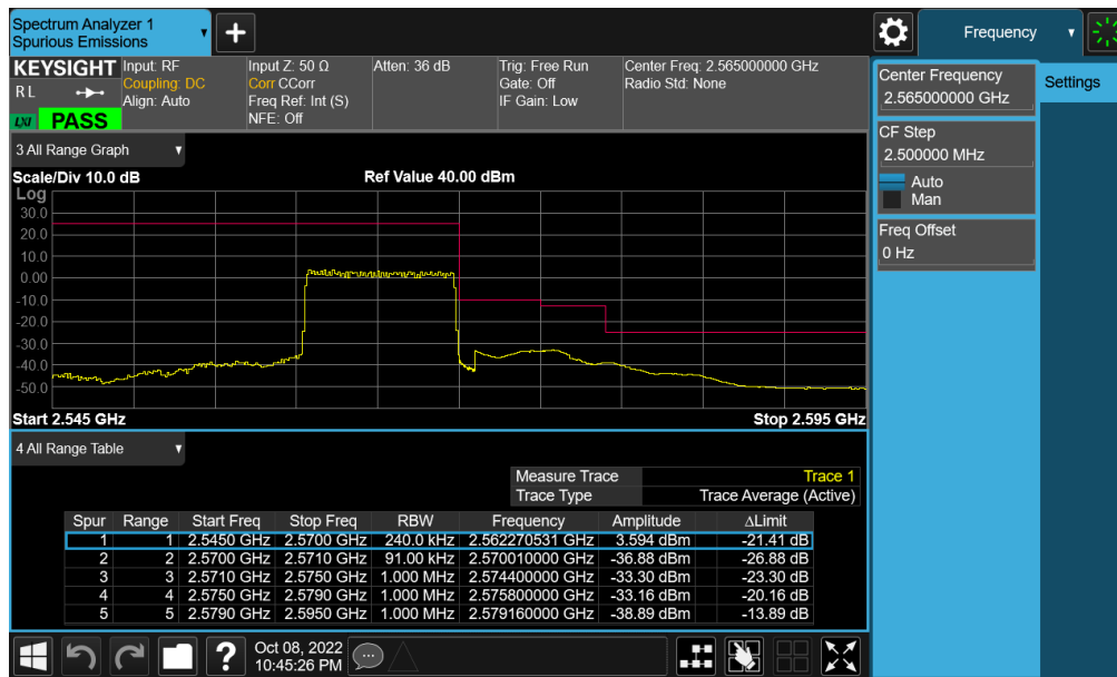
Plot 7-487. Upper Band Edge Plot (NR Band n7 - 10MHz CP-OFDM-QPSK – Full RB - Ant F)
