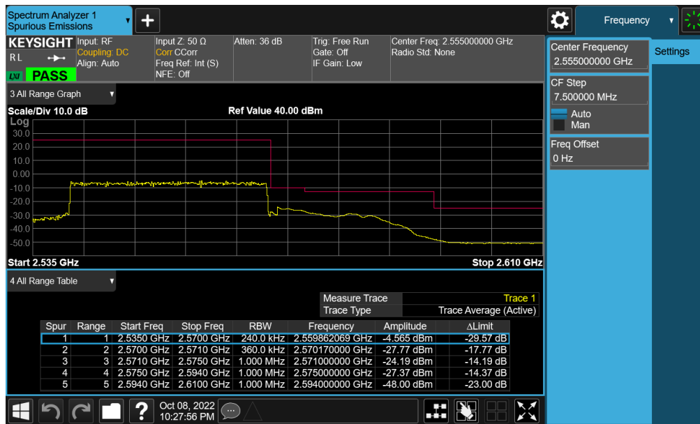
Plot 7-479. Upper Band Edge Plot (NR Band n7 - 30MHz CP-OFDM-QPSK – Full RB - ANT F)
