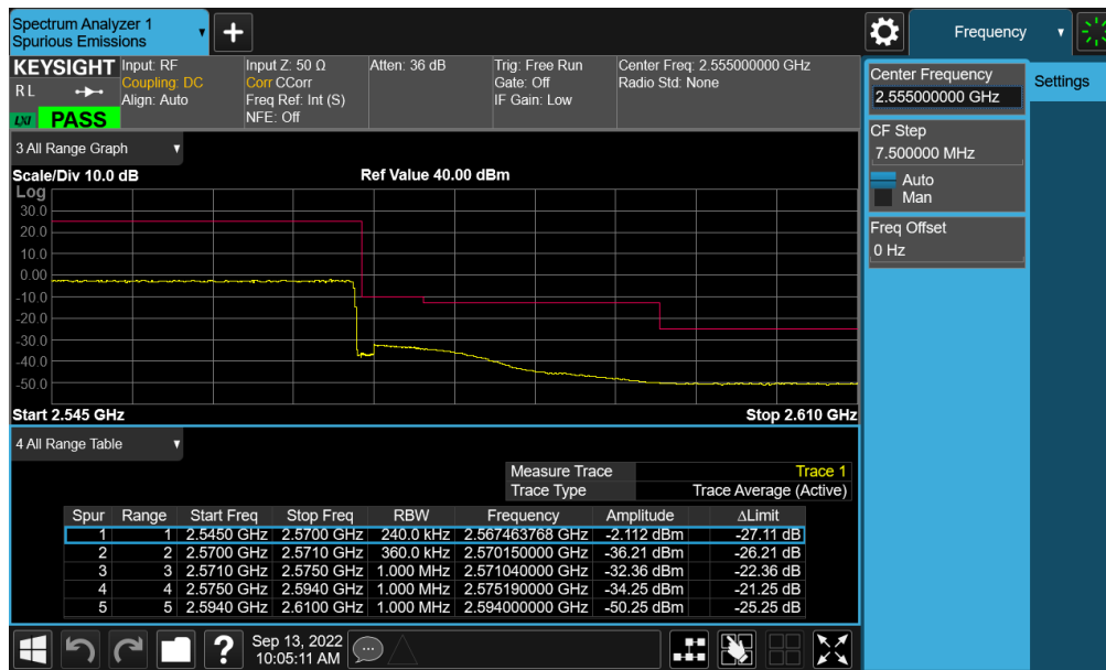
Plot 7-465. Upper Band Edge Plot (NR Band n7 - 30MHz CP-OFDM-QPSK – Full RB - ANT B)
