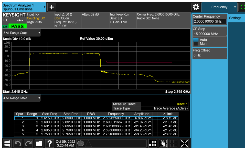
Plot 7-499. Upper ACP Plot (NR Band n41 - 60MHz CP-OFDM-QPSK – Full RB - Ant F)
