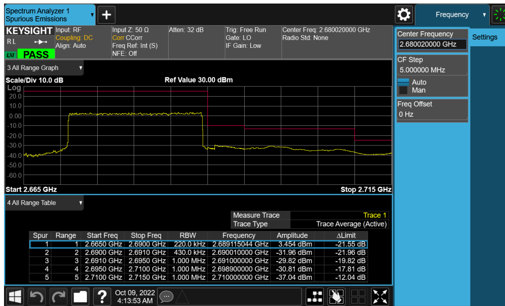
Plot 7-507. Upper ACP Plot (NR Band n41 - 20MHz CP-OFDM-QPSK – Full RB - Ant F)
