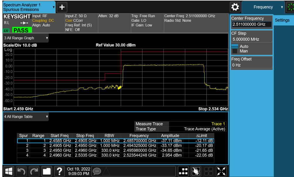
Plot 7-504. Lower ACP Plot (NR Band n41 - 30MHz CP-OFDM-QPSK – Full RB - Ant F)
