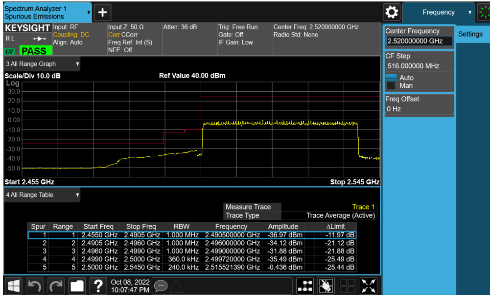
Plot 7-476. Lower Band Edge Plot (NR Band n7 - 40MHz CP-OFDM-QPSK – Full RB - ANT F)
