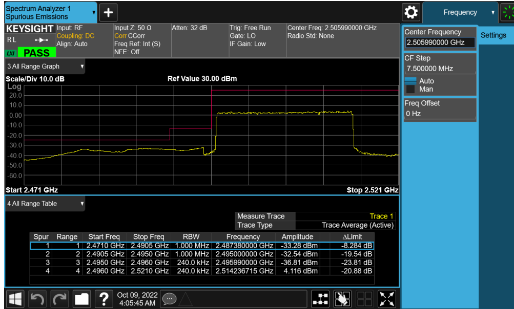
Plot 7-506. Lower ACP Plot (NR Band n41 - 20MHz CP-OFDM-QPSK – Full RB - Ant F)
