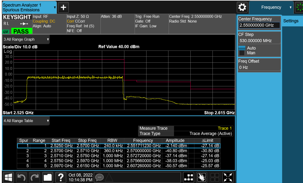
Plot 7-477. Upper Band Edge Plot (NR Band n7 - 40MHz CP-OFDM-QPSK – Full RB - ANT F)
