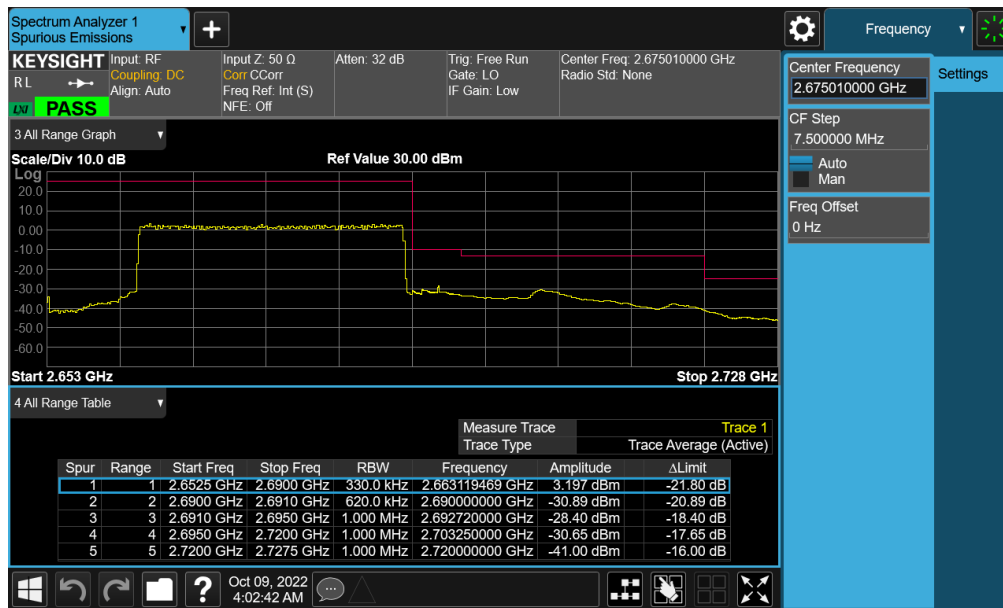
Plot 7-505. Upper ACP Plot (NR Band n41 - 30MHz CP-OFDM-QPSK – Full RB - Ant F)
