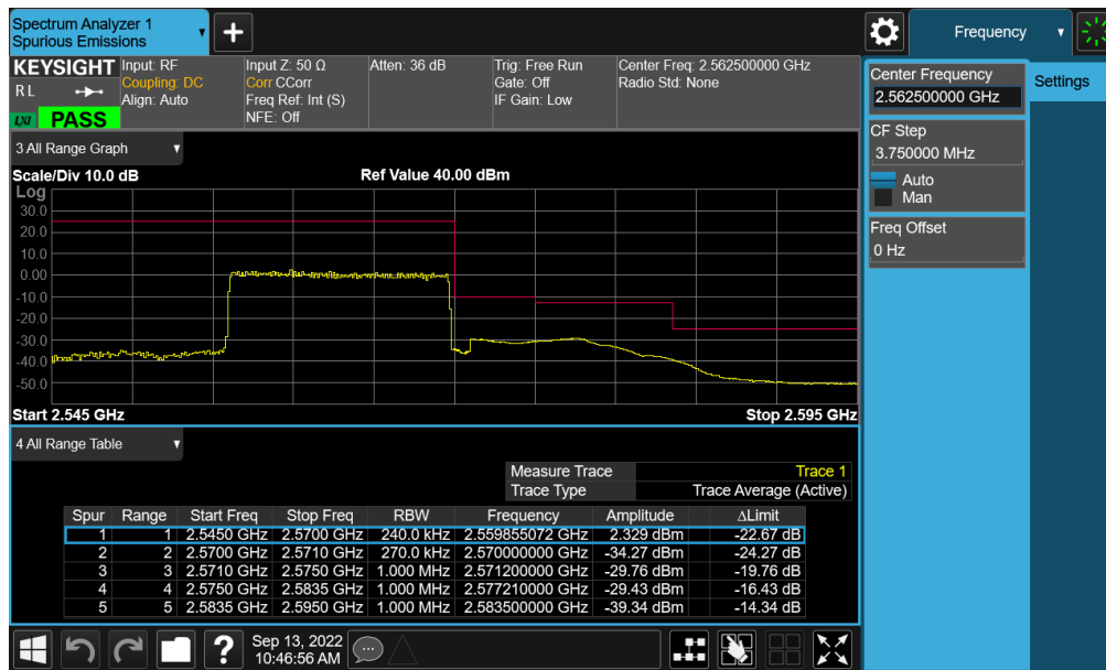
Plot 7-471. Upper Band Edge Plot (NR Band n7 - 15MHz CP-OFDM-QPSK – Full RB - ANT B)
