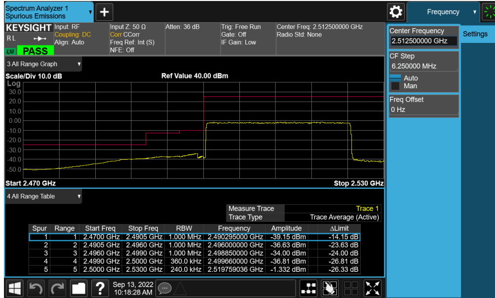
Plot 7-466. Lower Band Edge Plot (NR Band n7 - 25MHz CP-OFDM-QPSK – Full RB - ANT B)
