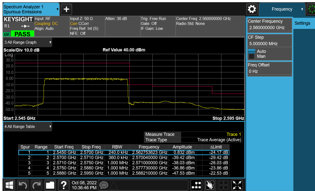
Plot 7-483. Upper Band Edge Plot (NR Band n7 - 20MHz CP-OFDM-QPSK – Full RB - Ant F)
