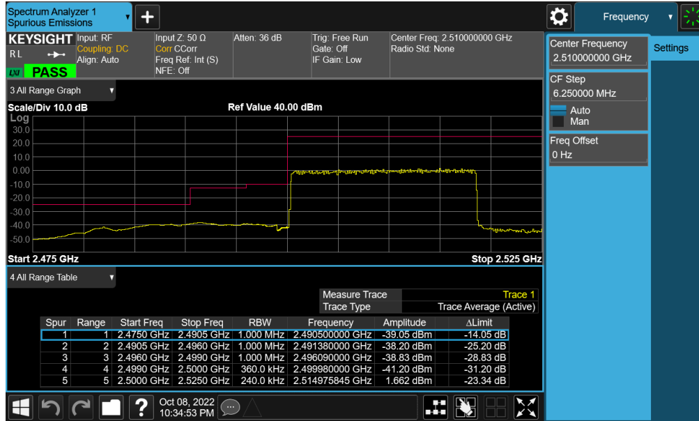
Plot 7-482. Lower Band Edge Plot (NR Band n7 - 20MHz CP-OFDM-QPSK – Full RB - Ant F)
