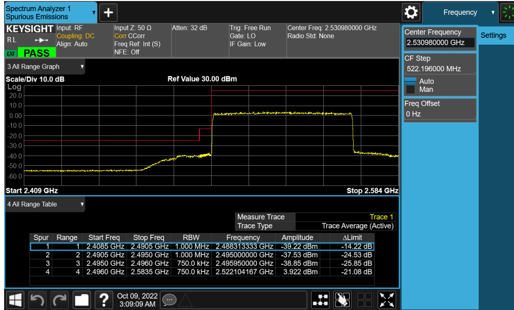
Plot 7-496. Lower ACP Plot (NR Band n41 - 70MHz CP-OFDM-QPSK – Full RB - Ant F)
