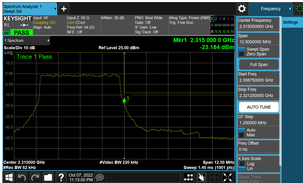
Plot 7-460. Upper Band Edge Plot (NR Band n30 - 5MHz CP-OFDM-QPSK – Full RB - Ant F)
