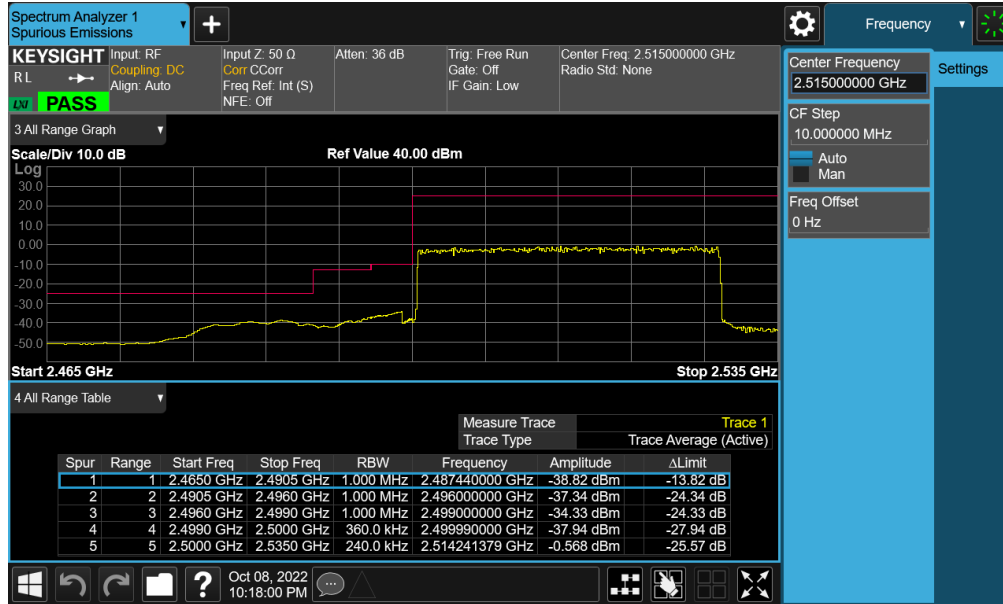
Plot 7-478. Lower Band Edge Plot (NR Band n7 - 30MHz CP-OFDM-QPSK – Full RB - ANT F)
