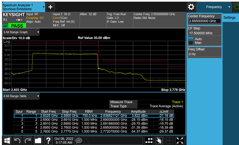
Plot 7-497. Upper ACP Plot (NR Band n41 - 70MHz CP-OFDM-QPSK – Full RB - Ant F)
