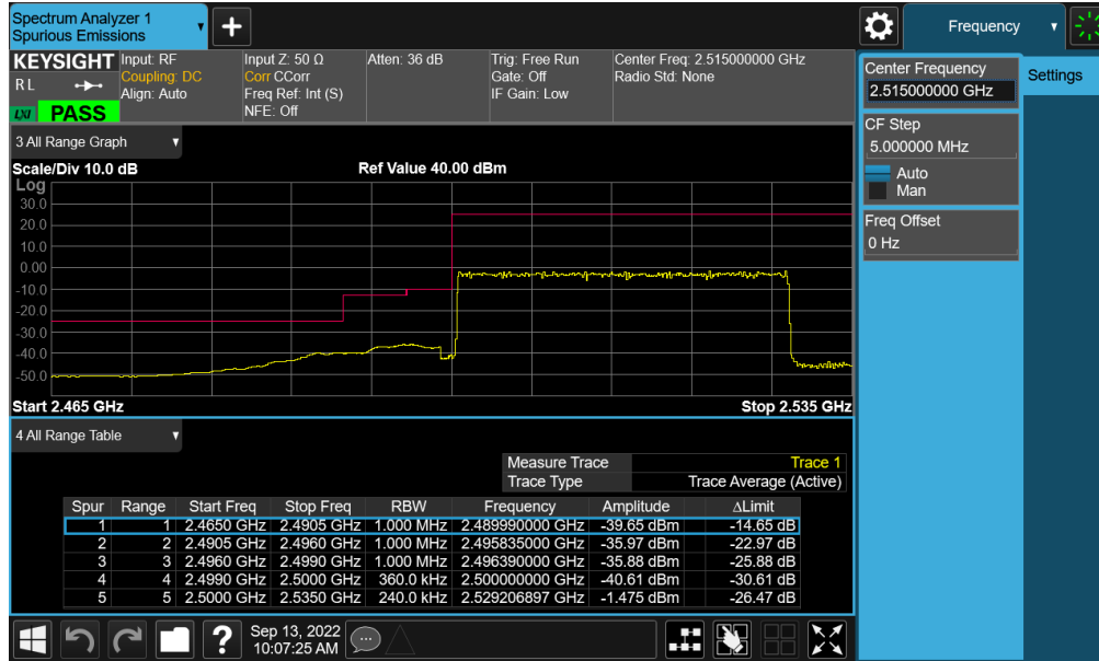
Plot 7-464. Lower Band Edge Plot (NR Band n7 - 30MHz CP-OFDM-QPSK – Full RB - ANT B)
