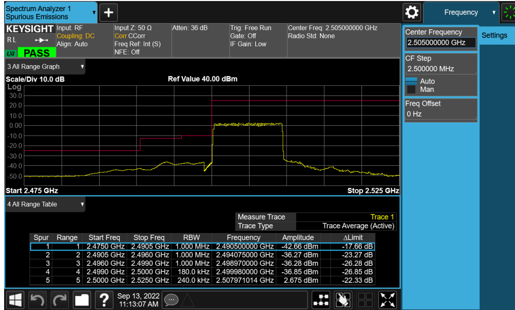
Plot 7-472. Lower Band Edge Plot (NR Band n7 - 10MHz CP-OFDM-QPSK – Full RB - ANT B)
