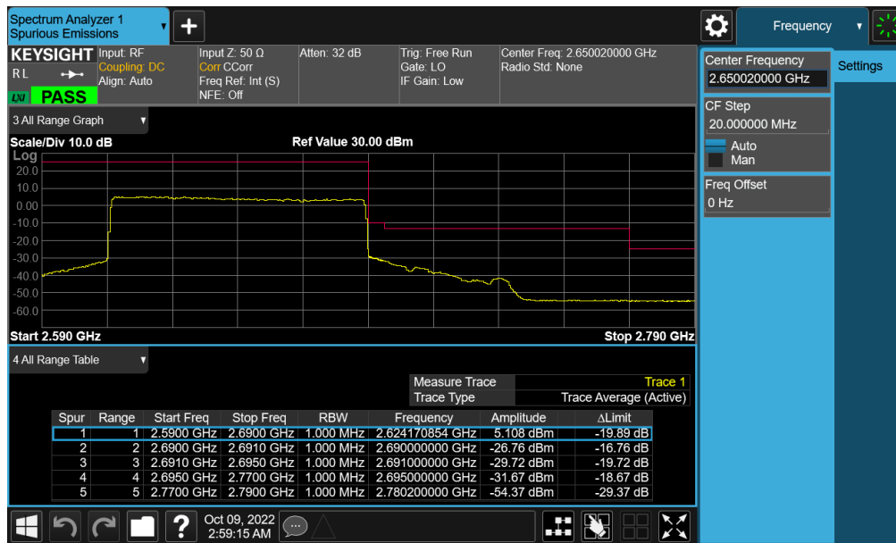
Plot 7-495. Upper ACP Plot (NR Band n41 - 80MHz CP-OFDM-QPSK – Full RB - Ant F)
