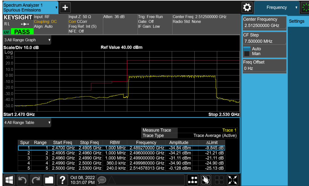
Plot 7-480. Lower Band Edge Plot (NR Band n7 - 25MHz CP-OFDM-QPSK – Full RB - ANT F)
