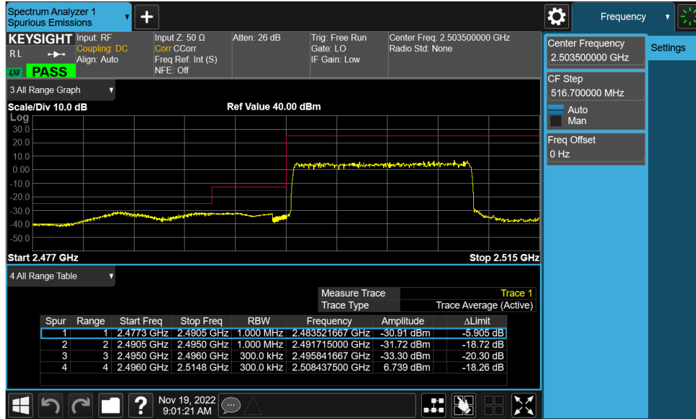
Plot 7-508. Lower ACP Plot (NR Band n41 - 15MHz CP-OFDM-QPSK – Full RB - Ant F)
