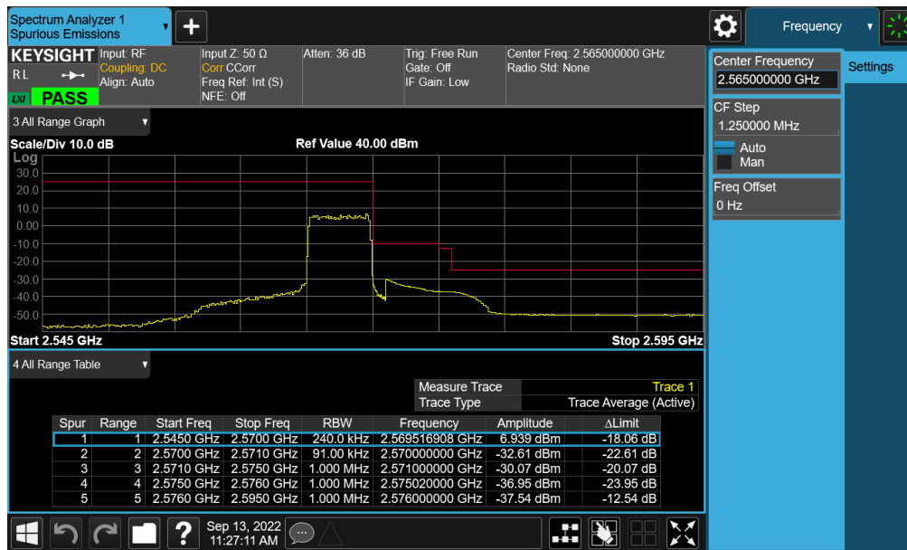
Plot 7-475. Upper Band Edge Plot (NR Band n7 - 5MHz CP-OFDM-QPSK – Full RB - ANT B)
