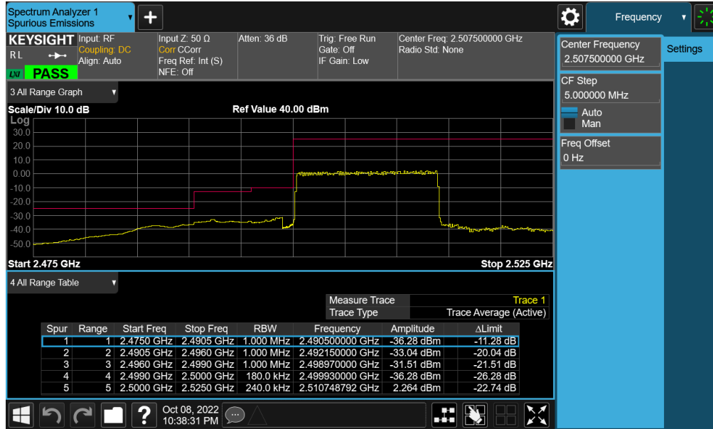
Plot 7-484. Lower Band Edge Plot (NR Band n7 - 15MHz CP-OFDM-QPSK – Full RB - Ant F)
