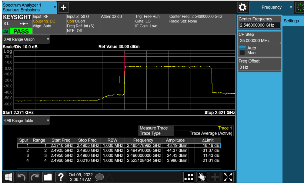
Plot 7-490. Lower ACP Plot (NR Band n41 - 100MHz CP-OFDM-QPSK – Full RB - Ant F)
