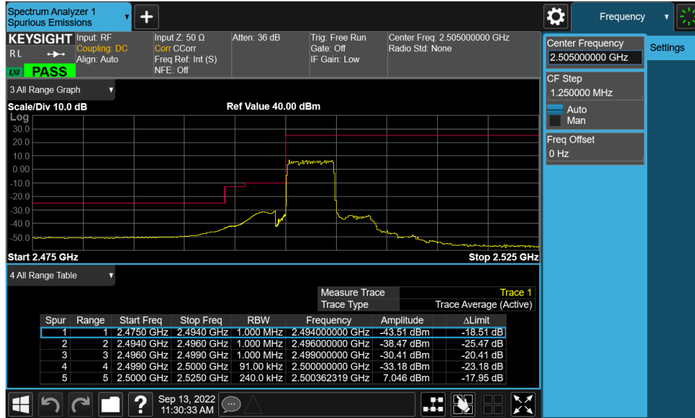
Plot 7-474. Lower Band Edge Plot (NR Band n7 - 5MHz CP-OFDM-QPSK – Full RB - ANT B)
