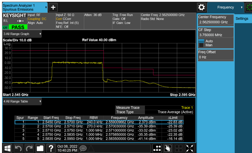
Plot 7-485. Upper Band Edge Plot (NR Band n7 - 15MHz CP-OFDM-QPSK – Full RB - Ant F)
