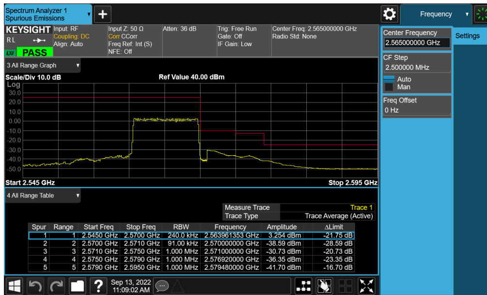
Plot 7-473. Upper Band Edge Plot (NR Band n7 - 10MHz CP-OFDM-QPSK – Full RB - ANT B)
