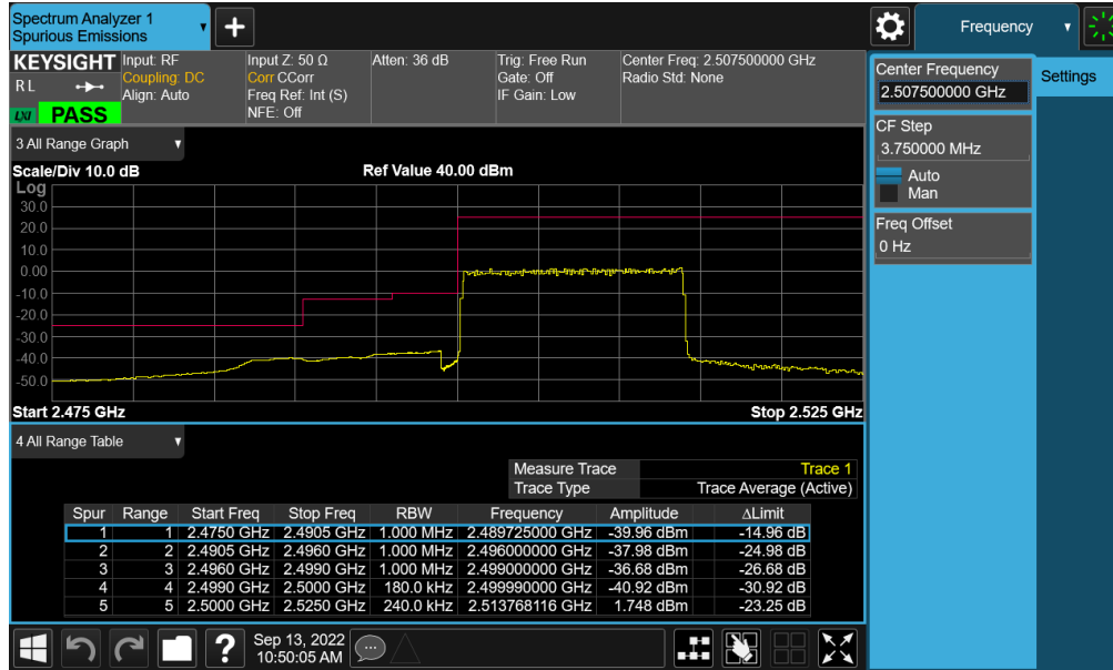
Plot 7-470. Lower Band Edge Plot (NR Band n7 - 15MHz CP-OFDM-QPSK – Full RB - ANT B)
