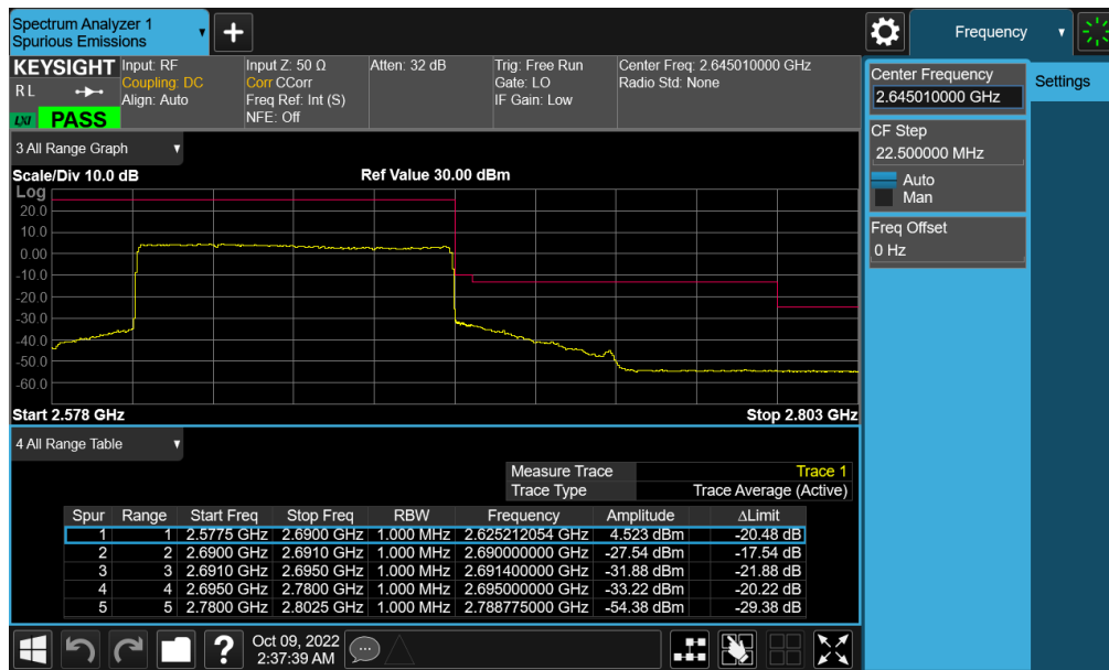
Plot 7-493. Upper ACP Plot (NR Band n41 - 90MHz CP-OFDM-QPSK – Full RB - Ant F)
