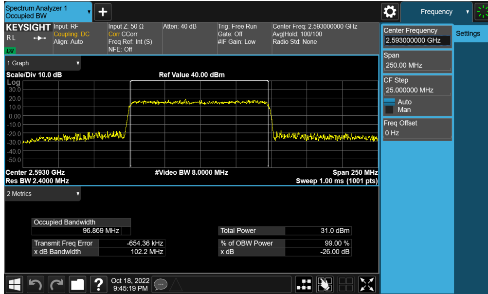
Plot 7-146. Occupied Bandwidth Plot (NR Band n41 - 100MHz 16-QAM - Full RB Switching - Ant B)
