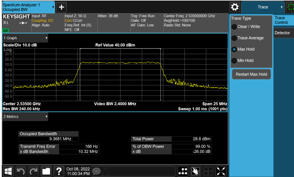
Plot 7-106. Occupied Bandwidth Plot (NR Band n7 - 10MHz QPSK - Full RB - Ant F)
