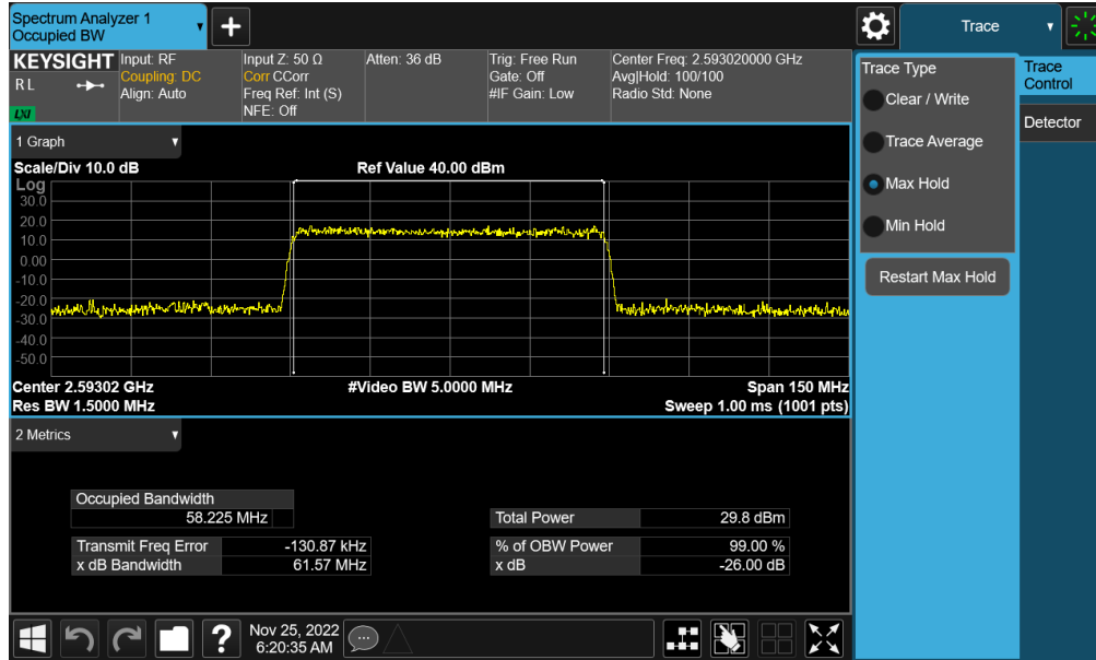
Plot 7-158. Occupied Bandwidth Plot (NR Band n41 - 60MHz 16-QAM - Full RB Switching - Ant B)
