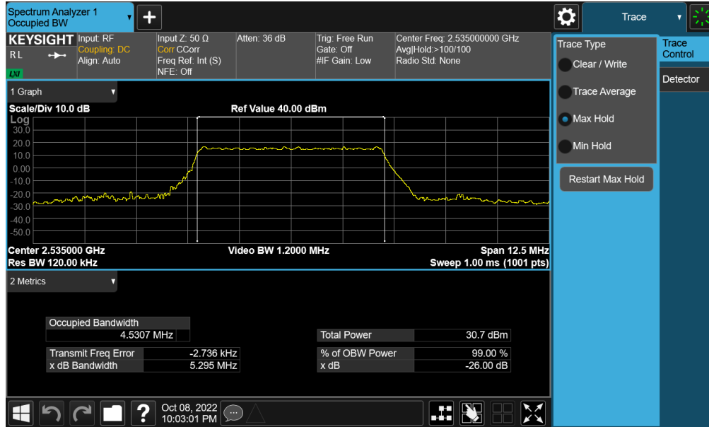
Plot 7-108. Occupied Bandwidth Plot (NR Band n7 - 5MHz \pi/2 BPSK - Full RB - Ant F)
