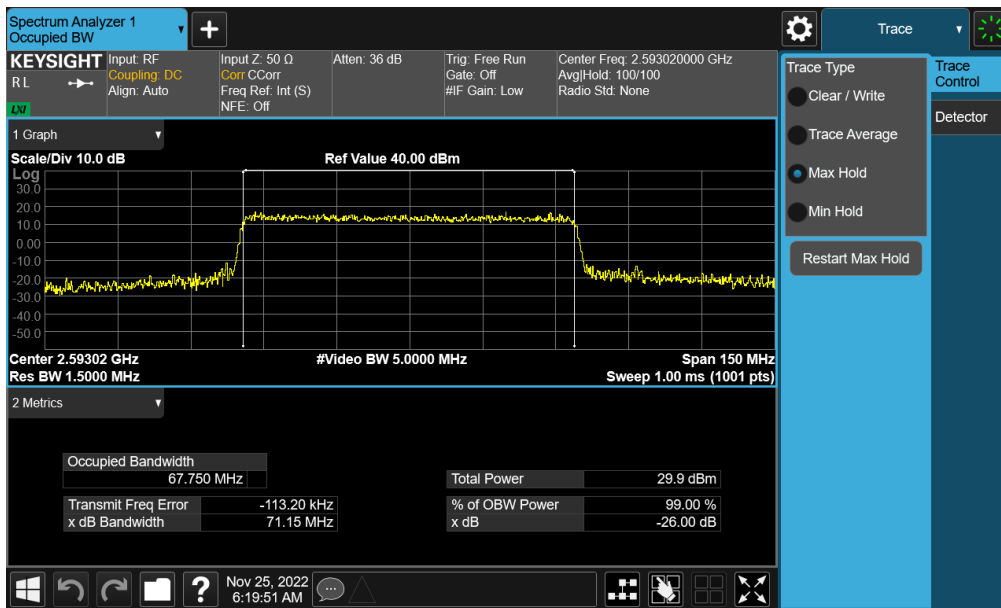
Plot 7-155. Occupied Bandwidth Plot (NR Band n41 - 70MHz 16-QAM - Full RB Switching - Ant B)
