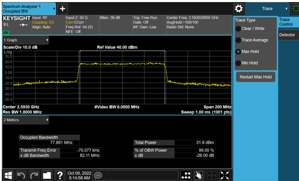
Plot 7-118. Occupied Bandwidth Plot (NR Band n41 - 80MHz QPSK - Full RB - Ant F)
