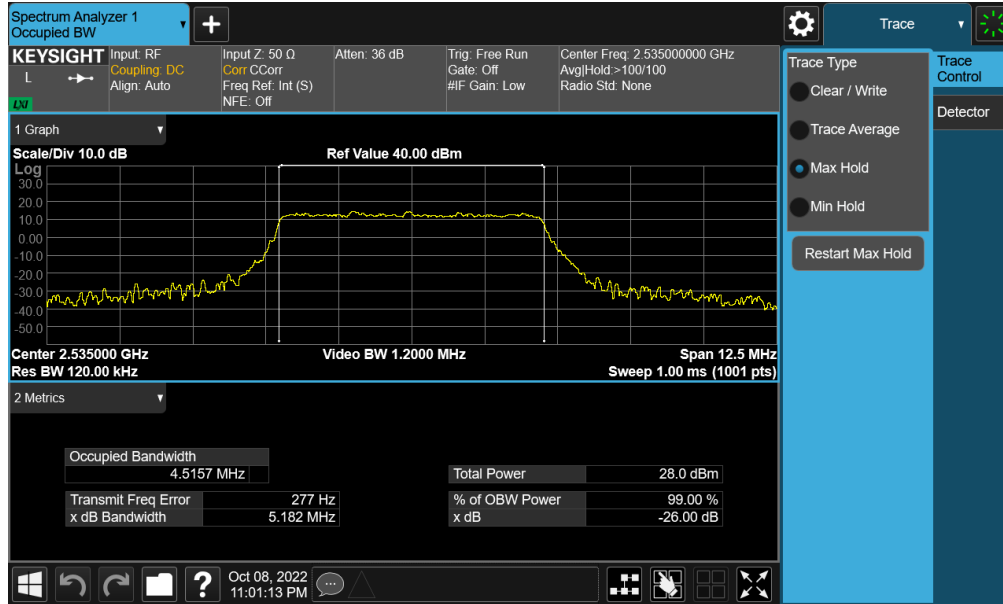
Plot 7-110. Occupied Bandwidth Plot (NR Band n7 - 5MHz 16-QAM - Full RB - Ant F)
