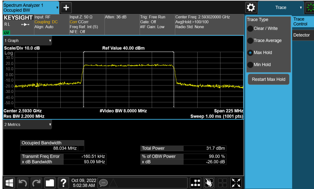
Plot 7-115. Occupied Bandwidth Plot (NR Band n41 - 90MHz QPSK - Full RB - Ant F)
