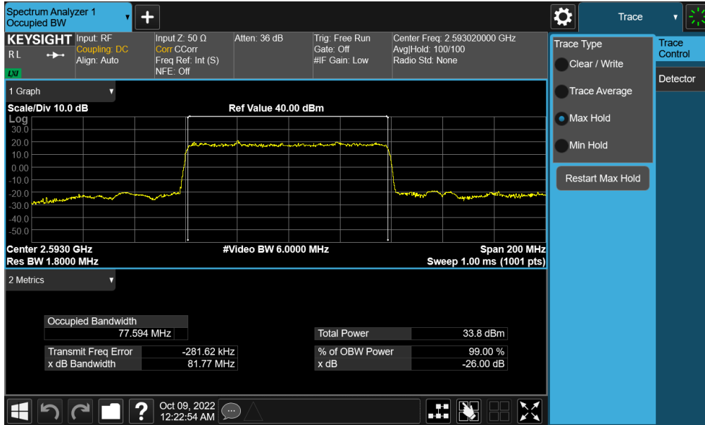
Plot 7-117. Occupied Bandwidth Plot (NR Band n41 - 80MHz \pi/2 BPSK - Full RB - Ant F)
