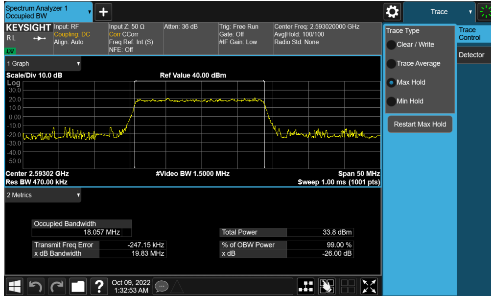
Plot 7-135. Occupied Bandwidth Plot (NR Band n41 - 20MHz \pi/2 BPSK - Full RB - Ant F)
