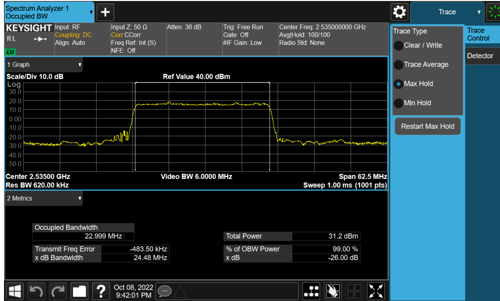
Plot 7-96. Occupied Bandwidth Plot (NR Band n7 - 25MHz \pi/2 BPSK - Full RB - Ant F)
