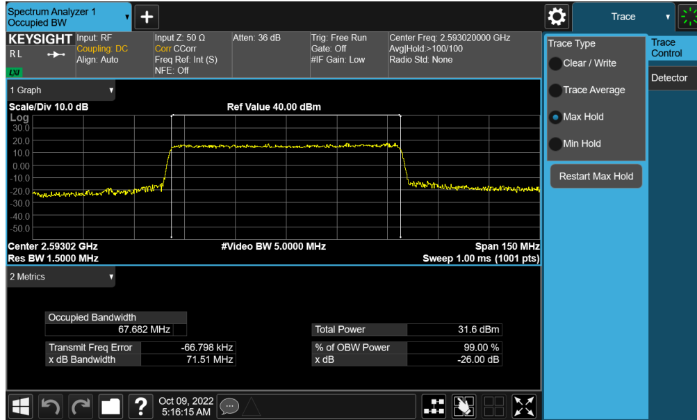
Plot 7-121. Occupied Bandwidth Plot (NR Band n41 - 70MHz QPSK - Full RB - Ant F)
