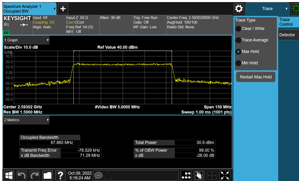
Plot 7-122. Occupied Bandwidth Plot (NR Band n41 - 70MHz 16-QAM - Full RB - Ant F)
