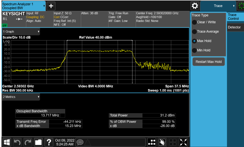
Plot 7-139. Occupied Bandwidth Plot (NR Band n41 - 15MHz QPSK - Full RB - Ant F)
