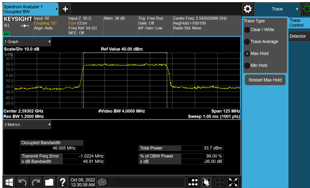
Plot 7-126. Occupied Bandwidth Plot (NR Band n41 - 50MHz \pi/2 BPSK - Full RB - Ant F)
