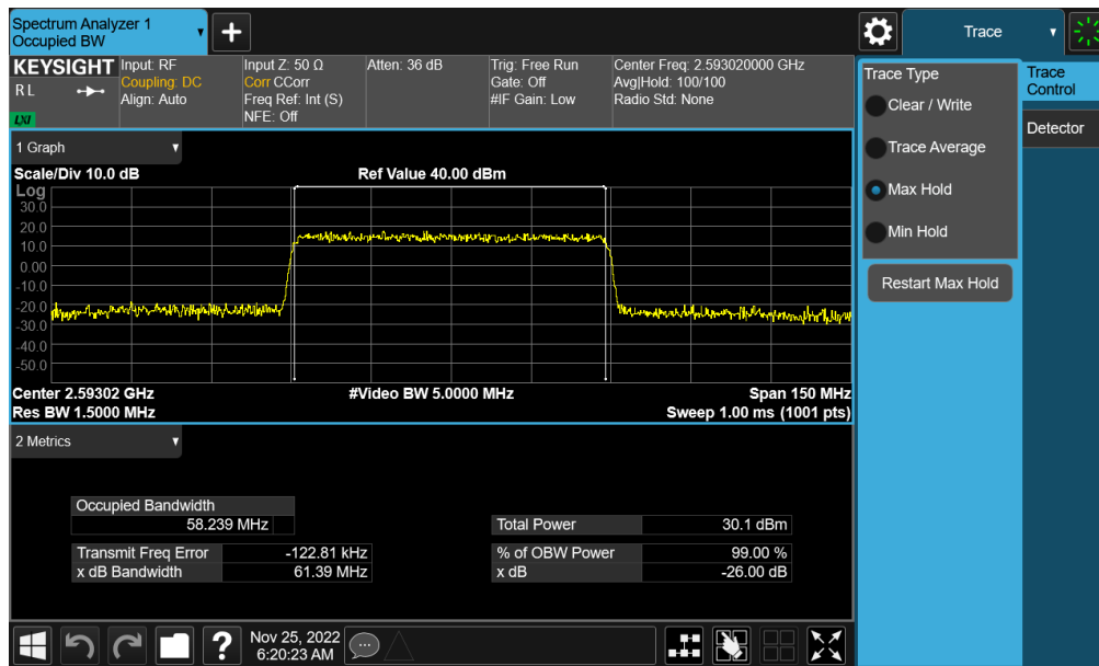
Plot 7-157. Occupied Bandwidth Plot (NR Band n41 - 60MHz QPSK - Full RB Switching - Ant B)
