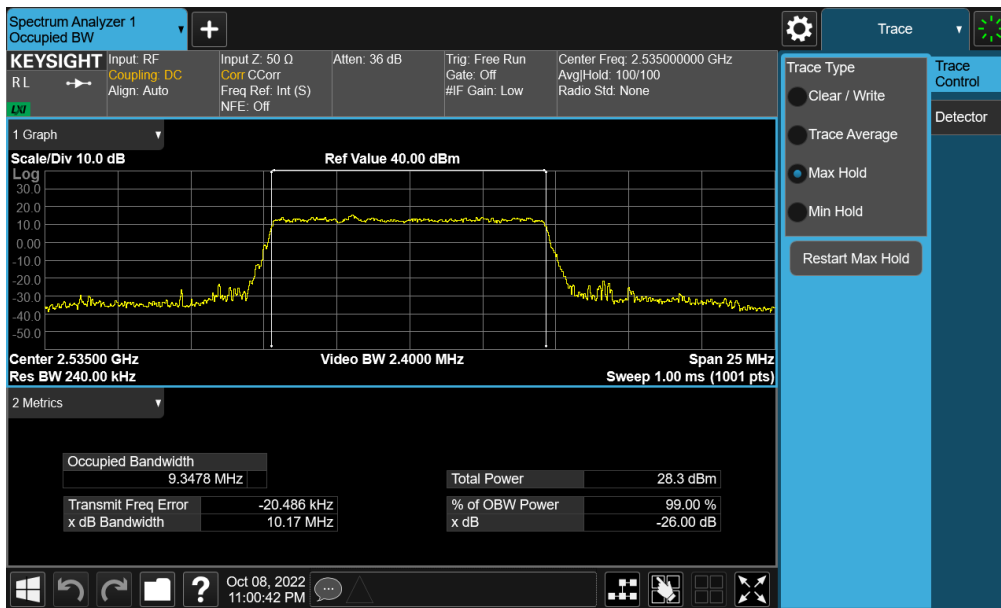
Plot 7-107. Occupied Bandwidth Plot (NR Band n7 - 10MHz 16-QAM - Full RB - Ant F)
