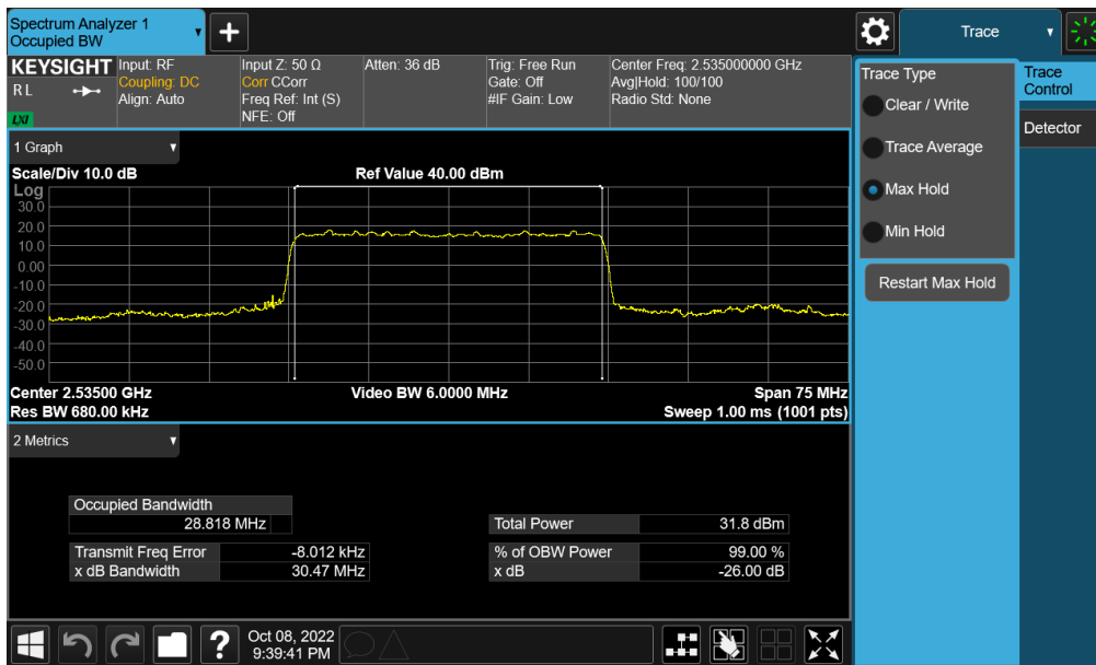
Plot 7-93. Occupied Bandwidth Plot (NR Band n7 - 30MHz \pi/2 BPSK - Full RB - Ant F)
