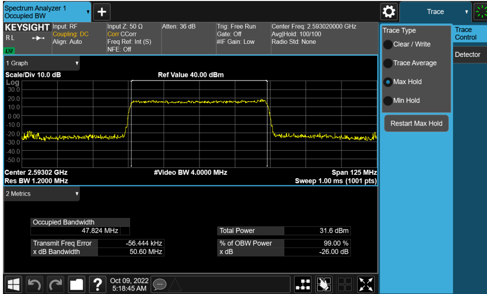
Plot 7-127. Occupied Bandwidth Plot (NR Band n41 - 50MHz QPSK - Full RB - Ant F)
