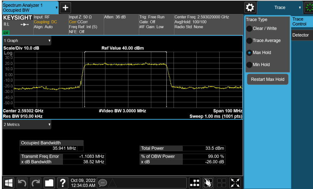
Plot 7-129. Occupied Bandwidth Plot (NR Band n41 - 40MHz \pi/2 BPSK - Full RB - Ant F)
