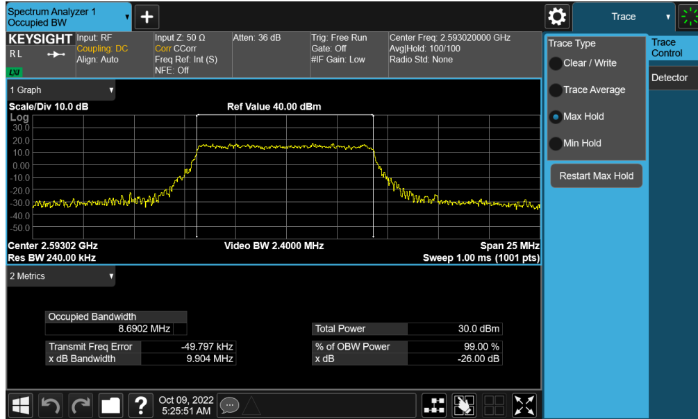
Plot 7-143. Occupied Bandwidth Plot (NR Band n41 - 10MHz 16-QAM - Full RB - Ant F)
