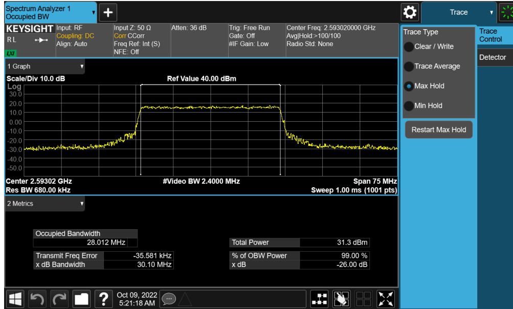
Plot 7-133. Occupied Bandwidth Plot (NR Band n41 - 30MHz QPSK - Full RB - Ant F)
