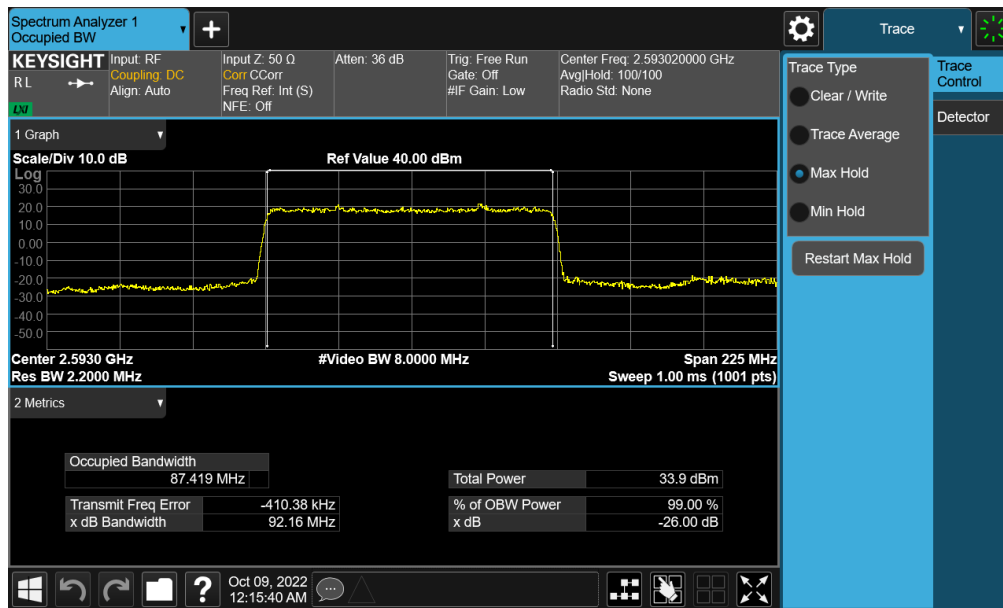
Plot 7-114. Occupied Bandwidth Plot (NR Band n41 - 90MHz \pi/2 BPSK - Full RB - Ant F)
