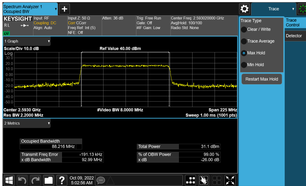
Plot 7-116. Occupied Bandwidth Plot (NR Band n41 - 90MHz 16-QAM - Full RB - Ant F)
