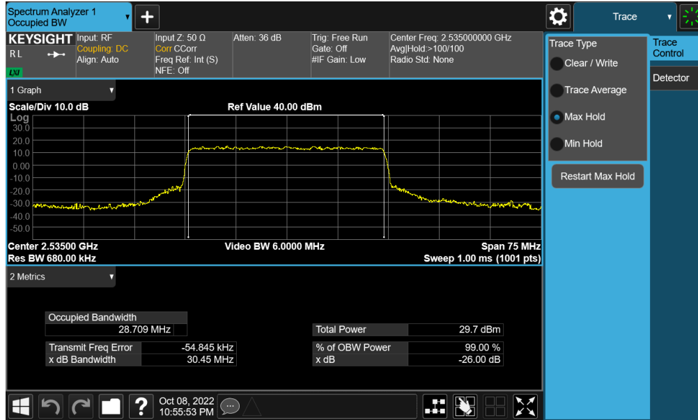
Plot 7-94. Occupied Bandwidth Plot (NR Band n7 - 30MHz QPSK - Full RB - Ant F)
