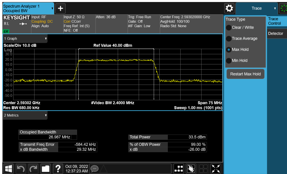
Plot 7-132. Occupied Bandwidth Plot (NR Band n41 - 30MHz \pi/2 BPSK - Full RB - Ant F)
