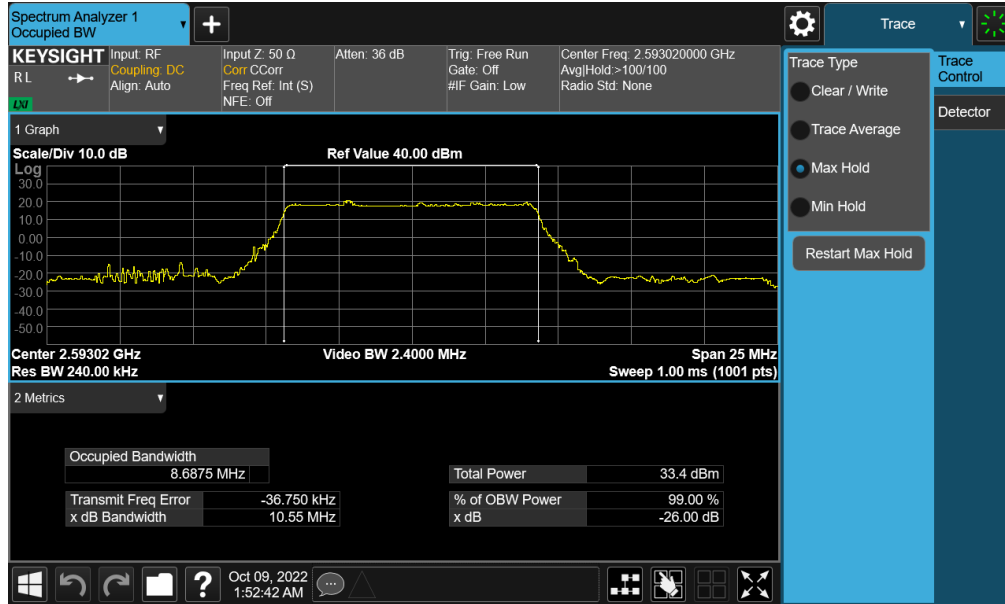
Plot 7-141. Occupied Bandwidth Plot (NR Band n41 - 10MHz \pi/2 BPSK - Full RB - Ant F)
