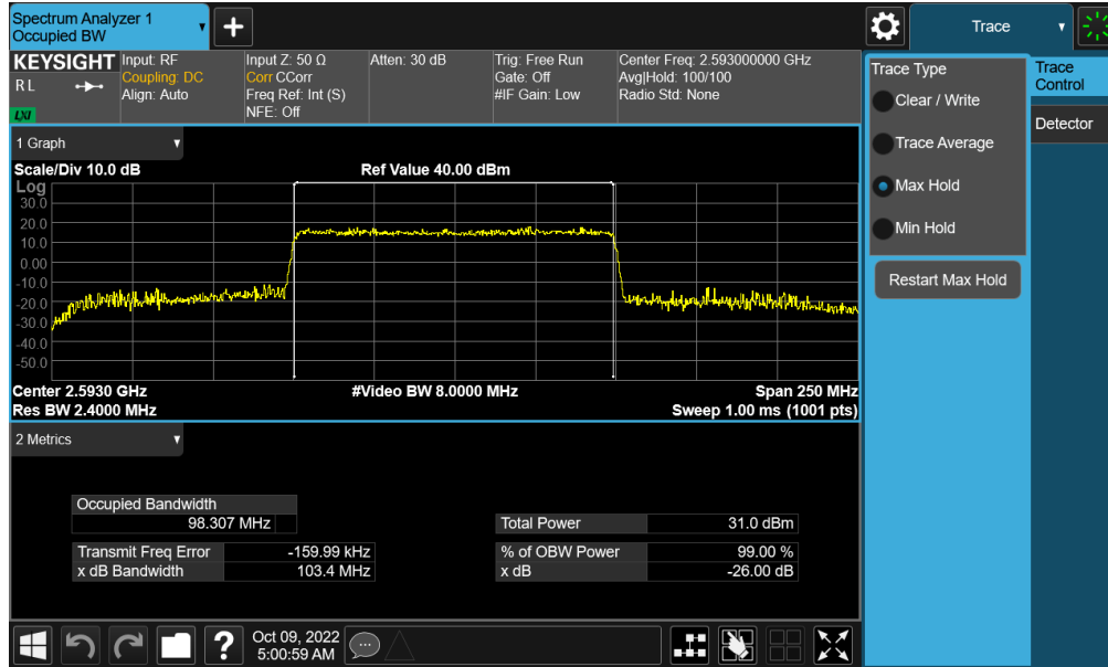
Plot 7-113. Occupied Bandwidth Plot (NR Band n41 - 100MHz 16-QAM - Full RB - Ant F)
