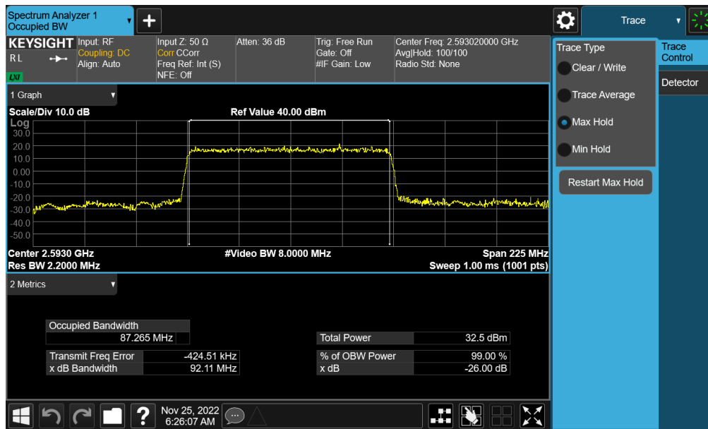
Plot 7-147. Occupied Bandwidth Plot (NR Band n41 - 90MHz \pi/2 BPSK - Full RB Switching - Ant B)
