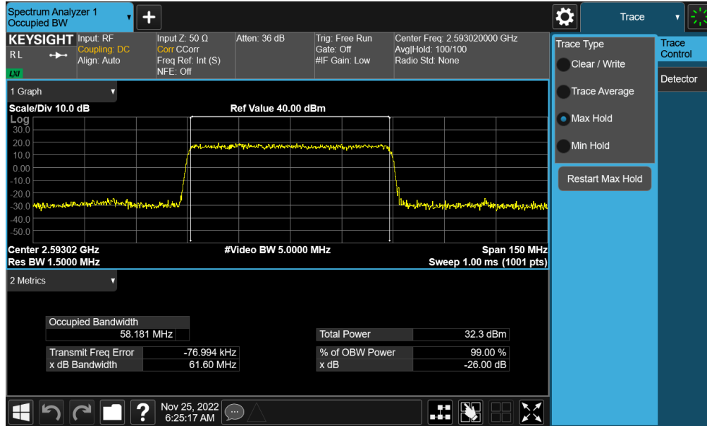
Plot 7-156. Occupied Bandwidth Plot (NR Band n41 - 60MHz \pi/2 BPSK - Full RB Switching - Ant B)
