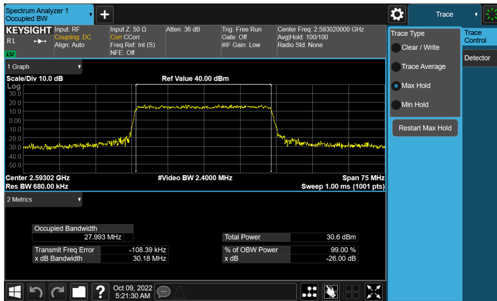
Plot 7-134. Occupied Bandwidth Plot (NR Band n41 - 30MHz 16-QAM - Full RB - Ant F)
