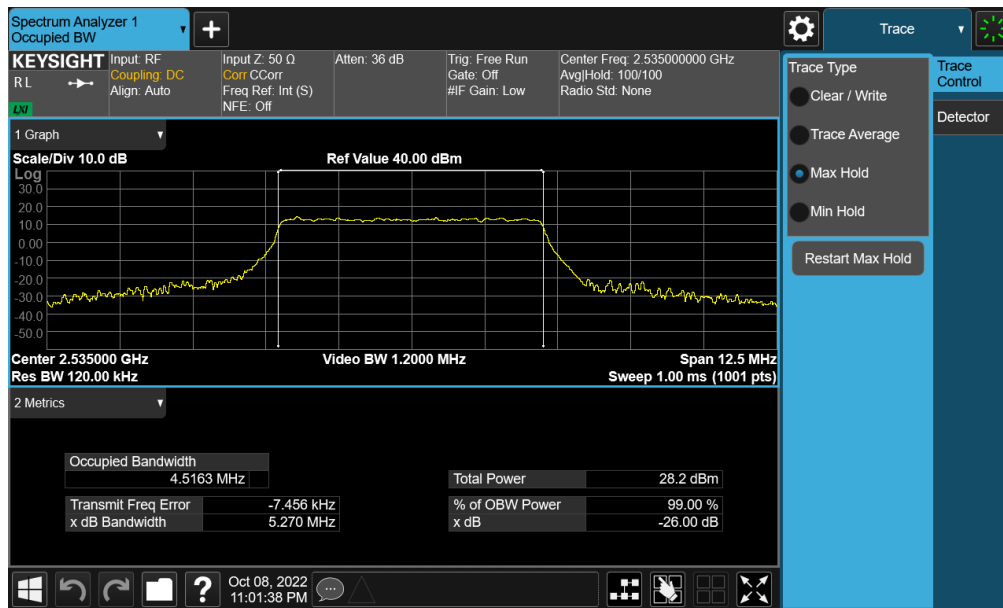
Plot 7-109. Occupied Bandwidth Plot (NR Band n7 - 5MHz QPSK - Full RB - Ant F)
