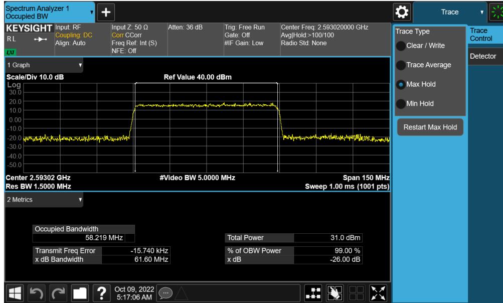
Plot 7-125. Occupied Bandwidth Plot (NR Band n41 - 60MHz 16-QAM - Full RB - Ant F)
