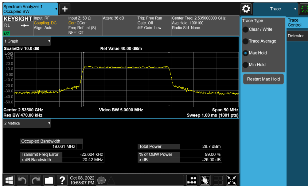
Plot 7-101. Occupied Bandwidth Plot (NR Band n7 - 20MHz 16-QAM - Full RB - Ant F)
