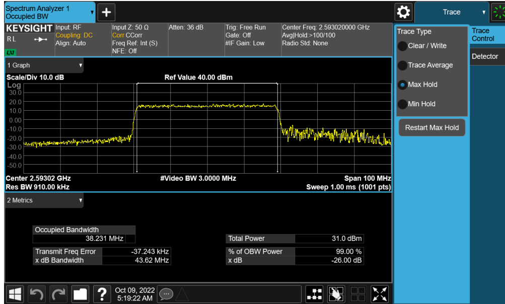
Plot 7-131. Occupied Bandwidth Plot (NR Band n41 - 40MHz 16-QAM - Full RB - Ant F)
