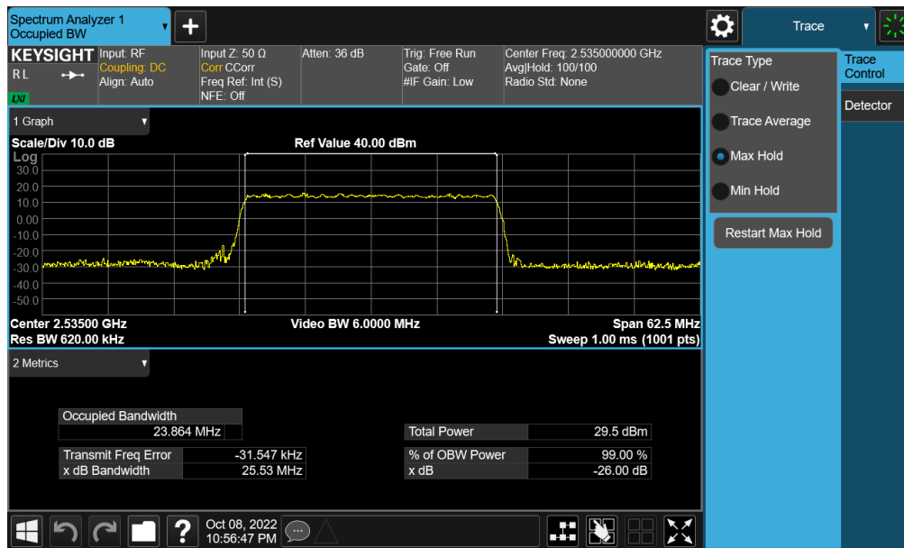
Plot 7-97. Occupied Bandwidth Plot (NR Band n7 - 25MHz QPSK - Full RB - Ant F)
