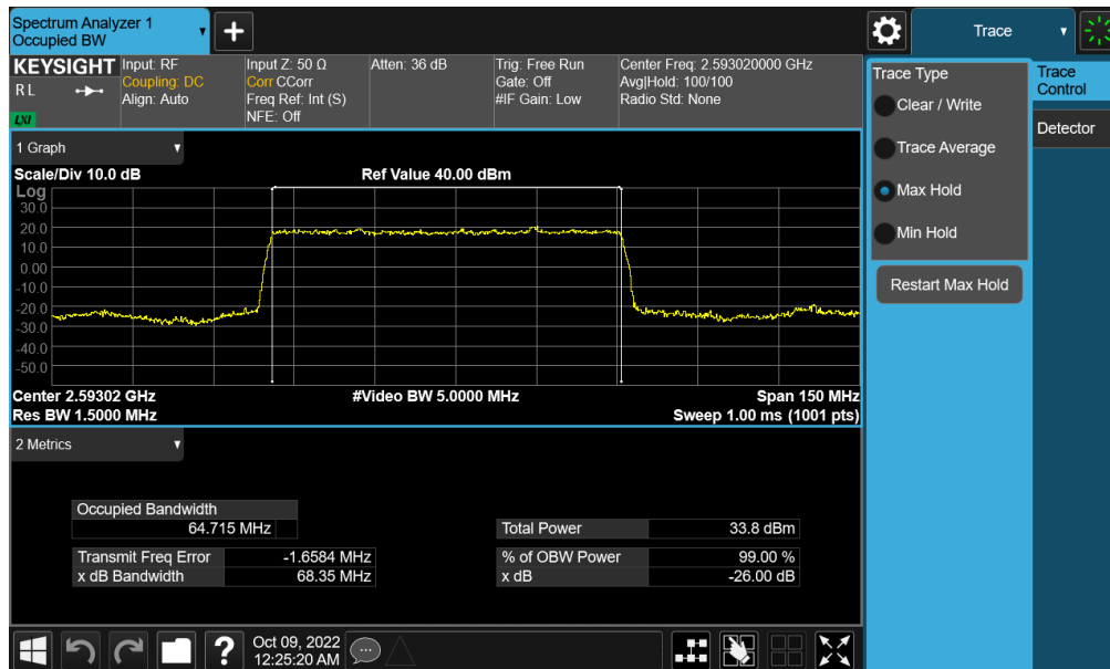
Plot 7-120. Occupied Bandwidth Plot (NR Band n41 - 70MHz \pi/2 BPSK - Full RB - Ant F)
