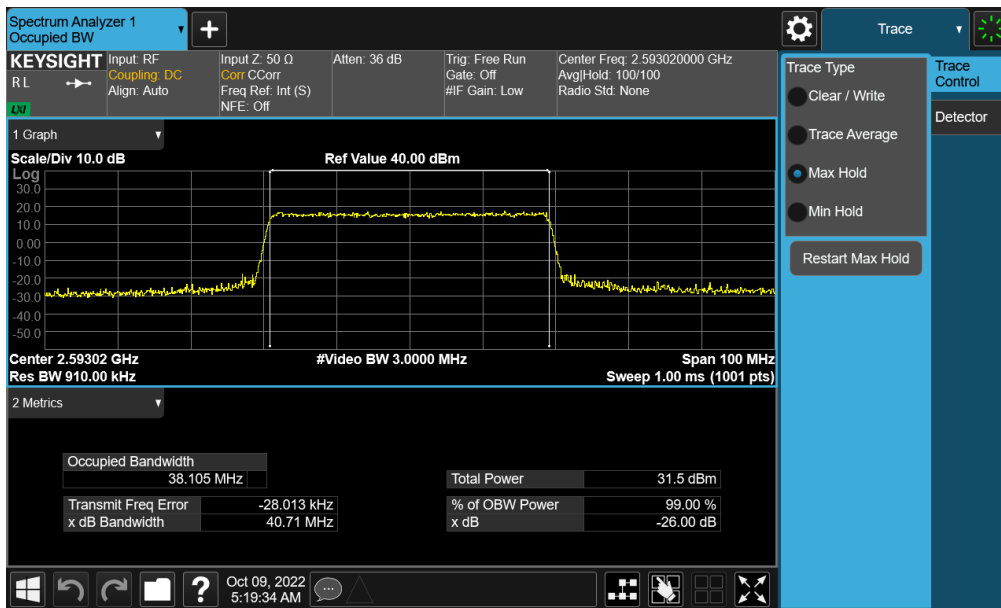
Plot 7-130. Occupied Bandwidth Plot (NR Band n41 - 40MHz QPSK - Full RB - Ant F)
