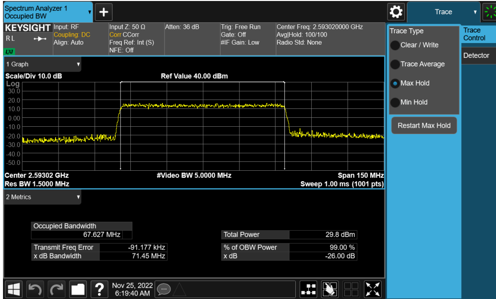
Plot 7-154. Occupied Bandwidth Plot (NR Band n41 - 70MHz QPSK - Full RB Switching - Ant B)
