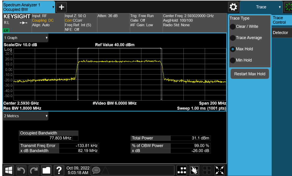
Plot 7-119. Occupied Bandwidth Plot (NR Band n41 - 80MHz 16-QAM - Full RB - Ant F)
