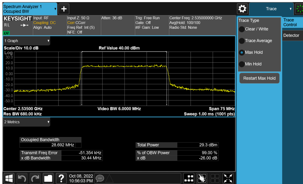
Plot 7-95. Occupied Bandwidth Plot (NR Band n7 - 30MHz 16-QAM - Full RB - Ant F)
