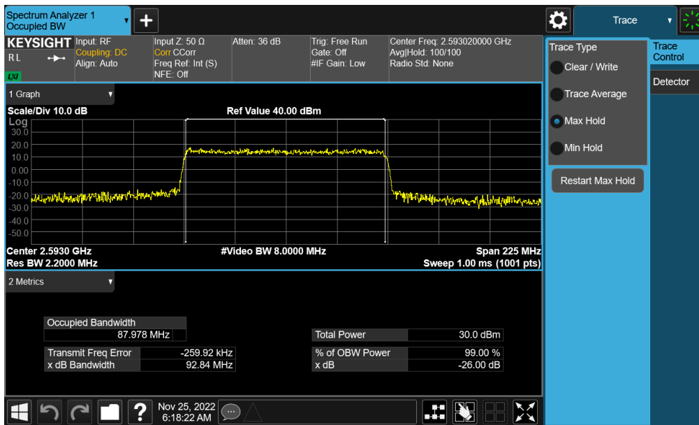
Plot 7-149. Occupied Bandwidth Plot (NR Band n41 - 90MHz 16-QAM - Full RB Switching - Ant B)
