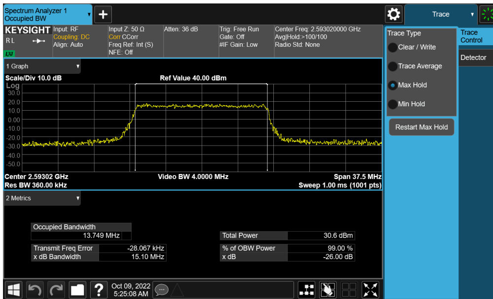
Plot 7-140. Occupied Bandwidth Plot (NR Band n41 - 15MHz 16-QAM - Full RB - Ant F)
