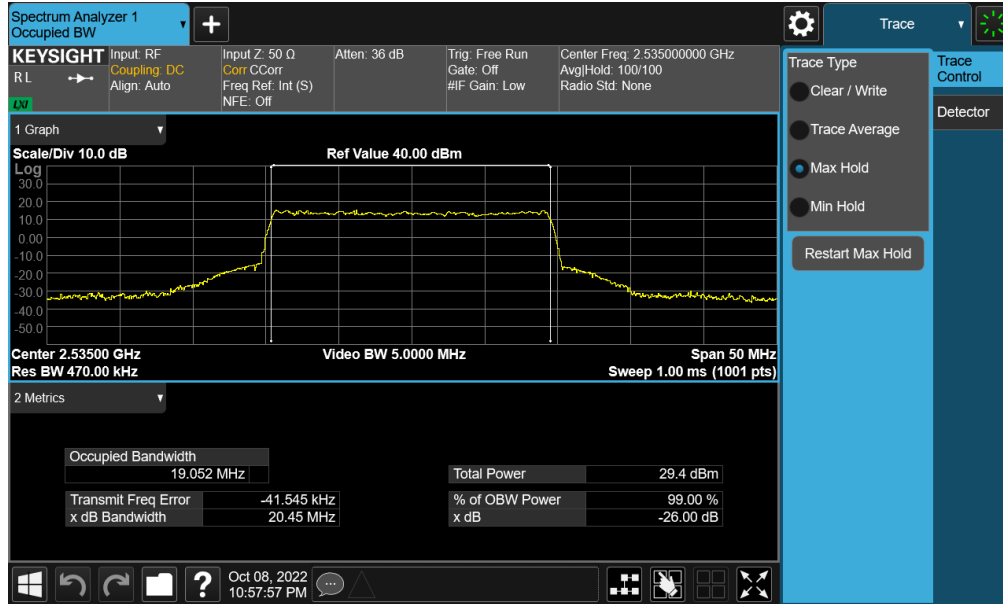
Plot 7-100. Occupied Bandwidth Plot (NR Band n7 - 20MHz QPSK - Full RB - Ant F)
