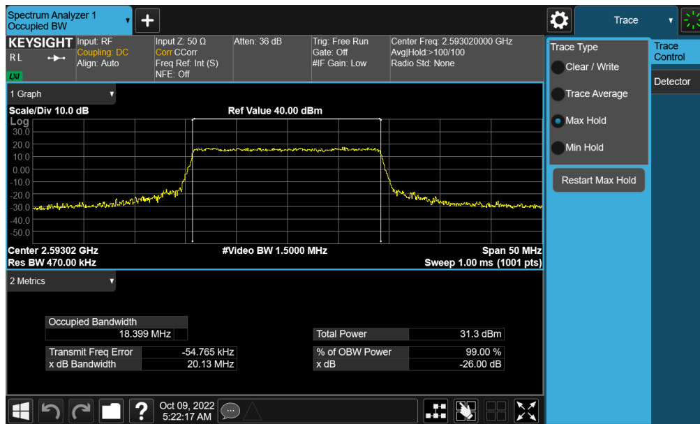
Plot 7-136. Occupied Bandwidth Plot (NR Band n41 - 20MHz QPSK - Full RB - Ant F)
