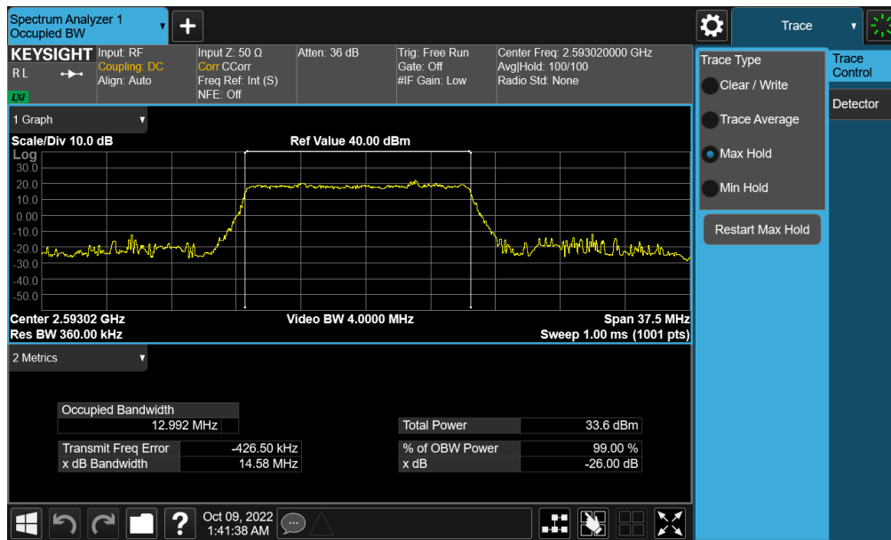
Plot 7-138. Occupied Bandwidth Plot (NR Band n41 - 15MHz \pi/2 BPSK - Full RB - Ant F)
