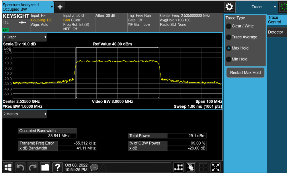
Plot 7-92. Occupied Bandwidth Plot (NR Band n7 - 40MHz 16-QAM - Full RB - Ant F)
