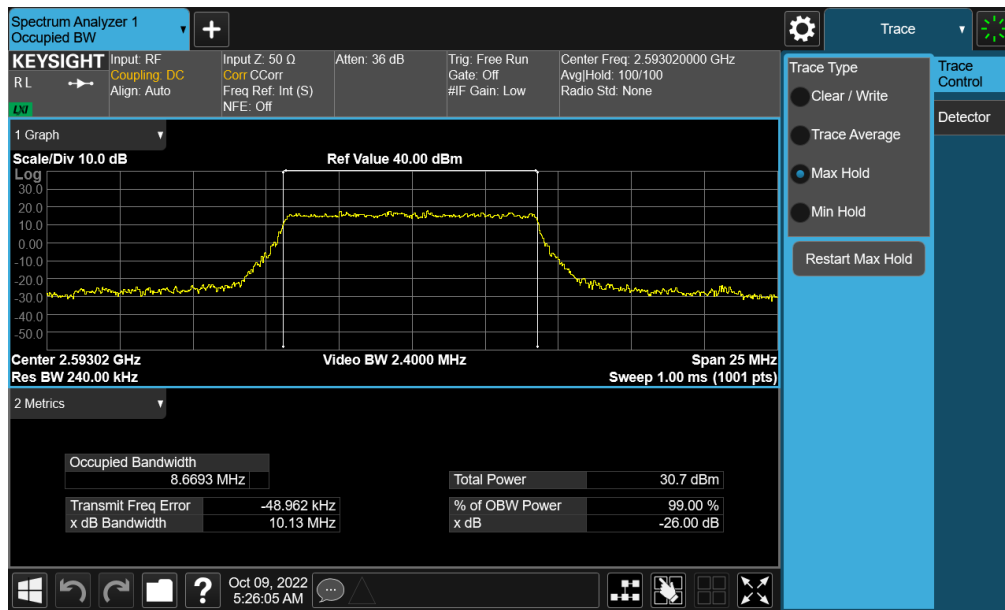
Plot 7-142. Occupied Bandwidth Plot (NR Band n41 - 10MHz QPSK - Full RB - Ant F)
