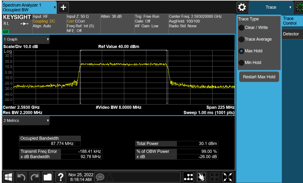
Plot 7-148. Occupied Bandwidth Plot (NR Band n41 - 90MHz QPSK - Full RB Switching - Ant B)
