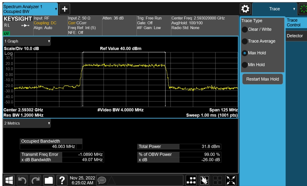
Plot 7-159. Occupied Bandwidth Plot (NR Band n41 - 50MHz \pi/2 BPSK - Full RB Switching - Ant B)
