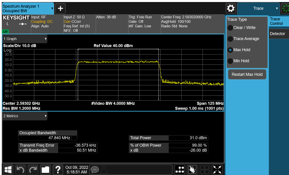
Plot 7-128. Occupied Bandwidth Plot (NR Band n41 - 50MHz 16-QAM - Full RB - Ant F)
