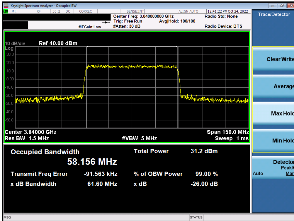
Plot 7-50. Occupied Bandwidth Plot (NR Band n77 - C-Band – 60MHz – QPSK - Full RB)
