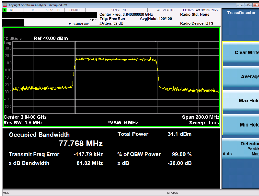
Plot 7-44. Occupied Bandwidth Plot (NR Band n77 - C-Band – 80MHz – QPSK - Full RB)
