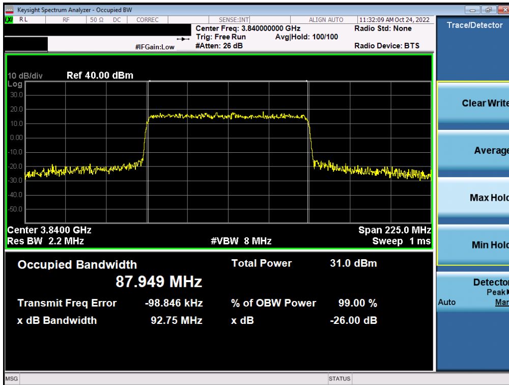
Plot 7-42. Occupied Bandwidth Plot (NR Band n77 - C-Band – 90MHz – 16-QAM - Full RB)
