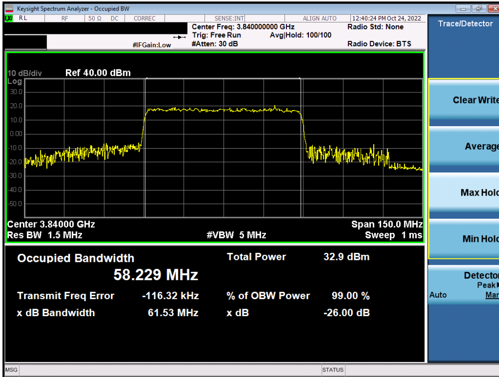
Plot 7-51. Occupied Bandwidth Plot (NR Band n77 - C-Band – 60MHz – 16-QAM - Full RB)
