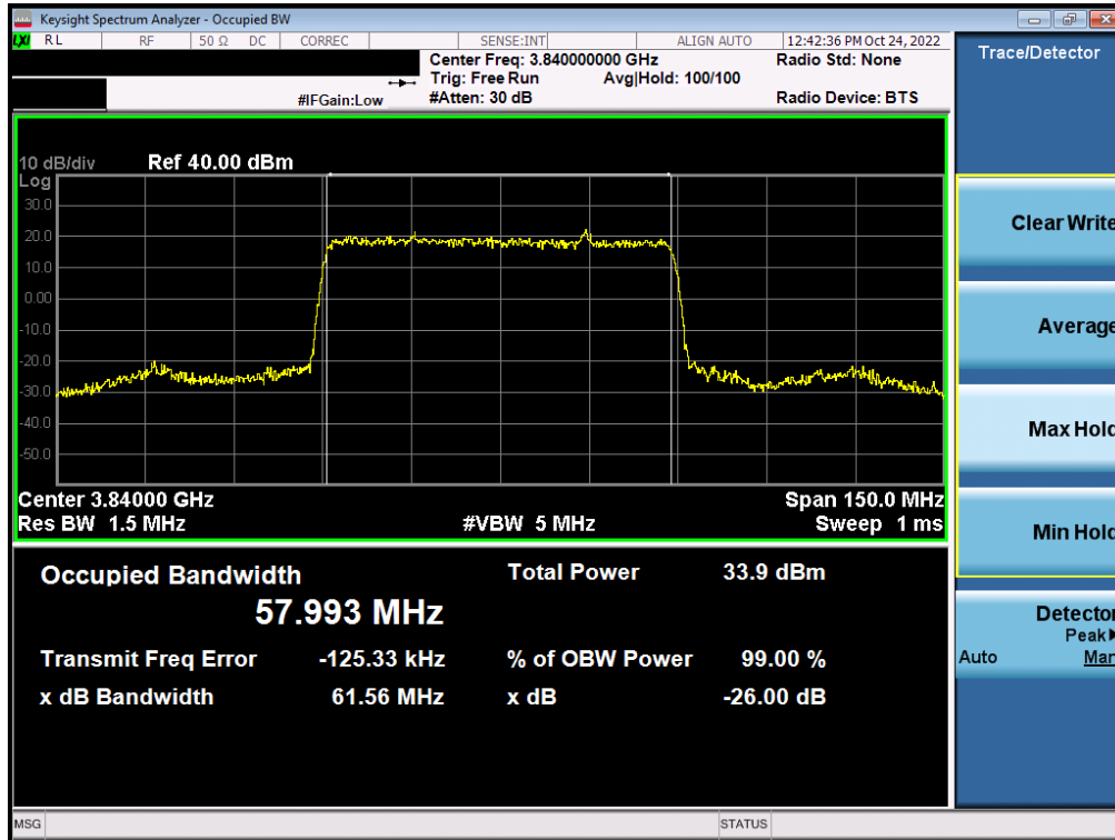
Plot 7-49. Occupied Bandwidth Plot (NR Band n77 - C-Band – 60MHz – \pi/2 BPSK - Full RB)
