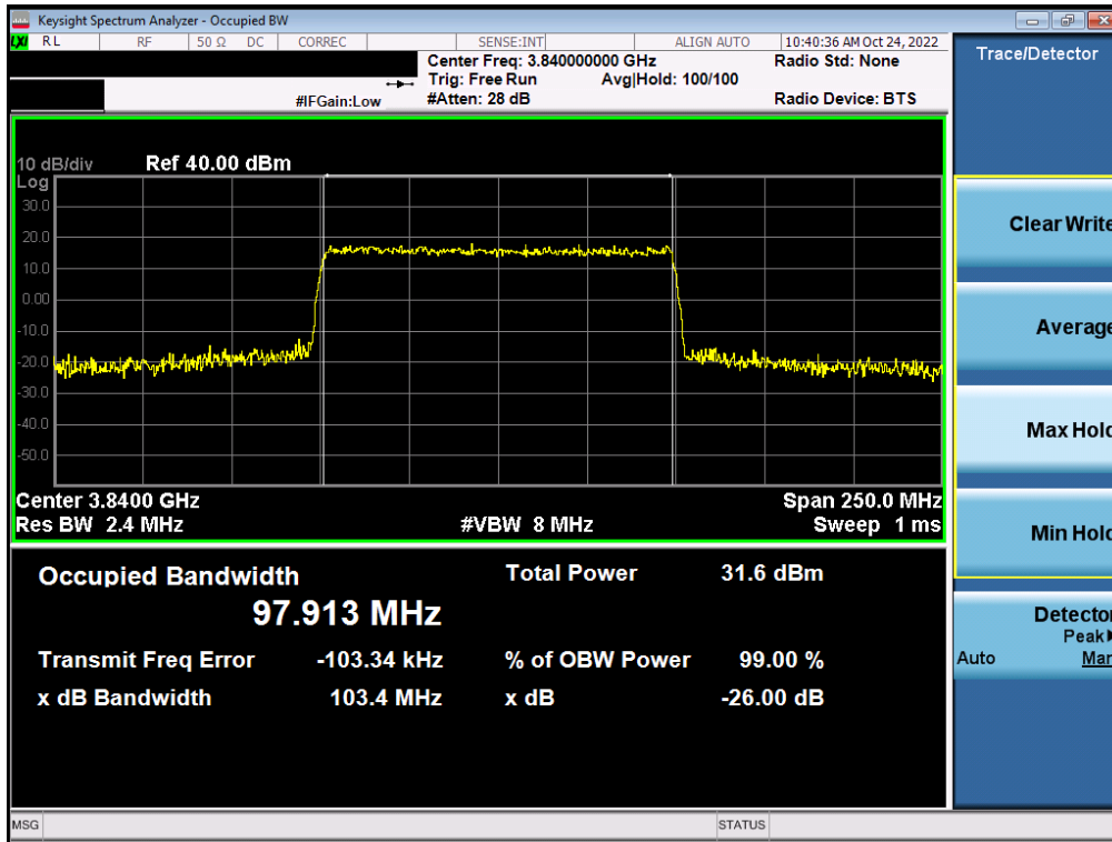
Plot 7-38. Occupied Bandwidth Plot (NR Band n77 - C-Band – 100MHz – QPSK - Full RB)
