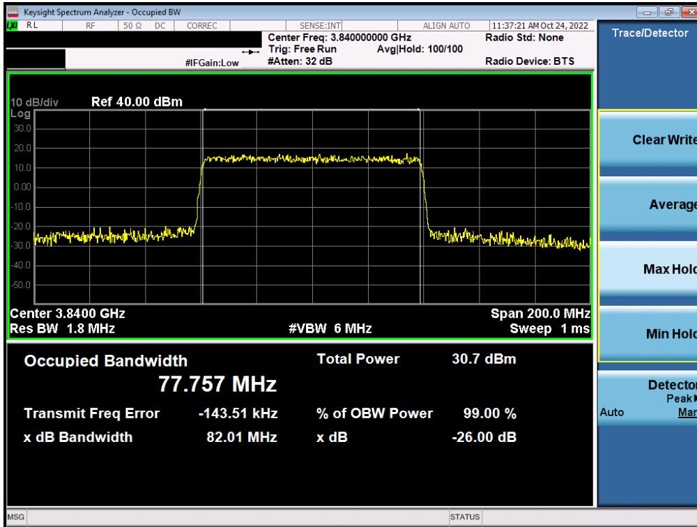
Plot 7-45. Occupied Bandwidth Plot (NR Band n77 - C-Band – 80MHz – 16-QAM - Full RB)
