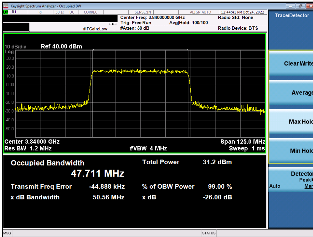
Plot 7-54. Occupied Bandwidth Plot (NR Band n77 - C-Band – 50MHz – 16-QAM - Full RB)
