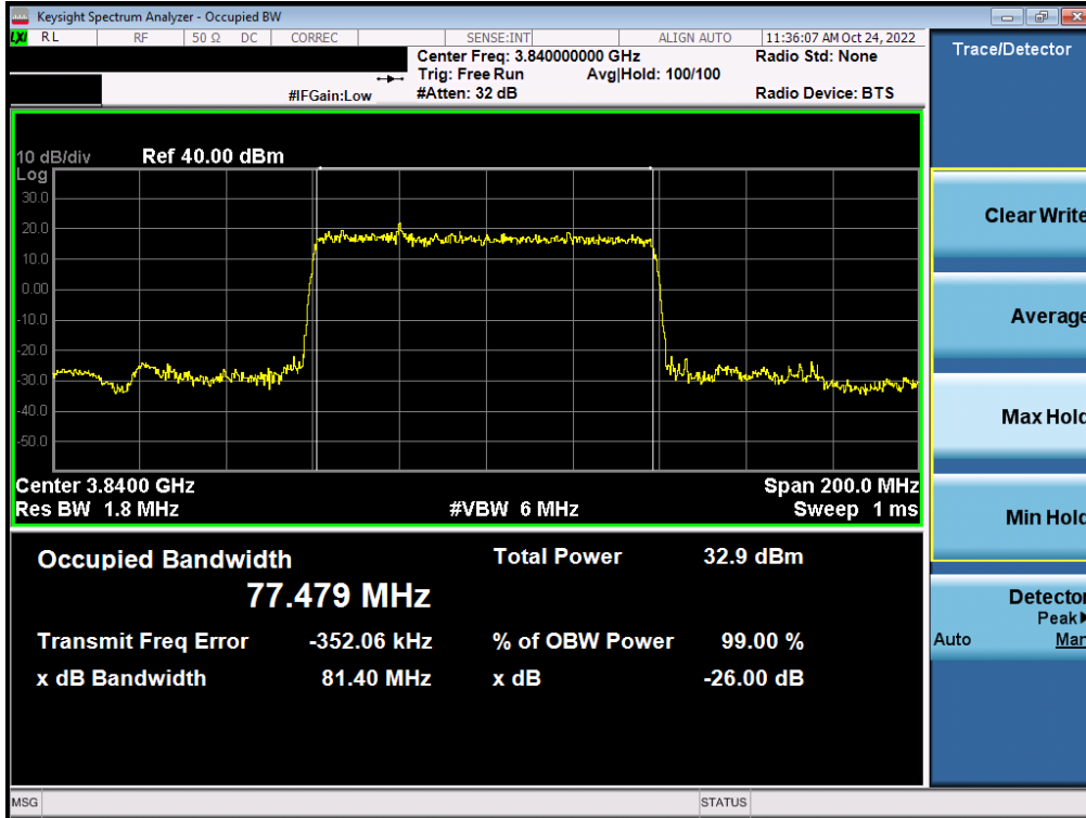
Plot 7-43. Occupied Bandwidth Plot (NR Band n77 - C-Band – 80MHz – \pi/2 BPSK - Full RB)
