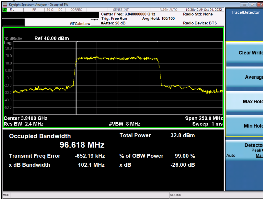
Plot 7-37. Occupied Bandwidth Plot (NR Band n77 - C-Band – 100MHz – \pi/2 BPSK - Full RB)
