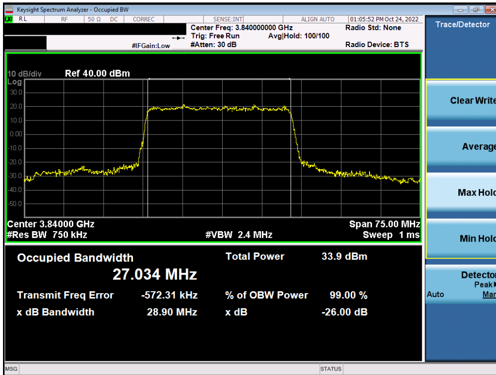
Plot 7-58. Occupied Bandwidth Plot (NR Band n77 - C-Band – 30MHz – \pi/2 BPSK - Full RB)
