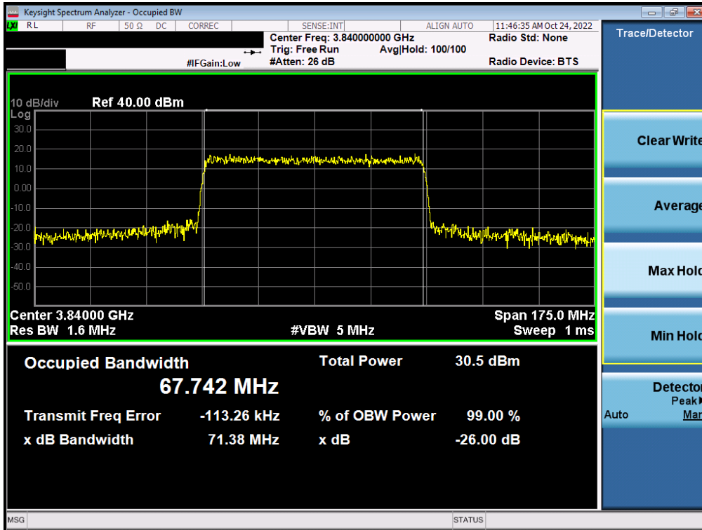
Plot 7-47. Occupied Bandwidth Plot (NR Band n77 - C-Band – 70MHz – QPSK - Full RB)
