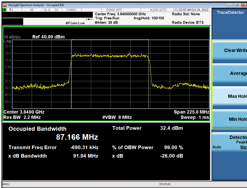
Plot 7-40. Occupied Bandwidth Plot (NR Band n77 - C-Band – 90MHz – \pi/2 BPSK - Full RB)
