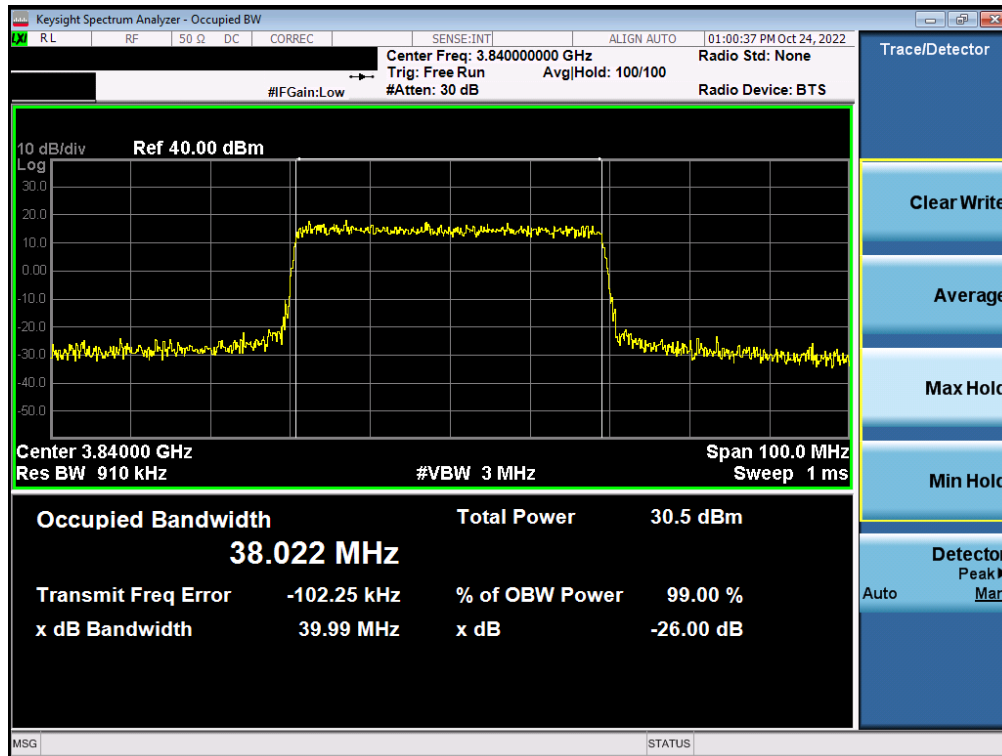
Plot 7-56. Occupied Bandwidth Plot (NR Band n77 - C-Band – 40MHz – QPSK - Full RB)
