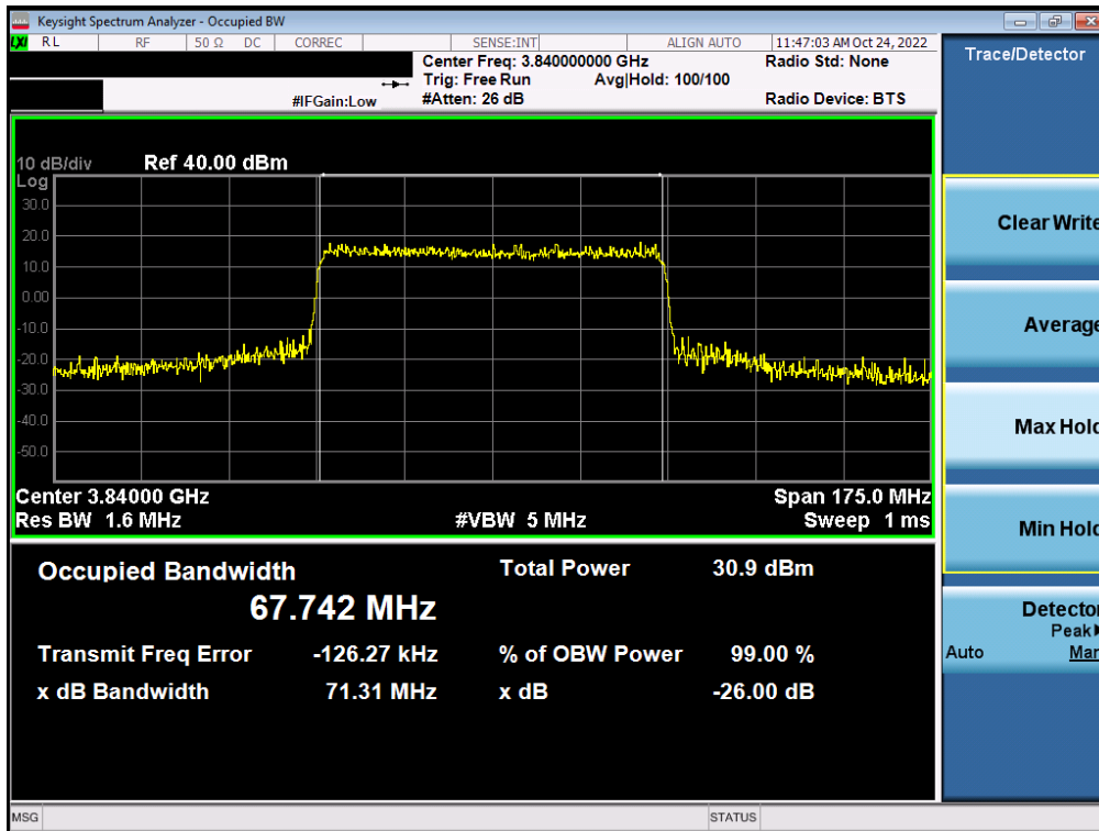
Plot 7-48. Occupied Bandwidth Plot (NR Band n77 - C-Band – 70MHz – 16-QAM - Full RB)
