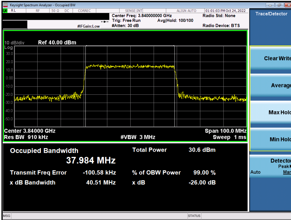
Plot 7-57. Occupied Bandwidth Plot (NR Band n77 - C-Band – 40MHz – 16-QAM - Full RB)
