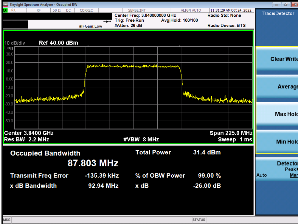
Plot 7-41. Occupied Bandwidth Plot (NR Band n77 - C-Band – 90MHz – QPSK - Full RB)
