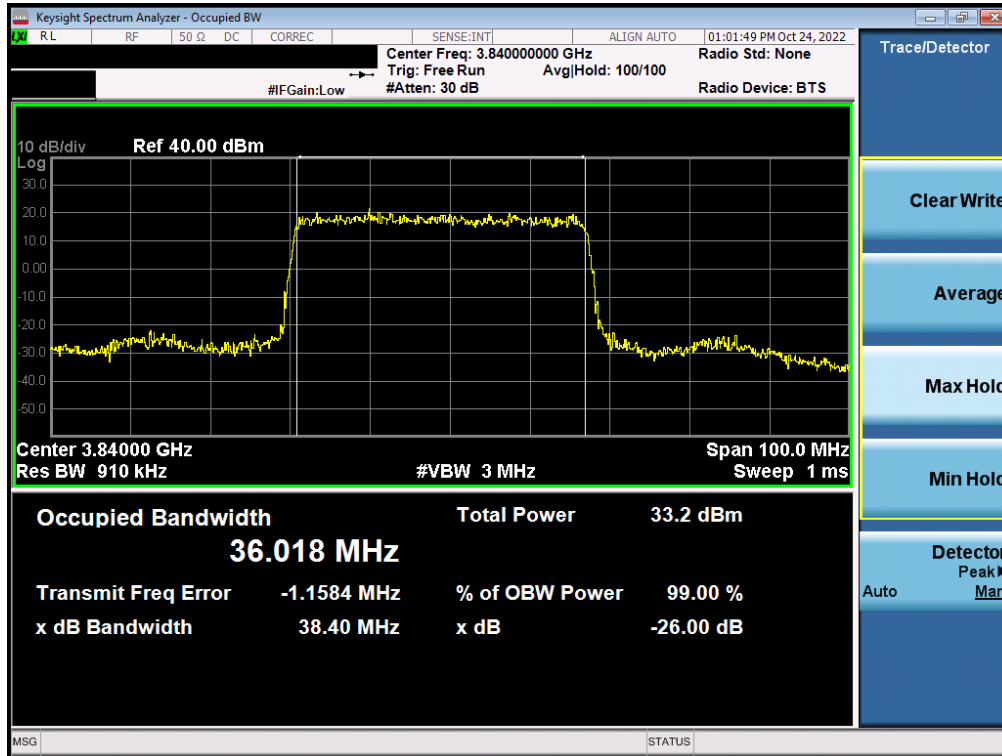
Plot 7-55. Occupied Bandwidth Plot (NR Band n77 - C-Band – 40MHz – \pi/2 BPSK - Full RB)
