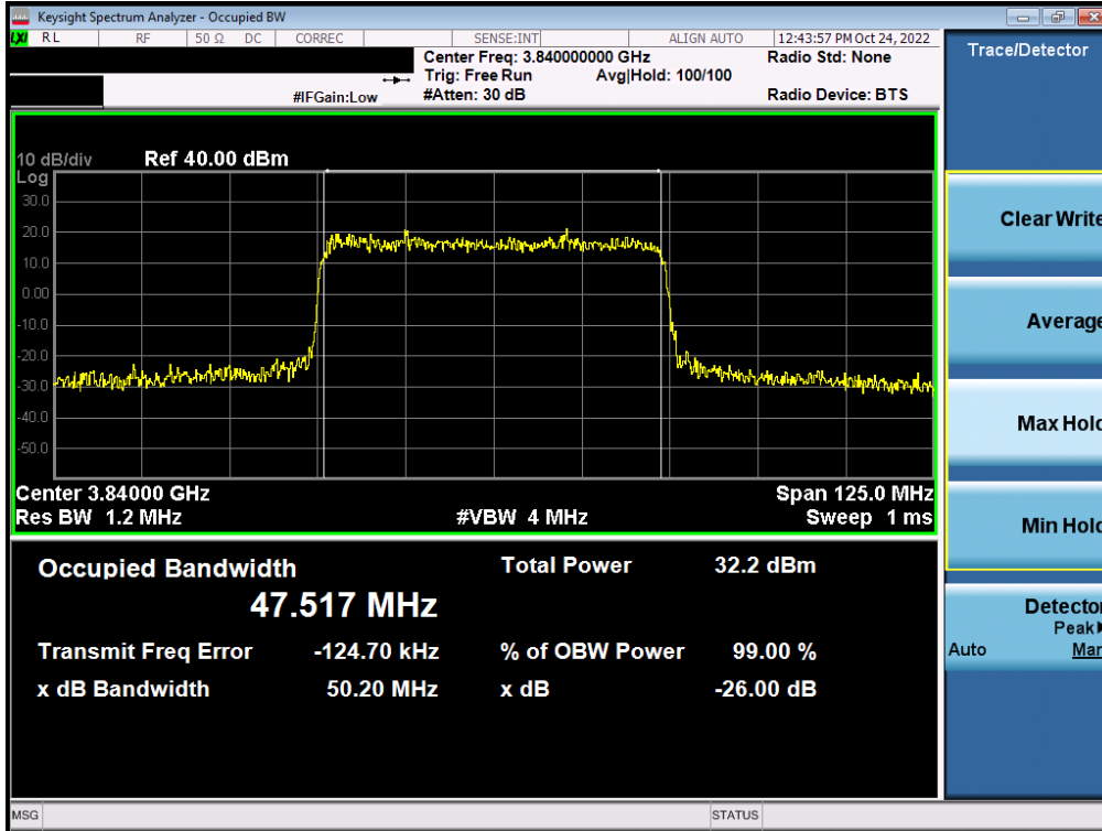
Plot 7-53. Occupied Bandwidth Plot (NR Band n77 - C-Band – 50MHz – QPSK - Full RB)
