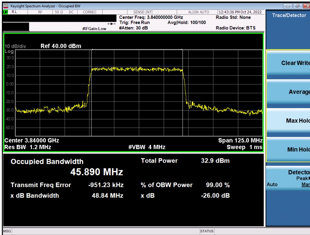
Plot 7-52. Occupied Bandwidth Plot (NR Band n77 - C-Band – 50MHz – \pi/2 BPSK - Full RB)
