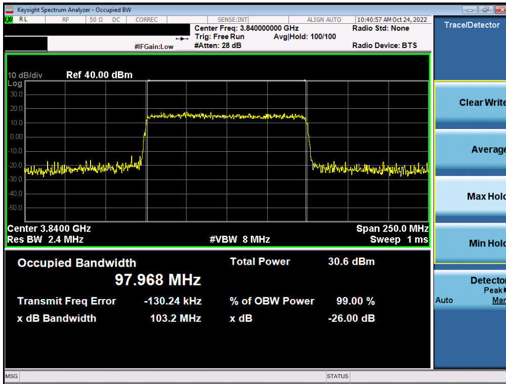
Plot 7-39. Occupied Bandwidth Plot (NR Band n77 - C-Band – 100MHz – 16-QAM - Full RB)
