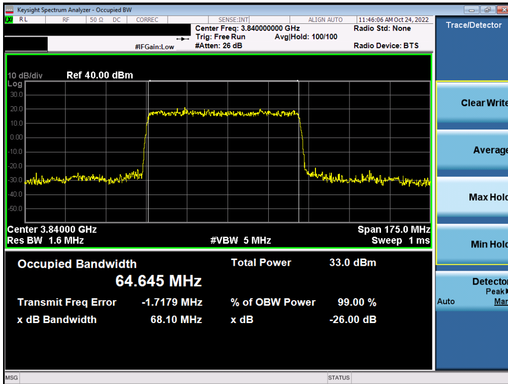
Plot 7-46. Occupied Bandwidth Plot (NR Band n77 - C-Band – 70MHz – \pi/2 BPSK - Full RB)
