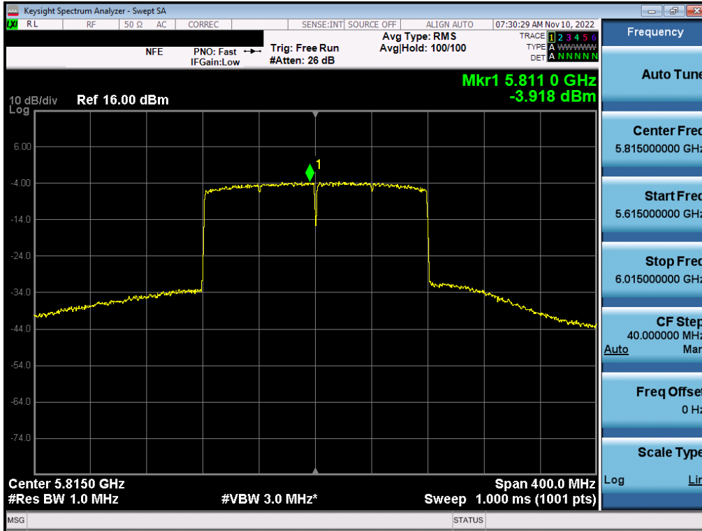
Plot 7-300. Power Spectral Density Plot MIMO ANT2 (160MHz(L) BW 802.11ax – Full Tones (UNII Band 3/4) – Ch. 163)
