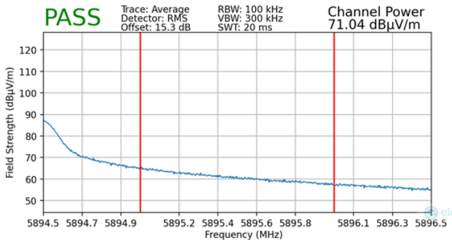
Plot 7-324. Radiated Upper Band Edge Plot MIMO (Average – UNII Band 4 – 106 Tones)
