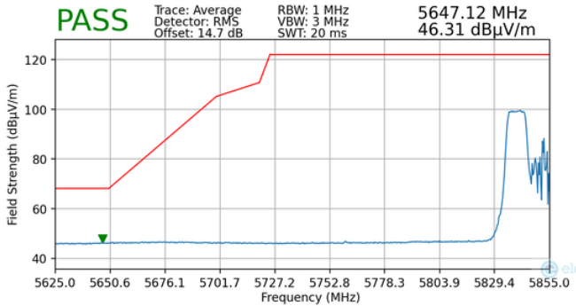
Plot 7-322. Radiated Lower Band Edge Plot MIMO (Average – UNII Band 4 – 106 Tones)
