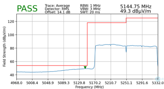
Plot 7-410. Radiated Lower Band Edge Plot MIMO (Average – UNII Band 1) with WCP
