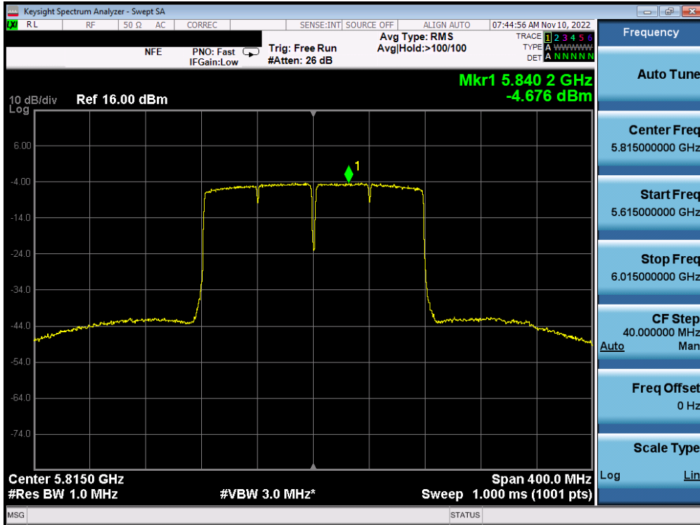
Plot 7-259. Power Spectral Density Plot MIMO ANT1 (160MHz BW 802.11ac (UNII Band 3/4) – Ch. 163)
