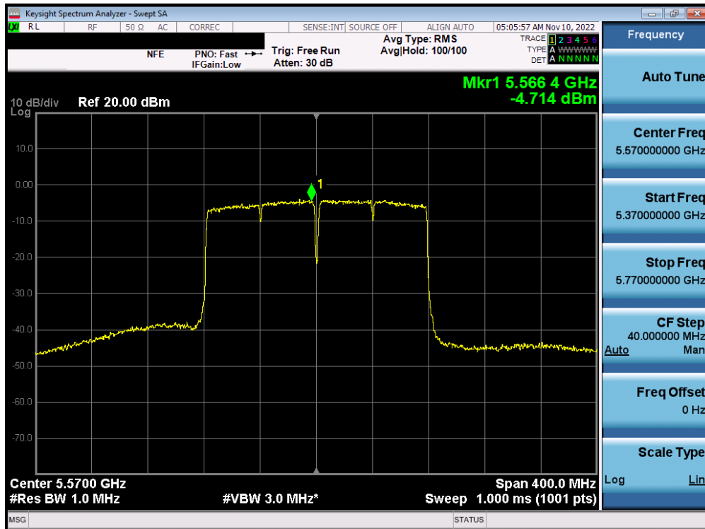
Plot 7-314. Power Spectral Density Plot MIMO ANT2 (160MHz BW 802.11ax (UNII Band 2C) – Ch. 114)
