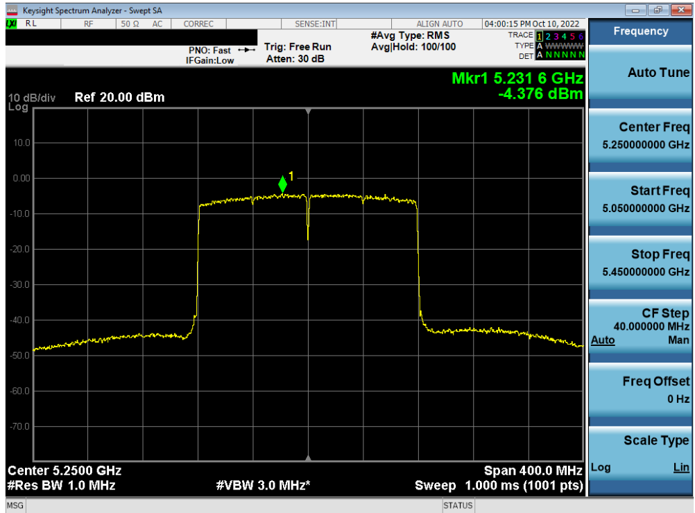
Plot 7-277. Power Spectral Density Plot MIMO ANT2 (160MHz BW 802.11ax (UNII Band 1/2A) – Ch. 50)
