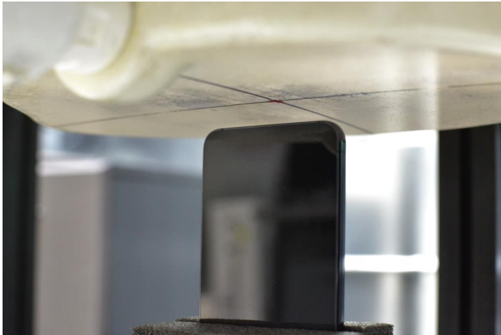
Test Setup Photo 12 – Body, Bottom Edge, 10 mm
