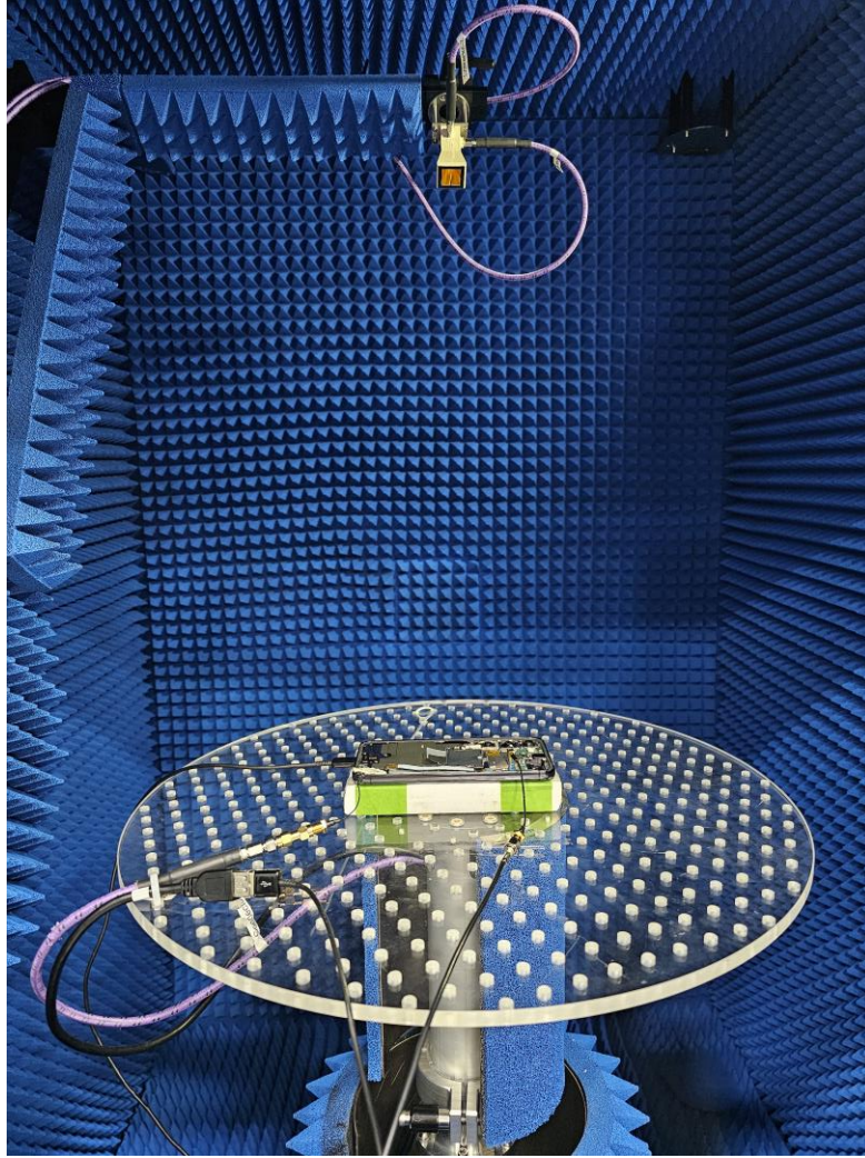
Test Setup Photo 8 – Radiated Power Test Setup (Figure 7-2)
