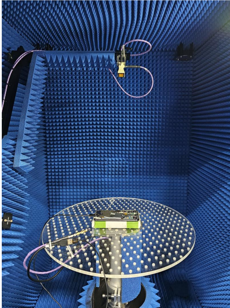
Test Setup Photo 7 – Radiated Power Test Setup (Figure 7-1)
