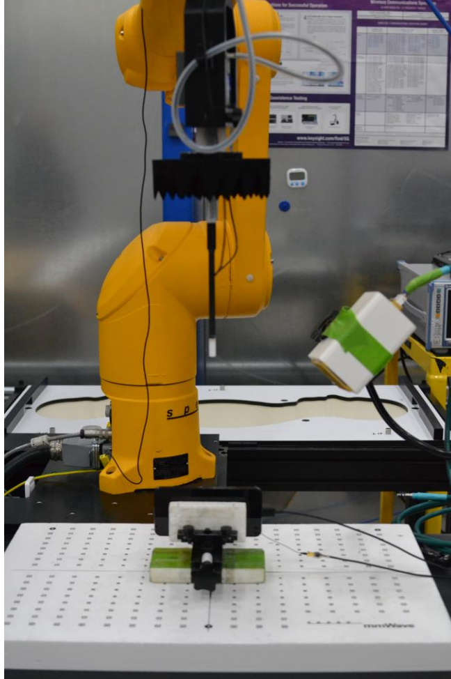
Test Setup Photo 9 – Power Density Test Setup (Figure 7-3)
