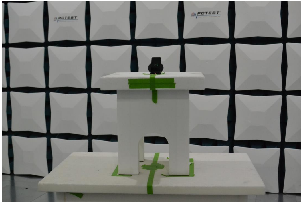
Figure 14. Test Setup – WPT Position – 1GHz-18GHz
