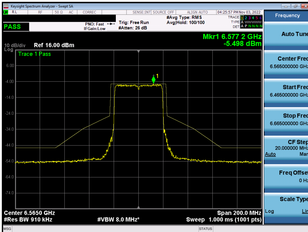
Plot 7-611. In-Band Emission Plot MIMO ANT2 (40MHz BW 802.11ax (Full Tone) (UNII Band 7) – Ch. 123) – LPI/SP
