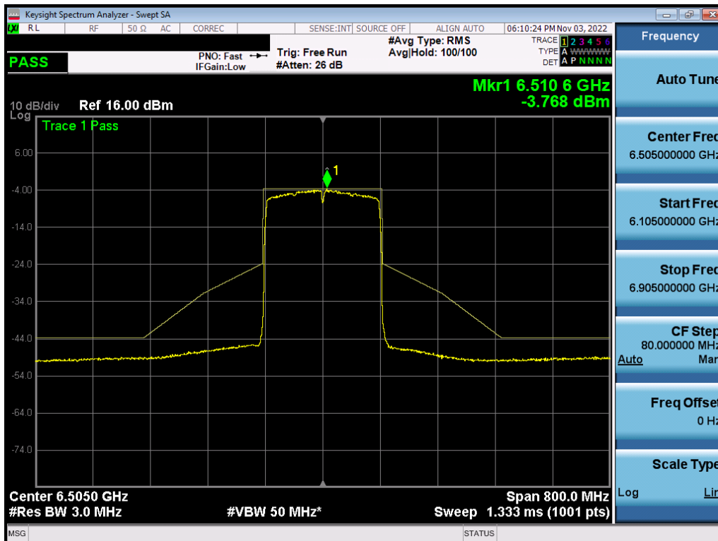
Plot 7-607. In-Band Emission Plot MIMO ANT2 (160MHz BW 802.11ax (Full Tone) (UNII Band 6) – Ch. 111) – LPI
