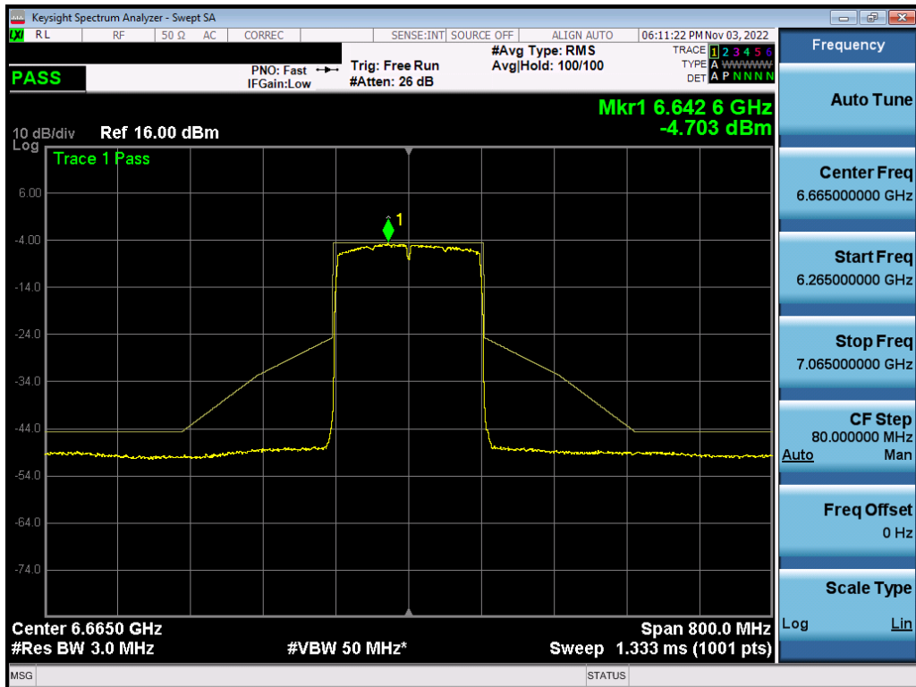
Plot 7-617. In-Band Emission Plot MIMO ANT2 (160MHz BW 802.11ax (Full Tone) (UNII Band 7) – Ch. 143) – LPI/SP
