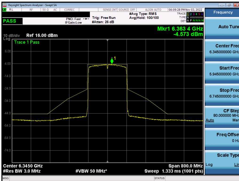
Plot 7-599. In-Band Emission Plot MIMO ANT2 (160MHz BW 802.11ax (Full Tone) (UNII Band 5) – Ch. 79) – LPI/SP
