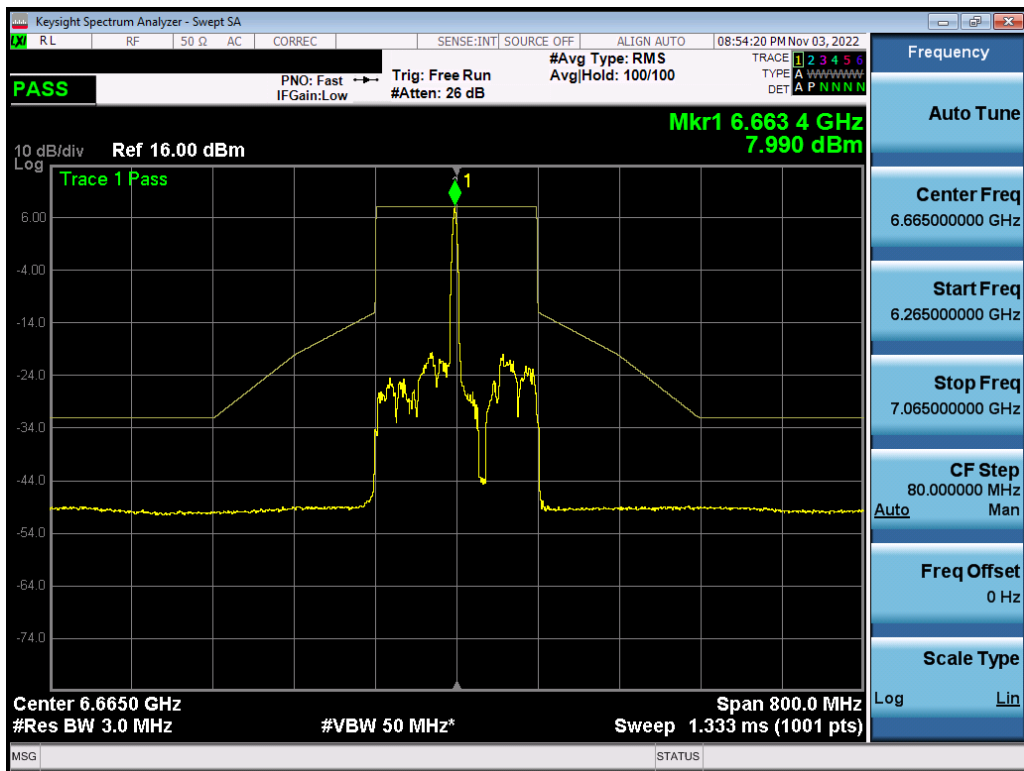
Plot 7-586. In-Band Emission Plot MIMO ANT2 (160MHz BW 802.11ax (26 Tones) (UNII Band 7) – Ch. 143) – SP
