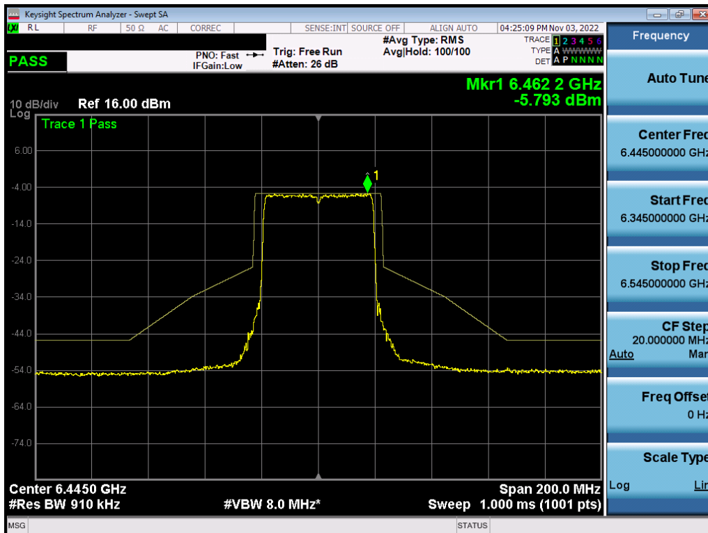
Plot 7-603. In-Band Emission Plot MIMO ANT2 (40MHz BW 802.11ax (Full Tone) (UNII Band 6) – Ch. 99) – LPI
