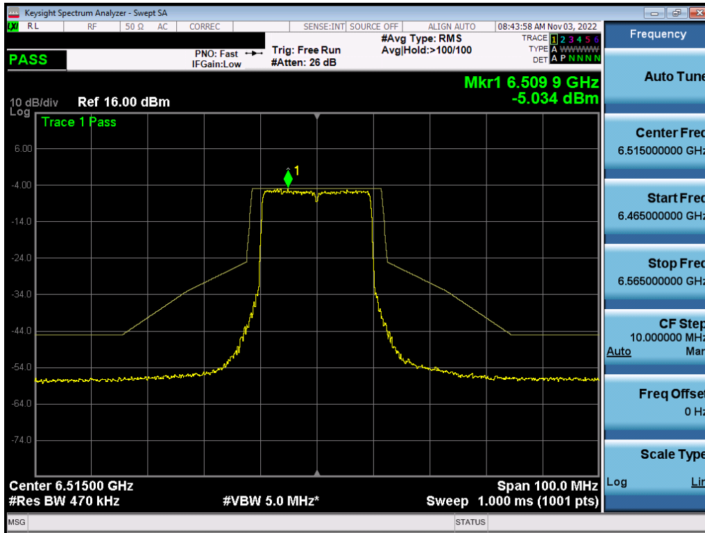
Plot 7-602. In-Band Emission Plot MIMO ANT2 (20MHz BW 802.11ax (Full Tone) (UNII Band 6) – Ch. 113) – LPI
