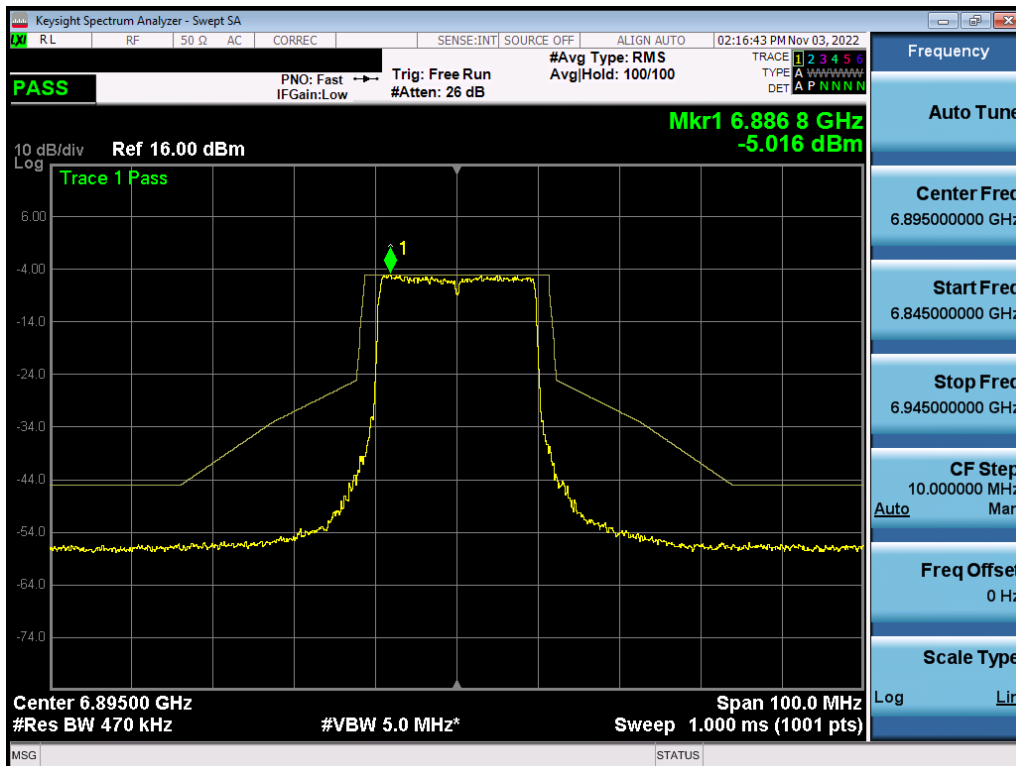
Plot 7-619. In-Band Emission Plot MIMO ANT2 (20MHz BW 802.11ax (Full Tone) (UNII Band 8) – Ch. 189) – LPI
