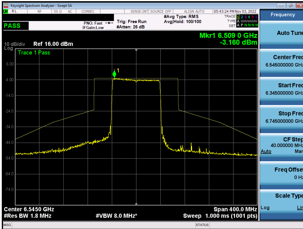
Plot 7-614. In-Band Emission Plot MIMO ANT2 (80MHz BW 802.11ax (Full Tone) (UNII Band 7) – Ch. 119) – LPI/SP
