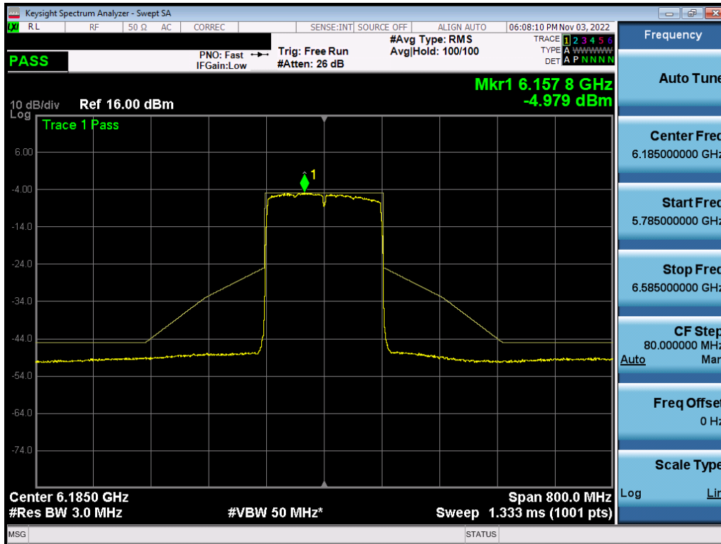
Plot 7-598. In-Band Emission Plot MIMO ANT2 160MHz BW 802.11ax (Full Tone) (UNII Band 5) – Ch. 47) – LPI/SP
