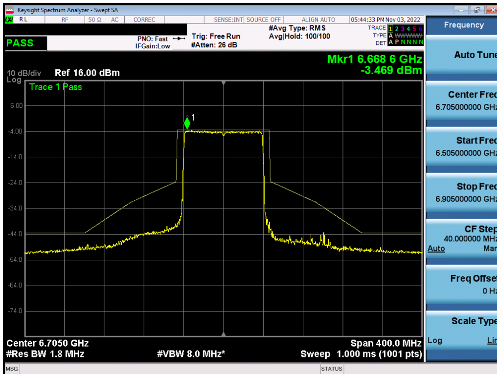
Plot 7-615. In-Band Emission Plot MIMO ANT2 (80MHz BW 802.11ax (Full Tone) (UNII Band 7) – Ch. 151) – LPI/SP
