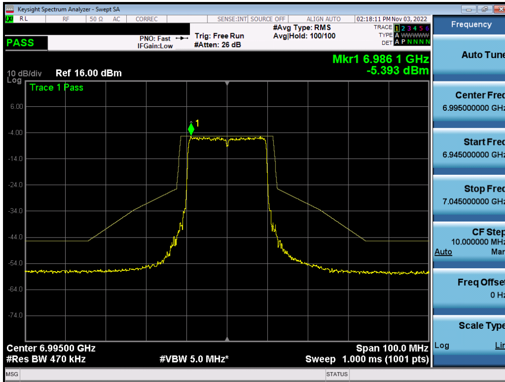
Plot 7-620. In-Band Emission Plot MIMO ANT2 (20MHz BW 802.11ax (Full Tone) (UNII Band 8) – Ch. 209) – LPI
