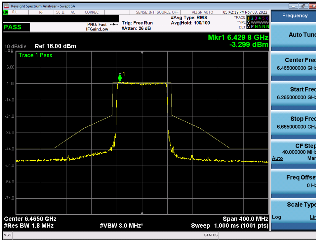
Plot 7-606. In-Band Emission Plot MIMO ANT2 (80MHz BW 802.11ax (Full Tone) (UNII Band 6) – Ch. 103) – LPI
