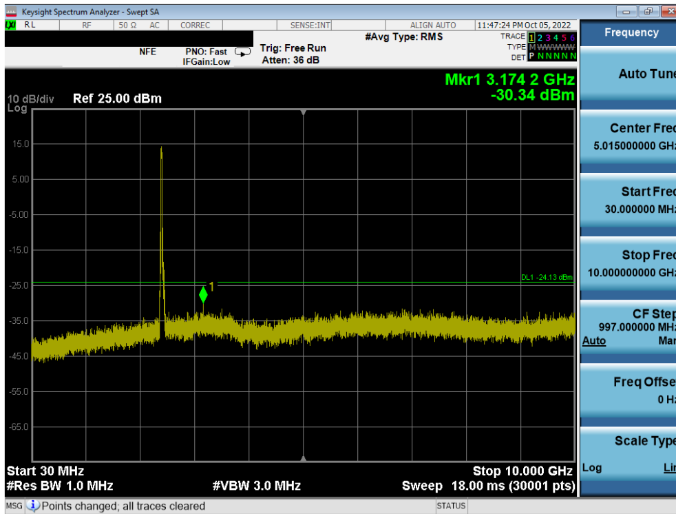
Plot 7-76. Conducted Spurious Plot MIMO ANT1 (802.11ax OFDMA – 242 Tones – Ch. 1)
