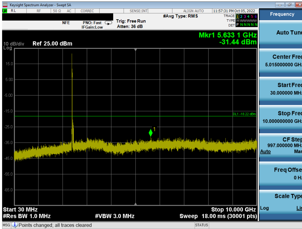
Plot 7-58. Conducted Spurious Plot SISO ANT2 (802.11ax OFDMA – 26 Tones – Ch. 1)
