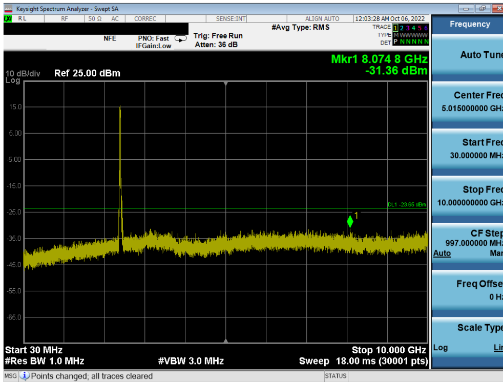
Plot 7-64. Conducted Spurious Plot SISO ANT2 (802.11ax OFDMA – 242 Tones – Ch. 1)
