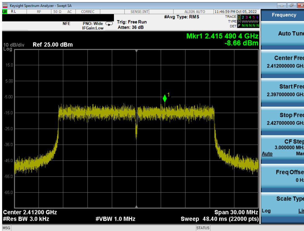
Plot 7-28. Power Spectral Density Plot MIMO ANT1 (802.11ax OFDMA – 242 Tones – Ch. 1)
