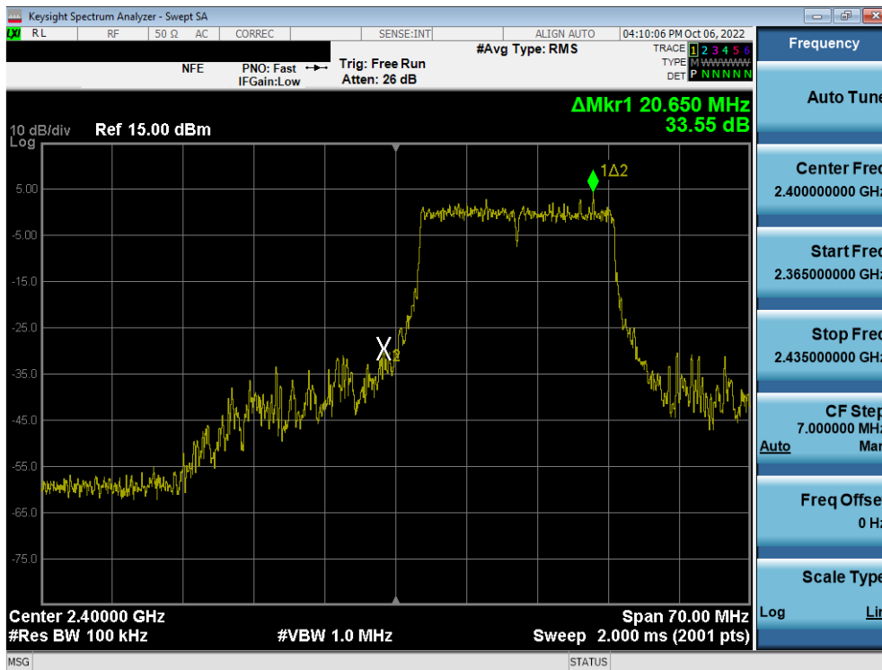
Plot 7-39. Band Edge Plot SISO ANT2 (802.11ax OFDMA – 242 Tones – Ch. 1)
