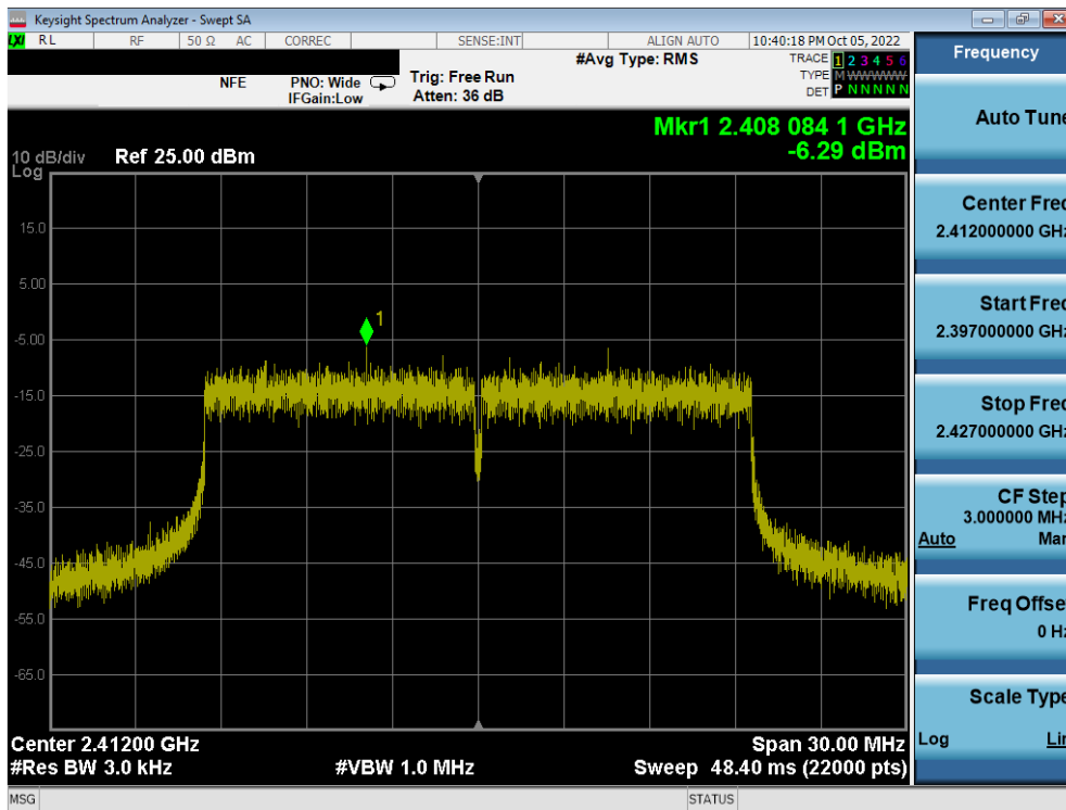
Plot 7-34. Power Spectral Density Plot MIMO ANT2 (802.11ax OFDMA – 242 Tones – Ch. 1)
