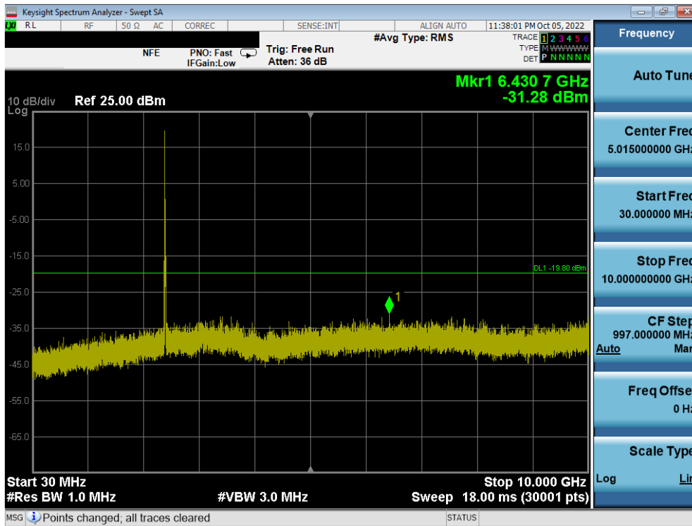
Plot 7-70. Conducted Spurious Plot MIMO ANT1 (802.11ax OFDMA – 26 Tones – Ch. 1)
