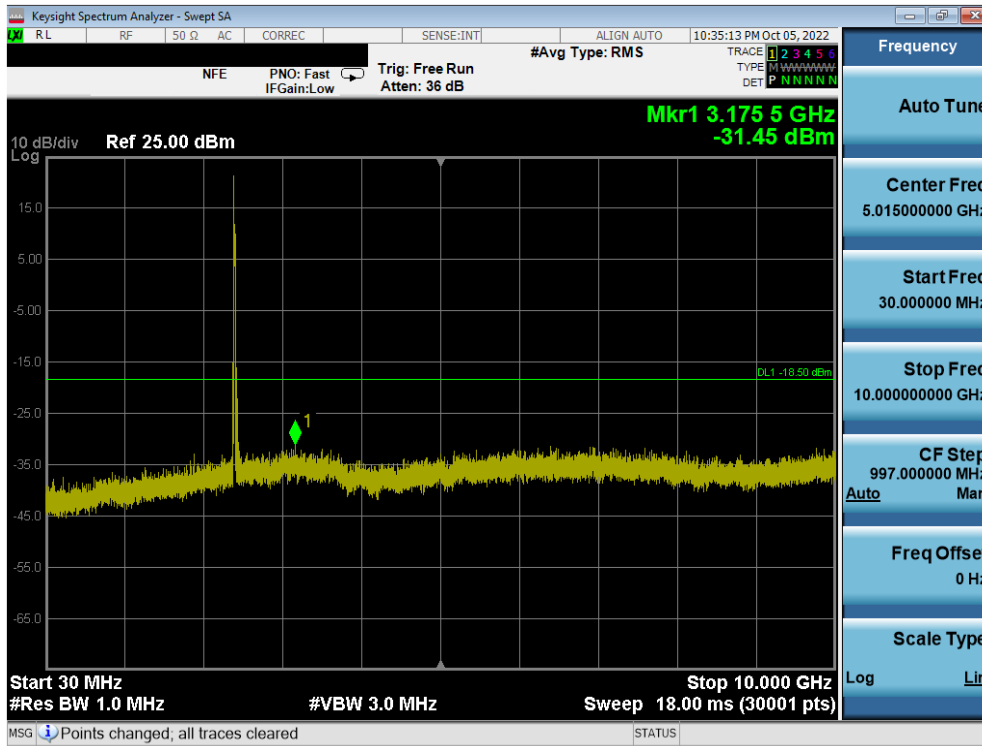
Plot 7-82. Conducted Spurious Plot MIMO ANT2 (802.11ax OFDMA – 26 Tones – Ch. 1)
