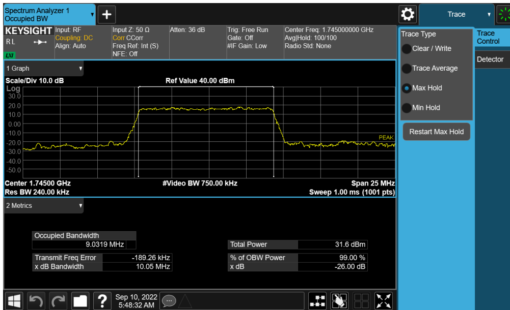
Plot 7-70. Occupied Bandwidth Plot (NR Band n66 - 10.0MHz DFT's BPSK - Full RB – Ant A)
