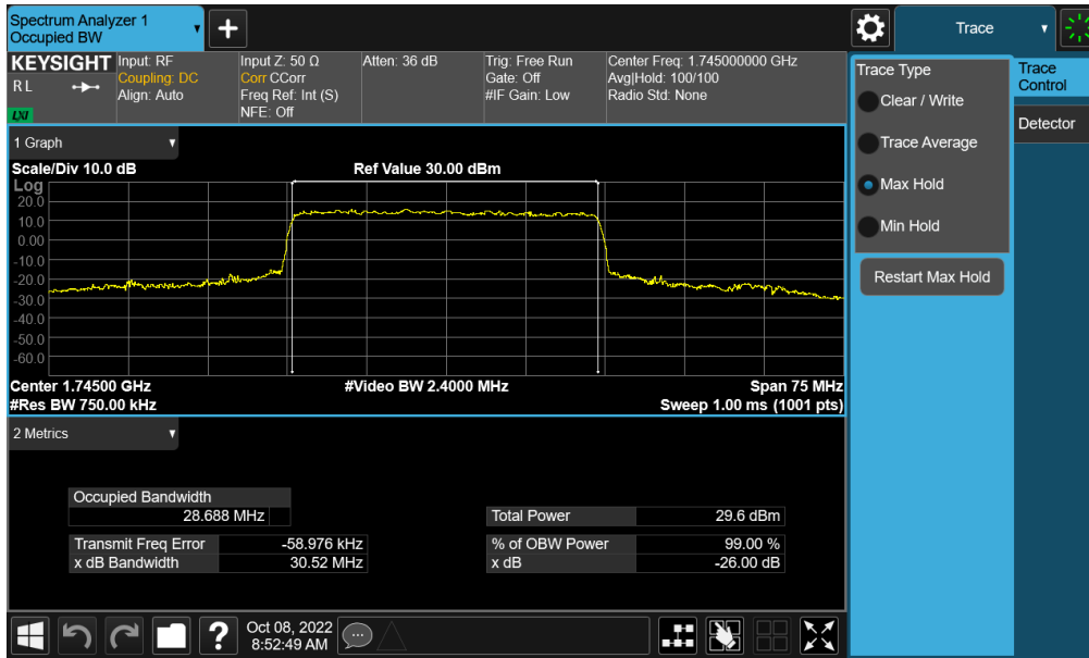
Plot 7-92. Occupied Bandwidth Plot (NR Band n66 - 30.0MHz CP-OFDM QPSK - Full RB – Ant F)
