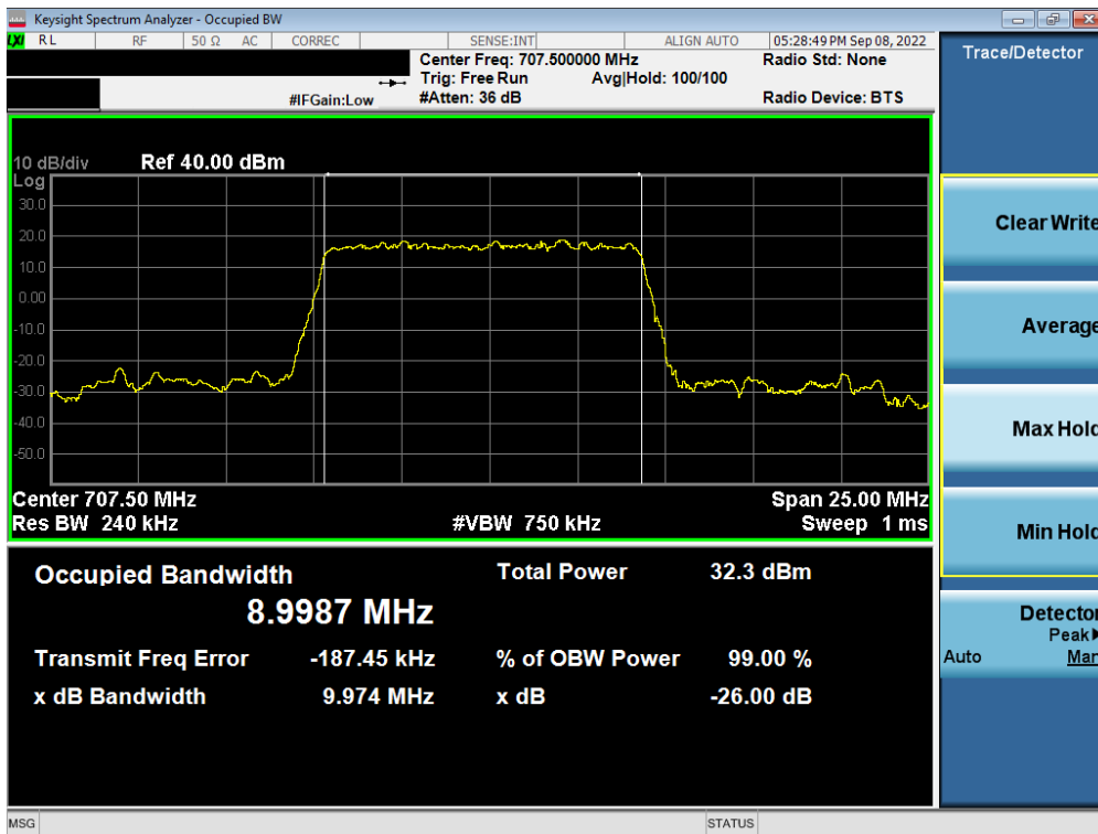
Plot 7-36. Occupied Bandwidth Plot (NR Band n12 - 10MHz DFT's BPSK - Full RB – Ant A)
