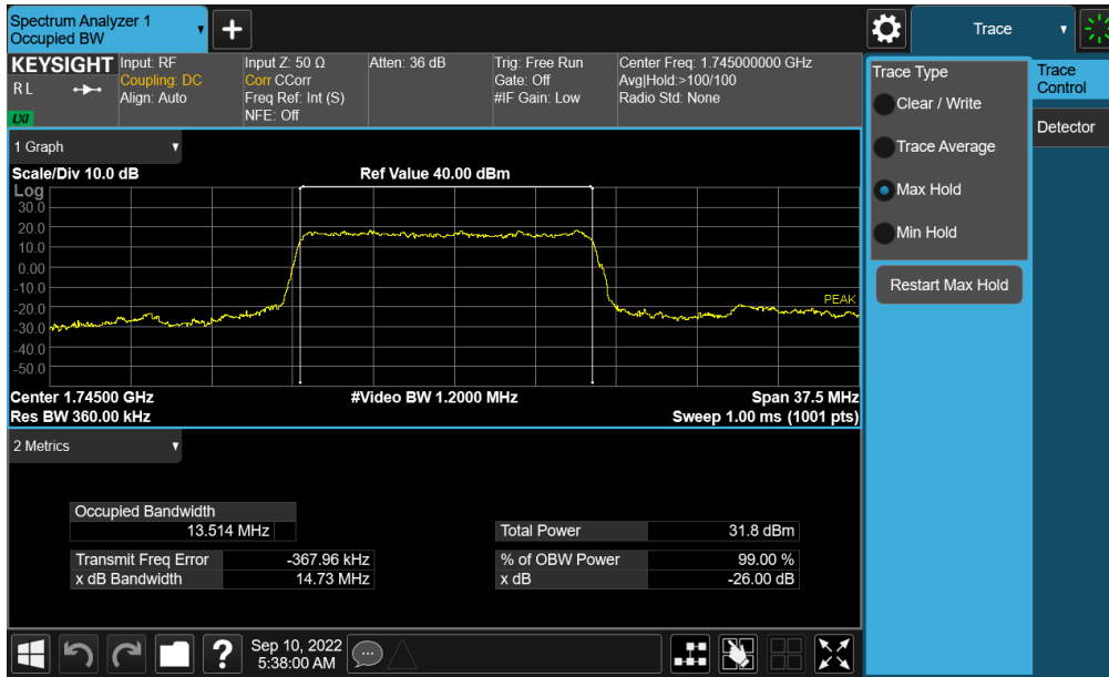
Plot 7-67. Occupied Bandwidth Plot (NR Band n66 - 15.0MHz DFT's BPSK - Full RB – Ant A)
