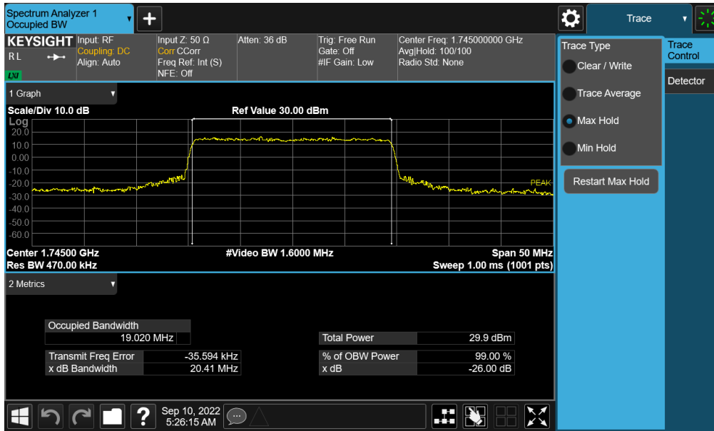
Plot 7-65. Occupied Bandwidth Plot (NR Band n66 - 20.0MHz CP-OFDM QPSK - Full RB – Ant A)
