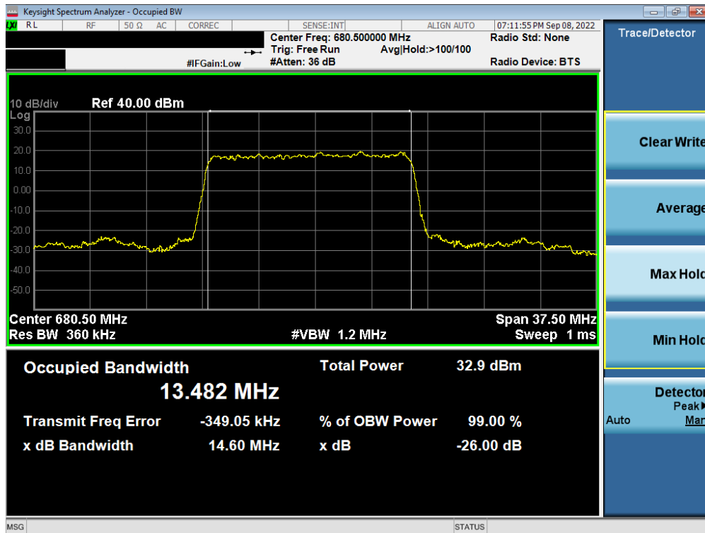
Plot 7-24. Occupied Bandwidth Plot (NR Band n71 - 15MHz DFT's BPSK - Full RB – Ant A)
