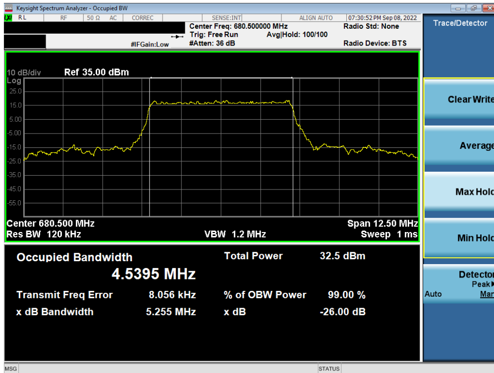
Plot 7-30. Occupied Bandwidth Plot (NR Band n71 - 5MHz DFT's BPSK - Full RB – Ant A)
