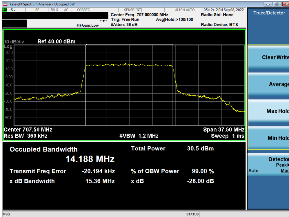
Plot 7-34. Occupied Bandwidth Plot (NR Band n12 - 15MHz CP-OFDM QPSK - Full RB – Ant A)
