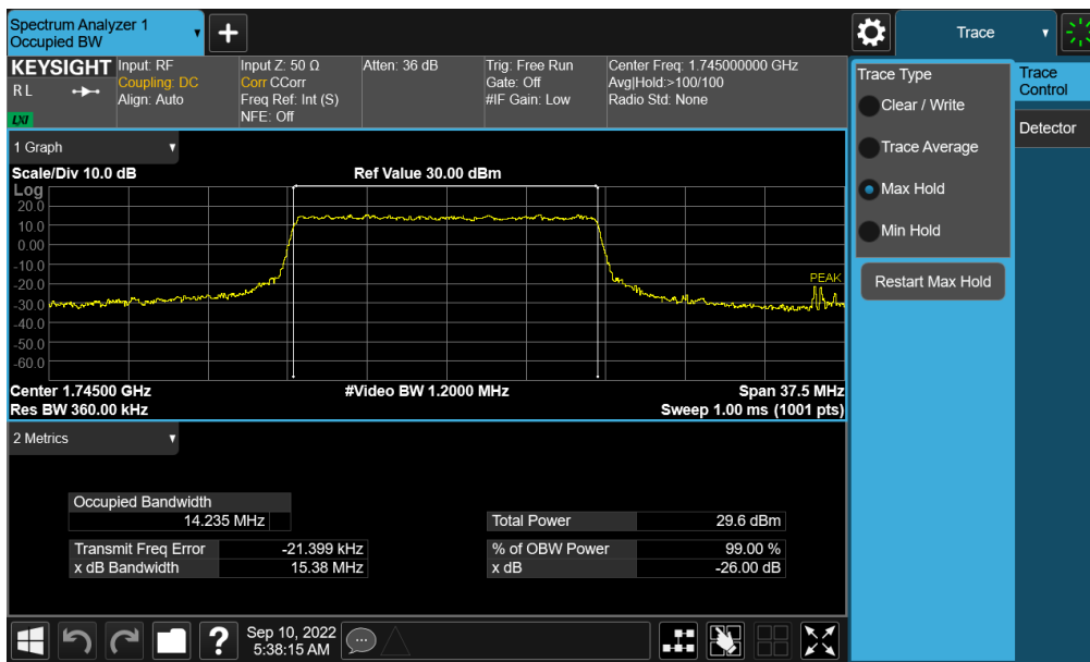
Plot 7-68. Occupied Bandwidth Plot (NR Band n66 - 15.0MHz CP-OFDM QPSK - Full RB – Ant A)
