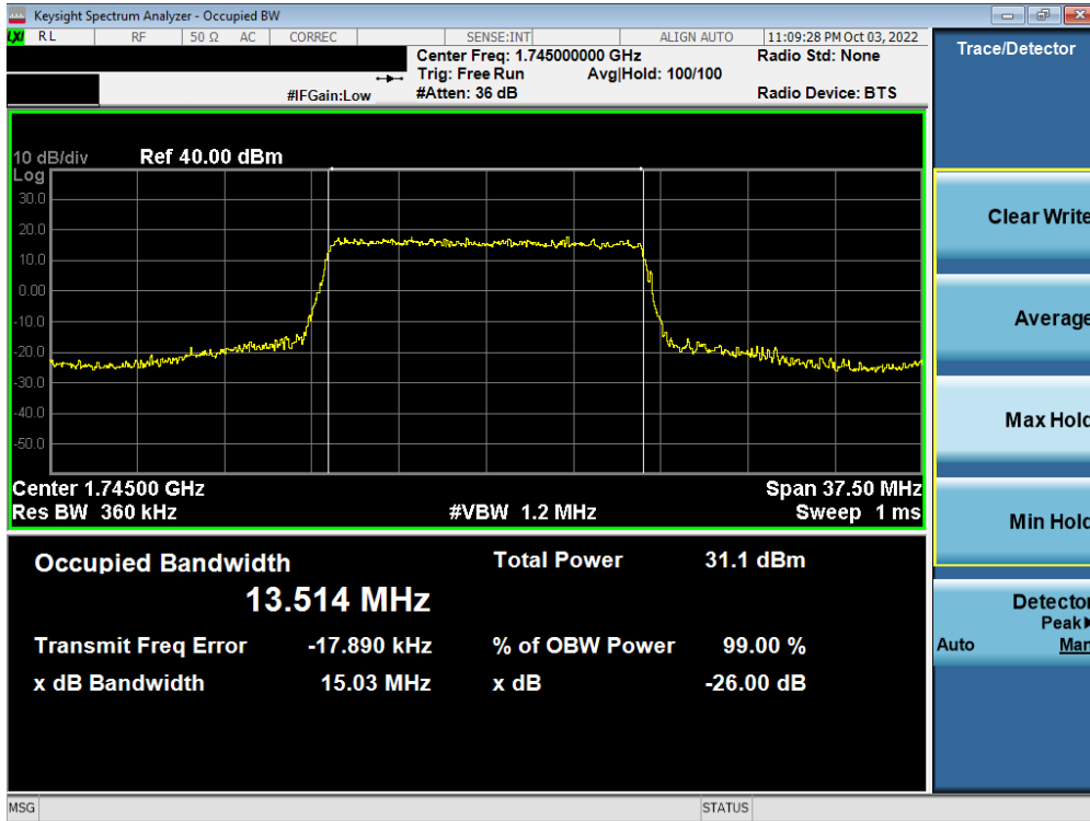
Plot 7-78. Occupied Bandwidth Plot (LTE Band 66/4 - 15MHz QPSK - Full RB - Ant F)
