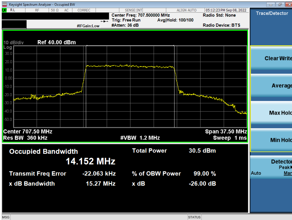
Plot 7-35. Occupied Bandwidth Plot (NR Band n12 - 15MHz CP-OFDM 16-QAM - Full RB – Ant A)
