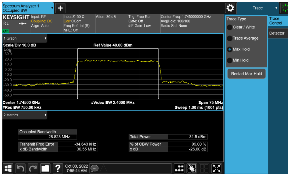
Plot 7-91. Occupied Bandwidth Plot (NR Band n66 - 30.0MHz DFT's BPSK - Full RB – Ant F)
