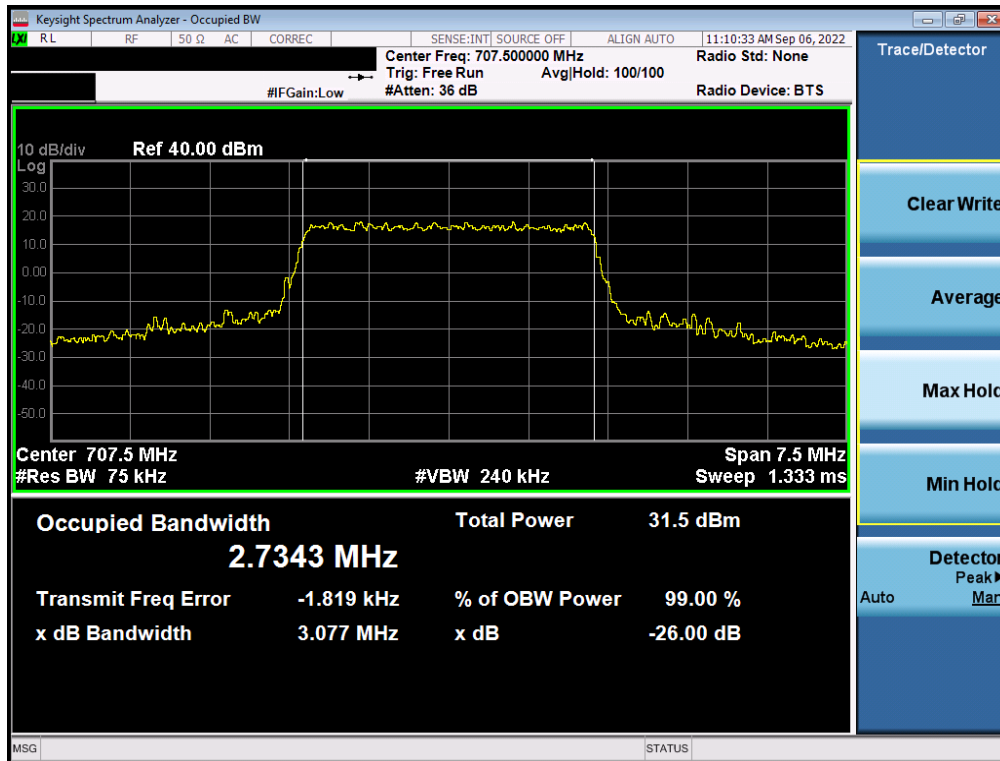
Plot 7-14. Occupied Bandwidth Plot (LTE Band 12 - 3MHz 16-QAM - Full RB Configuration)
