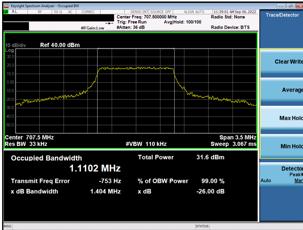
Plot 7-16. Occupied Bandwidth Plot (LTE Band 12 – 1.4MHz 16-QAM - Full RB Configuration)
