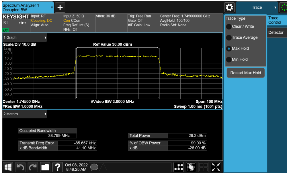
Plot 7-90. Occupied Bandwidth Plot (NR Band n66 - 40.0MHz CP-OFDM 16QAM - Full RB – Ant F)
