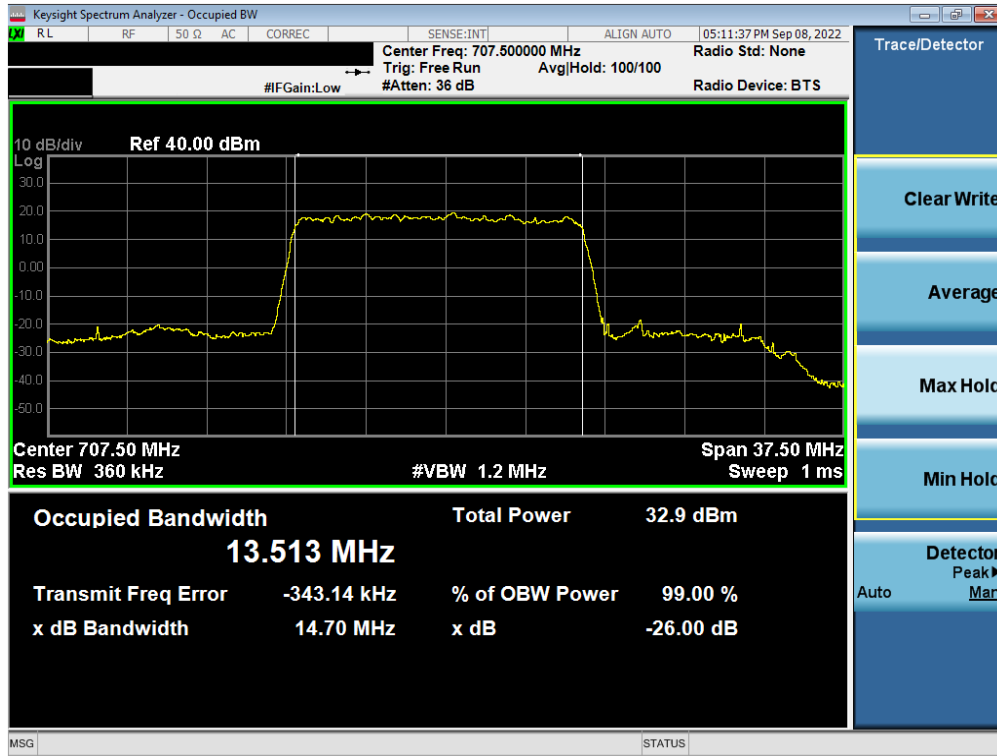
Plot 7-33. Occupied Bandwidth Plot (NR Band n12 - 15MHz DFT's BPSK - Full RB – Ant A)
