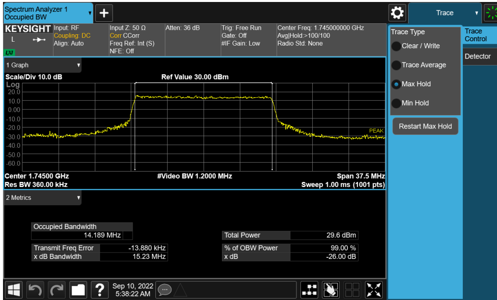
Plot 7-69. Occupied Bandwidth Plot (NR Band n66 - 15.0MHz CP-OFDM 16QAM - Full RB – Ant A)
