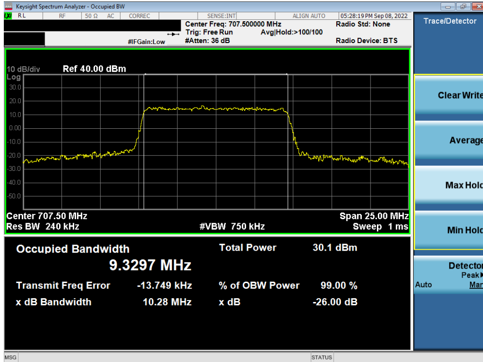
Plot 7-37. Occupied Bandwidth Plot (NR Band n12 - 10MHz CP-OFDM QPSK - Full RB – Ant A)
