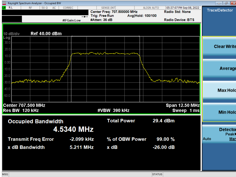
Plot 7-41. Occupied Bandwidth Plot (NR Band n12 - 5MHz CP-OFDM 16-QAM - Full RB – Ant A)
