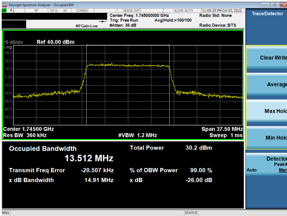
Plot 7-79. Occupied Bandwidth Plot (LTE Band 66/4 - 15MHz 16-QAM - Full RB - Ant F)
