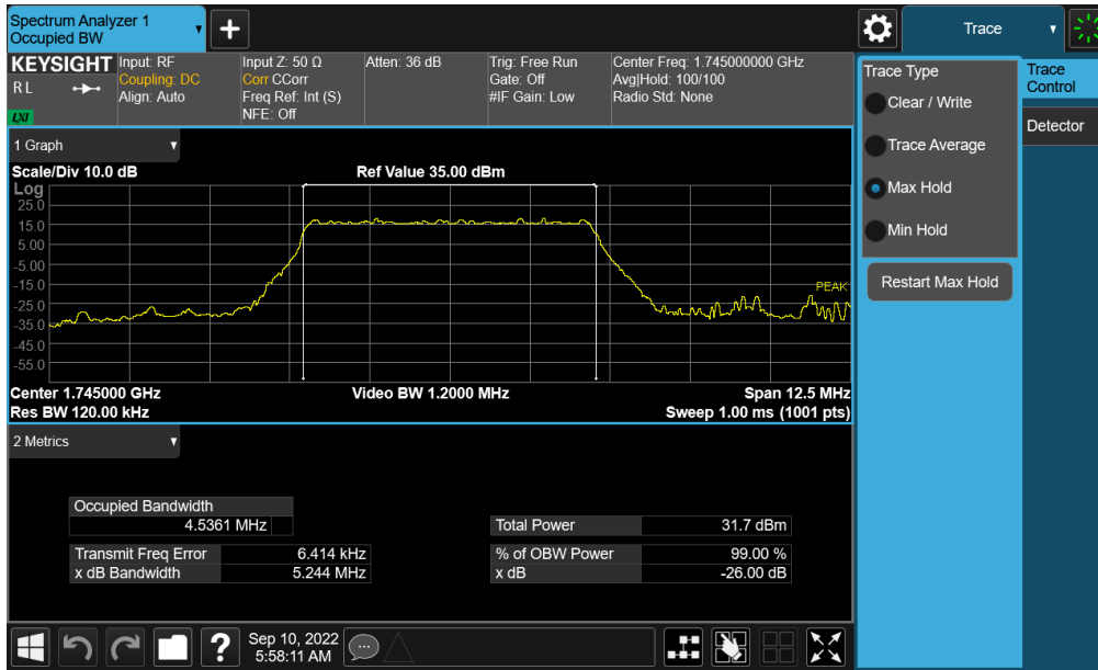
Plot 7-73. Occupied Bandwidth Plot (NR Band n66 - 5.0MHz DFT's BPSK - Full RB – Ant A)
