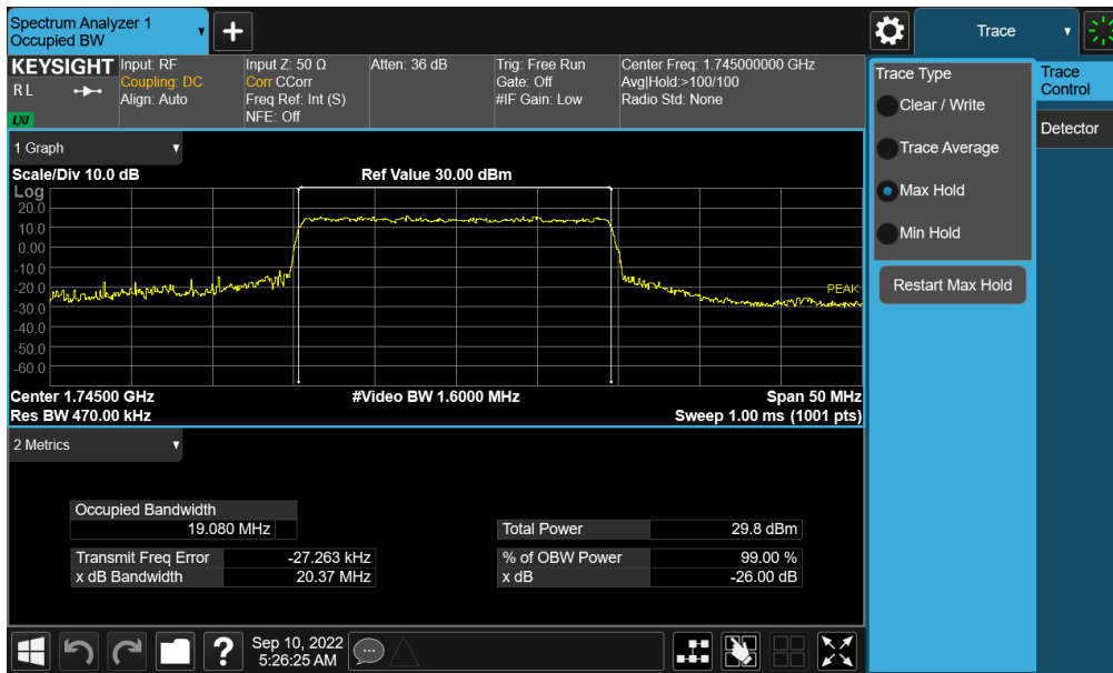
Plot 7-66. Occupied Bandwidth Plot (NR Band n66 - 20.0MHz CP-OFDM 16QAM - Full RB – Ant A)
