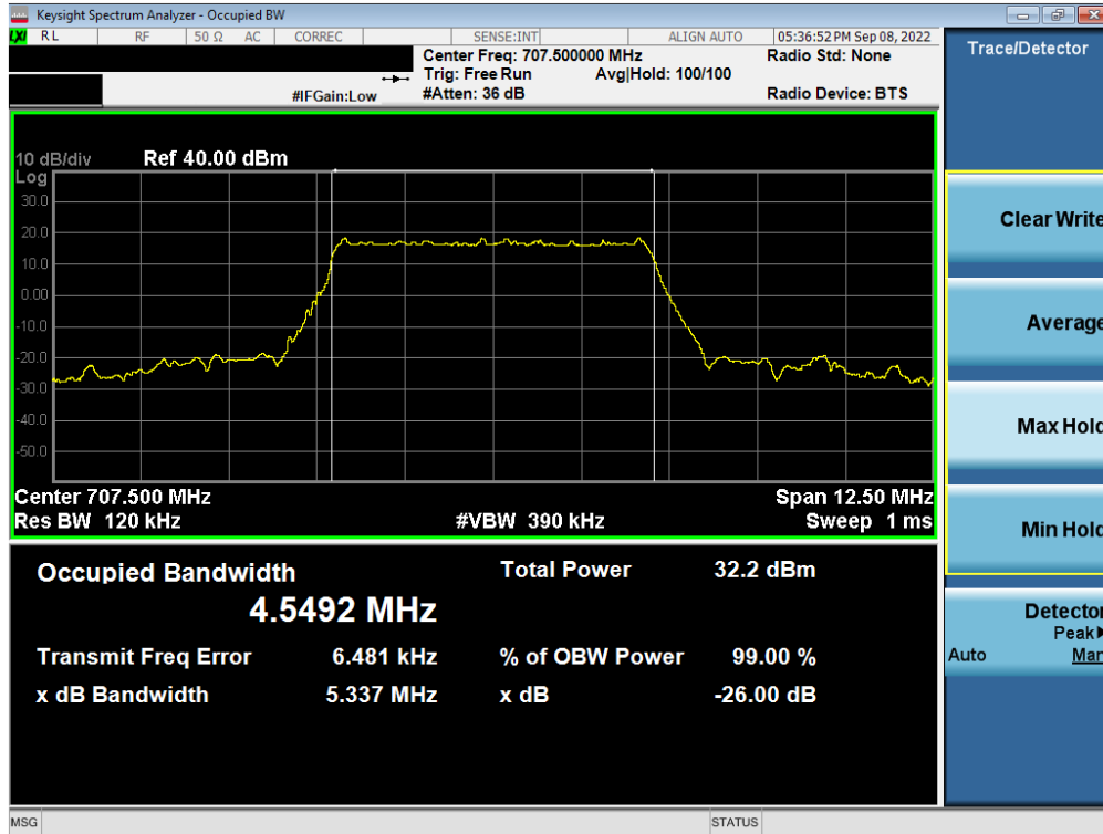
Plot 7-39. Occupied Bandwidth Plot (NR Band n12 - 5MHz DFT's BPSK - Full RB – Ant A)
