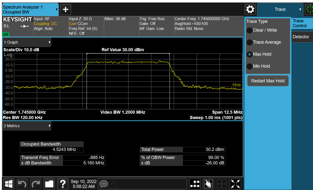
Plot 7-74. Occupied Bandwidth Plot (NR Band n66 - 5.0MHz CP-OFDM QPSK - Full RB – Ant A)
