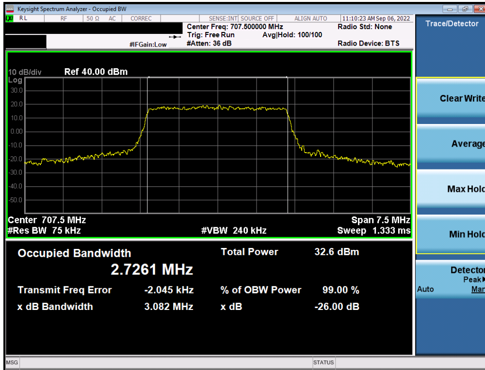
Plot 7-13. Occupied Bandwidth Plot (LTE Band 12 - 3MHz QPSK - Full RB Configuration)
