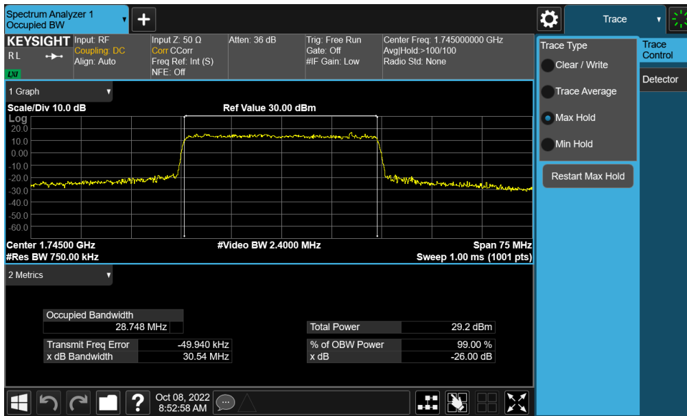
Plot 7-93. Occupied Bandwidth Plot (NR Band n66 - 30.0MHz CP-OFDM 16QAM - Full RB – Ant F)
