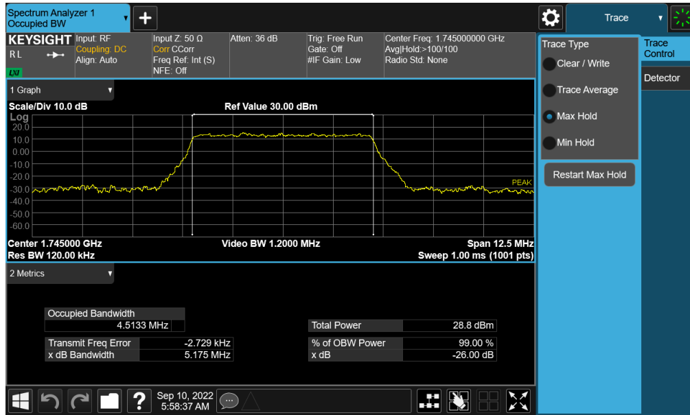
Plot 7-75. Occupied Bandwidth Plot (NR Band n66 - 5.0MHz CP-OFDM 16QAM - Full RB – Ant A)
