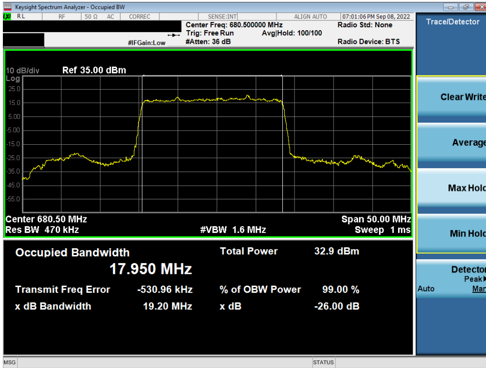
Plot 7-21. Occupied Bandwidth Plot (NR Band n71 - 20MHz DFT's BPSK - Full RB – Ant A)
