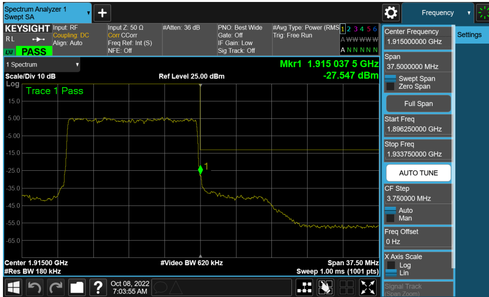
Plot 7-254. Upper Band Edge Plot (NR Band n25 - 15MHz QPSK – Full RB - Ant F)
