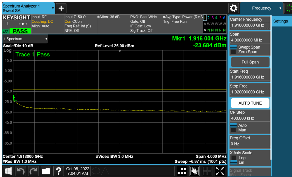
Plot 7-255. Extended Upper Band Edge Plot (NR Band n25 - 15MHz QPSK – Full RB - Ant F)
