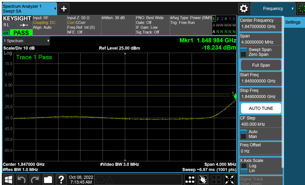
Plot 7-257. Extended Lower Band Edge Plot (NR Band n25/2 - 10MHz QPSK – Full RB - Ant F)
