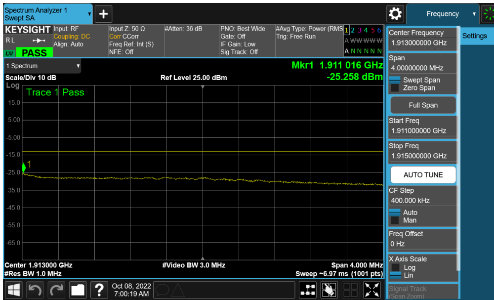
Plot 7-247. Extended Upper Band Edge Plot (NR Band n2 - 20MHz QPSK – Full RB - Ant F)
