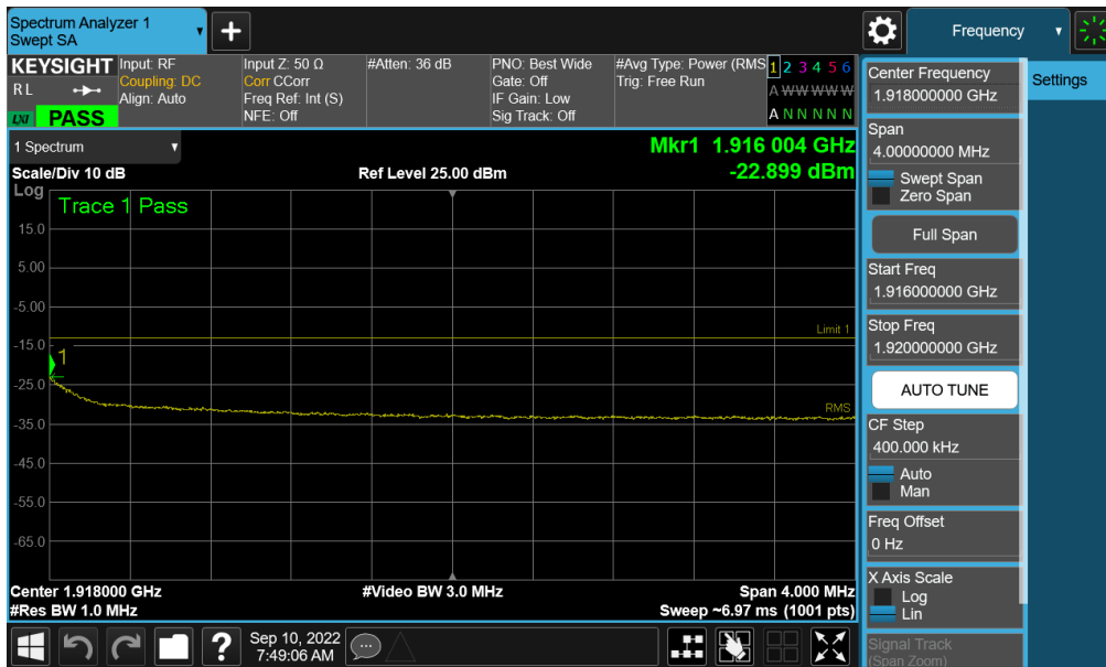
Plot 7-219. Extended Upper Band Edge Plot (NR Band n25 - 15MHz QPSK – Full RB - Ant A)
