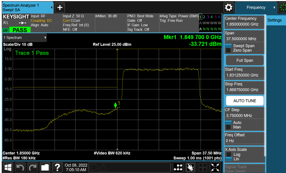
Plot 7-250. Lower Band Edge Plot (NR Band n25/2 - 15MHz QPSK – Full RB - Ant F)
