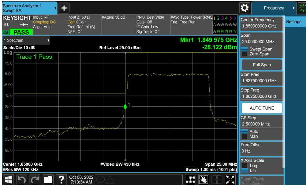
Plot 7-256. Lower Band Edge Plot (NR Band n25/2 - 10MHz QPSK – Full RB - Ant F)
