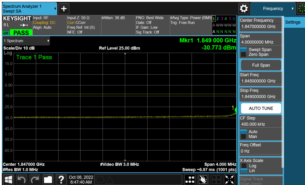
Plot 7-241. Extended Lower Band Edge Plot (NR Band n25 - 25MHz QPSK – Full RB - Ant F)
