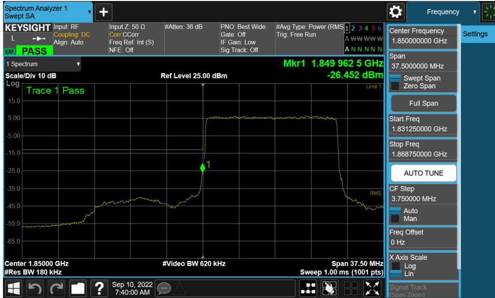
Plot 7-214. Lower Band Edge Plot (NR Band n25/2 - 15MHz QPSK – Full RB - Ant A)
