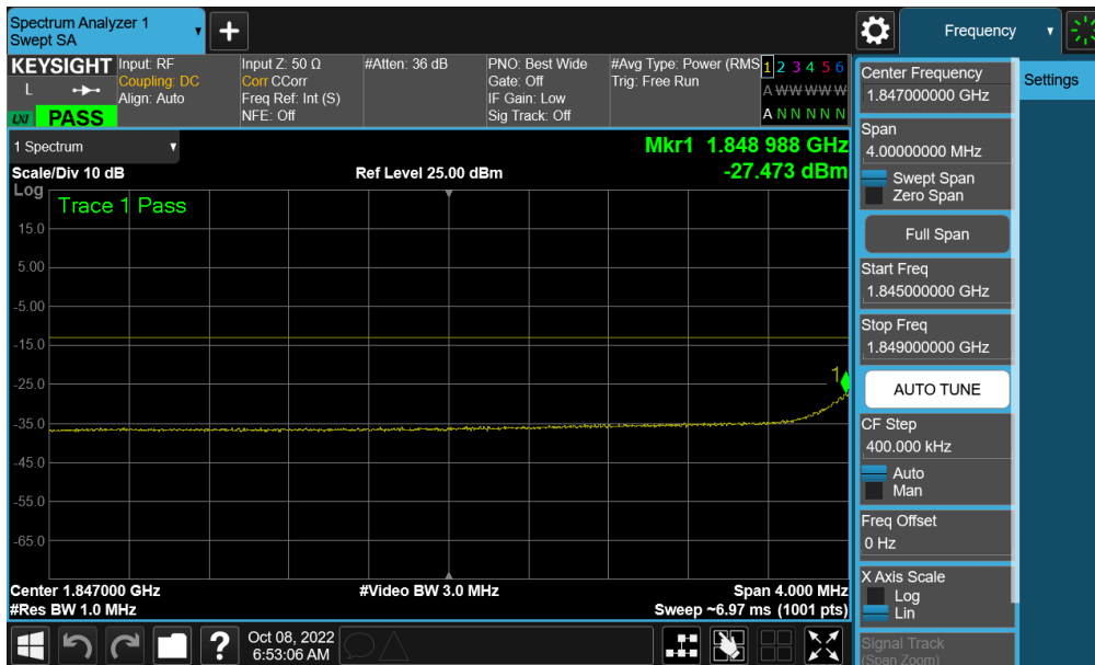
Plot 7-245. Extended Lower Band Edge Plot (NR Band n25/2 - 20MHz QPSK – Full RB - Ant F)
