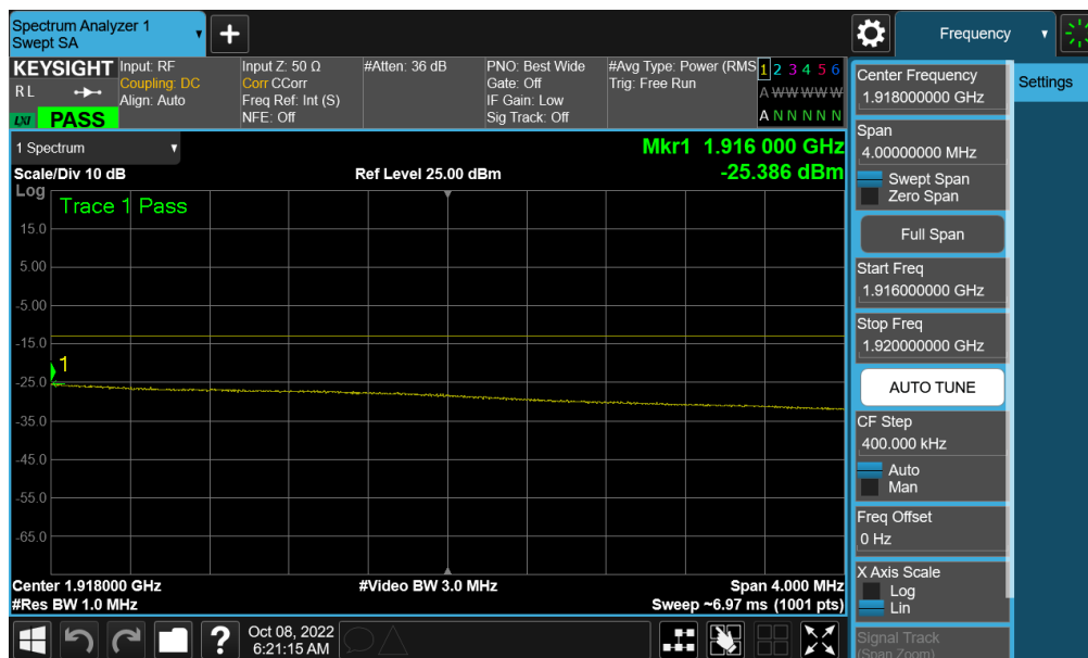
Plot 7-239. Extended Upper Band Edge Plot (NR Band n25 - 30MHz QPSK – Full RB - Ant F)
