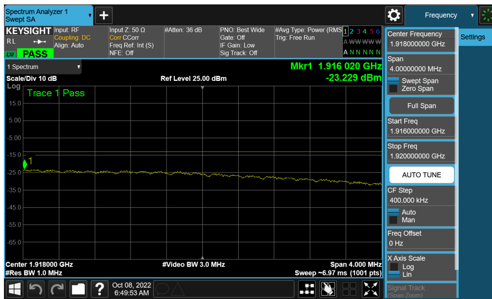
Plot 7-243. Extended Upper Band Edge Plot (NR Band n25 - 25MHz QPSK – Full RB - Ant F)
