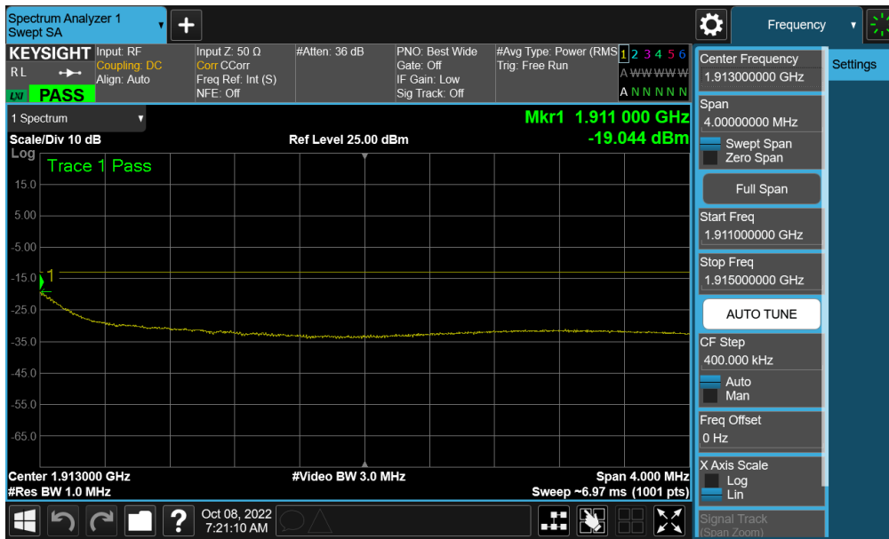
Plot 7-259. Extended Upper Band Edge Plot (NR Band n2 - 10MHz QPSK – Full RB - Ant F)
