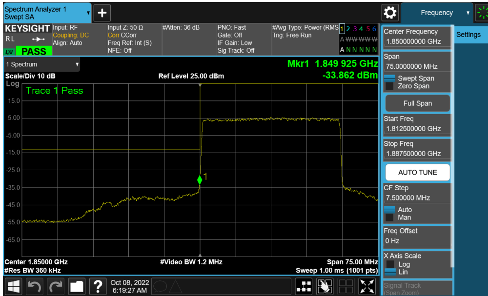
Plot 7-236. Lower Band Edge Plot (NR Band n25 - 30MHz QPSK – Full RB - Ant F)
