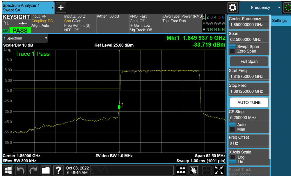
Plot 7-240. Lower Band Edge Plot (NR Band n25 - 25MHz QPSK – Full RB - Ant F)
