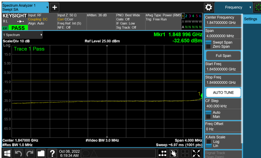
Plot 7-237. Extended Lower Band Edge Plot (NR Band n25 - 30MHz QPSK – Full RB - Ant F)
