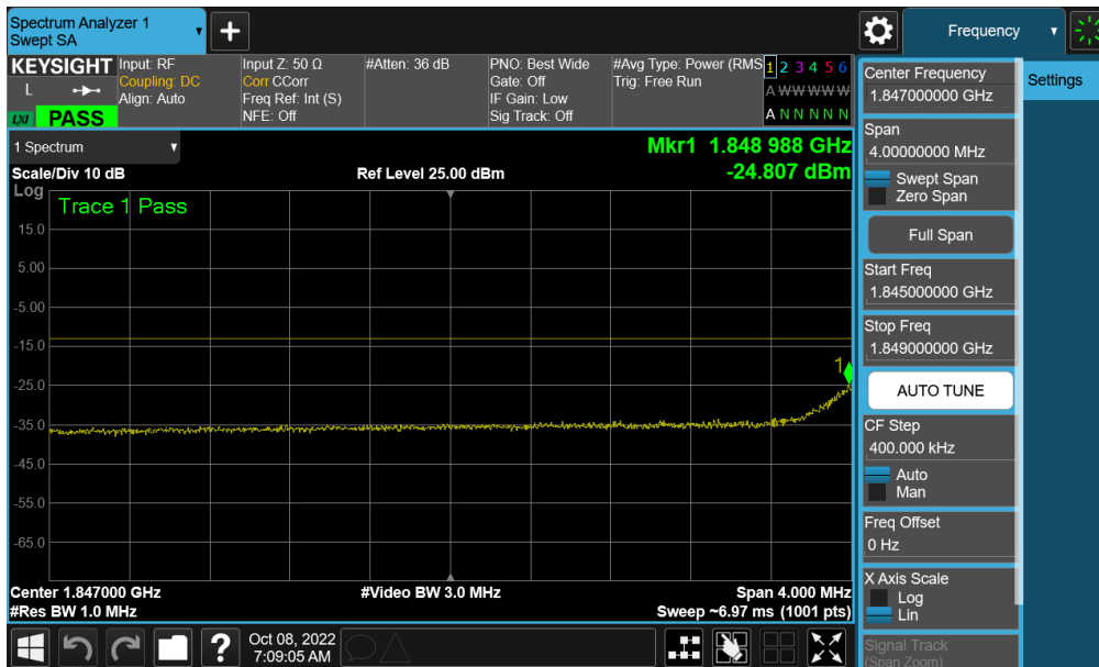
Plot 7-251. Extended Lower Band Edge Plot (NR Band n25/2 - 15MHz QPSK – Full RB - Ant F)
