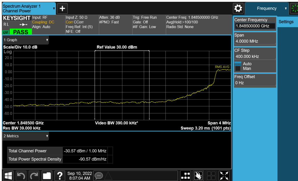
Plot 7-227. Extended Lower Band Edge Plot (NR Band n25/2 – 5MHz QPSK – Full RB - Ant A)
