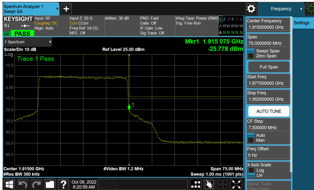
Plot 7-238. Upper Band Edge Plot (NR Band n25 - 30MHz QPSK – Full RB - Ant F)
