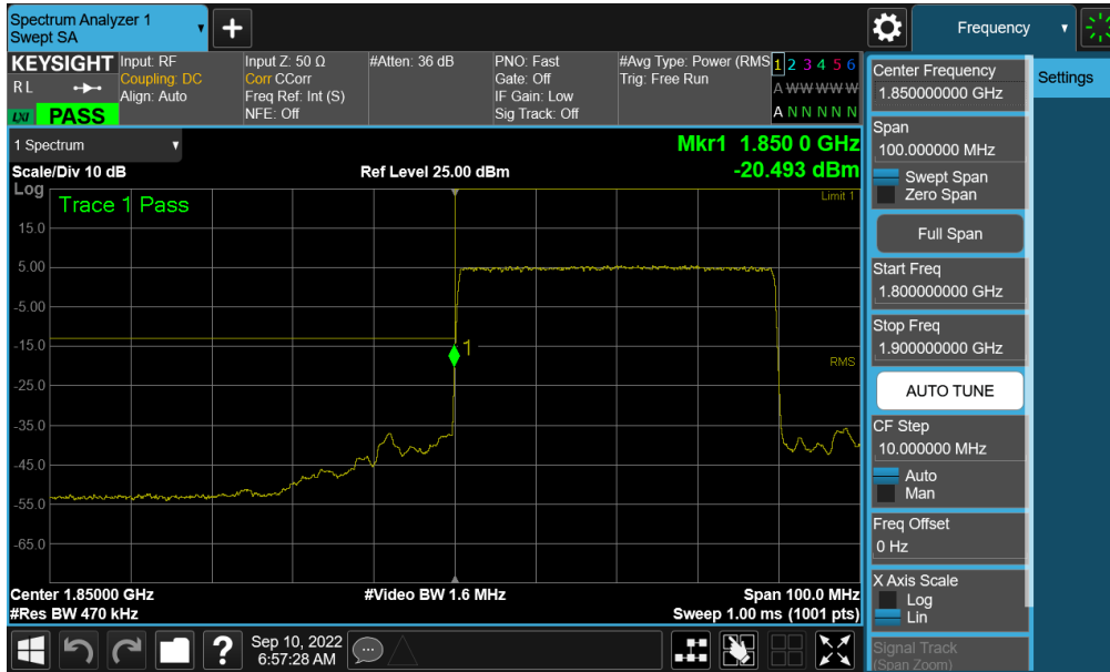
Plot 7-196. Lower Band Edge Plot (NR Band n25 - 40MHz QPSK – Full RB - Ant A)
