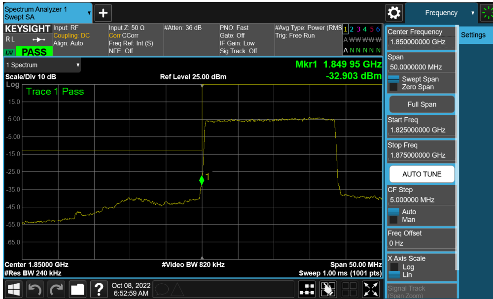
Plot 7-244. Lower Band Edge Plot (NR Band n25/2 - 20MHz QPSK – Full RB - Ant F)
