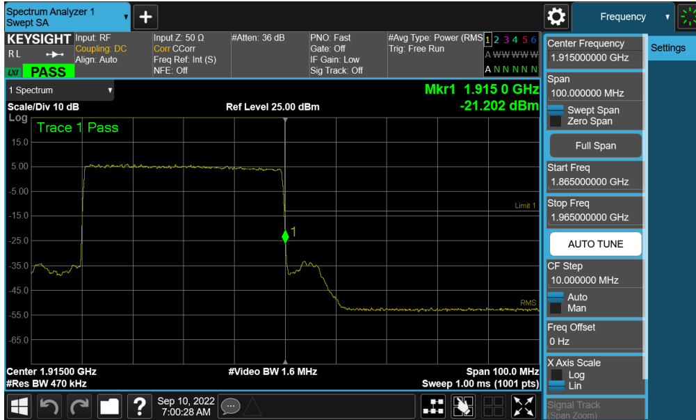
Plot 7-198. Upper Band Edge Plot (NR Band n25 - 40MHz QPSK – Full RB - Ant A)
