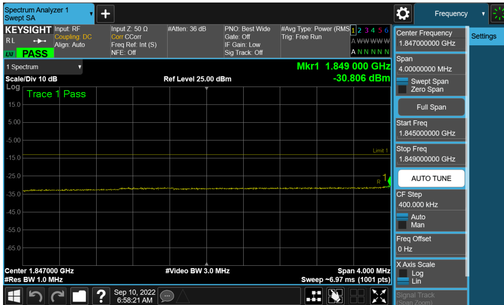
Plot 7-197. Extended Lower Band Edge Plot (NR Band n25 - 40MHz QPSK – Full RB - Ant A)
