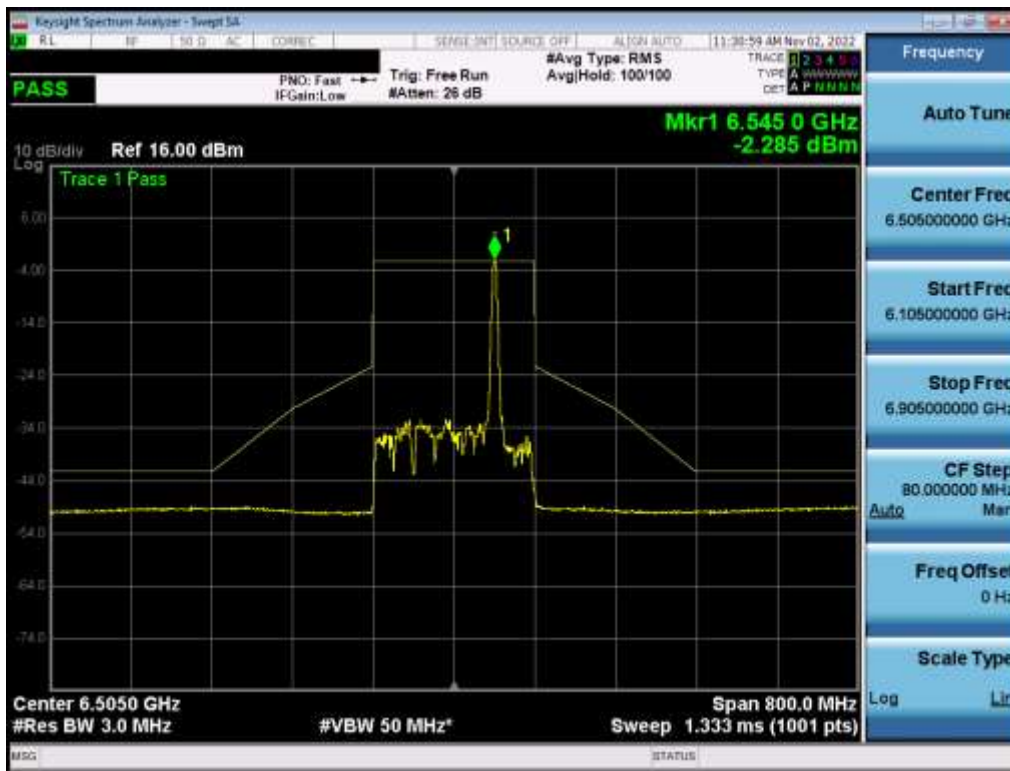
Plot 7-438. In-Band Emission Plot MIMO ANT1 (160MHz BW 802.11ax (26 Tones) (UNII Band 6) – Ch. 111) – LPI
