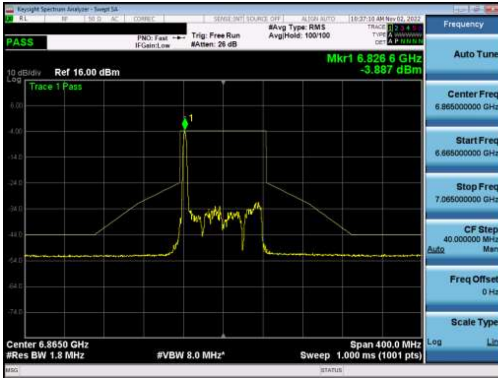
Plot 7-447. In-Band Emission Plot MIMO ANT1 (80MHz BW 802.11ax (26 Tones) (UNII Band 7) – Ch. 183) – LPI
