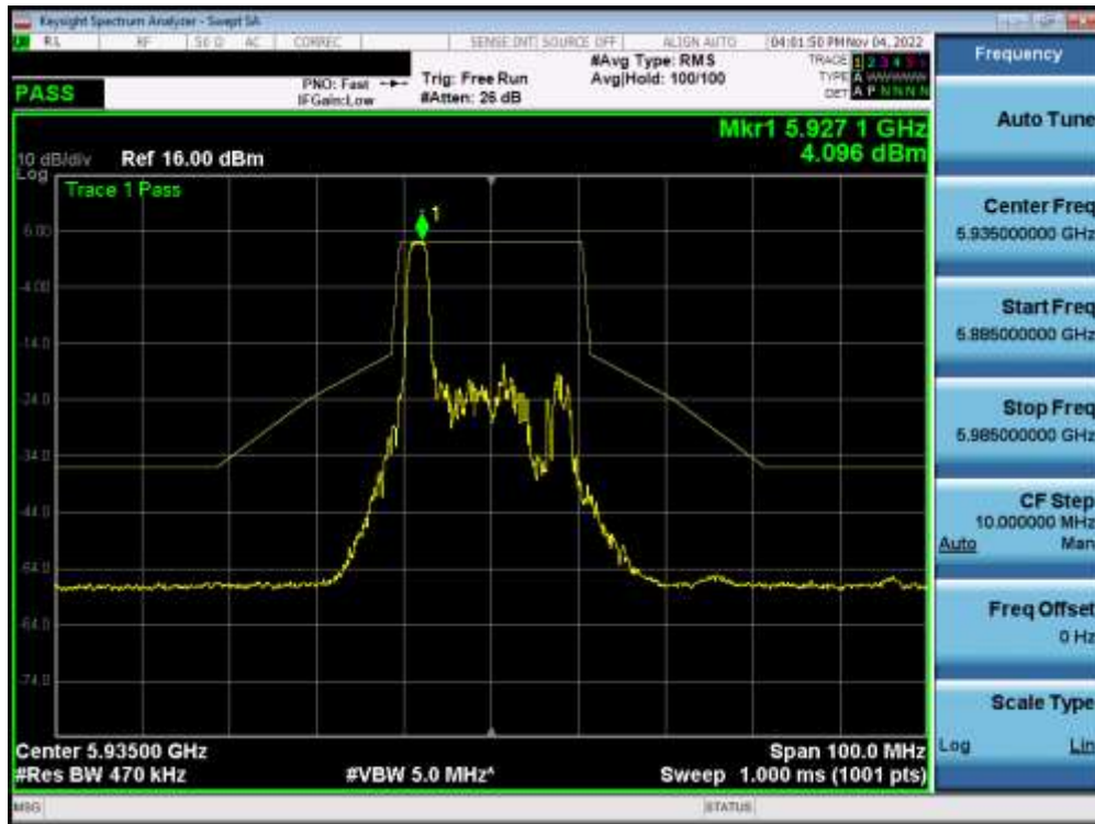
Plot 7-459. In-Band Emission Plot MIMO ANT1 (20MHz BW 802.11ax (26 Tones) UNII Band 5) – Ch. 2 - SP
