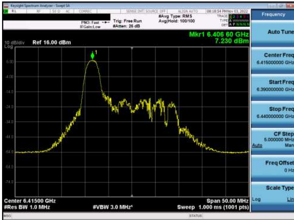
Plot 7-355. Power Spectral Density Plot MIMO ANT2 (20MHz BW 802.11ax (26 Tones) UNII Band 5) – Ch. 93) – SP
