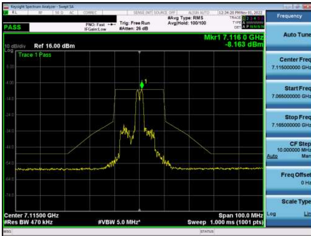
Plot 7-452. In-Band Emission Plot MIMO ANT1 (20MHz BW 802.11ax (26 Tones) (UNII Band 8) – Ch. 233) – LPI
