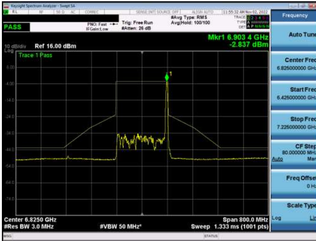
Plot 7-449. In-Band Emission Plot MIMO ANT1 (160MHz BW 802.11ax (26 Tones) (UNII Band 7) – Ch. 175) – LPI
