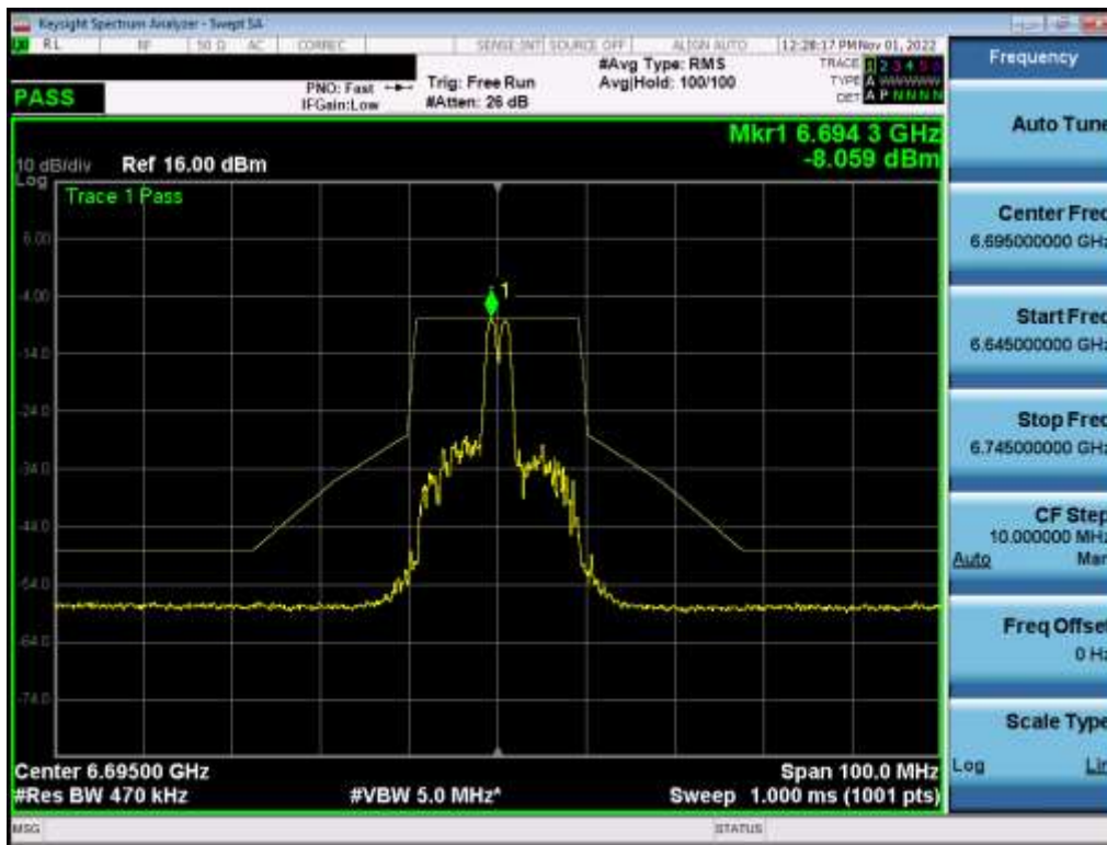
Plot 7-440. In-Band Emission Plot MIMO ANT1 (20MHz BW 802.11ax (26 Tones) (UNII Band 7) – Ch. 149) – LPI
