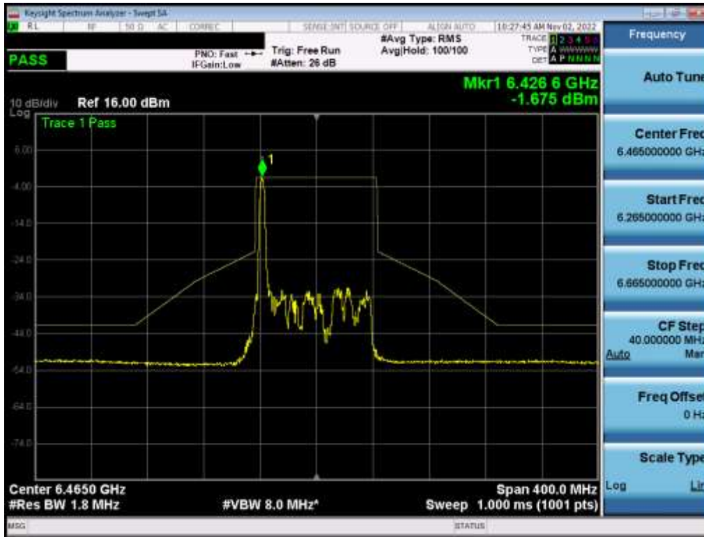
Plot 7-437. In-Band Emission Plot MIMO ANT1 (80MHz BW 802.11ax (26 Tones) (UNII Band 6) – Ch. 103) – LPI
