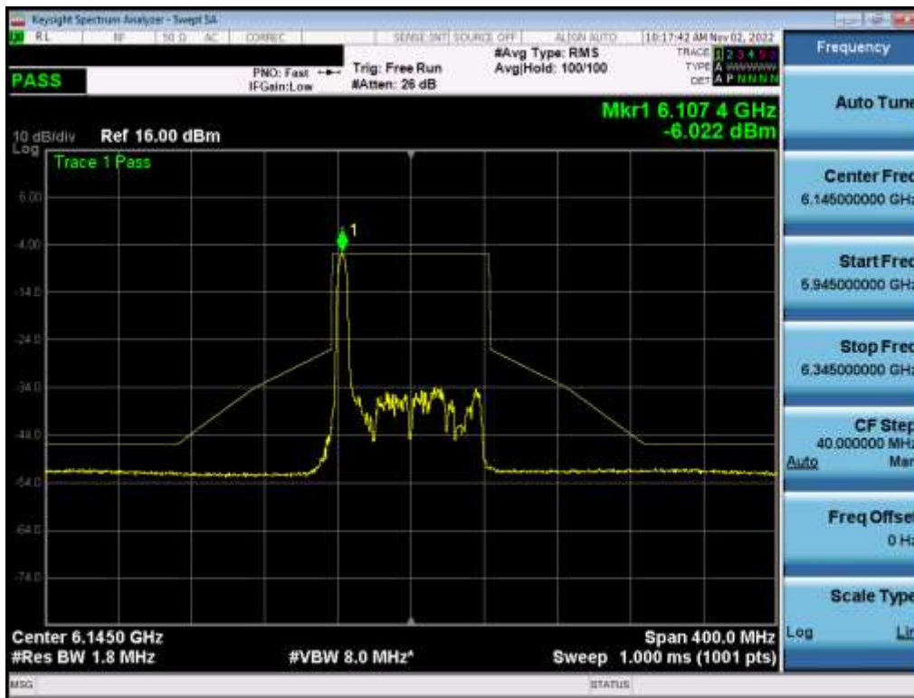
Plot 7-426. In-Band Emission Plot MIMO ANT1 (80MHz BW 802.11ax (26 Tones) (UNII Band 5) – Ch. 39) – LPI
