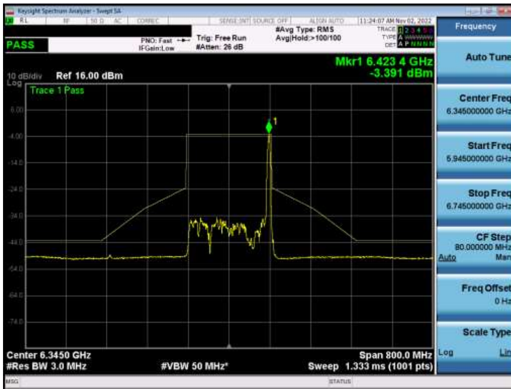
Plot 7-430. In-Band Emission Plot MIMO ANT1 (160MHz BW 802.11ax (26 Tones) (UNII Band 5) – Ch. 79) – LPI
