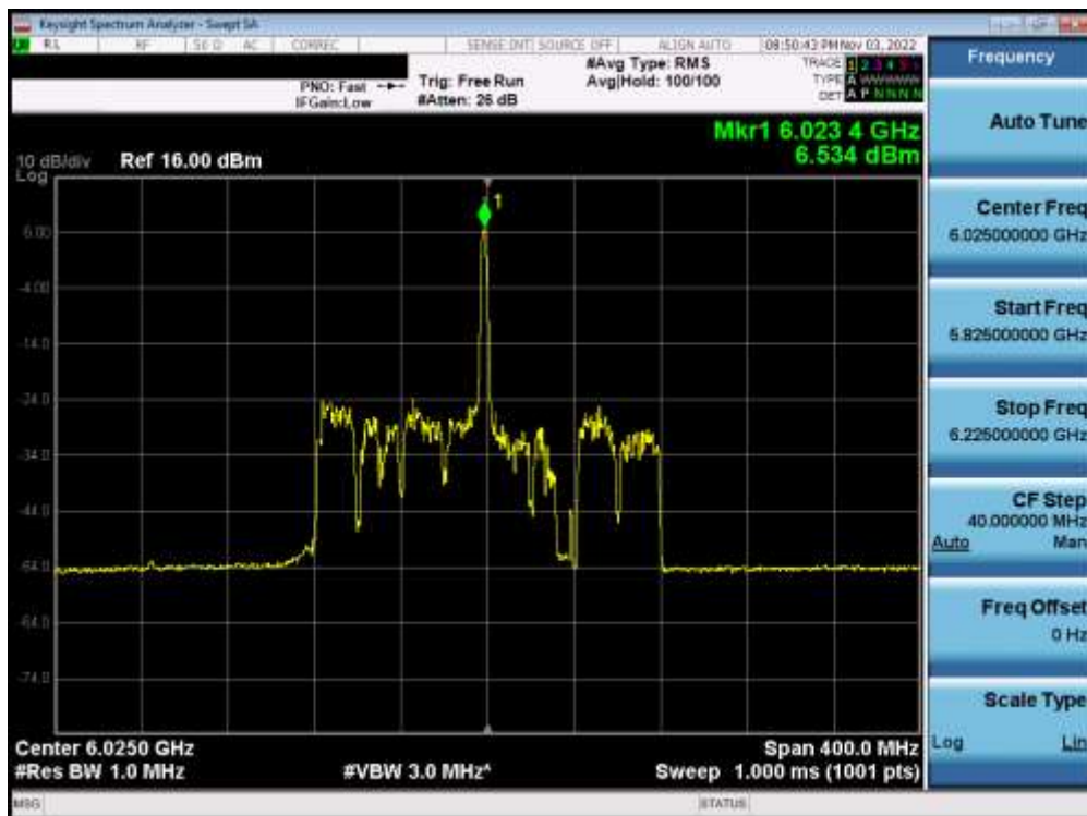
Plot 7-362. Power Spectral Density Plot MIMO ANT2 (160MHz BW 802.11ax (26 Tones) (UNII Band 5) – Ch. 15) – SP
