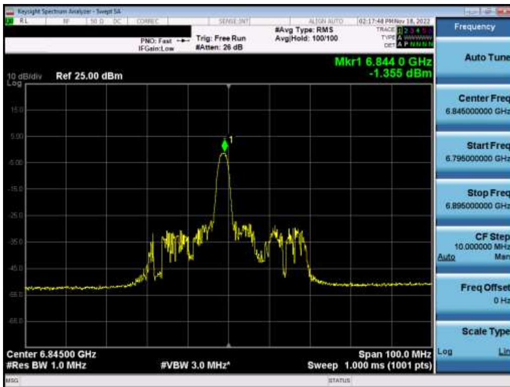
Plot 7-338. Power Spectral Density Plot MIMO ANT2 (40MHz BW 802.11ax (26 Tones) (UNII Band 7) – Ch. 179) – LPI
