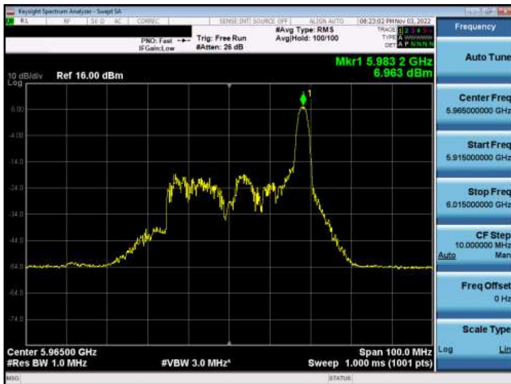
Plot 7-356. Power Spectral Density Plot MIMO ANT2 (40MHz BW 802.11ax (26 Tones) (UNII Band 5) – Ch. 3) – SP
