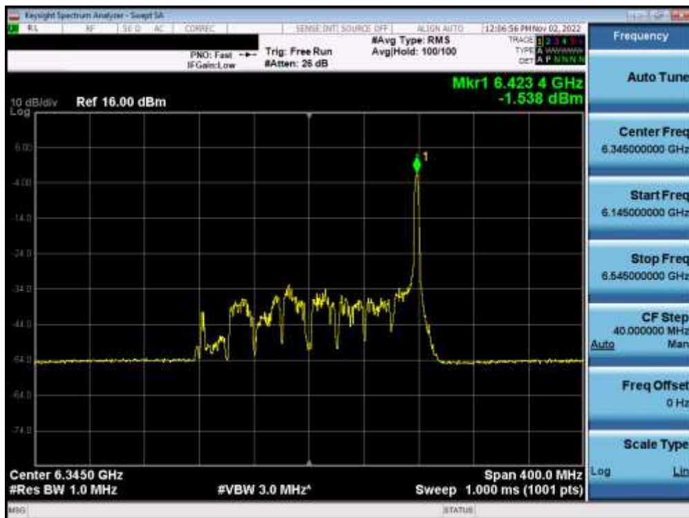
Plot 7-324. Power Spectral Density Plot MIMO ANT2 (160MHz BW 802.11ax (26 Tones) (UNII Band 5) – Ch. 79) – LPI
