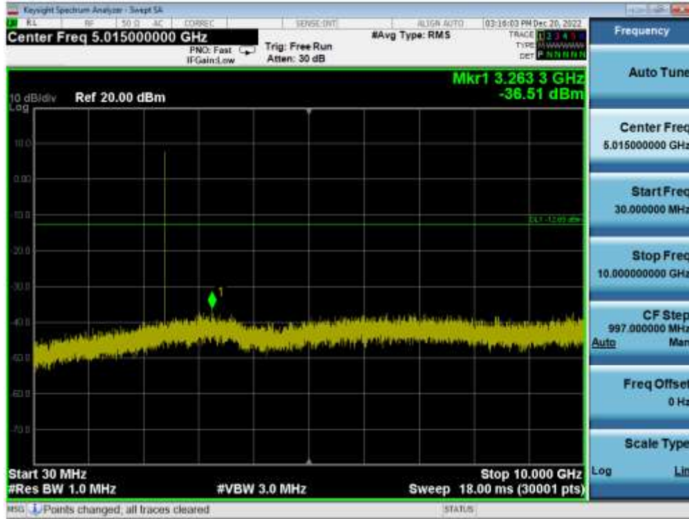
Plot 7-73. Conducted Spurious Plot (Bluetooth (LE), 2Mbps – Ch. 0) – ANT 2
