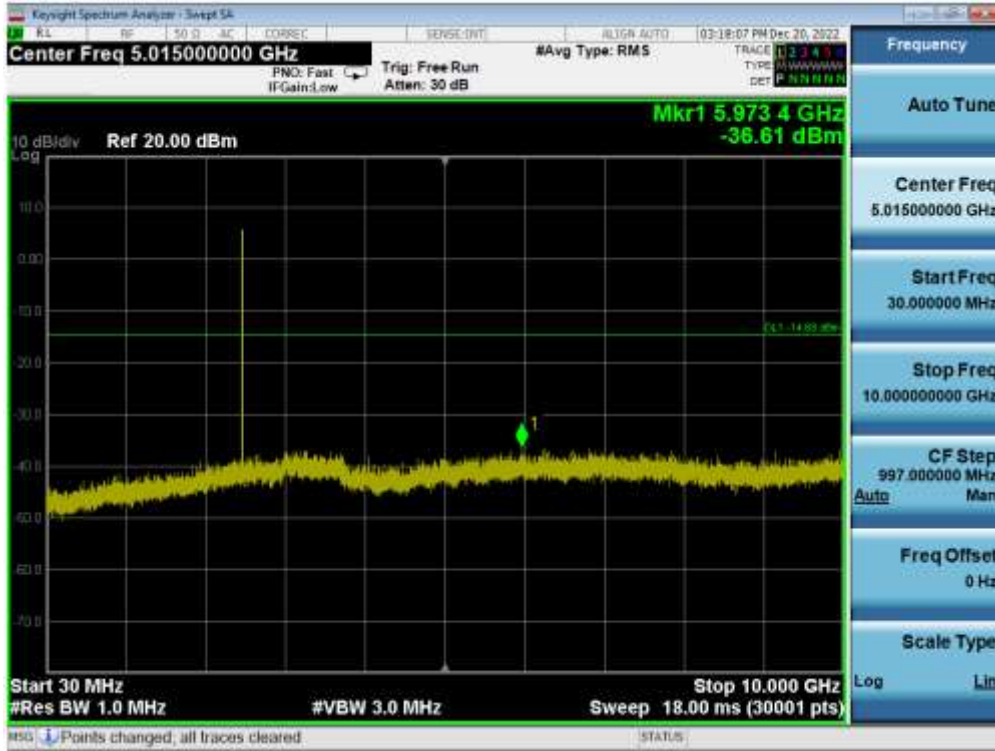
Plot 7-77. Conducted Spurious Plot (Bluetooth (LE), 2Mbps – Ch. 39) – ANT 2
