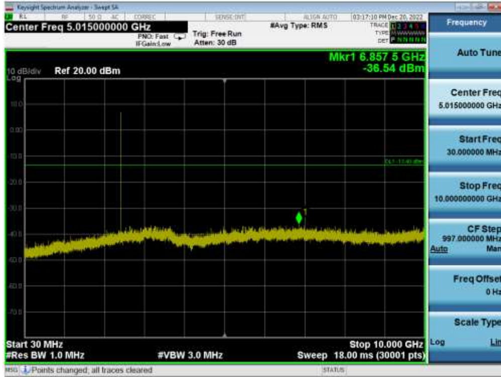
Plot 7-75. Conducted Spurious Plot (Bluetooth (LE), 2Mbps – Ch. 19) – ANT 2
