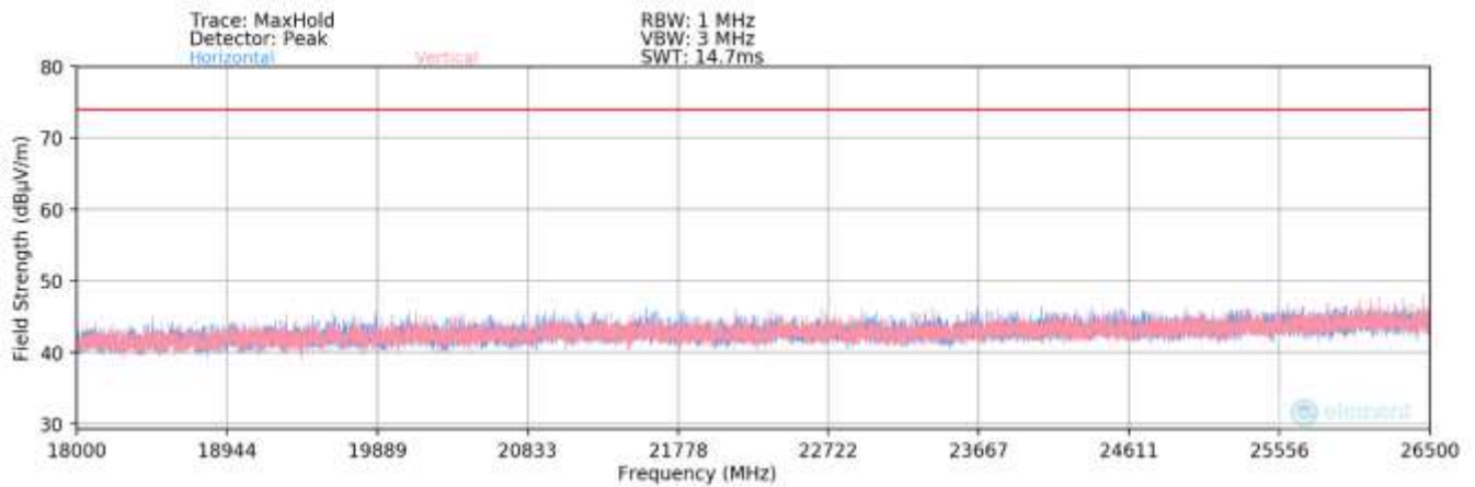
Plot 7-121. Radiated Spurious Plot above 18GHz MIMO (802.11ax OFDMA – 242 Tones)
