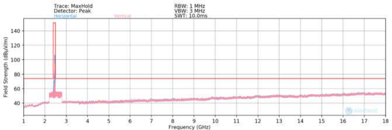
Plot 7-111. Radiated Spurious Plot above 1GHz SISO ANT2 (802.11ax OFDMA – 242 Tones – Ch. 11)
