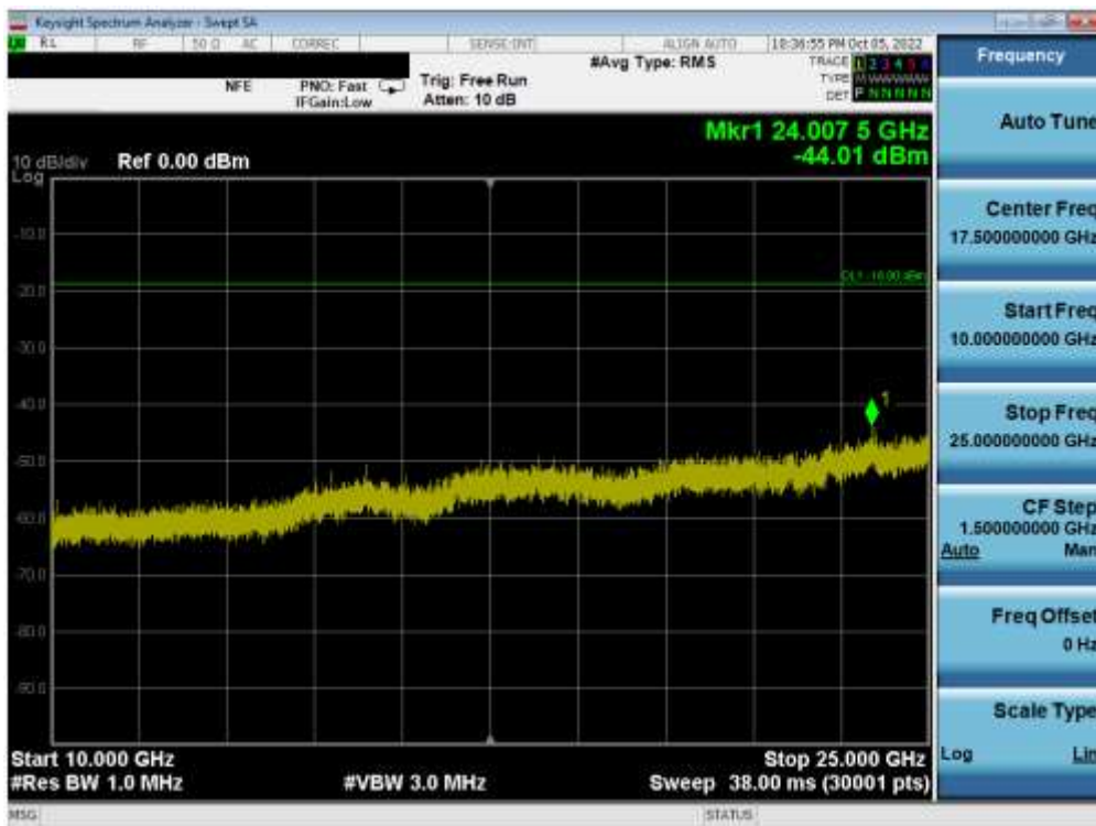
Plot 7-97. Conducted Spurious Plot MIMO ANT2 (802.11ax OFDMA – 26 Tones – Ch. 6)
