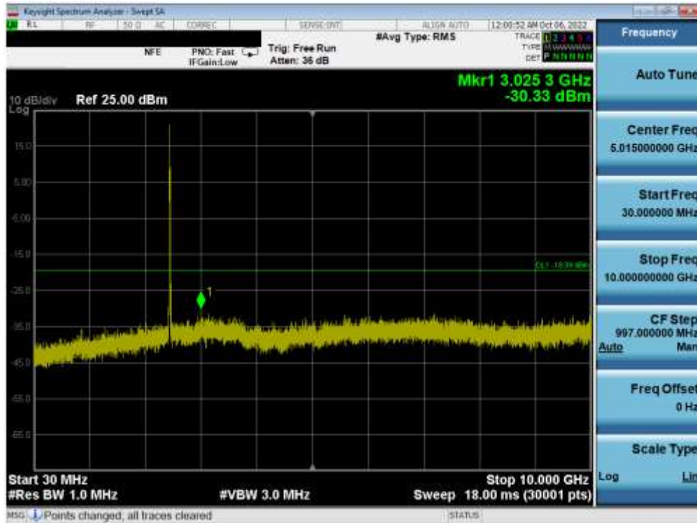
Plot 7-74. Conducted Spurious Plot SISO ANT2 (802.11ax OFDMA – 26 Tones – Ch. 11)
