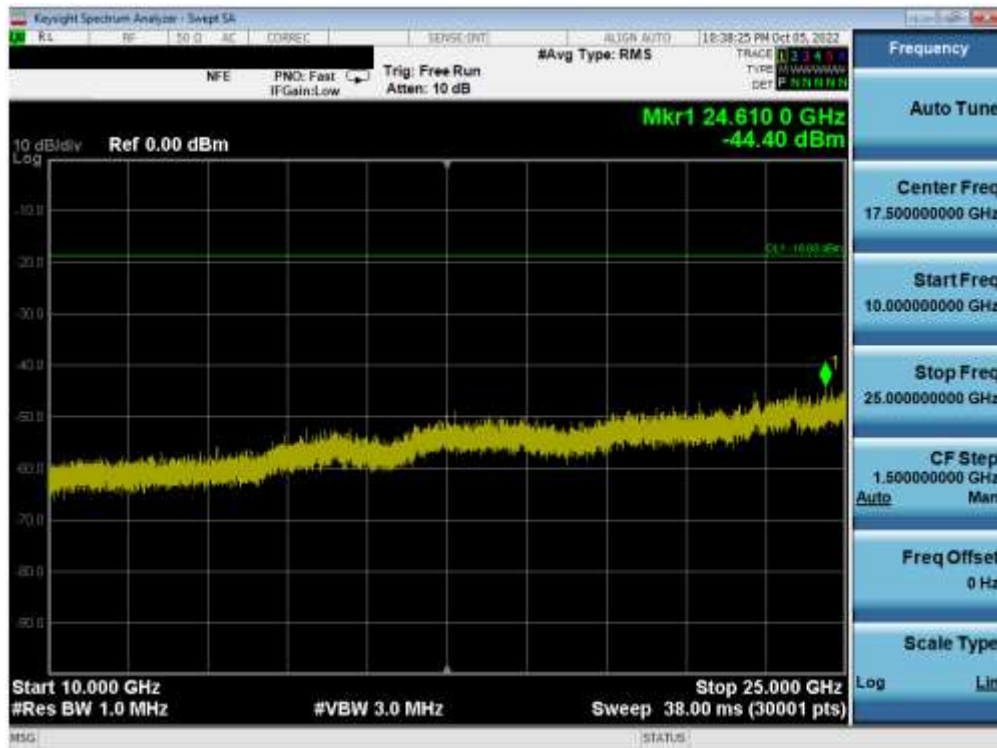
Plot 7-99. Conducted Spurious Plot MIMO ANT2 (802.11ax OFDMA – 26 Tones – Ch. 11)
