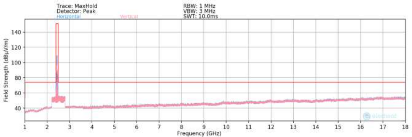
Plot 7-110. Radiated Spurious Plot above 1GHz SISO ANT2 (802.11ax OFDMA – 242 Tones – Ch. 6)
