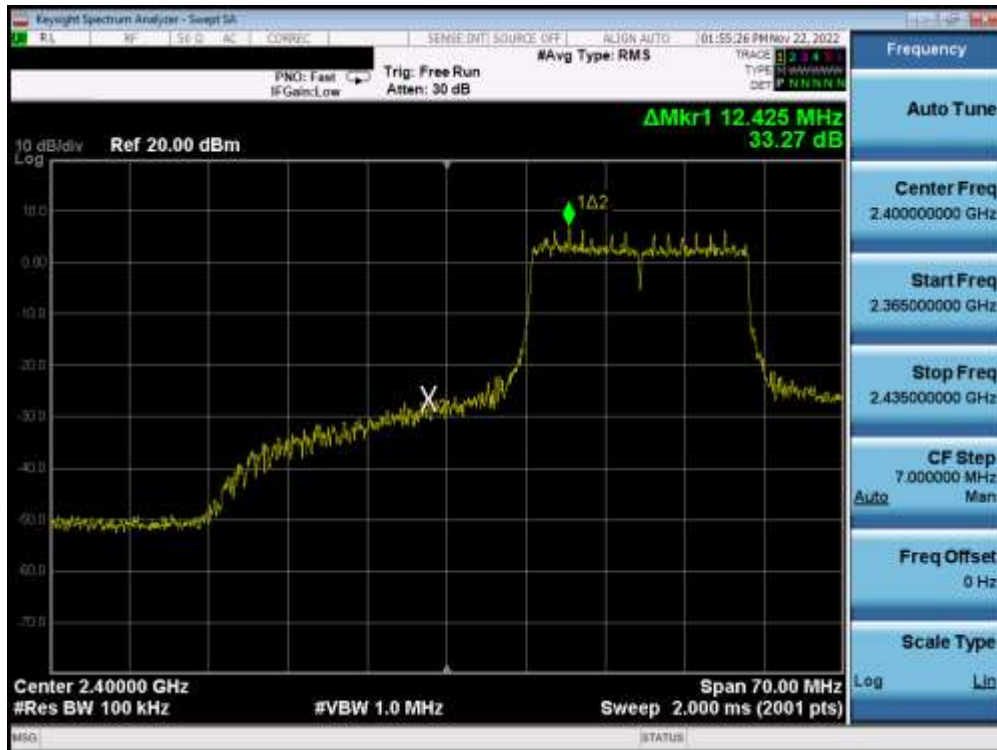
Plot 7-53. Band Edge Plot MIMO ANT1 (802.11ax OFDMA – 242 Tones – Ch. 2)
