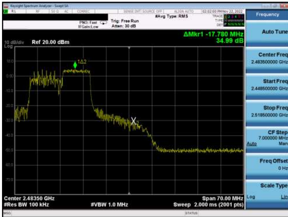
Plot 7-60. Band Edge Plot MIMO ANT2 (802.11ax OFDMA – 106 Tones – Ch. 11)
