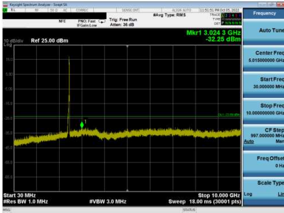
Plot 7-92. Conducted Spurious Plot MIMO ANT1 (802.11ax OFDMA – 242 Tones – Ch. 11)
