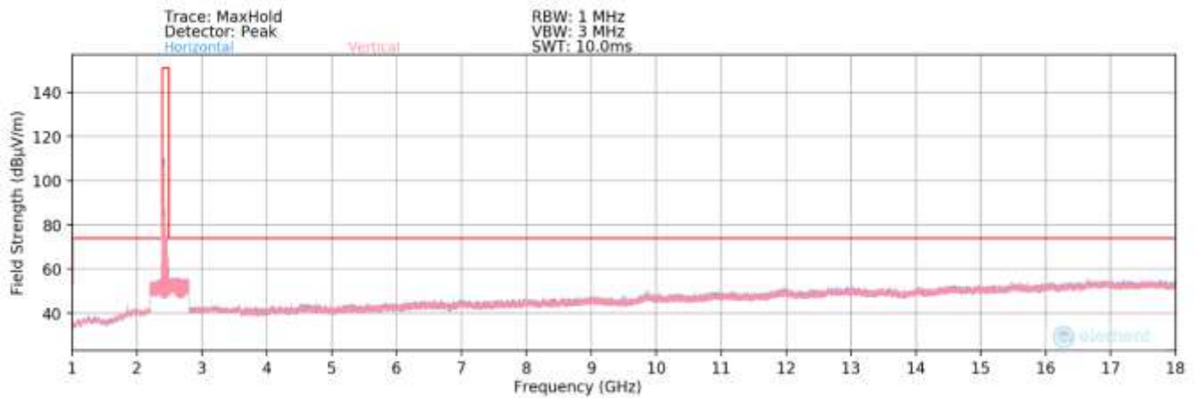
Plot 7-117. Radiated Spurious Plot above 1GHz MIMO (802.11ax OFDMA – 242 Tones – Ch. 1)
