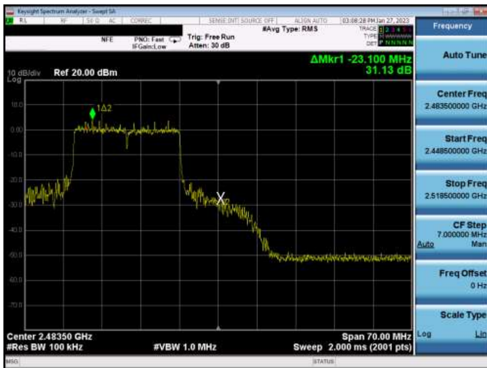
Plot 7-68. Band Edge Plot MIMO ANT2 (802.11ax OFDMA – 242 Tones – Ch. 12)
