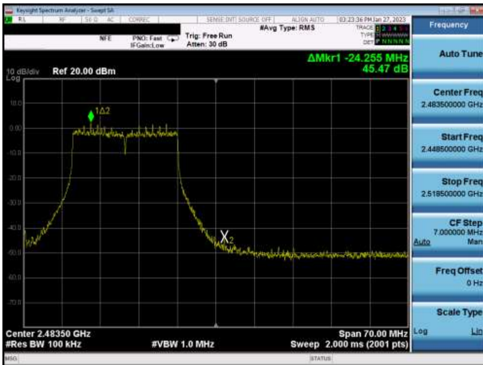
Plot 7-57. Band Edge Plot MIMO ANT1 (802.11ax OFDMA – 242 Tones – Ch. 12)
