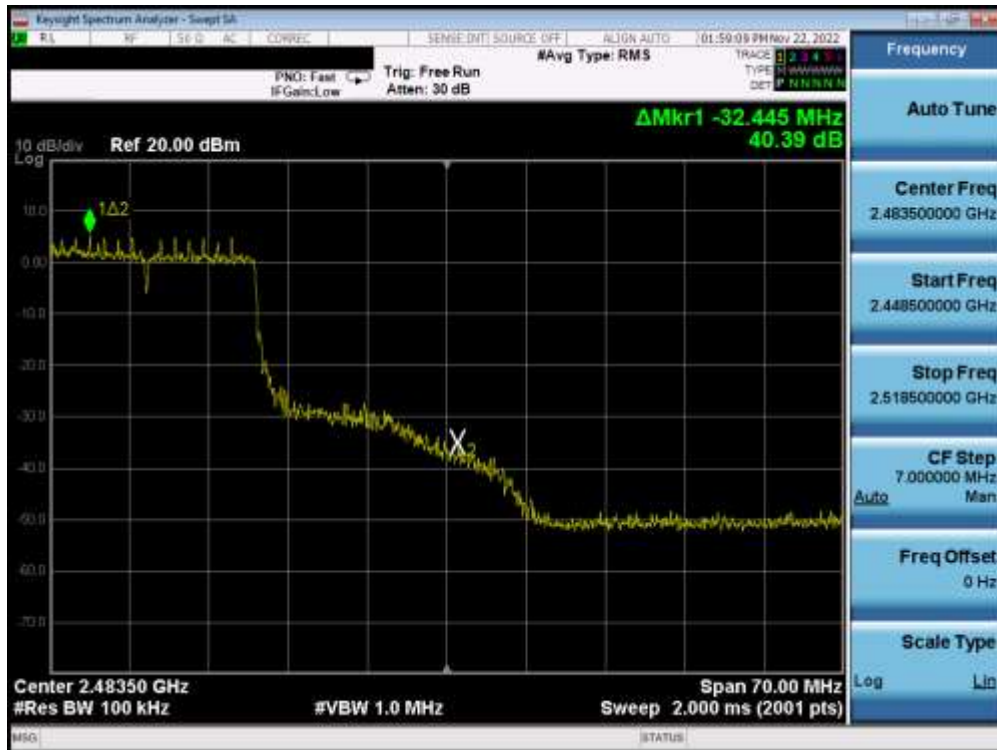
Plot 7-55. Band Edge Plot MIMO ANT1 (802.11ax OFDMA – 242 Tones – Ch. 10)
