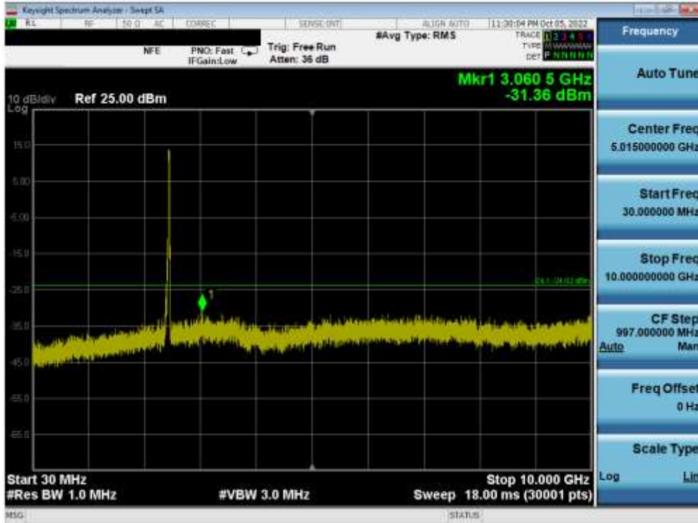
Plot 7-104. Conducted Spurious Plot MIMO ANT2 (802.11ax OFDMA – 242 Tones – Ch. 11)
