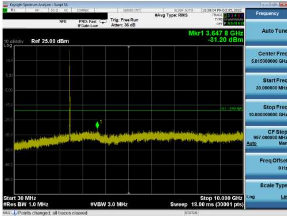
Plot 7-98. Conducted Spurious Plot MIMO ANT2 (802.11ax OFDMA – 26 Tones – Ch. 11)
