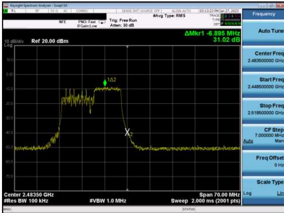
Plot 7-62. Band Edge Plot MIMO ANT2 (802.11ax OFDMA – 106 Tones – Ch. 13)
