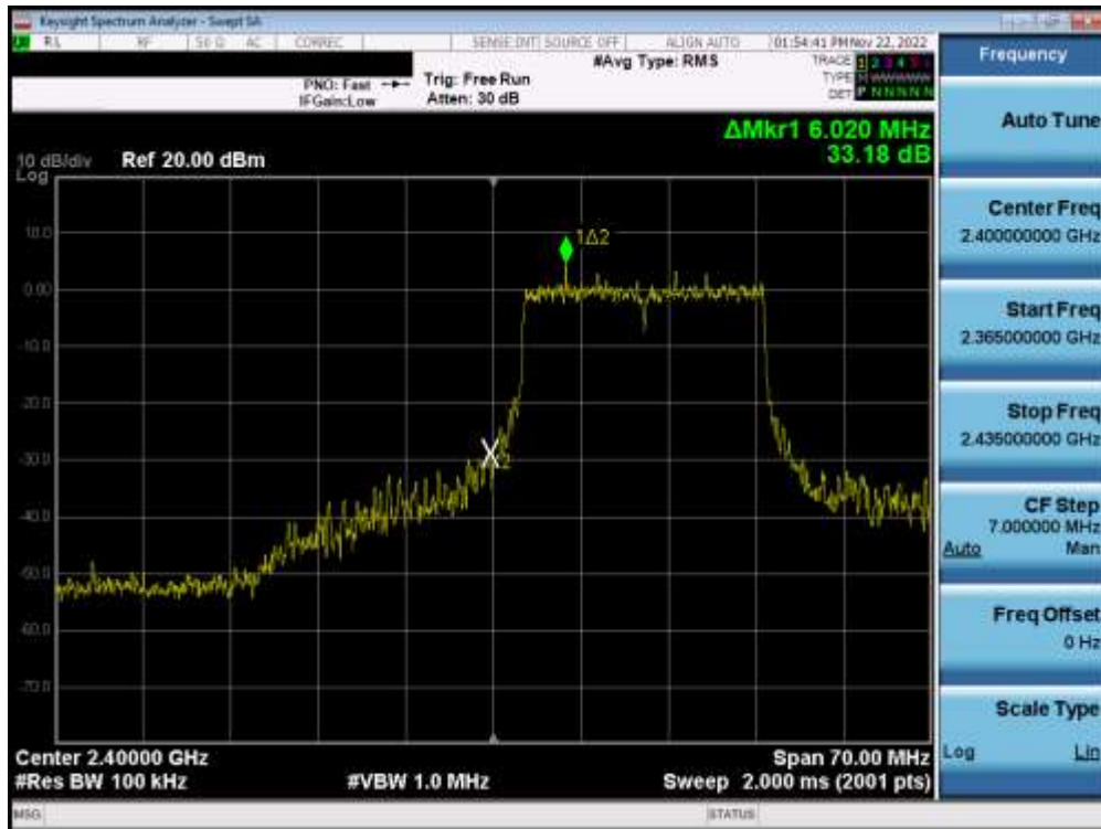
Plot 7-52. Band Edge Plot MIMO ANT1 (802.11ax OFDMA – 242 Tones – Ch. 1)
