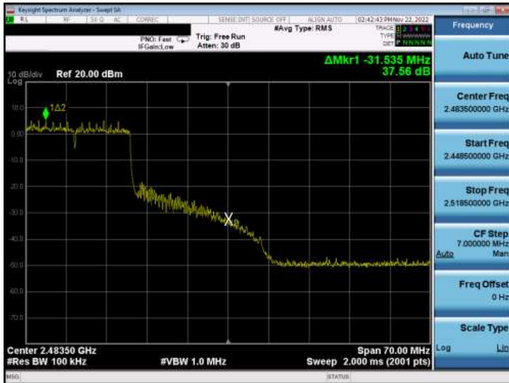
Plot 7-66. Band Edge Plot MIMO ANT2 (802.11ax OFDMA – 242 Tones – Ch. 10)
