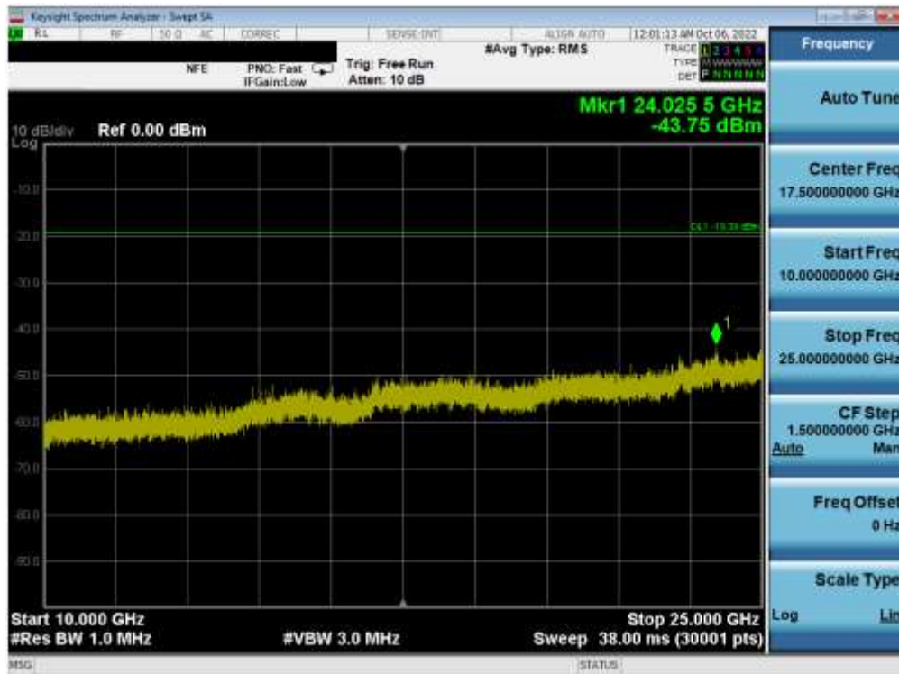
Plot 7-75. Conducted Spurious Plot SISO ANT2 (802.11ax OFDMA – 26 Tones – Ch. 11)
