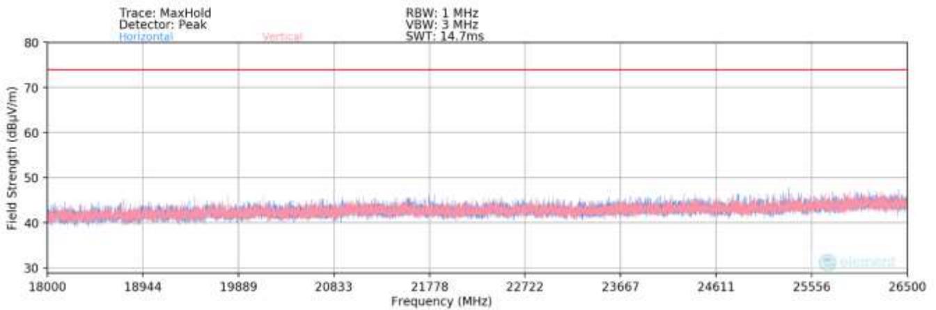
Plot 7-113. Radiated Spurious Plot above 18GHz SISO ANT2 (802.11ax OFDMA – 242 Tones)
