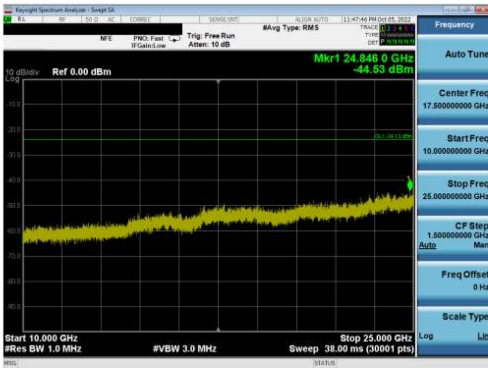
Plot 7-89. Conducted Spurious Plot MIMO ANT1 (802.11ax OFDMA – 242 Tones – Ch. 1)
