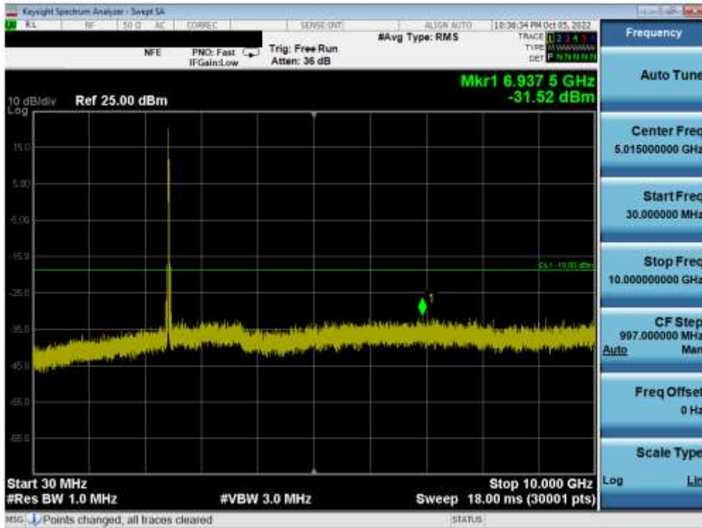
Plot 7-96. Conducted Spurious Plot MIMO ANT2 (802.11ax OFDMA – 26 Tones – Ch. 6)
