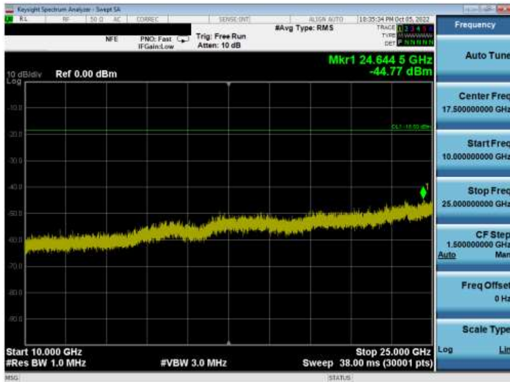
Plot 7-95. Conducted Spurious Plot MIMO ANT2 (802.11ax OFDMA – 26 Tones – Ch. 1)
