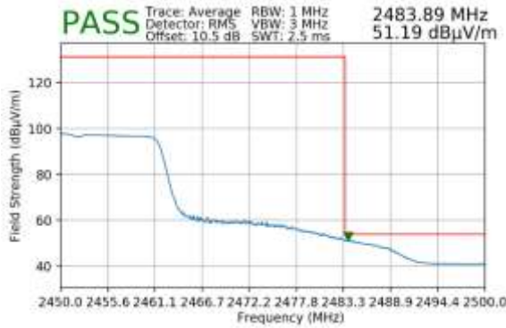
Plot 7-134. Radiated Restricted Upper Band Edge Measurement SISO ANT2 (Average – 242 Tones)
