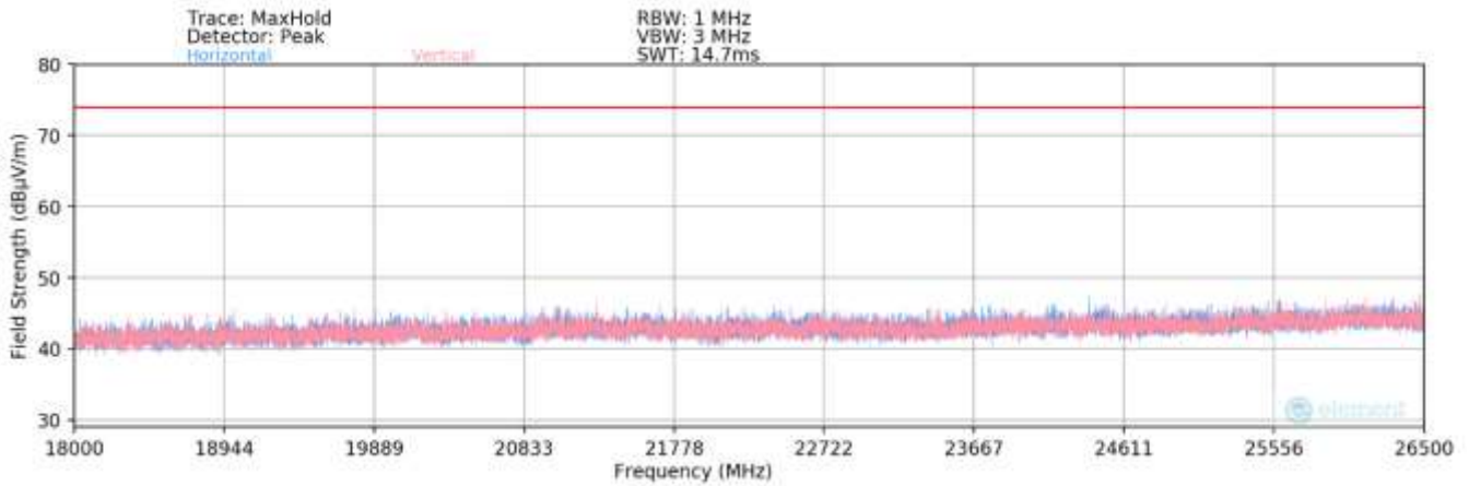
Plot 7-112. Radiated Spurious Plot above 18GHz SISO ANT2 (802.11ax OFDMA – 26 Tones)
