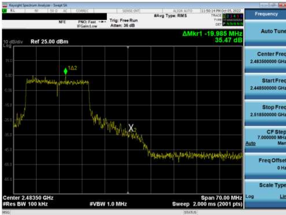
Plot 7-56. Band Edge Plot MIMO ANT1 (802.11ax OFDMA – 242 Tones – Ch. 11)
