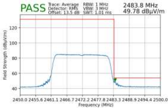
Plot 7-142. Radiated Restricted Upper Band Edge Measurement SISO ANT2 (Average – 242 Tones)
