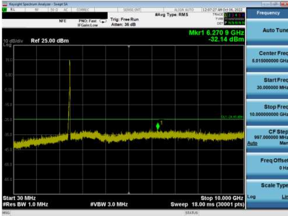
Plot 7-80. Conducted Spurious Plot SISO ANT2 (802.11ax OFDMA – 242 Tones – Ch. 11)
