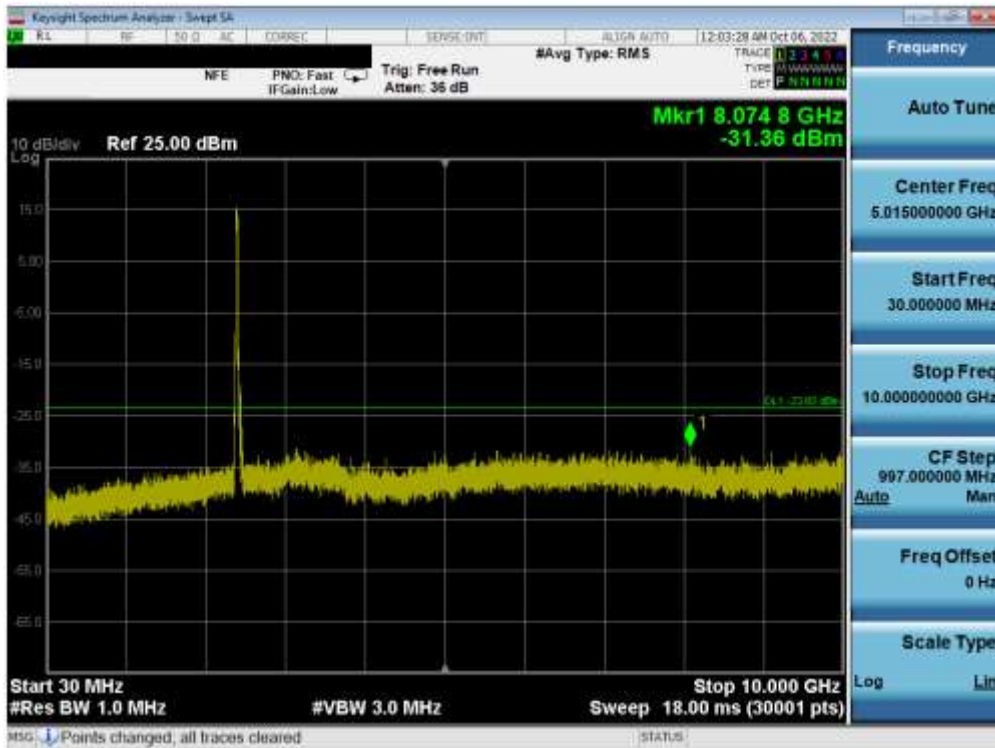
Plot 7-76. Conducted Spurious Plot SISO ANT2 (802.11ax OFDMA – 242 Tones – Ch. 1)
