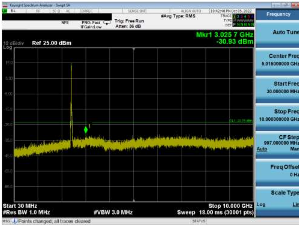
Plot 7-100. Conducted Spurious Plot MIMO ANT2 (802.11ax OFDMA – 242 Tones – Ch. 1)
