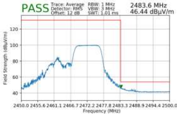
Plot 7-148. Radiated Restricted Upper Band Edge Measurement MIMO (Average – 106 Tones)
