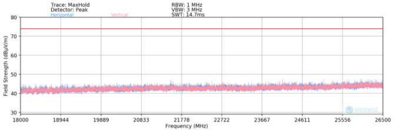
Plot 7-120. Radiated Spurious Plot above 18GHz MIMO (802.11ax OFDMA – 26 Tones)
