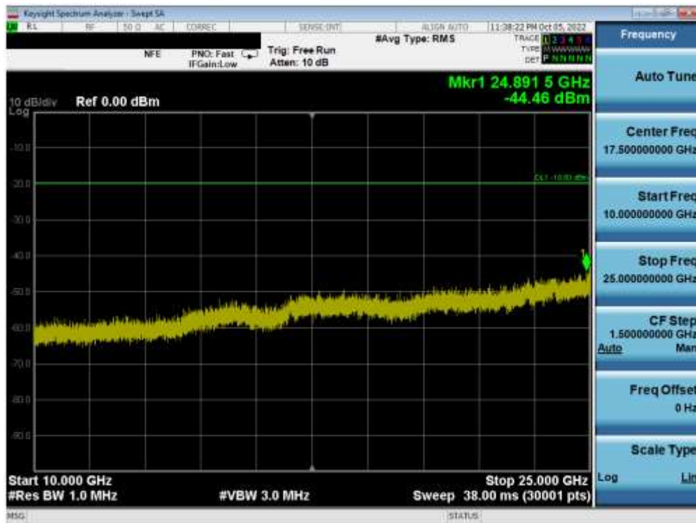
Plot 7-83. Conducted Spurious Plot MIMO ANT1 (802.11ax OFDMA – 26 Tones – Ch. 1)
