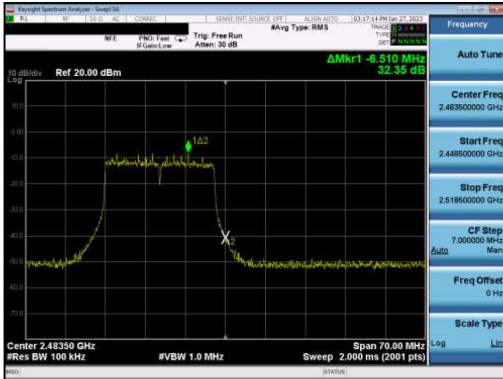
Plot 7-58. Band Edge Plot MIMO ANT1 (802.11ax OFDMA – 242 Tones – Ch. 13)
