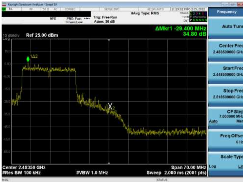
Plot 7-67. Band Edge Plot MIMO ANT2 (802.11ax OFDMA – 242 Tones – Ch. 11)
