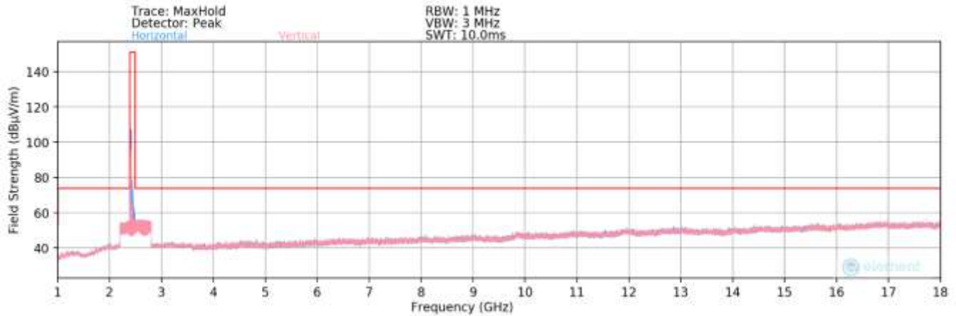
Plot 7-109. Radiated Spurious Plot above 1GHz SISO ANT2 (802.11ax OFDMA – 242 Tones – Ch. 1)
