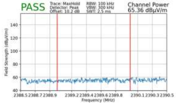
Plot 7-131. Radiated Restricted Lower Band Edge Measurement SISO ANT2 (Peak – 242 Tones)
