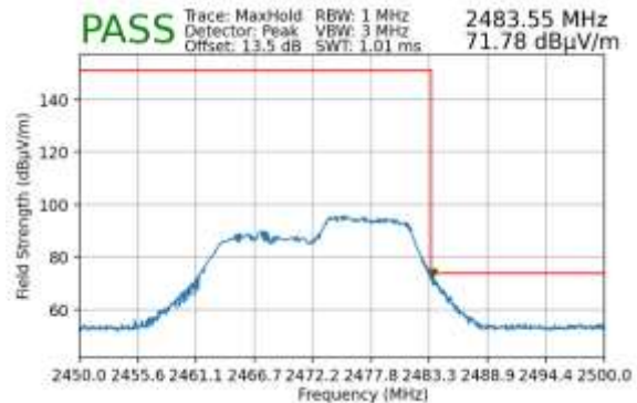
Plot 7-129. Radiated Restricted Upper Band Edge Measurement SISO ANT2 (Peak – 106 Tones)
