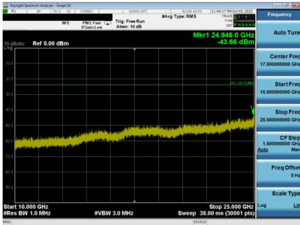
Plot 7-91. Conducted Spurious Plot MIMO ANT1 (802.11ax OFDMA – 242 Tones – Ch. 6)
