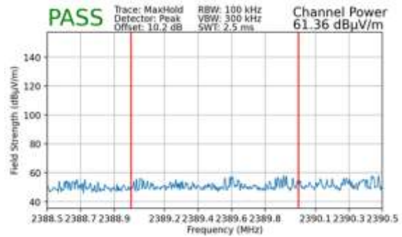
Plot 7-153. Radiated Restricted Lower Band Edge Measurement MIMO (Peak – 242 Tones)
