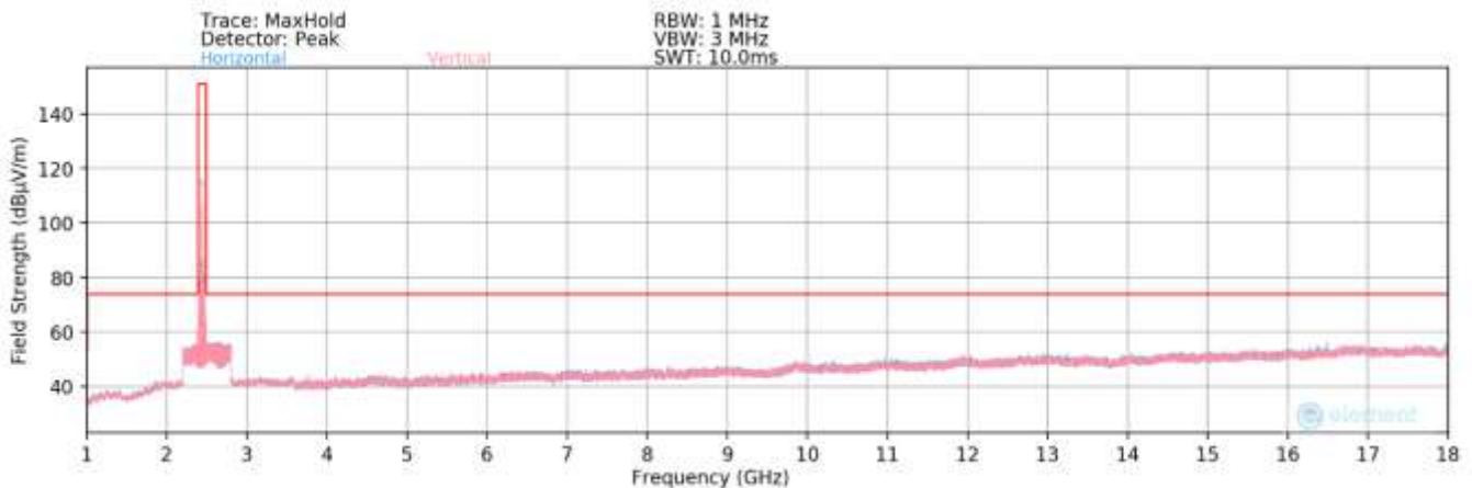
Plot 7-115. Radiated Spurious Plot above 1GHz MIMO (802.11ax OFDMA – 26 Tones – Ch. 6)
