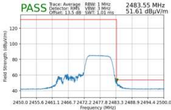
Plot 7-128. Radiated Restricted Upper Band Edge Measurement SISO ANT2 (Average – 106 Tones)
