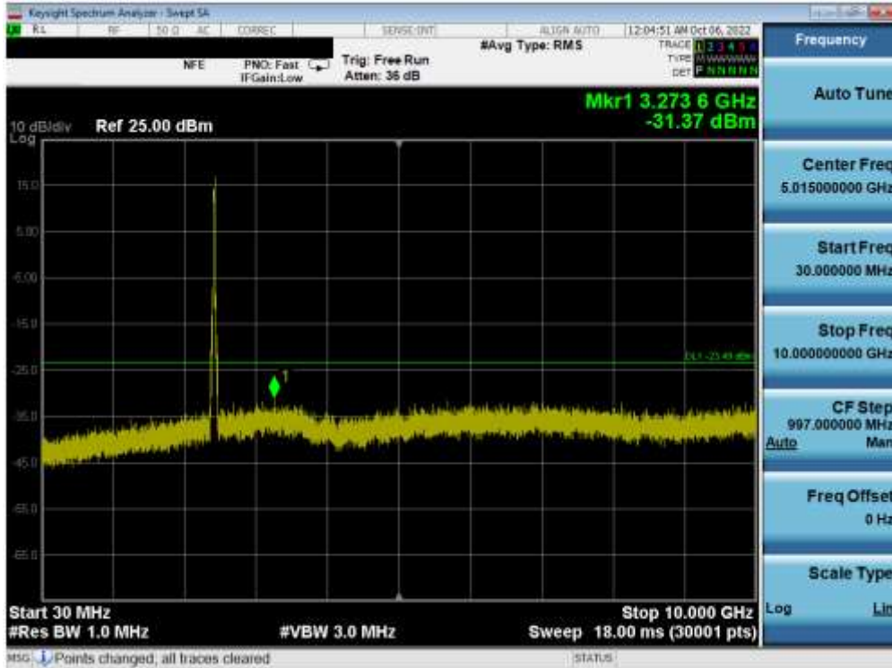
Plot 7-78. Conducted Spurious Plot SISO ANT2 (802.11ax OFDMA – 242 Tones – Ch. 6)
