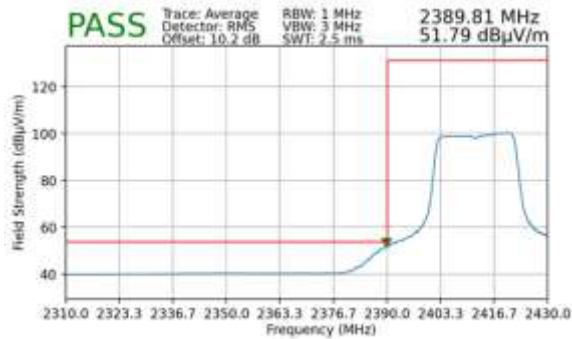
Plot 7-152. Radiated Restricted Lower Band Edge Measurement MIMO (Average – 242 Tones)
