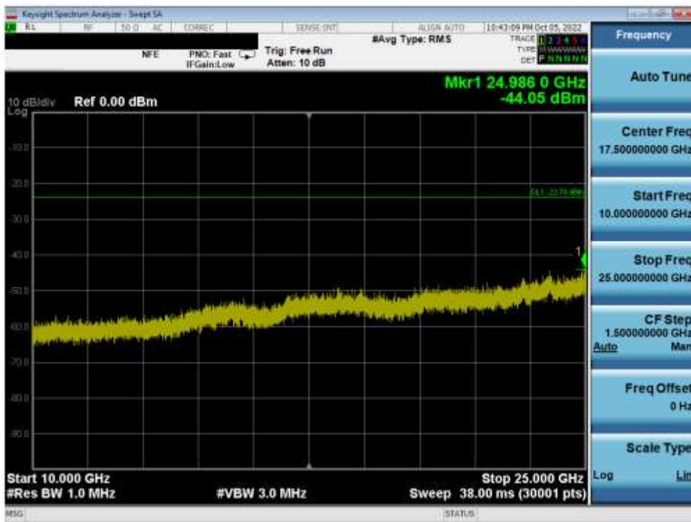
Plot 7-101. Conducted Spurious Plot MIMO ANT2 (802.11ax OFDMA – 242 Tones – Ch. 1)
