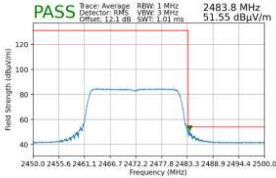
Plot 7-164. Radiated Restricted Upper Band Edge Measurement MIMO (Average – 242 Tones)
