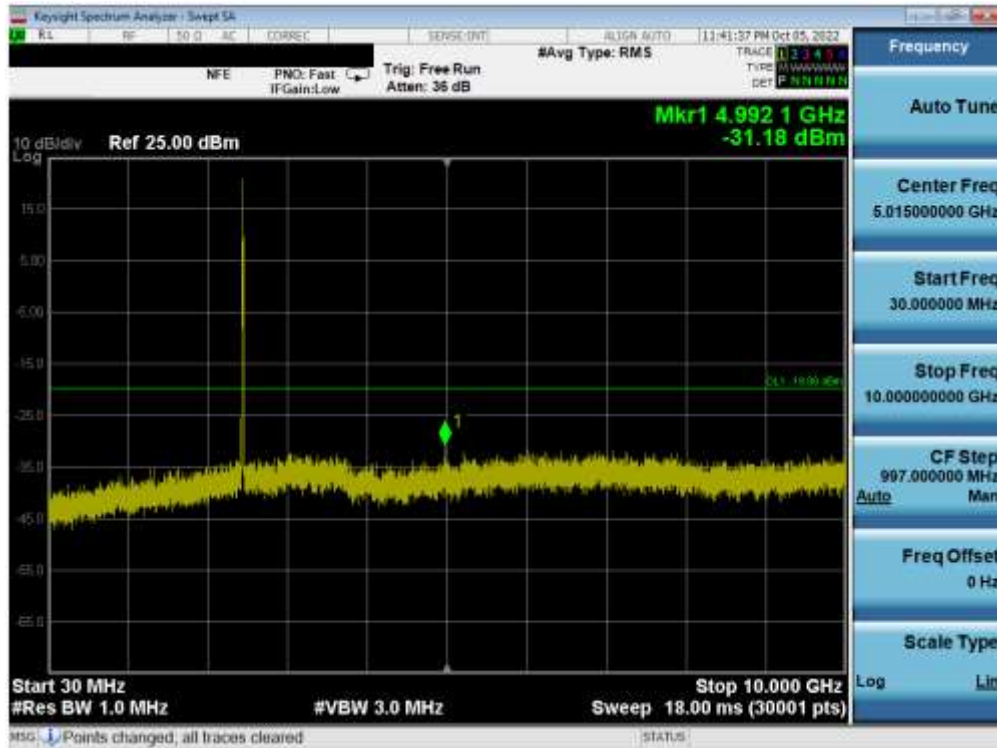
Plot 7-86. Conducted Spurious Plot MIMO ANT1 (802.11ax OFDMA – 26 Tones – Ch. 11)
