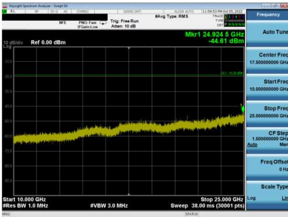
Plot 7-73. Conducted Spurious Plot SISO ANT2 (802.11ax OFDMA – 26 Tones – Ch. 6)
