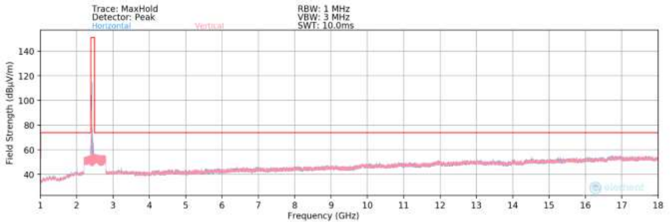
Plot 7-106. Radiated Spurious Plot above 1GHz SISO ANT2 (802.11ax OFDMA – 26 Tones – Ch. 1)
