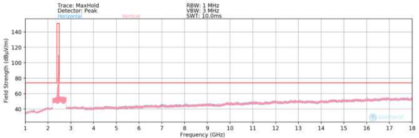
Plot 7-119. Radiated Spurious Plot above 1GHz MIMO (802.11ax OFDMA – 242 Tones – Ch. 11)
