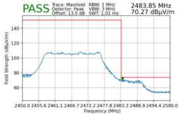
Plot 7-141. Radiated Restricted Upper Band Edge Measurement SISO ANT2 (Peak – 242 Tones)
