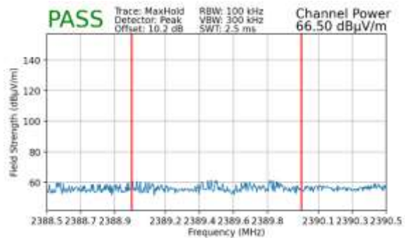
Plot 7-155. Radiated Restricted Lower Band Edge Measurement MIMO (Peak – 242 Tones)
