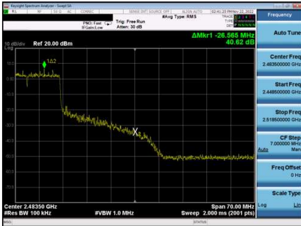
Plot 7-65. Band Edge Plot MIMO ANT2 (802.11ax OFDMA – 242 Tones – Ch. 9)
