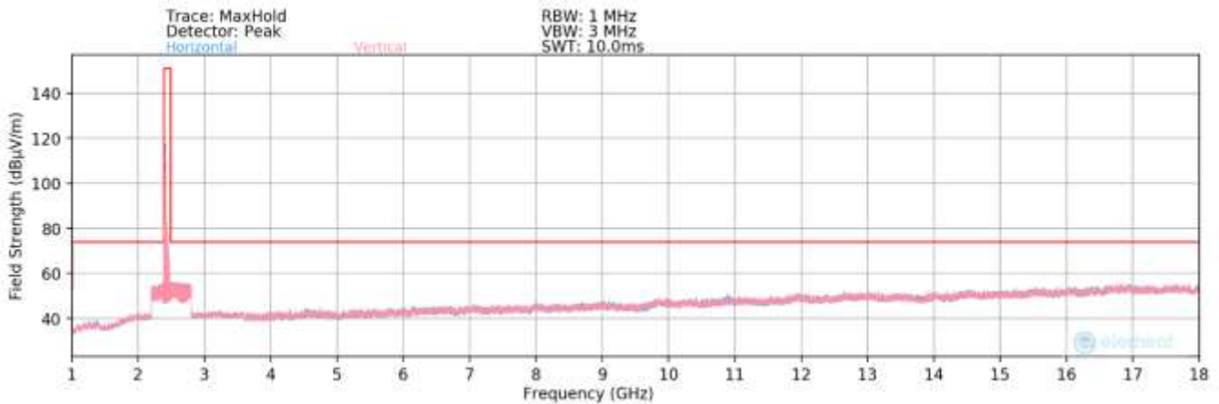
Plot 7-114. Radiated Spurious Plot above 1GHz MIMO (802.11ax OFDMA – 26 Tones – Ch. 1)
