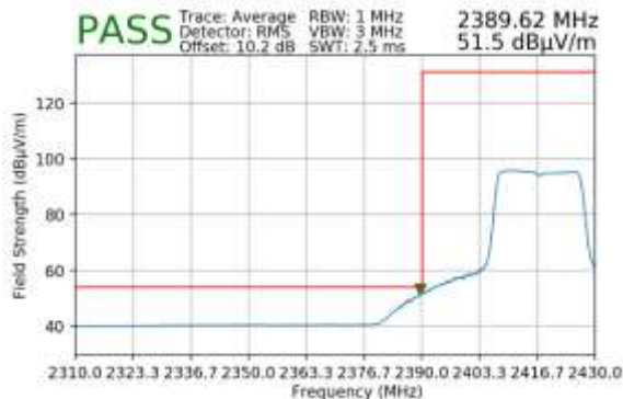
Plot 7-132. Radiated Restricted Lower Band Edge Measurement SISO ANT2 (Average – 242 Tones)
