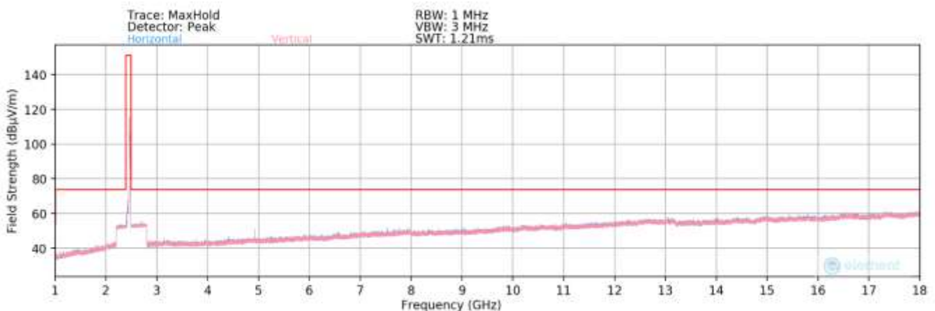
Plot 7-116. Radiated Spurious Plot above 1GHz MIMO (802.11ax OFDMA – 26 Tones – Ch. 11)
