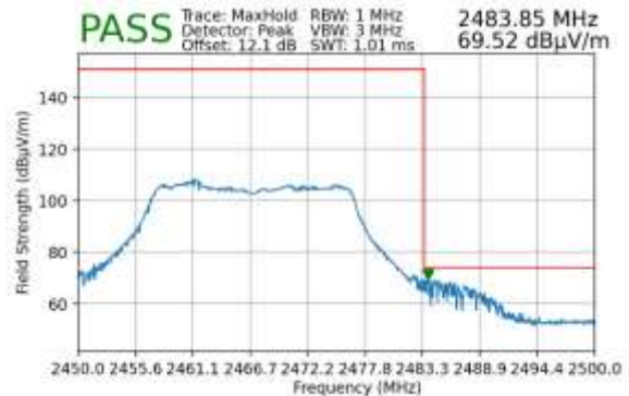
Plot 7-163. Radiated Restricted Upper Band Edge Measurement MIMO (Peak – 242 Tones)
