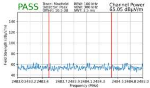
Plot 7-125. Radiated Restricted Upper Band Edge Measurement SISO ANT2 (Peak – 106 Tones)
