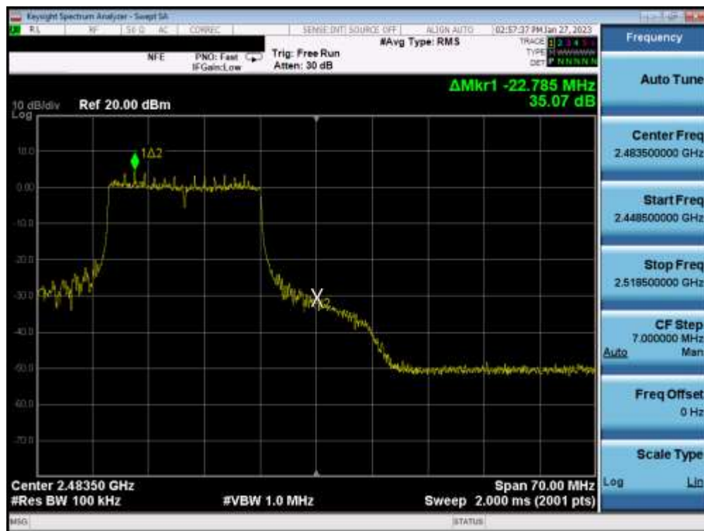
Plot 7-46. Band Edge Plot SISO ANT2 (802.11ax OFDMA – 242 Tones – Ch. 12)
