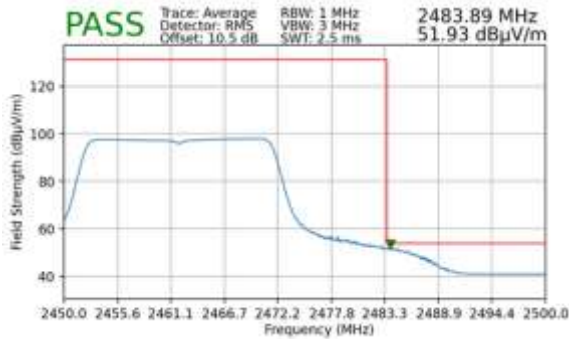
Plot 7-160. Radiated Restricted Upper Band Edge Measurement MIMO (Average – 242 Tones)
