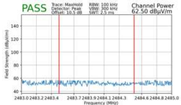
Plot 7-159. Radiated Restricted Upper Band Edge Measurement MIMO (Peak – 242 Tones)
