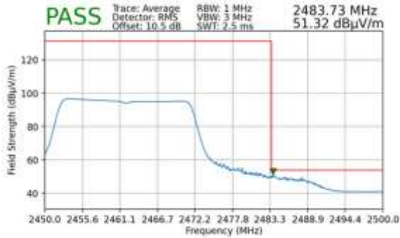
Plot 7-138. Radiated Restricted Upper Band Edge Measurement SISO ANT2 (Average – 242 Tones)
