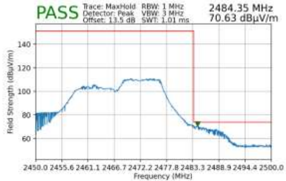
Plot 7-127. Radiated Restricted Upper Band Edge Measurement SISO ANT2 (Peak – 106 Tones)
