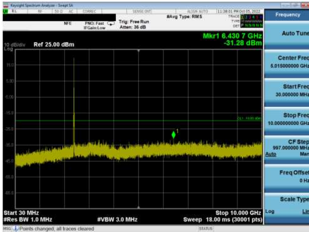
Plot 7-82. Conducted Spurious Plot MIMO ANT1 (802.11ax OFDMA – 26 Tones – Ch. 1)
