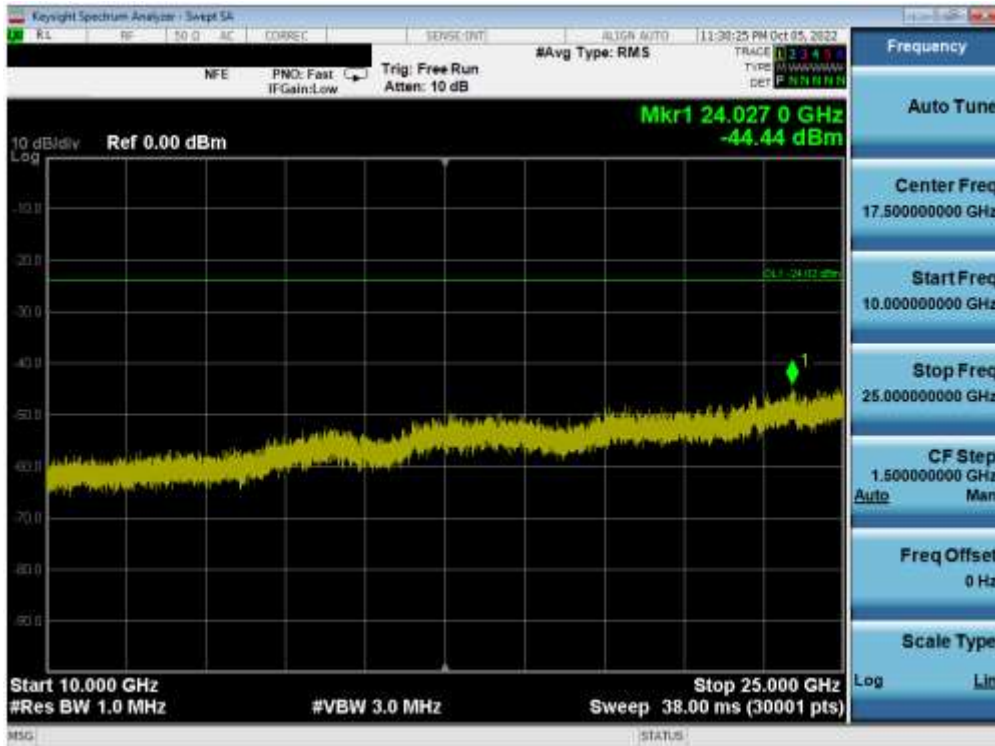
Plot 7-105. Conducted Spurious Plot MIMO ANT2 (802.11ax OFDMA – 242 Tones – Ch. 11)
