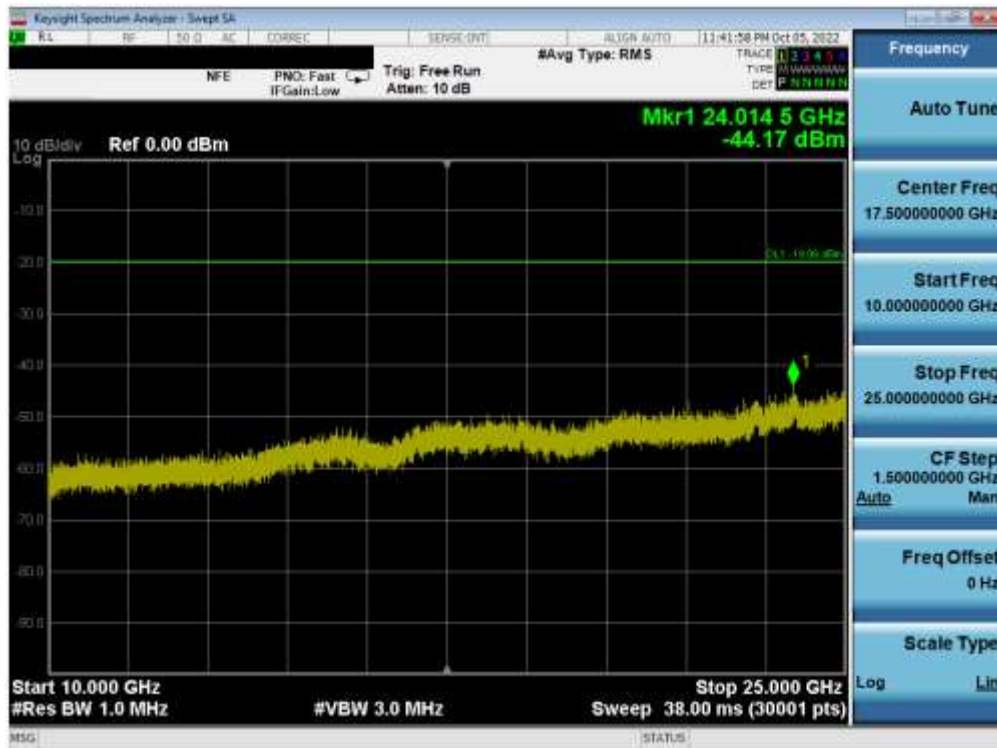
Plot 7-87. Conducted Spurious Plot MIMO ANT1 (802.11ax OFDMA – 26 Tones – Ch. 11)
