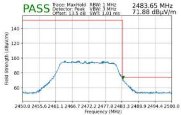
Plot 7-143. Radiated Restricted Upper Band Edge Measurement SISO ANT2 (Peak – 242 Tones)
