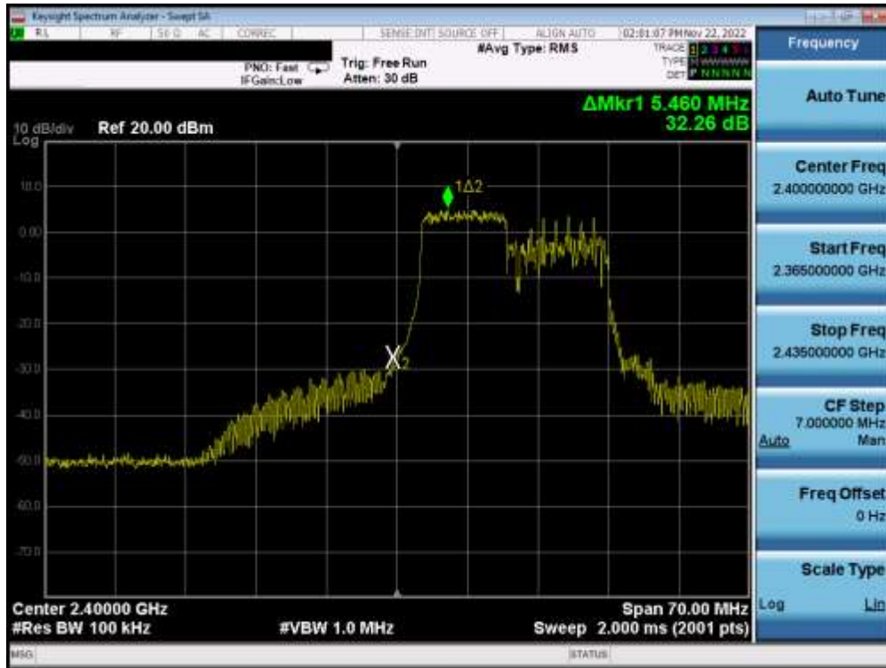
Plot 7-59. Band Edge Plot MIMO ANT2 (802.11ax OFDMA – 106 Tones – Ch. 1)
