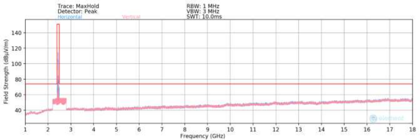
Plot 7-107. Radiated Spurious Plot above 1GHz SISO ANT2 (802.11ax OFDMA – 26 Tones – Ch. 6)
