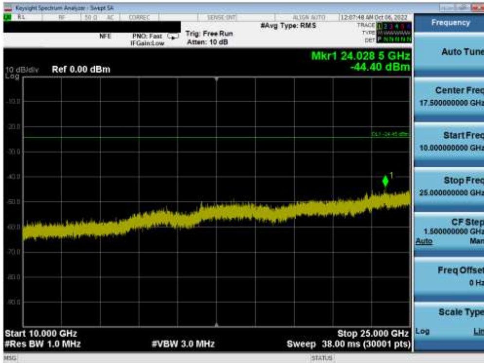
Plot 7-81. Conducted Spurious Plot SISO ANT2 (802.11ax OFDMA – 242 Tones – Ch. 11)
