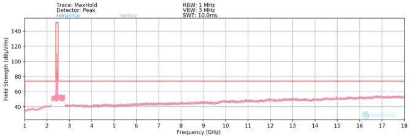
Plot 7-118. Radiated Spurious Plot above 1GHz MIMO (802.11ax OFDMA – 242 Tones – Ch. 6)
