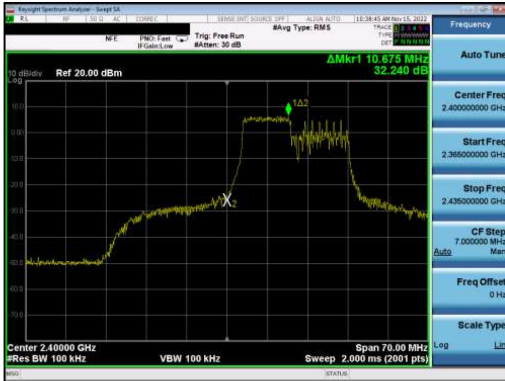
Plot 7-48. Band Edge Plot MIMO ANT1 (802.11ax OFDMA – 106 Tones – Ch. 1)
