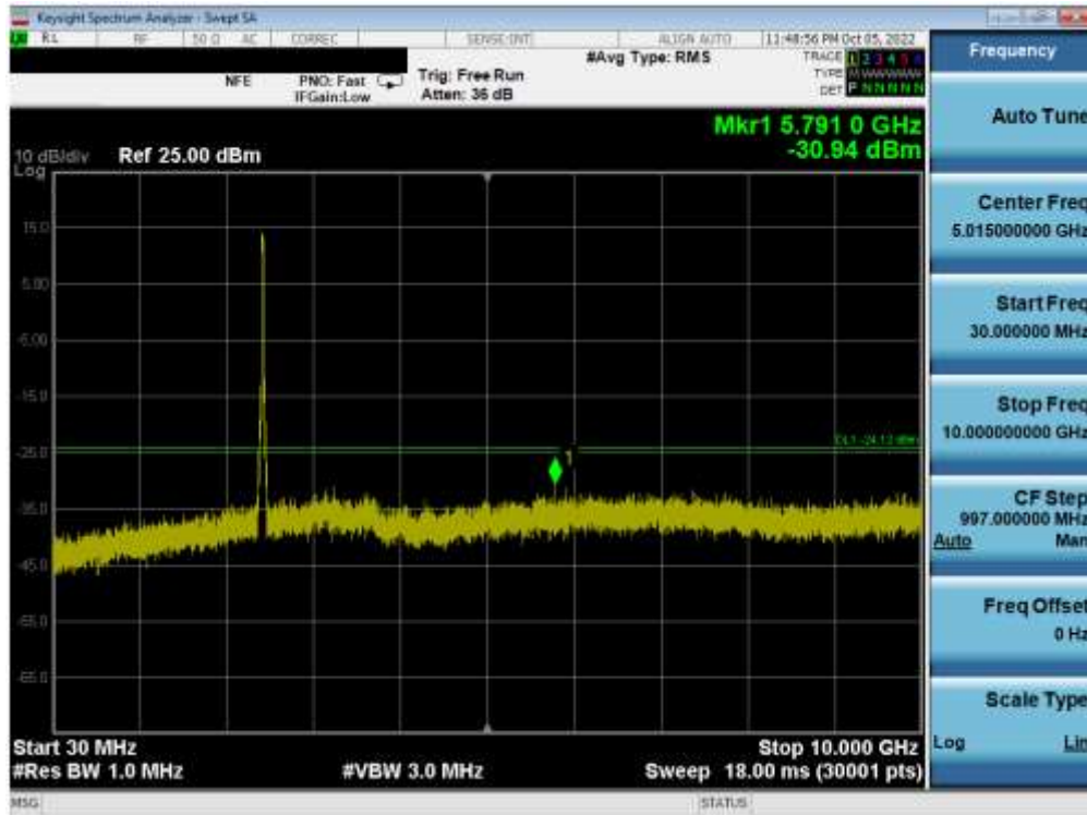
Plot 7-90. Conducted Spurious Plot MIMO ANT1 (802.11ax OFDMA – 242 Tones – Ch. 6)
