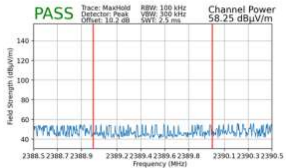
Plot 7-145. Radiated Restricted Lower Band Edge Measurement MIMO (Peak – 106 Tones)
