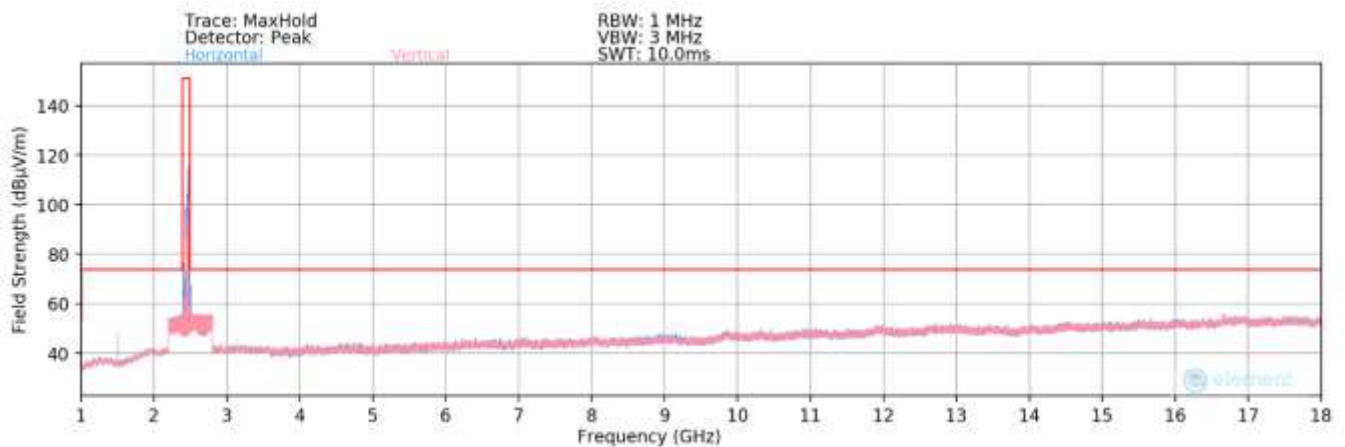
Plot 7-108. Radiated Spurious Plot above 1GHz SISO ANT2 (802.11ax OFDMA – 26 Tones – Ch. 11)
