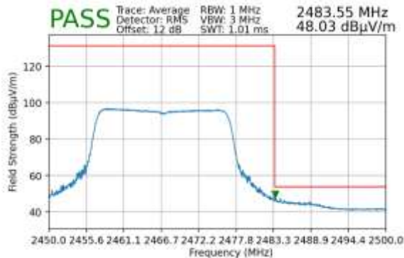
Plot 7-162. Radiated Restricted Upper Band Edge Measurement MIMO (Average – 242 Tones)
