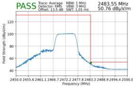
Plot 7-126. Radiated Restricted Upper Band Edge Measurement SISO ANT2 (Average – 106 Tones)
