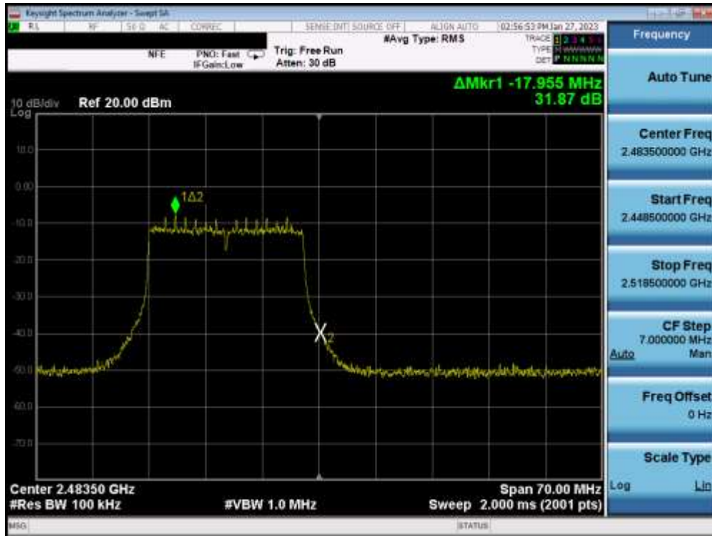
Plot 7-47. Band Edge Plot SISO ANT2 (802.11ax OFDMA – 242 Tones – Ch. 13)
