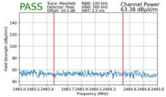
Plot 7-139. Radiated Restricted Upper Band Edge Measurement SISO ANT2 (Peak – 242 Tones)
