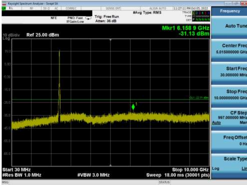
Plot 7-102. Conducted Spurious Plot MIMO ANT2 (802.11ax OFDMA – 242 Tones – Ch. 6)
