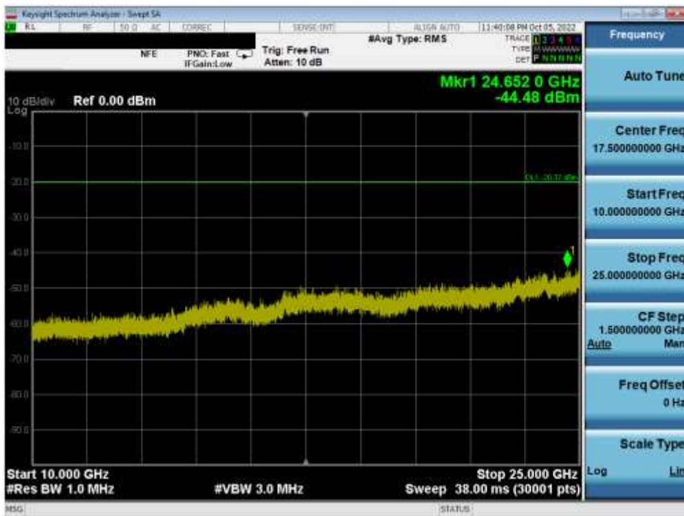
Plot 7-85. Conducted Spurious Plot MIMO ANT1 (802.11ax OFDMA – 26 Tones – Ch. 6)
