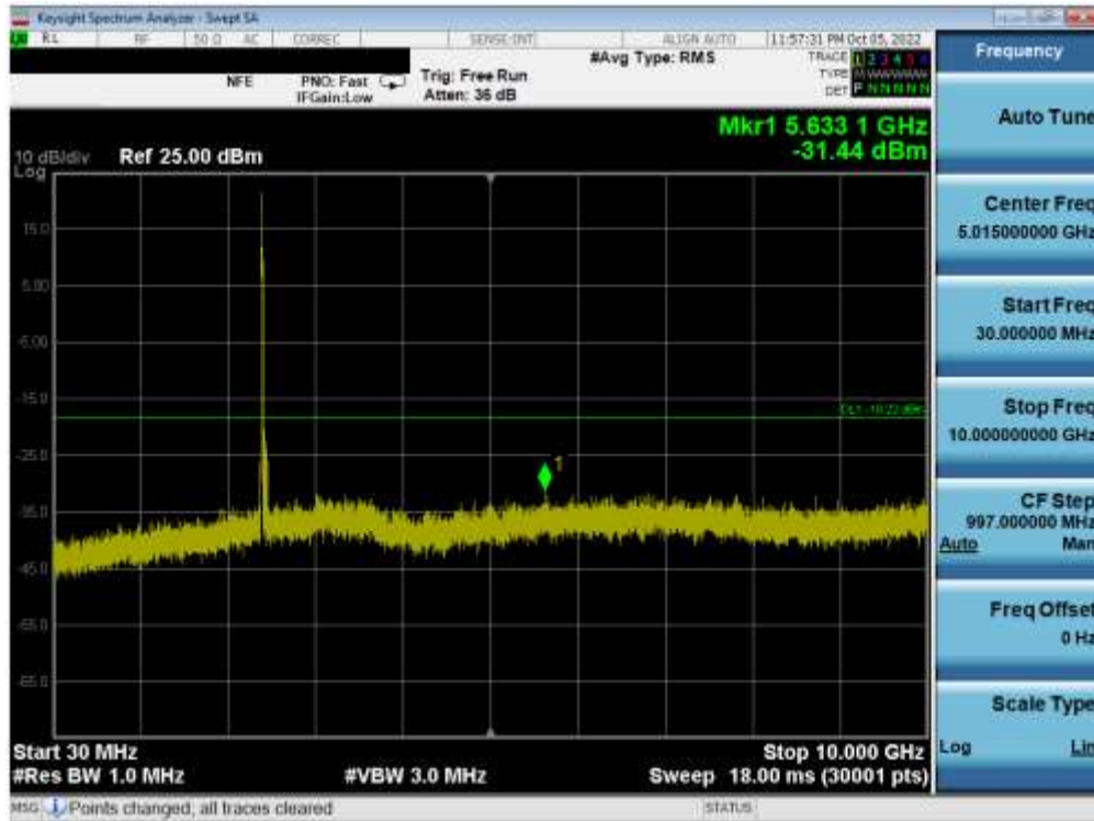
Plot 7-70. Conducted Spurious Plot SISO ANT2 (802.11ax OFDMA – 26 Tones – Ch. 1)
