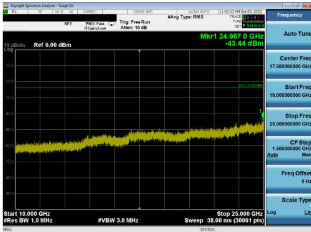
Plot 7-93. Conducted Spurious Plot MIMO ANT1 (802.11ax OFDMA – 242 Tones – Ch. 11)
