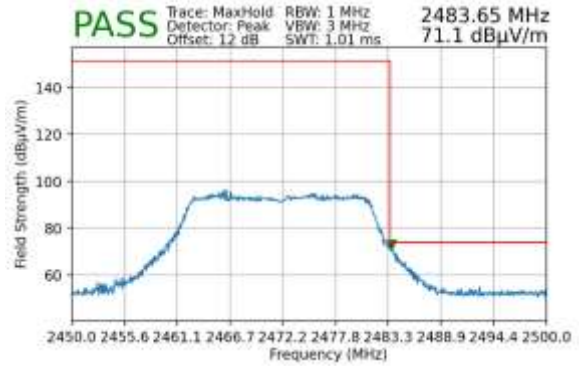
Plot 7-165. Radiated Restricted Upper Band Edge Measurement MIMO (Peak – 242 Tones)
