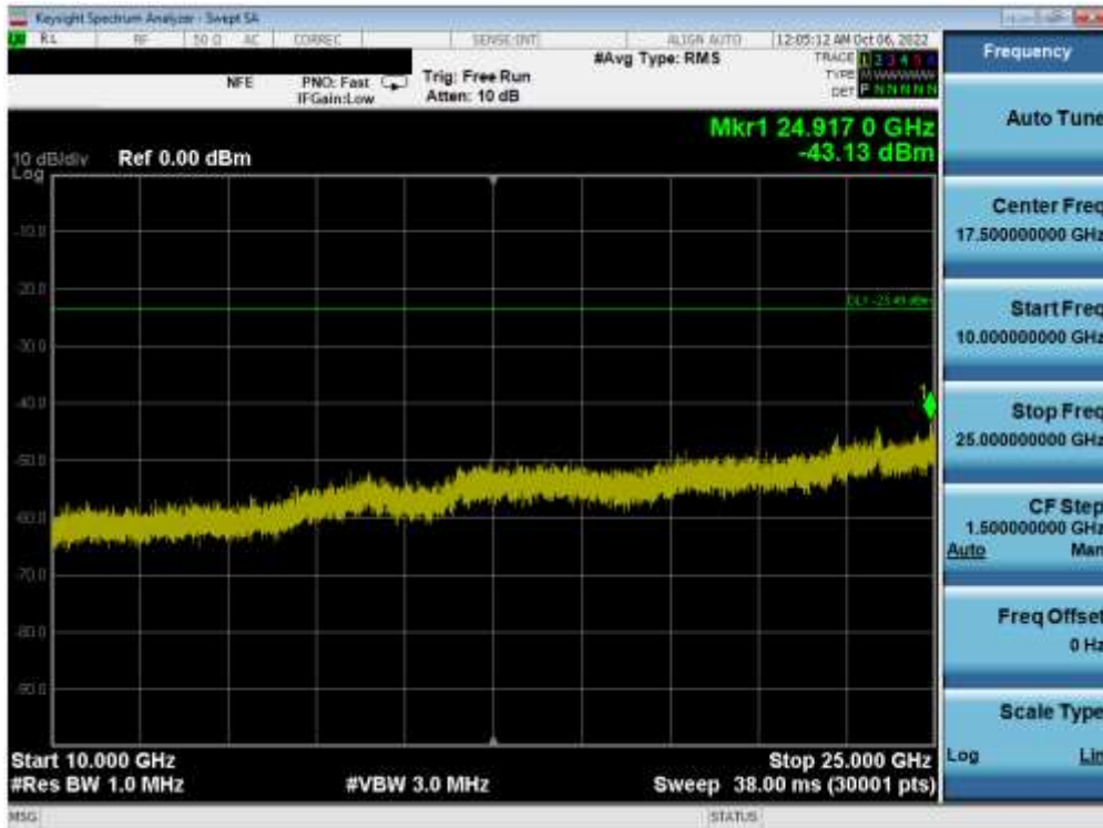
Plot 7-79. Conducted Spurious Plot SISO ANT2 (802.11ax OFDMA – 242 Tones – Ch. 6)
