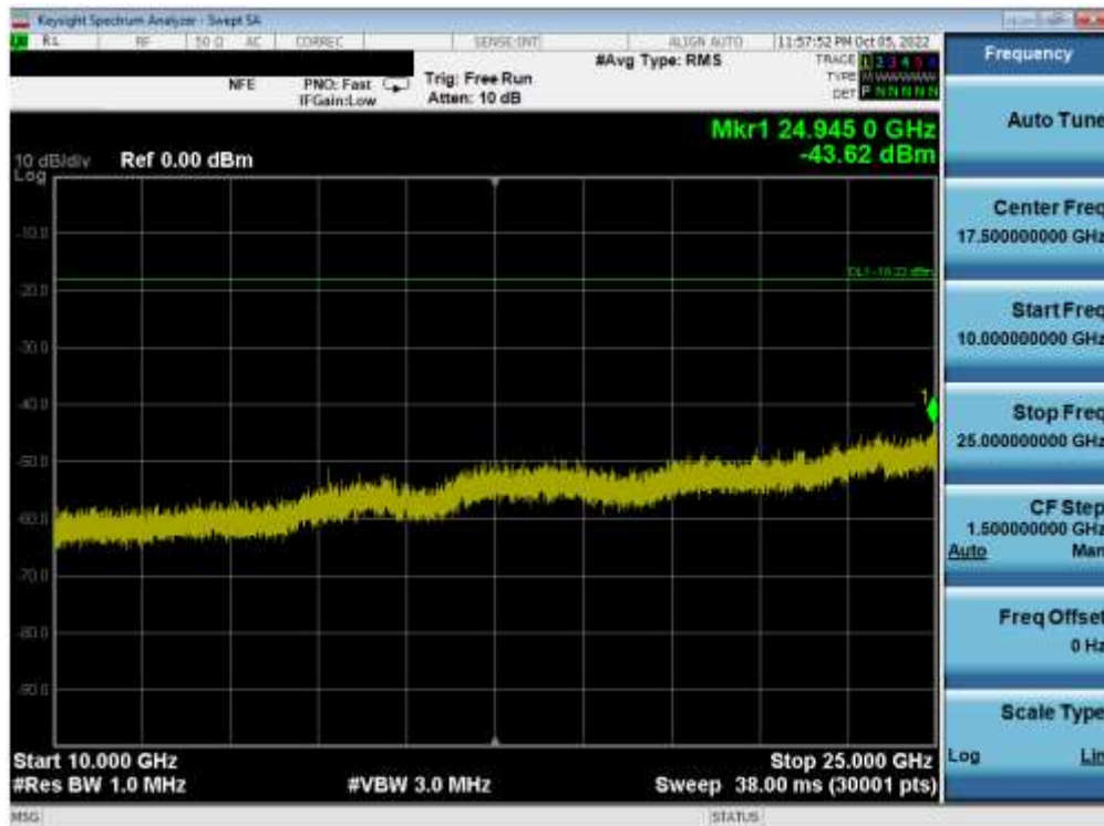
Plot 7-71. Conducted Spurious Plot SISO ANT2 (802.11ax OFDMA – 26 Tones – Ch. 1)
