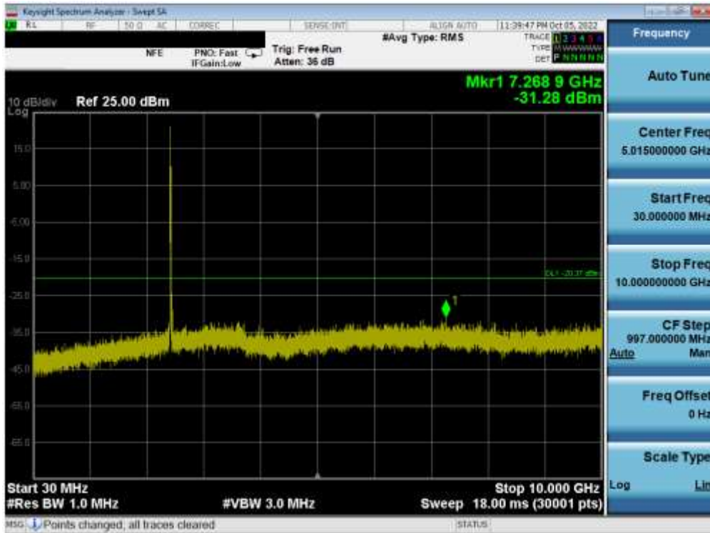
Plot 7-84. Conducted Spurious Plot MIMO ANT1 (802.11ax OFDMA – 26 Tones – Ch. 6)
