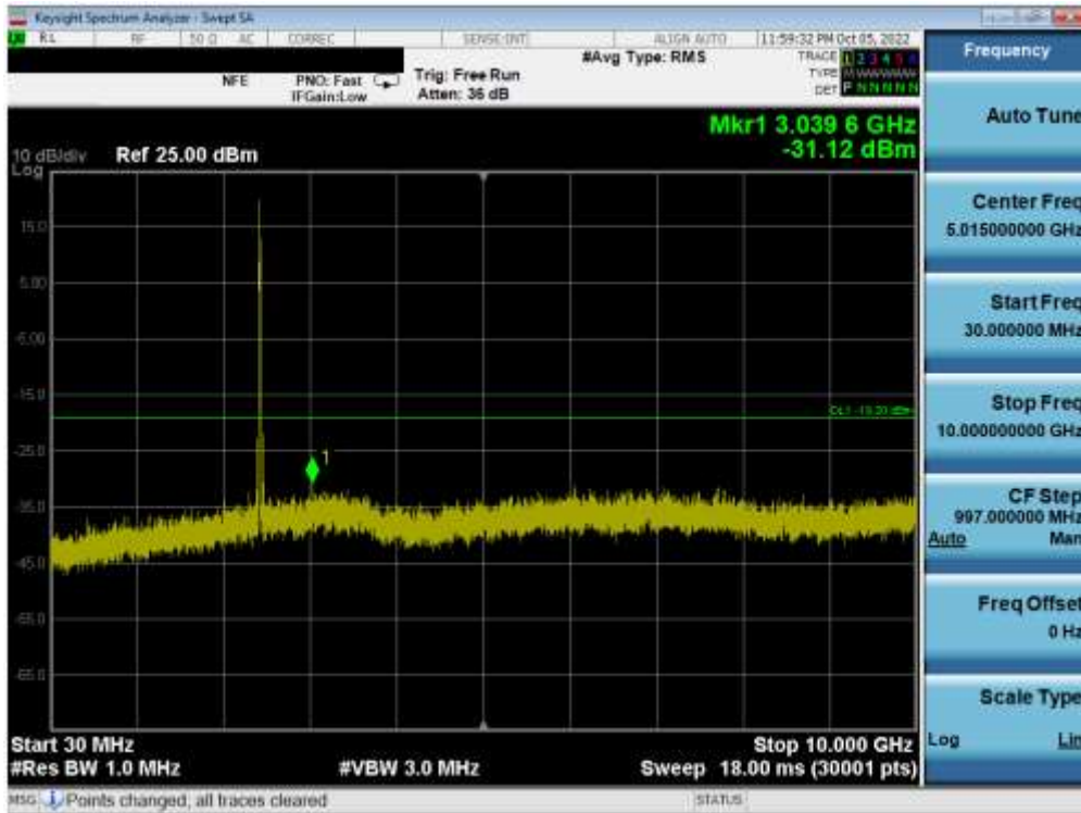
Plot 7-72. Conducted Spurious Plot SISO ANT2 (802.11ax OFDMA – 26 Tones – Ch. 6)
