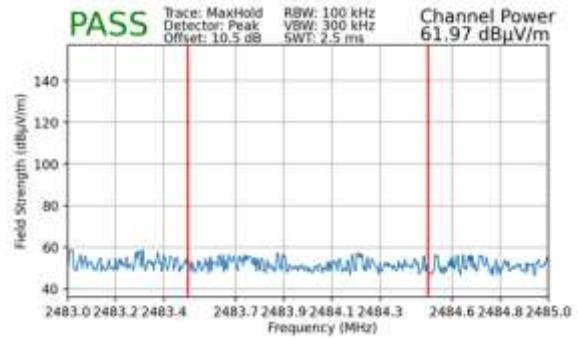
Plot 7-161. Radiated Restricted Upper Band Edge Measurement MIMO (Peak – 242 Tones)
