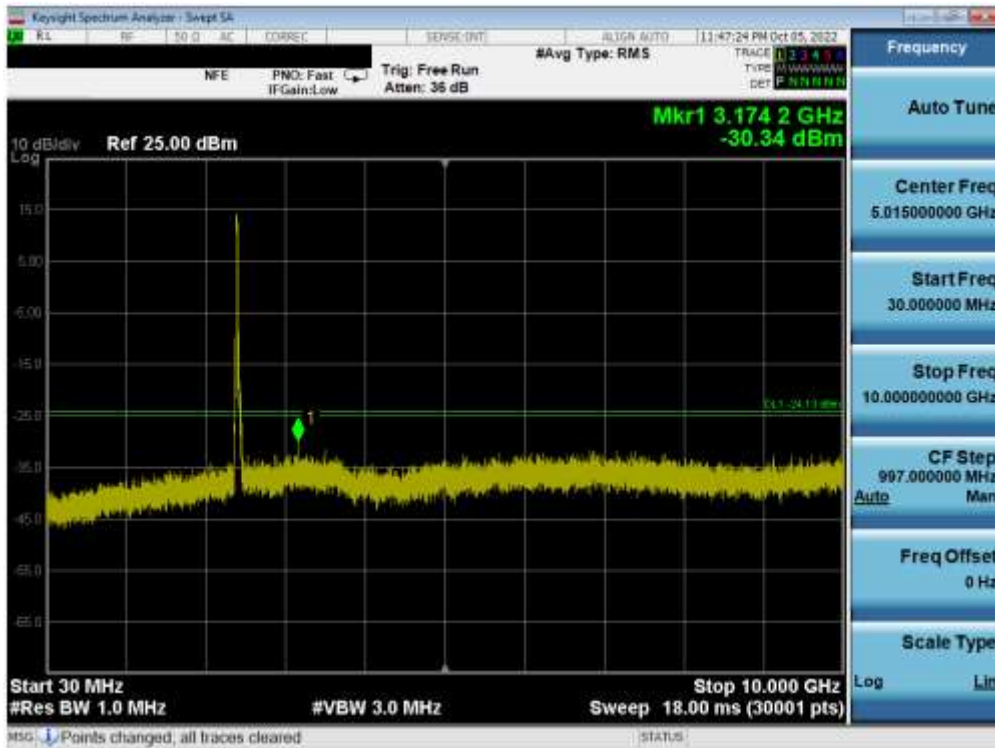
Plot 7-88. Conducted Spurious Plot MIMO ANT1 (802.11ax OFDMA – 242 Tones – Ch. 1)
