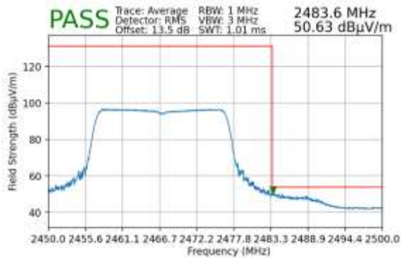
Plot 7-140. Radiated Restricted Upper Band Edge Measurement SISO ANT2 (Average – 242 Tones)
