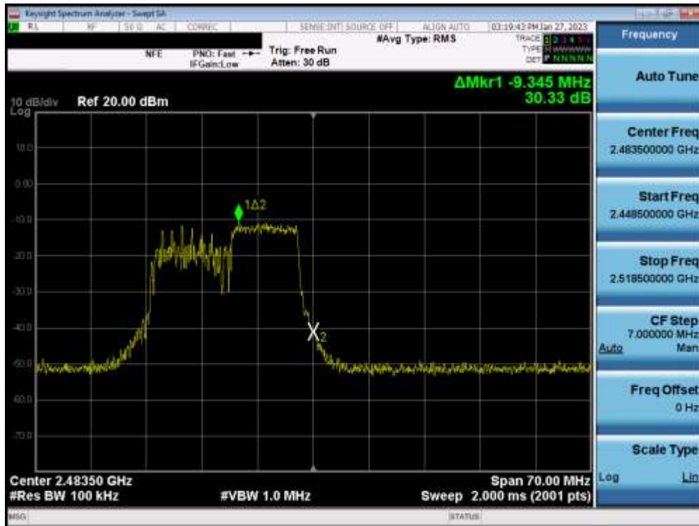
Plot 7-51. Band Edge Plot MIMO ANT1 (802.11ax OFDMA – 106 Tones – Ch. 11)
