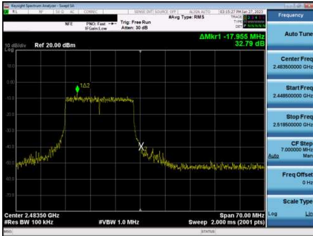
Plot 7-69. Band Edge Plot MIMO ANT2 (802.11ax OFDMA – 242 Tones – Ch. 13)
