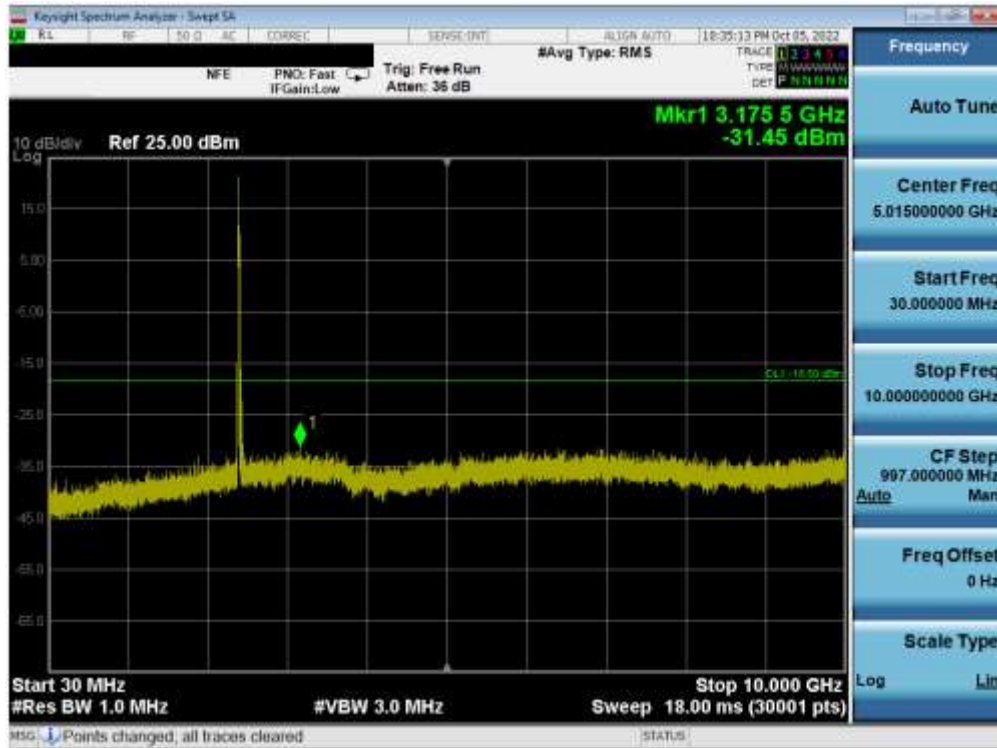
Plot 7-94. Conducted Spurious Plot MIMO ANT2 (802.11ax OFDMA – 26 Tones – Ch. 1)
