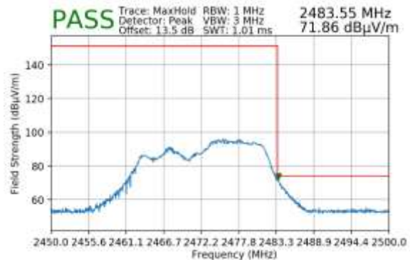
Plot 7-151. Radiated Restricted Upper Band Edge Measurement MIMO (Peak – 106 Tones)
