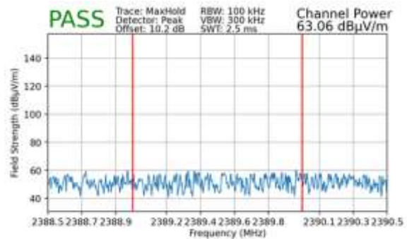
Plot 7-123. Radiated Restricted Lower Band Edge Measurement SISO ANT2 (Peak – 106 Tones)
