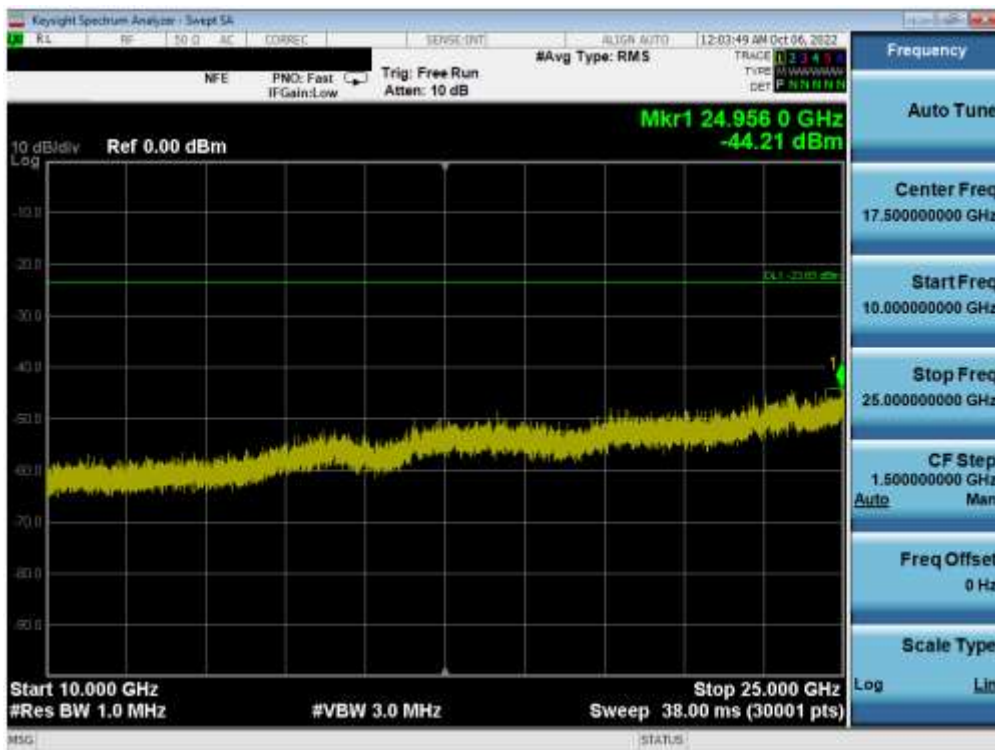
Plot 7-77. Conducted Spurious Plot SISO ANT2 (802.11ax OFDMA – 242 Tones – Ch. 1)
