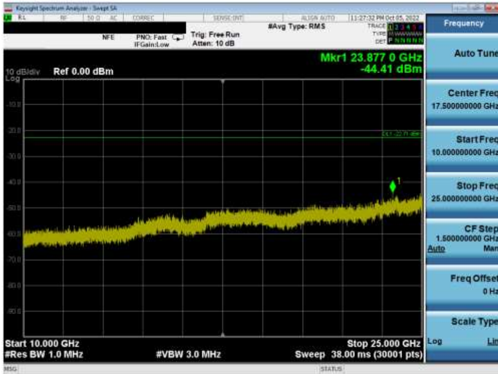
Plot 7-103. Conducted Spurious Plot MIMO ANT2 (802.11ax OFDMA – 242 Tones – Ch. 6)
