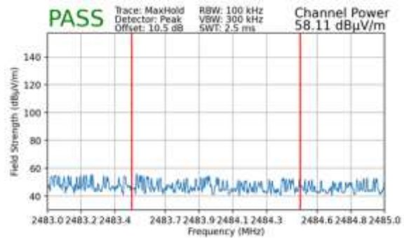
Plot 7-147. Radiated Restricted Upper Band Edge Measurement MIMO (Peak – 106 Tones)
