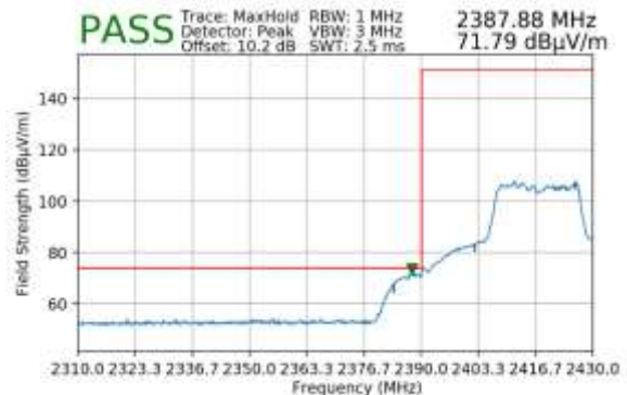
Plot 7-133. Radiated Restricted Lower Band Edge Measurement SISO ANT2 (Peak – 242 Tones)
