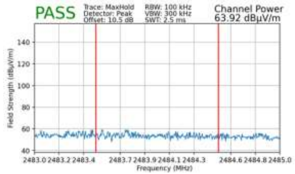
Plot 7-137. Radiated Restricted Upper Band Edge Measurement SISO ANT2 (Peak – 242 Tones)
