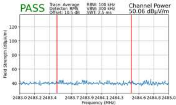
Plot 7-124. Radiated Restricted Upper Band Edge Measurement SISO ANT2 (Average – 106 Tones)
