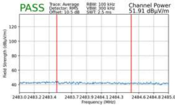
Plot 7-136. Radiated Restricted Upper Band Edge Measurement SISO ANT2 (Average – 242 Tones)
