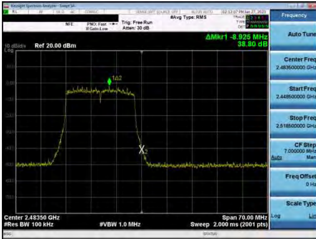
Plot 7-93. Band Edge Plot (802.11ax (2.4GHz) – Ch. 13) SISO ANT 2
