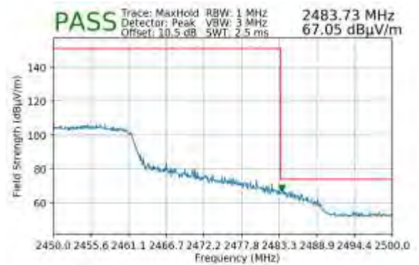
Plot 7-167. Radiated Restricted Upper Band Edge Measurement SISO ANT2 (Peak)
