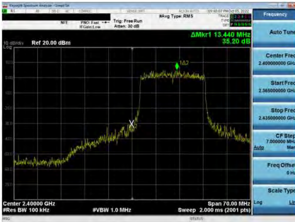
Plot 7-129. Band Edge Plot (802.11ax (2.4GHz) – Ch. 1) MIMO ANT 2
