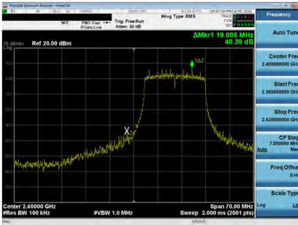
Plot 7-123. Band Edge Plot (802.11n (2.4GHz) – Ch. 1) MIMO ANT 2
