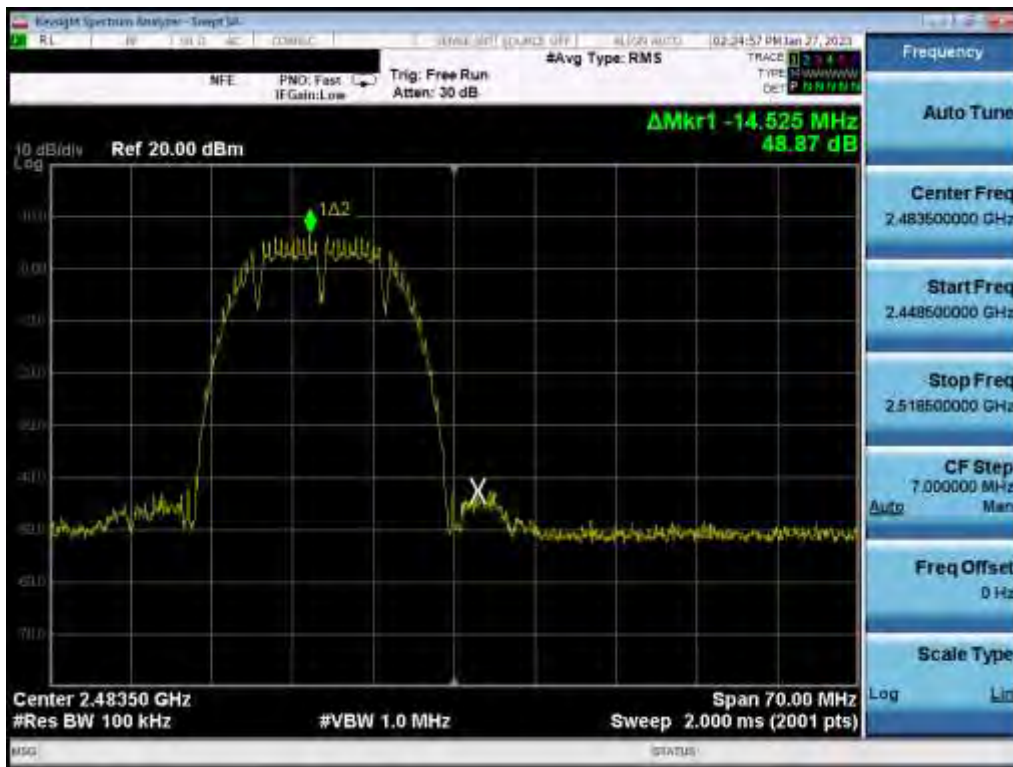
Plot 7-118. Band Edge Plot (802.11b – Ch. 13) MIMO ANT 2
