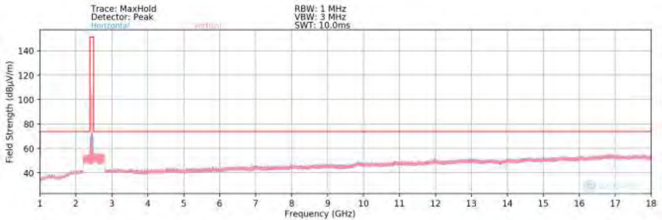
Plot 7-159. Radiated Spurious Plot above 1GHz (802.11b – Ch. 6) MIMO
