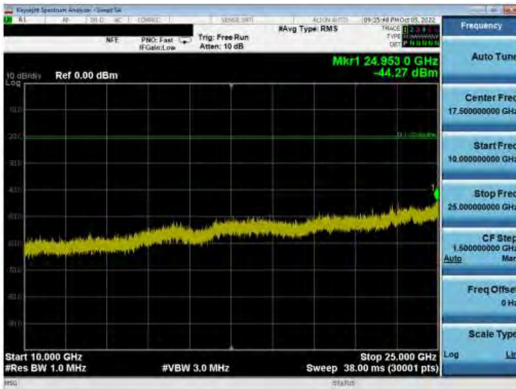
Plot 7-145. Conducted Spurious Plot (802.11b – Ch. 6) MIMO ANT 1
