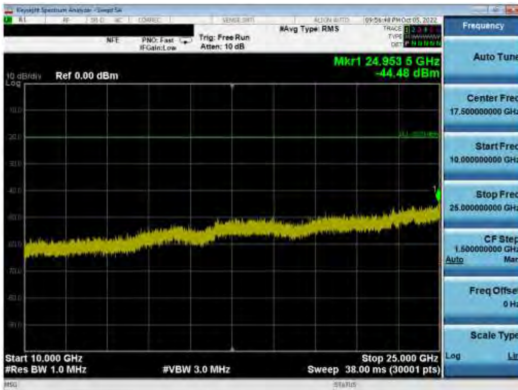
Plot 7-149. Conducted Spurious Plot (802.11b – Ch. 1) MIMO ANT 2
