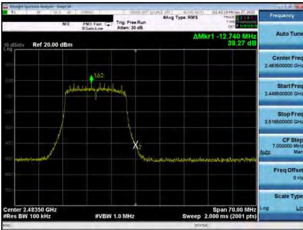
Plot 7-107. Band Edge Plot (802.11n (2.4GHz) – Ch. 13) MIMO ANT 1
