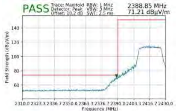
Plot 7-179. Radiated Restricted Lower Band Edge Measurement MIMO (Peak)
