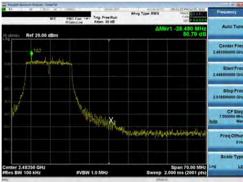
Plot 7-99. Band Edge Plot (802.11g – Ch. 11) MIMO ANT 1
