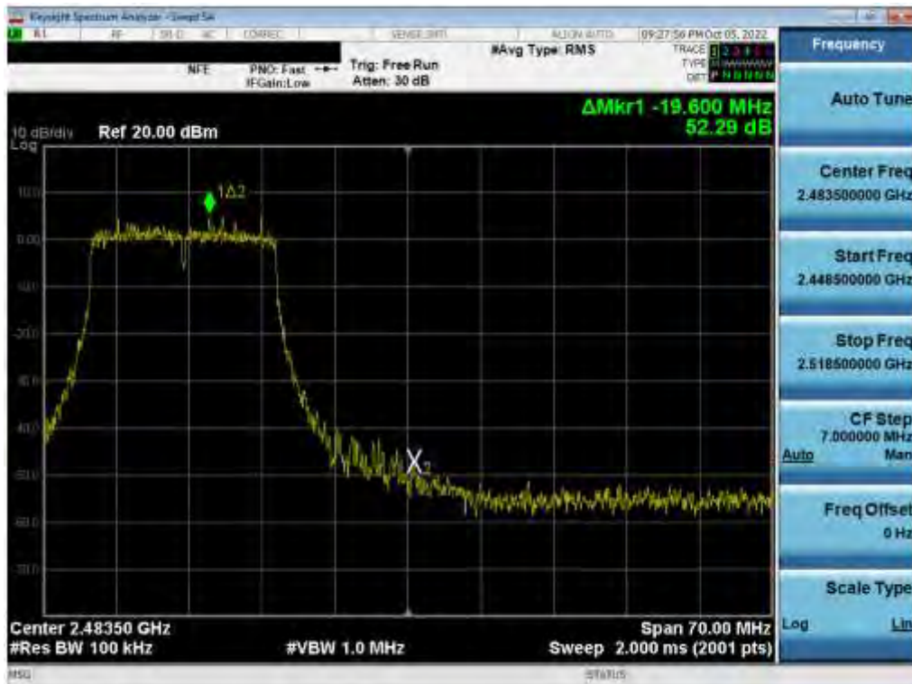
Plot 7-105. Band Edge Plot (802.11n (2.4GHz) – Ch. 11) MIMO ANT 1
