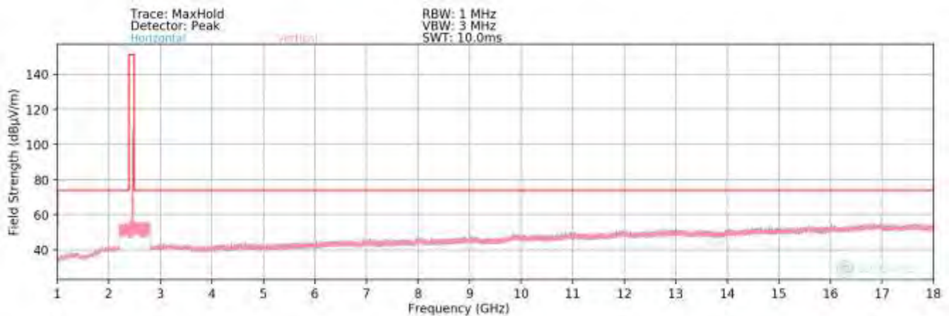
Plot 7-160. Radiated Spurious Plot above 1GHz (802.11b – Ch. 11) MIMO
