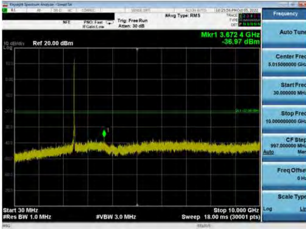
Plot 7-140. Conducted Spurious Plot (802.11b – Ch. 11) SISO ANT 2
