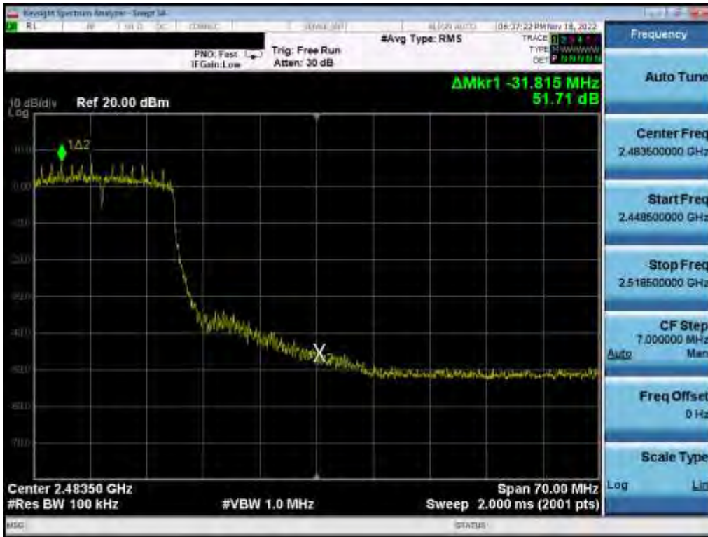
Plot 7-83. Band Edge Plot (802.11n (2.4GHz) – Ch. 10) SISO ANT 2
