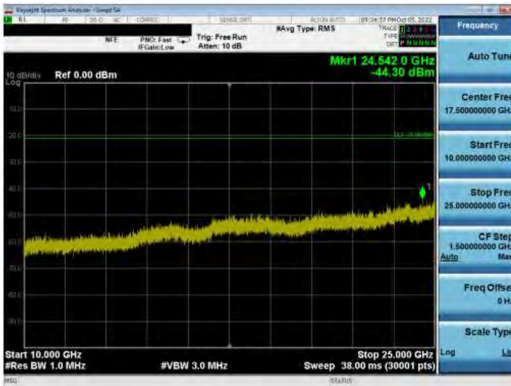
Plot 7-143. Conducted Spurious Plot (802.11b – Ch. 1) MIMO ANT 1
