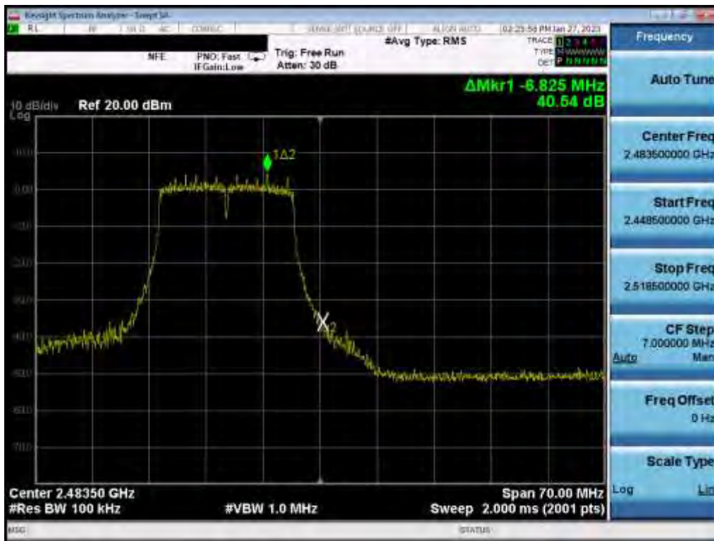
Plot 7-122. Band Edge Plot (802.11g – Ch. 13) MIMO ANT 2
