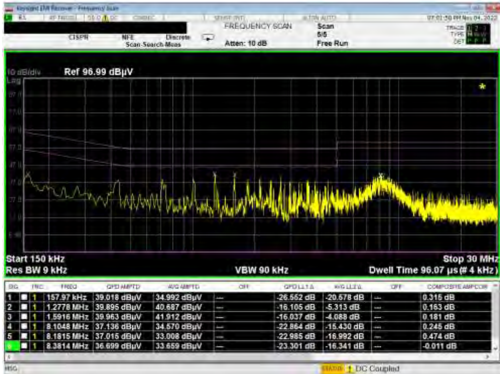
Plot 7-196. Line Conducted Plot with 802.11b (N) with WCP
