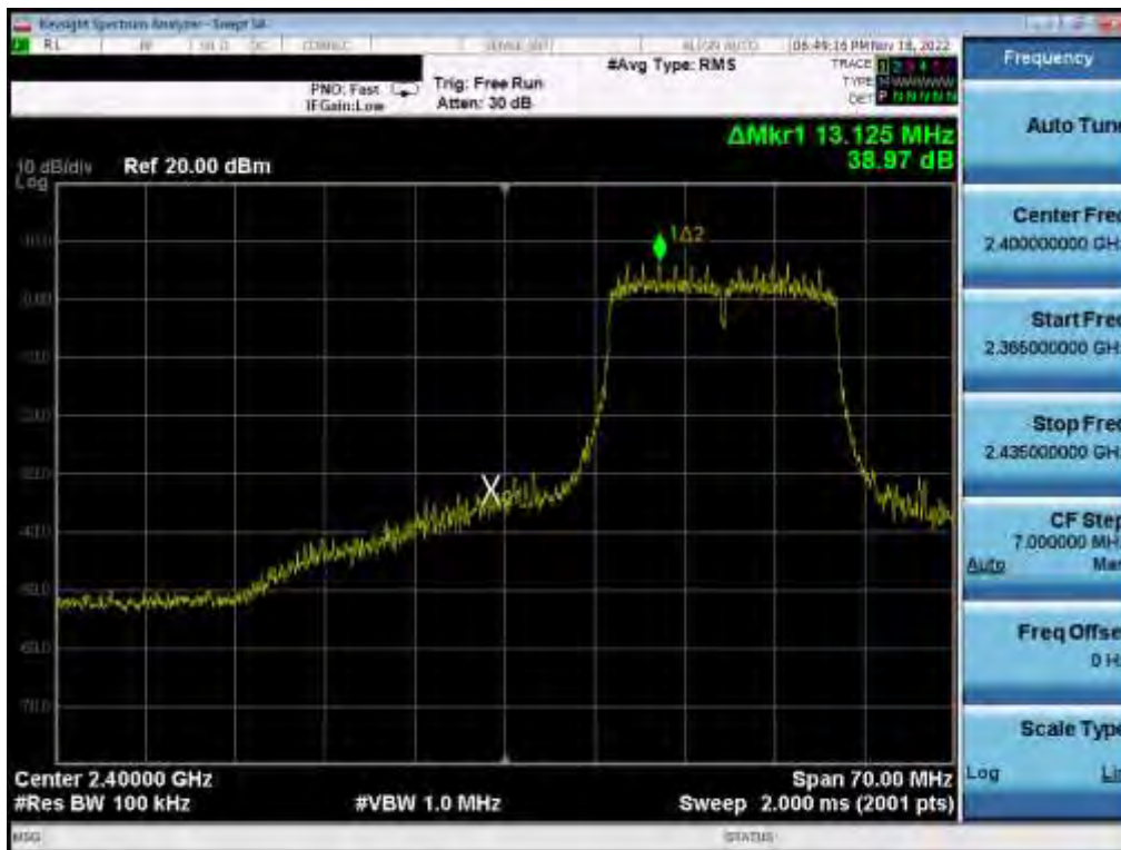
Plot 7-124. Band Edge Plot (802.11n (2.4GHz) – Ch. 2) MIMO ANT 2
