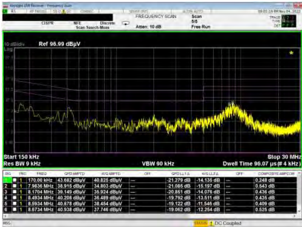
Plot 7-193. Line Conducted Plot with 802.11b (L1)
