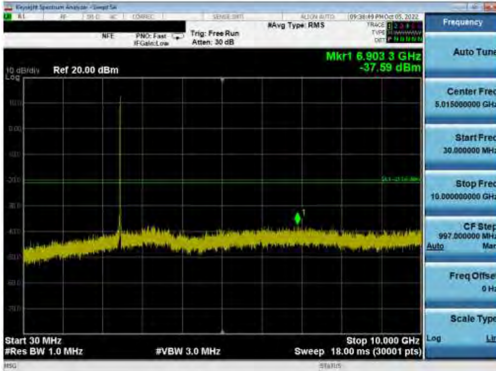
Plot 7-146. Conducted Spurious Plot (802.11b – Ch. 11) MIMO ANT 1
