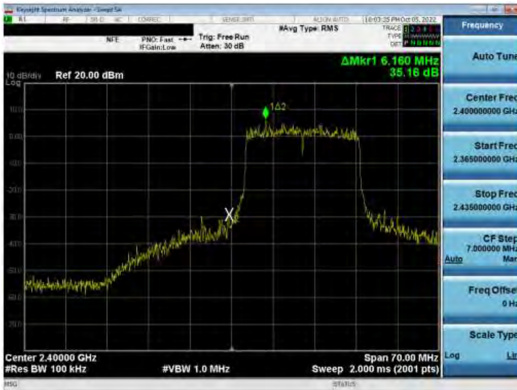
Plot 7-87. Band Edge Plot (802.11ax (2.4GHz) – Ch. 1) SISO ANT 2
