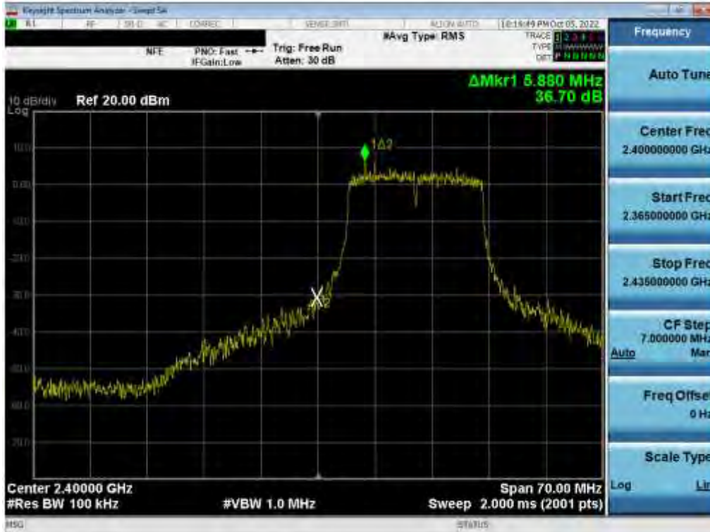
Plot 7-77. Band Edge Plot (802.11g– Ch. 1) SISO ANT 2
