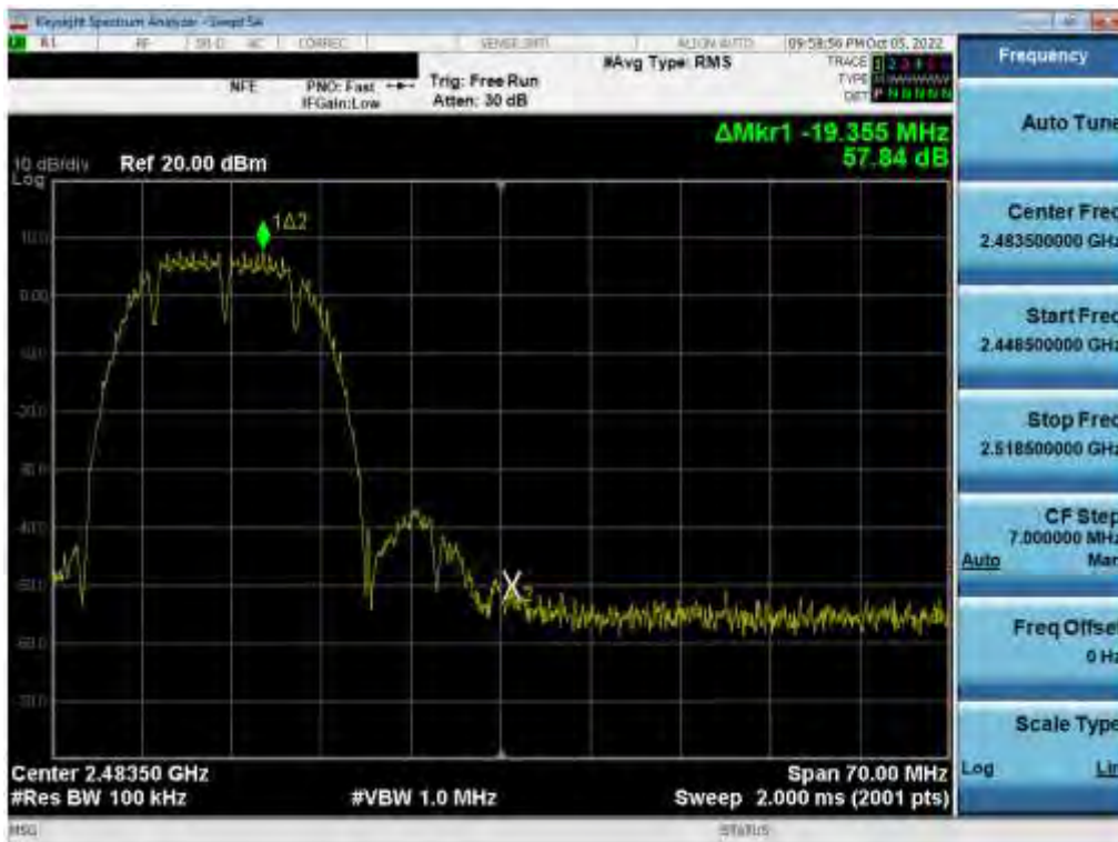
Plot 7-116. Band Edge Plot (802.11b – Ch. 11) MIMO ANT 2
