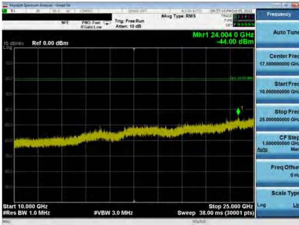
Plot 7-147. Conducted Spurious Plot (802.11b – Ch. 11) MIMO ANT 1
