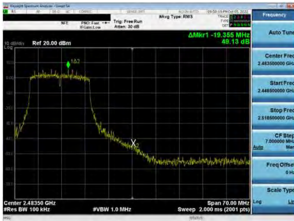
Plot 7-126. Band Edge Plot (802.11n (2.4GHz) – Ch. 11) MIMO ANT 2
