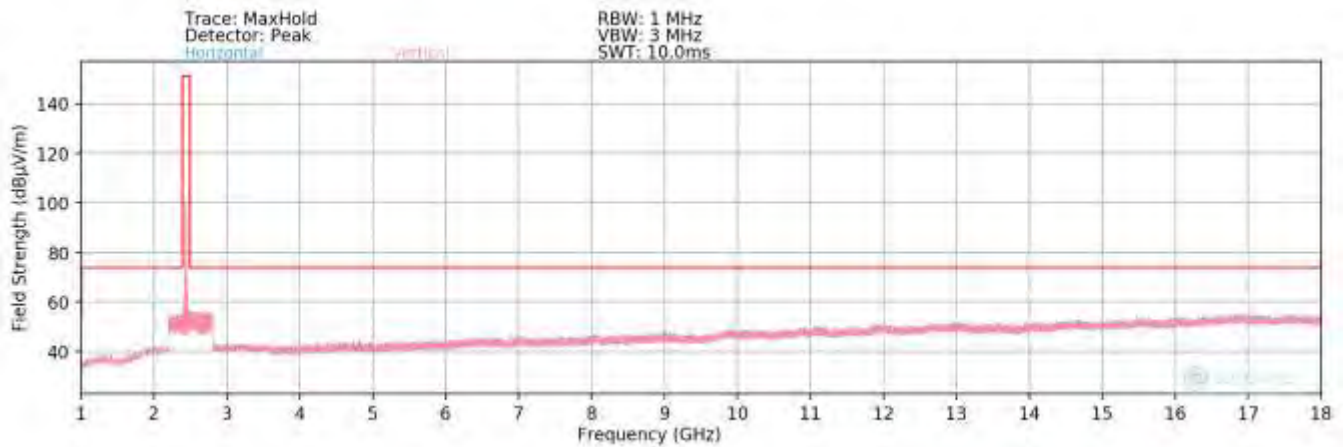
Plot 7-155. Radiated Spurious Plot above 1GHz (802.11b – Ch. 6) SISO ANT 2
