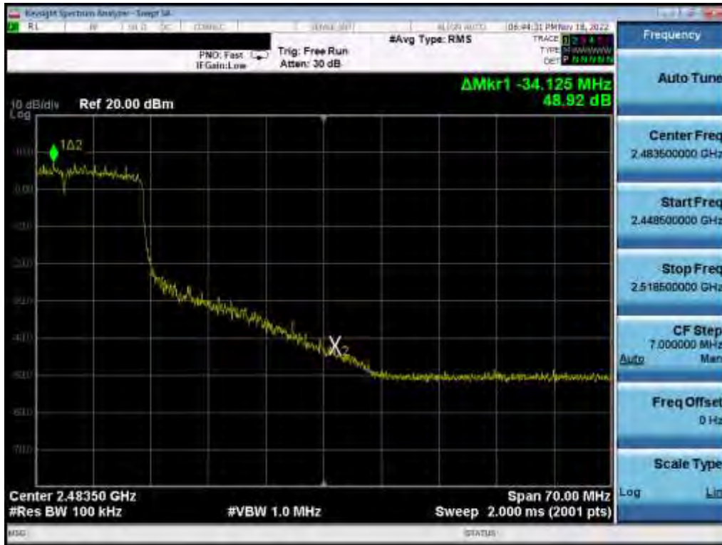
Plot 7-110. Band Edge Plot (802.11ax (2.4GHz) – Ch. 9) MIMO ANT 1
