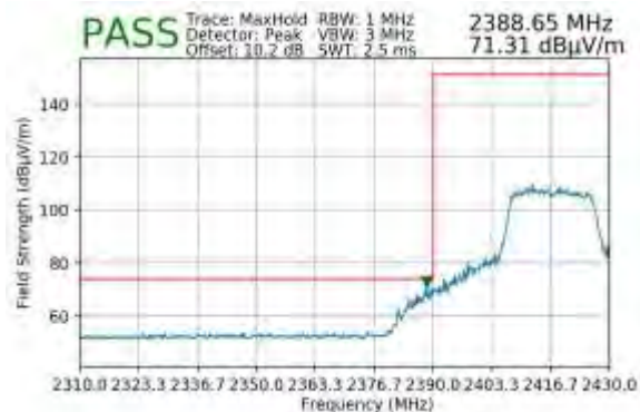
Plot 7-165. Radiated Restricted Lower Band Edge Measurement SISO ANT2 (Peak)
