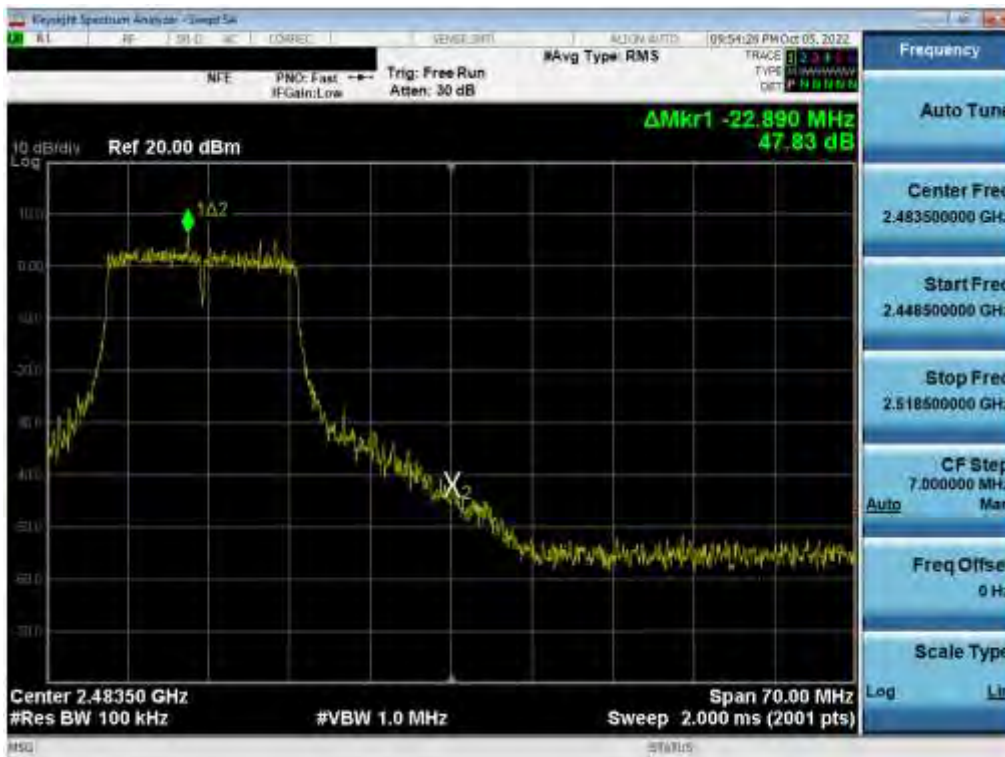
Plot 7-120. Band Edge Plot (802.11g – Ch. 11) MIMO ANT 2
