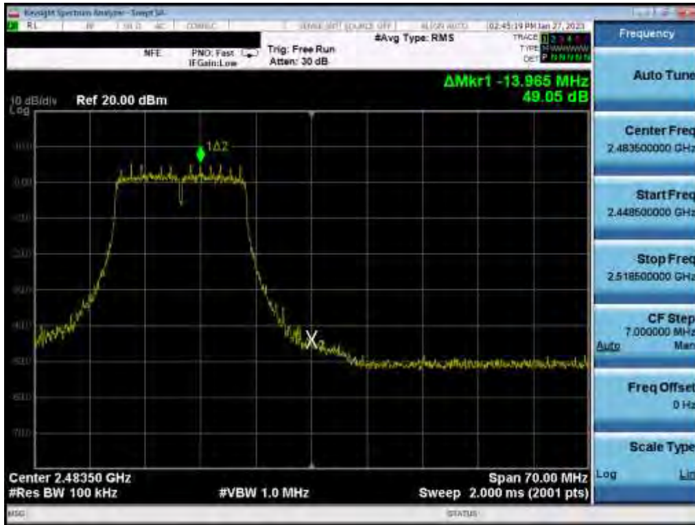
Plot 7-100. Band Edge Plot (802.11g – Ch. 12) MIMO ANT 1
