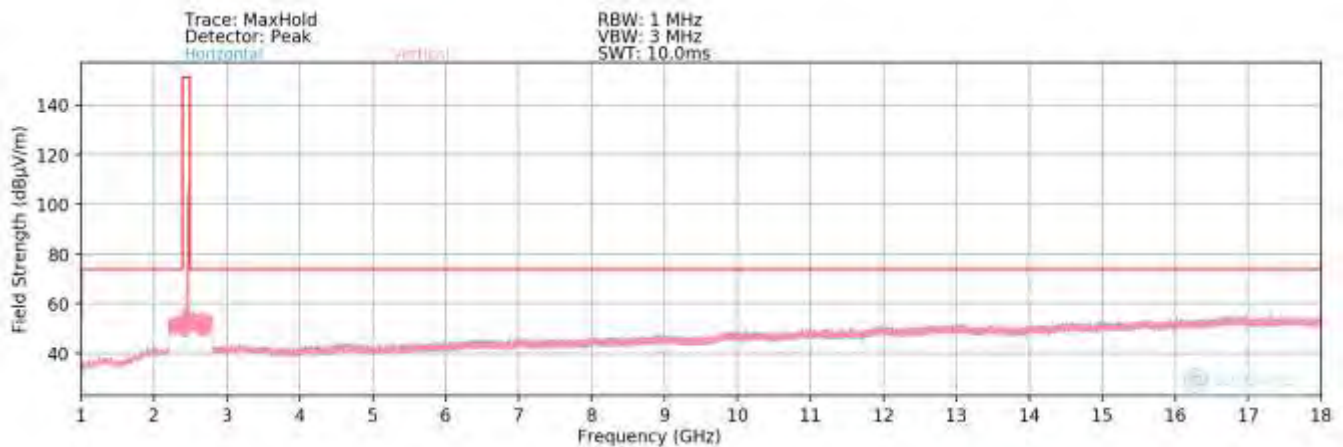
Plot 7-156. Radiated Spurious Plot above 1GHz (802.11b – Ch. 11) SISO ANT 2
