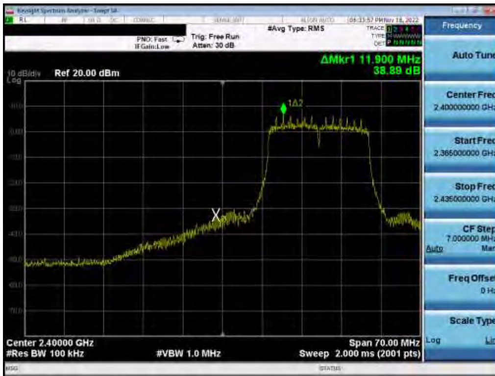
Plot 7-82. Band Edge Plot (802.11n (2.4GHz) – Ch. 2) SISO ANT 2
