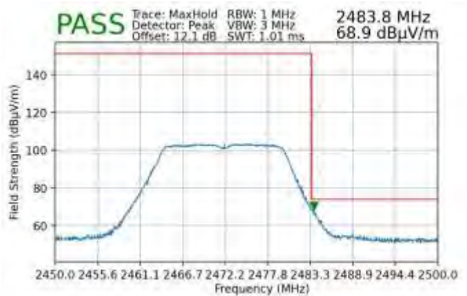
Plot 7-175. Radiated Restricted Upper Band Edge Measurement SISO ANT2 (Peak)
