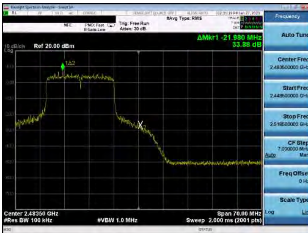
Plot 7-134. Band Edge Plot (802.11ax (2.4GHz) – Ch. 12) MIMO ANT 2
