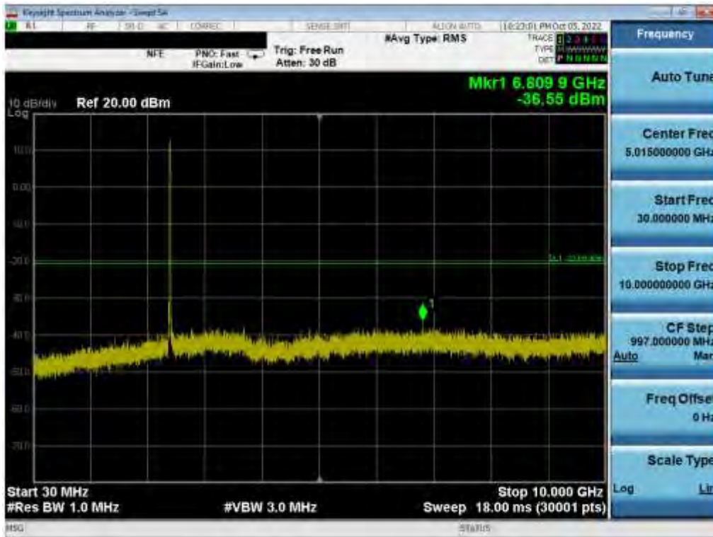
Plot 7-136. Conducted Spurious Plot (802.11b – Ch. 1) SISO ANT 2
