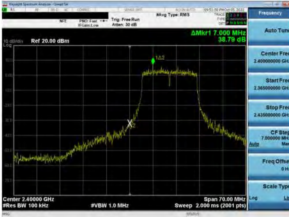
Plot 7-119. Band Edge Plot (802.11g– Ch. 1) MIMO ANT 2
