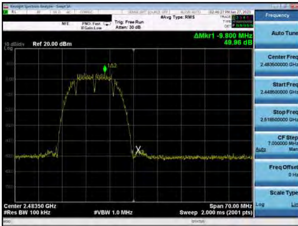
Plot 7-97. Band Edge Plot (802.11b – Ch. 13) MIMO ANT 1
