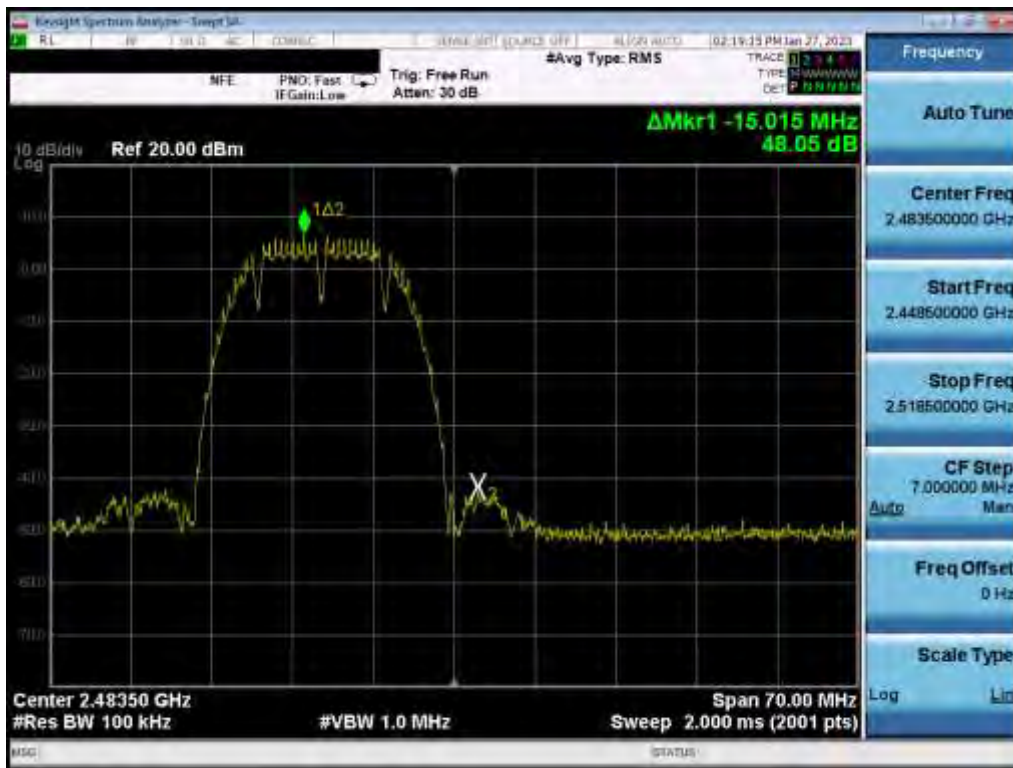
Plot 7-76. Band Edge Plot (802.11b – Ch. 13) SISO ANT 2
