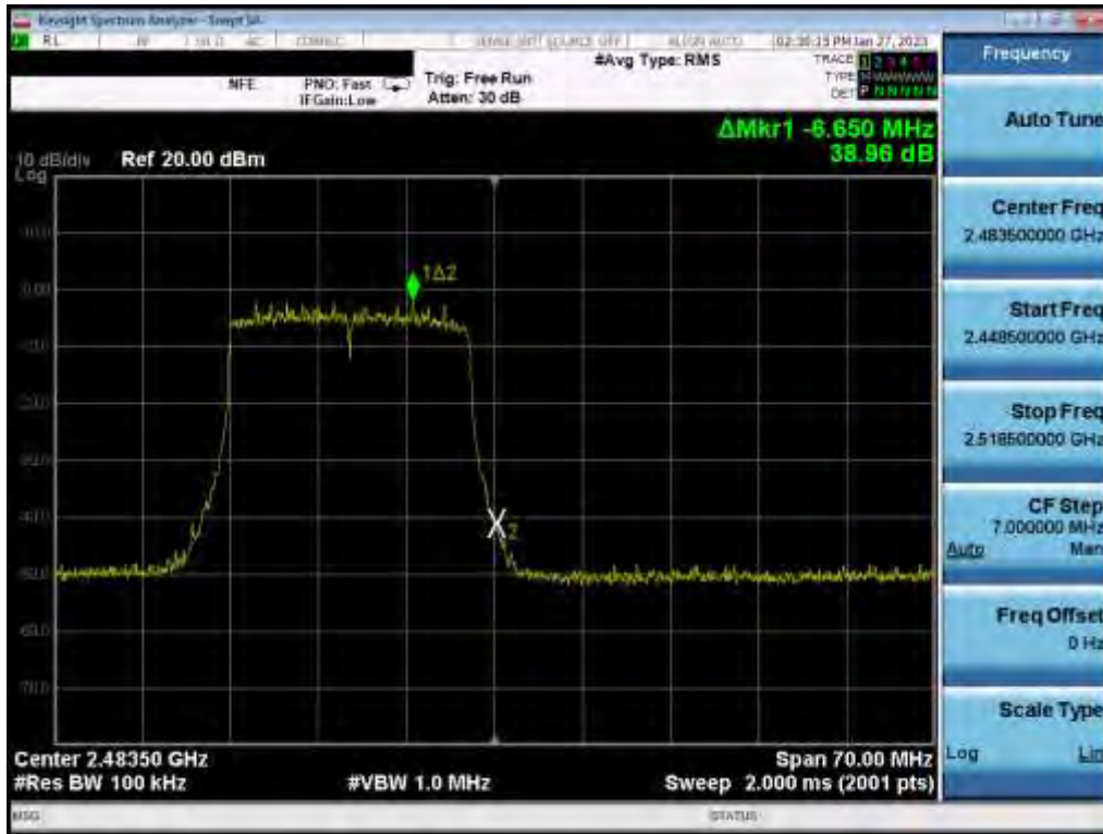
Plot 7-135. Band Edge Plot (802.11ax (2.4GHz) – Ch. 13) MIMO ANT 2
