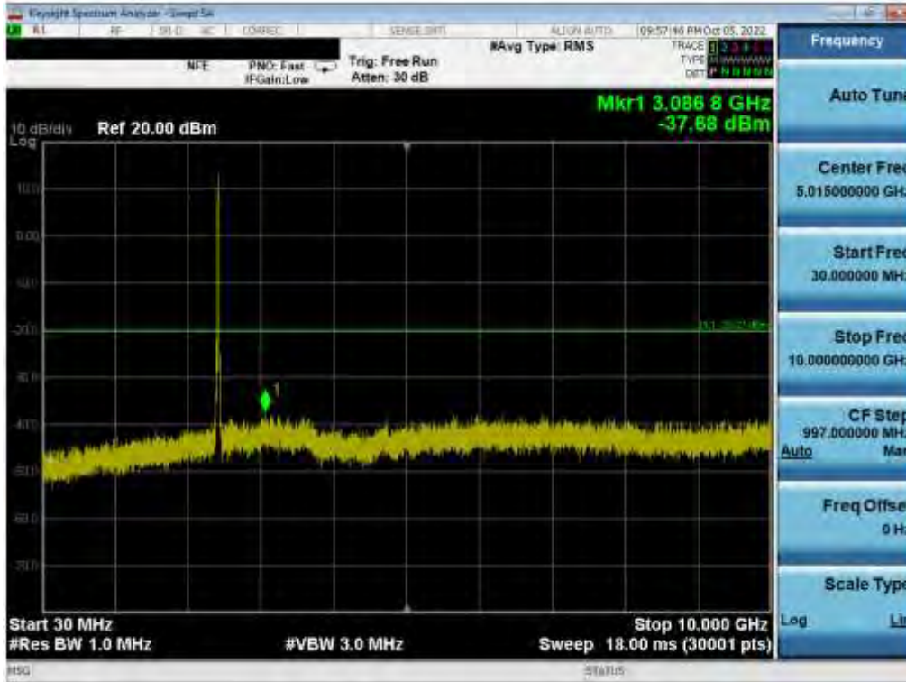
Plot 7-150. Conducted Spurious Plot (802.11b – Ch. 6) MIMO ANT 2
