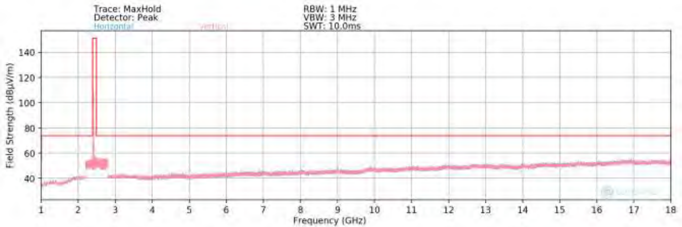
Plot 7-158. Radiated Spurious Plot above 1GHz (802.11b – Ch. 1) MIMO
