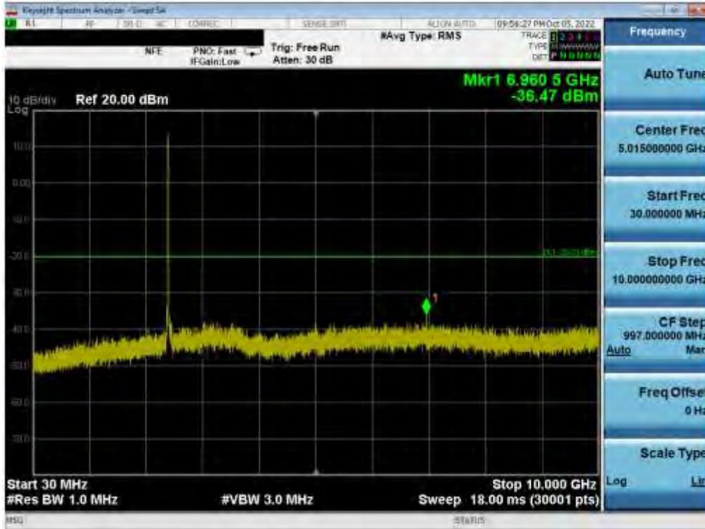
Plot 7-148. Conducted Spurious Plot (802.11b – Ch. 1) MIMO ANT 2
