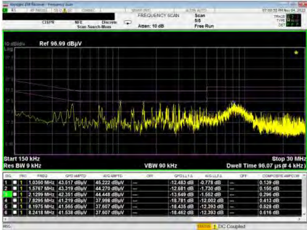
Plot 7-195. Line Conducted Plot with 802.11b (L1) with WCP
