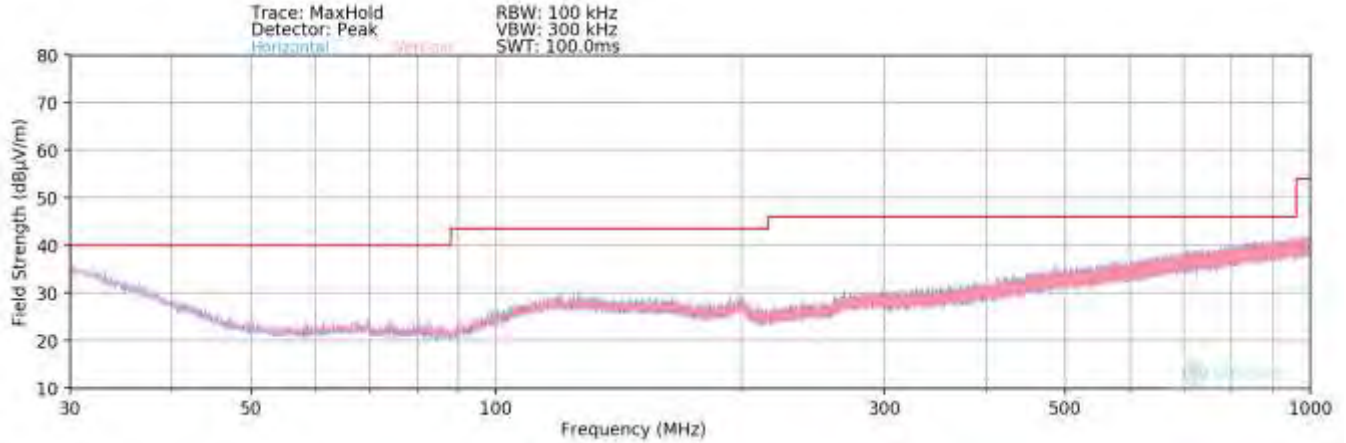
Plot 7-192. Radiated Spurious Plot below 1GHz MIMO
