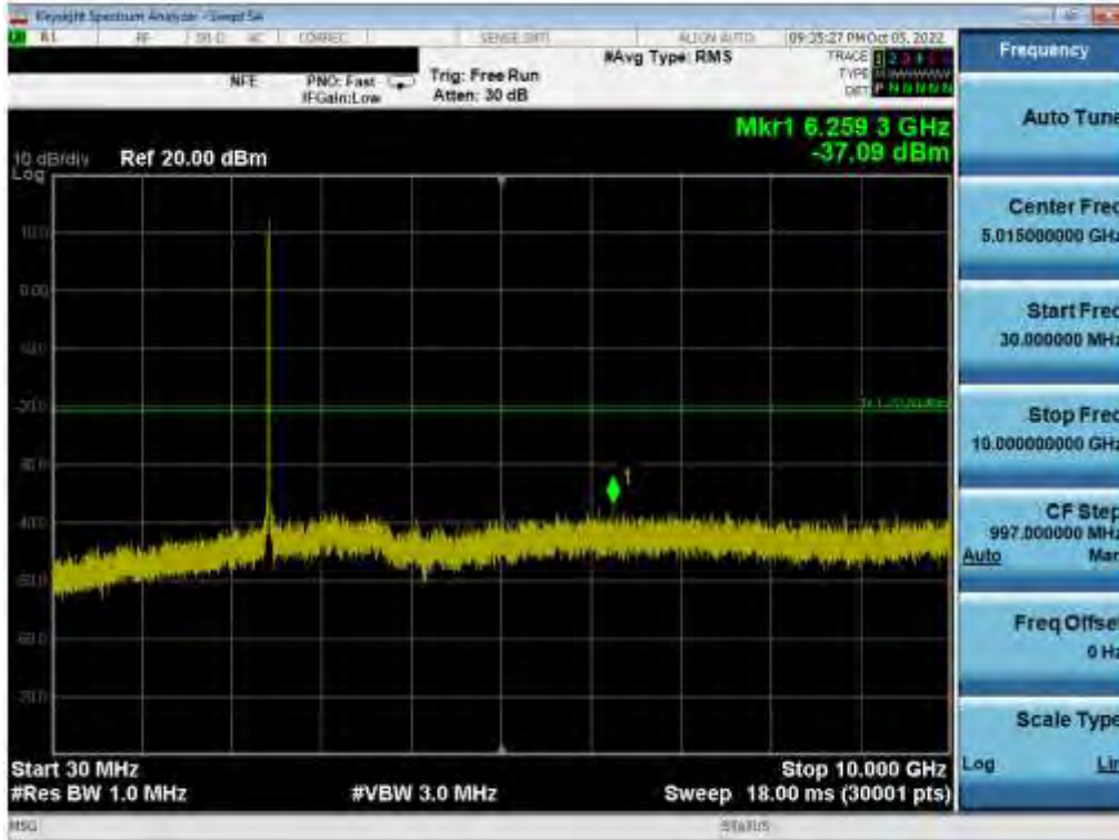
Plot 7-144. Conducted Spurious Plot (802.11b – Ch. 6) MIMO ANT 1
