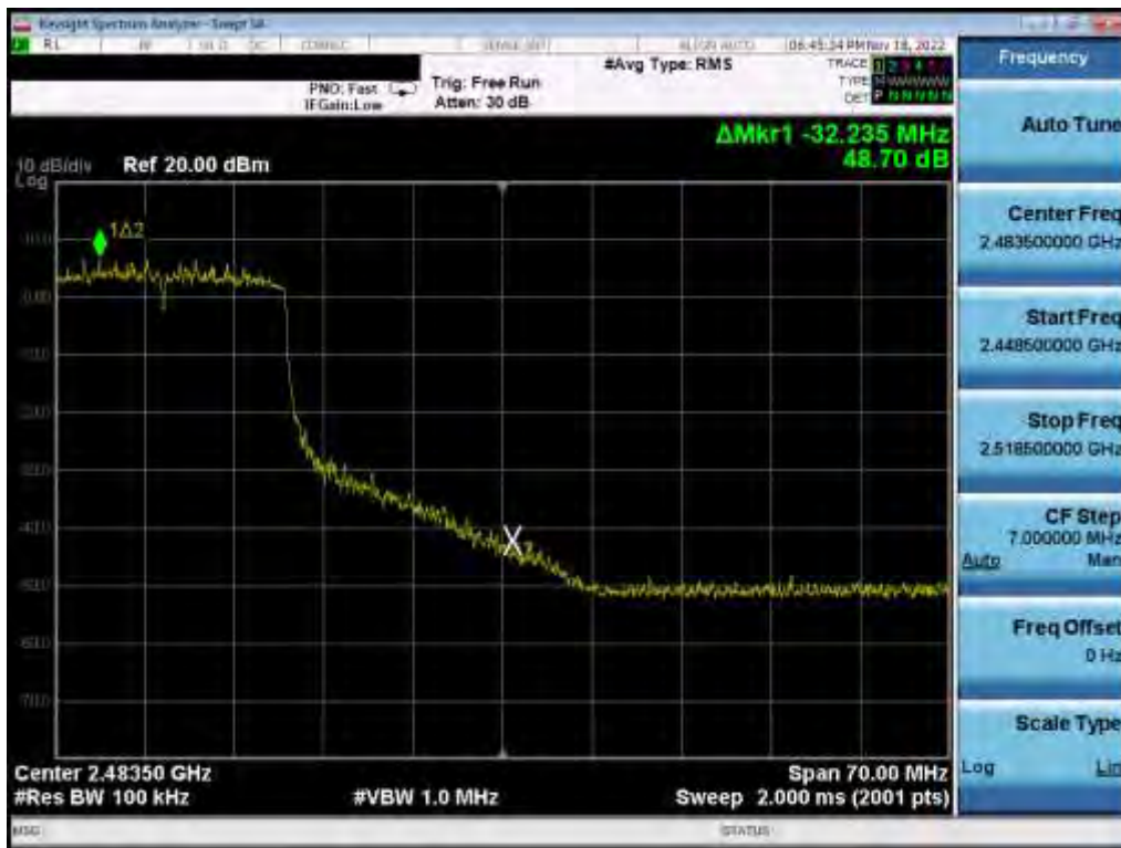
Plot 7-111. Band Edge Plot (802.11ax (2.4GHz) – Ch. 10) MIMO ANT 1
