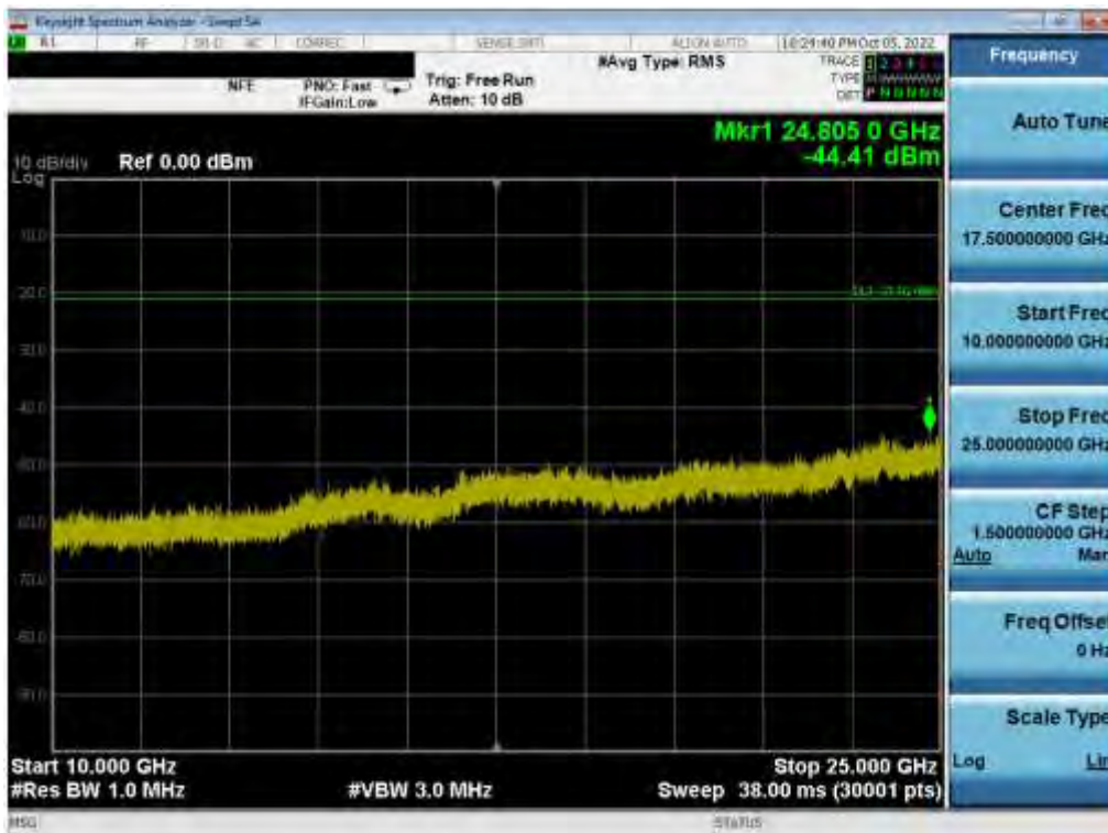
Plot 7-139. Conducted Spurious Plot (802.11b – Ch. 6) SISO ANT 2
