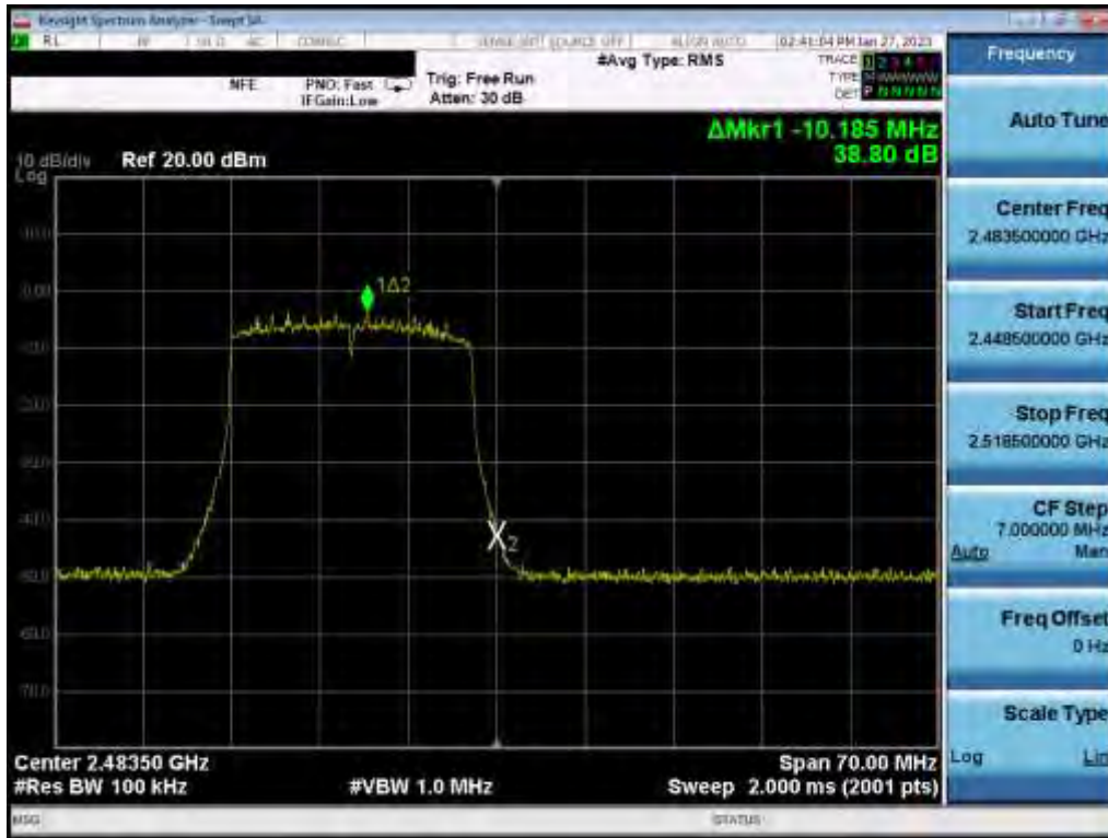
Plot 7-114. Band Edge Plot (802.11ax (2.4GHz) – Ch. 13) MIMO ANT 1
