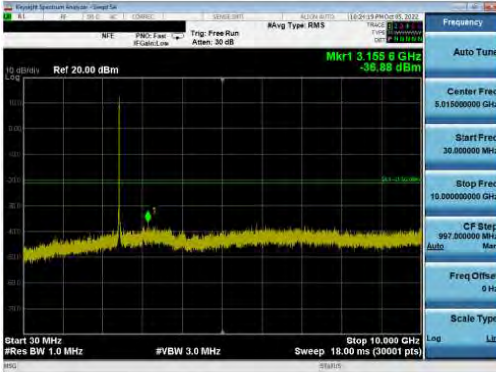
Plot 7-138. Conducted Spurious Plot (802.11b – Ch. 6) SISO ANT 2
