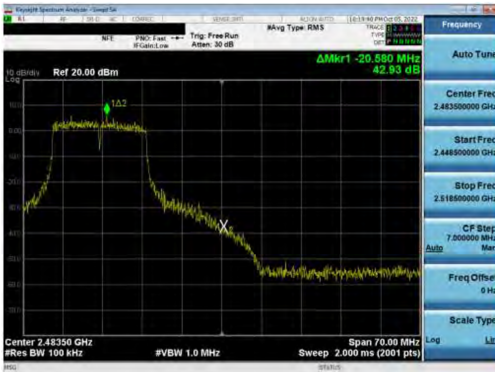
Plot 7-78. Band Edge Plot (802.11g – Ch. 11) SISO ANT 2
