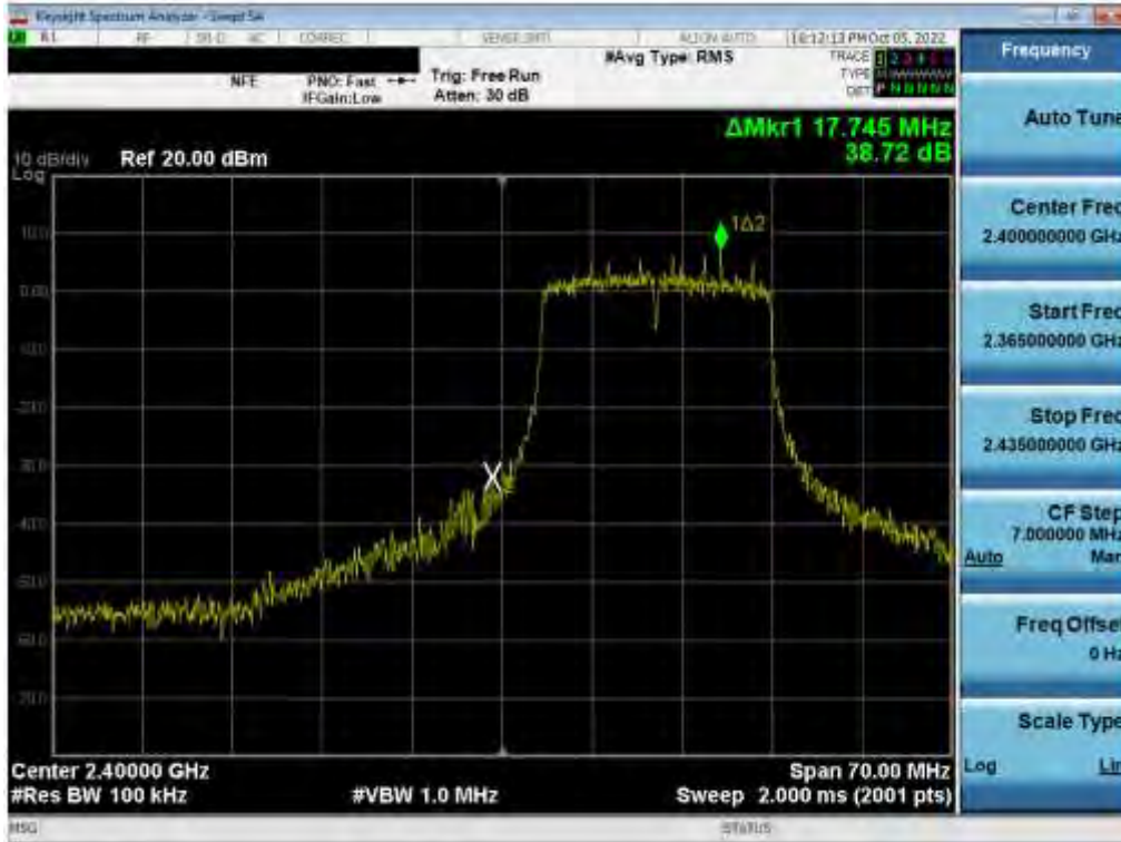
Plot 7-81. Band Edge Plot (802.11n (2.4GHz) – Ch. 1) SISO ANT 2
