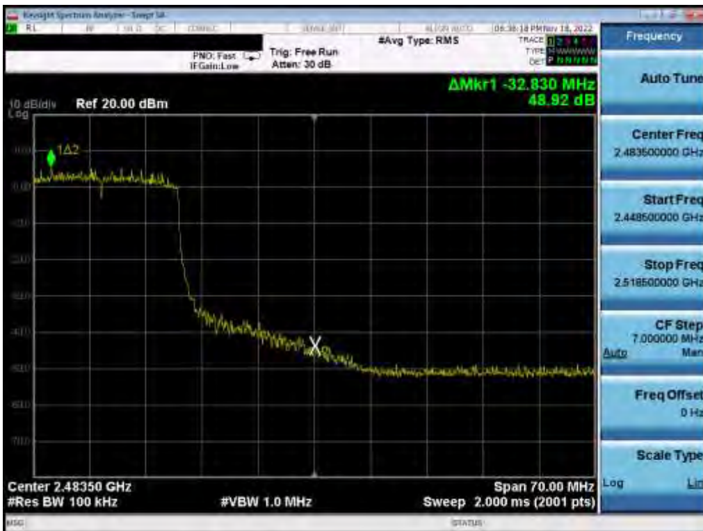
Plot 7-90. Band Edge Plot (802.11ax (2.4GHz) – Ch. 10) SISO ANT 2
