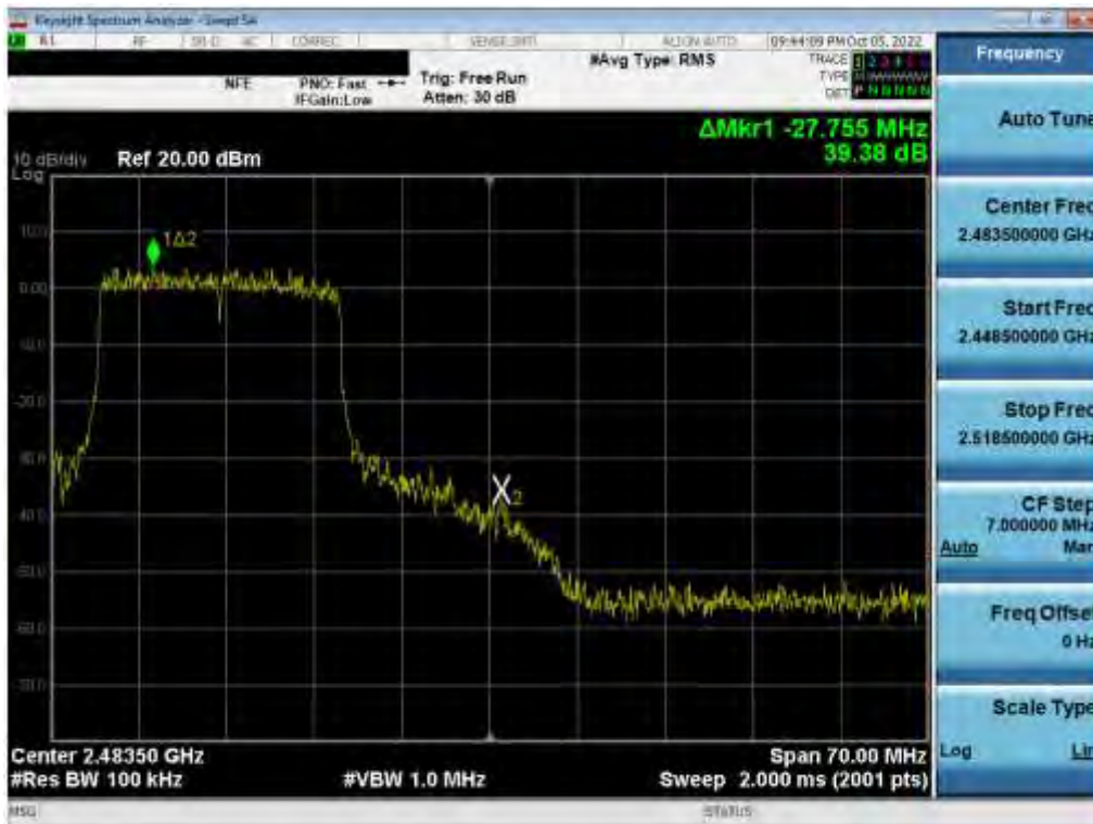
Plot 7-133. Band Edge Plot (802.11ax (2.4GHz) – Ch. 11) MIMO ANT 2
