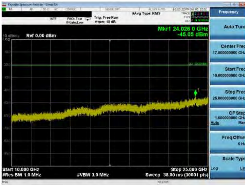
Plot 7-137. Conducted Spurious Plot (802.11b – Ch. 1) SISO ANT 2
