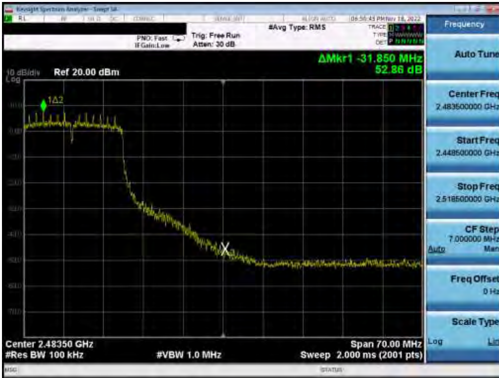
Plot 7-104. Band Edge Plot (802.11n (2.4GHz) – Ch. 10) MIMO ANT 1
