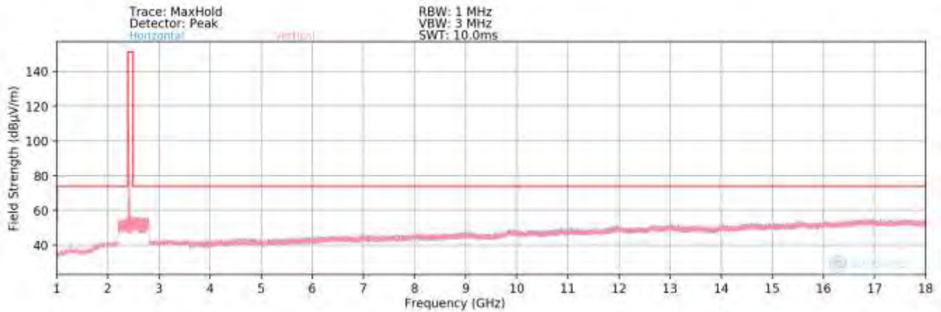
Plot 7-154. Radiated Spurious Plot above 1GHz (802.11b – Ch. 1) SISO ANT 2
