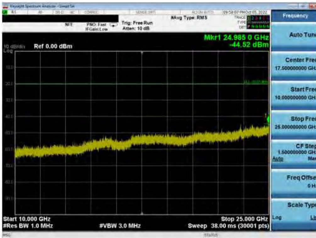
Plot 7-151. Conducted Spurious Plot (802.11b – Ch. 6) MIMO ANT 2
