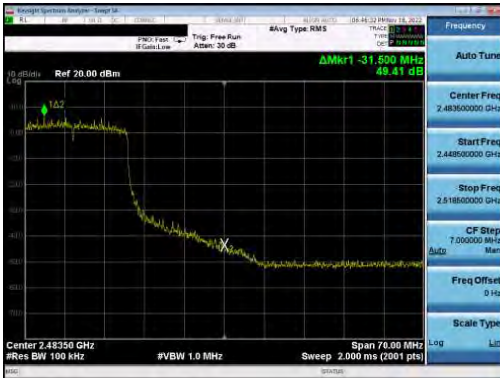
Plot 7-132. Band Edge Plot (802.11ax (2.4GHz) – Ch. 10) MIMO ANT 2
