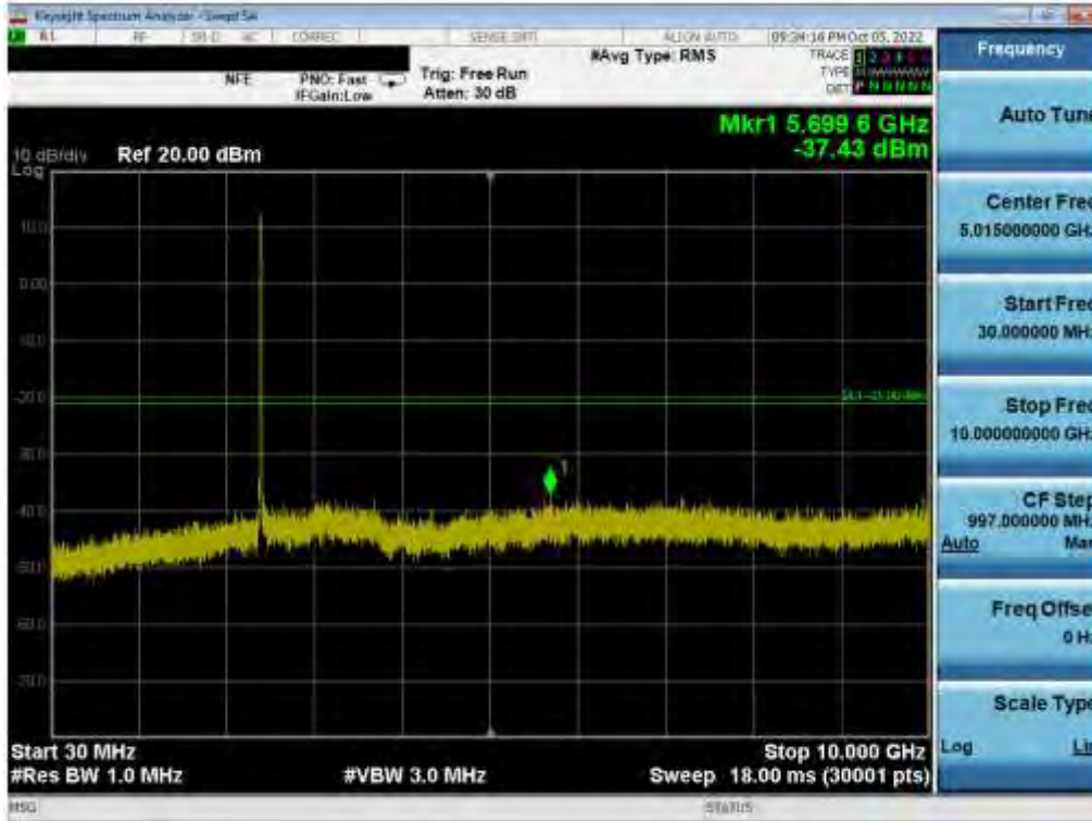
Plot 7-142. Conducted Spurious Plot (802.11b – Ch. 1) MIMO ANT 1
