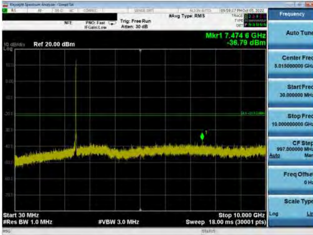
Plot 7-152. Conducted Spurious Plot (802.11b – Ch. 11) MIMO ANT 2
