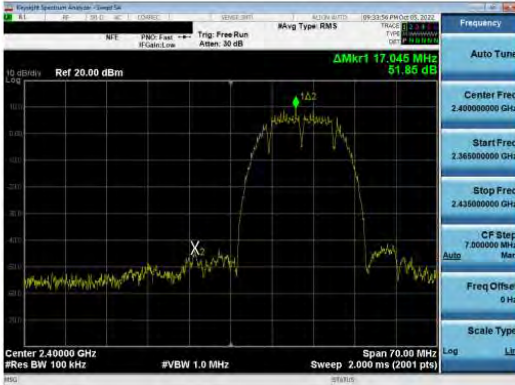
Plot 7-94. Band Edge Plot (802.11b – Ch. 1) MIMO ANT 1
