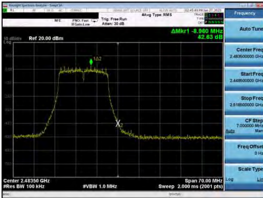
Plot 7-101. Band Edge Plot (802.11g – Ch. 13) MIMO ANT 1
