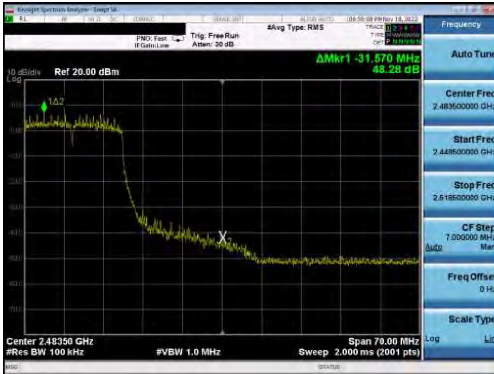
Plot 7-125. Band Edge Plot (802.11n (2.4GHz) – Ch. 10) MIMO ANT 2
