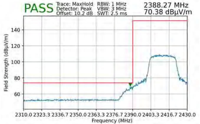
Plot 7-163. Radiated Restricted Lower Band Edge Measurement SISO ANT2 (Peak)
