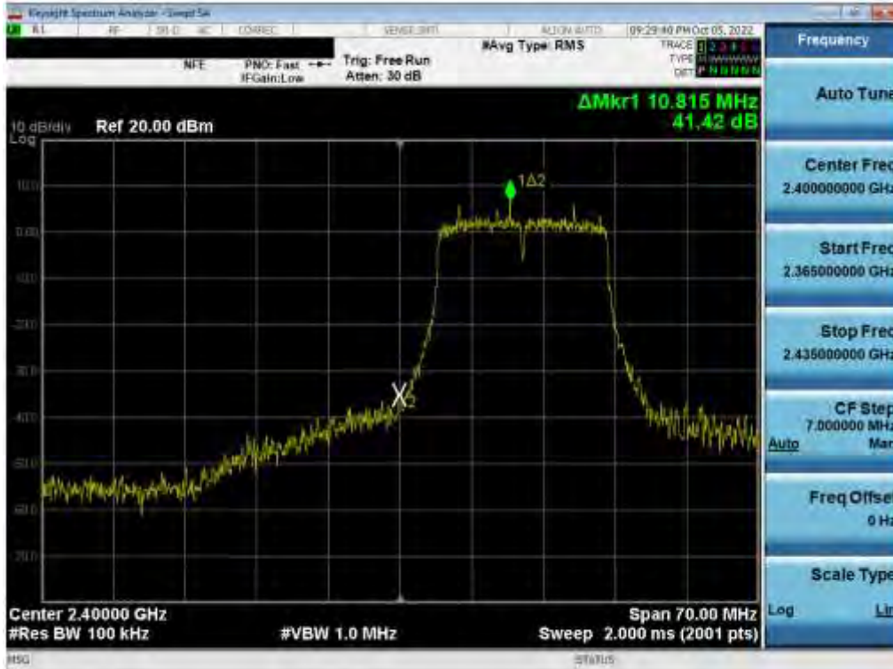
Plot 7-98. Band Edge Plot (802.11g– Ch. 1) MIMO ANT 1
