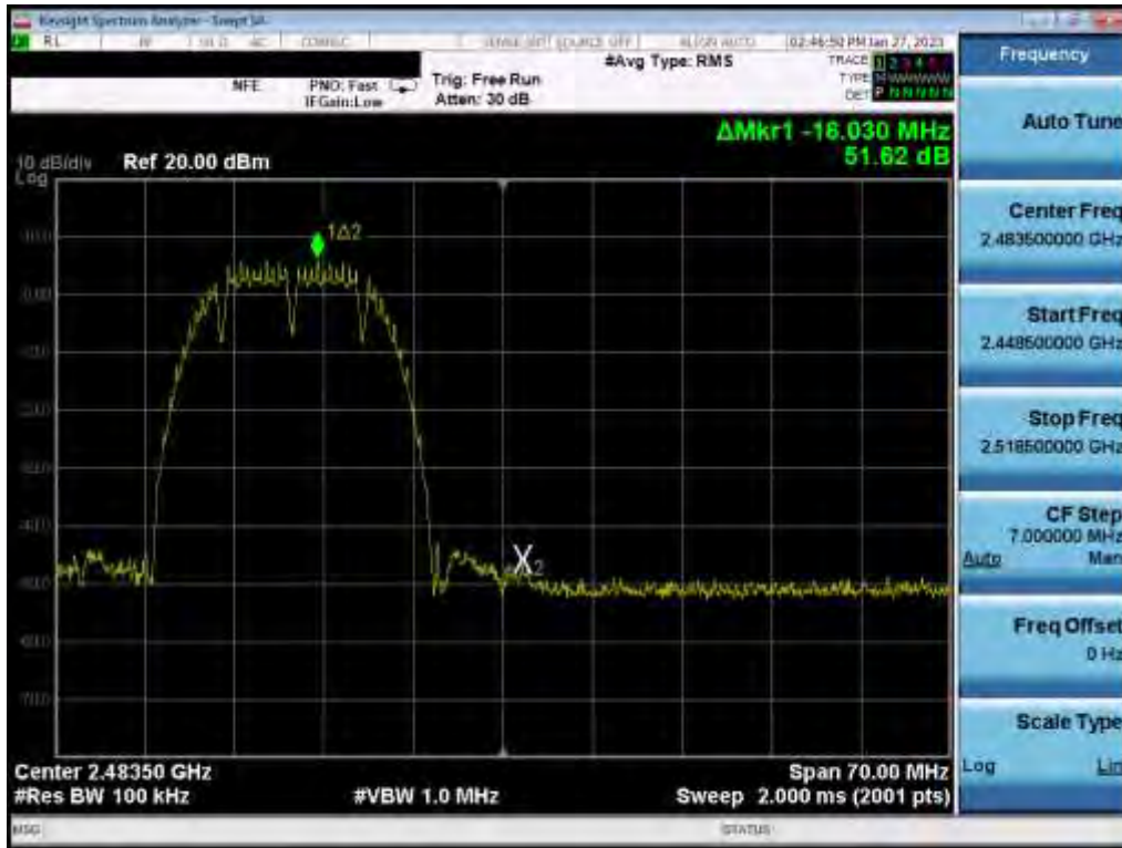
Plot 7-96. Band Edge Plot (802.11b – Ch. 12) MIMO ANT 1
