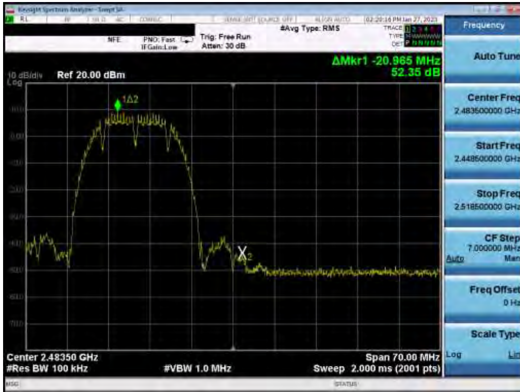
Plot 7-75. Band Edge Plot (802.11b – Ch. 12) SISO ANT 2
