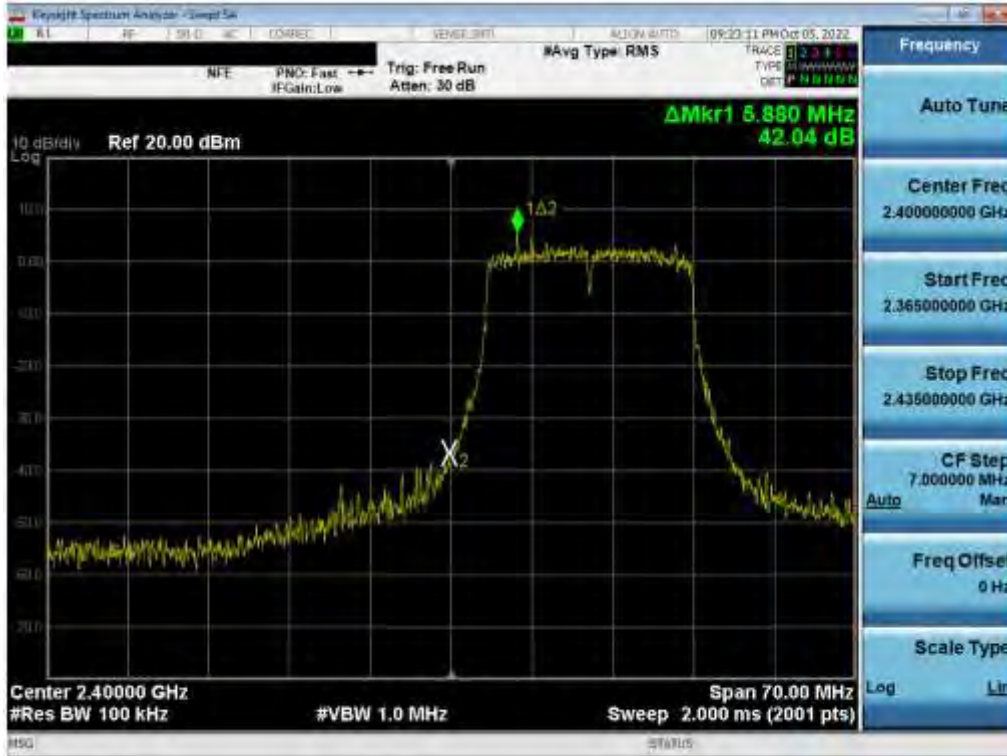
Plot 7-102. Band Edge Plot (802.11n (2.4GHz) – Ch. 1) MIMO ANT 1
