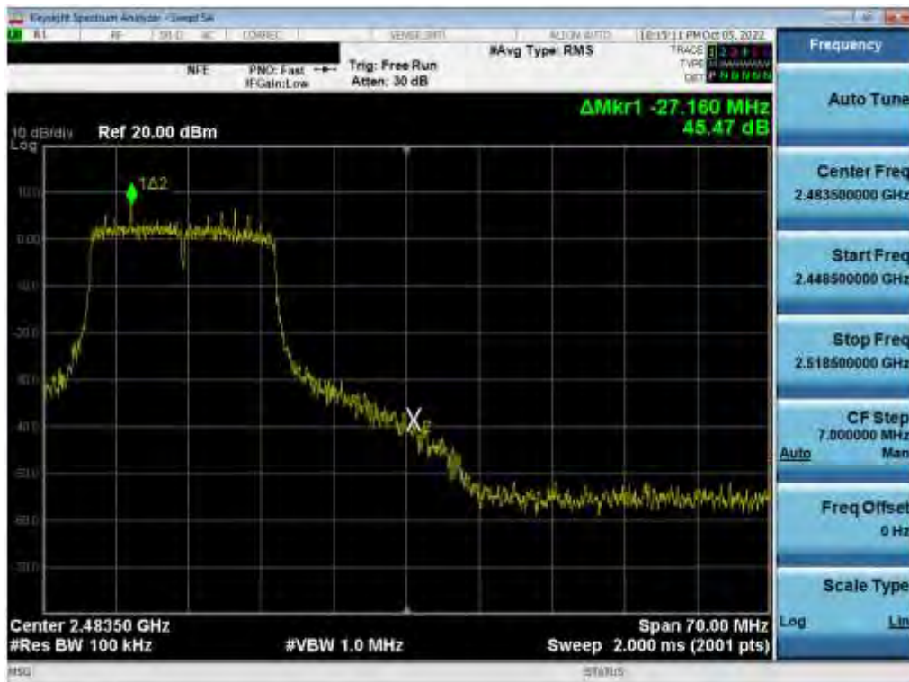
Plot 7-84. Band Edge Plot (802.11n (2.4GHz) – Ch. 11) SISO ANT 2
