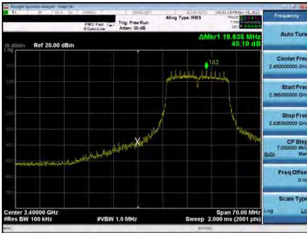
Plot 7-103. Band Edge Plot (802.11n (2.4GHz) – Ch. 2) MIMO ANT 1
