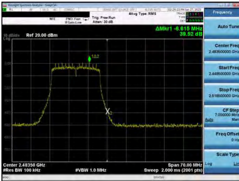
Plot 7-128. Band Edge Plot (802.11n (2.4GHz) – Ch. 13) MIMO ANT 2
