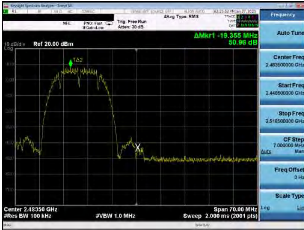
Plot 7-117. Band Edge Plot (802.11b – Ch. 12) MIMO ANT 2
