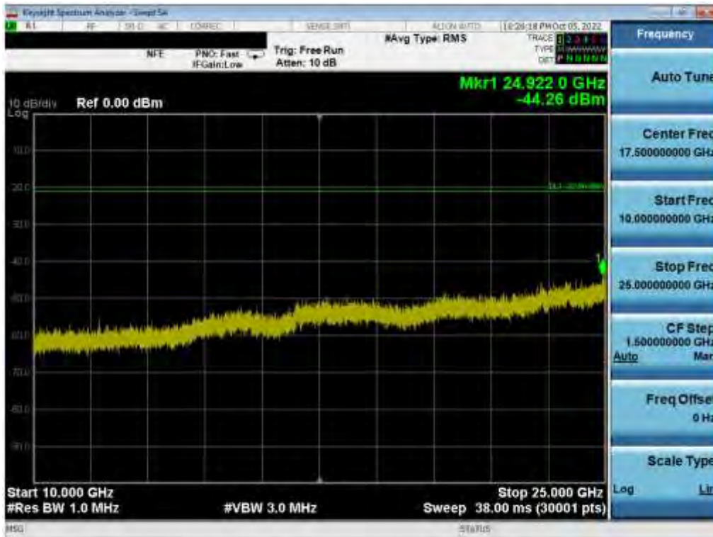
Plot 7-141. Conducted Spurious Plot (802.11b – Ch. 11) SISO ANT 2
