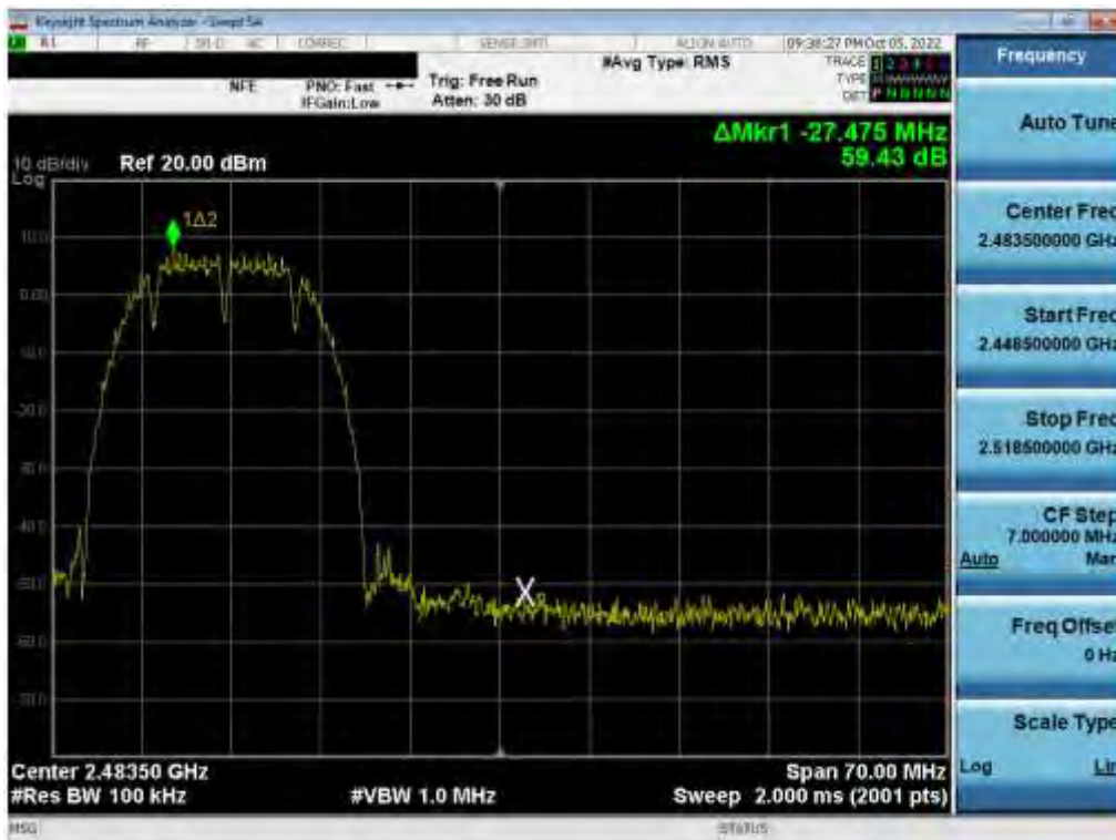
Plot 7-95. Band Edge Plot (802.11b – Ch. 11) MIMO ANT 1
