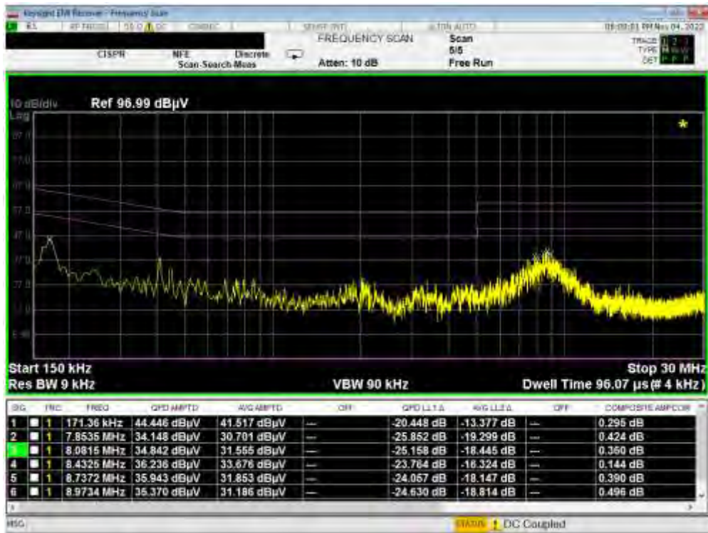
Plot 7-194. Line Conducted Plot with 802.11b (N)
