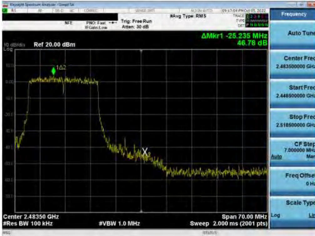
Plot 7-112. Band Edge Plot (802.11ax (2.4GHz) – Ch. 11) MIMO ANT 1
