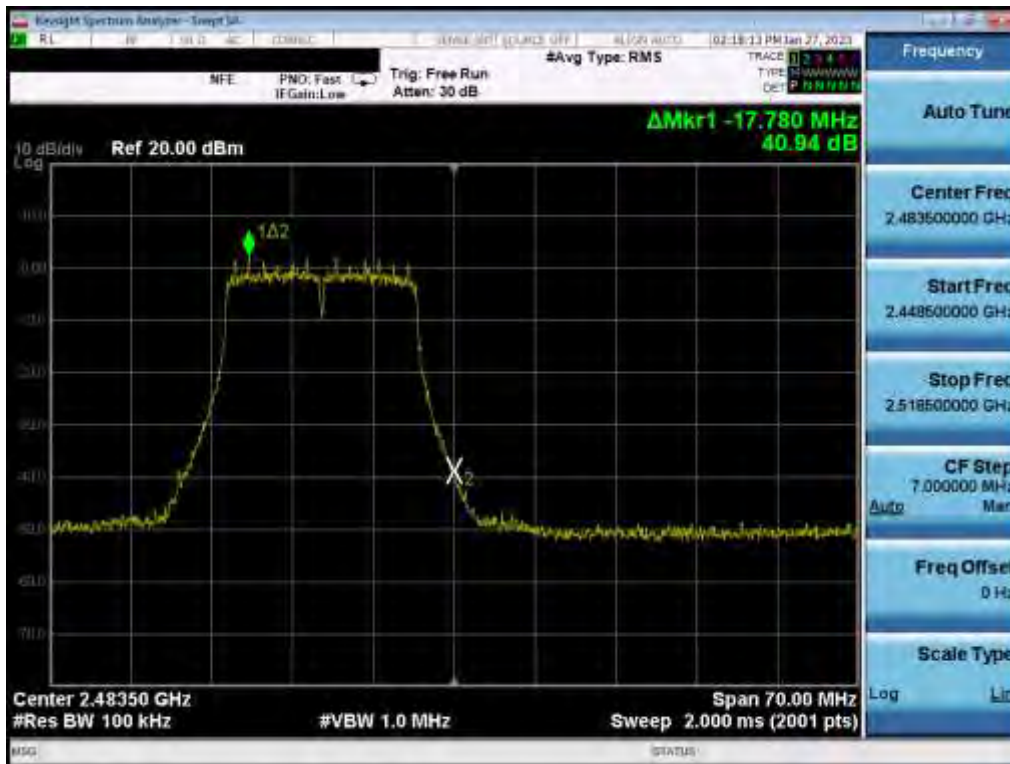
Plot 7-80. Band Edge Plot (802.11g – Ch. 13) SISO ANT 2
