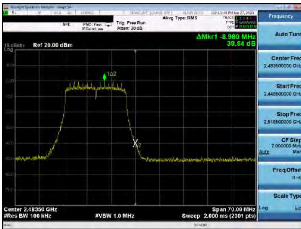
Plot 7-86. Band Edge Plot (802.11n (2.4GHz) – Ch. 13) SISO ANT 2
