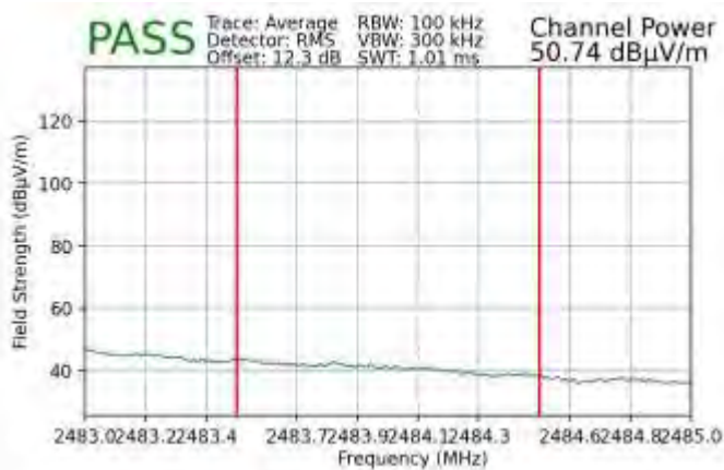
Plot 7-174. Radiated Restricted Upper Band Edge Measurement SISO ANT2 (Average)
