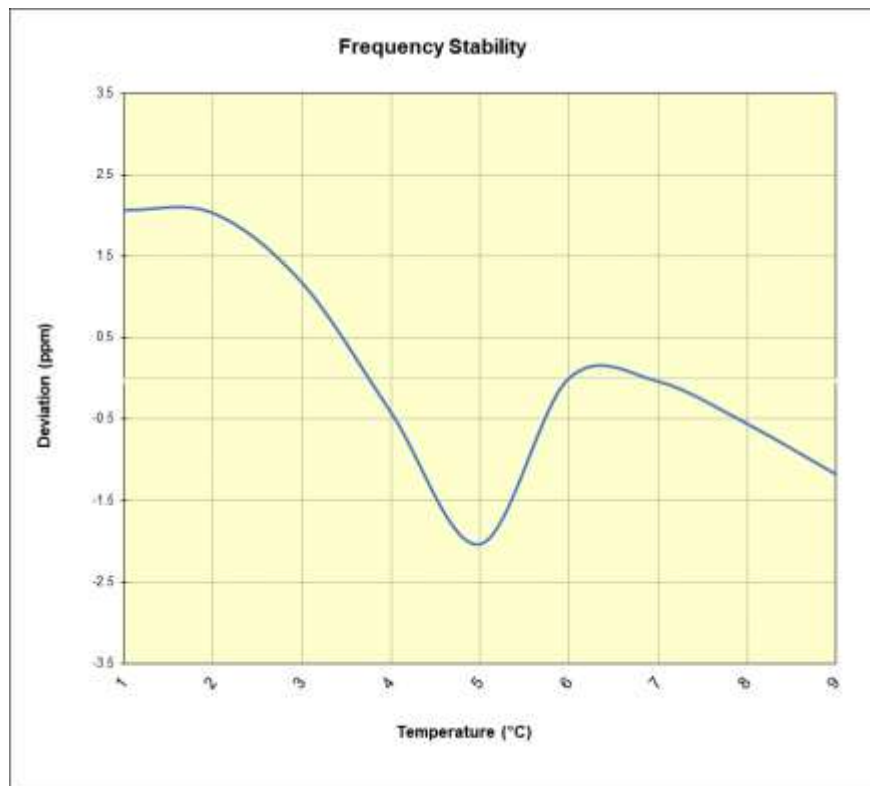
Plot 7-24. LTE Band 26 Frequency Stability Chart
