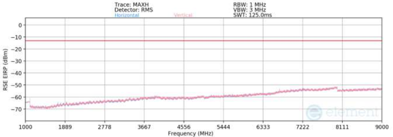
Plot 7-23. Radiated Spurious Plot (LTE Band 26 – Above 1GHz)
